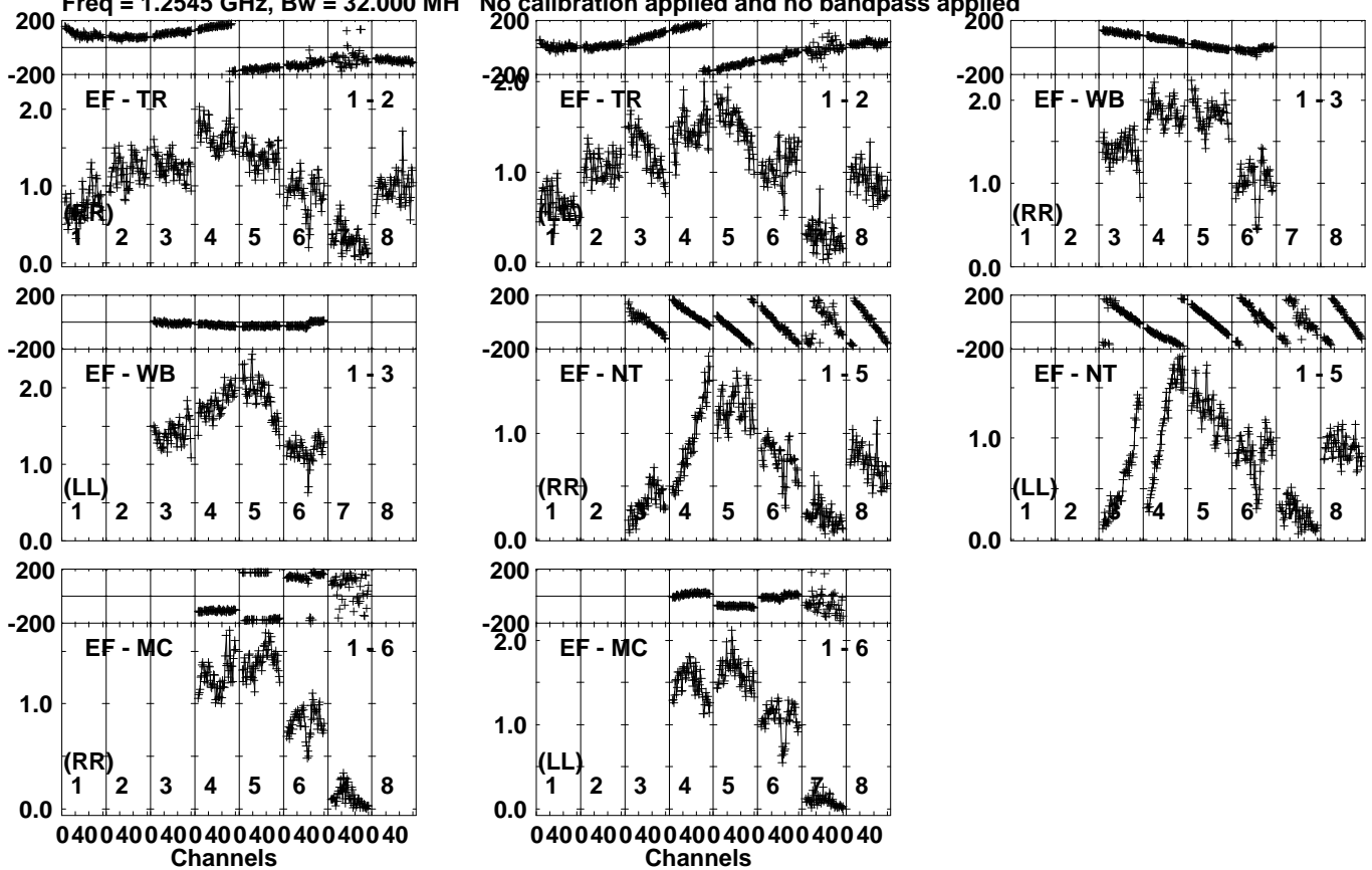
Lower frame: Milli Ampl Jy Top frame: Phas deg Vector averaged cross-power spectrum Several baselines displayed Timerange: 01/00:03:45 to 01/00:04:43
