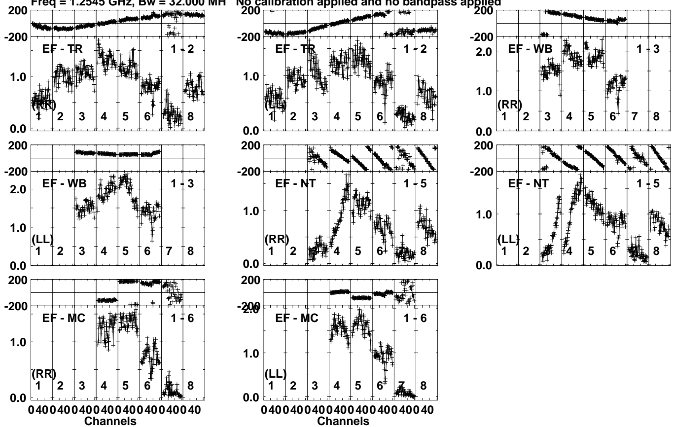
Lower frame: Milli Ampl Jy Top frame: Phas deg Vector averaged cross-power spectrum Several baselines displayed Timerange: 00/23:27:52 to 00/23:29:22
