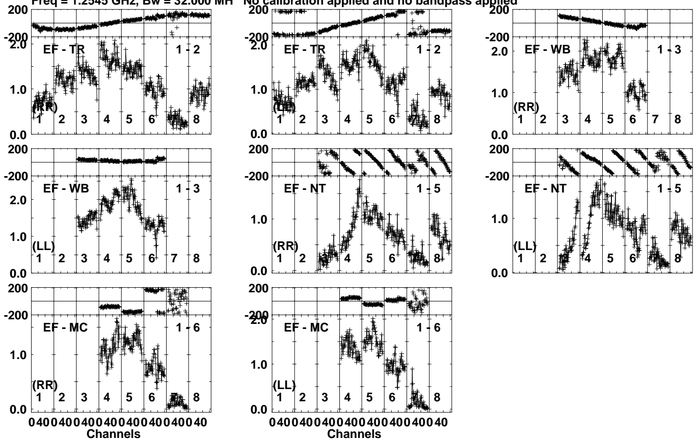
Lower frame: Milli Ampl Jy Top frame: Phas deg Vector averaged cross-power spectrum Several baselines displayed Timerange: 00/22:29:24 to 00/22:30:58
