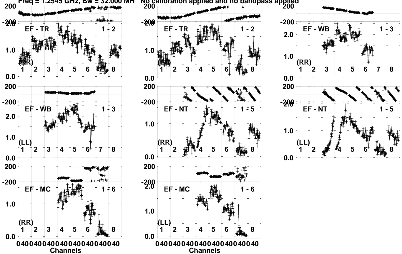
Lower frame: Milli Ampl Jy Top frame: Phas deg Vector averaged cross-power spectrum Several baselines displayed Timerange: 00/23:48:36 to 00/23:49:34
