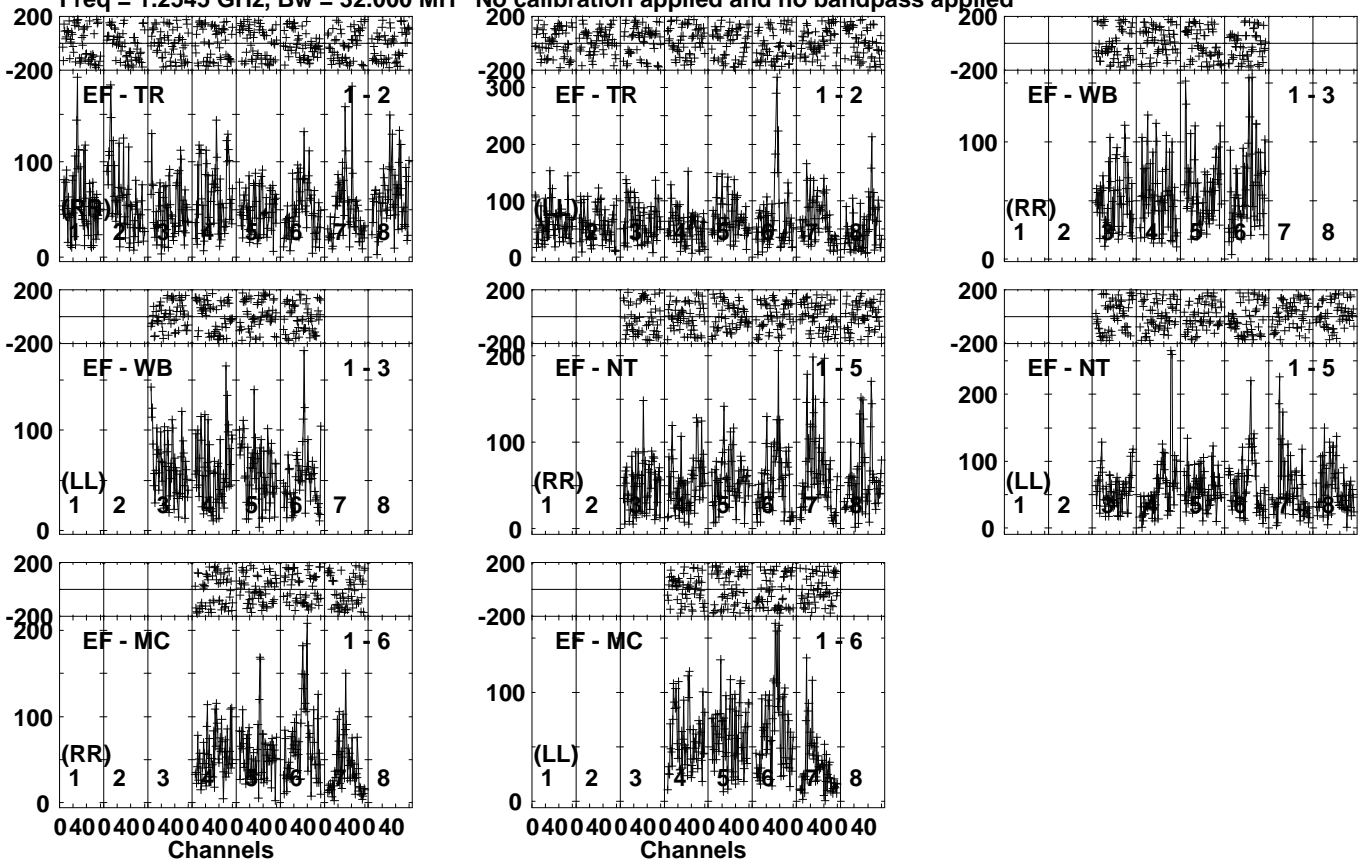
Lower frame: Micro Ampl Jy Top frame: Phas deg Vector averaged cross-power spectrum Several baselines displayed Timerange: 00/23:21:52 to 00/23:27:50
