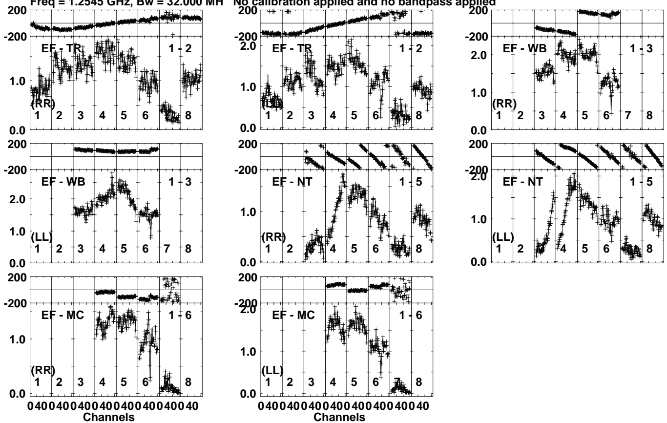
Lower frame: Milli Ampl Jy Top frame: Phas deg Vector averaged cross-power spectrum Several baselines displayed Timerange: 01/00:59:21 to 01/01:00:19
