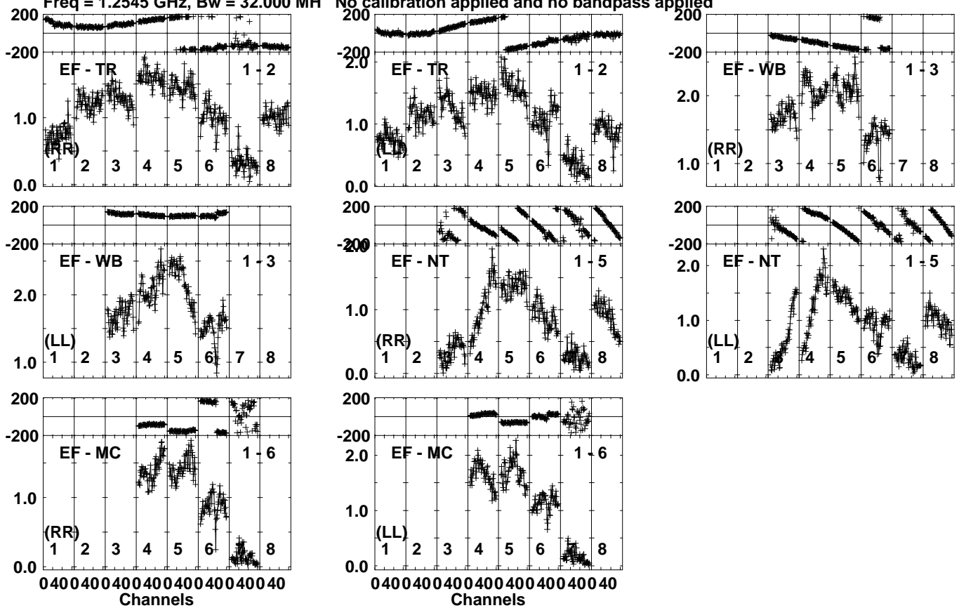
Lower frame: Milli Ampl Jy Top frame: Phas deg Vector averaged cross-power spectrum Several baselines displayed Timerange: 01/01:34:10 to 01/01:35:38
