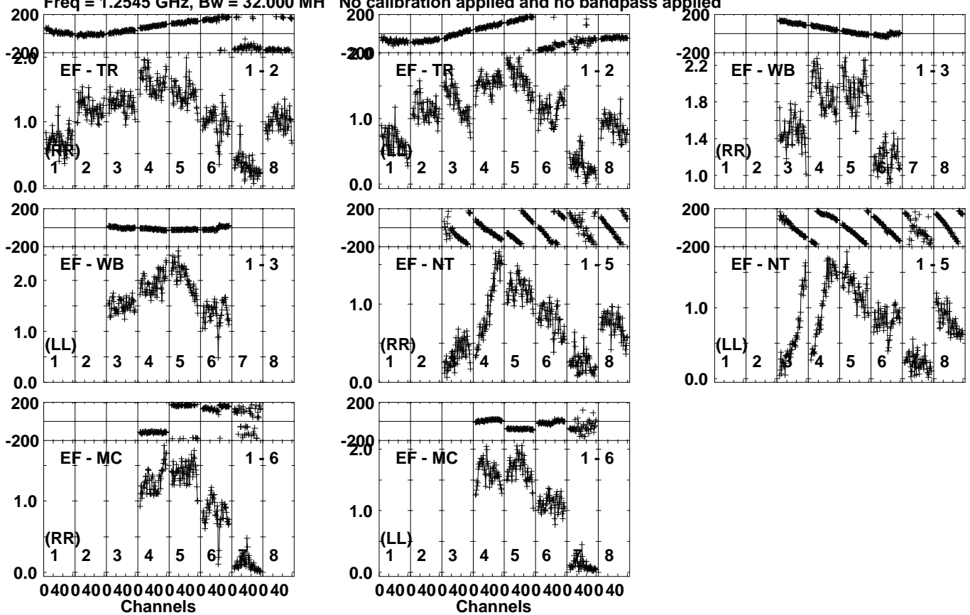
Lower frame: Milli Ampl Jy Top frame: Phas deg Vector averaged cross-power spectrum Several baselines displayed Timerange: 00/23:55:36 to 00/23:57:04
