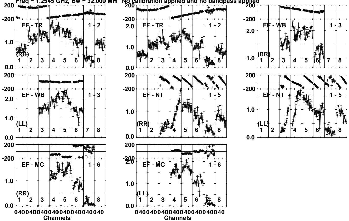
Lower frame: Milli Ampl Jy Top frame: Phas deg Vector averaged cross-power spectrum Several baselines displayed Timerange: 01/00:08:13 to 01/00:09:39
