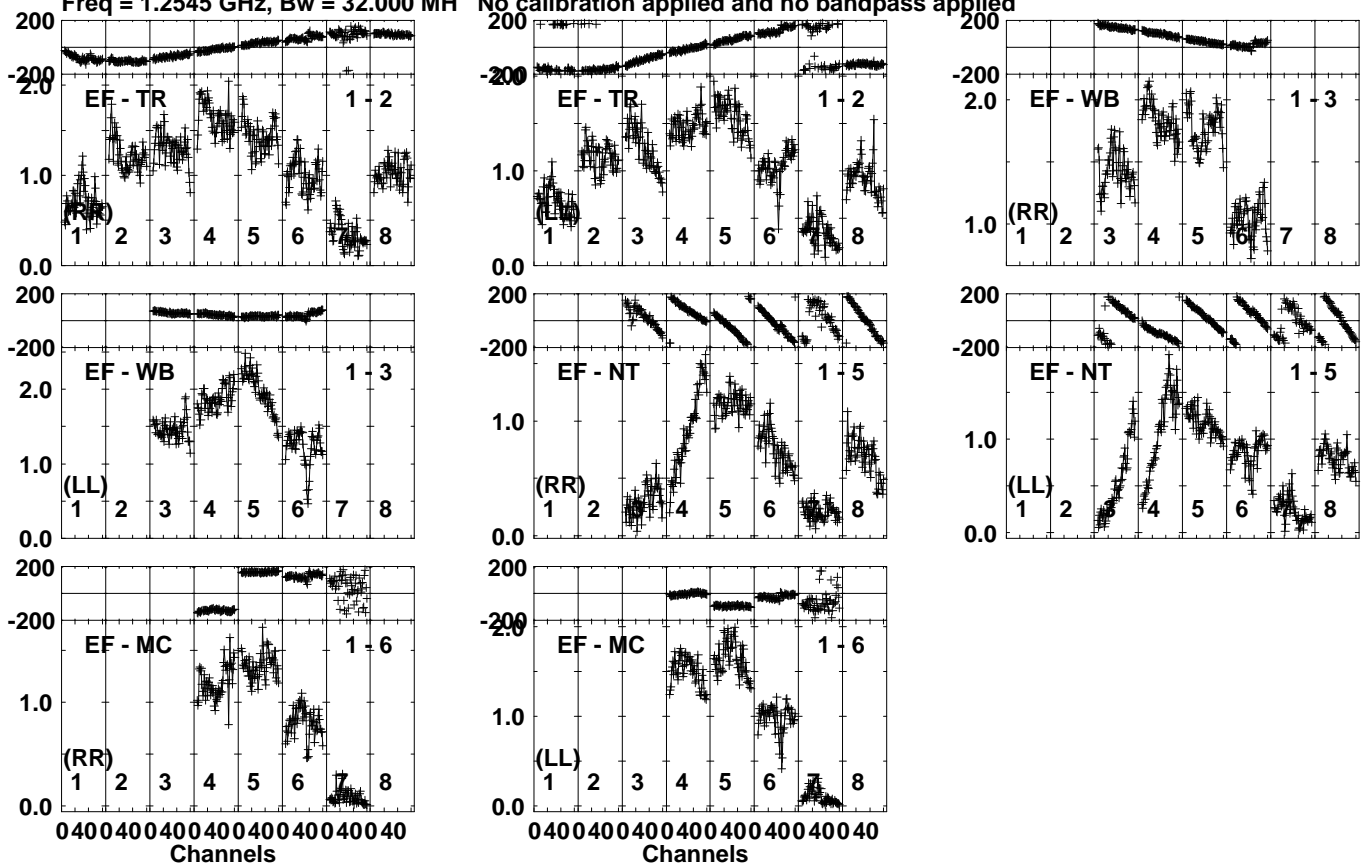
Lower frame: Milli Ampl Jy Top frame: Phas deg Vector averaged cross-power spectrum Several baselines displayed Timerange: 00/23:33:26 to 00/23:34:24
