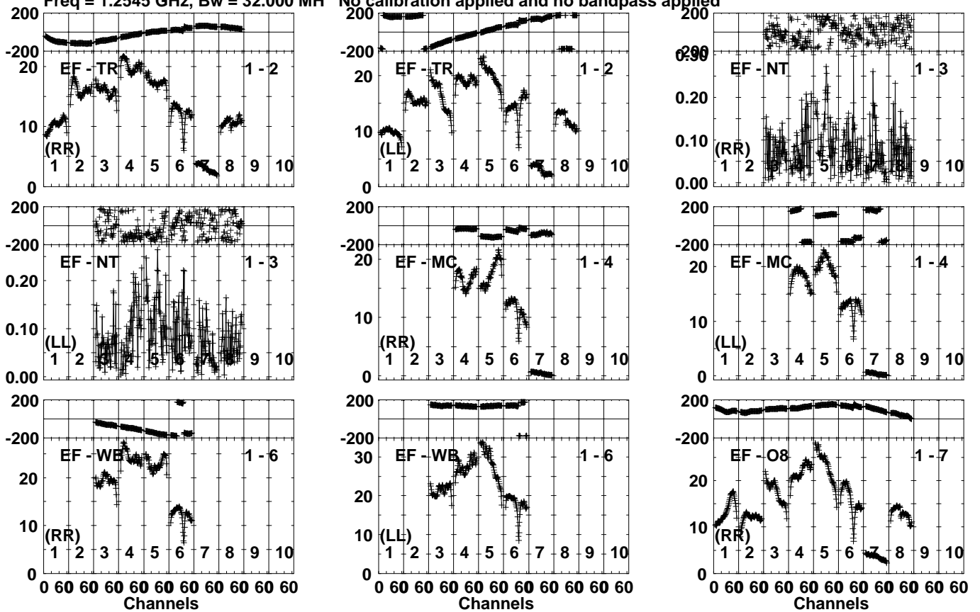
Lower frame: Milli Ampl Jy Top frame: Phas deg Vector averaged cross-power spectrum Several baselines displayed Timerange: 01/07:52:02 to 01/07:56:00
