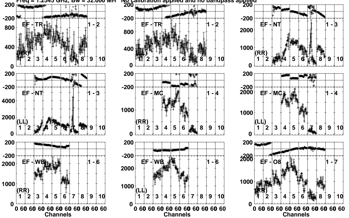
Lower frame: Micro Ampl Jy Top frame: Phas deg Vector averaged cross-power spectrum Several baselines displayed Timerange: 01/01:06:04 to 01/01:07:30
