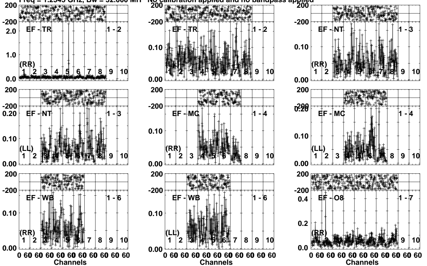
Lower frame: Milli Ampl Jy Top frame: Phas deg Vector averaged cross-power spectrum Several baselines displayed Timerange: 00/23:36:37 to 00/23:42:35
