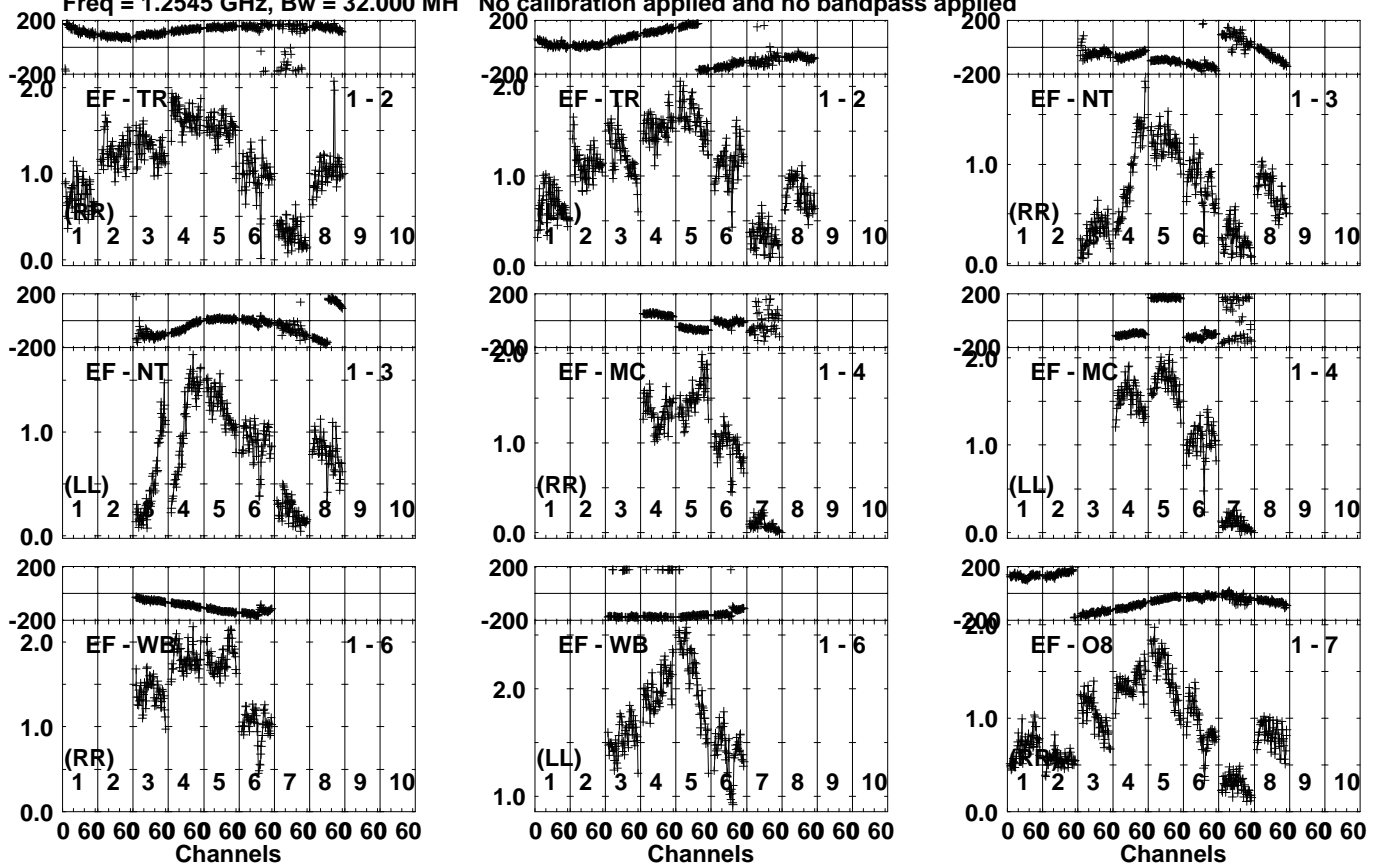
Lower frame: Milli Ampl Jy Top frame: Phas deg Vector averaged cross-power spectrum Several baselines displayed Timerange: 00/23:35:37 to 00/23:36:35
