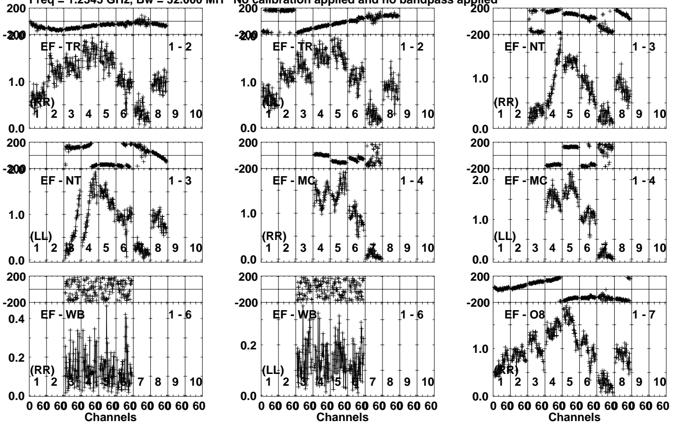
Lower frame: Milli Ampl Jy Top frame: Phas deg Vector averaged cross-power spectrum Several baselines displayed Timerange: 01/00:03:25 to 01/00:04:23
