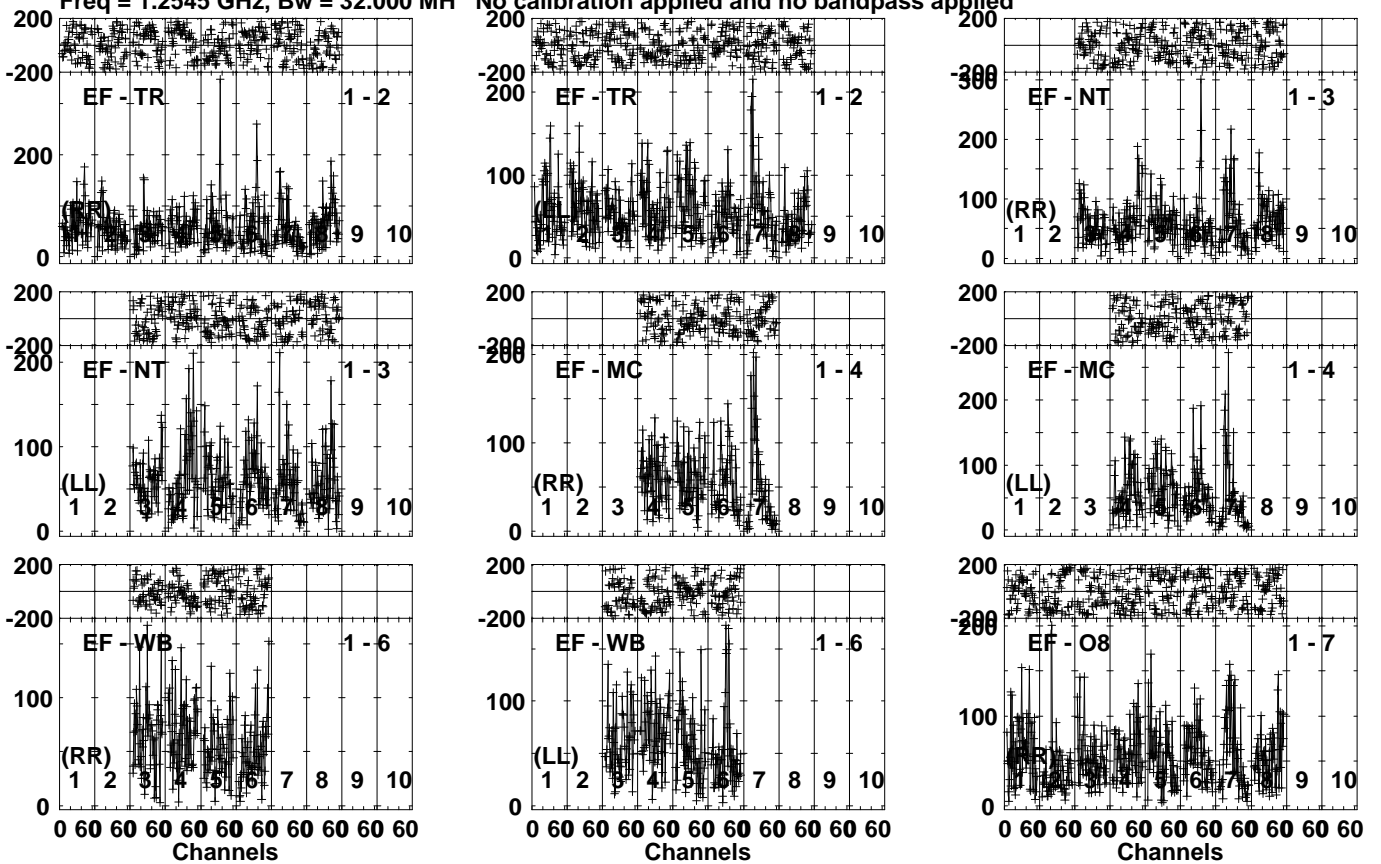
Lower frame: Micro Ampl Jy Top frame: Phas deg Vector averaged cross-power spectrum Several baselines displayed Timerange: 00/23:01:13 to 00/23:07:11
