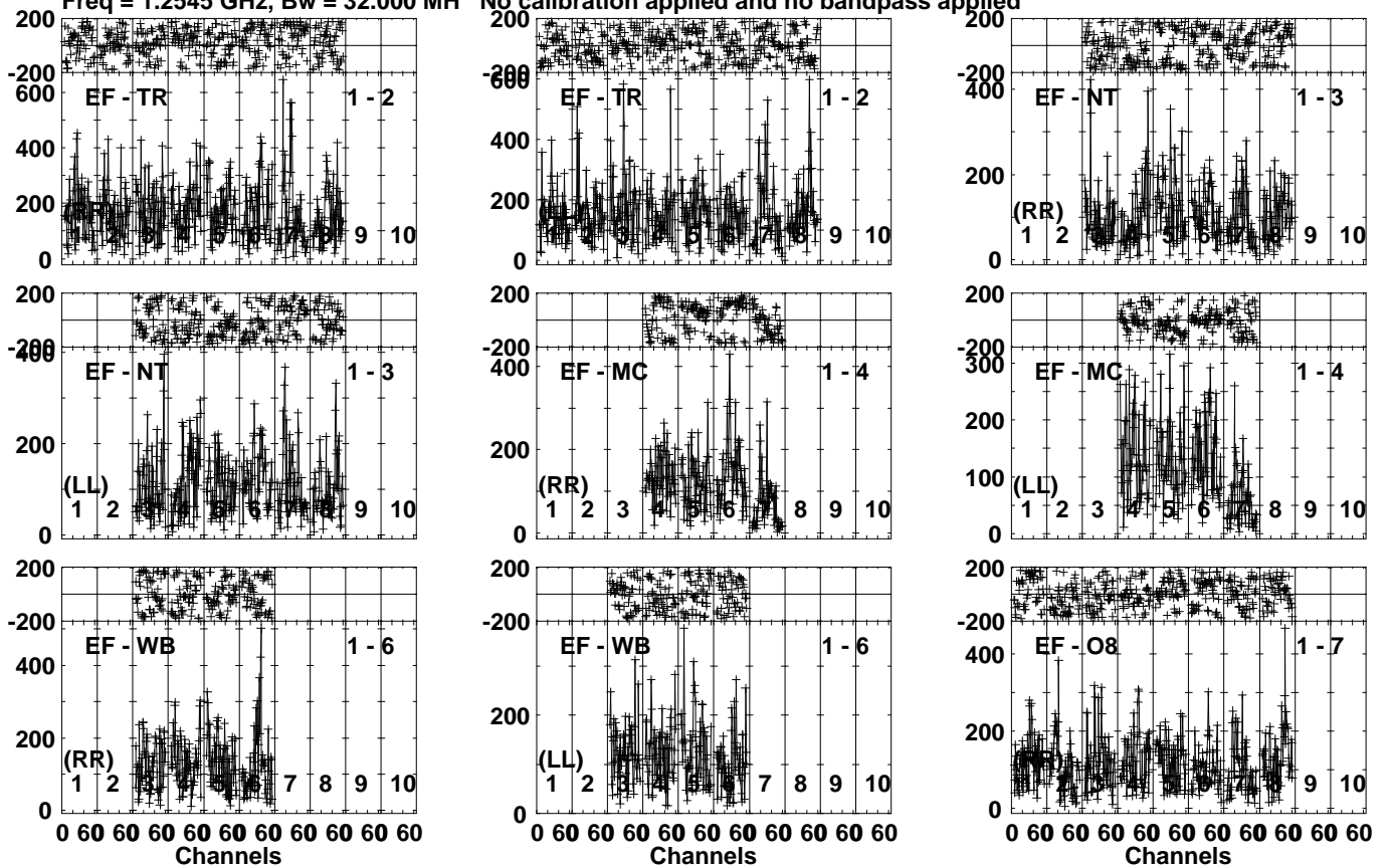
Lower frame: Micro Ampl Jy Top frame: Phas deg Vector averaged cross-power spectrum Several baselines displayed Timerange: 01/00:10:25 to 01/00:11:53
