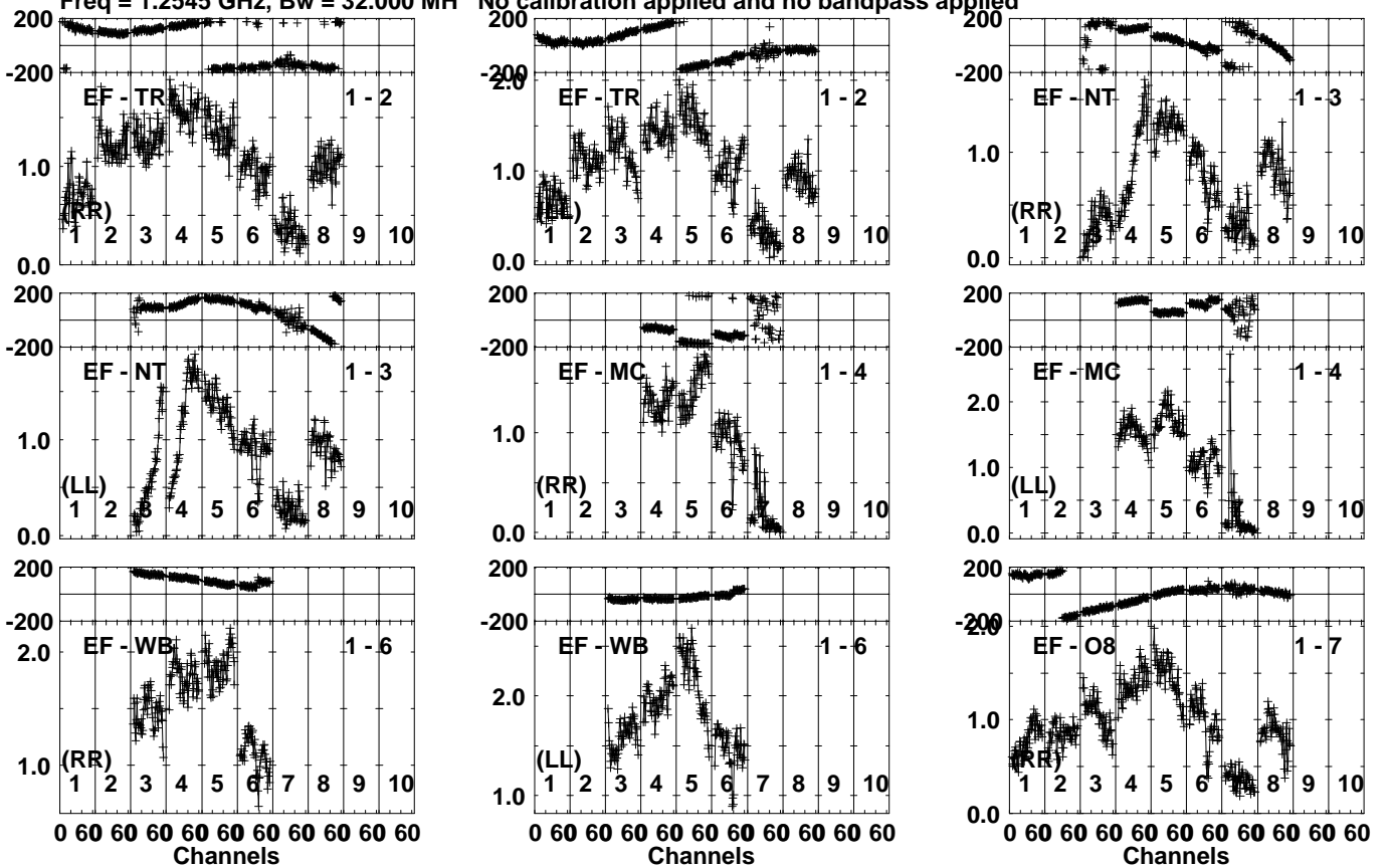
Lower frame: Milli Ampl Jy Top frame: Phas deg Vector averaged cross-power spectrum Several baselines displayed Timerange: 01/01:01:34 to 01/01:02:32
