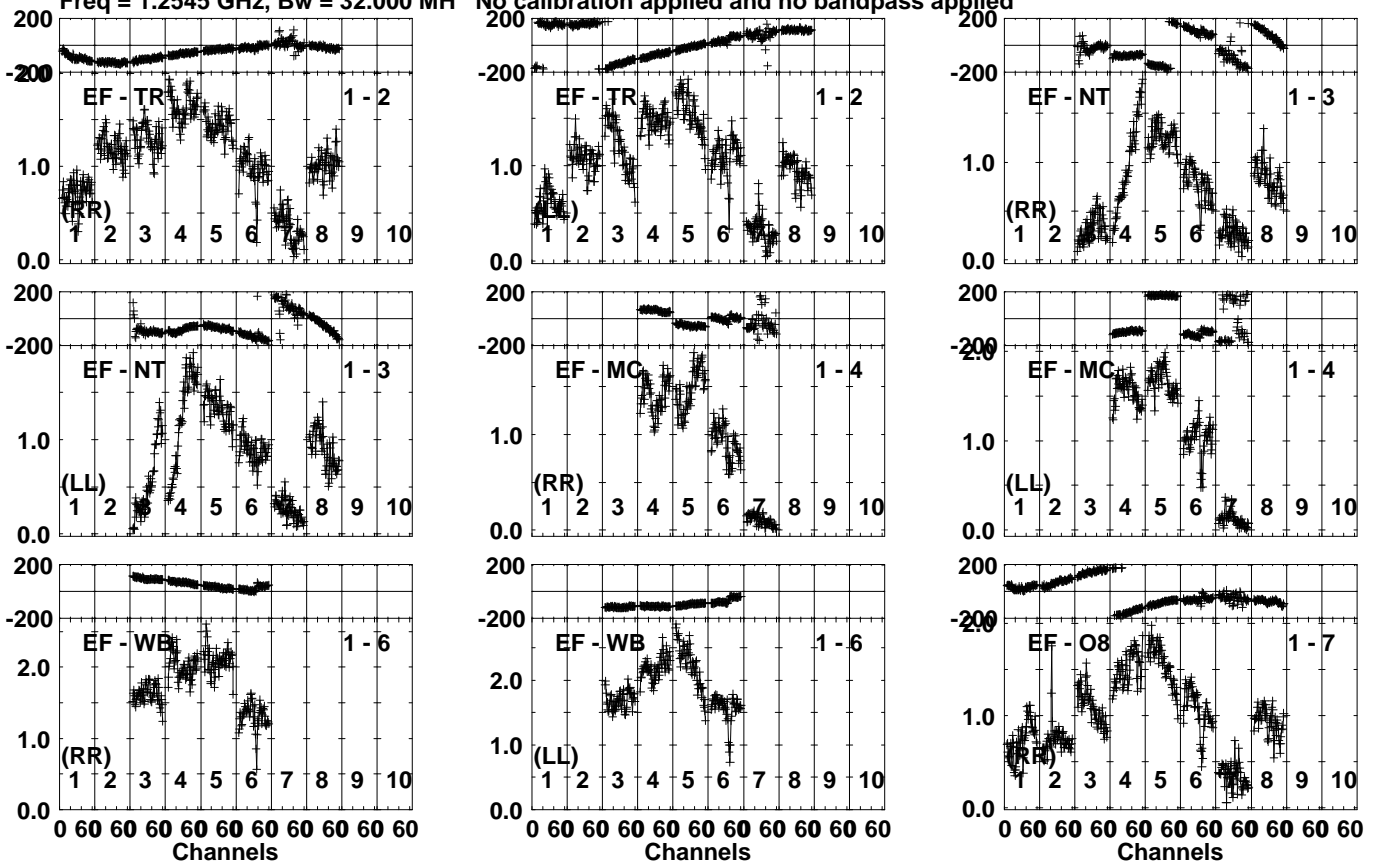
Lower frame: Milli Ampl Jy Top frame: Phas deg Vector averaged cross-power spectrum Several baselines displayed Timerange: 01/01:36:25 to 01/01:37:55
