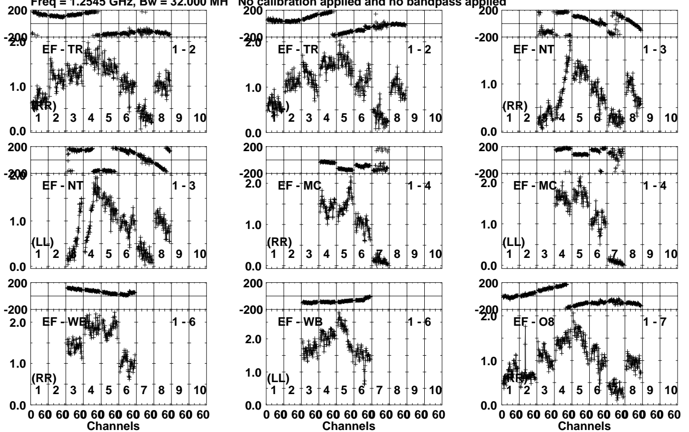
Lower frame: Milli Ampl Jy Top frame: Phas deg Vector averaged cross-power spectrum Several baselines displayed Timerange: 01/01:21:13 to 01/01:22:41
