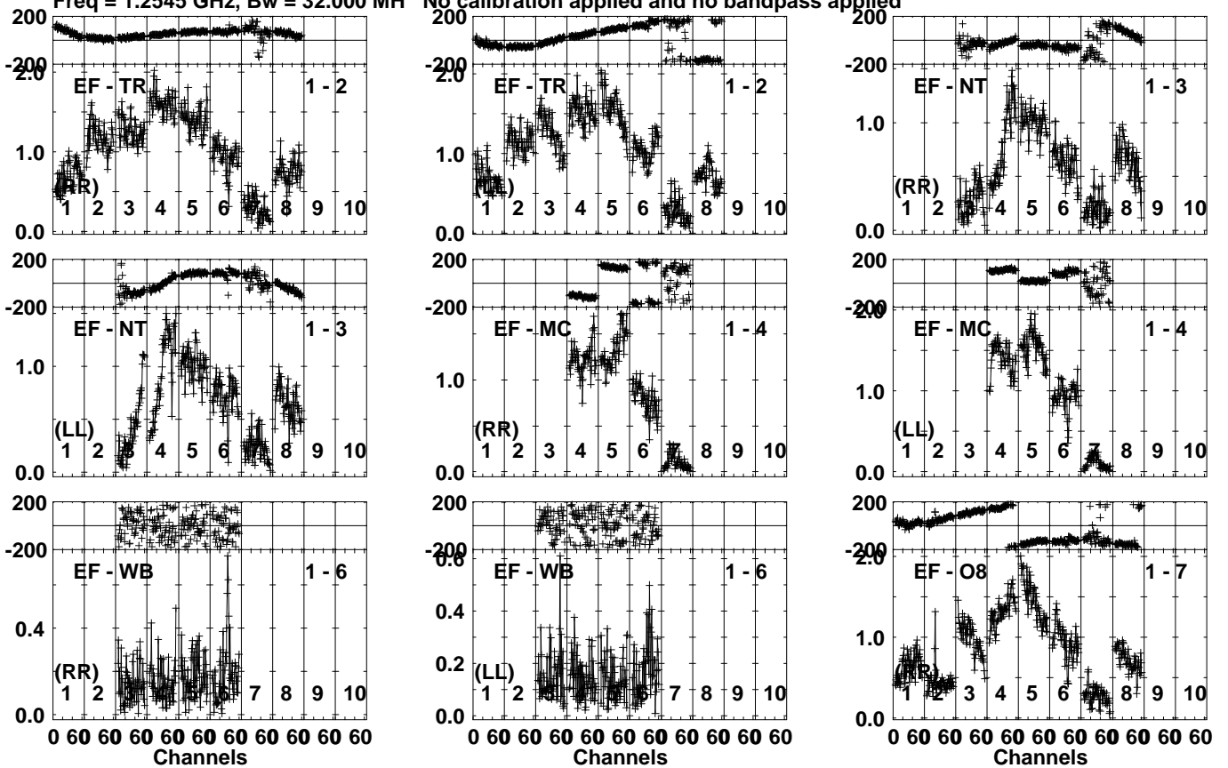
Lower frame: Milli Ampl Jy Top frame: Phas deg Vector averaged cross-power spectrum Several baselines displayed Timerange: 00/22:16:35 to 00/22:18:07
