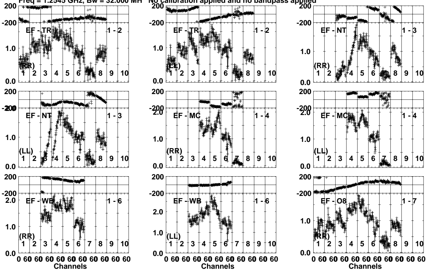
Lower frame: Milli Ampl Jy Top frame: Phas deg Vector averaged cross-power spectrum Several baselines displayed Timerange: 01/00:53:25 to 01/00:54:53
