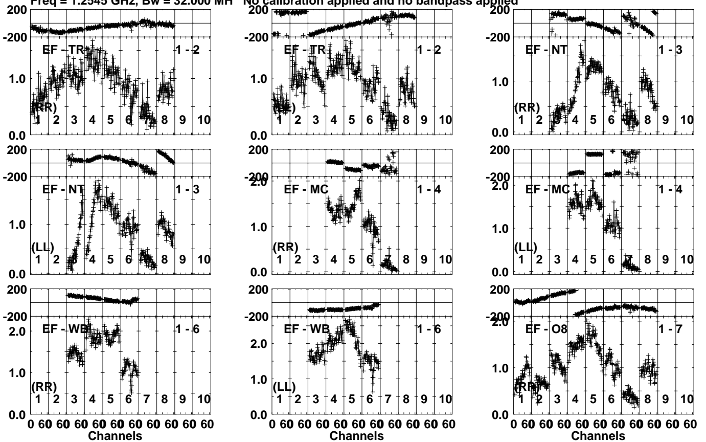
Lower frame: Milli Ampl Jy Top frame: Phas deg Vector averaged cross-power spectrum Several baselines displayed Timerange: 01/01:29:25 to 01/01:30:23
