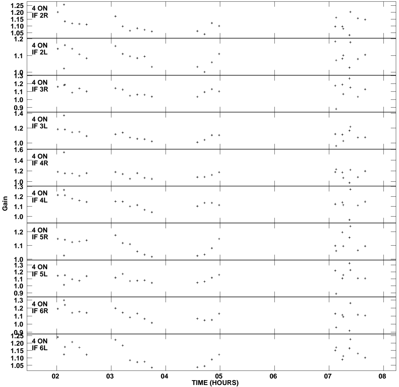
Plot file version 6 created 16-MAR-2007 12:21:08 Gain amp vs UTC time for J1206+3941.MULTI.1 SN 2 Rpol & Lpol IF 1 - 8
