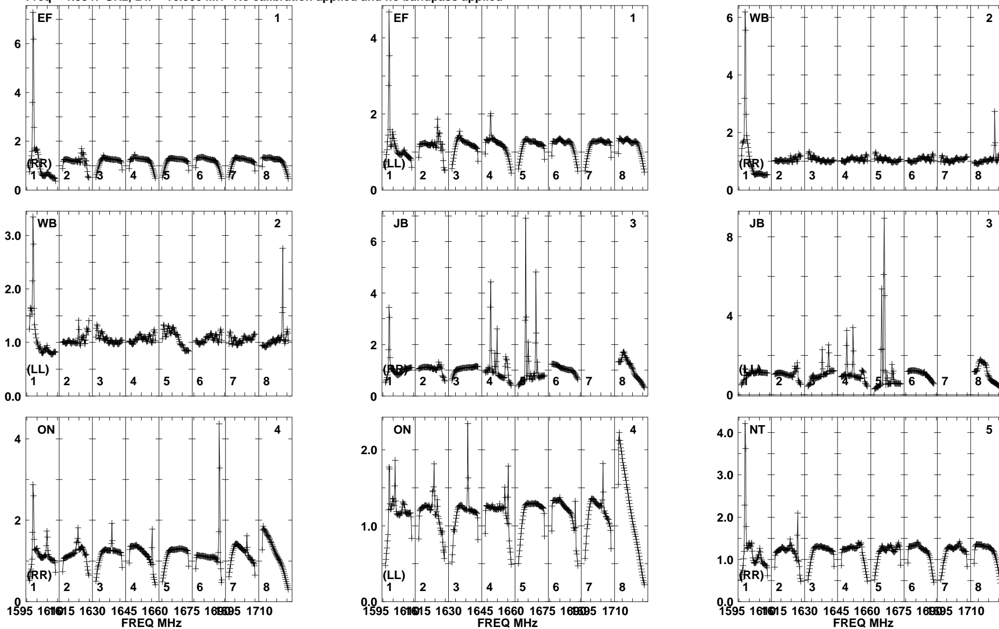
Lower frame: Real Jy Total-power spectrum Antenna: EF (01) Timerange: 01/10:21:56 to 01/10:22:44
