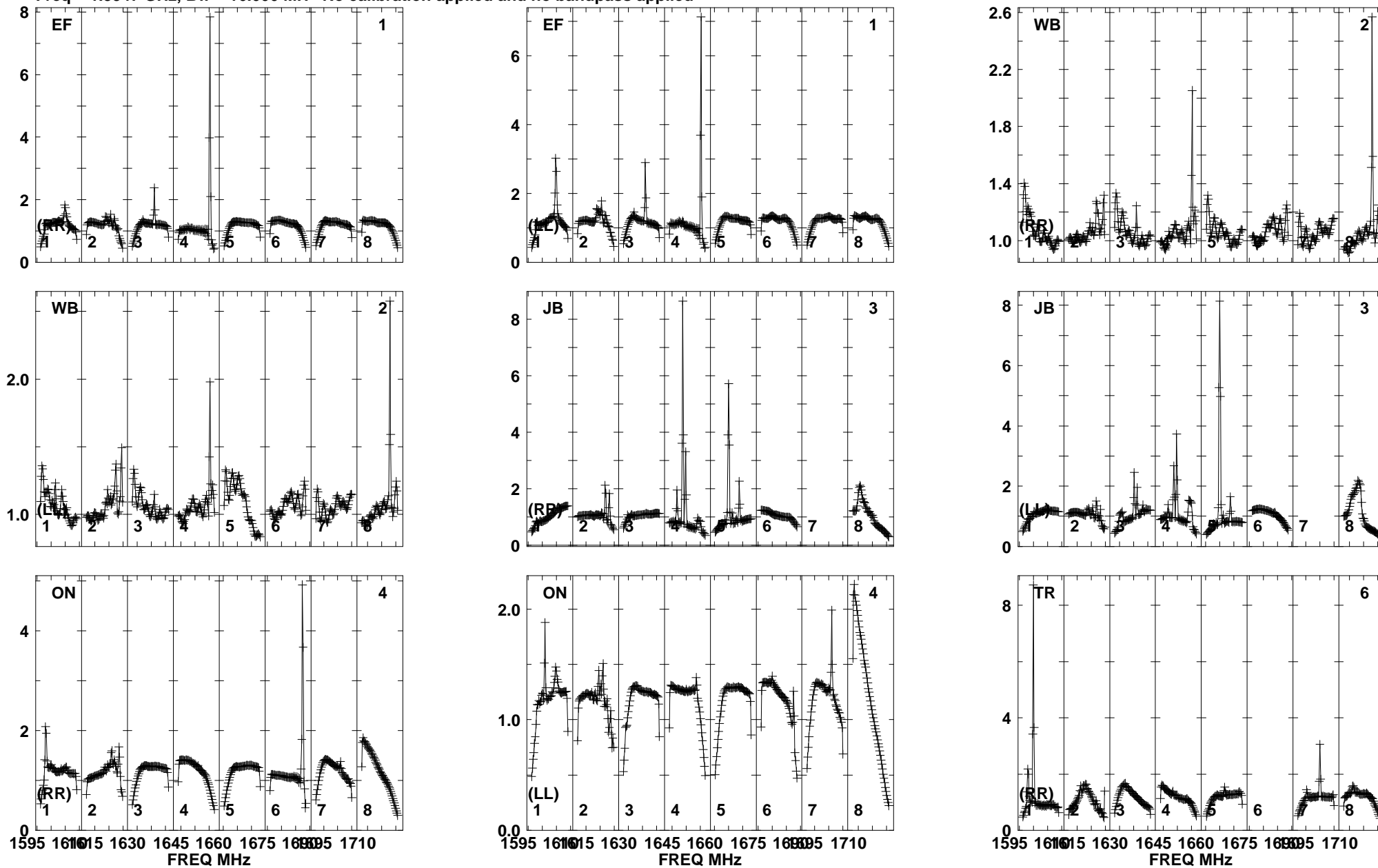
Lower frame: Real Jy Total-power spectrum Antenna: EF (01) Timerange: 01/10:51:30 to 01/10:55:24
