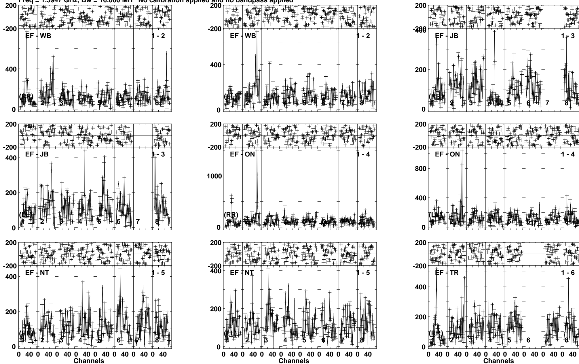
Lower frame: Micro Ampl Jy Top frame: Phas deg Vector averaged cross-power spectrum Baseline: EF (01) - WB (02) Timerange: 01/07:31:22 to 01/07:35:15
