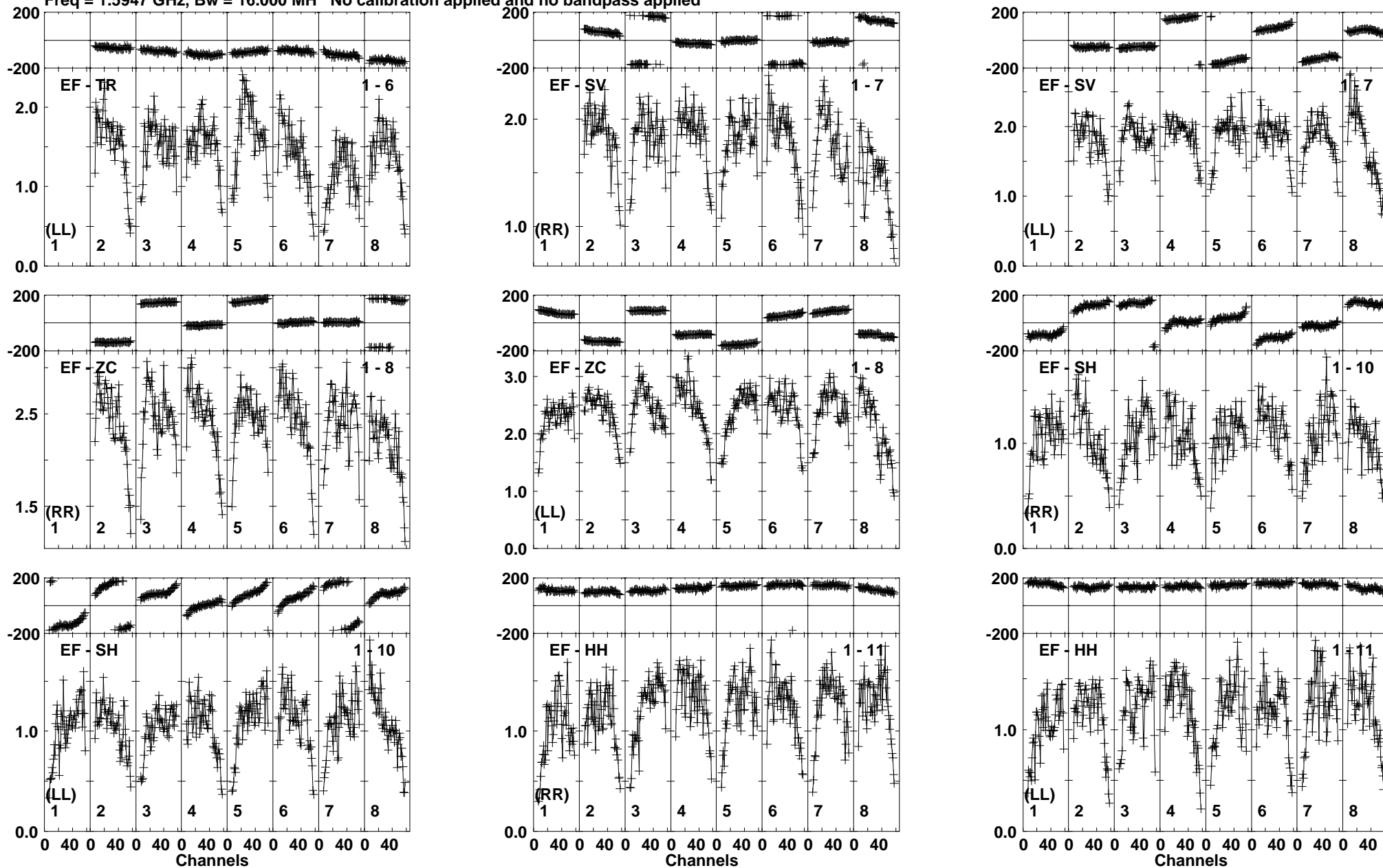
Lower frame: Milli Ampl Jy Top frame: Phas deg Vector averaged cross-power spectrum Baseline: EF (01) - TR (06) Timerange: 01/03:17:53 to 01/03:19:25
