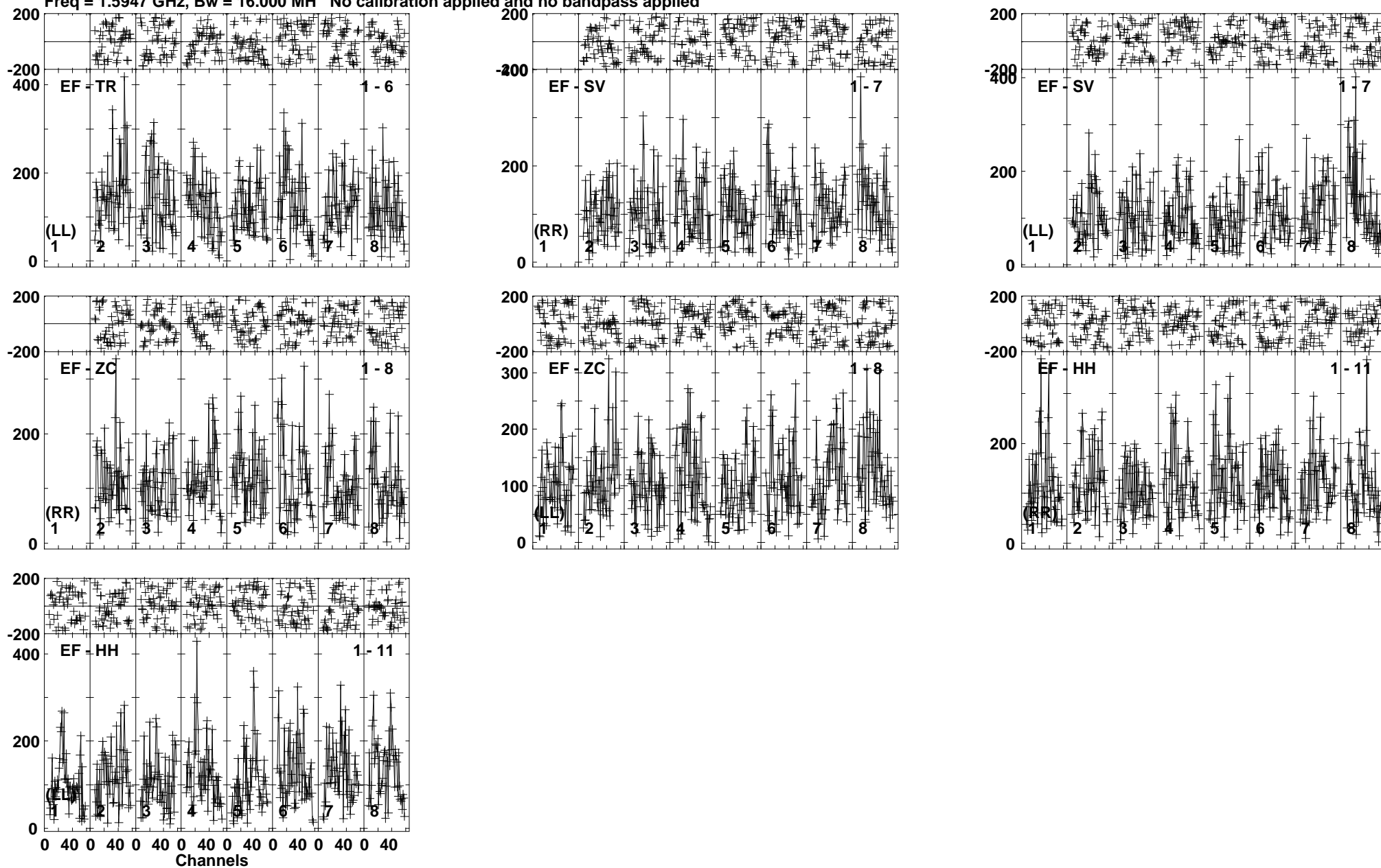
Lower frame: Micro Ampl Jy Top frame: Phas deg Vector averaged cross-power spectrum Baseline: EF (01) - TR (06) Timerange: 01/06:48:23 to 01/06:52:15
