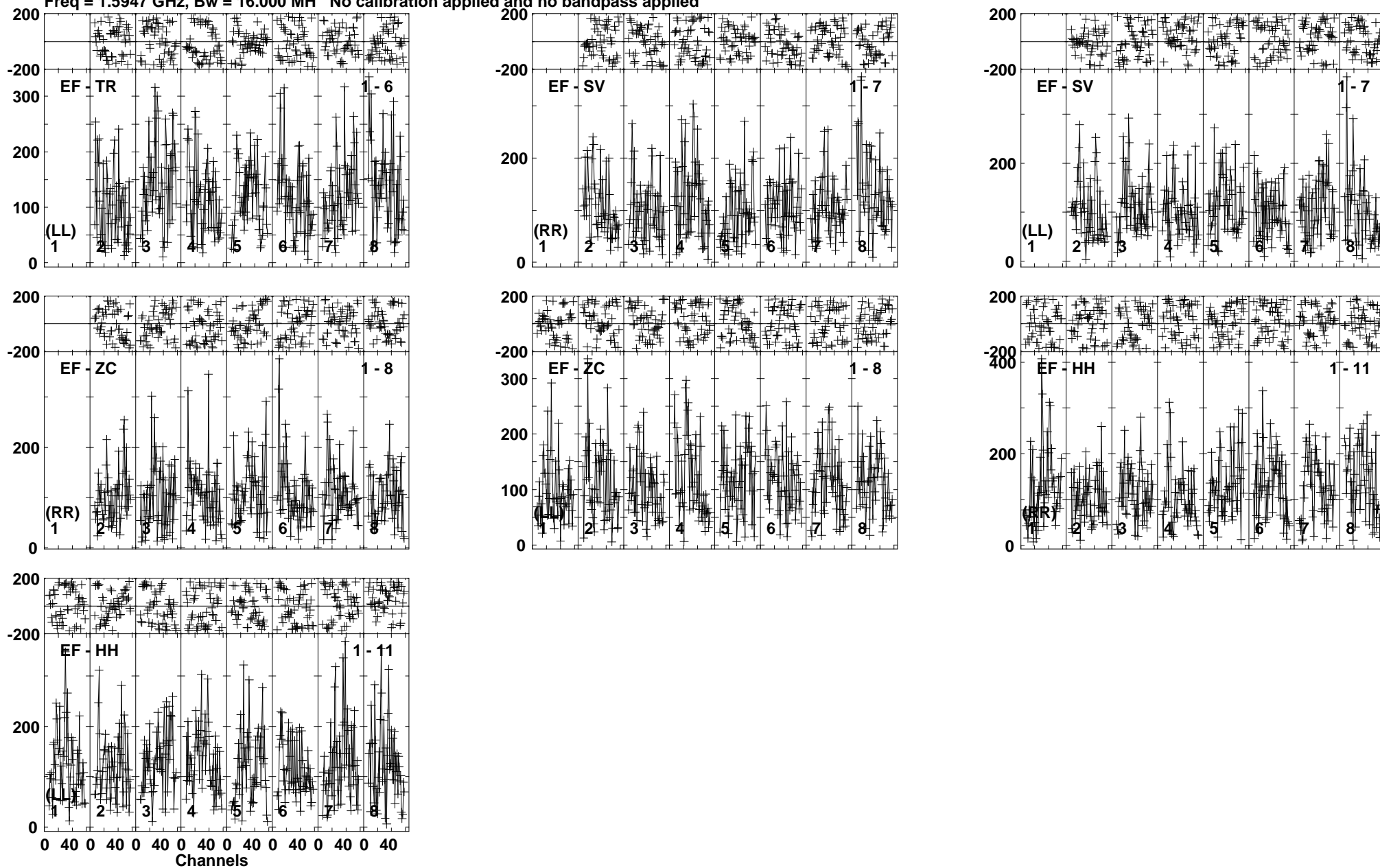
Lower frame: Micro Ampl Jy Top frame: Phas deg Vector averaged cross-power spectrum Baseline: EF (01) - TR (06) Timerange: 01/05:15:27 to 01/05:19:20
