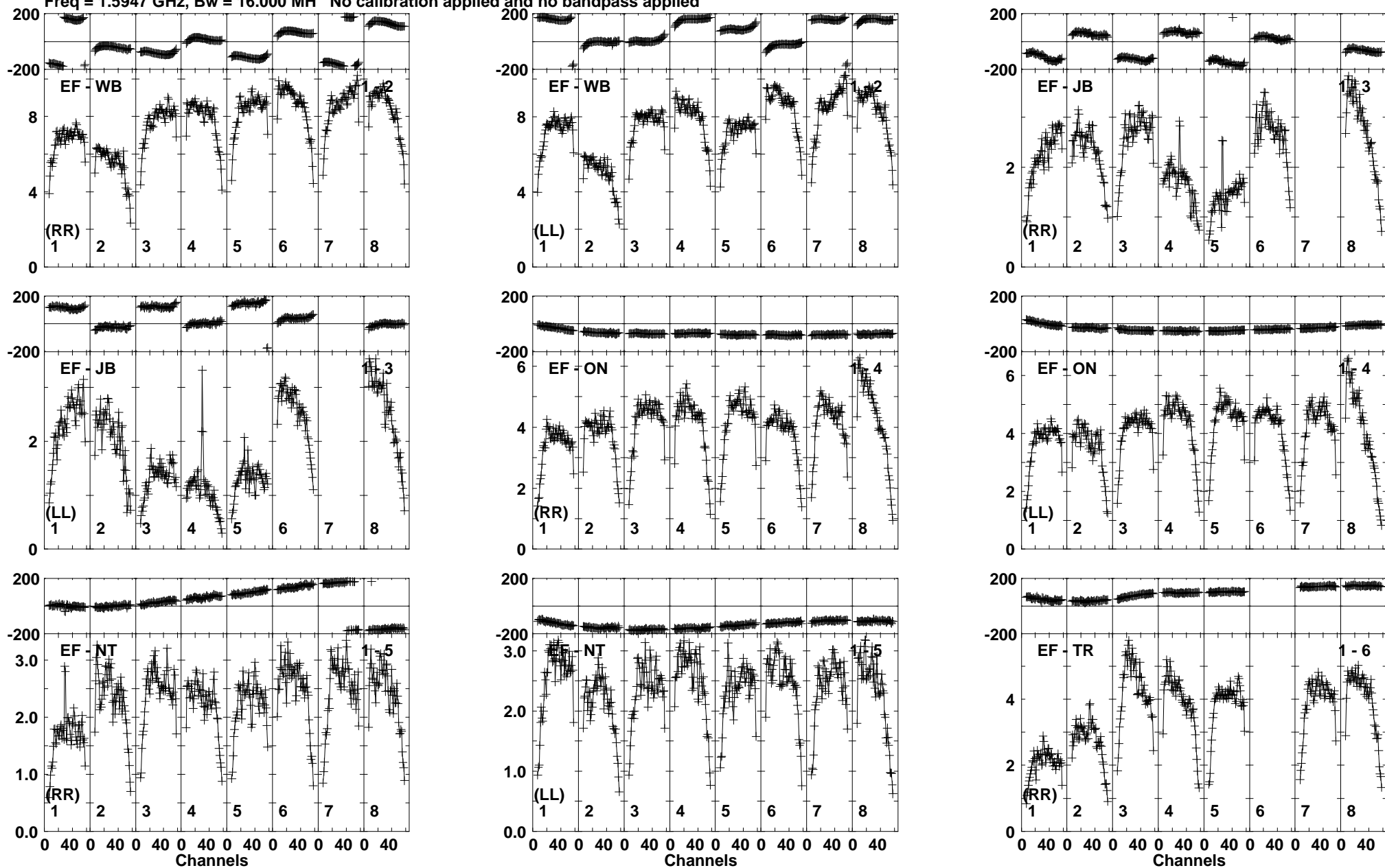
Lower frame: Milli Ampl Jy Top frame: Phas deg Vector averaged cross-power spectrum Baseline: EF (01) - WB (02) Timerange: 01/06:11:51 to 01/06:12:39
