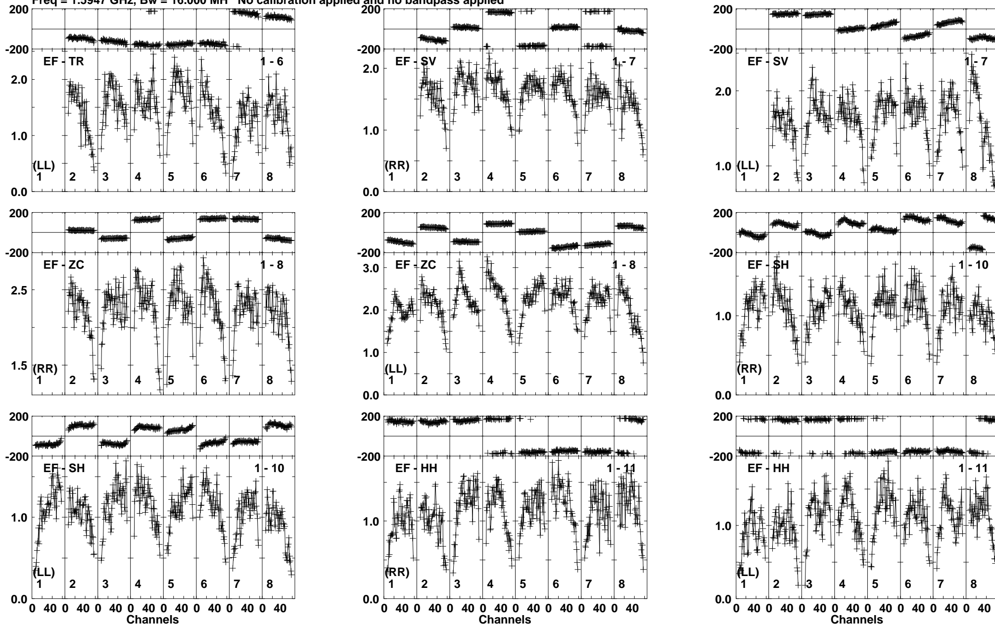
Lower frame: Milli Ampl Jy Top frame: Phas deg Vector averaged cross-power spectrum Baseline: EF (01) - TR (06) Timerange: 01/02:20:47 to 01/02:22:19
