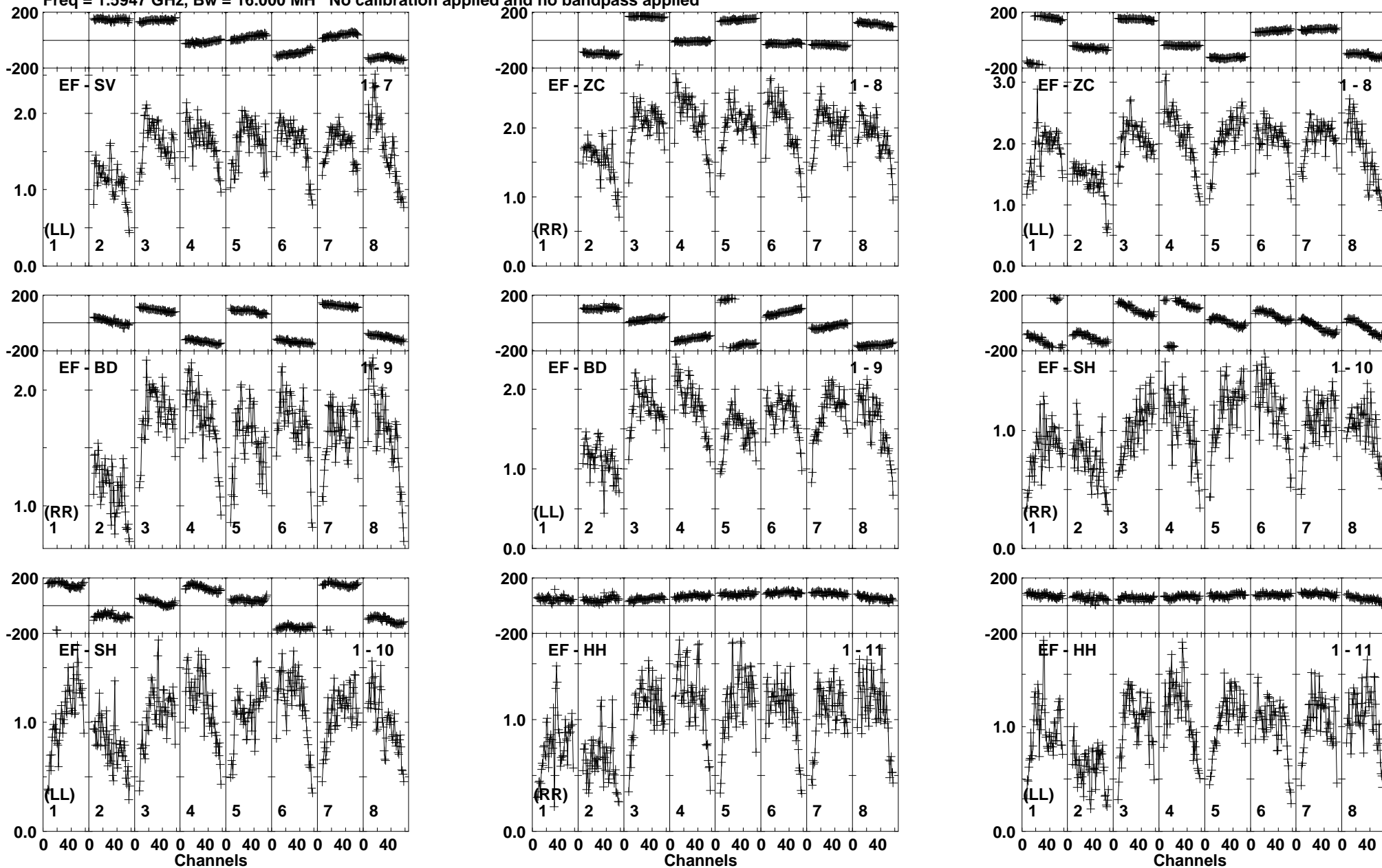
Lower frame: Milli Ampl Jy Top frame: Phas deg Vector averaged cross-power spectrum Baseline: EF (01) - SV (07) Timerange: 01/01:37:46 to 01/01:39:19
