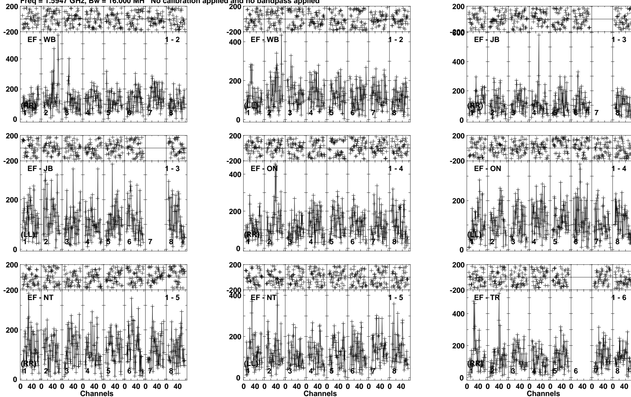
Lower frame: Micro Ampl Jy Top frame: Phas deg Vector averaged cross-power spectrum Baseline: EF (01) - WB (02) Timerange: 01/09:11:26 to 01/09:15:19
