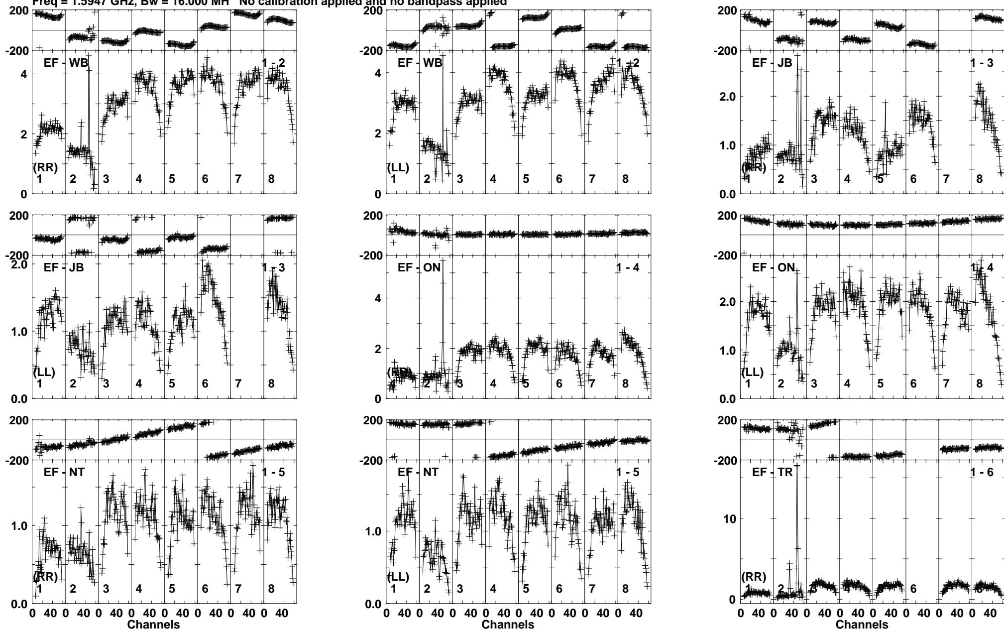
Lower frame: Milli Ampl Jy Top frame: Phas deg Vector averaged cross-power spectrum Baseline: EF (01) - WB (02) Timerange: 01/10:05:36 to 01/10:07:10
