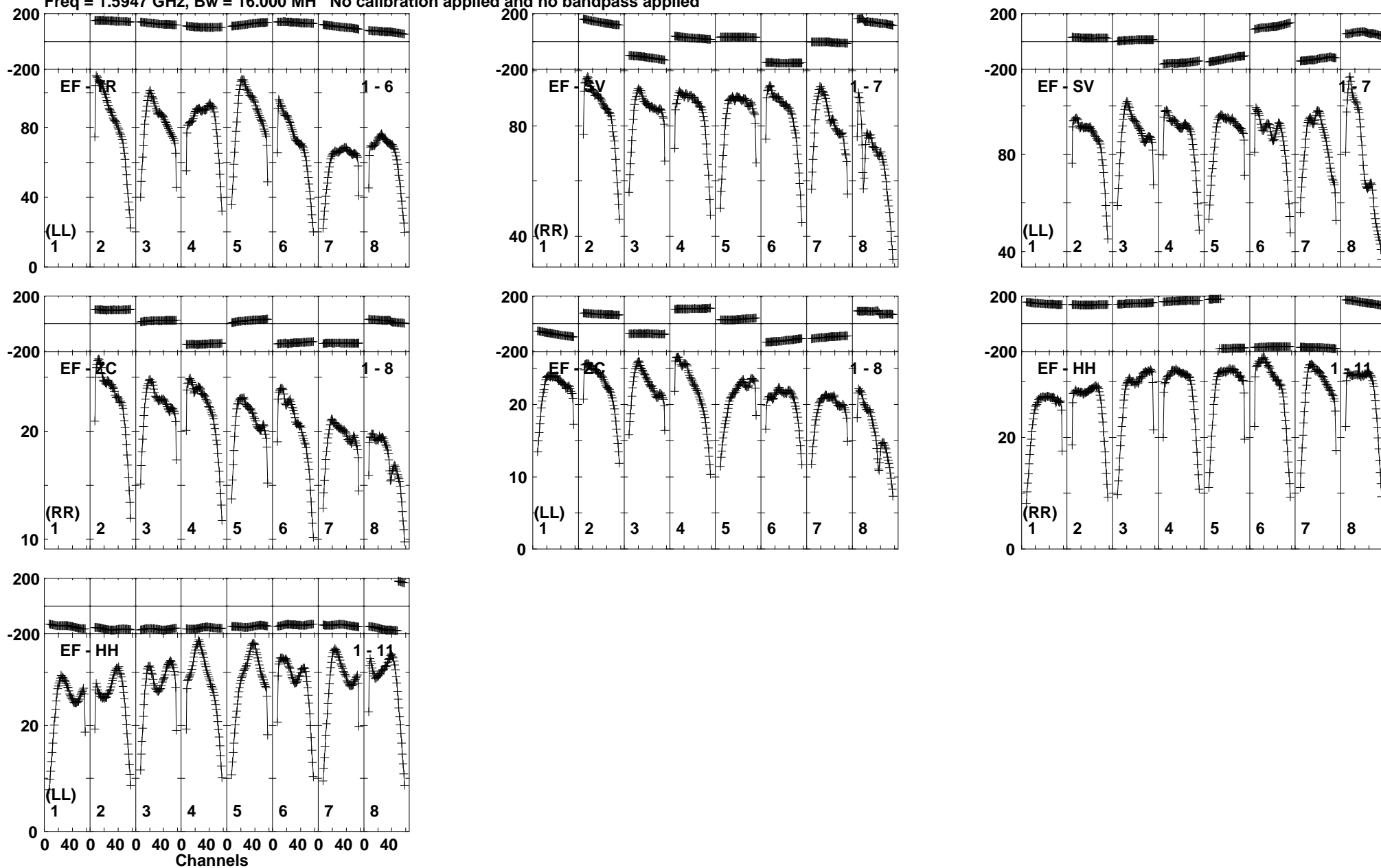
Lower frame: Milli Ampl Jy Top frame: Phas deg Vector averaged cross-power spectrum Baseline: EF (01) - TR (06) Timerange: 01/04:30:26 to 01/04:33:25
