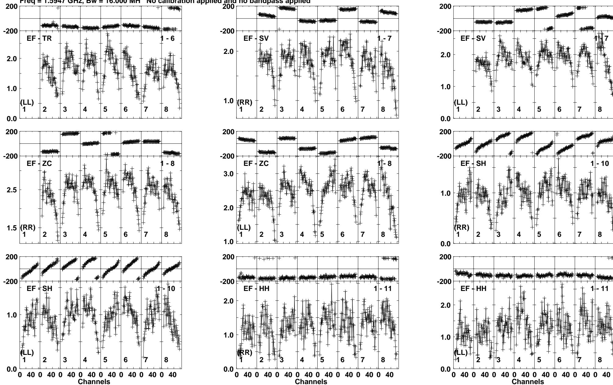
Lower frame: Milli Ampl Jy Top frame: Phas deg Vector averaged cross-power spectrum Baseline: EF (01) - TR (06) Timerange: 01/04:08:03 to 01/04:09:35
