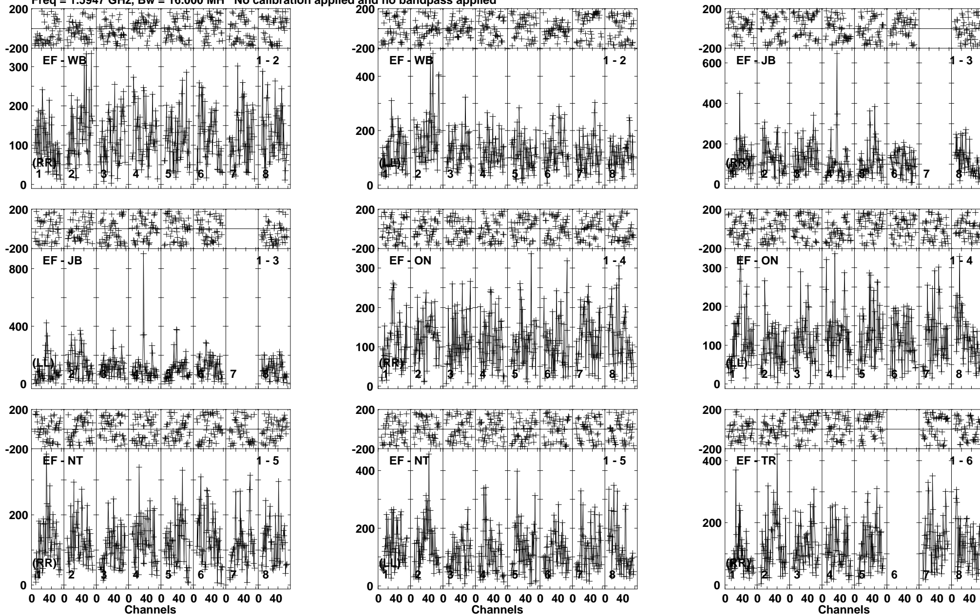
Lower frame: Micro Ampl Jy Top frame: Phas deg Vector averaged cross-power spectrum Baseline: EF (01) - WB (02) Timerange: 01/05:58:28 to 01/06:02:19
