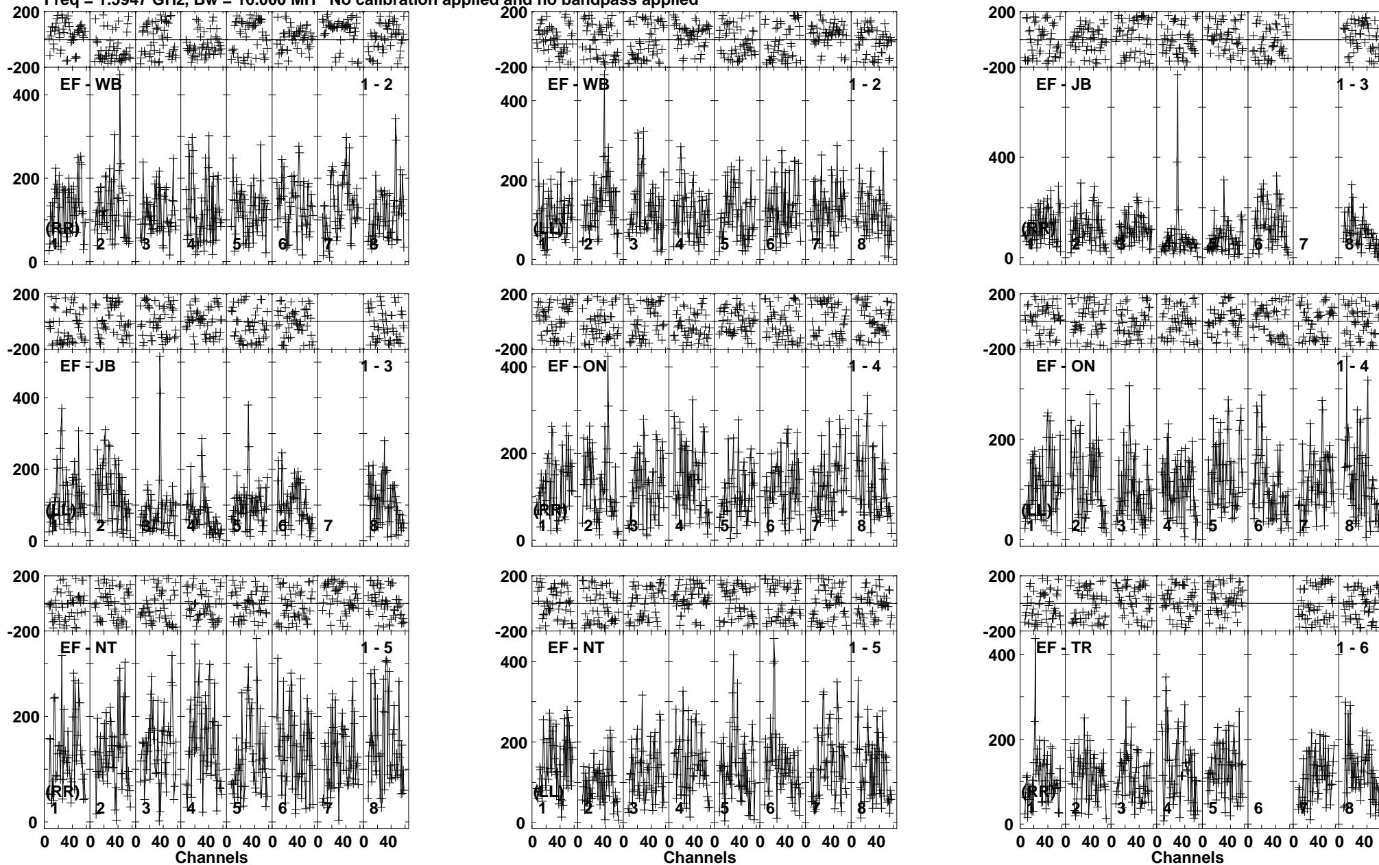
Lower frame: Micro Ampl Jy Top frame: Phas deg Vector averaged cross-power spectrum Baseline: EF (01) - WB (02) Timerange: 01/03:42:31 to 01/03:46:24
