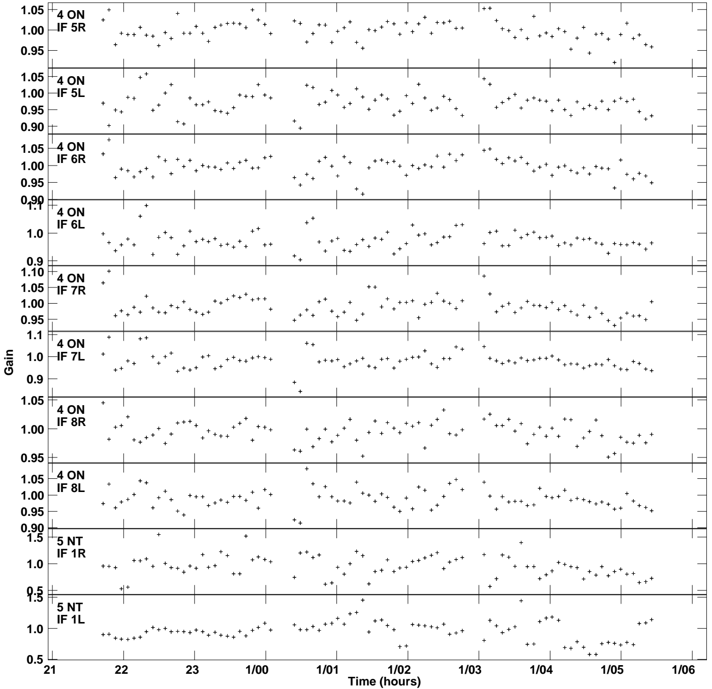
Plot file version 5 created 10-SEP-2014 17:42:21 Gain amp vs UTC time for J1754+6452.MULTI.1 SN 2 Rpol & Lpol IF 1 - 8
