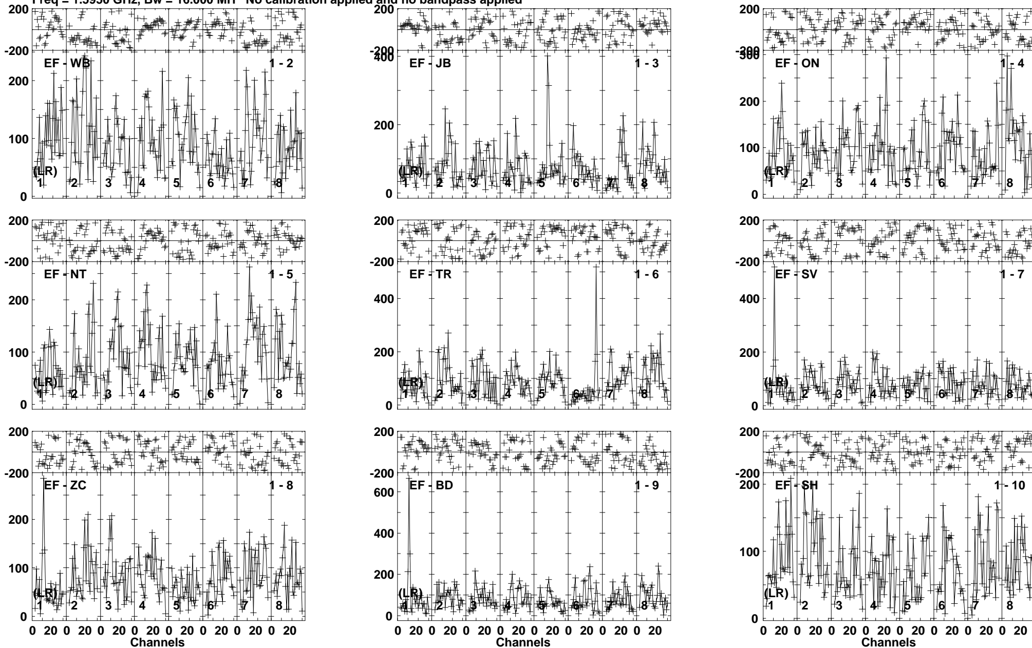
Lower frame: Micro Ampl Jy Top frame: Phas deg Vector averaged cross-power spectrum Baseline: EF (01) - WB (02) Timerange: 00/22:04:34 to 00/22:07:58
