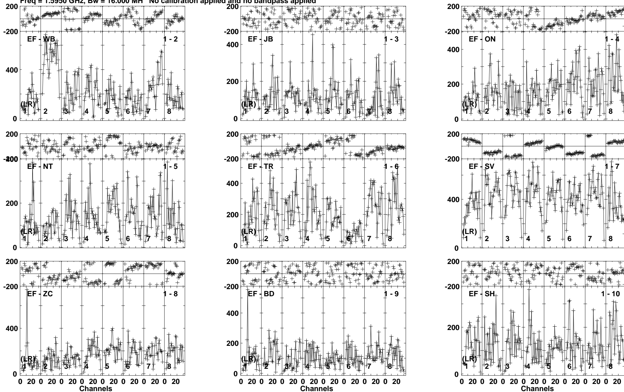
Lower frame: Micro Ampl Jy Top frame: Phas deg Vector averaged cross-power spectrum Baseline: EF (01) - WB (02) Timerange: 01/03:14:03 to 01/03:15:29
