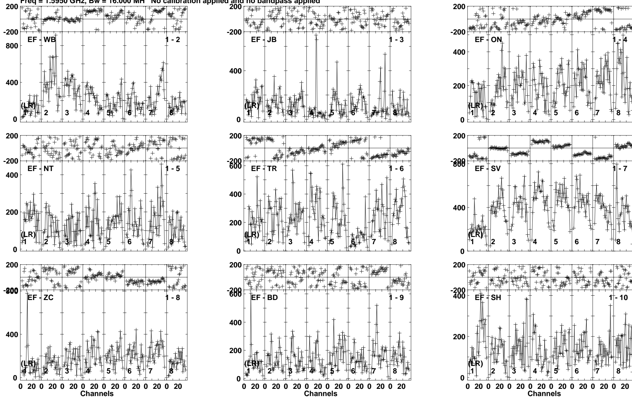
Lower frame: Micro Ampl Jy Top frame: Phas deg Vector averaged cross-power spectrum Baseline: EF (01) - WB (02) Timerange: 01/04:48:33 to 01/04:49:59
