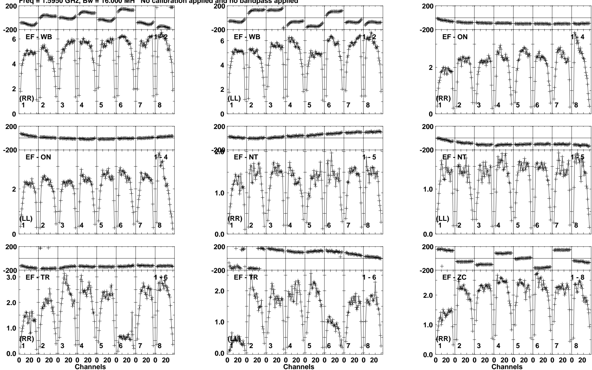
Lower frame: Milli Ampl Jy Top frame: Phas deg Vector averaged cross-power spectrum Baseline: EF (01) - WB (02) Timerange: 01/00:03:34 to 01/00:04:58
