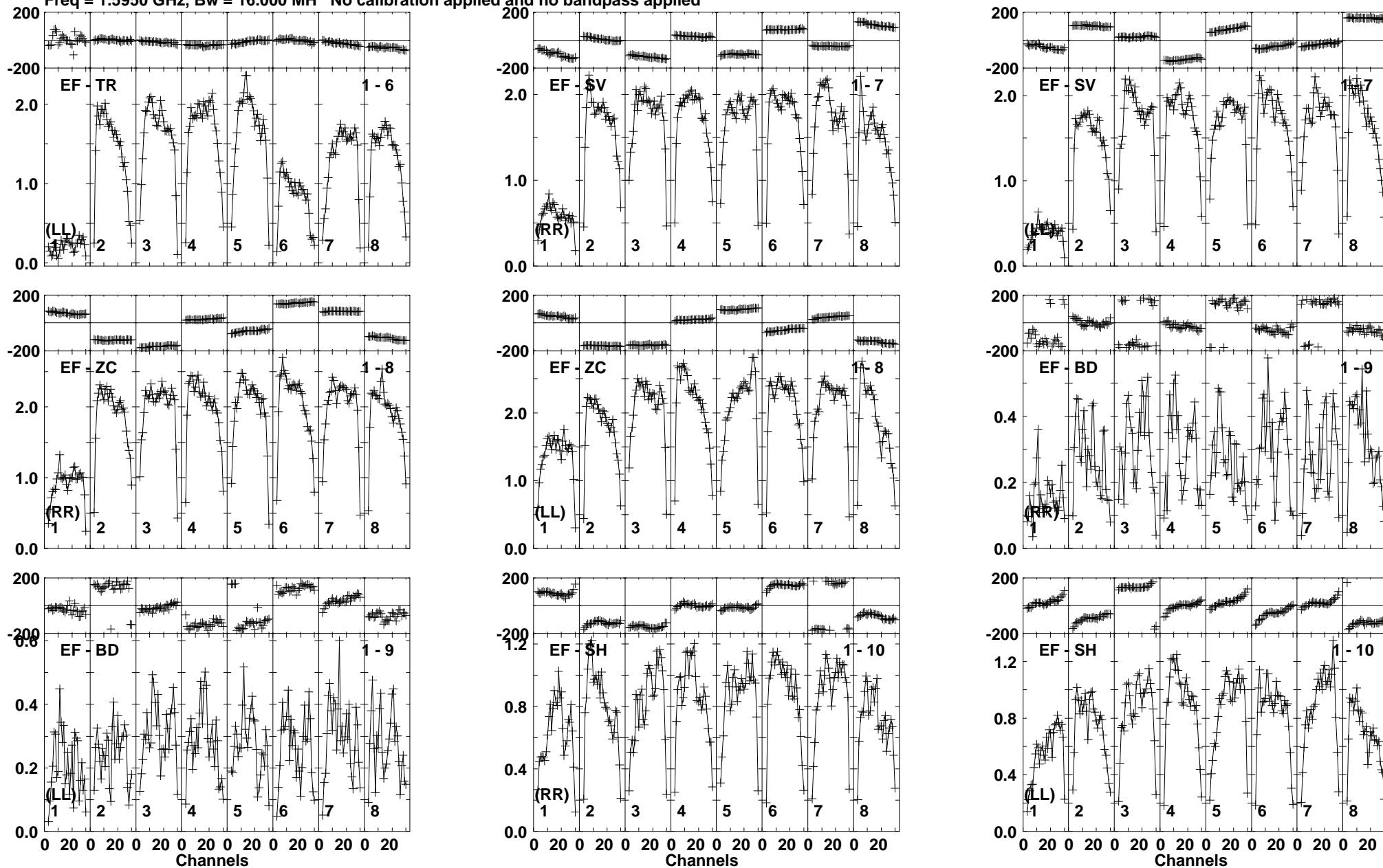
Lower frame: Milli Ampl Jy Top frame: Phas deg Vector averaged cross-power spectrum Baseline: EF (01) - TR (06) Timerange: 01/04:06:33 to 01/04:07:59
