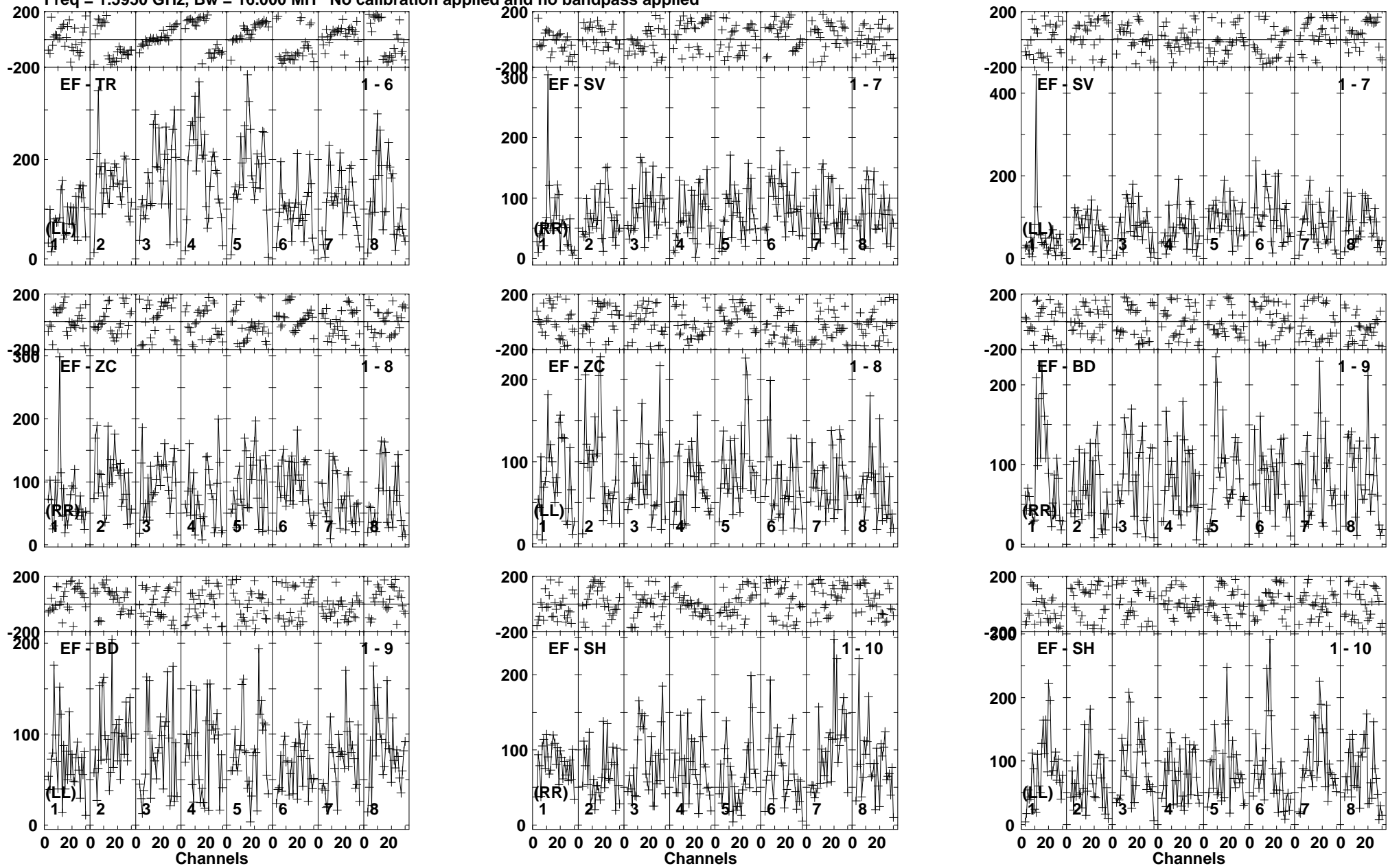
Lower frame: Micro Ampl Jy Top frame: Phas deg Vector averaged cross-power spectrum Baseline: EF (01) - TR (06) Timerange: 01/03:52:03 to 01/03:55:29
