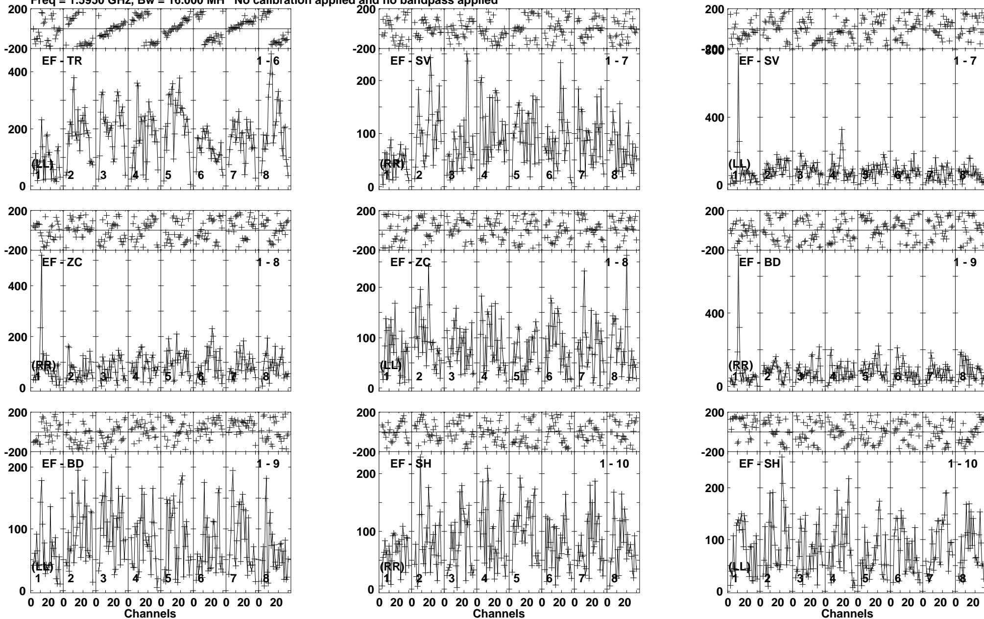
Lower frame: Micro Ampl Jy Top frame: Phas deg Vector averaged cross-power spectrum Baseline: EF (01) - TR (06) Timerange: 01/01:49:04 to 01/01:52:28
