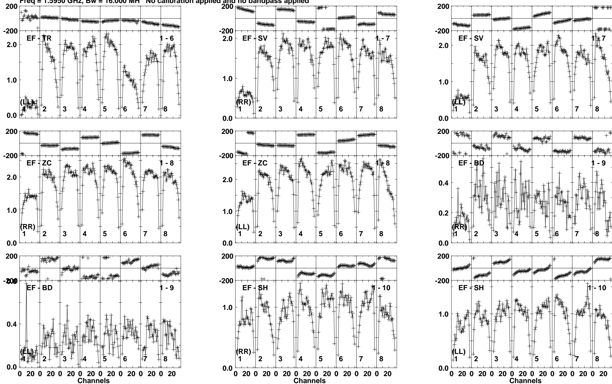
Lower frame: Milli Ampl Jy Top frame: Phas deg Vector averaged cross-power spectrum Baseline: EF (01) - TR (06) Timerange: 01/01:37:03 to 01/01:38:29
