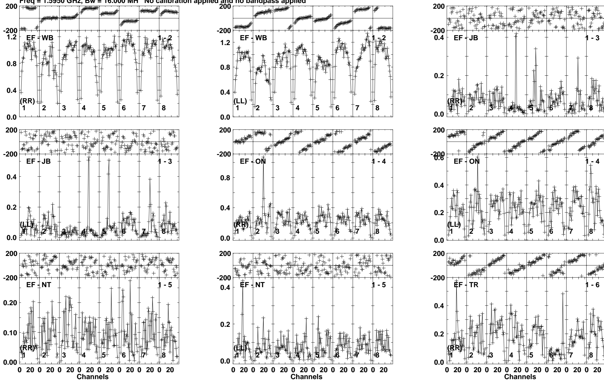
Lower frame: Milli Ampl Jy Top frame: Phas deg Vector averaged cross-power spectrum Baseline: EF (01) - WB (02) Timerange: 01/00:00:04 to 01/00:03:28
