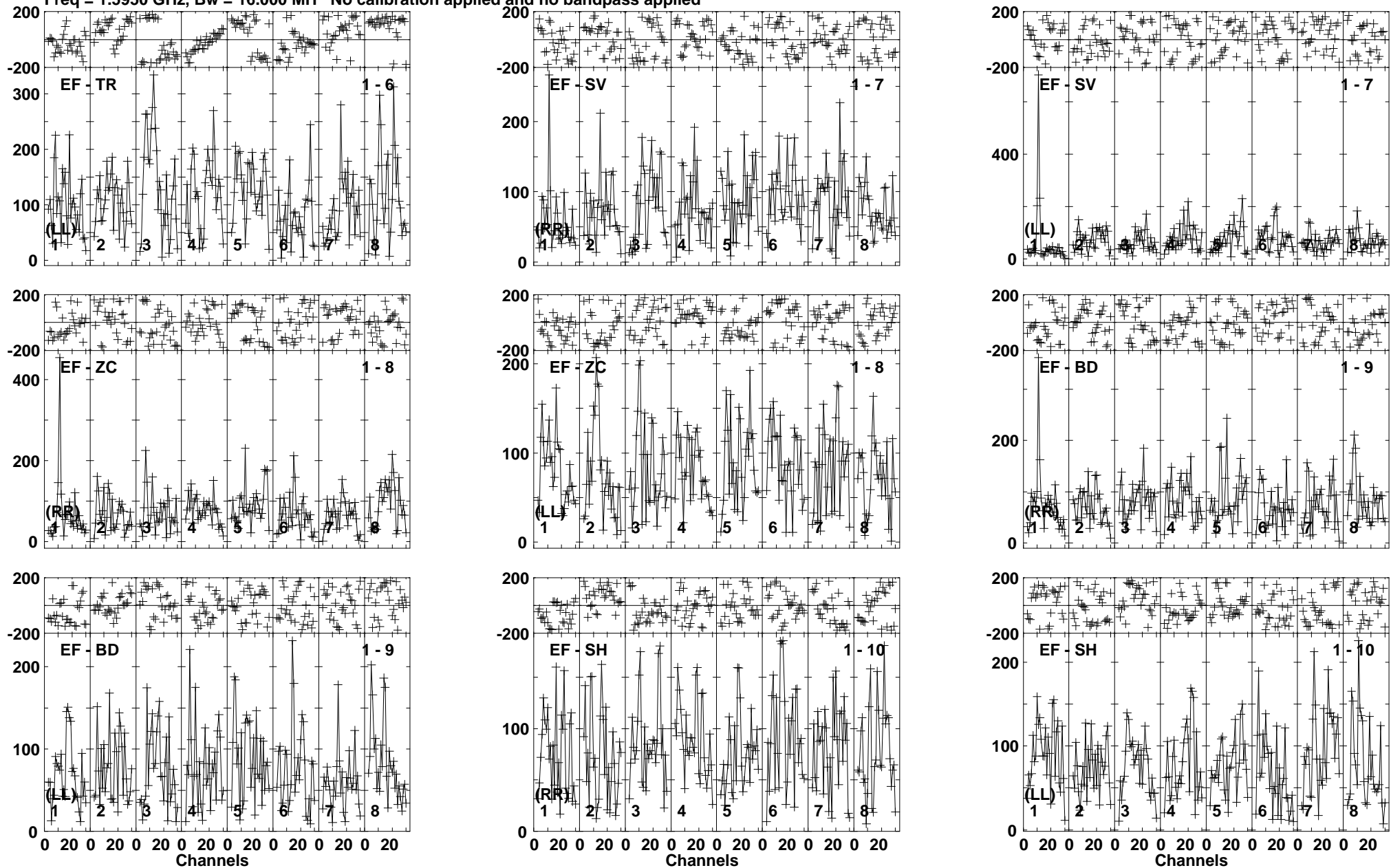
Lower frame: Micro Ampl Jy Top frame: Phas deg Vector averaged cross-power spectrum Baseline: EF (01) - TR (06) Timerange: 01/05:21:34 to 01/05:24:58
