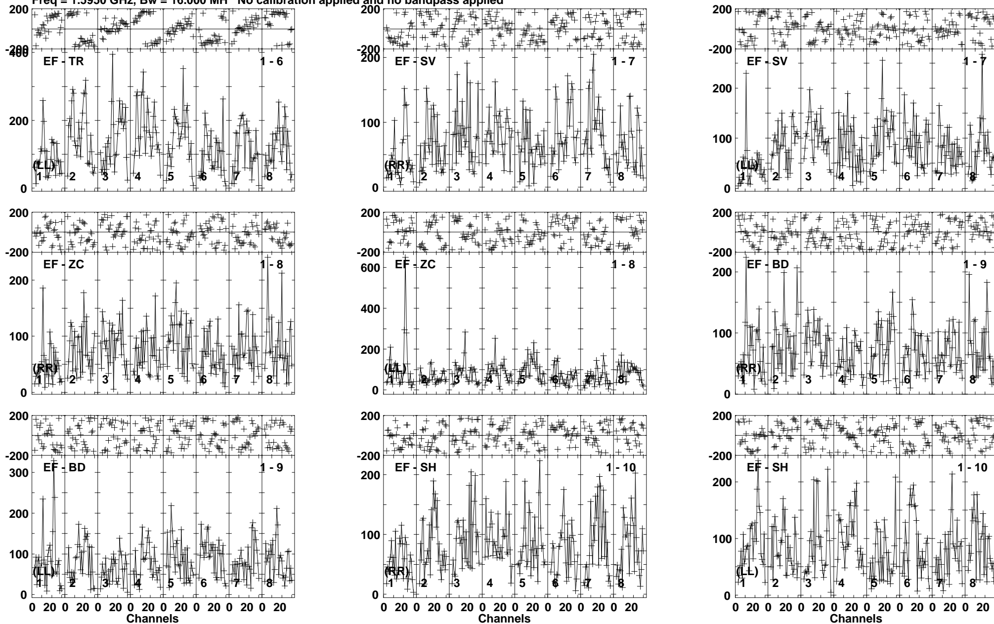
Lower frame: Micro Ampl Jy Top frame: Phas deg Vector averaged cross-power spectrum Baseline: EF (01) - TR (06) Timerange: 01/04:13:03 to 01/04:16:29
