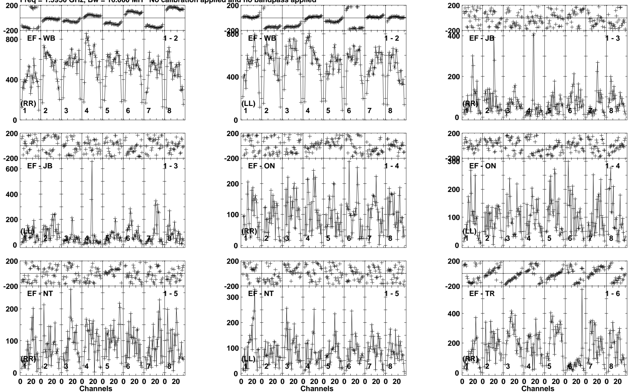
Lower frame: Micro Ampl Jy Top frame: Phas deg Vector averaged cross-power spectrum Baseline: EF (01) - WB (02) Timerange: 01/04:08:04 to 01/04:11:28
