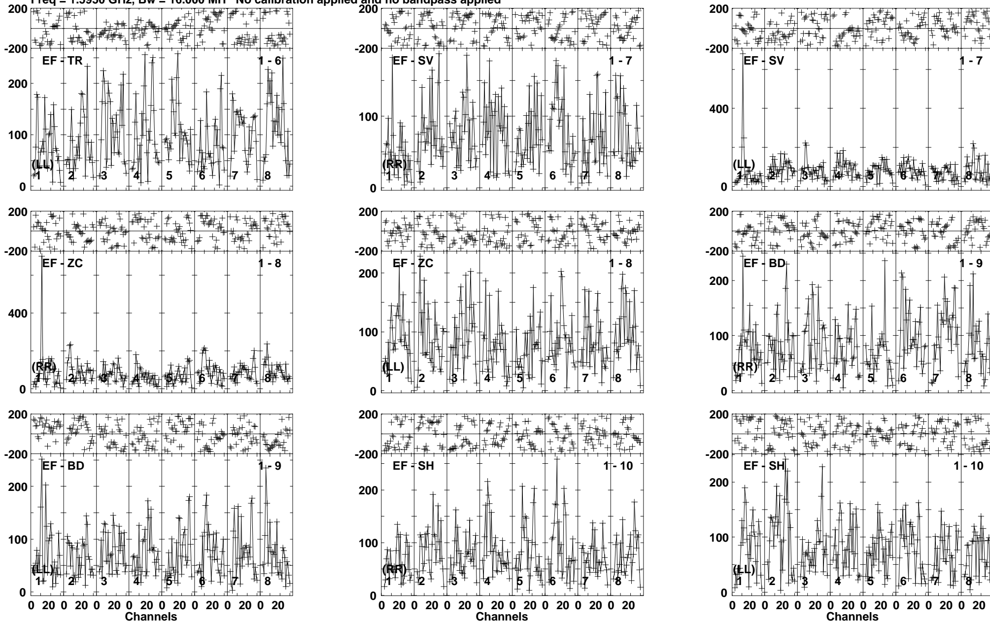
Lower frame: Micro Ampl Jy Top frame: Phas deg Vector averaged cross-power spectrum Baseline: EF (01) - TR (06) Timerange: 00/21:43:34 to 00/21:46:58
