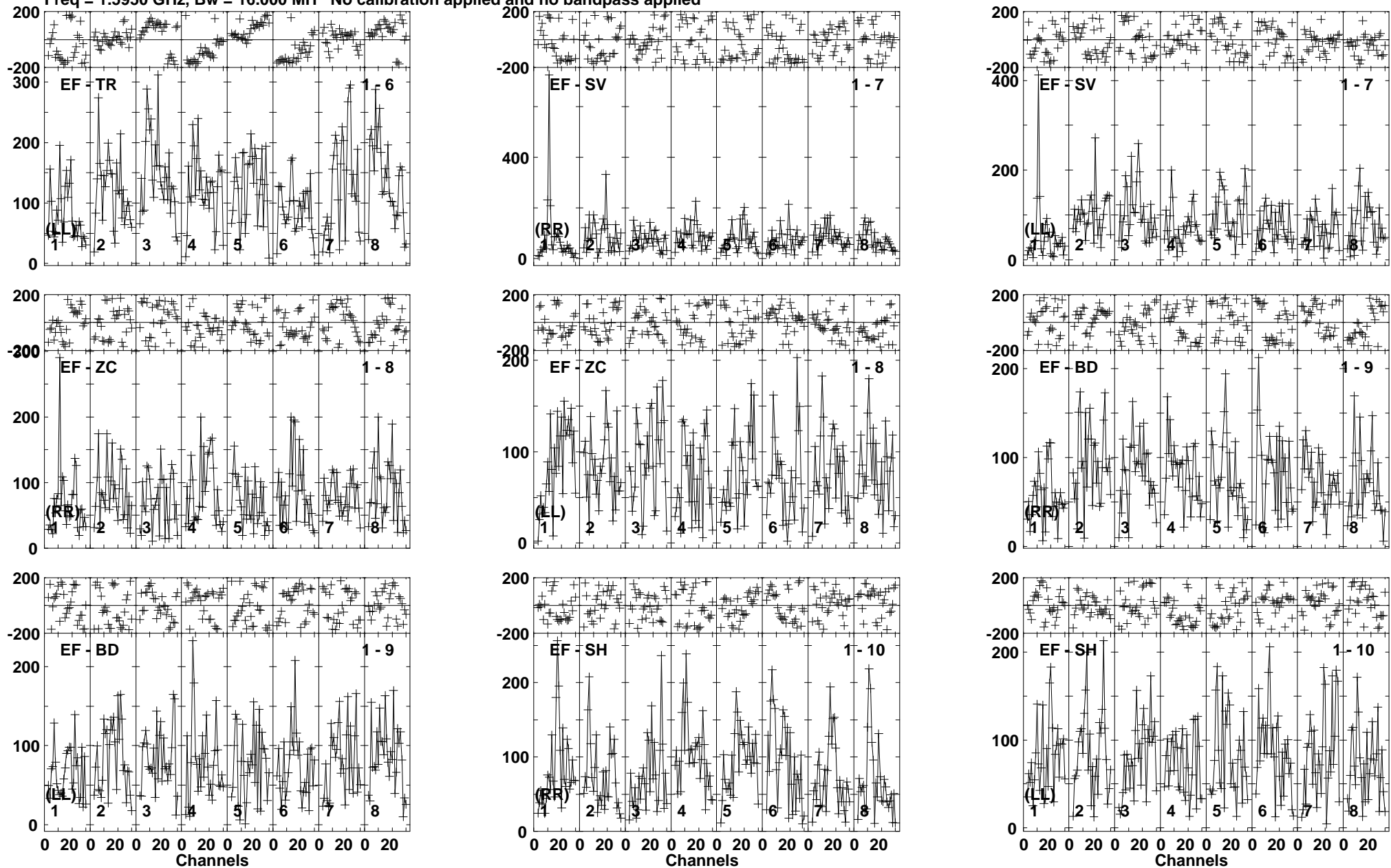
Lower frame: Micro Ampl Jy Top frame: Phas deg Vector averaged cross-power spectrum Baseline: EF (01) - TR (06) Timerange: 01/05:05:33 to 01/05:08:59
