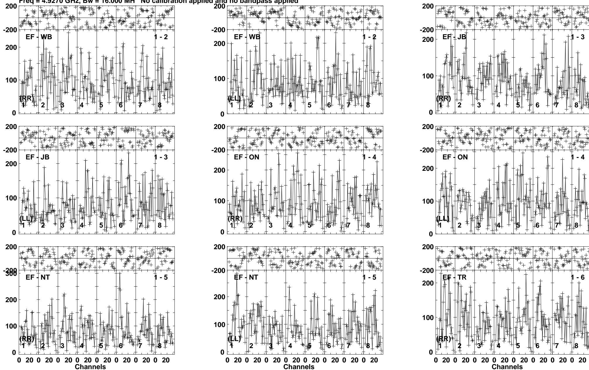
Lower frame: Micro Ampl Jy Top frame: Phas deg Vector averaged cross-power spectrum Baseline: EF (01) - WB (02) Timerange: 01/01:06:04 to 01/01:09:28
