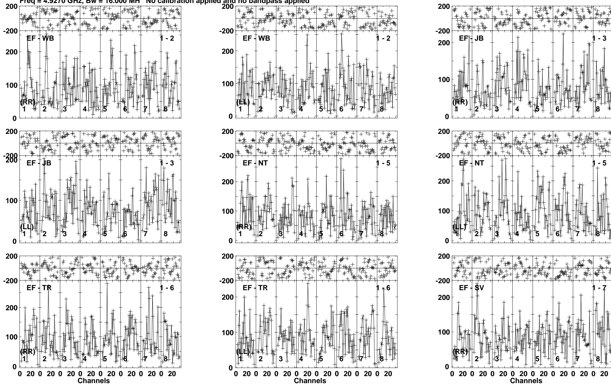
Lower frame: Micro Ampl Jy Top frame: Phas deg Vector averaged cross-power spectrum Baseline: EF (01) - WB (02) Timerange: 01/03:25:34 to 01/03:28:58
