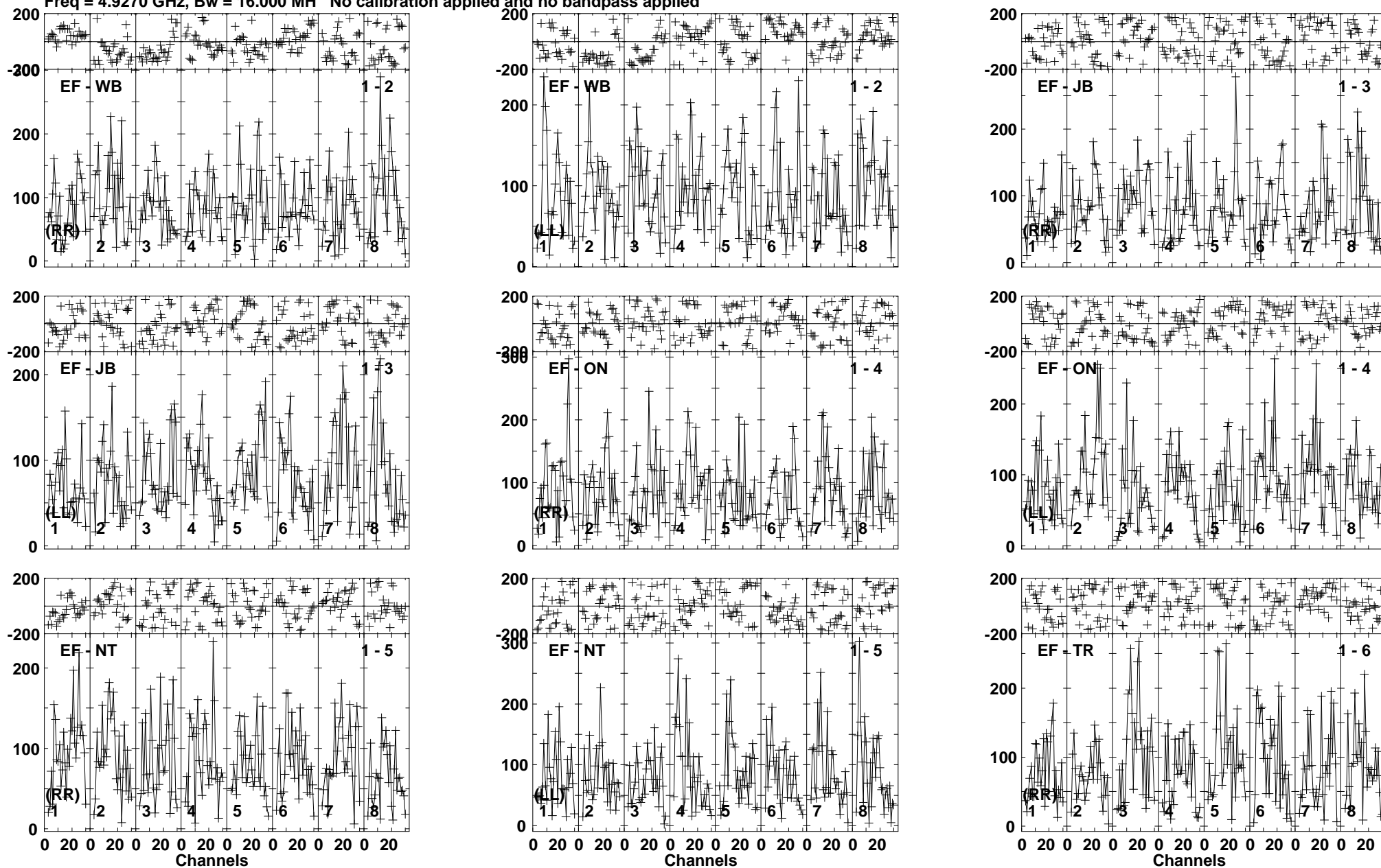
Lower frame: Micro Ampl Jy Top frame: Phas deg Vector averaged cross-power spectrum Baseline: EF (01) - WB (02) Timerange: 01/00:18:34 to 01/00:21:58
