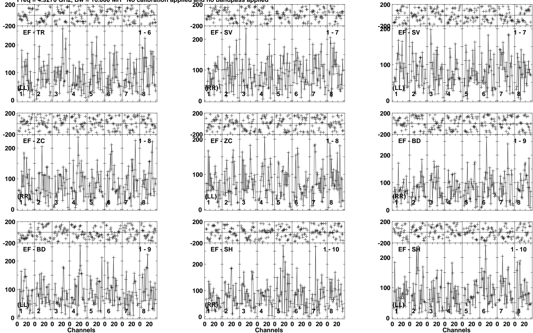
Lower frame: Micro Ampl Jy Top frame: Phas deg Vector averaged cross-power spectrum Baseline: EF (01) - TR (06) Timerange: 01/01:06:04 to 01/01:09:28
