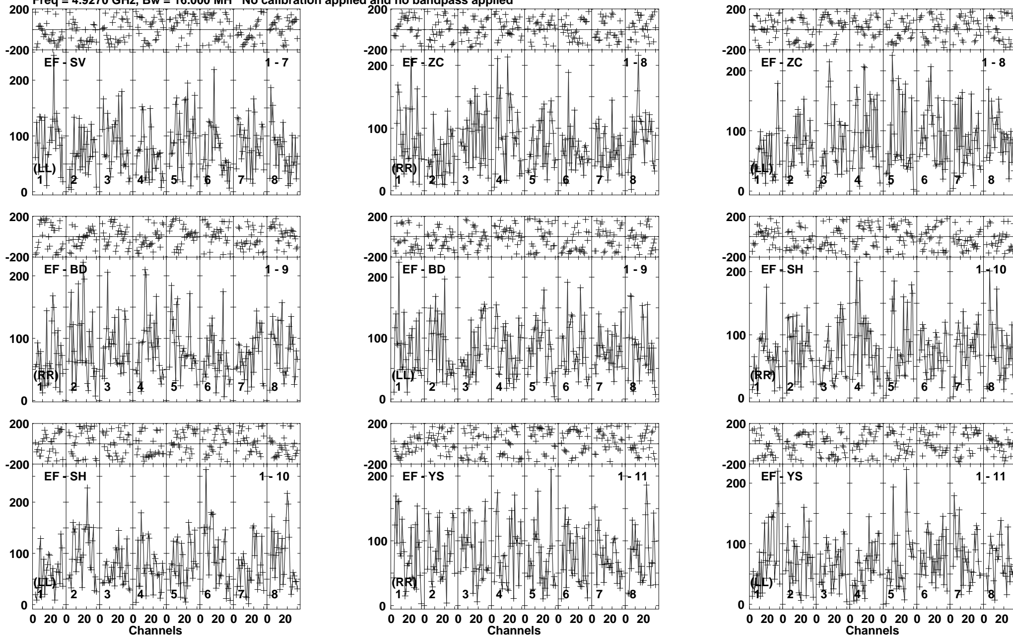
Lower frame: Micro Ampl Jy Top frame: Phas deg Vector averaged cross-power spectrum Baseline: EF (01) - SV (07) Timerange: 01/03:31:04 to 01/03:34:28
