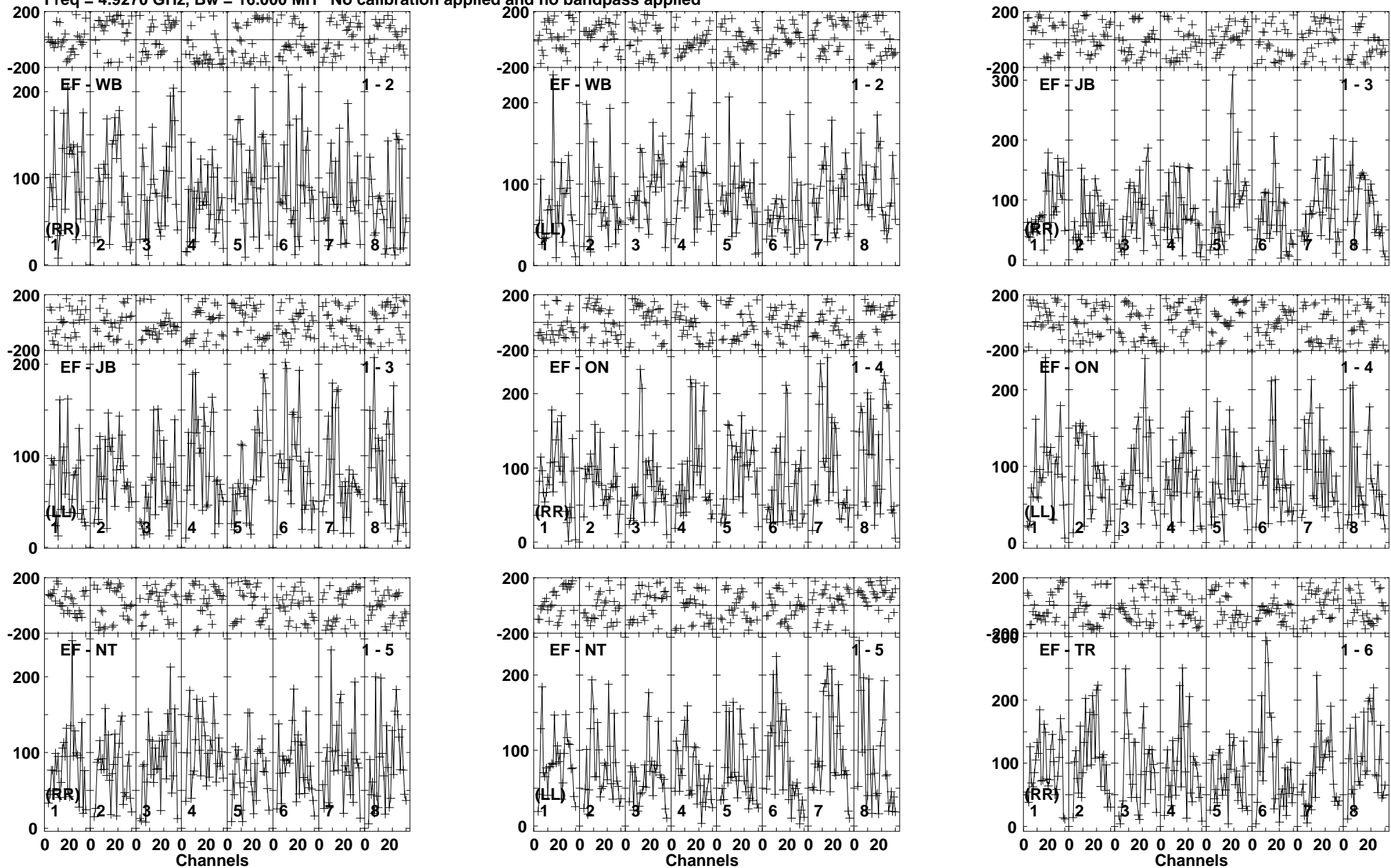
Lower frame: Micro Ampl Jy Top frame: Phas deg Vector averaged cross-power spectrum Baseline: EF (01) - WB (02) Timerange: 01/01:11:04 to 01/01:14:28
