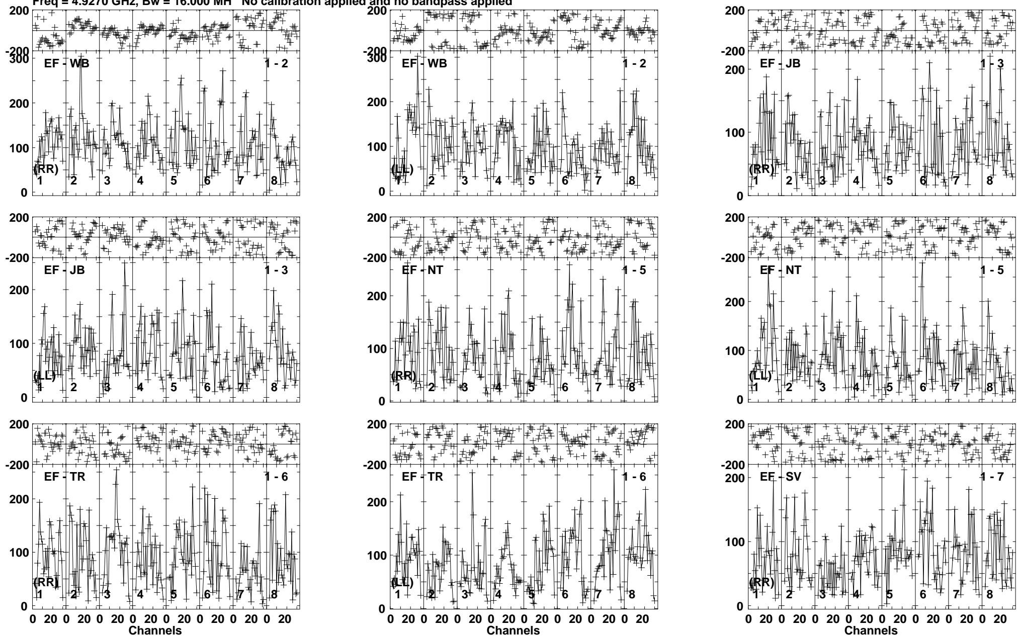
Lower frame: Micro Ampl Jy Top frame: Phas deg Vector averaged cross-power spectrum Baseline: EF (01) - WB (02) Timerange: 01/05:00:04 to 01/05:03:28
