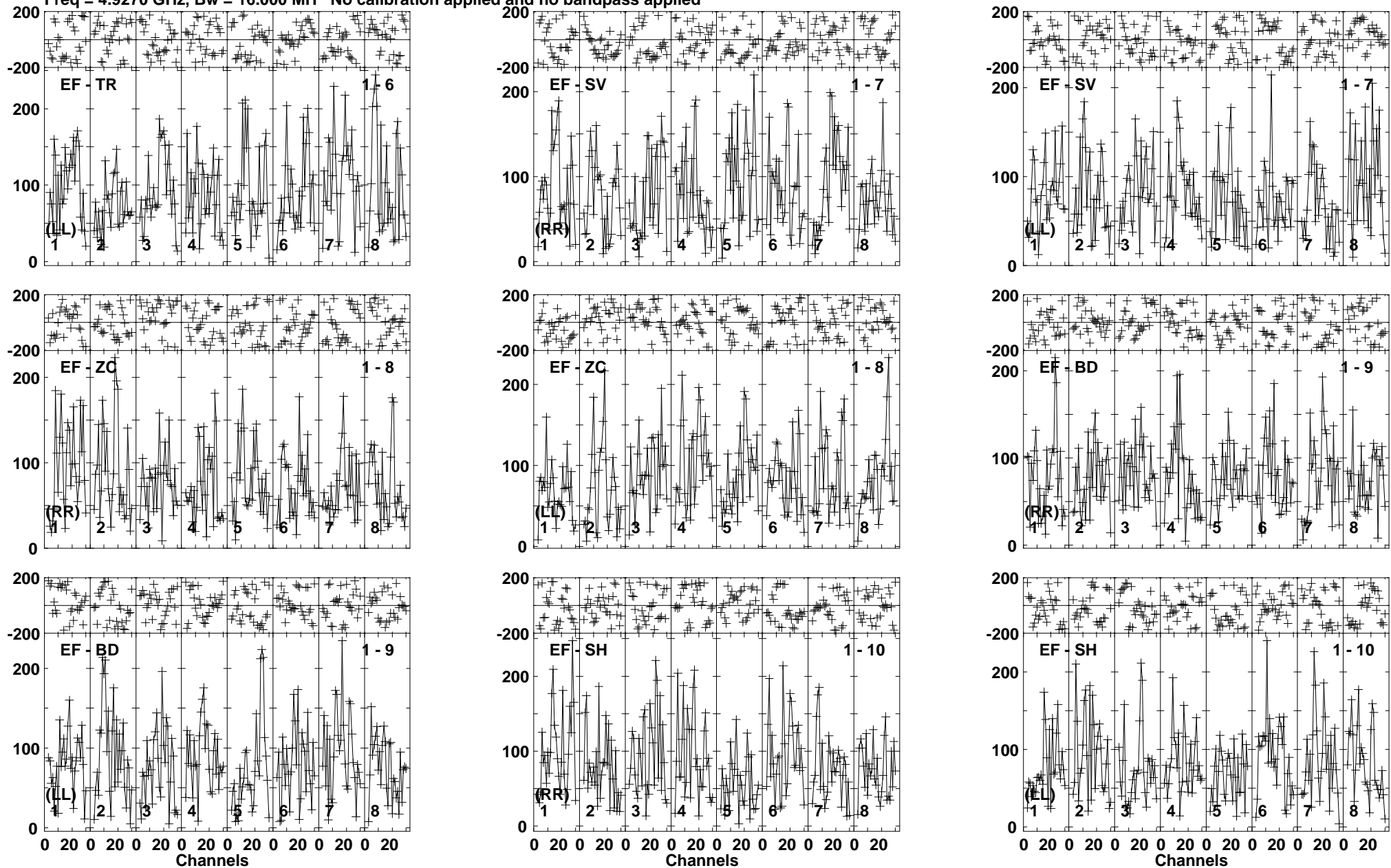
Lower frame: Micro Ampl Jy Top frame: Phas deg Vector averaged cross-power spectrum Baseline: EF (01) - TR (06) Timerange: 01/01:11:04 to 01/01:14:28
