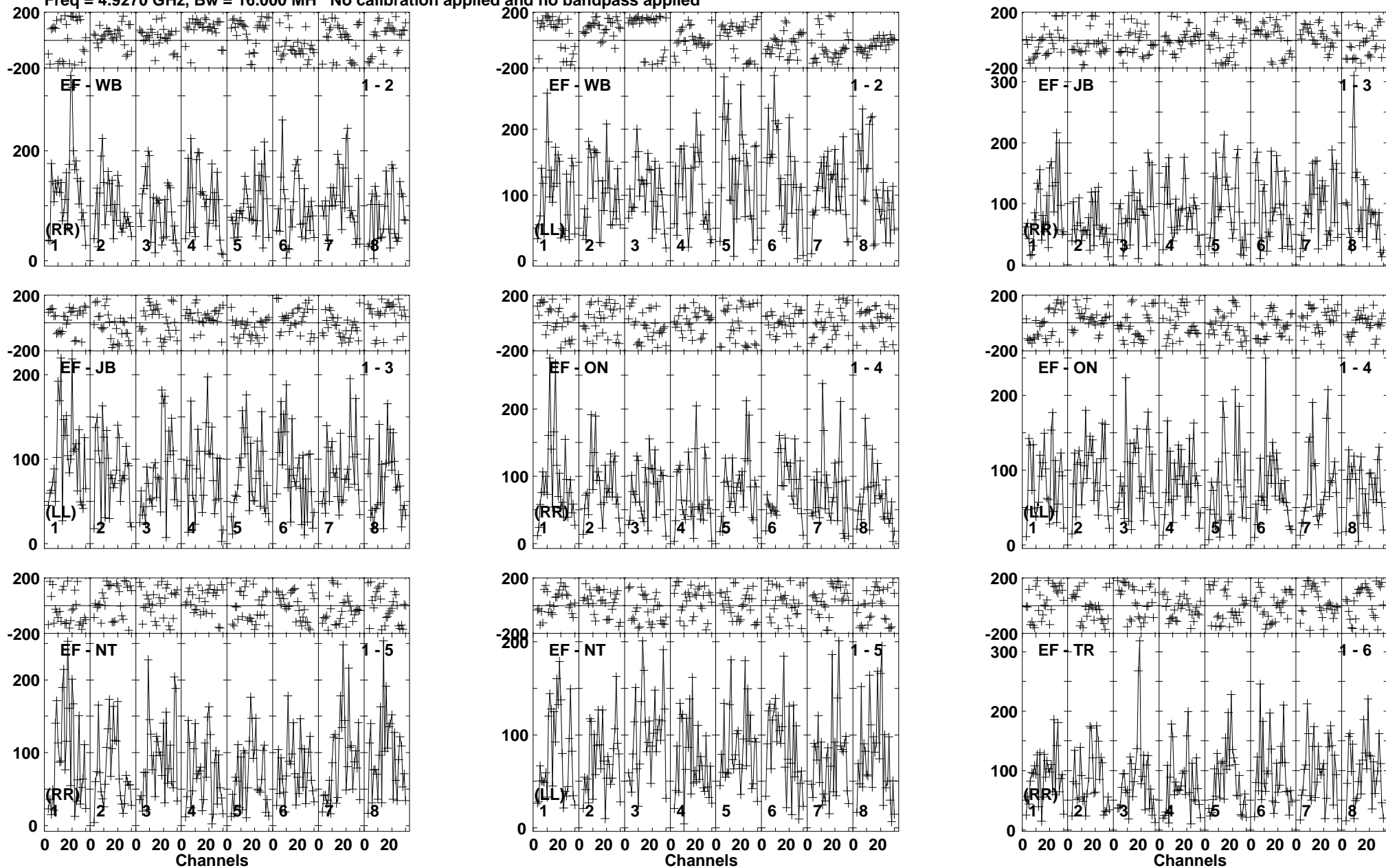
Lower frame: Micro Ampl Jy Top frame: Phas deg Vector averaged cross-power spectrum Baseline: EF (01) - WB (02) Timerange: 00/22:57:04 to 00/23:00:28
