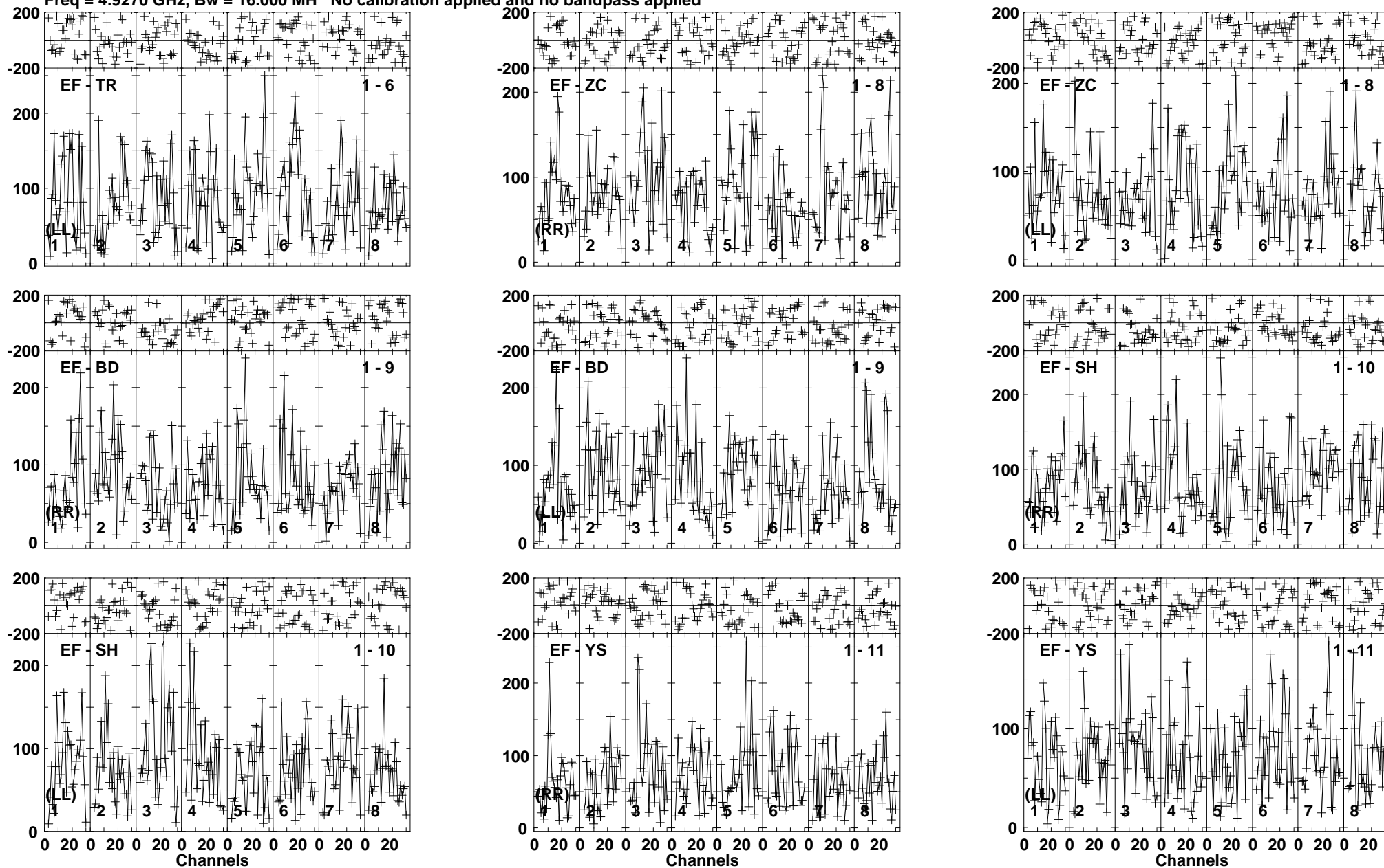
Lower frame: Micro Ampl Jy Top frame: Phas deg Vector averaged cross-power spectrum Baseline: EF (01) - TR (06) Timerange: 00/23:18:04 to 00/23:21:28
