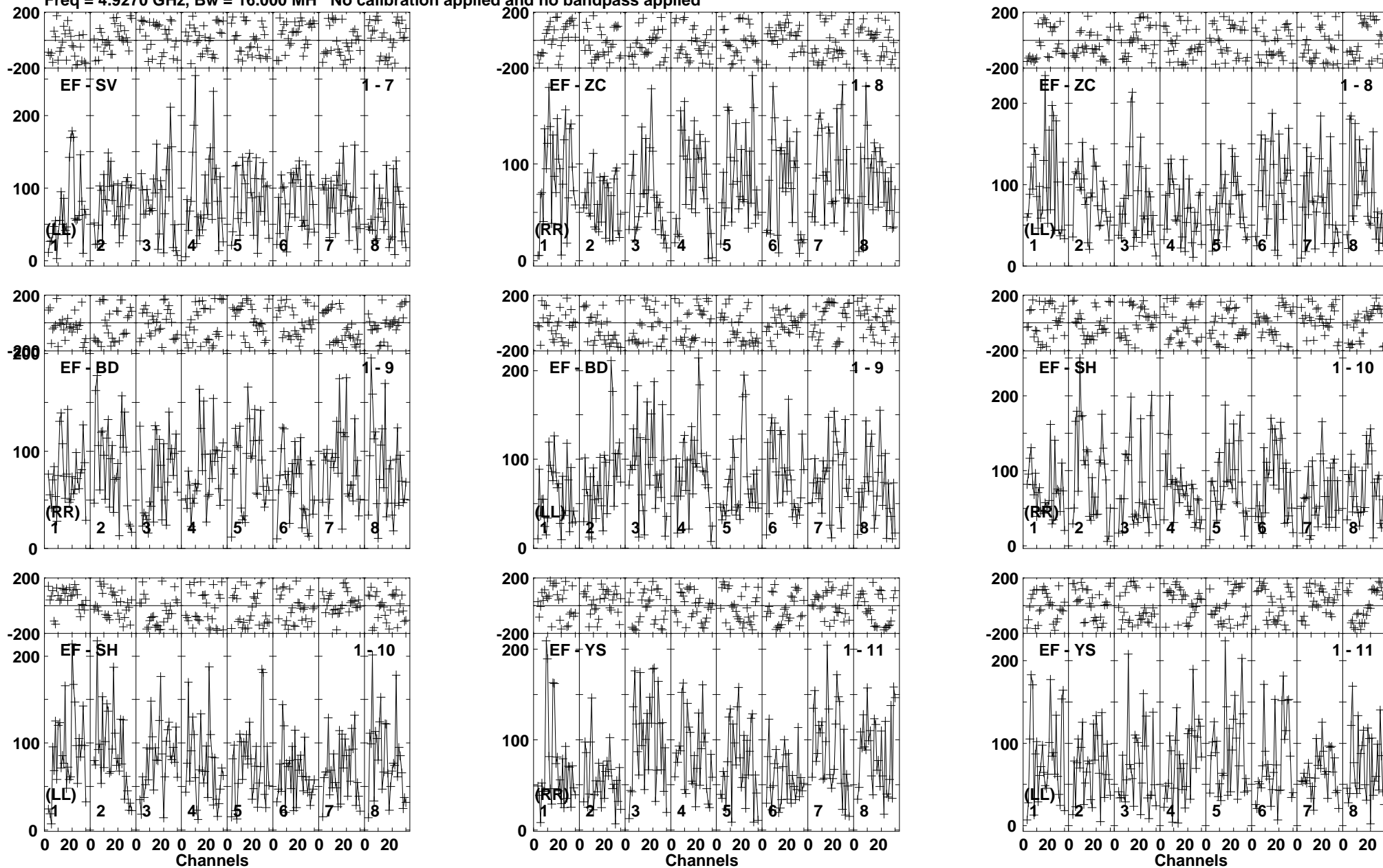
Lower frame: Micro Ampl Jy Top frame: Phas deg Vector averaged cross-power spectrum Baseline: EF (01) - SV (07) Timerange: 01/03:15:04 to 01/03:18:28
