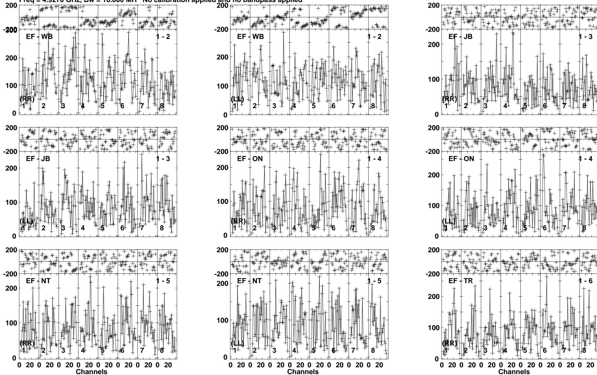
Lower frame: Micro Ampl Jy Top frame: Phas deg Vector averaged cross-power spectrum Baseline: EF (01) - WB (02) Timerange: 00:22:31:04 to 00:22:34:28
