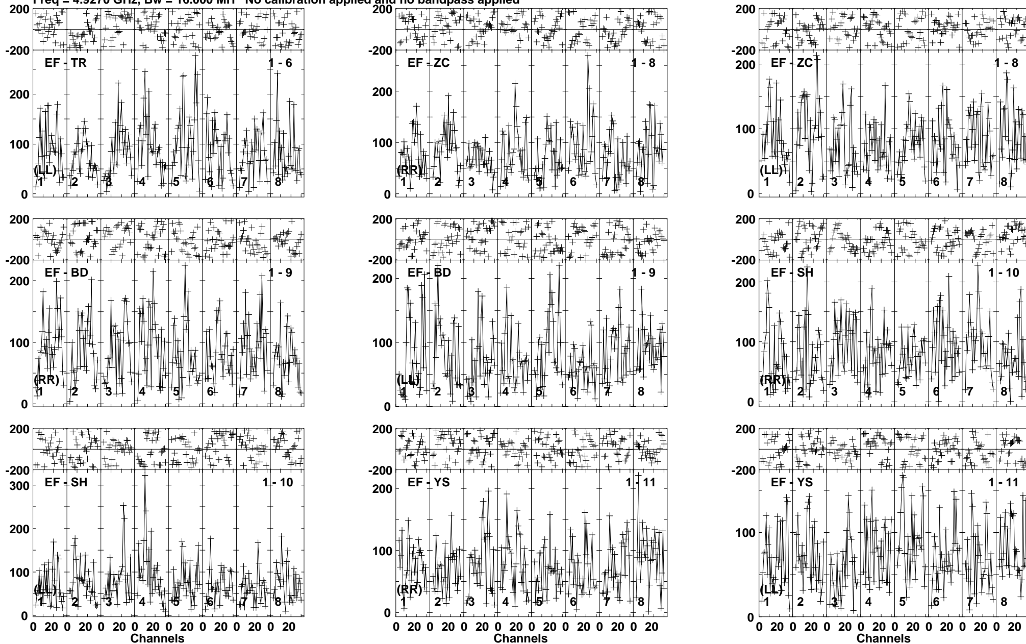
Lower frame: Micro Ampl Jy Top frame: Phas deg Vector averaged cross-power spectrum Baseline: EF (01) - TR (06) Timerange: 00/22:25:34 to 00/22:28:58
