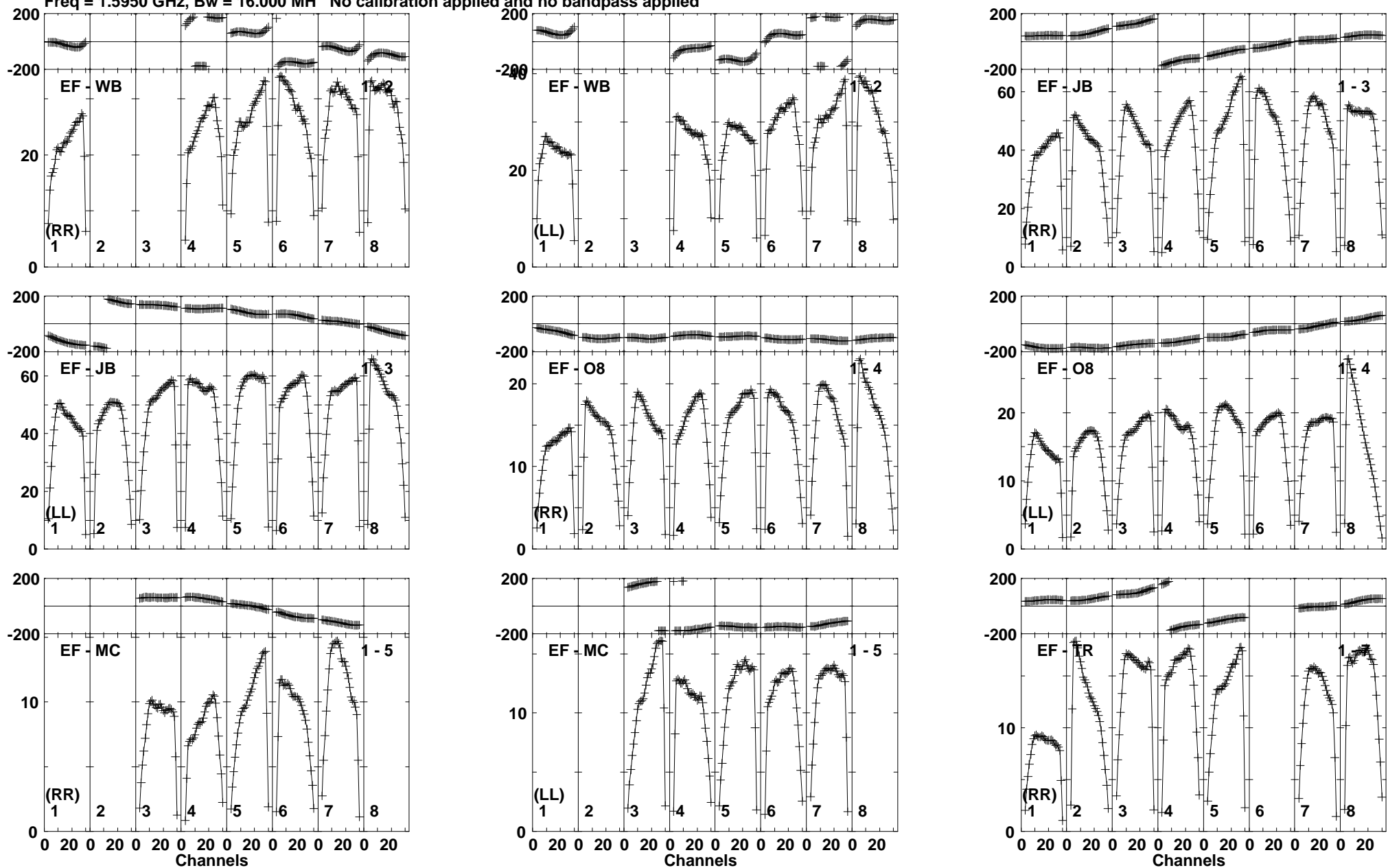
Lower frame: Milli Ampl Jy Top frame: Phas deg Vector averaged cross-power spectrum Baseline: EF (01) - WB (02) Timerange: 00/18:54:33 to 00/18:57:29
