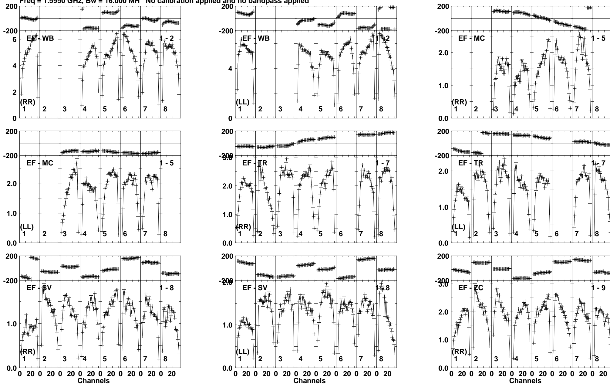
Lower frame: Milli Ampl Jy Top frame: Phas deg Vector averaged cross-power spectrum Baseline: EF (01) - WB (02) Timerange: 00/15:15:13 to 00/15:16:29
