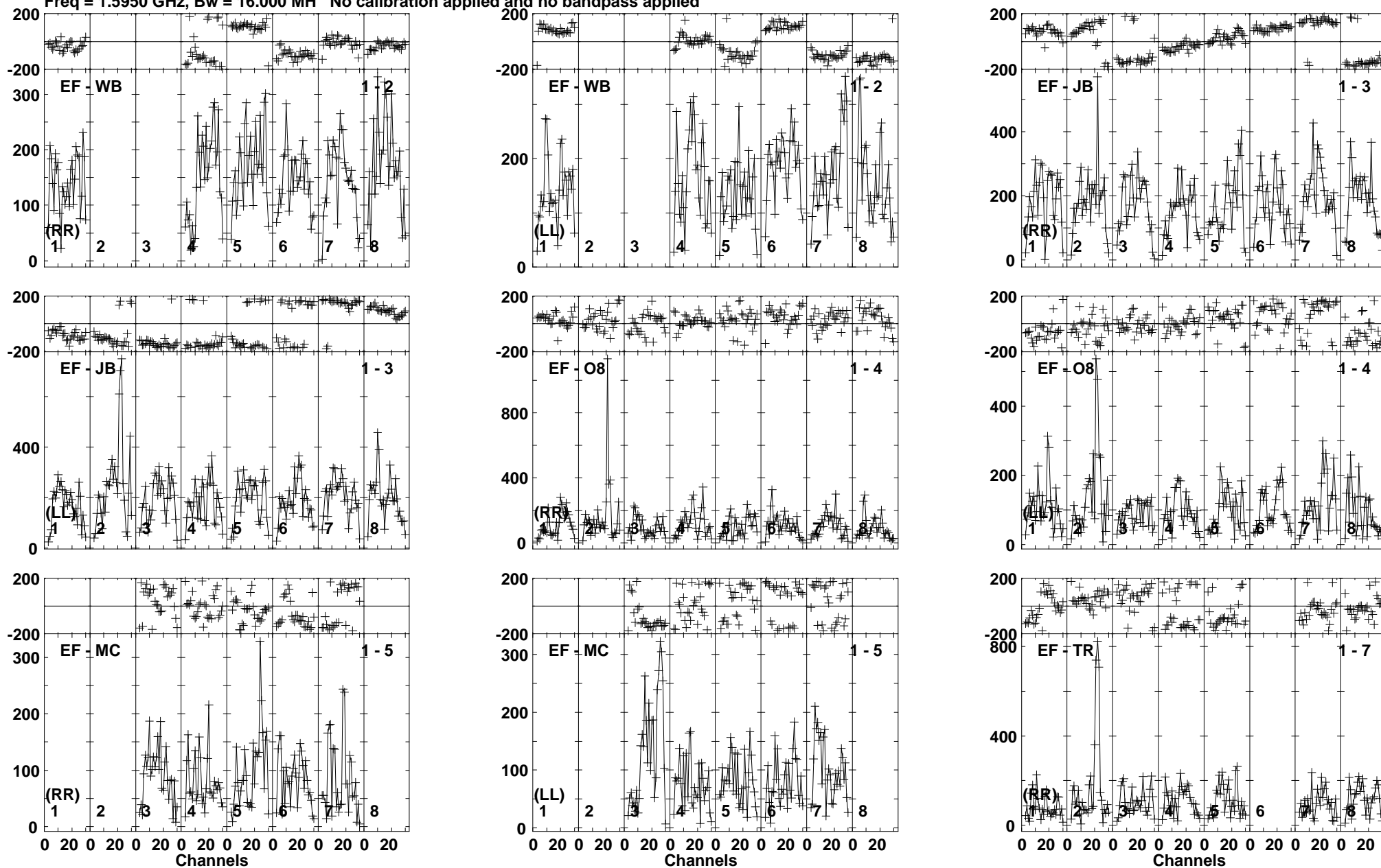
Lower frame: Micro Ampl Jy Top frame: Phas deg Vector averaged cross-power spectrum Baseline: EF (01) - WB (02) Timerange: 00/16:33:36 to 00/16:36:58
