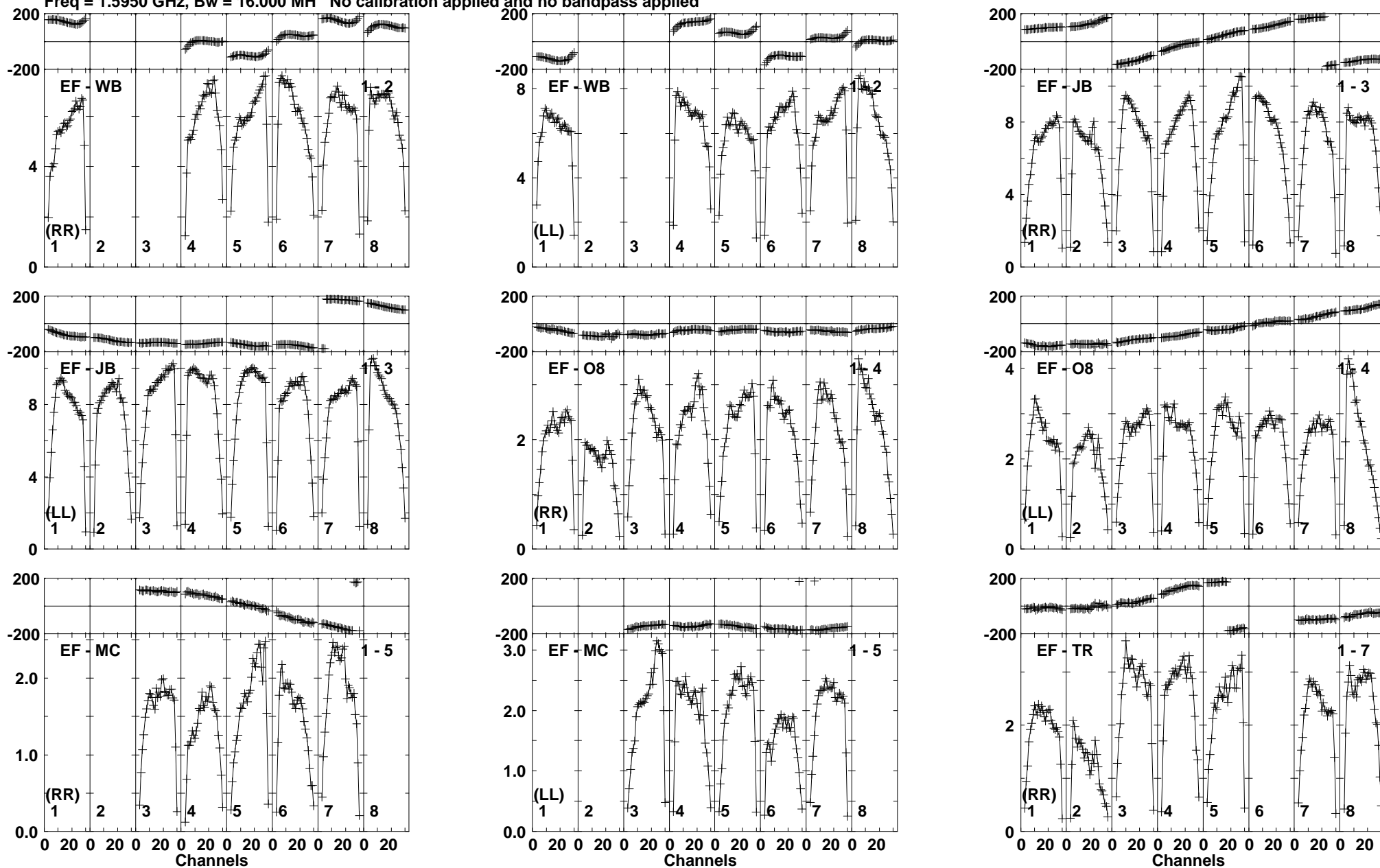
Lower frame: Milli Ampl Jy Top frame: Phas deg Vector averaged cross-power spectrum Baseline: EF (01) - WB (02) Timerange: 00/16:00:36 to 00/16:01:58
