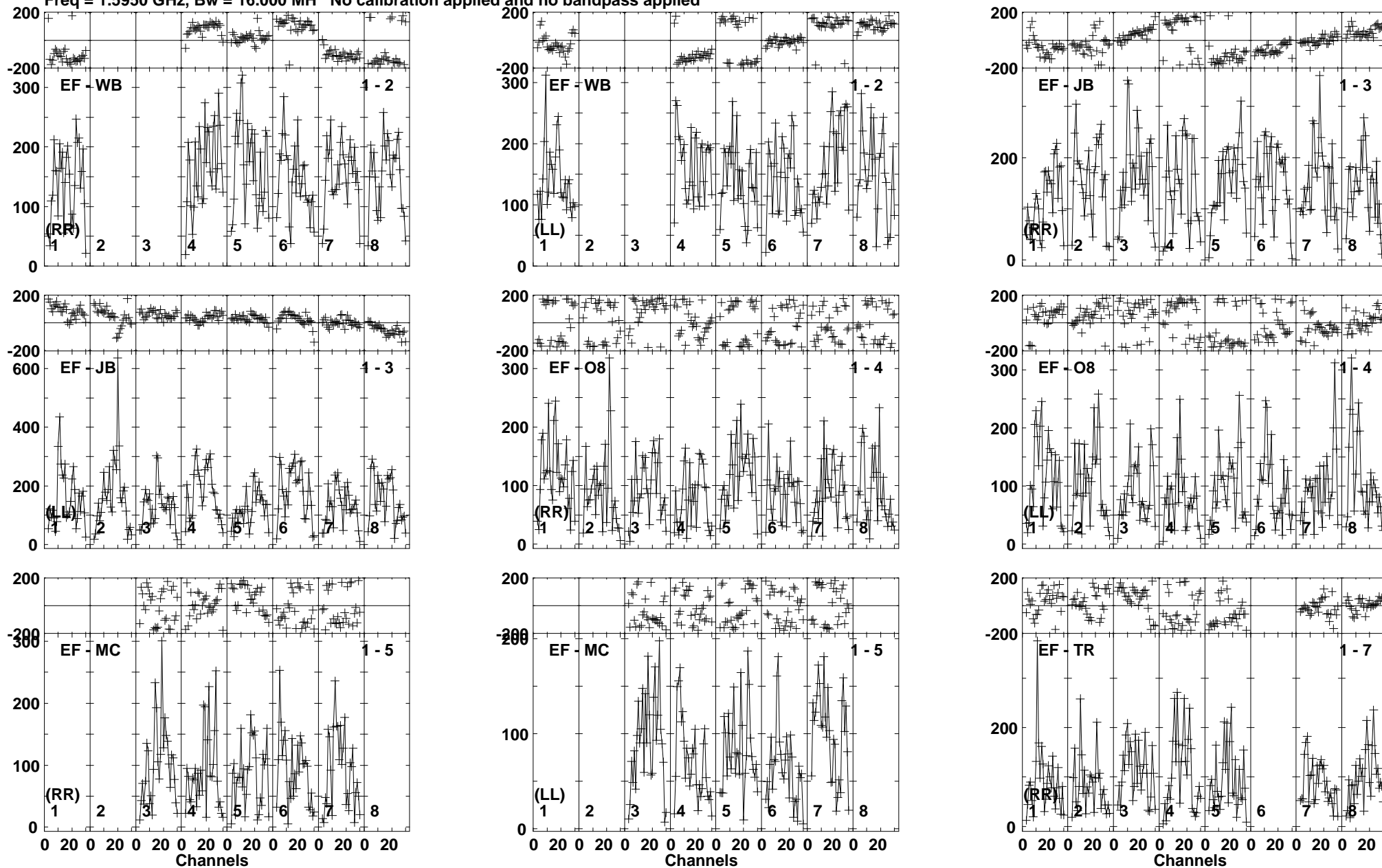
Lower frame: Micro Ampl Jy Top frame: Phas deg Vector averaged cross-power spectrum Baseline: EF (01) - WB (02) Timerange: 00/16:02:06 to 00/16:05:28
