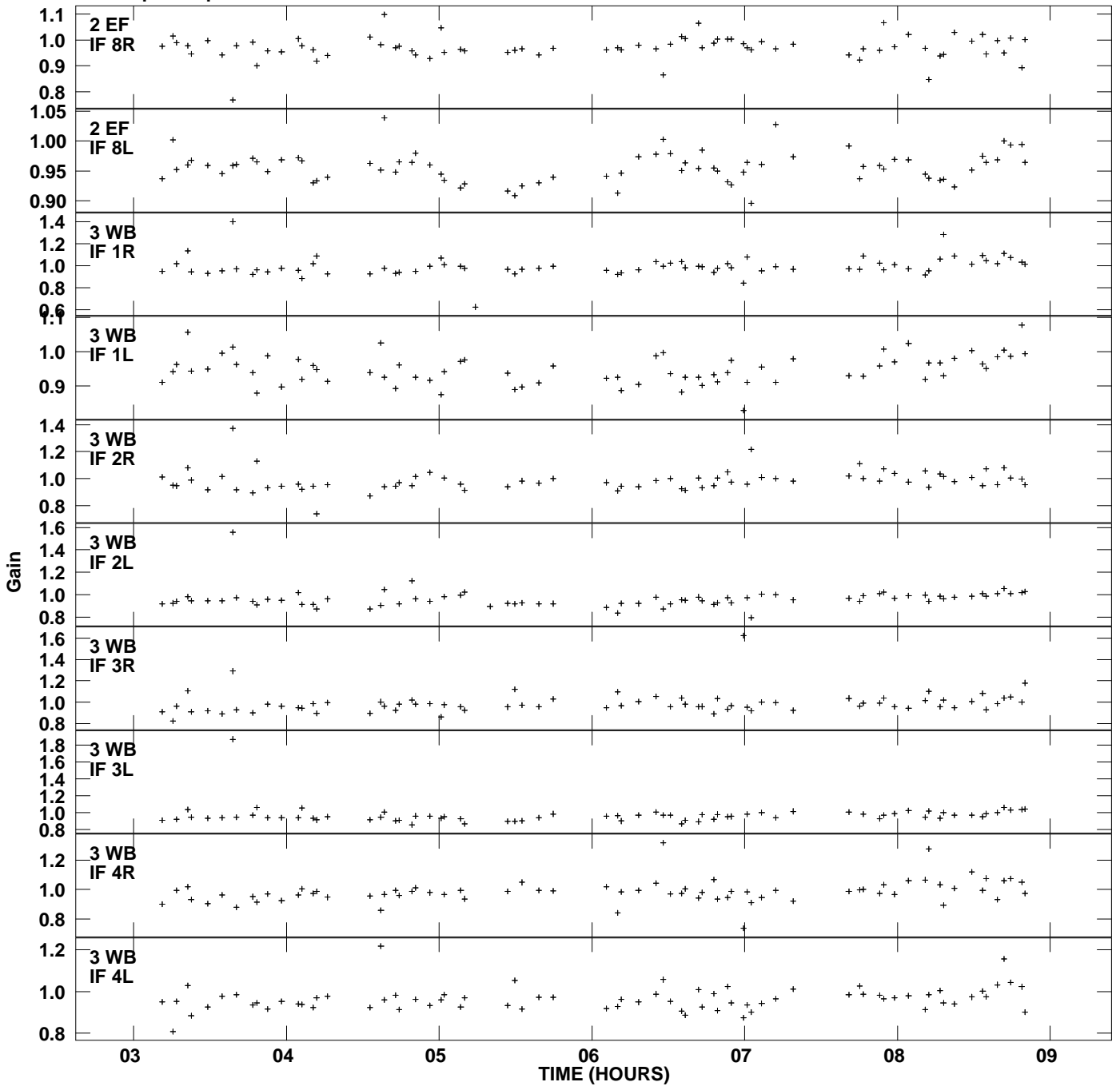
Plot file version 4 created 11-JUL-2007 03:58:20 Gain amp vs UTC time for J1825-0737.MULTI.1 SN 2 Rpol & Lpol IF 1 - 8
