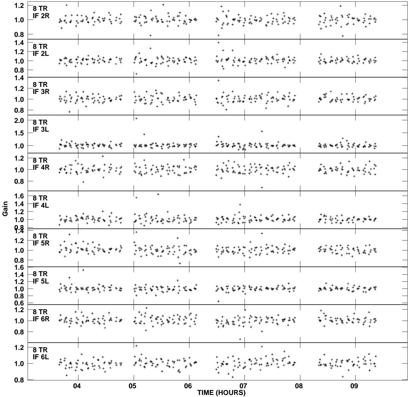
Plot file version 12 created 17-JUN-2009 01:29:07 Gain amp vs UTC time for J1834-0301.MULTI.1 SN 6 Rpol & Lpol IF 1 - 8
