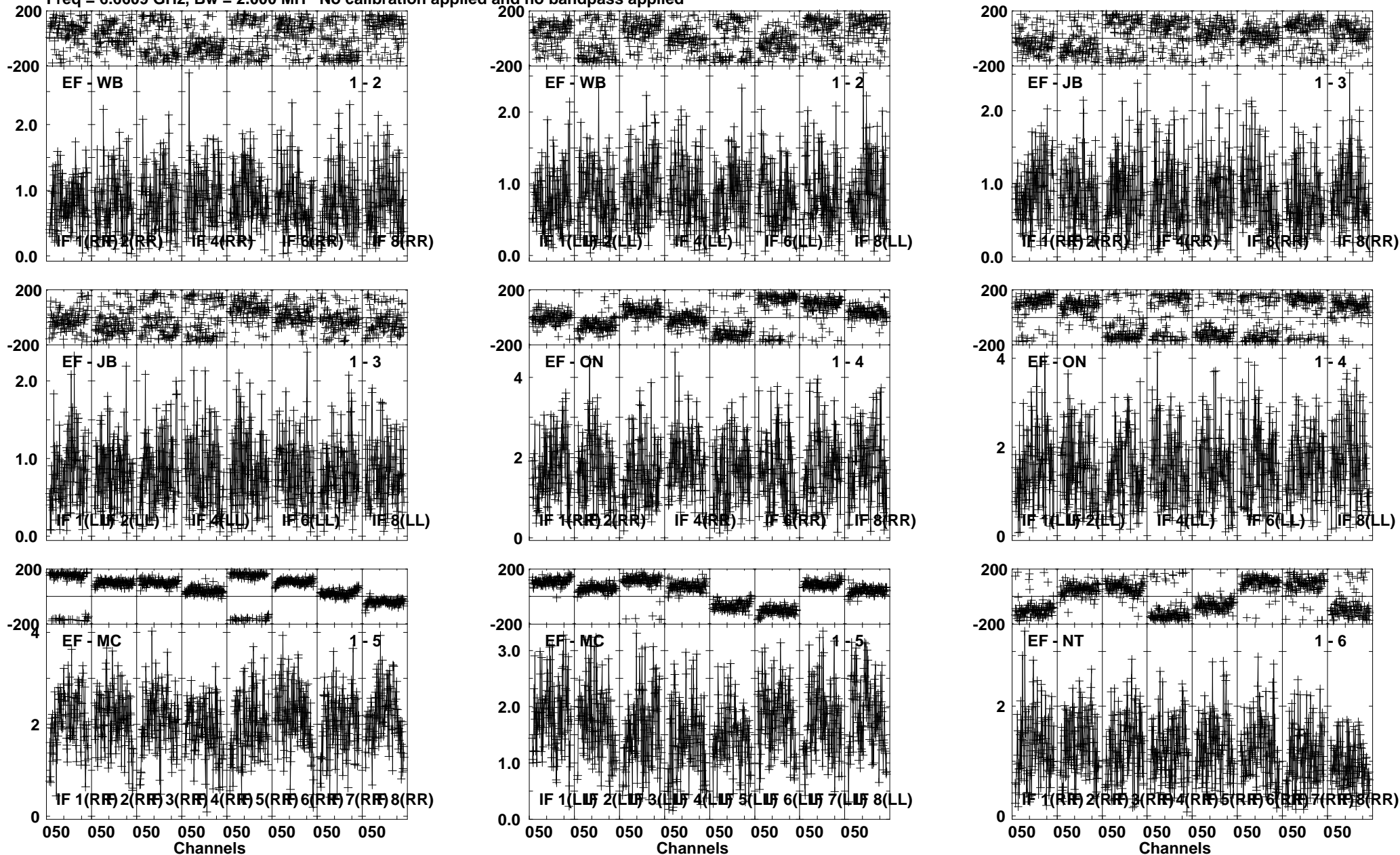
Lower frame: Milli Ampl Jy Top frame: Phas deg Vector averaged cross-power spectrum Several baselines displayed Timerange: 00/13:06:07 to 00/13:08:15
