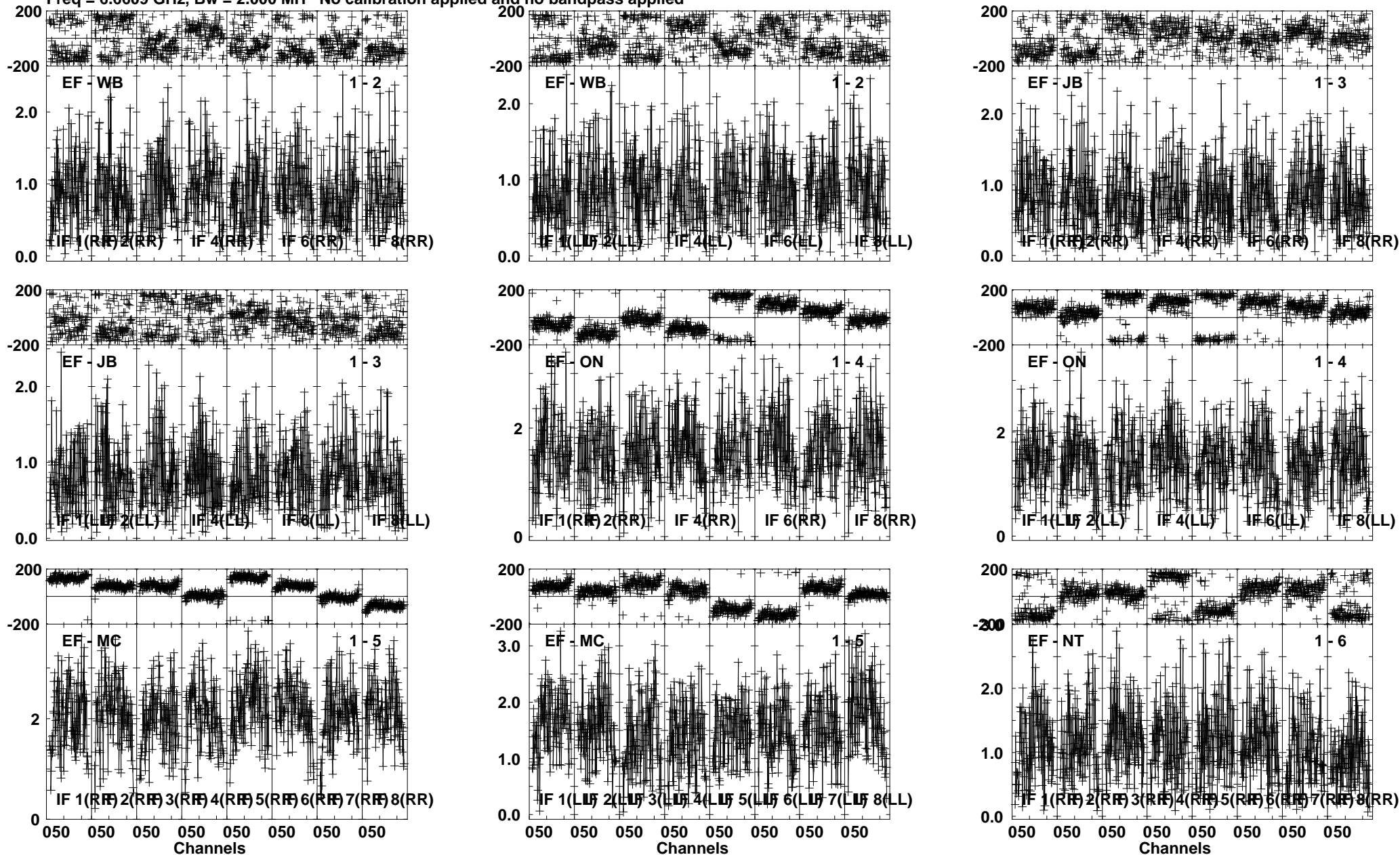
Lower frame: Milli Amp Jy Top frame: Phas deg Vector averaged cross-power spectrum Several baselines displayed Timerange: 00/13:02:06 to 00/13:04:15
