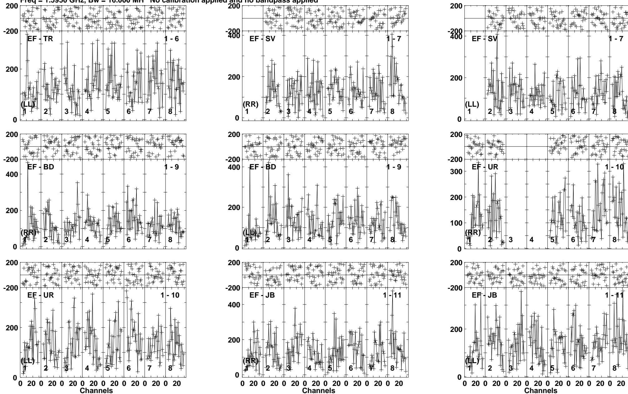
Lower frame: Micro Ampl Jy Top frame: Phas deg Vector averaged cross-power spectrum Baseline: EF (01) - TR (06) Timerange: 00/07:58:53 to 00/08:02:29
