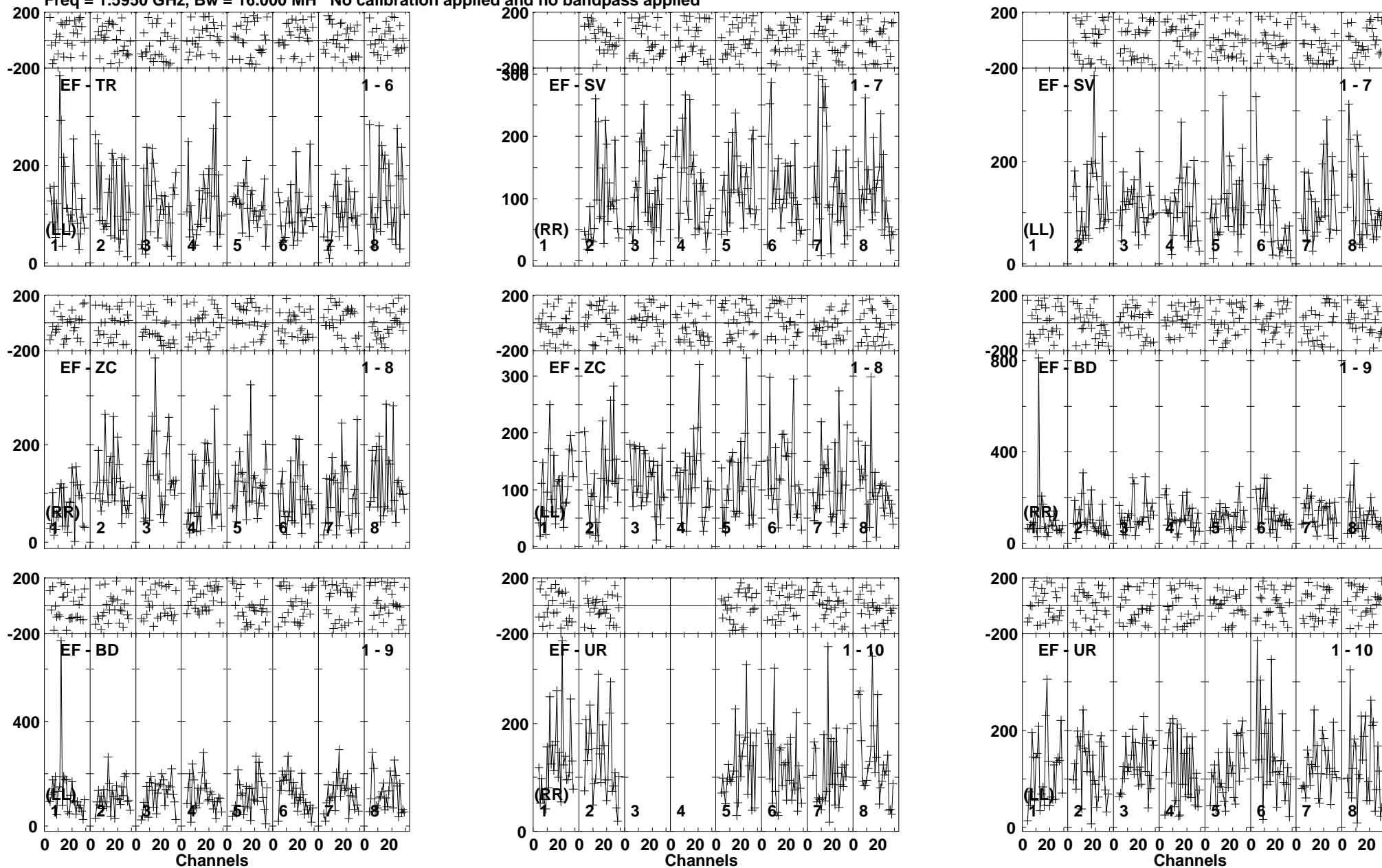
Lower frame: Micro Ampl Jy Top frame: Phas deg Vector averaged cross-power spectrum Baseline: EF (01) - TR (06) Timerange: 00/10:02:24 to 00/10:06:08
