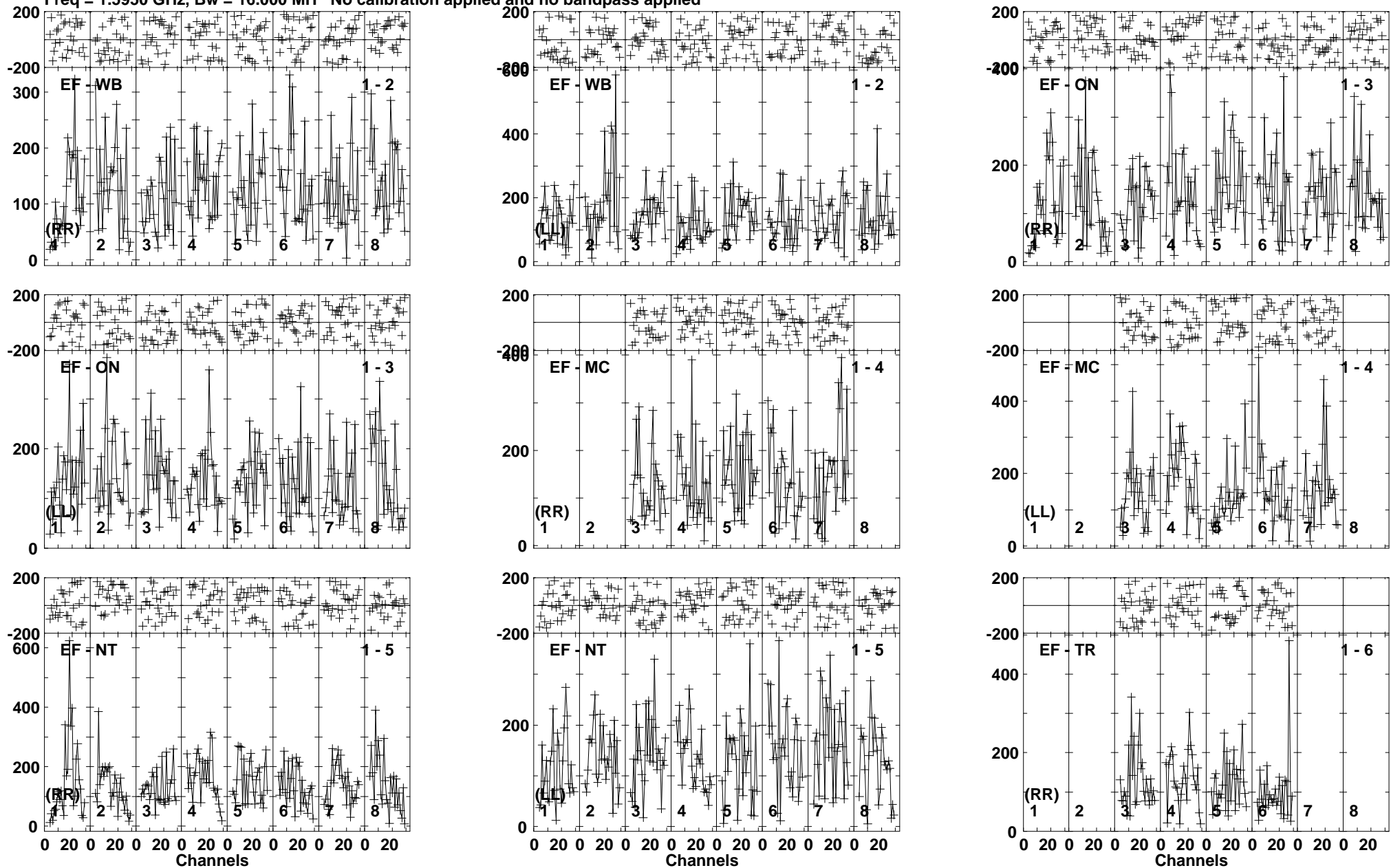
Lower frame: Micro Ampl Jy Top frame: Phas deg Vector averaged cross-power spectrum Baseline: EF (01) - WB (02) Timerange: 00/07:58:53 to 00/08:02:29
