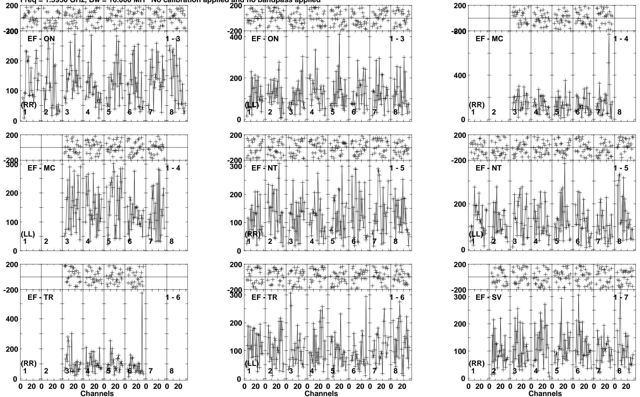
Lower frame: Micro Ampl Jy Top frame: Phas deg Vector averaged cross-power spectrum Baseline: EF (01) - ON (03) Timerange: 00/02:46:01 to 00/02:49:49
