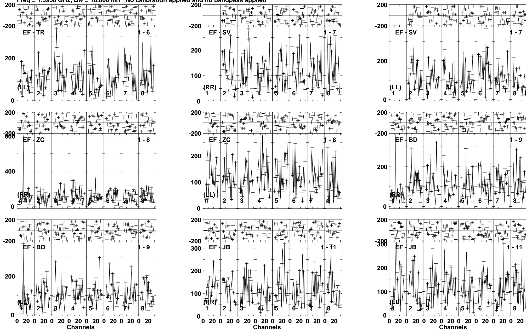
Lower frame: Micro Ampl Jy Top frame: Phas deg Vector averaged cross-power spectrum Baseline: EF (01) - TR (06) Timerange: 00/05:28:03 to 00/05:31:49
