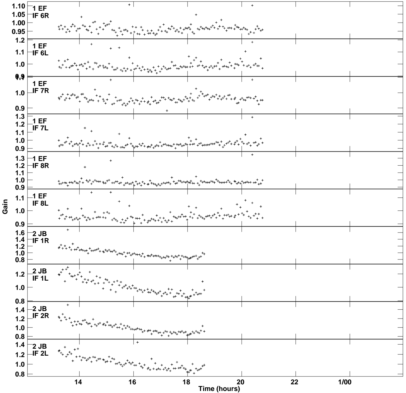
Plot file version 2 created 20-NOV-2015 11:15:16 Gain amp vs UTC time for J2136+4301.MULTI.1 SN 2 Rpol & Lpol IF 1 - 8
