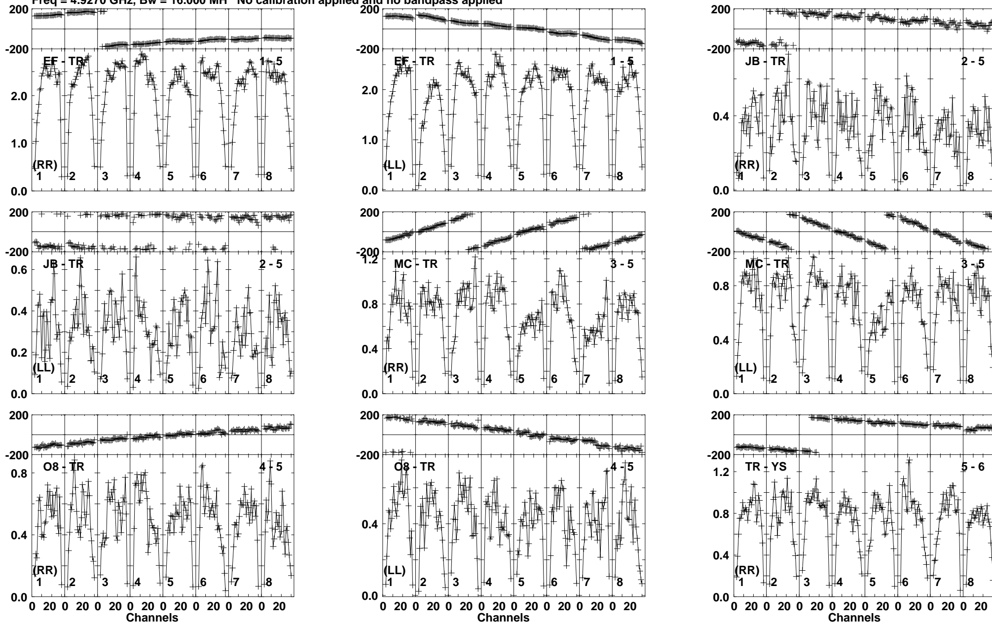
Lower frame: Milli Ampl Jy Top frame: Phas deg Vector averaged cross-power spectrum Baseline: EF (01) - TR (05) Timerange: 00/18:18:01 to 00/18:19:29
