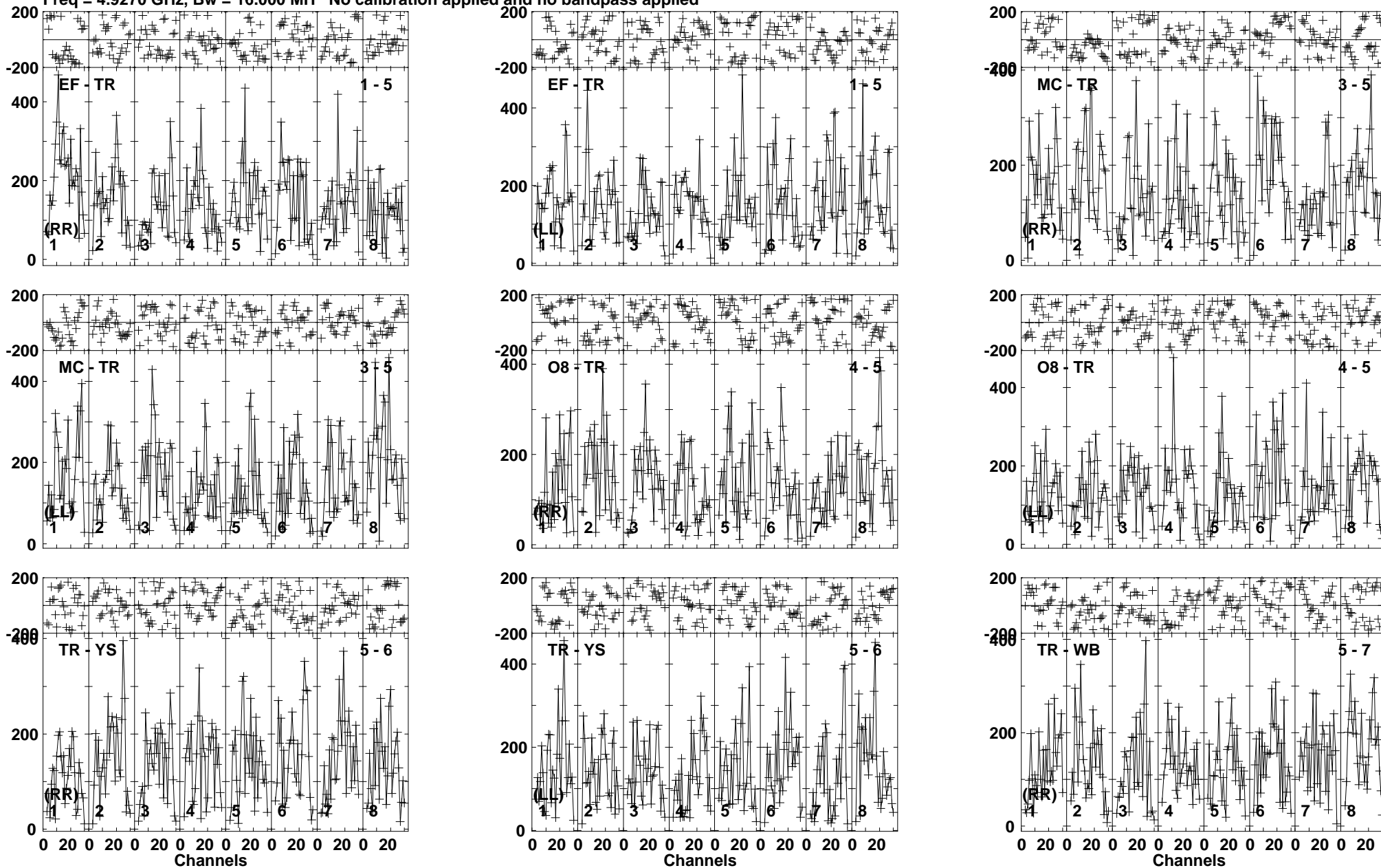
Lower frame: Micro Ampl Jy Top frame: Phas deg Vector averaged cross-power spectrum Baseline: EF (01) - TR (05) Timerange: 00/19:53:42 to 00/19:55:38
