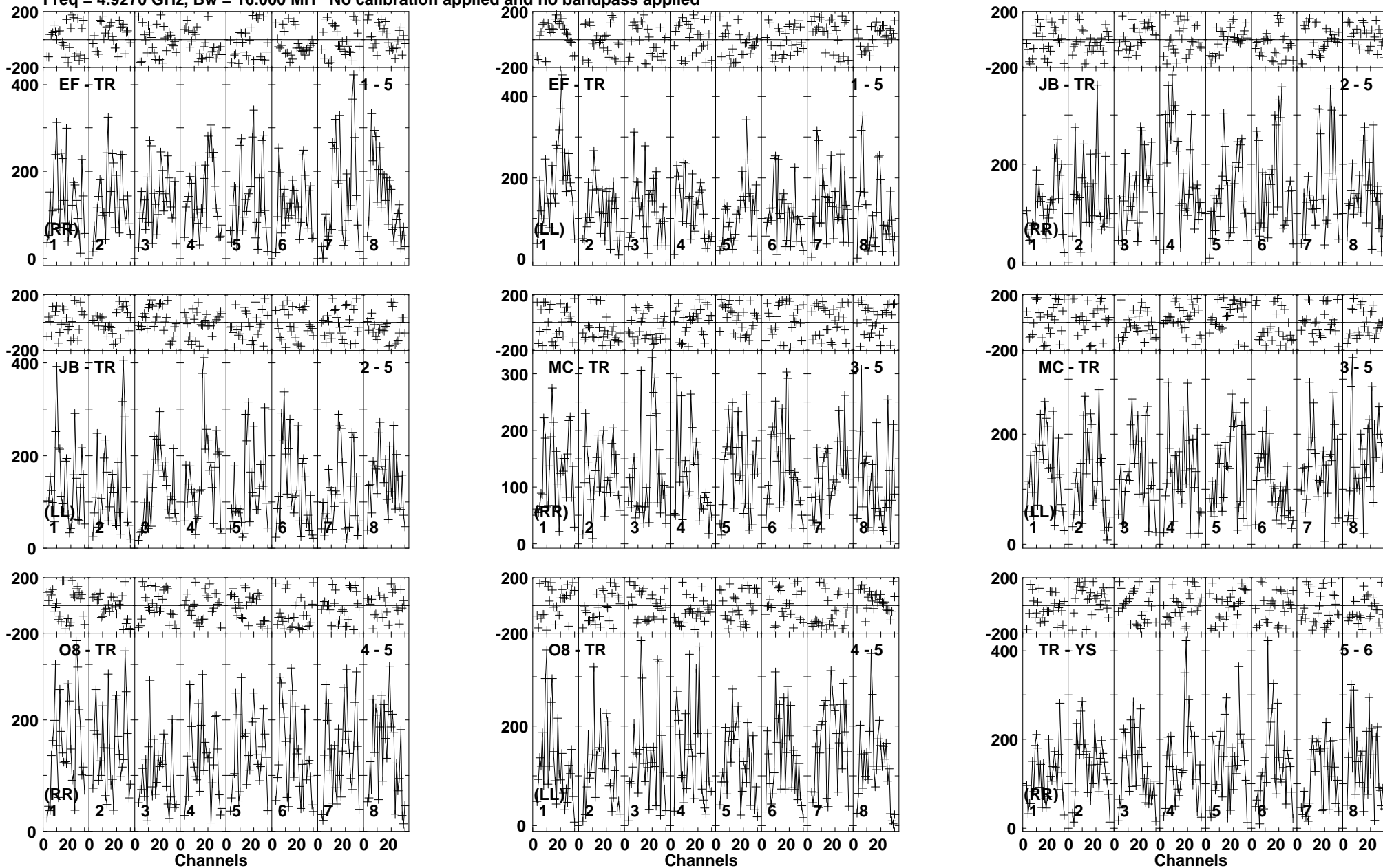
Lower frame: Micro Ampl Jy Top frame: Phas deg Vector averaged cross-power spectrum Baseline: EF (01) - TR (05) Timerange: 00/15:40:01 to 00/15:42:09
