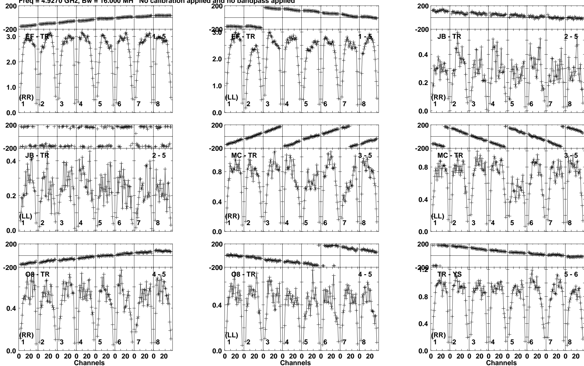
Lower frame: Milli Ampl Jy Top frame: Phas deg Vector averaged cross-power spectrum Baseline: EF (01) - TR (05) Timerange: 00/13:13:22 to 00/13:16:18
