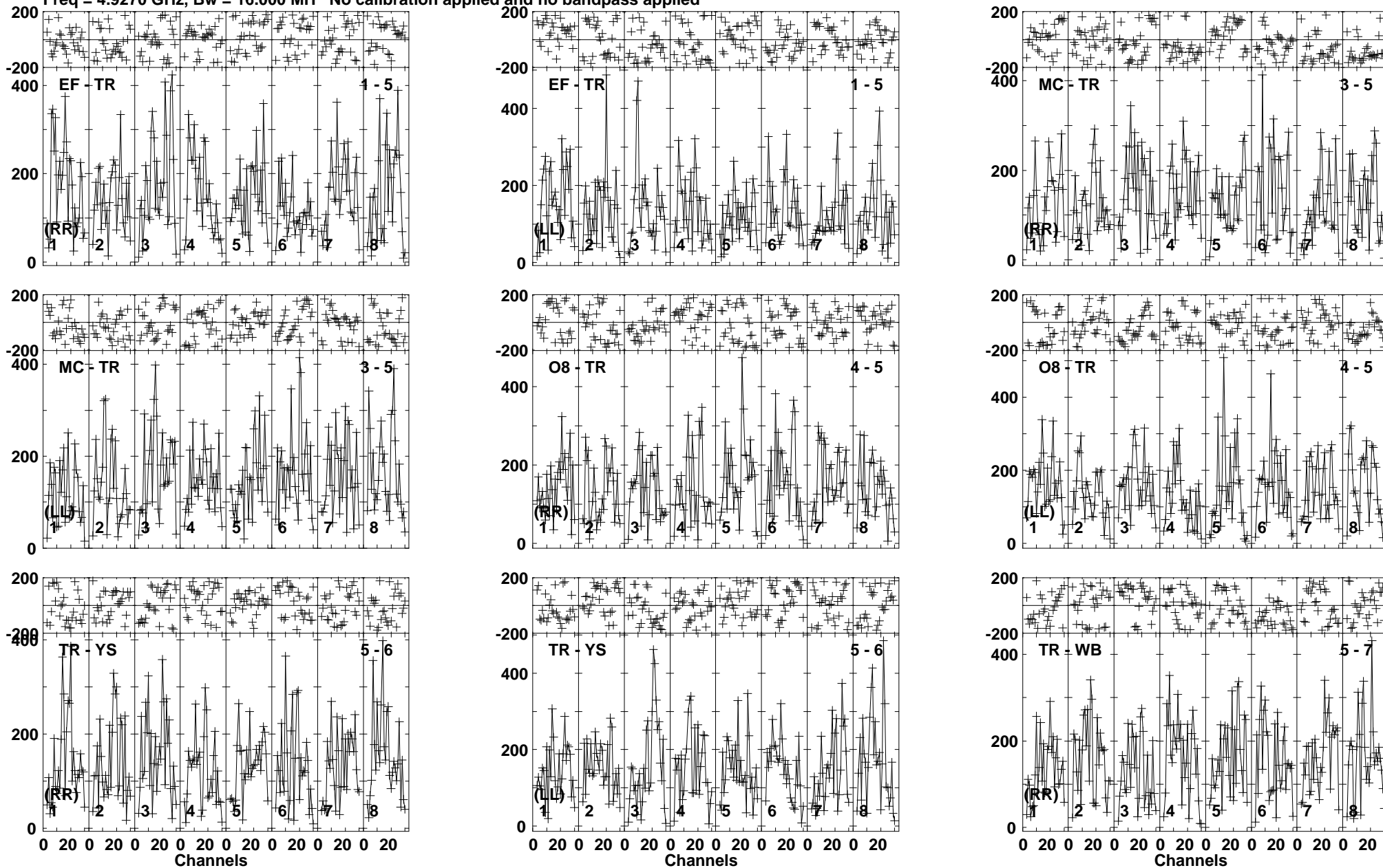
Lower frame: Micro Ampl Jy Top frame: Phas deg Vector averaged cross-power spectrum Baseline: EF (01) - TR (05) Timerange: 00/18:37:31 to 00/18:39:29
