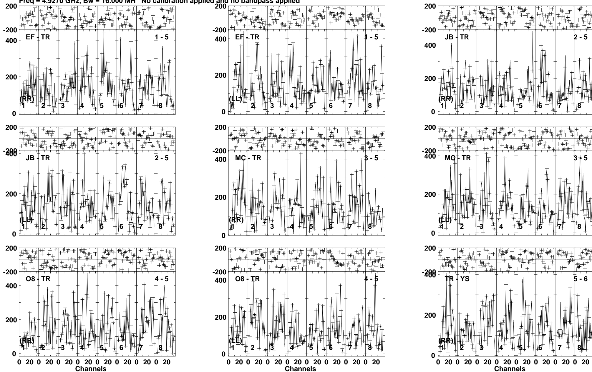
Lower frame: Micro Ampl Jy Top frame: Phas deg Vector averaged cross-power spectrum Baseline: EF (01) - TR (05) Timerange: 00/13:23:22 to 00/13:25:18
