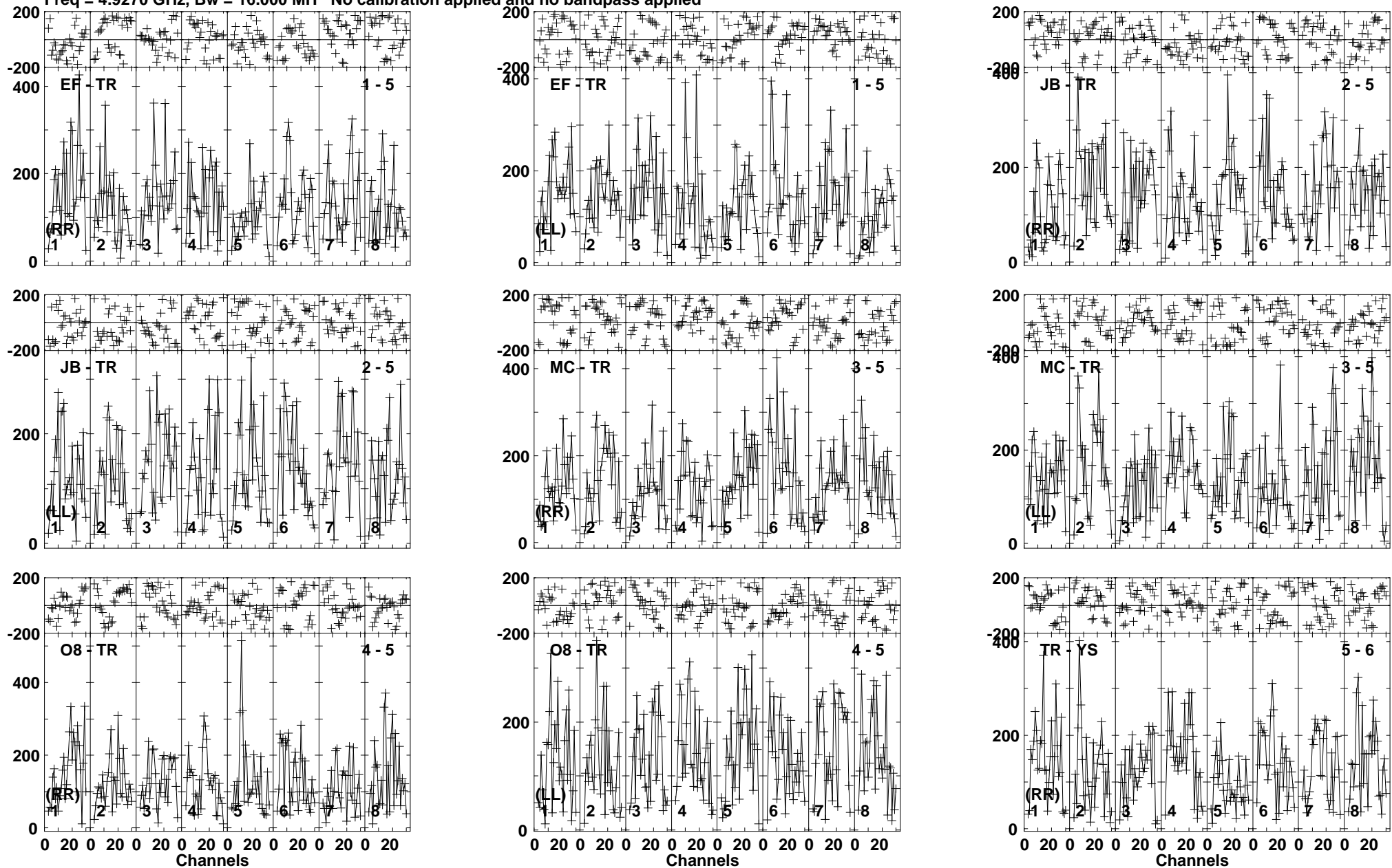
Lower frame: Micro Ampl Jy Top frame: Phas deg Vector averaged cross-power spectrum Baseline: EF (01) - TR (05) Timerange: 00/16:02:31 to 00/16:04:39
