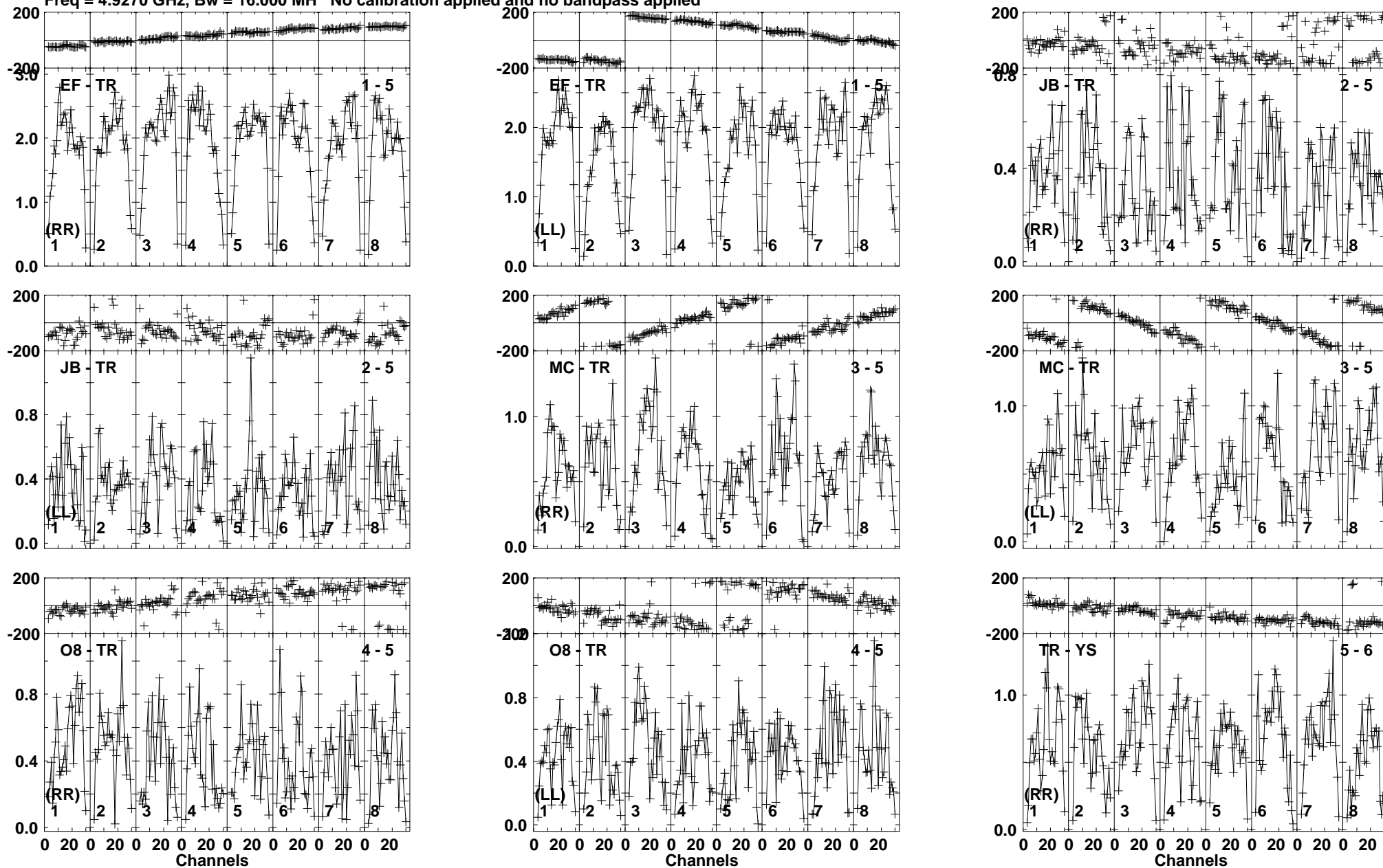
Lower frame: Milli Ampl Jy Top frame: Phas deg Vector averaged cross-power spectrum Baseline: EF (01) - TR (05) Timerange: 00/16:39:21 to 00/16:40:39
