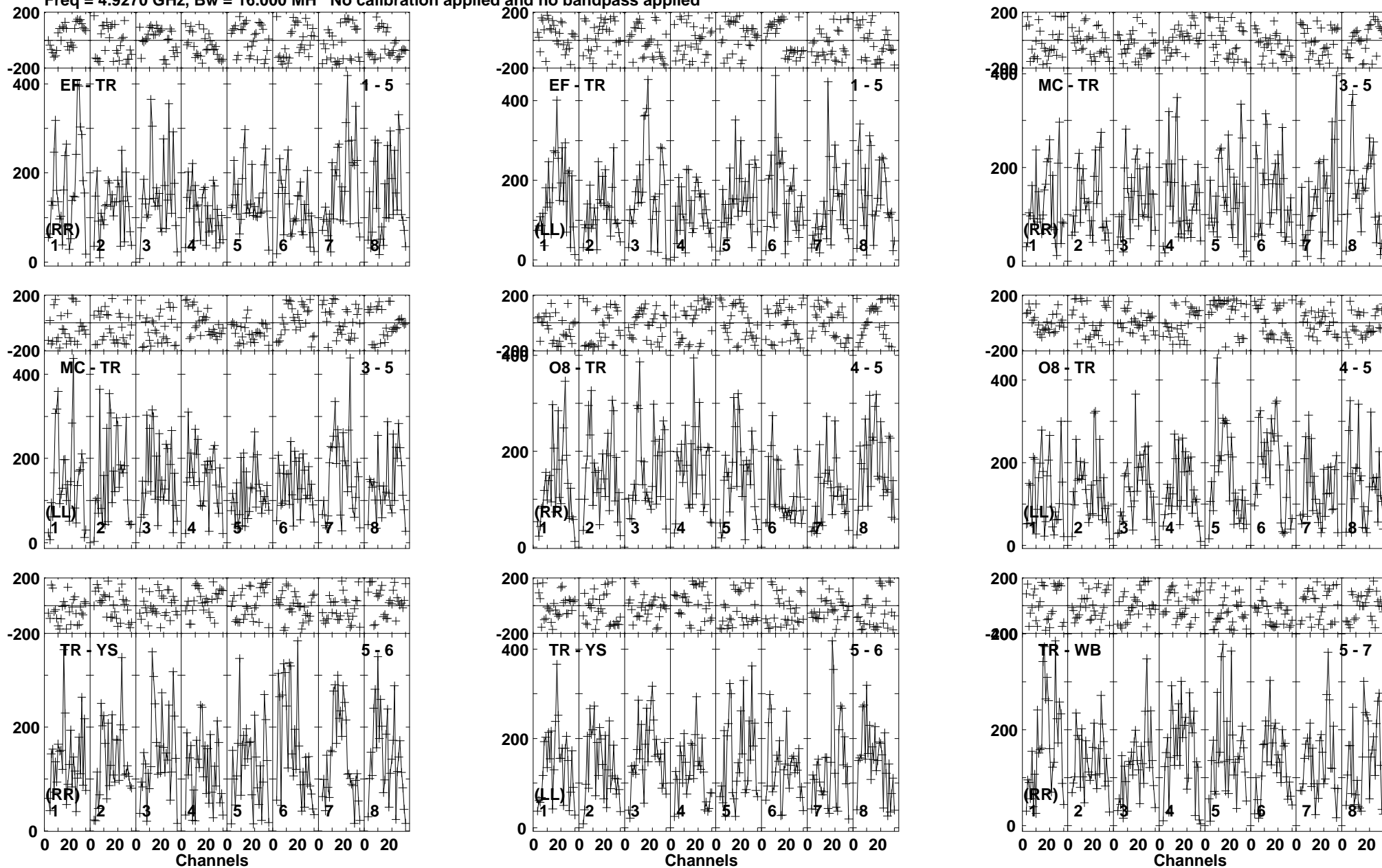
Lower frame: Micro Ampl Jy Top frame: Phas deg Vector averaged cross-power spectrum Baseline: EF (01) - TR (05) Timerange: 00/19:58:12 to 00/20:00:12
