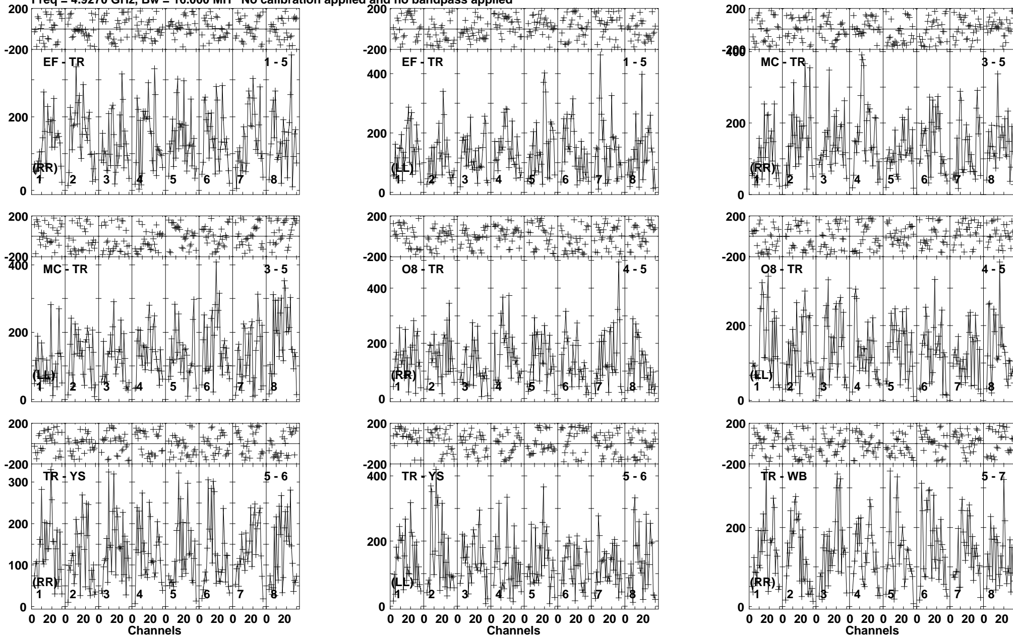
Lower frame: Micro Ampl Jy Top frame: Phas deg Vector averaged cross-power spectrum Baseline: EF (01) - TR (05) Timerange: 00/19:15:31 to 00/19:17:39
