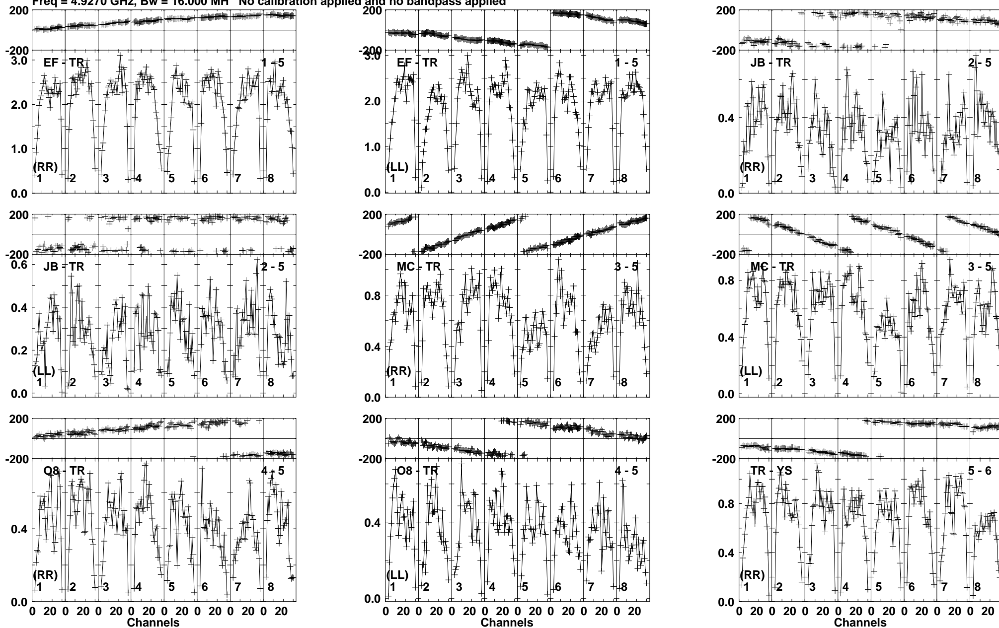
Lower frame: Milli Ampl Jy Top frame: Phas deg Vector averaged cross-power spectrum Baseline: EF (01) - TR (05) Timerange: 00/17:39:41 to 00/17:41:09
