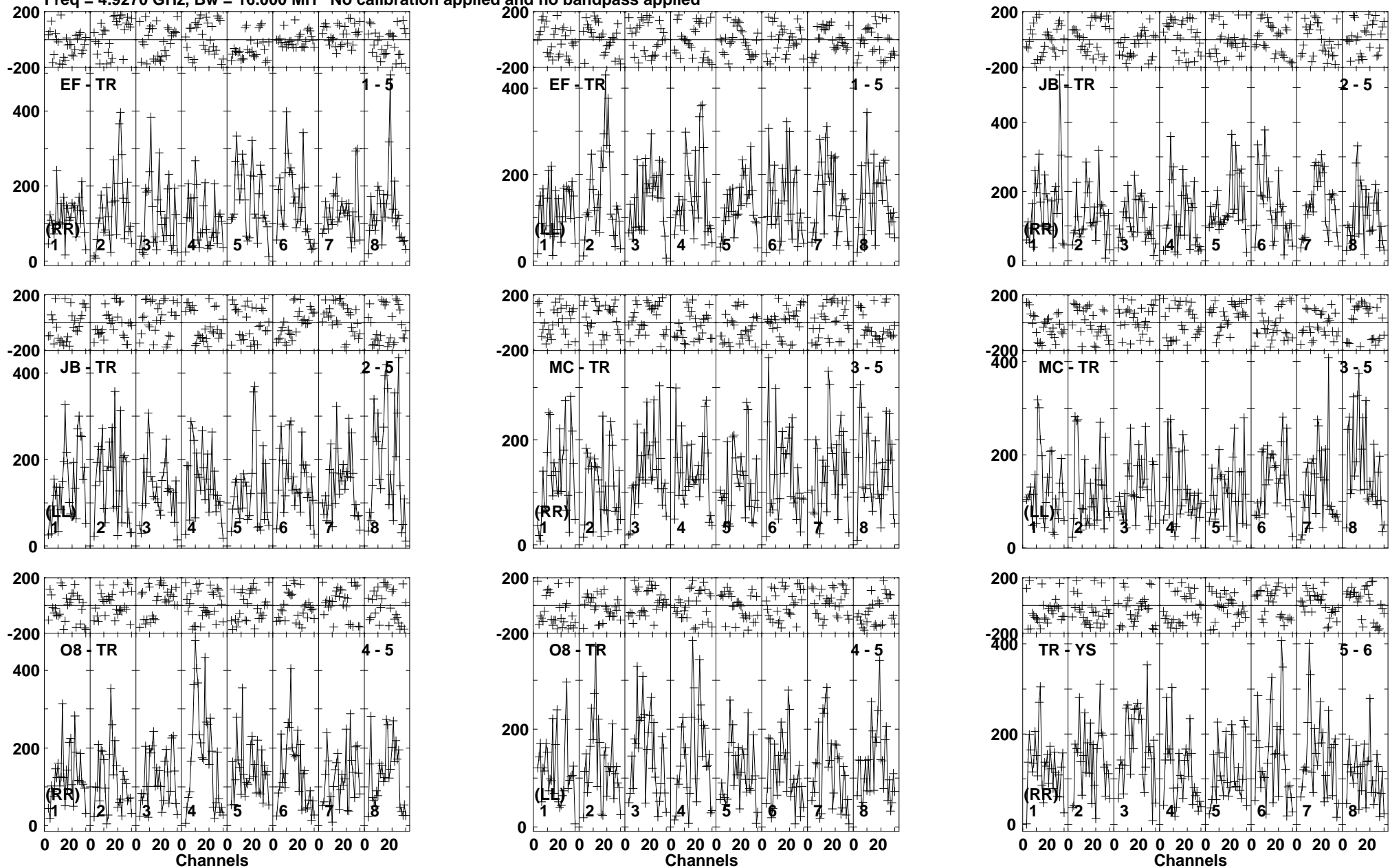
Lower frame: Micro Ampl Jy Top frame: Phas deg Vector averaged cross-power spectrum Baseline: EF (01) - TR (05) Timerange: 00/14:35:21 to 00/14:37:29
