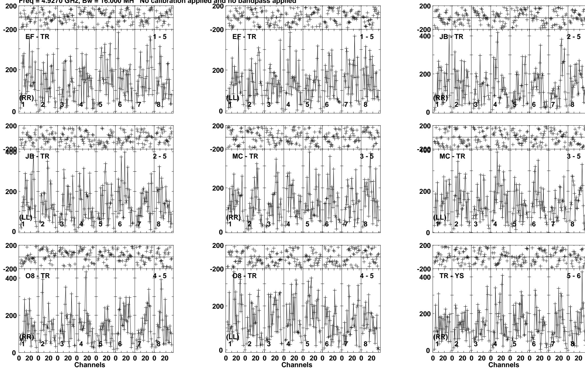
Lower frame: Micro Ampl Jy Top frame: Phas deg Vector averaged cross-power spectrum Baseline: EF (01) - TR (05) Timerange: 00:17:44:41 to 00:17:46:49
