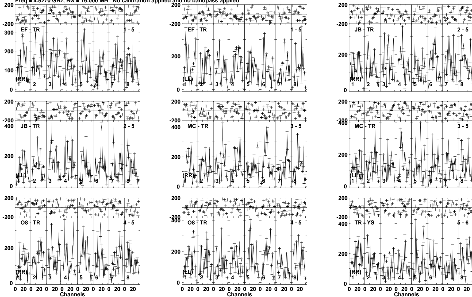
Lower frame: Micro Ampl Jy Top frame: Phas deg Vector averaged cross-power spectrum Baseline: EF (01) - TR (05) Timerange: 00/13:42:22 to 00/13:44:28
