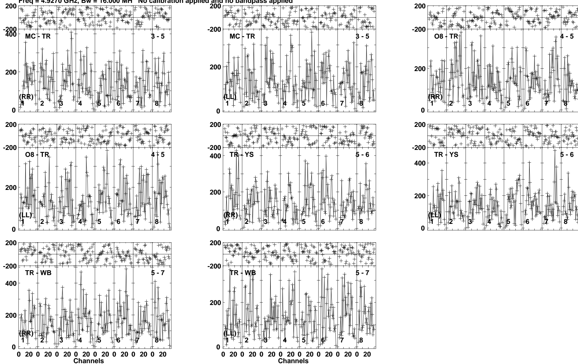
Lower frame: Micro Ampl Jy Top frame: Phas deg Vector averaged cross-power spectrum Baseline: MC (03) - TR (05) Timerange: 00/21:59:22 to 00/22:01:28
