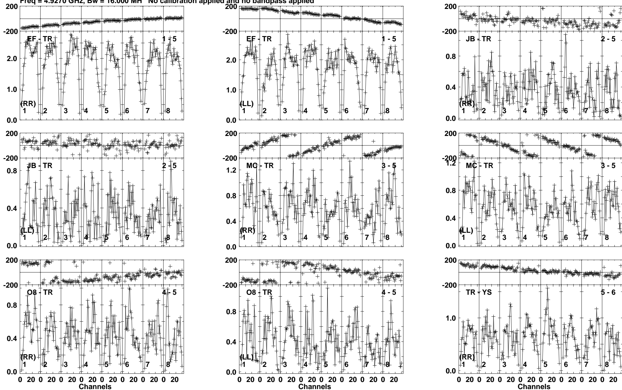
Lower frame: Milli Ampl Jy Top frame: Phas deg Vector averaged cross-power spectrum Baseline: EF (01) - TR (05) Timerange: 00:15:57:11 to 00:15:58:29
