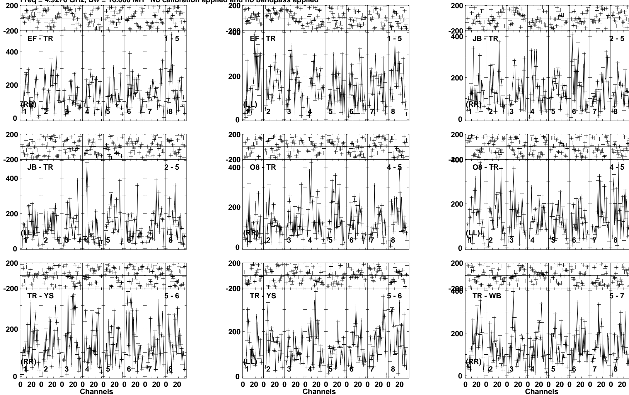
Lower frame: Micro Ampl Jy Top frame: Phas deg Vector averaged cross-power spectrum Baseline: EF (01) - TR (05) Timerange: 00/17:11:11 to 00/17:13:19
