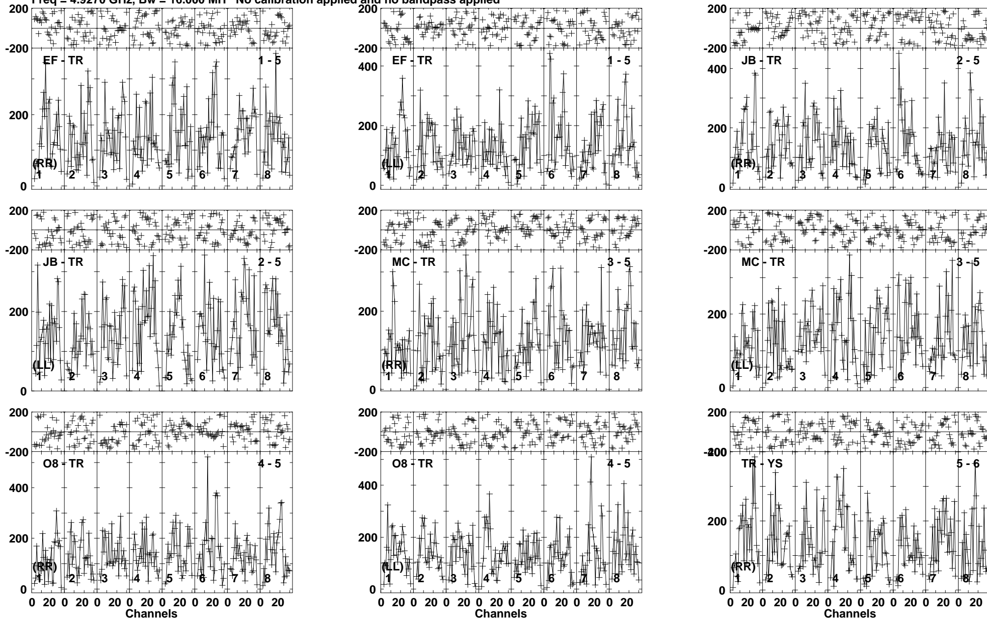
Lower frame: Micro Ampl Jy Top frame: Phas deg Vector averaged cross-power spectrum Baseline: EF (01) - TR (05) Timerange: 00/18:19:31 to 00/18:21:39
