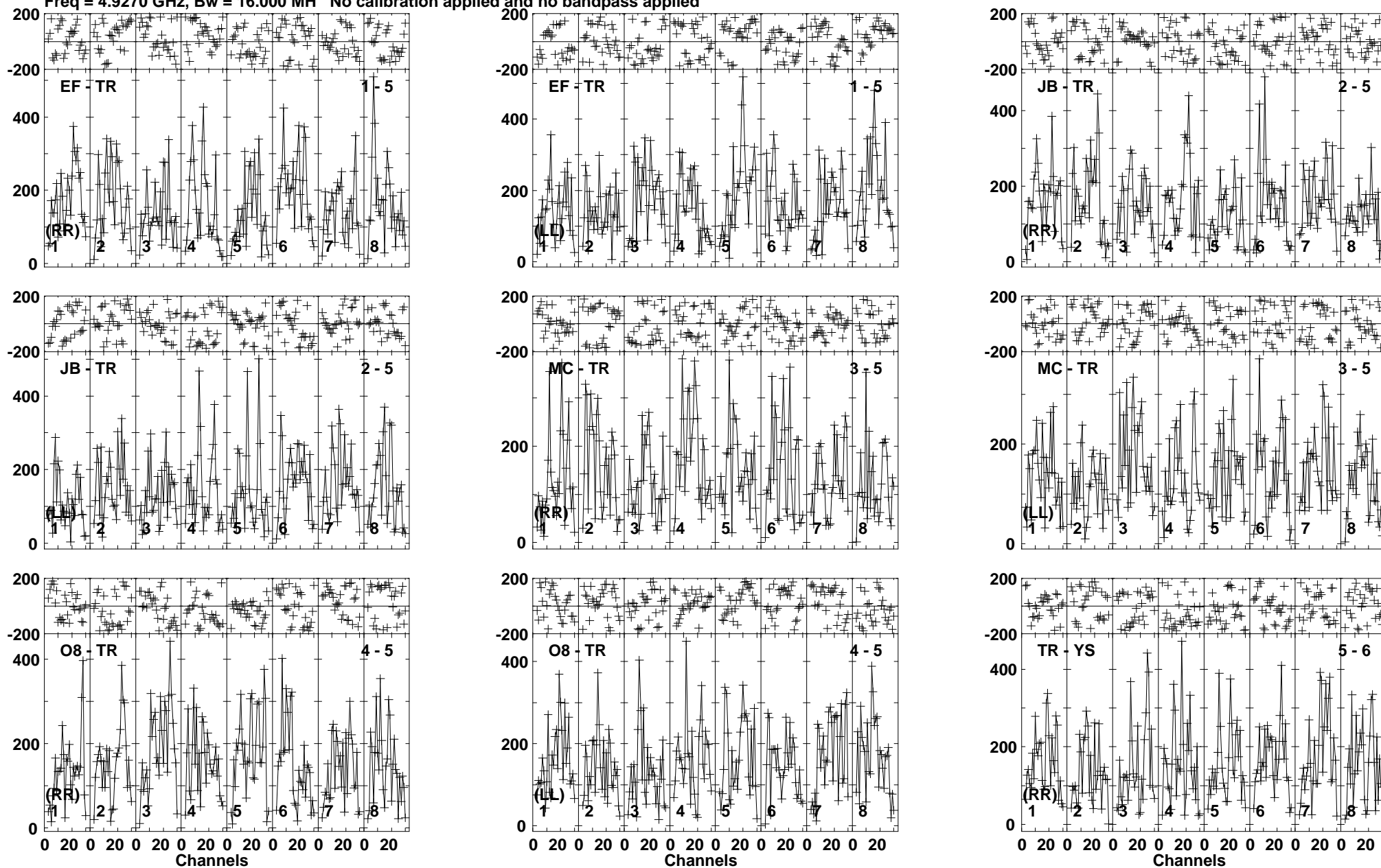
Lower frame: Micro Ampl Jy Top frame: Phas deg Vector averaged cross-power spectrum Baseline: EF (01) - TR (05) Timerange: 00/15:02:01 to 00/15:03:59
