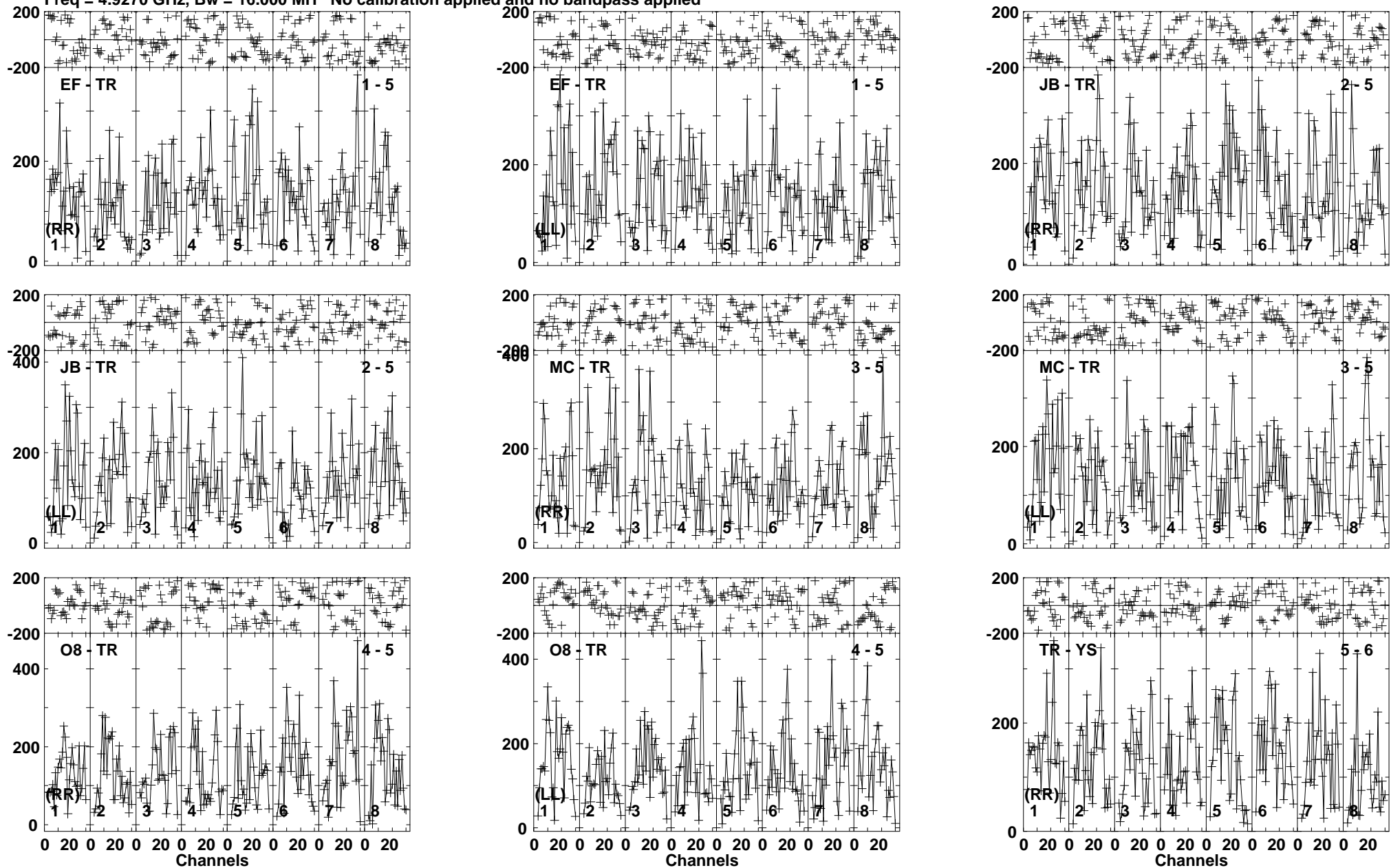
Lower frame: Micro Ampl Jy Top frame: Phas deg Vector averaged cross-power spectrum Baseline: EF (01) - TR (05) Timerange: 00/16:14:01 to 00/16:16:09
