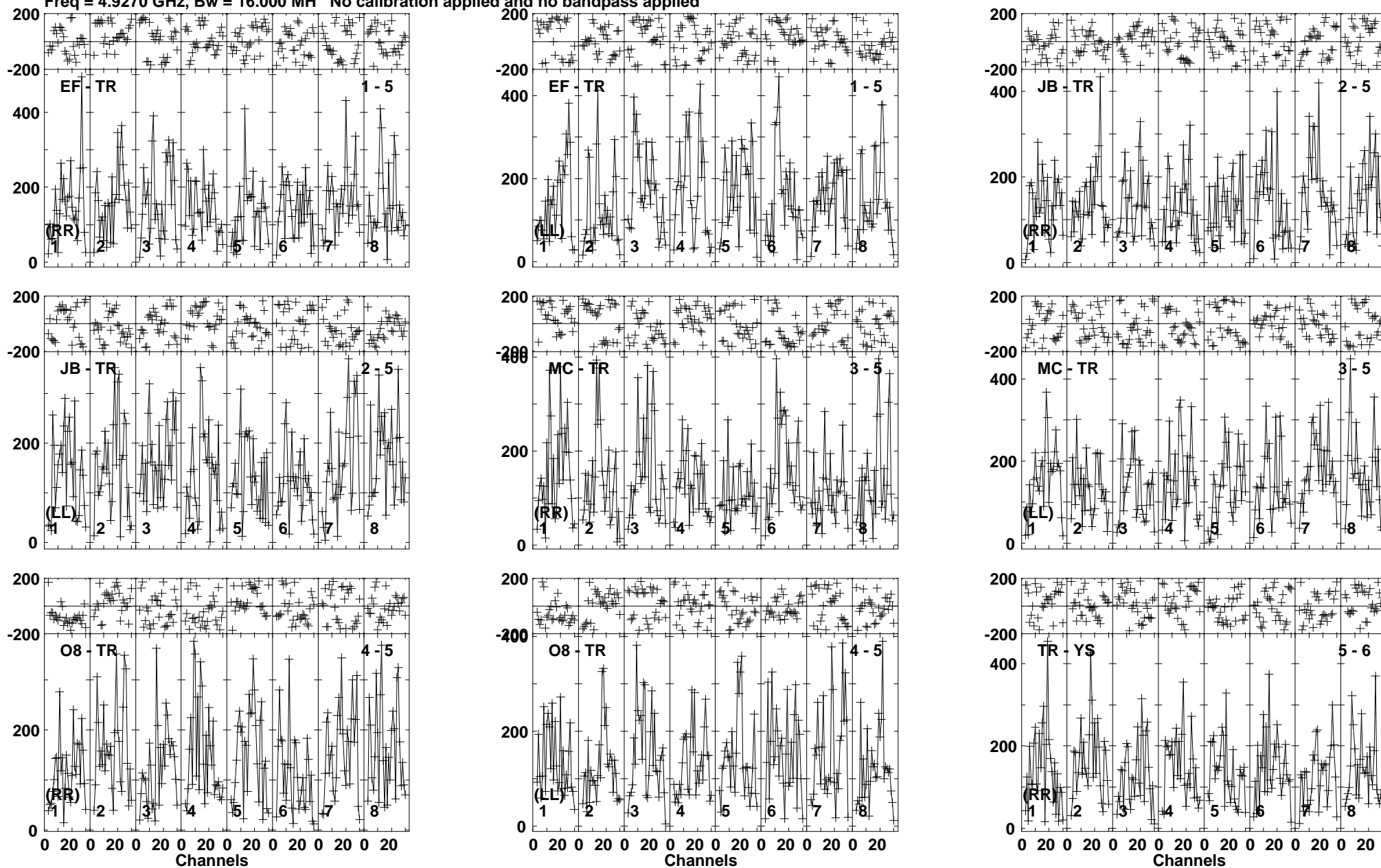
Lower frame: Micro Ampl Jy Top frame: Phas deg Vector averaged cross-power spectrum Baseline: EF (01) - TR (05) Timerange: 00/16:40:41 to 00/16:42:39
