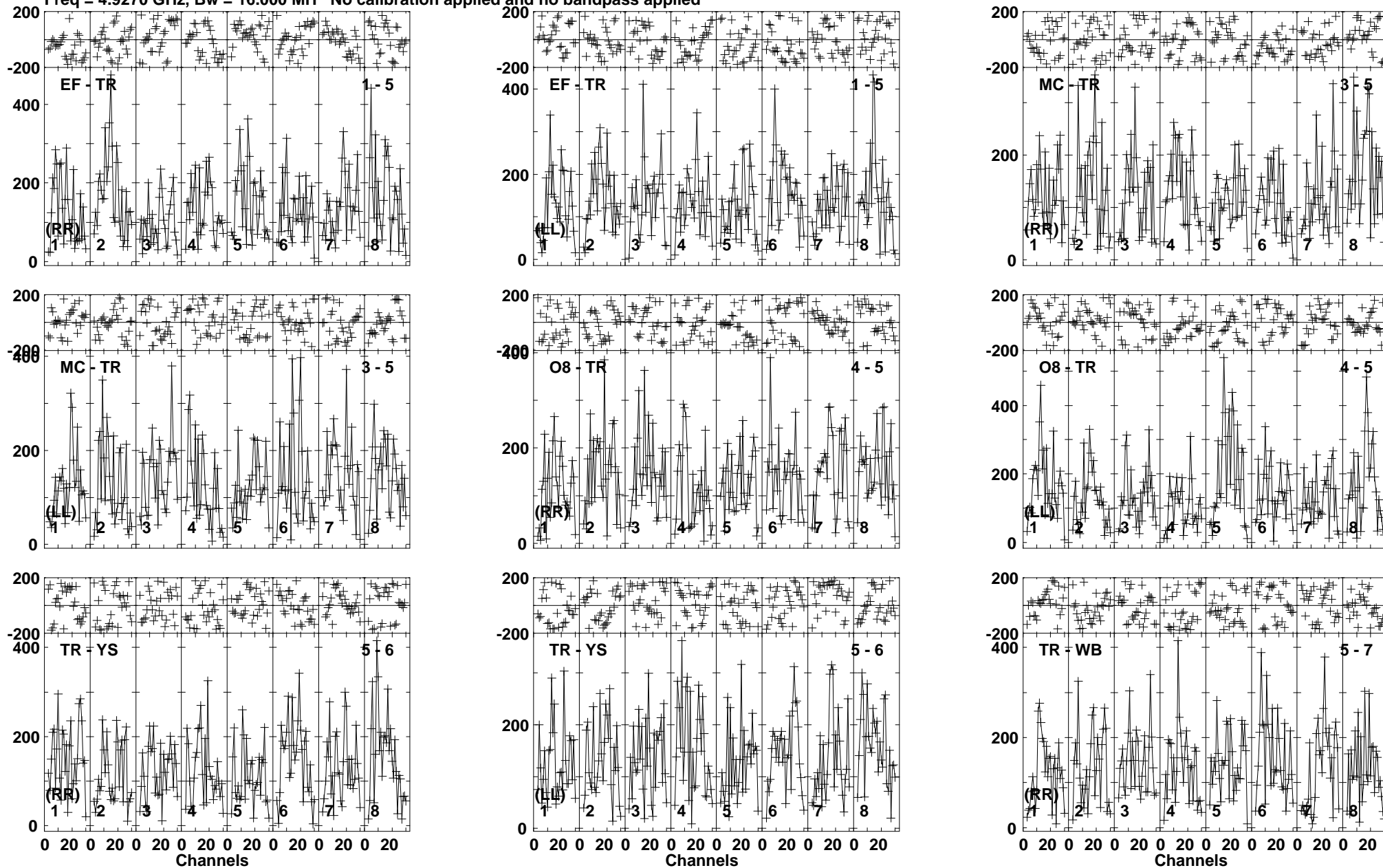
Lower frame: Micro Ampl Jy Top frame: Phas deg Vector averaged cross-power spectrum Baseline: EF (01) - TR (05) Timerange: 00/19:30:31 to 00/19:32:39
