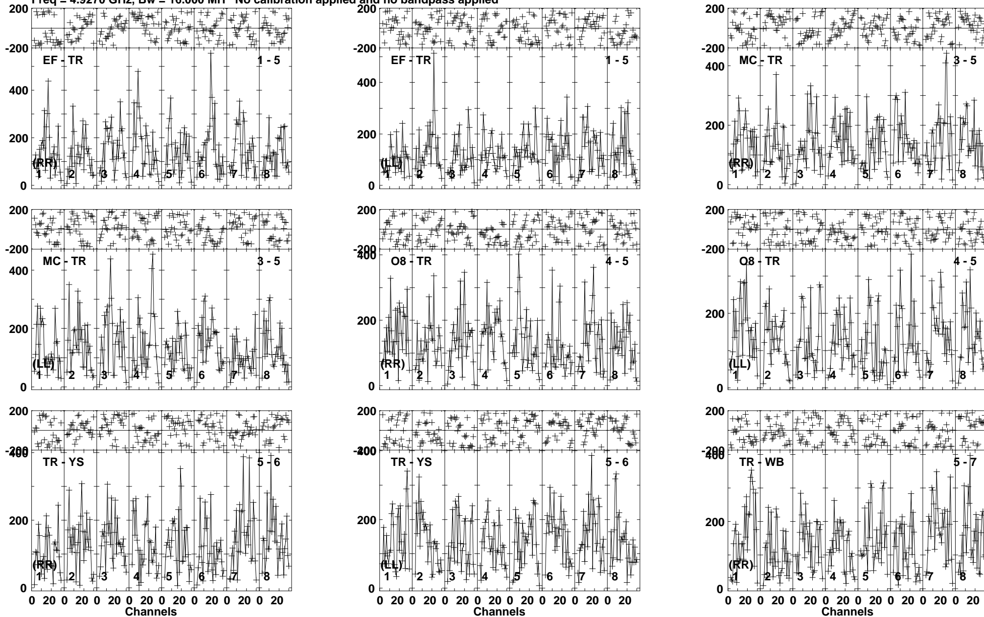
Lower frame: Micro Ampl Jy Top frame: Phas deg Vector averaged cross-power spectrum Baseline: EF (01) - TR (05) Timerange: 00/19:08:01 to 00/19:10:09
