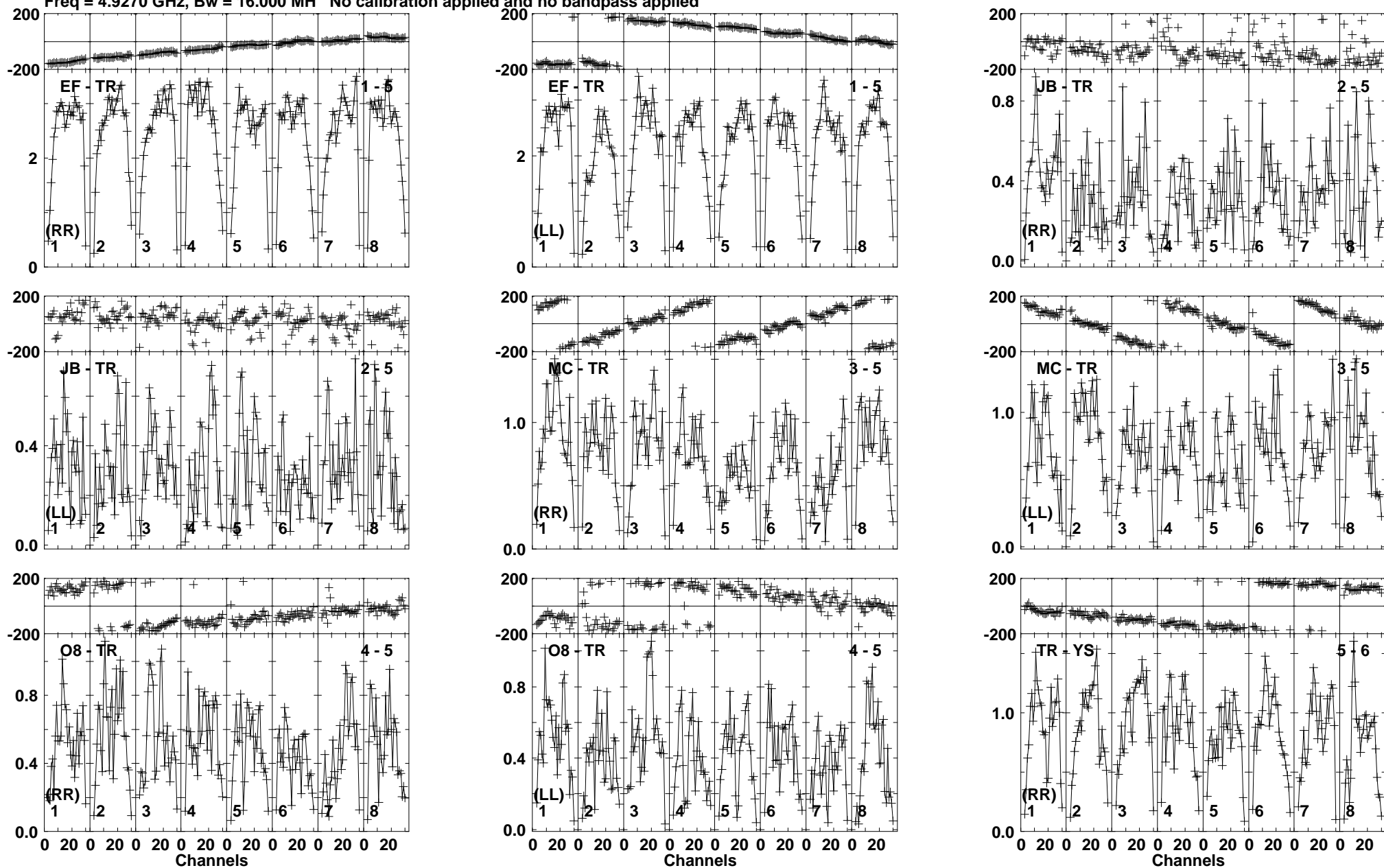
Lower frame: Milli Ampl Jy Top frame: Phas deg Vector averaged cross-power spectrum Baseline: EF (01) - TR (05) Timerange: 00/13:22:02 to 00/13:23:18
