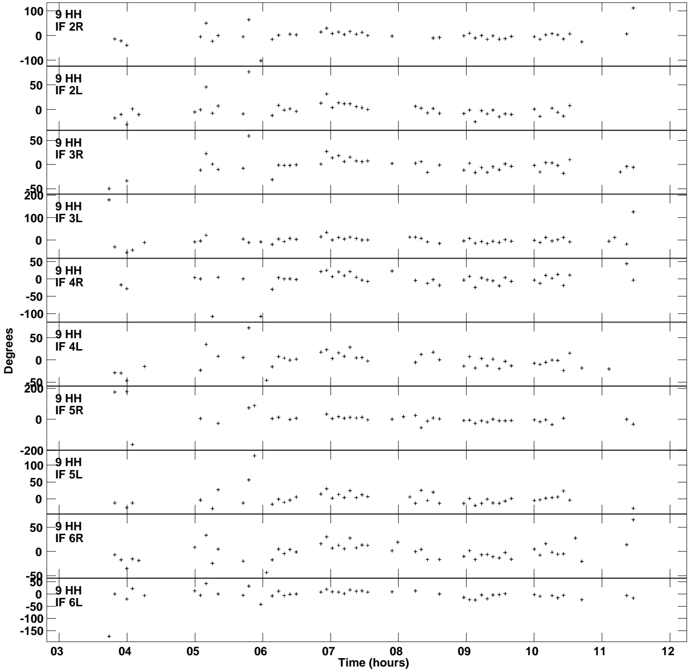
Plot file version 14 created 16-AUG-2016 17:54:01 Gain phs vs UTC time for J1832-2039.MULTI.1 SN 1 Rpol & Lpol IF 1 - 8
