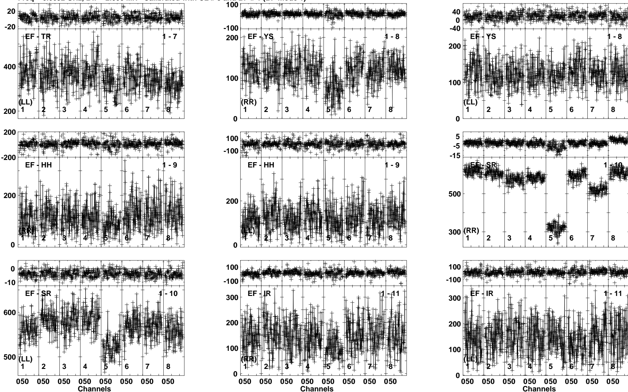
Lower frame: Milli Ampl Jy Top frame: Phas deg Vector averaged cross-power spectrum Baseline: EF (01) - TR (07) Timerange: 00/06:06:47 to 00/06:09:39
