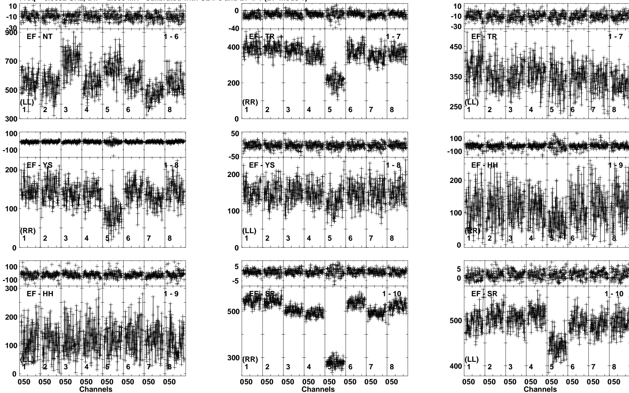
Lower frame: Milli Ampl Jy Top frame: Phas deg Vector averaged cross-power spectrum Baseline: EF (01) - NT (06) Timerange: 00/07:21:11 to 00/07:24:09
