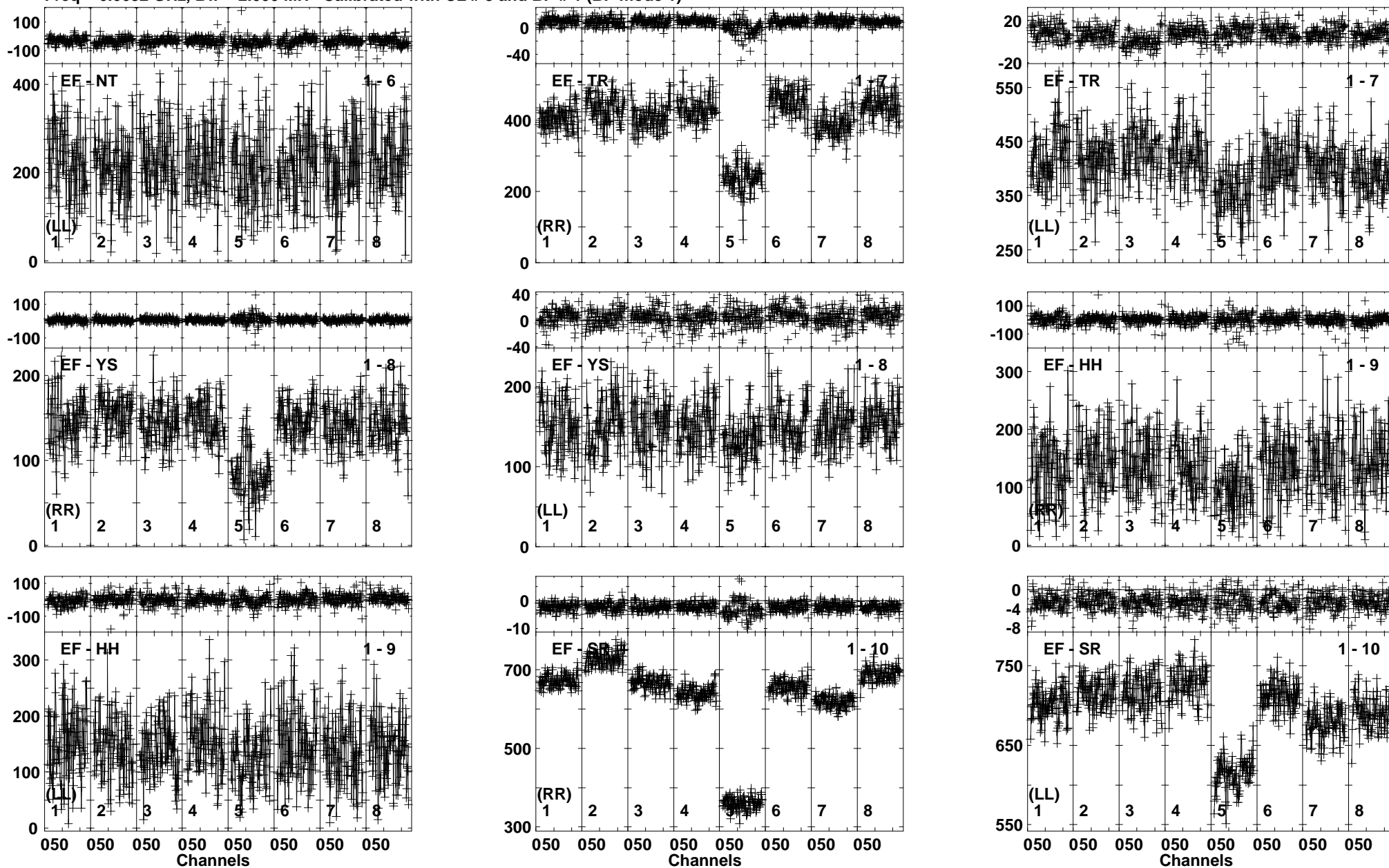
Lower frame: Milli Ampl Jy Top frame: Phas deg Vector averaged cross-power spectrum Baseline: EF (01) - NT (06) Timerange: 00/06:28:01 to 00/06:30:59
