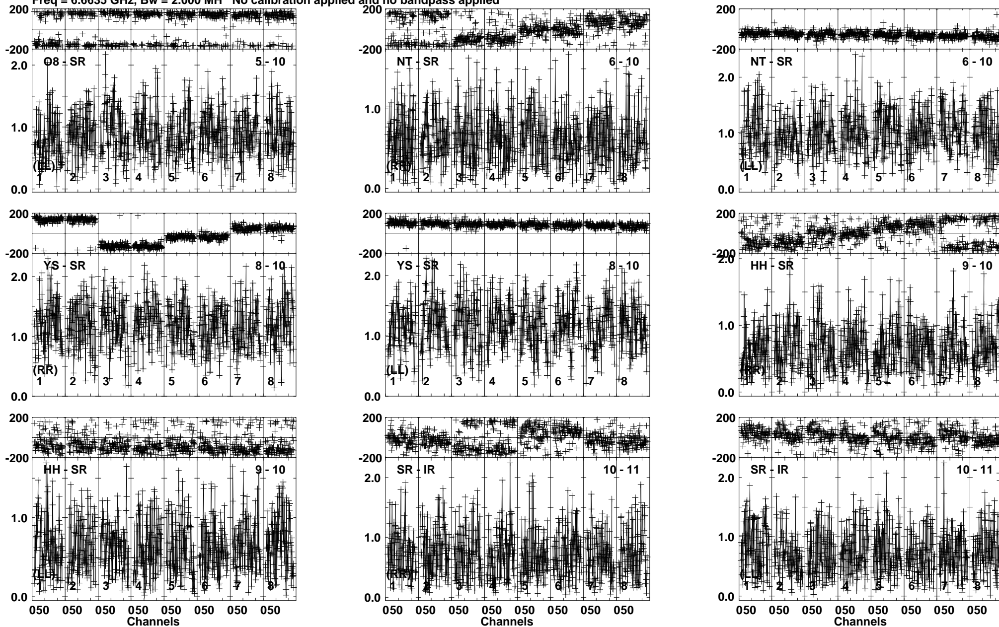
Lower frame: Milli Ampl Jy Top frame: Phas deg Vector averaged cross-power spectrum Baseline: O8 (05) - SR (10) Timerange: 00/06:45:48 to 00/06:48:40
