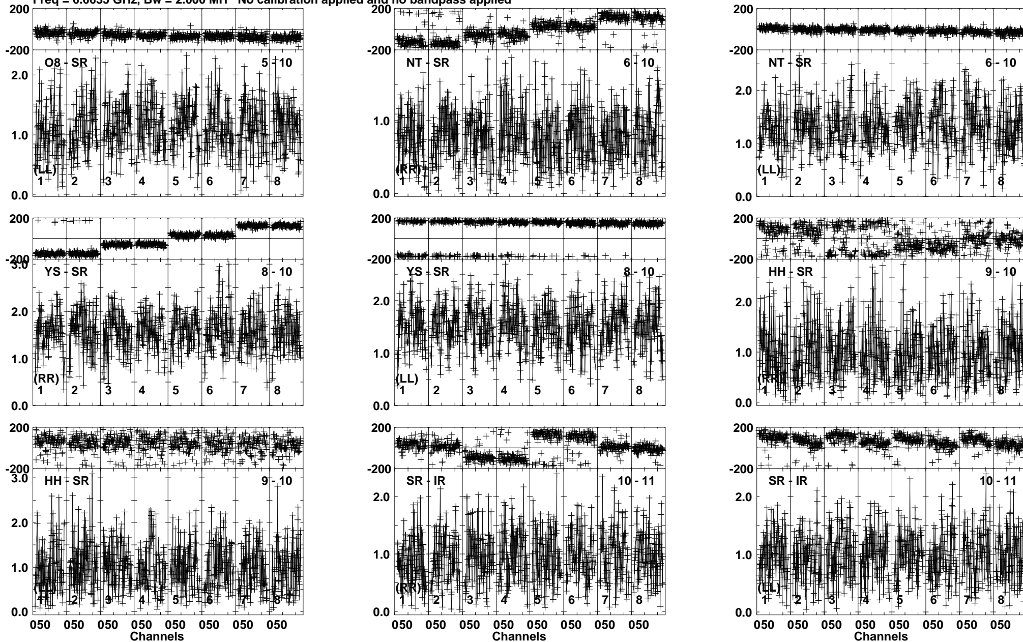
Lower frame: Milli Ampl Jy Top frame: Phas deg Vector averaged cross-power spectrum Baseline: O8 (05) - SR (10) Timerange: 00/07:37:48 to 00/07:40:40
