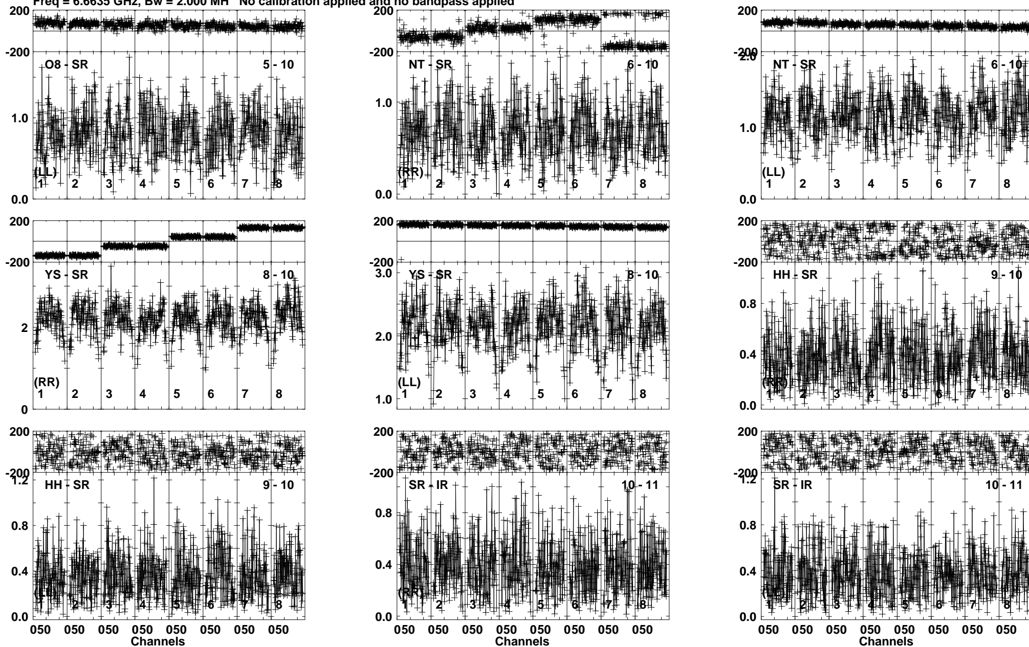
Lower frame: Milli Ampl Jy Top frame: Phas deg Vector averaged cross-power spectrum Baseline: O8 (05) - SR (10) Timerange: 00/11:12:52 to 00/11:17:50
