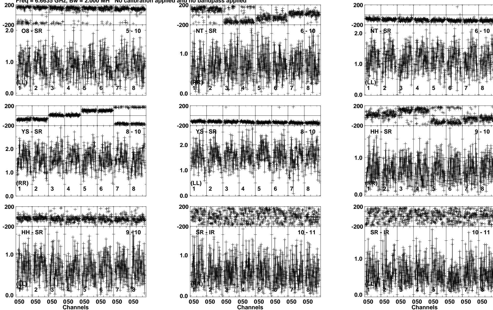
Lower frame: Milli Ampl Jy Top frame: Phas deg Vector averaged cross-power spectrum Baseline: O8 (05) - SR (10) Timerange: 00/08:45:37 to 00/08:48:35
