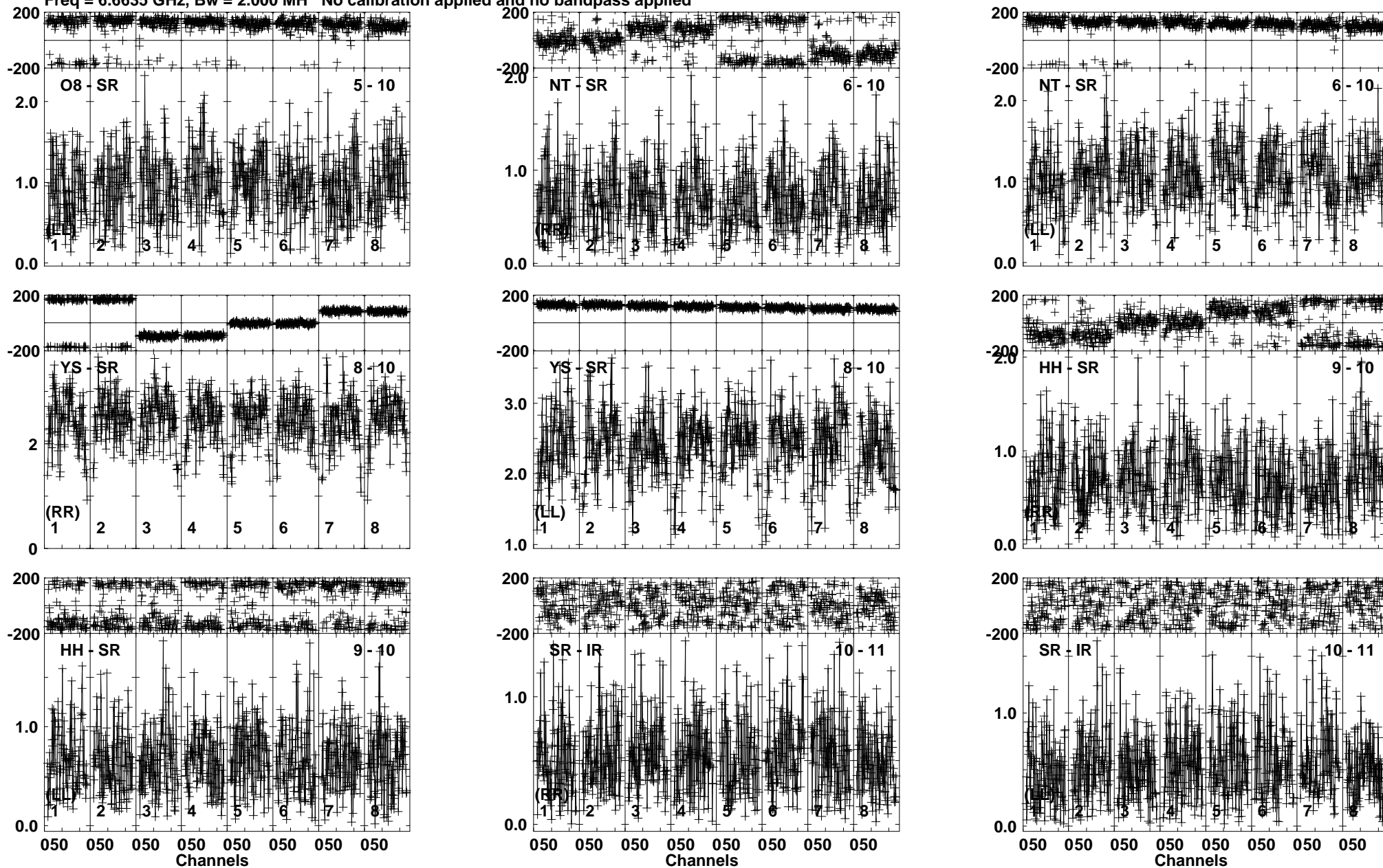
Lower frame: Milli Ampl Jy Top frame: Phas deg Vector averaged cross-power spectrum Baseline: O8 (05) - SR (10) Timerange: 00/10:15:46 to 00/10:18:40
