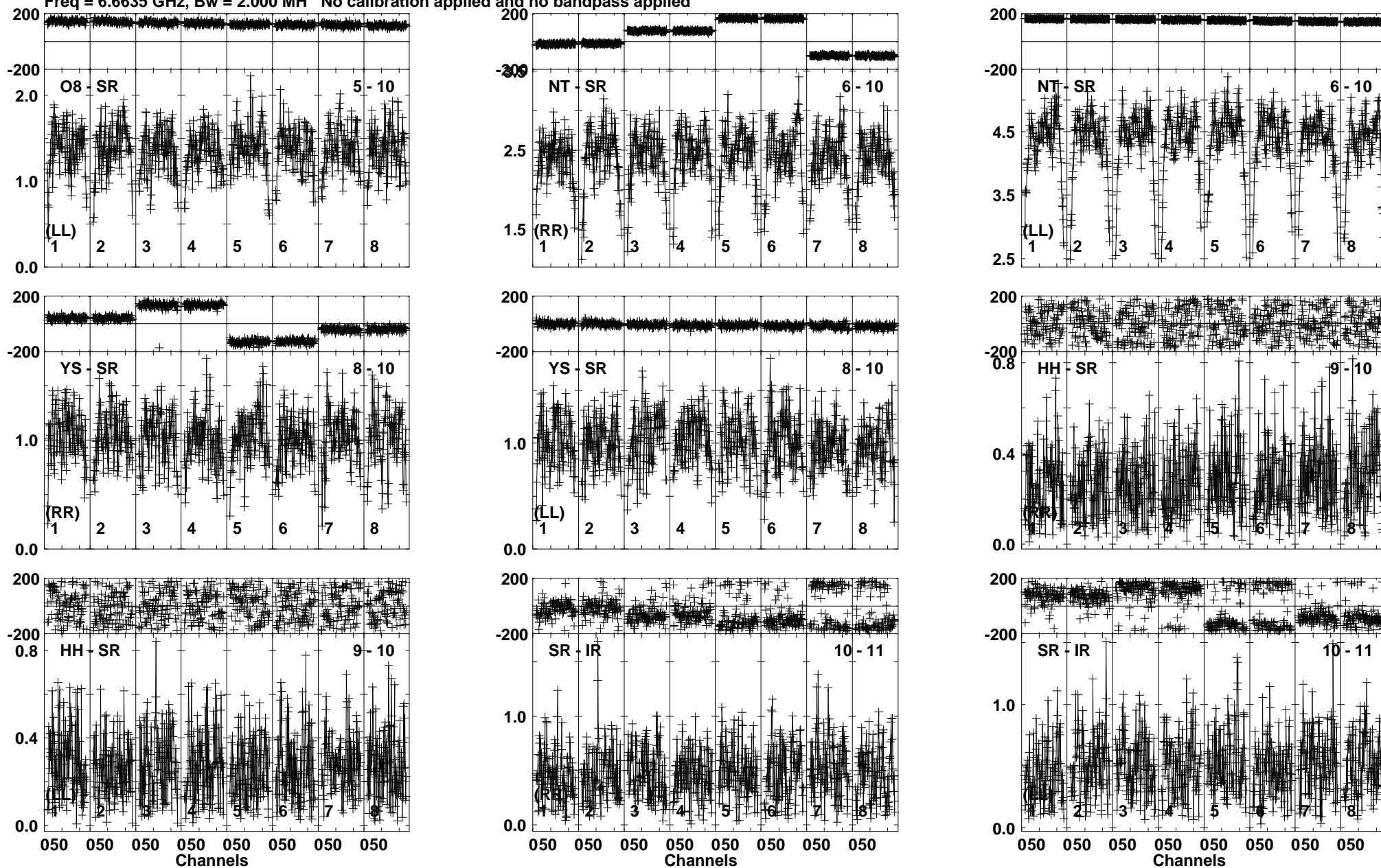
Lower frame: Milli Ampl Jy Top frame: Phas deg Vector averaged cross-power spectrum Baseline: O8 (05) - SR (10) Timerange: 00/02:51:06 to 00/02:59:04
