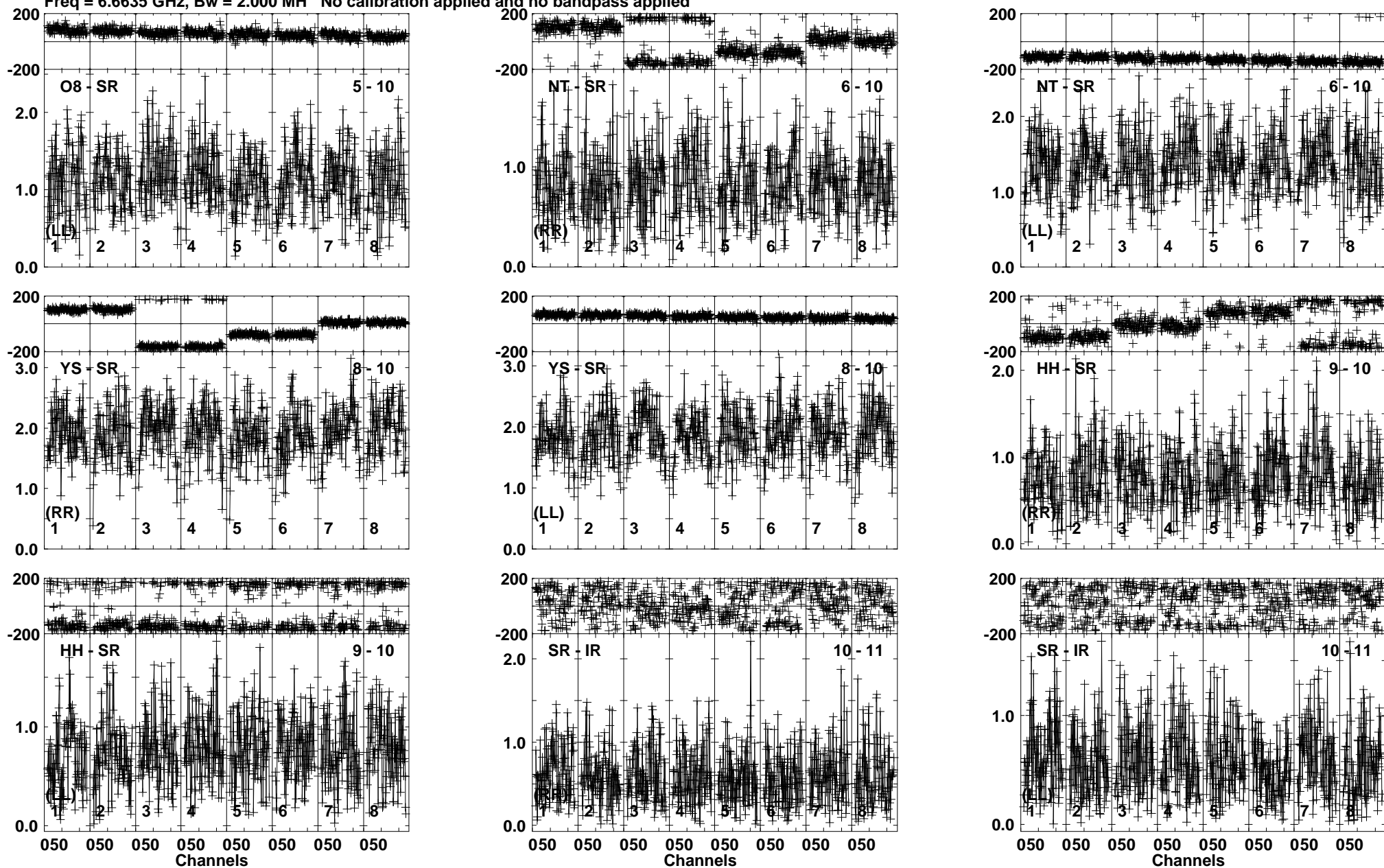
Lower frame: Milli Ampl Jy Top frame: Phas deg Vector averaged cross-power spectrum Baseline: O8 (05) - SR (10) Timerange: 00/08:30:02 to 00/08:33:00
