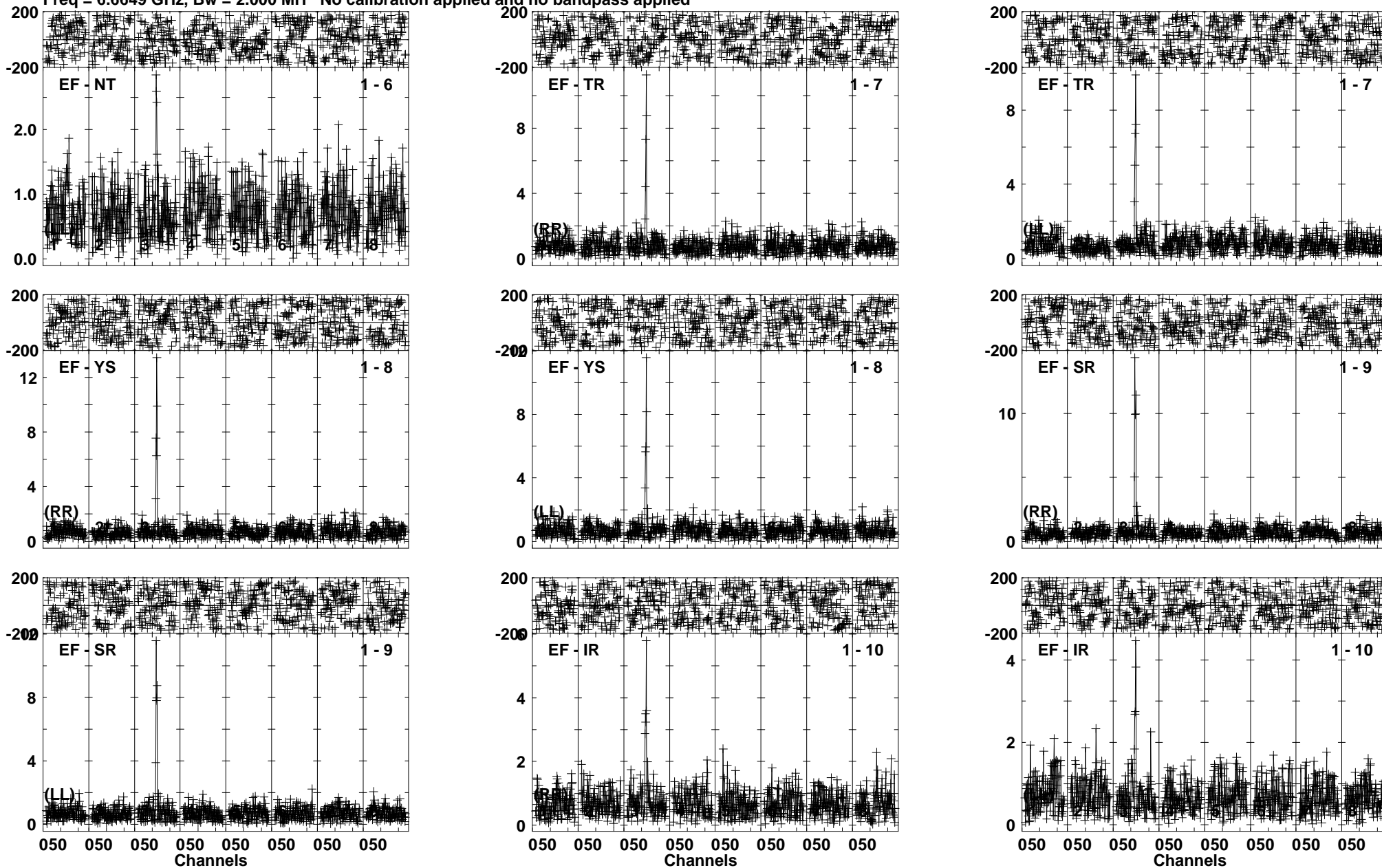
Lower frame: Milli Ampl Jy Top frame: Phas deg Vector averaged cross-power spectrum Baseline: EF (01) - NT (06) Timerange: 00/01:31:01 to 00/01:32:59
