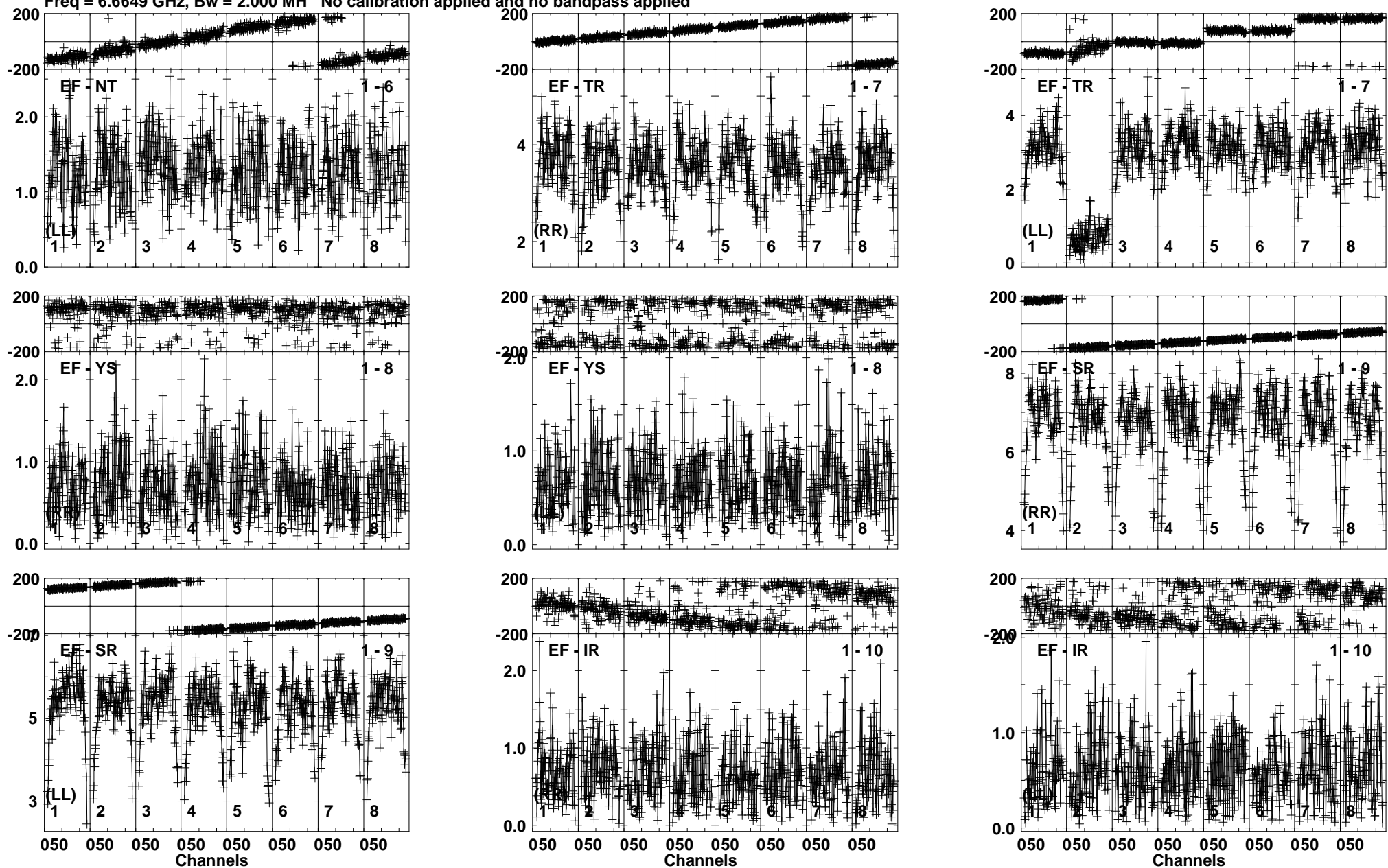
Lower frame: Milli Ampl Jy Top frame: Phas deg Vector averaged cross-power spectrum Baseline: EF (01) - NT (06) Timerange: 00/08:06:36 to 00/08:09:34
