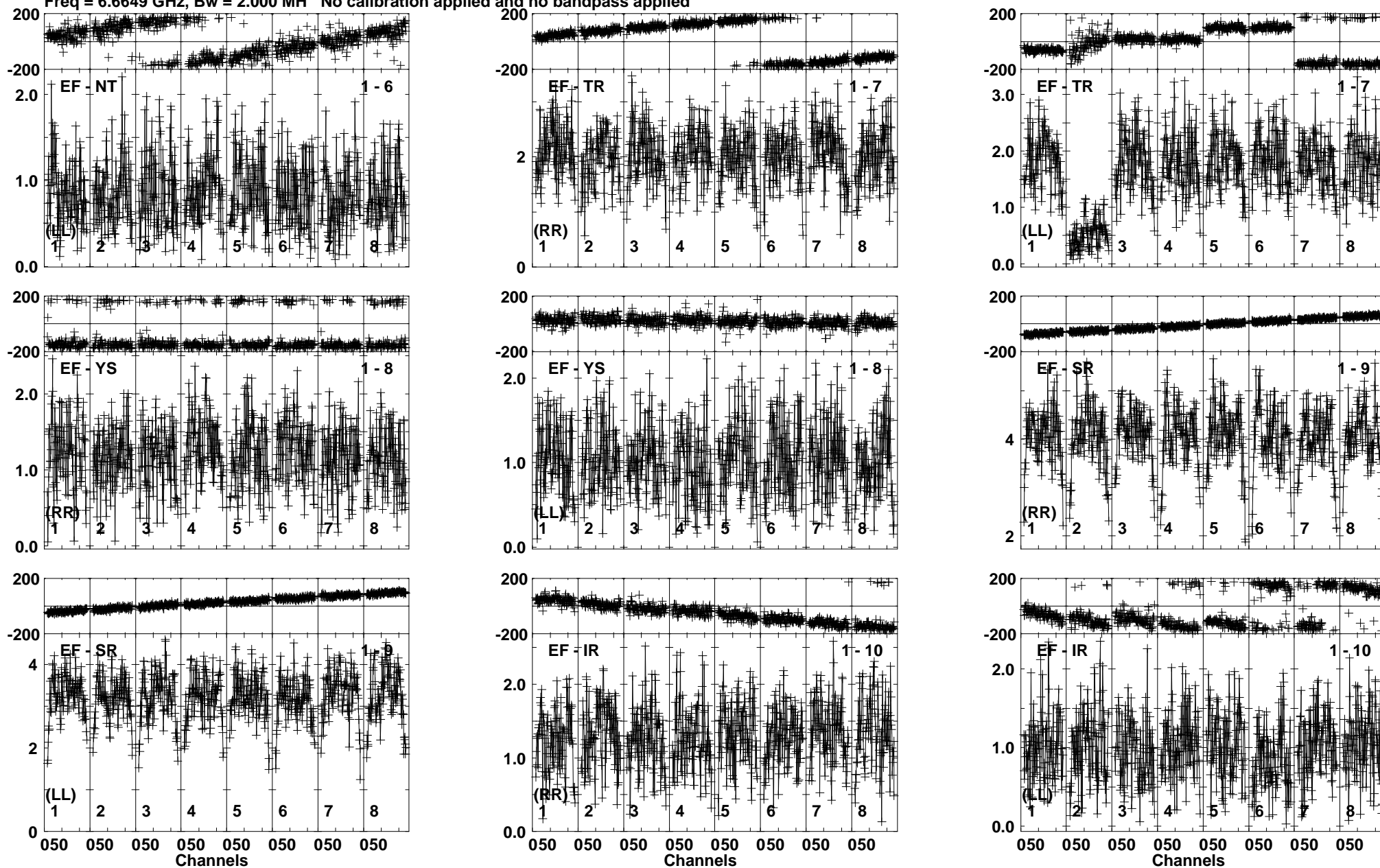
Lower frame: Milli Ampl Jy Top frame: Phas deg Vector averaged cross-power spectrum Baseline: EF (01) - NT (06) Timerange: 00/03:27:41 to 00/03:30:39
