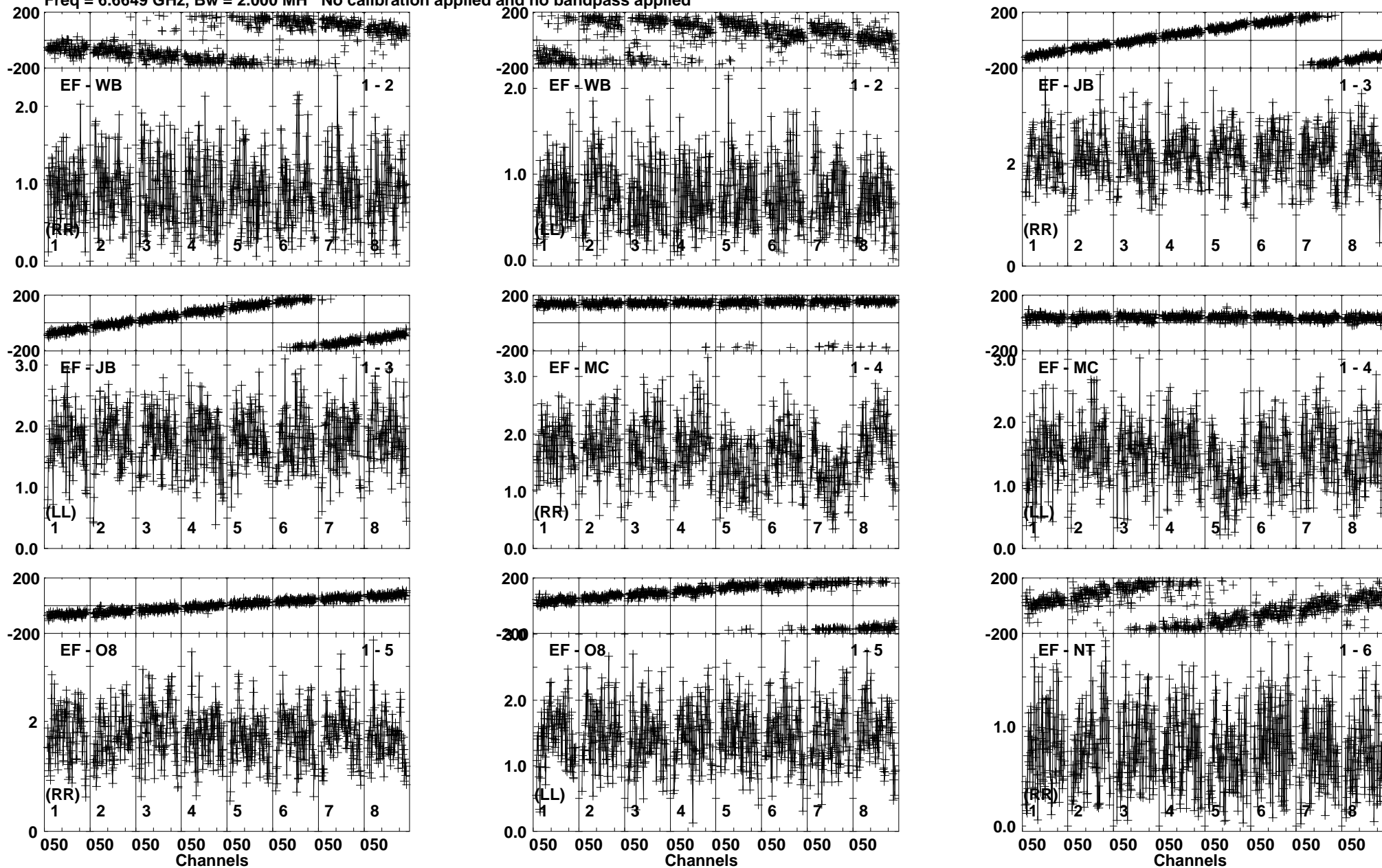
Lower frame: Milli Ampl Jy Top frame: Phas deg Vector averaged cross-power spectrum Baseline: EF (01) - WB (02) Timerange: 00/01:28:01 to 00/01:30:59
