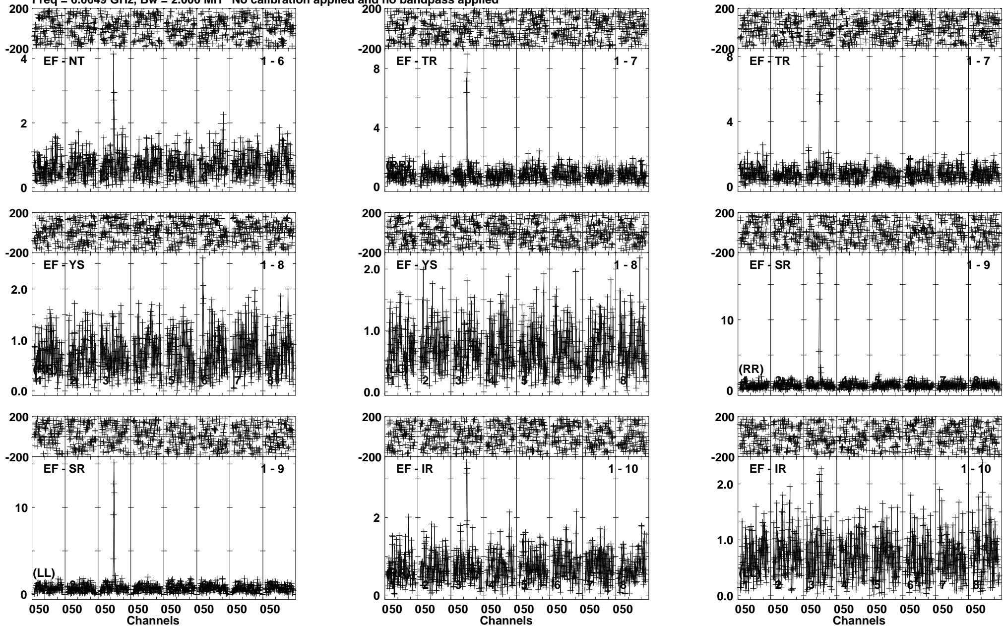
Lower frame: Milli Ampl Jy Top frame: Phas deg Vector averaged cross-power spectrum Baseline: EF (01) - NT (06) Timerange: 00/08:04:36 to 00/08:06:34
