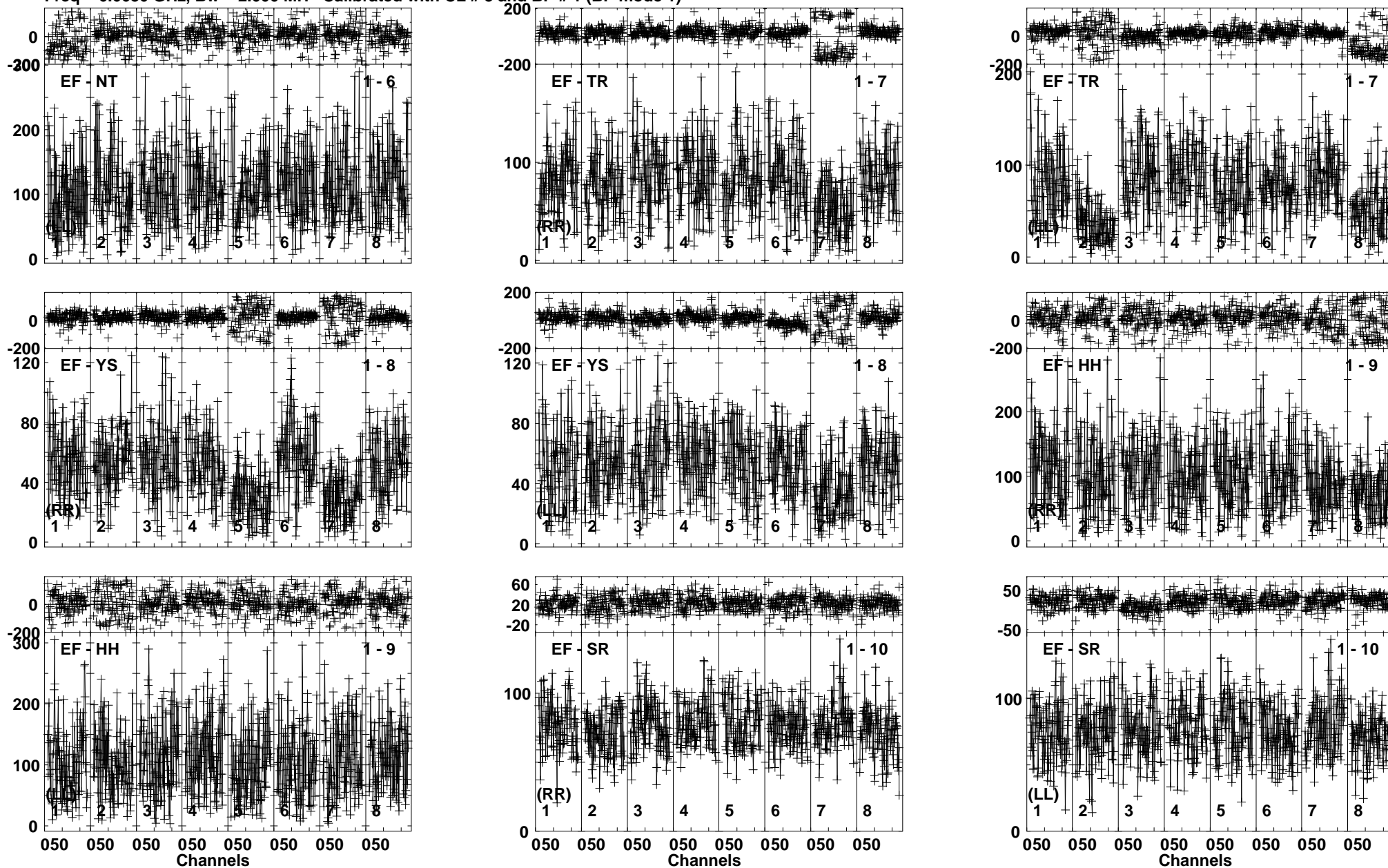
Lower frame: Milli Ampl Jy Top frame: Phas deg Vector averaged cross-power spectrum Baseline: EF (01) - NT (06) Timerange: 00/21:18:26 to 00/21:21:24
