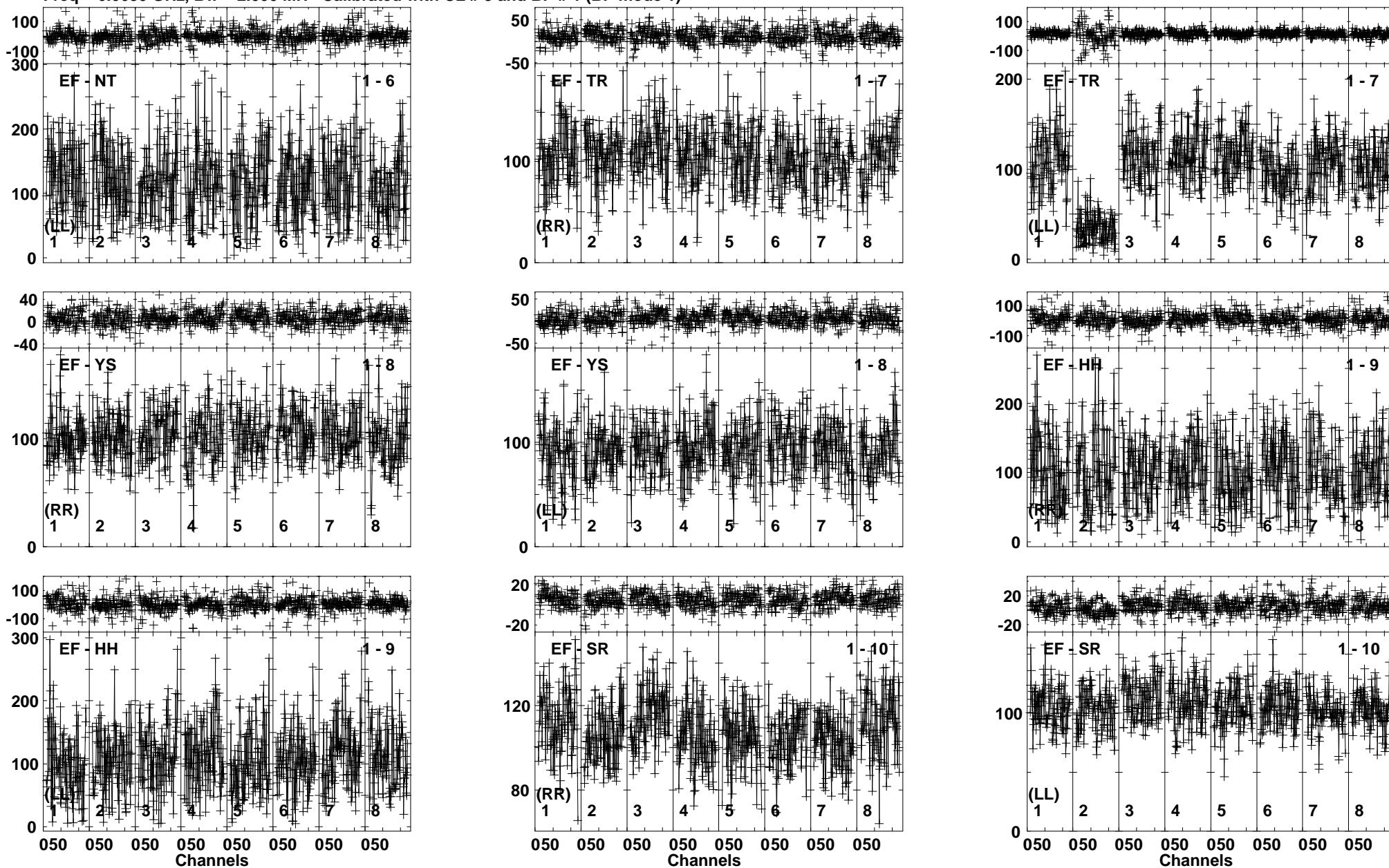
Lower frame: Milli Ampl Jy Top frame: Phas deg Vector averaged cross-power spectrum Baseline: EF (01) - NT (06) Timerange: 01/01:58:56 to 01/02:01:54
