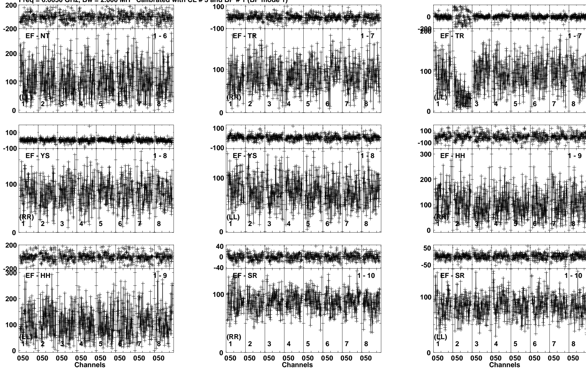
Lower frame: Milli Ampl Jy Top frame: Phas deg Vector averaged cross-power spectrum Baseline: EF (01) - NT (06) Timerange: 01/00:14:41 to 01/00:17:39
