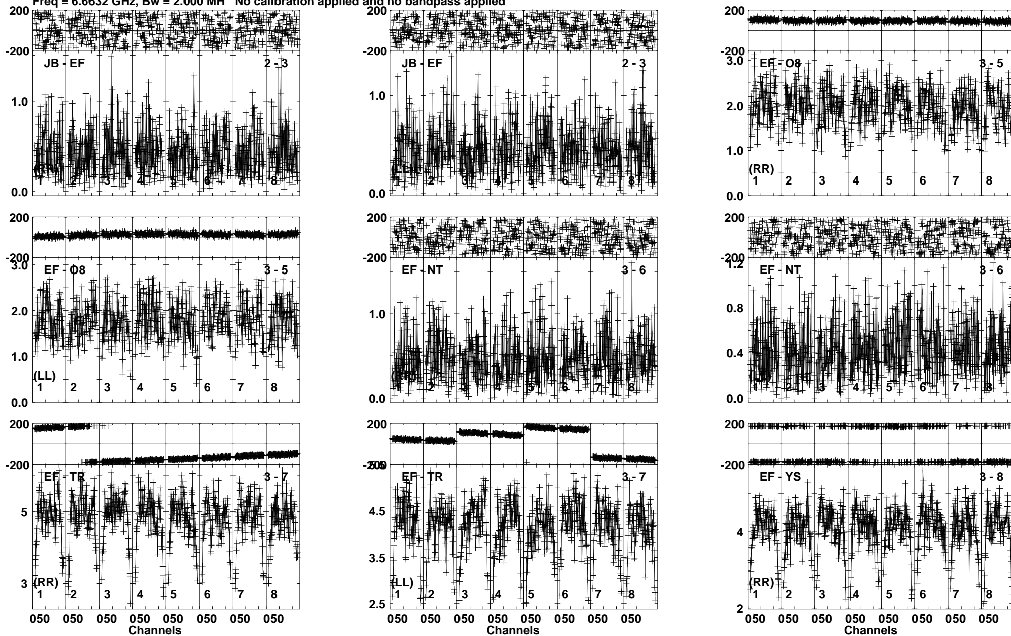
Lower frame: Milli Ampl Jy Top frame: Phas deg Vector averaged cross-power spectrum Baseline: JB (02) - EF (03) Timerange: 00/07:52:51 to 00/07:55:49
