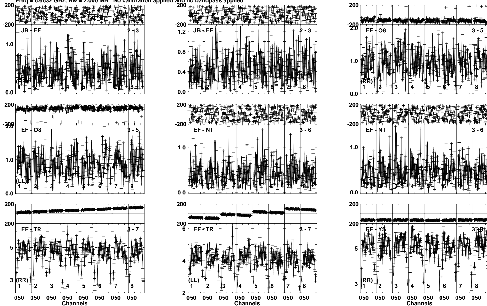
Lower frame: Milli Ampl Jy Top frame: Phas deg Vector averaged cross-power spectrum Baseline: JB (02) - EF (03) Timerange: 00/05:40:06 to 00/05:43:04
