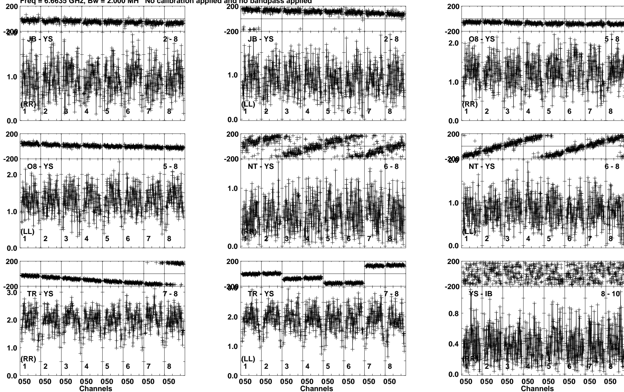
Lower frame: Milli Ampl Jy Top frame: Phas deg Vector averaged cross-power spectrum Baseline: JB (02) - YS (08) Timerange: 00/03:18:12 to 00/03:26:10
