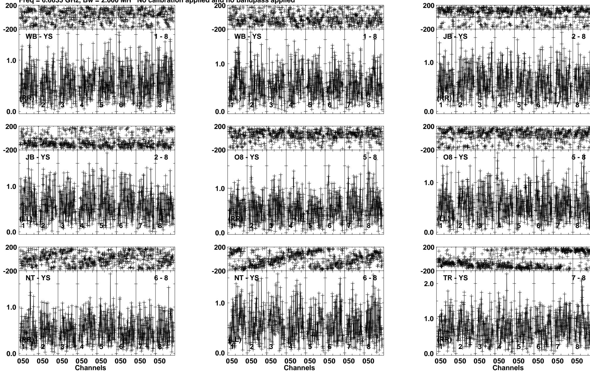
Lower frame: Milli Ampl Jy Top frame: Phas deg Vector averaged cross-power spectrum Baseline: WB (01) - YS (08) Timerange: 00/04:53:37 to 00/04:56:35
