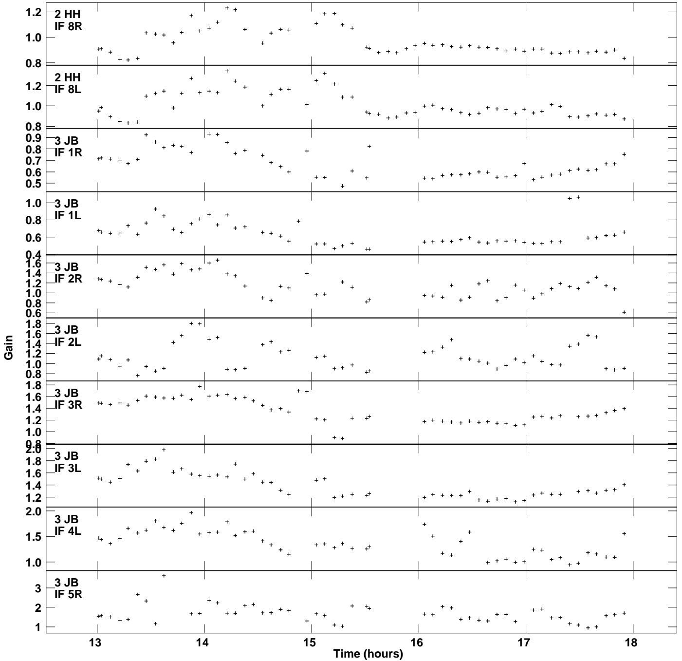
Plot file version 4 created 26-SEP-2015 17:47:44 Gain amp vs UTC time for J1642+2523.MULTI.1 SN 2 Rpol & Lpol IF 1 - 8
