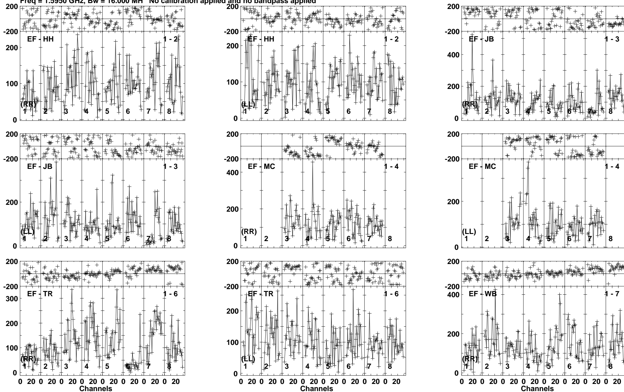
Lower frame: Micro Ampl Jy Top frame: Phas deg Vector averaged cross-power spectrum Baseline: EF (01) - HH (02) Timerange: 00/16:59:22 to 00/17:02:48
