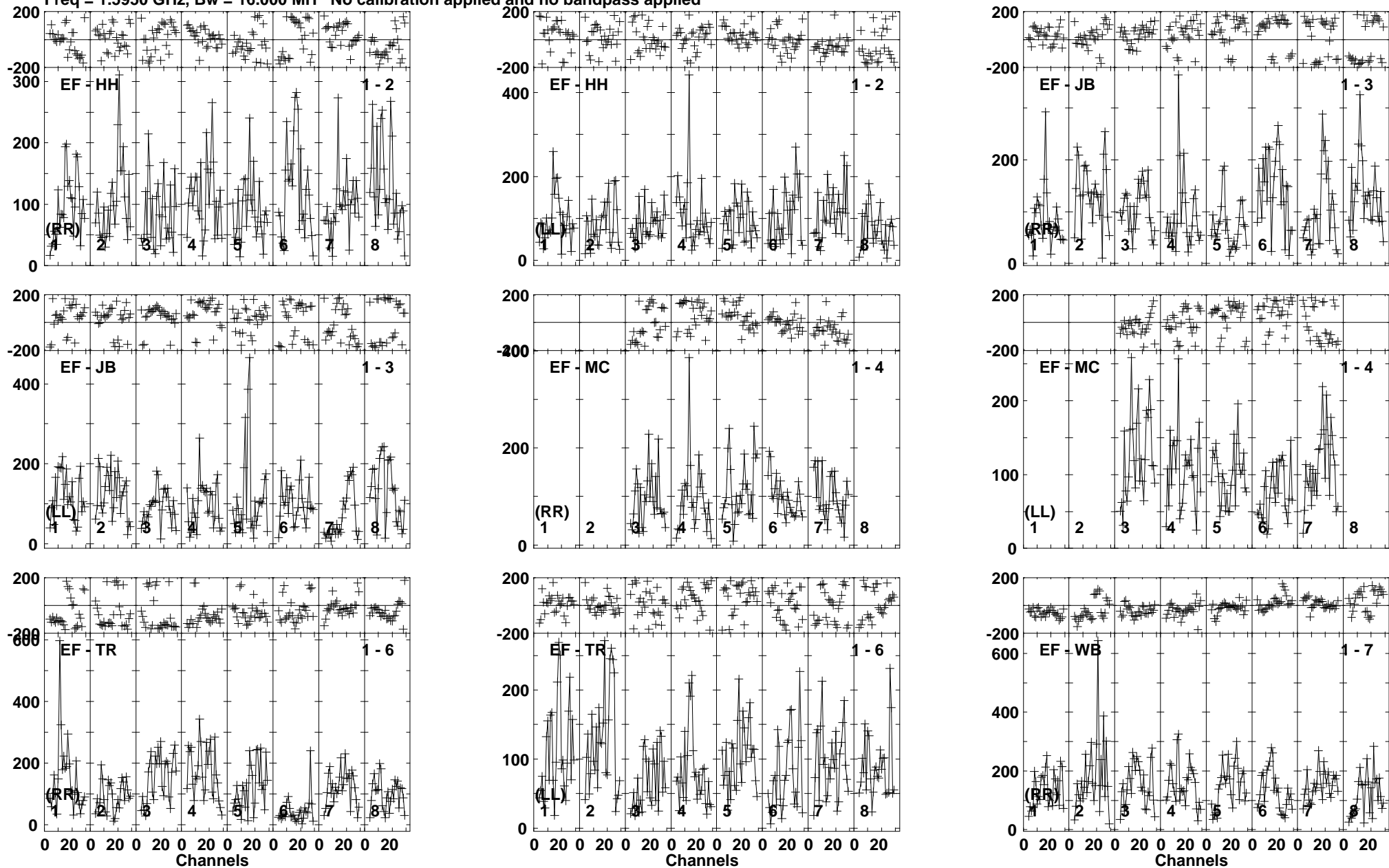
Lower frame: Micro Ampl Jy Top frame: Phas deg Vector average cross-power spectrum Baseline: EF (01) - HH (02) Timerange: 00/16:44:12 to 00/16:47:38
