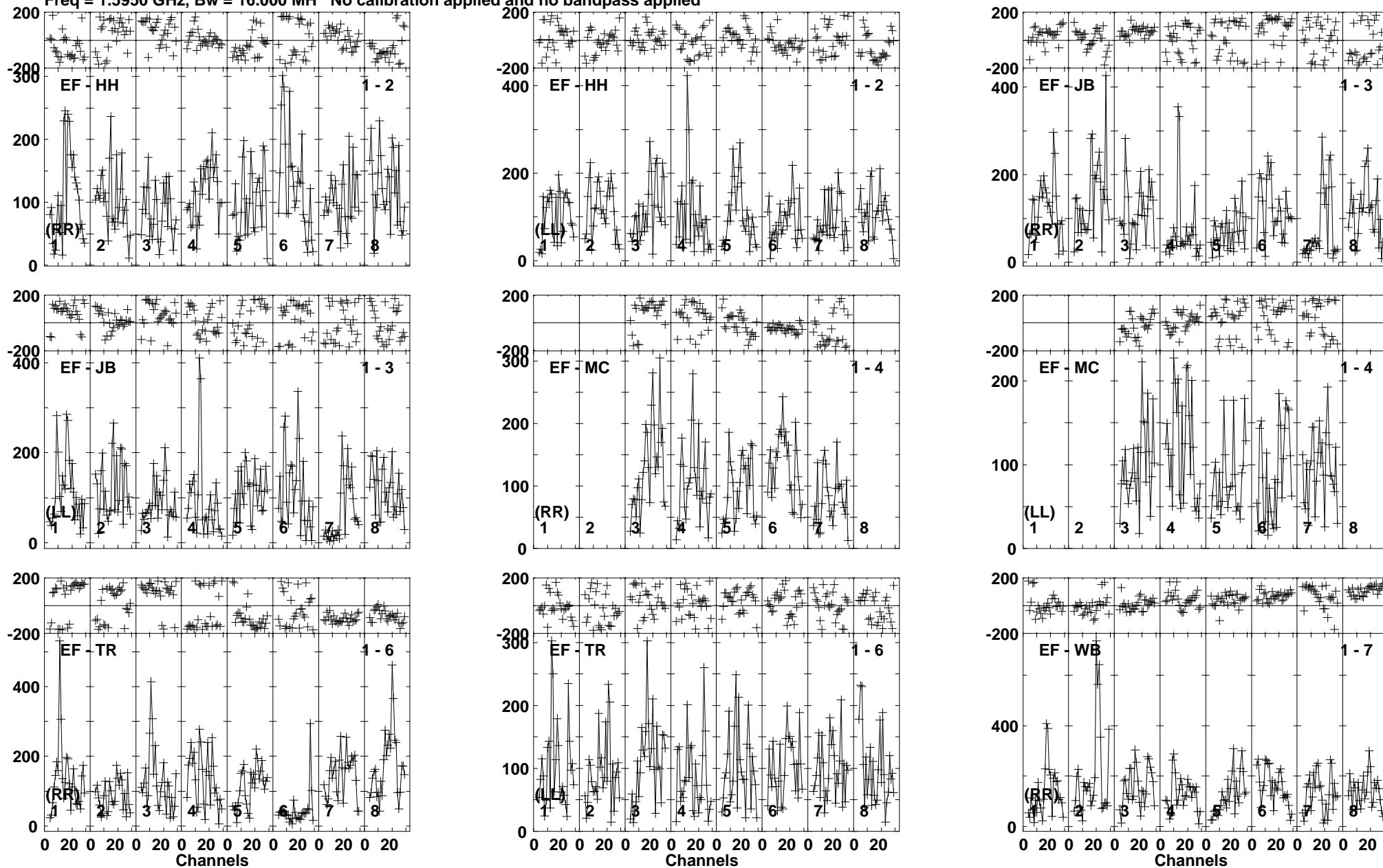
Lower frame: Micro Ampl Jy Top frame: Phas deg Vector averaged cross-power spectrum Baseline: EF (01) - HH (02) Timerange: 00/16:34:02 to 00/16:37:28
