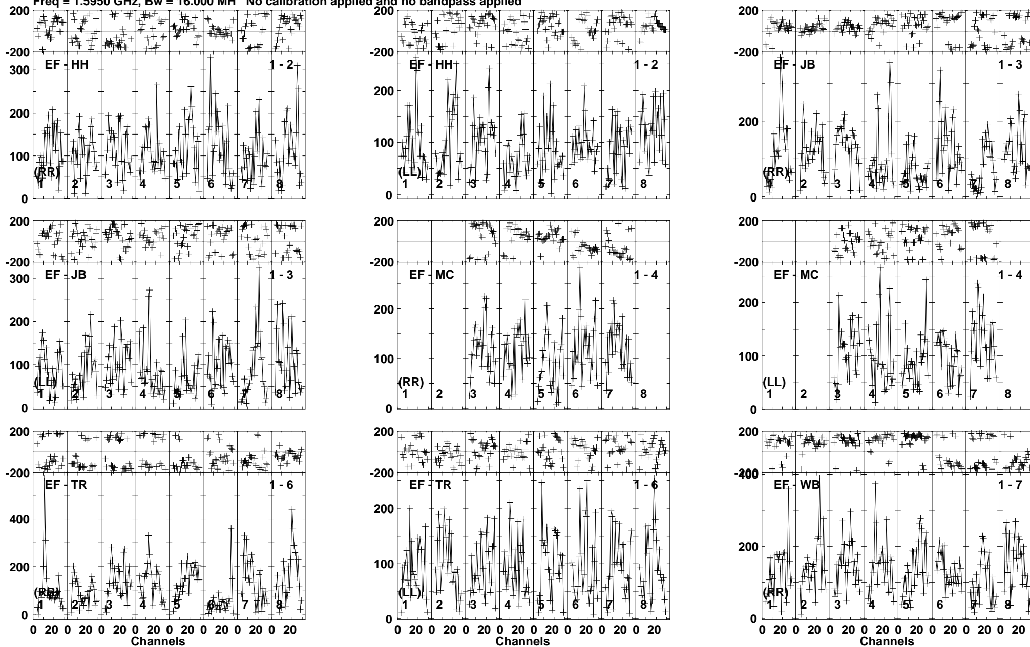
Lower frame: Micro Ampl Jy Top frame: Phas deg Vector averaged cross-power spectrum Baseline: EF (01) - HH (02) Timerange: 00/16:13:42 to 00/16:17:08
