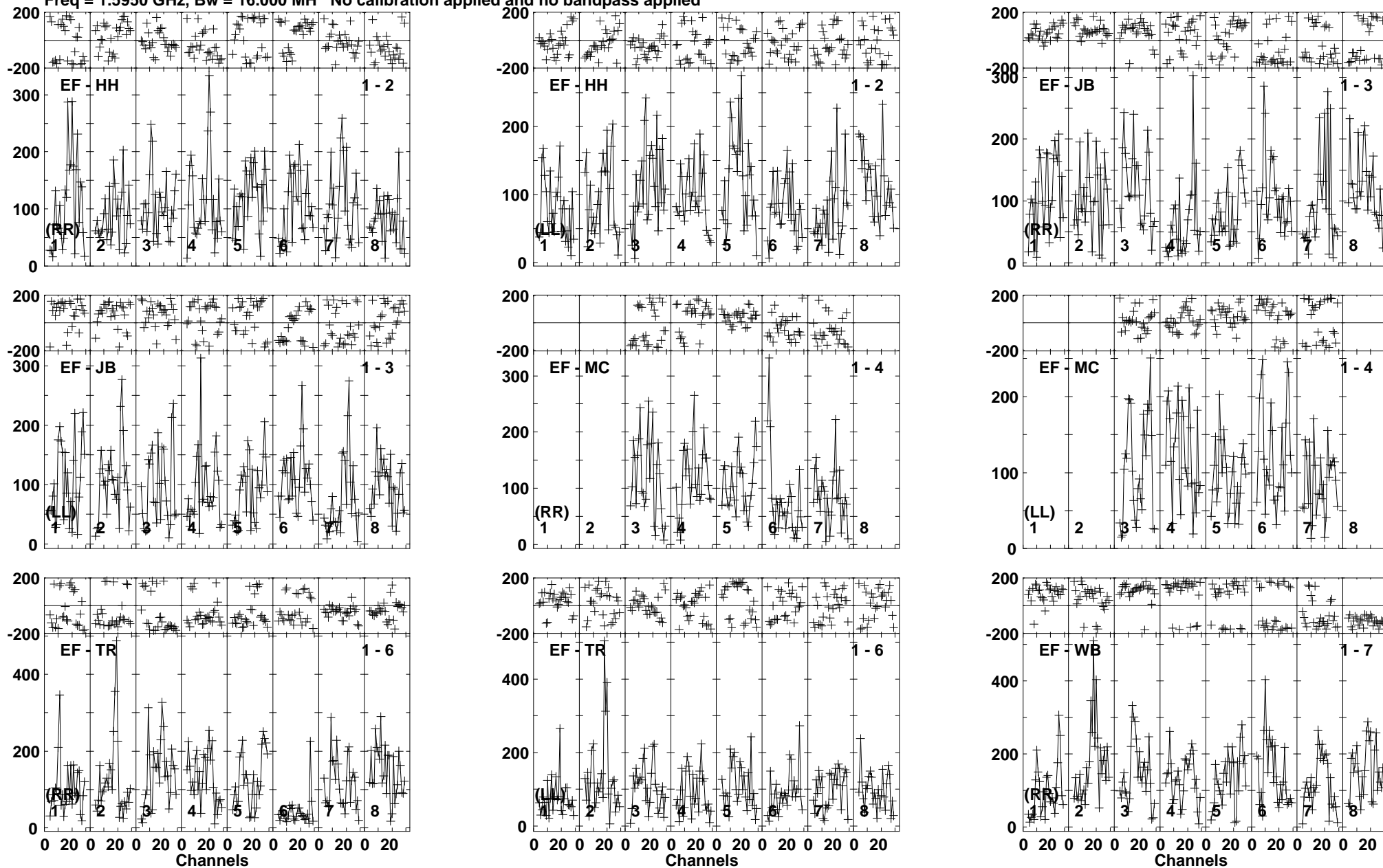
Lower frame: Micro Ampl Jy Top frame: Phas deg Vector averaged cross-power spectrum Baseline: EF (01) - HH (02) Timerange: 00/16:08:32 to 00/16:11:58
