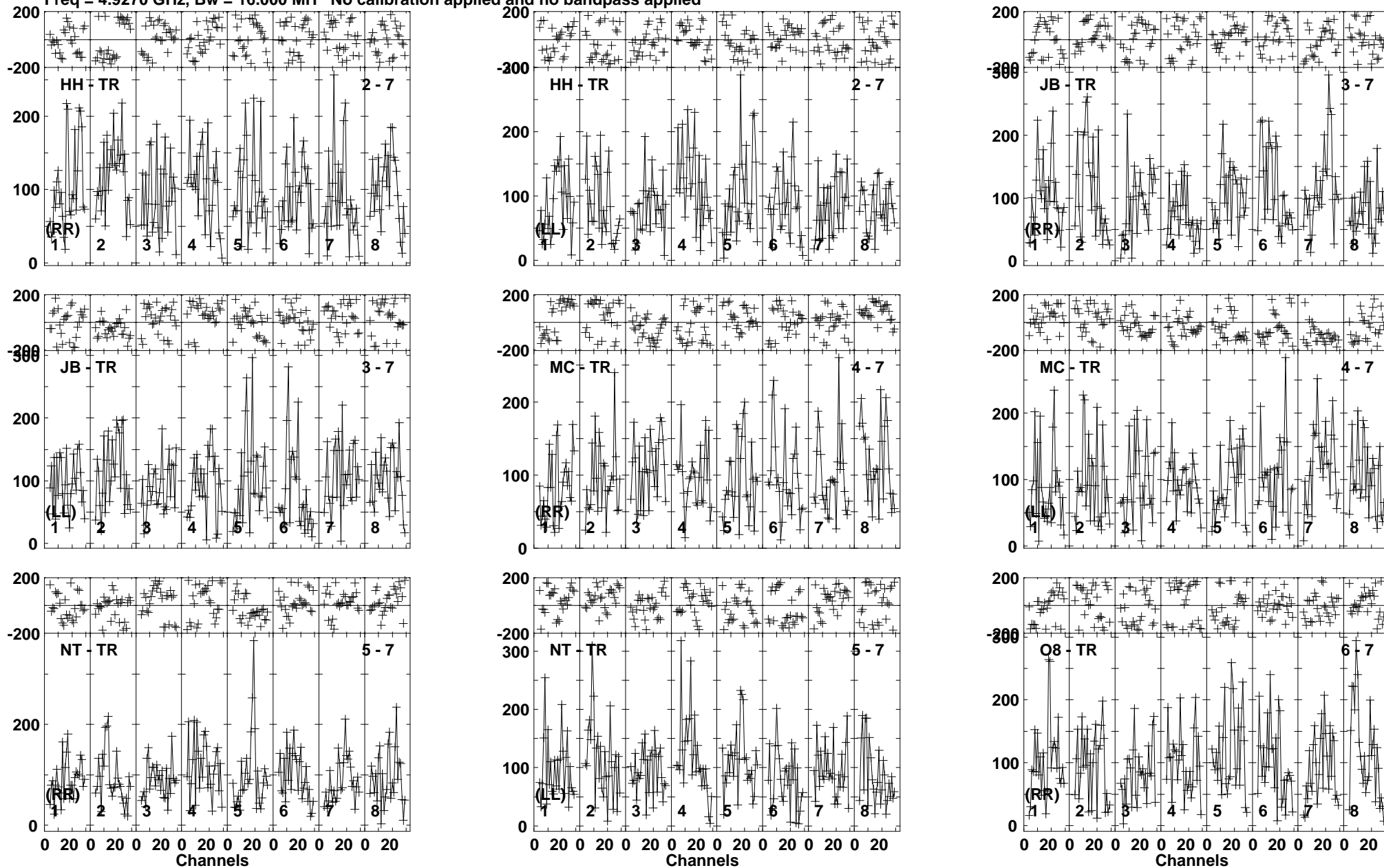
Lower frame: Micro Ampl Jy Top frame: Phas deg Vector averaged cross-power spectrum Baseline: HH (02) - TR (07) Timerange: 00/14:37:52 to 00/14:41:18
