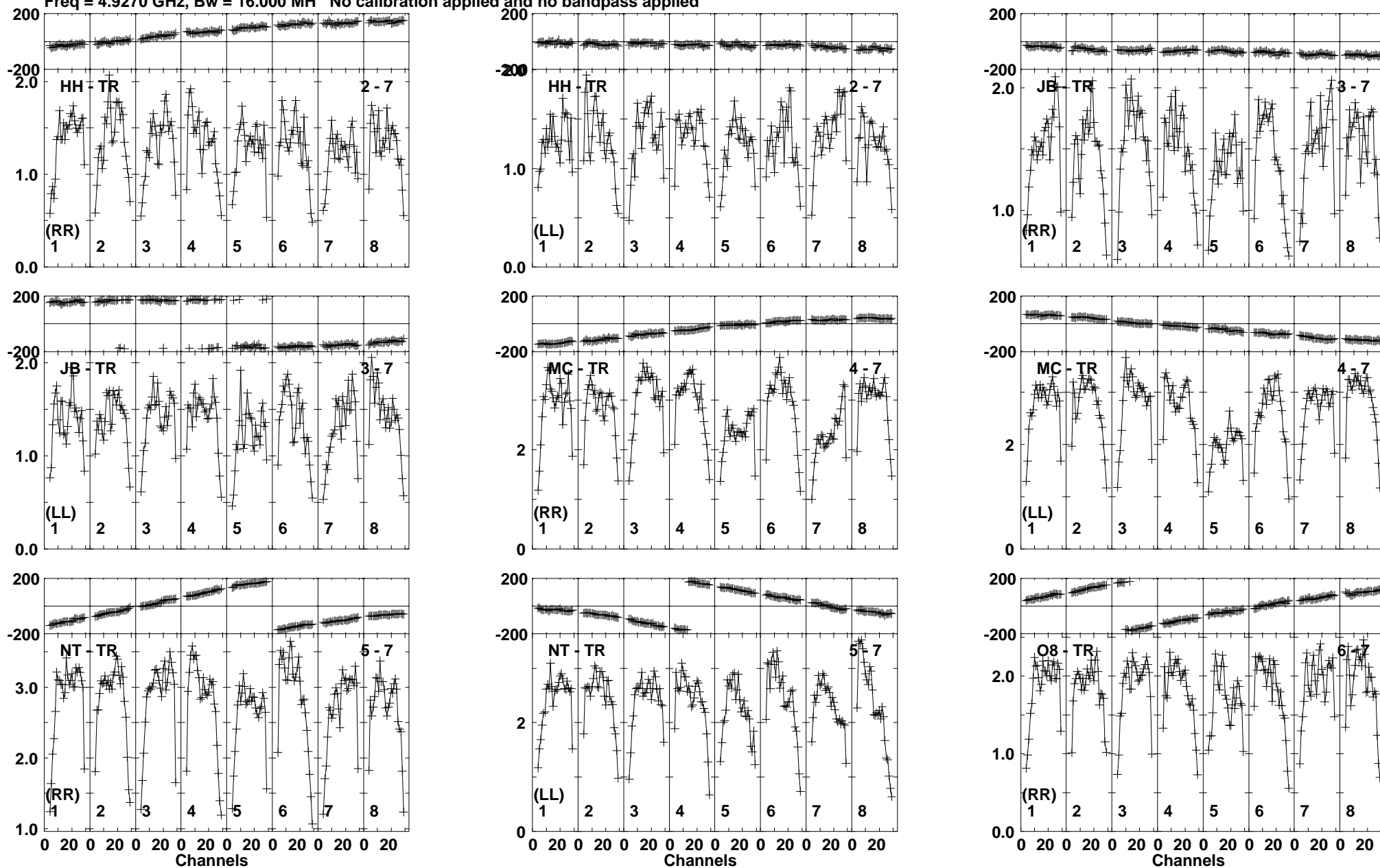
Lower frame: Milli Ampl Jy Top frame: Phas deg Vector averaged cross-power spectrum Baseline: HH (02) - TR (07) Timerange: 00/13:43:32 to 00/13:44:18
