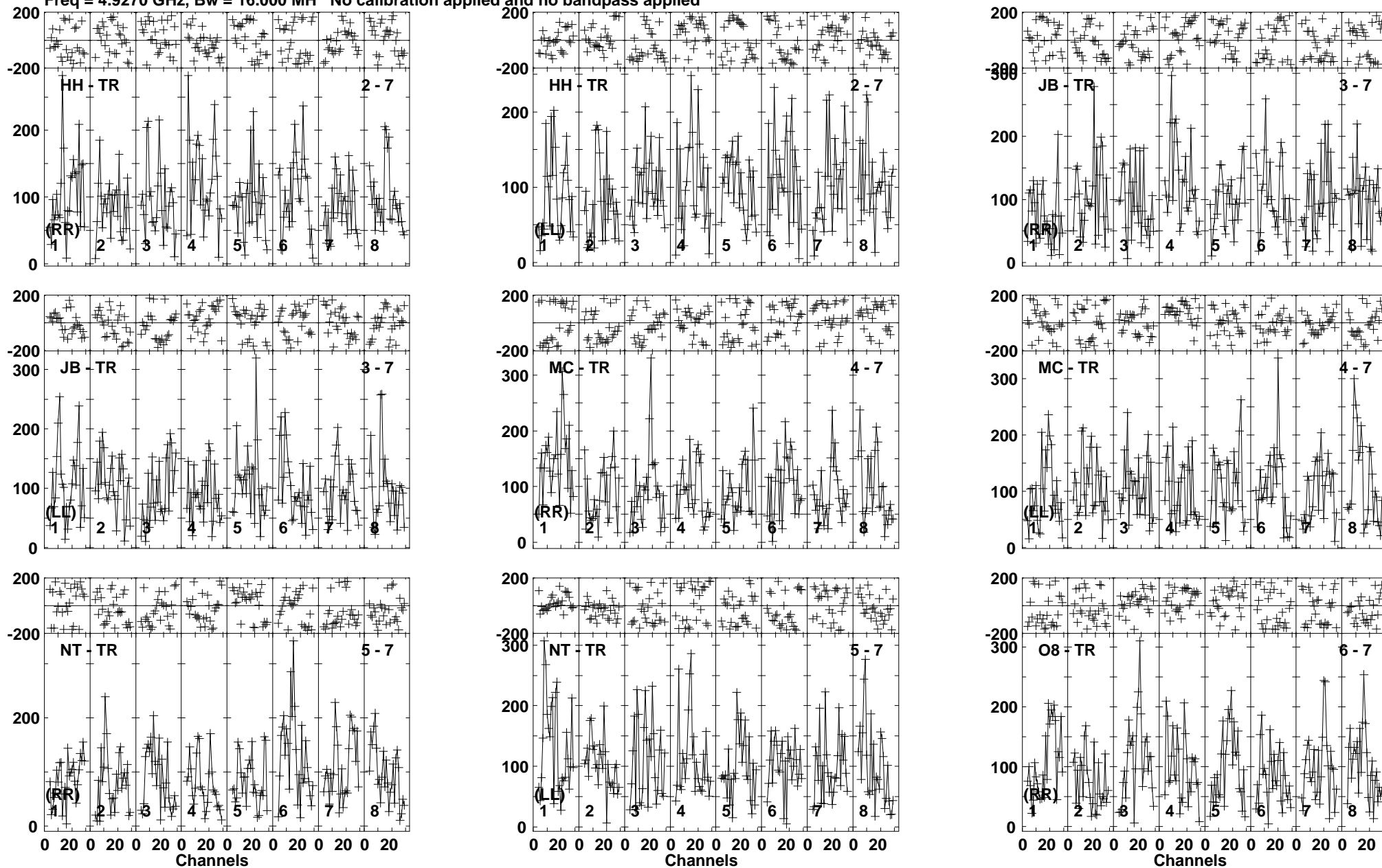
Lower frame: Micro Ampl Jy Top frame: Phas deg Vector averaged cross-power spectrum Baseline: HH (02) - TR (07) Timerange: 00/15:43:52 to 00/15:47:18
