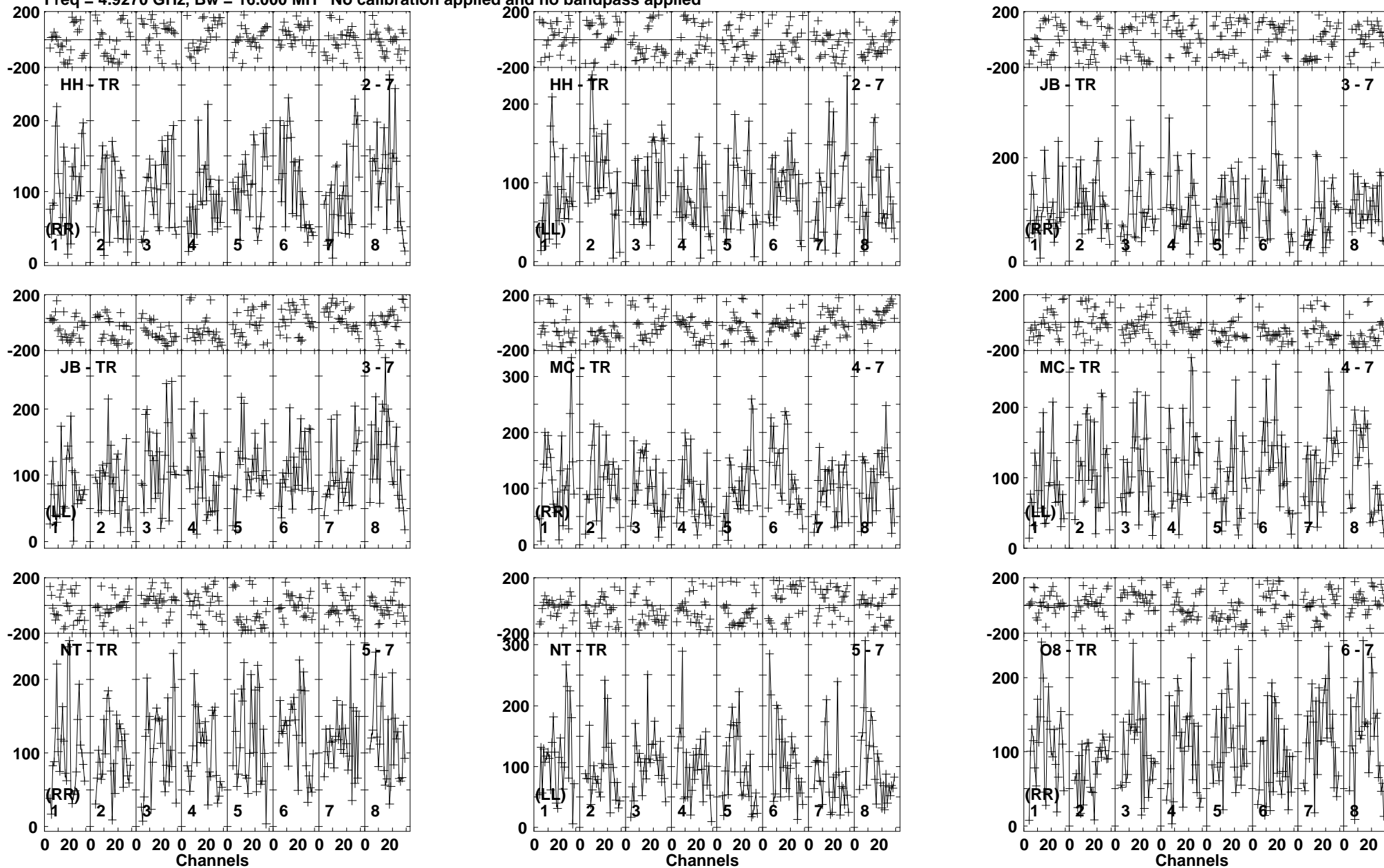
Lower frame: Micro Ampl Jy Top frame: Phas deg Vector averaged cross-power spectrum Baseline: HH (02) - TR (07) Timerange: 00/14:32:42 to 00/14:36:08
