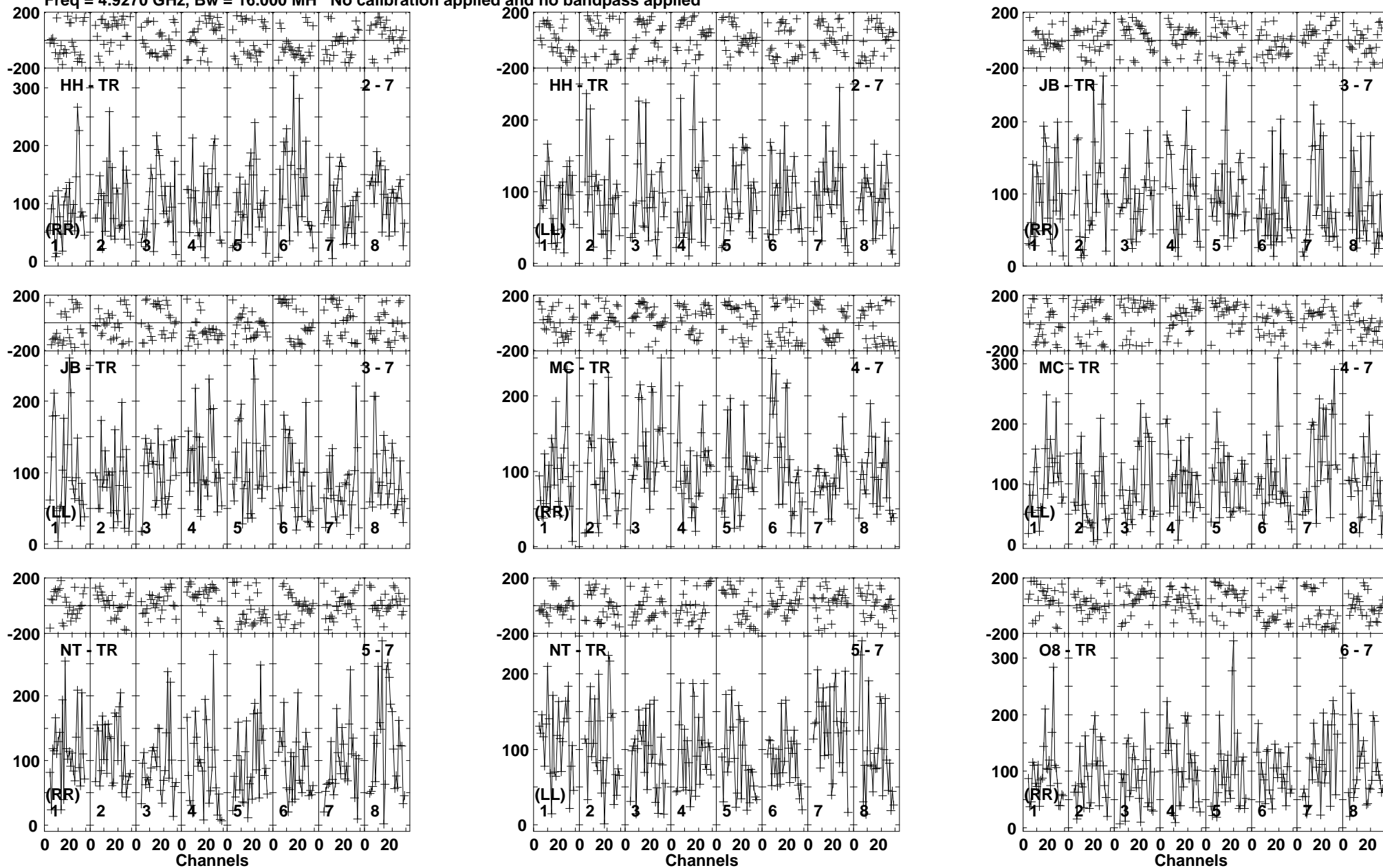
Lower frame: Micro Ampl Jy Top frame: Phas deg Vector averaged cross-power spectrum Baseline: HH (02) - TR (07) Timerange: 00/13:34:22 to 00/13:37:48
