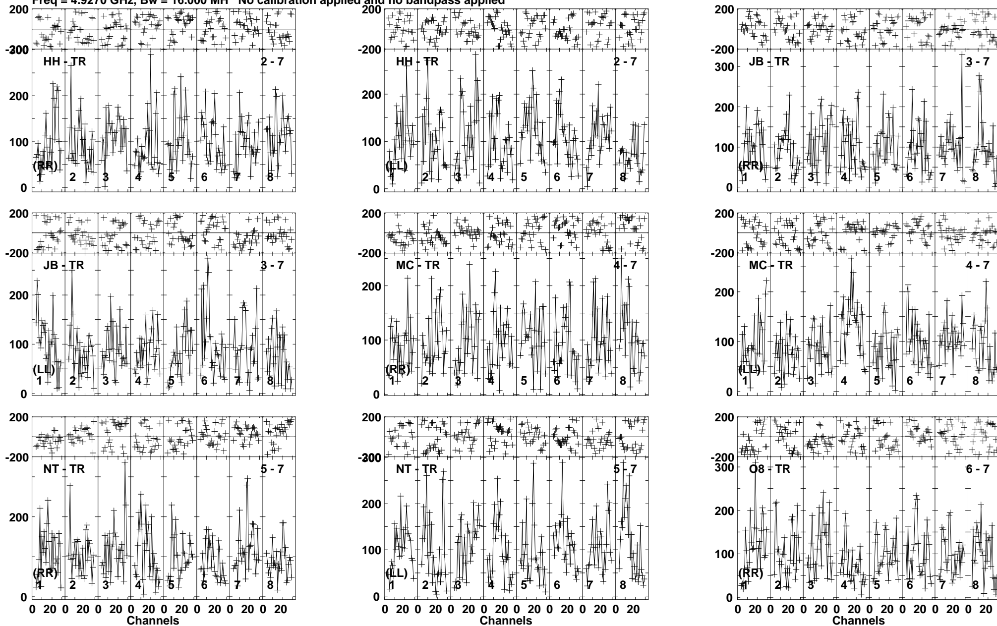
Lower frame: Micro Ampl Jy Top frame: Phas deg Vector averaged cross-power spectrum Baseline: HH (02) - TR (07) Timerange: 00/15:18:32 to 00/15:21:58
