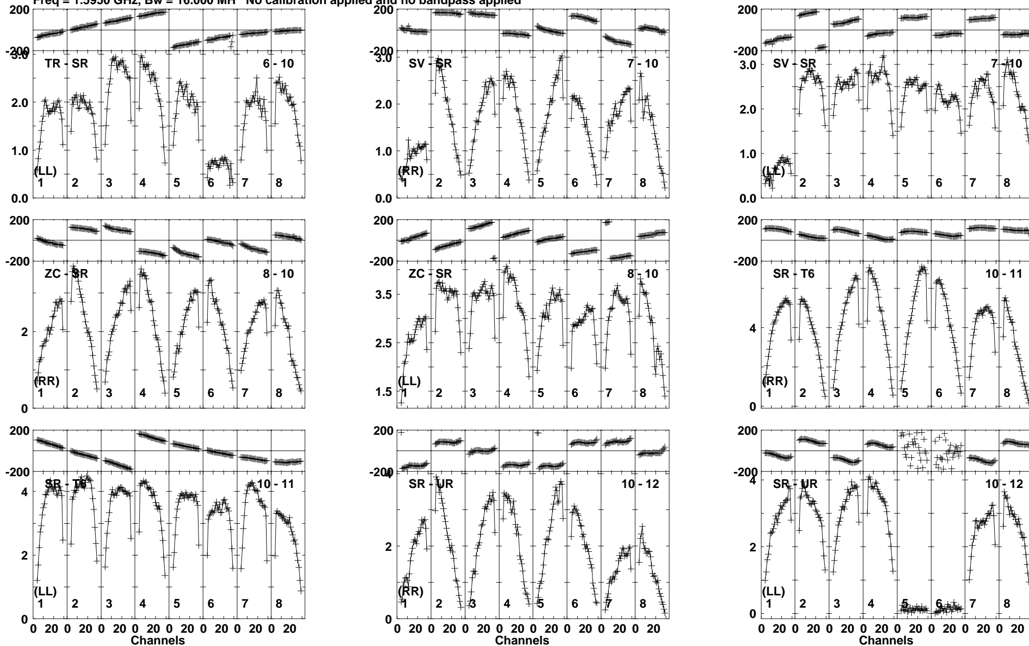
Lower frame: Milli Ampl Jy Top frame: Phas deg Vector averaged cross-power spectrum Baseline: TR (06) - SR (10) Timerange: 00/00:23:00 to 00/00:24:30
