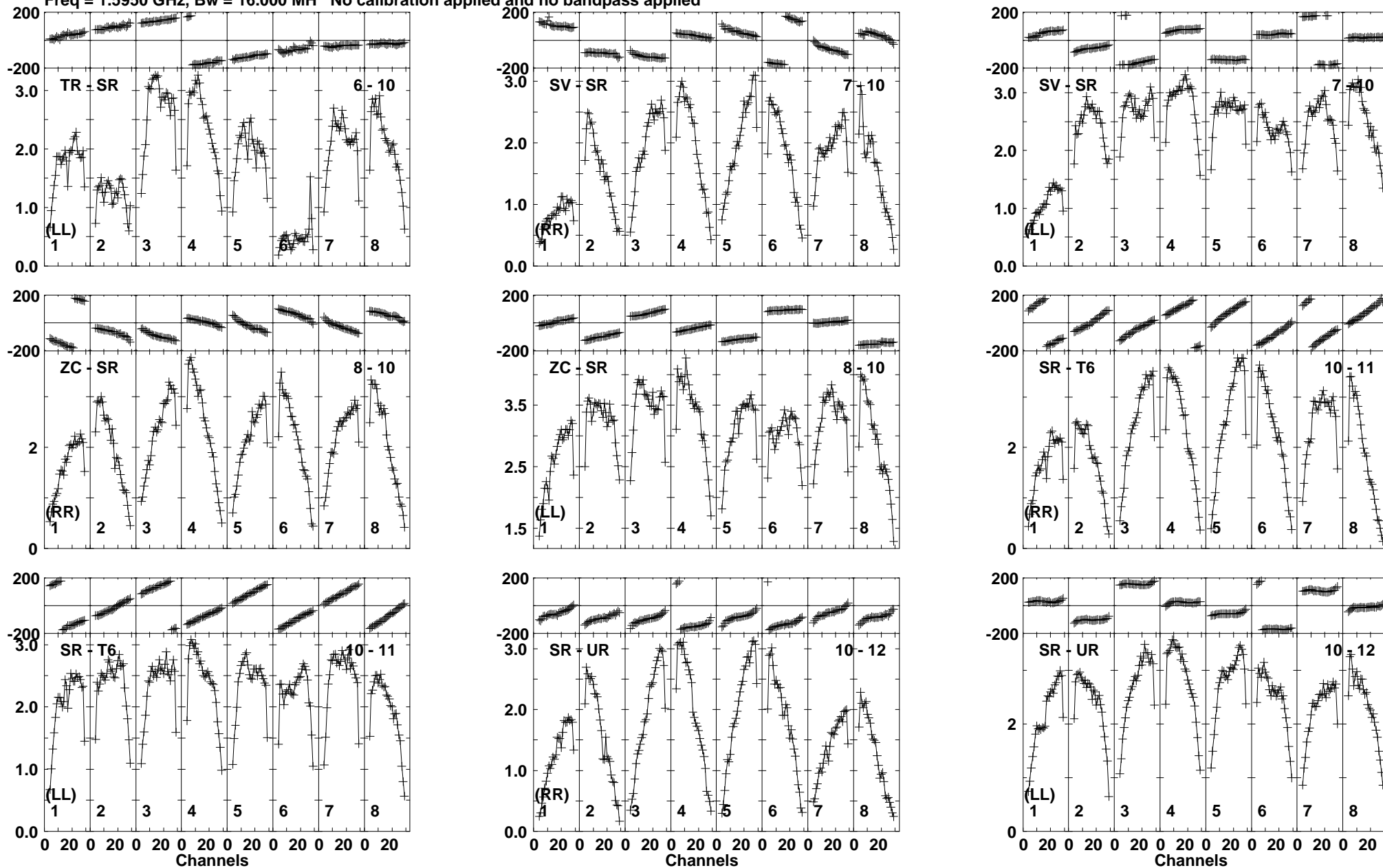
Lower frame: Milli Ampl Jy Top frame: Phas deg Vector averaged cross-power spectrum Baseline: TR (06) - SR (10) Timerange: 00/03:40:07 to 00/03:41:30
