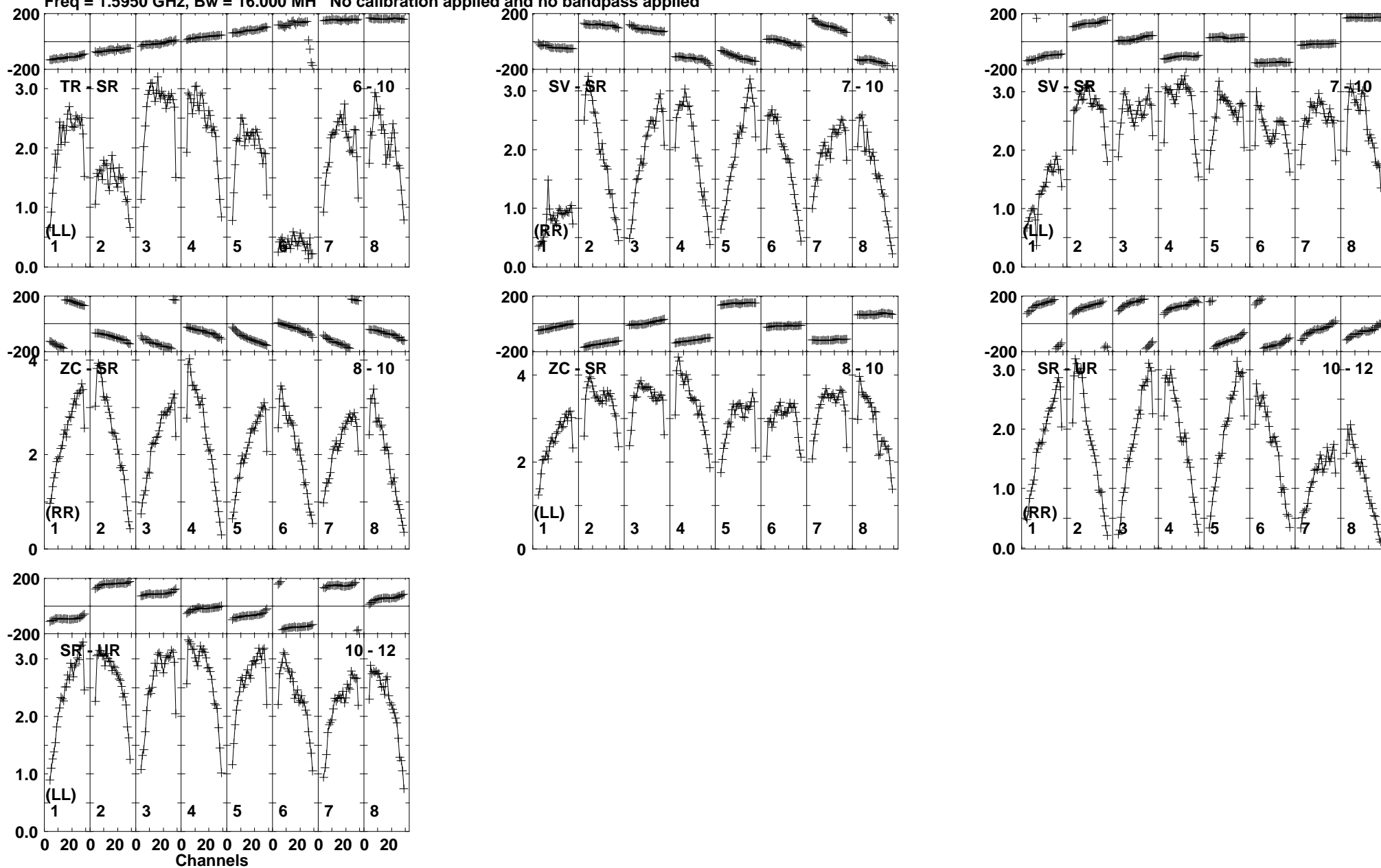
Lower frame: Milli Ampl Jy Top frame: Phas deg Vector averaged cross-power spectrum Baseline: TR (06) - SR (10) Timerange: 00/04:23:08 to 00/04:24:30
