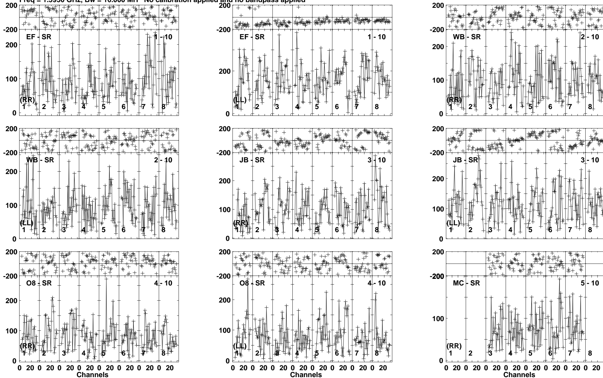
Lower frame: Micro Ampl Jy Top frame: Phas deg Vector averaged cross-power spectrum Baseline: EF (01) - SR (10) Timerange: 00/00:18:38 to 00/00:22:00
