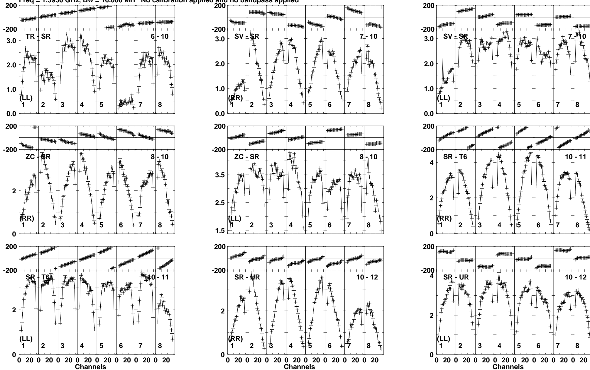
Lower frame: Milli Ampl Jy Top frame: Phas deg Vector averaged cross-power spectrum Baseline: TR (06) - SR (10) Timerange: 00/03:24:07 to 00/03:25:30
