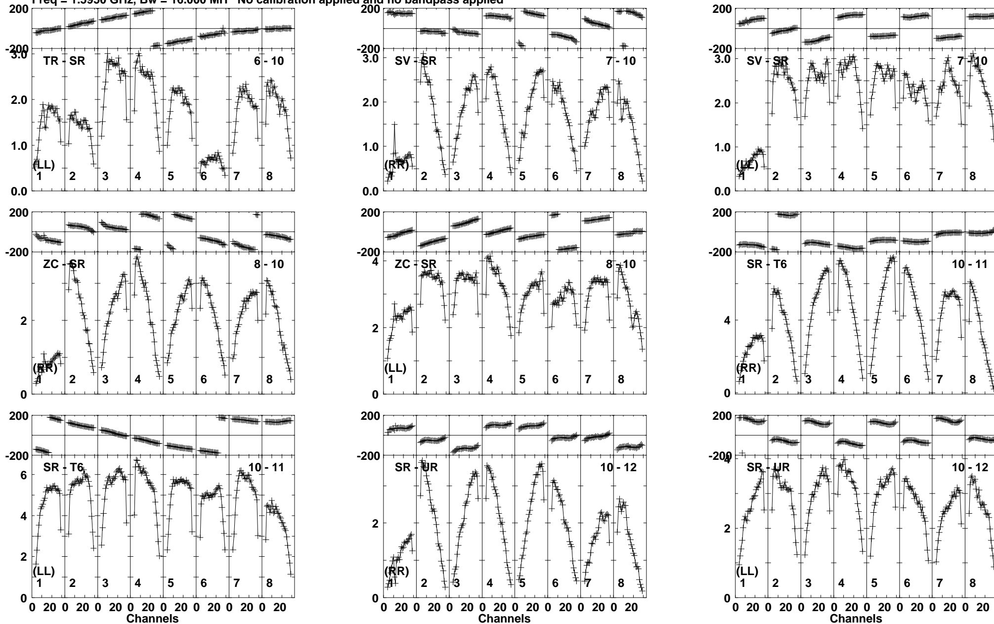
Lower frame: Milli Ampl Jy Top frame: Phas deg Vector averaged cross-power spectrum Baseline: TR (06) - SR (10) Timerange: 00/00:45:00 to 00/00:46:29
