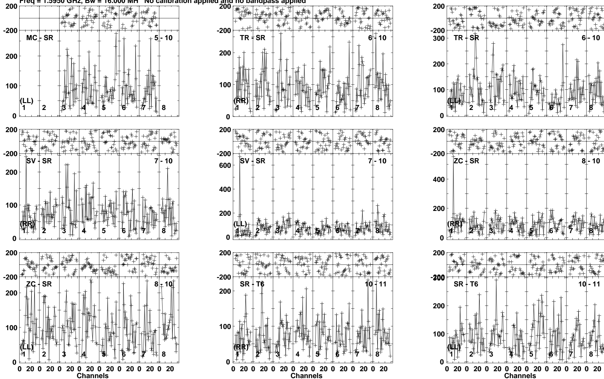
Lower frame: Micro Ampl Jy Top frame: Phas deg Vector averaged cross-power spectrum Baseline: MC (05) - SR (10) Timerange: 00/03:04:33 to 00/03:08:00
