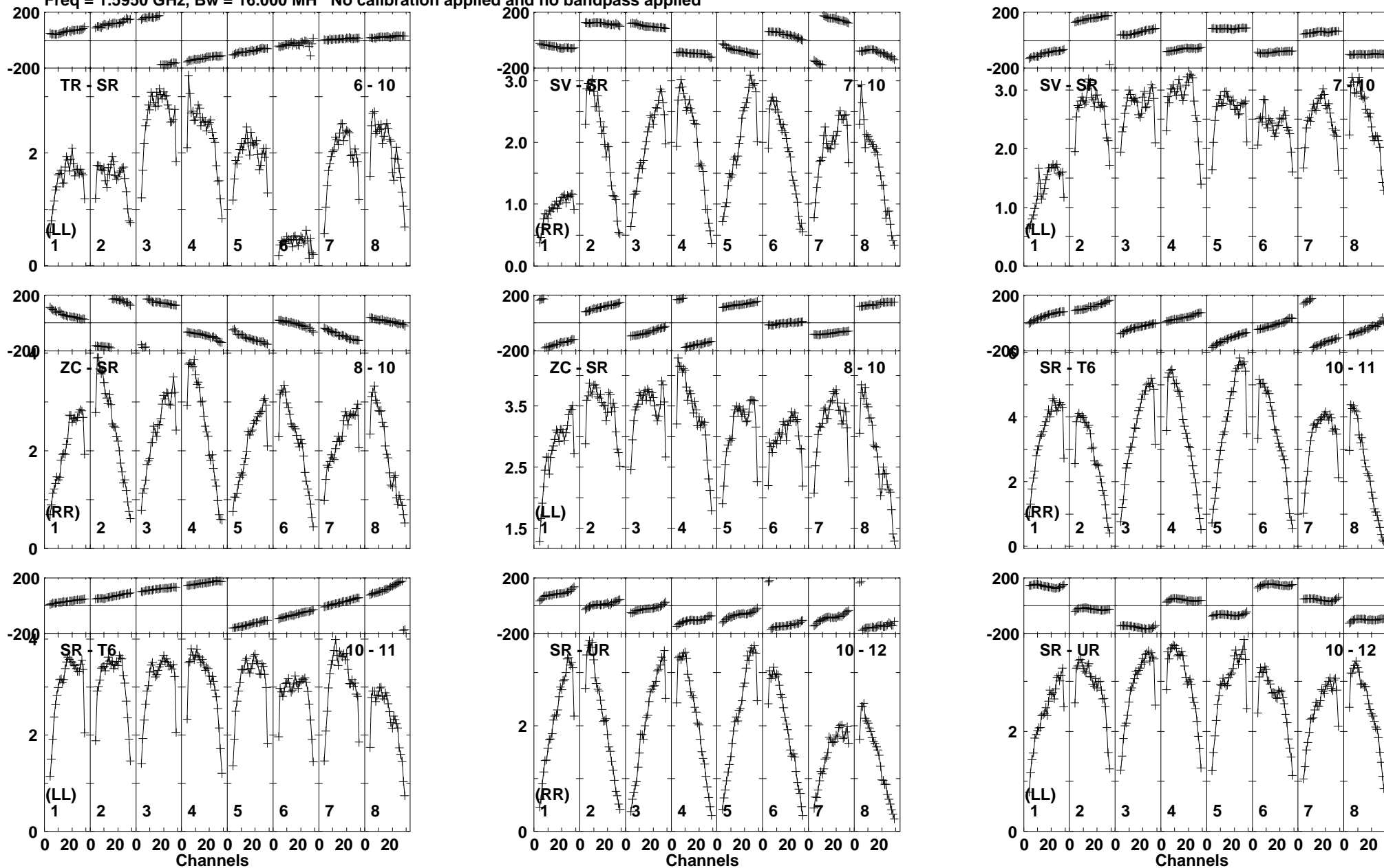
Lower frame: Milli Ampl Jy Top frame: Phas deg Vector averaged cross-power spectrum Baseline: TR (06) - SR (10) Timerange: 00:02:47:07 to 00:02:48:30
