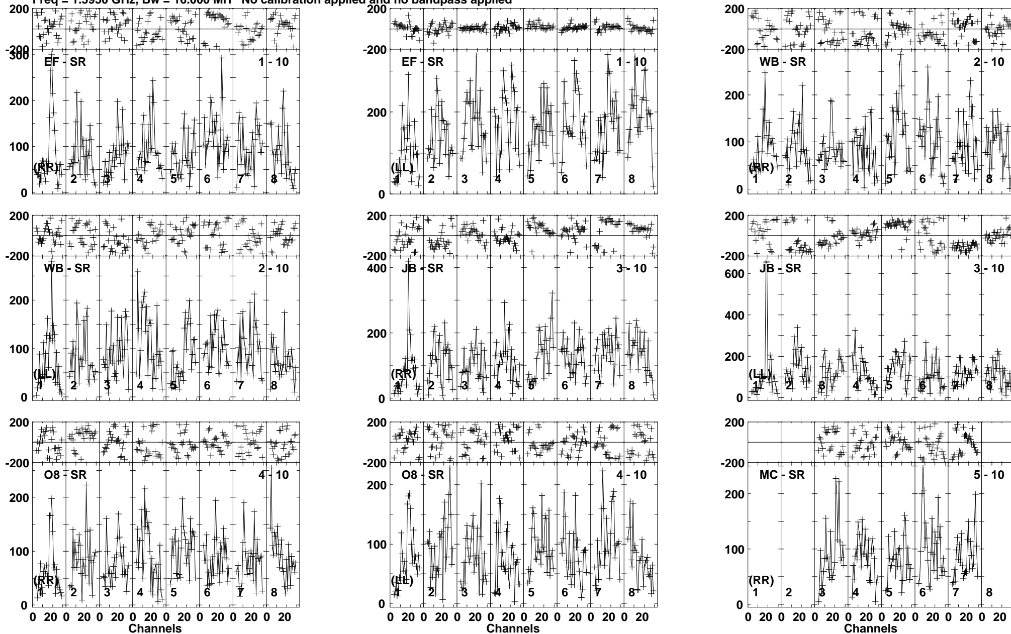
Lower frame: Micro Ampl Jy Top frame: Phas deg Vector averaged cross-power spectrum Baseline: EF (01) - SR (10) Timerange: 00/02:16:38 to 00/02:20:00
