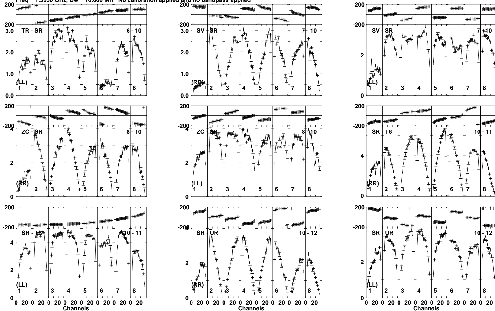
Lower frame: Milli Ampl Jy Top frame: Phas deg Vector averaged cross-power spectrum Baseline: TR (06) - SR (10) Timerange: 00/02:20:08 to 00/02:21:29
