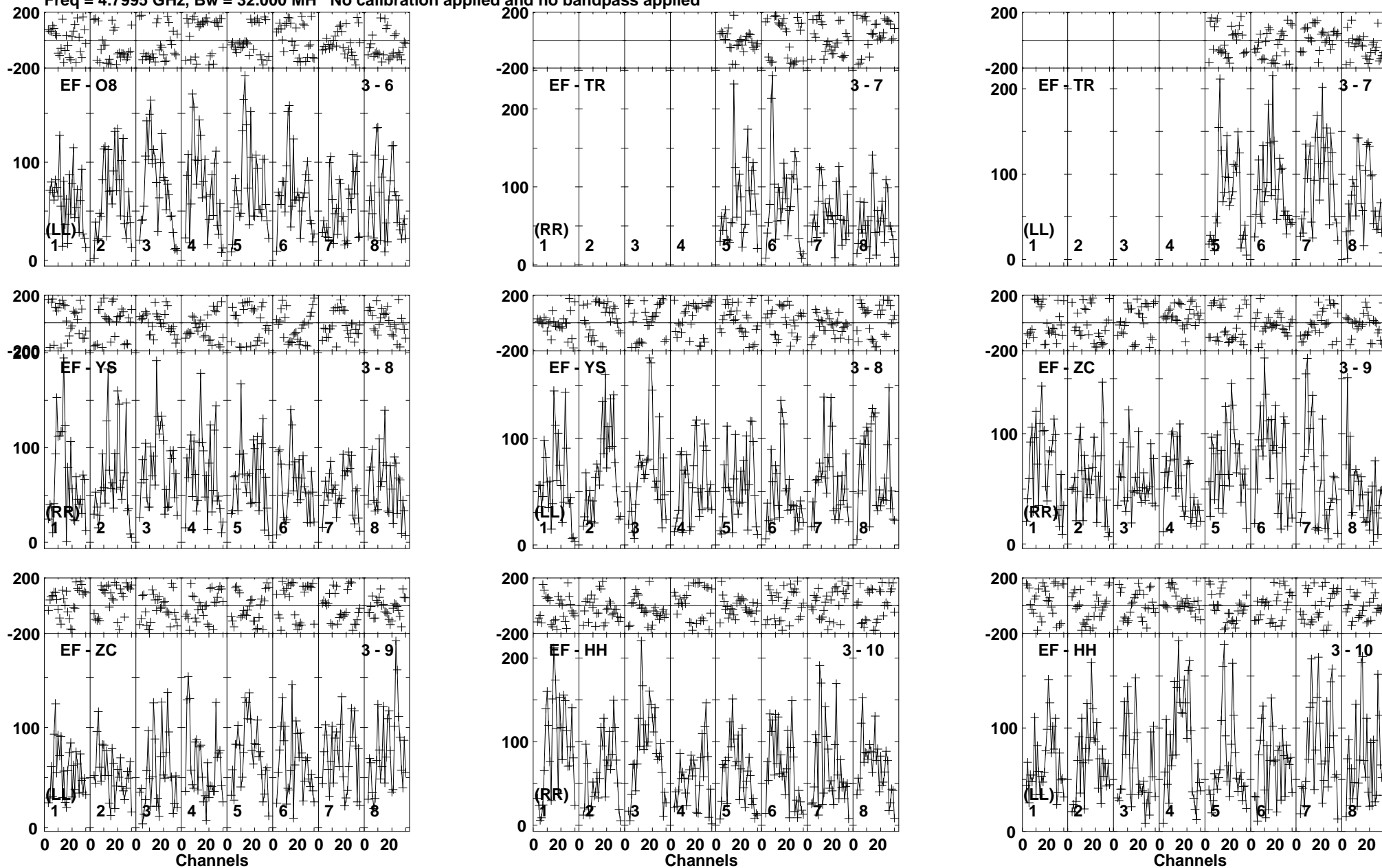
Lower frame: Micro Ampl Jy Top frame: Phas deg Vector averaged cross-power spectrum Baseline: EF (03) - O8 (06) Timerange: 00/15:05:04 to 00/15:07:08
