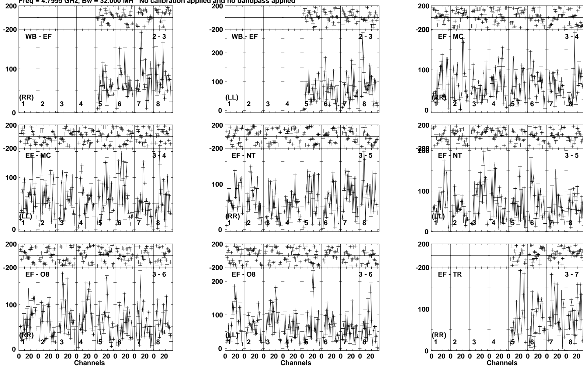
Lower frame: Micro Ampl Jy Top frame: Phas deg Vector averaged cross-power spectrum Baseline: WB (02) - EF (03) Timerange: 00/15:01:36 to 00/15:03:38
