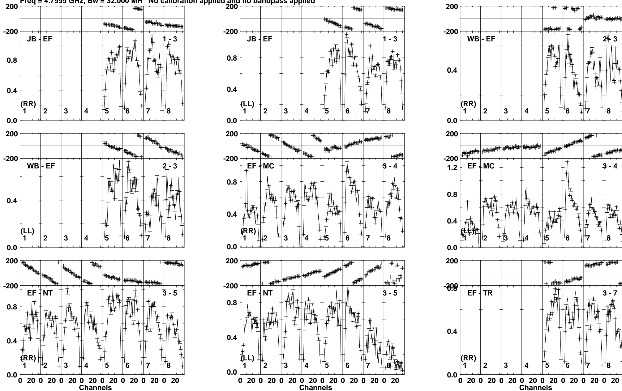
Lower frame: Milli Ampl Jy Top frame: Phas deg Vector averaged cross-power spectrum Baseline: JB (01) - EF (03) Timerange: 00/18:01:11 to 00/18:01:59
