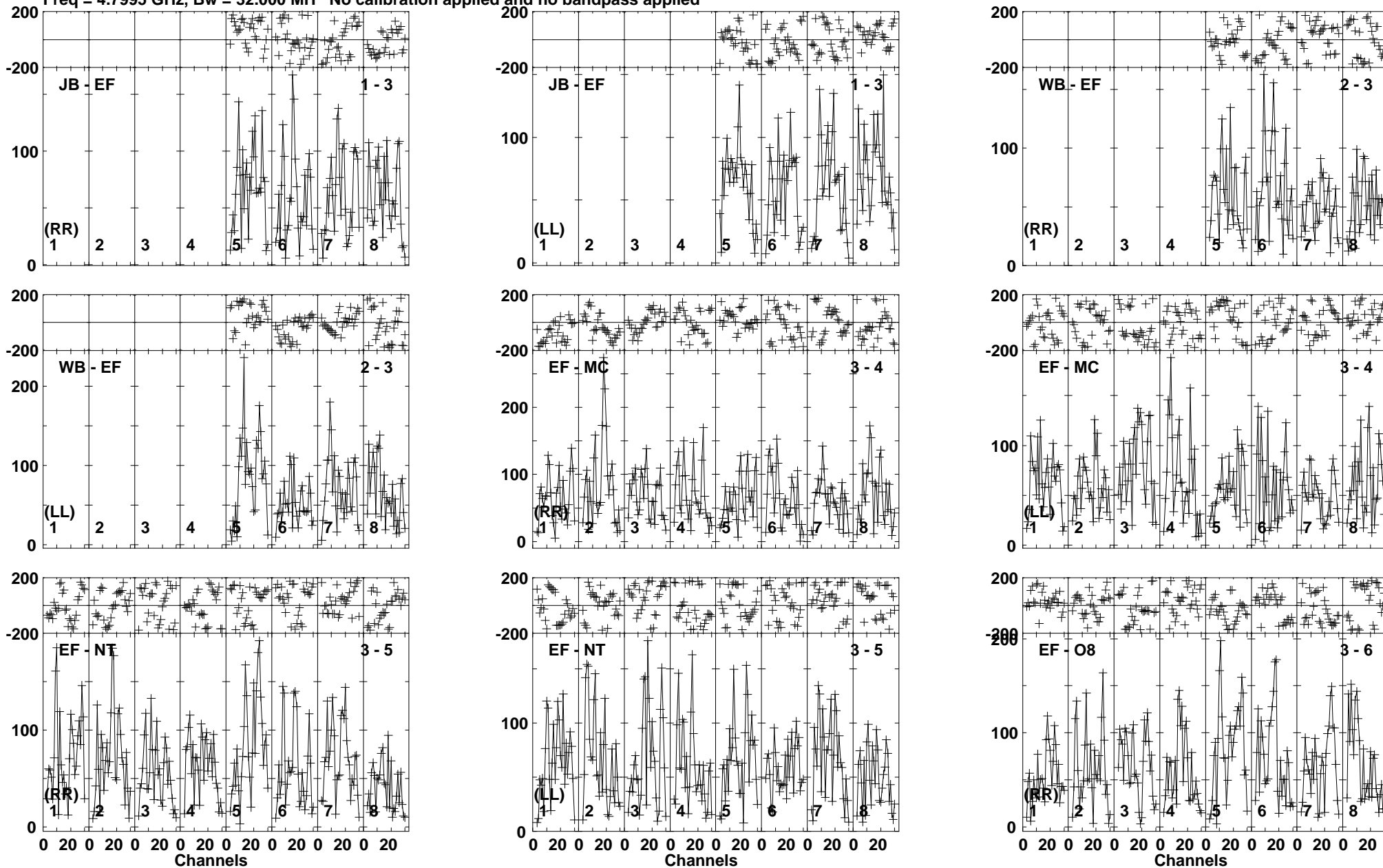
Lower frame: Micro Ampl Jy Top frame: Phas deg Vector averaged cross-power spectrum Baseline: JB (01) - EF (03) Timerange: 00/14:33:34 to 00/14:35:38
