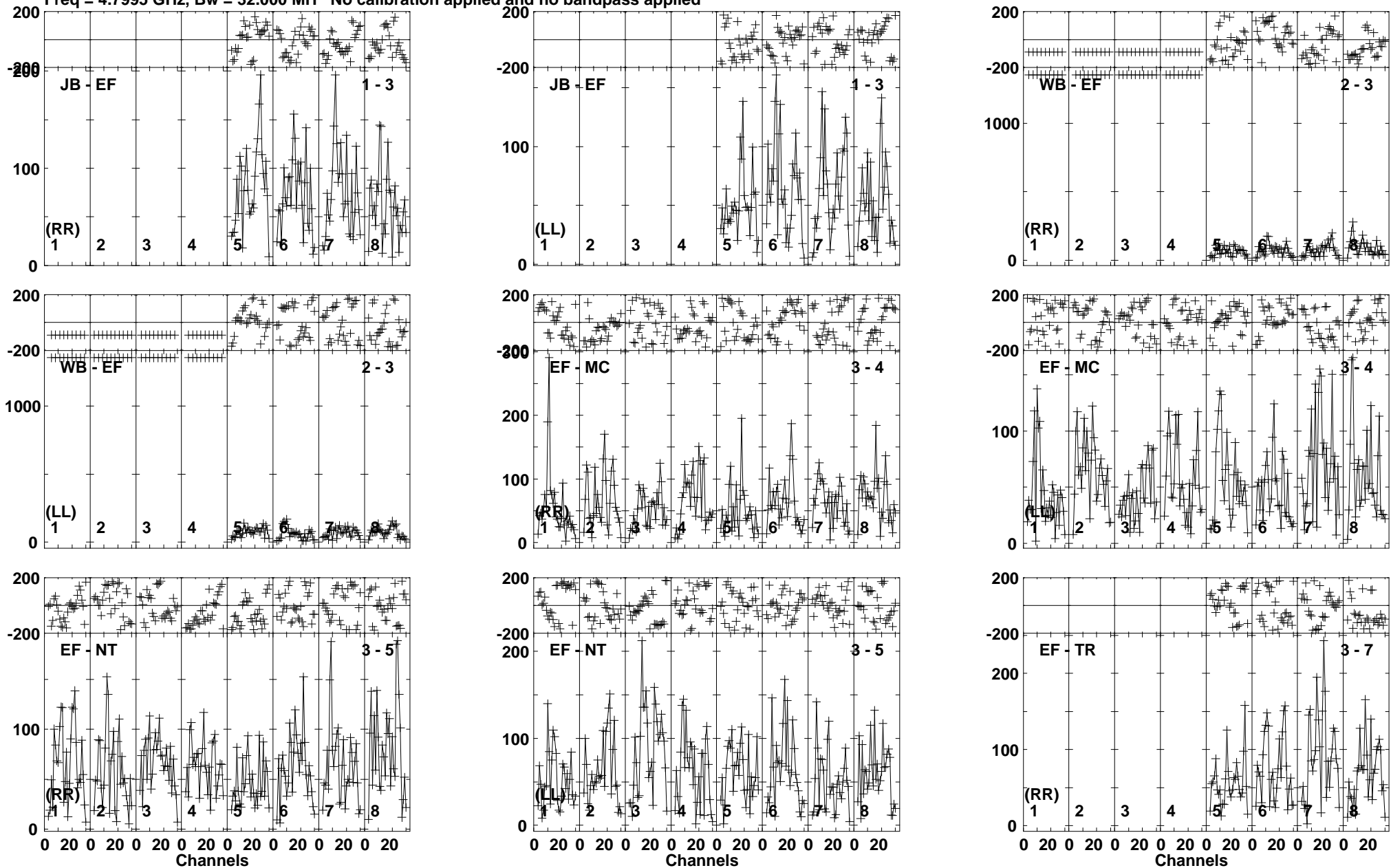
Lower frame: Micro Ampl Jy Top frame: Phas deg Vector averaged cross-power spectrum Baseline: JB (01) - EF (03) Timerange: 00/17:41:04 to 00/17:43:08
