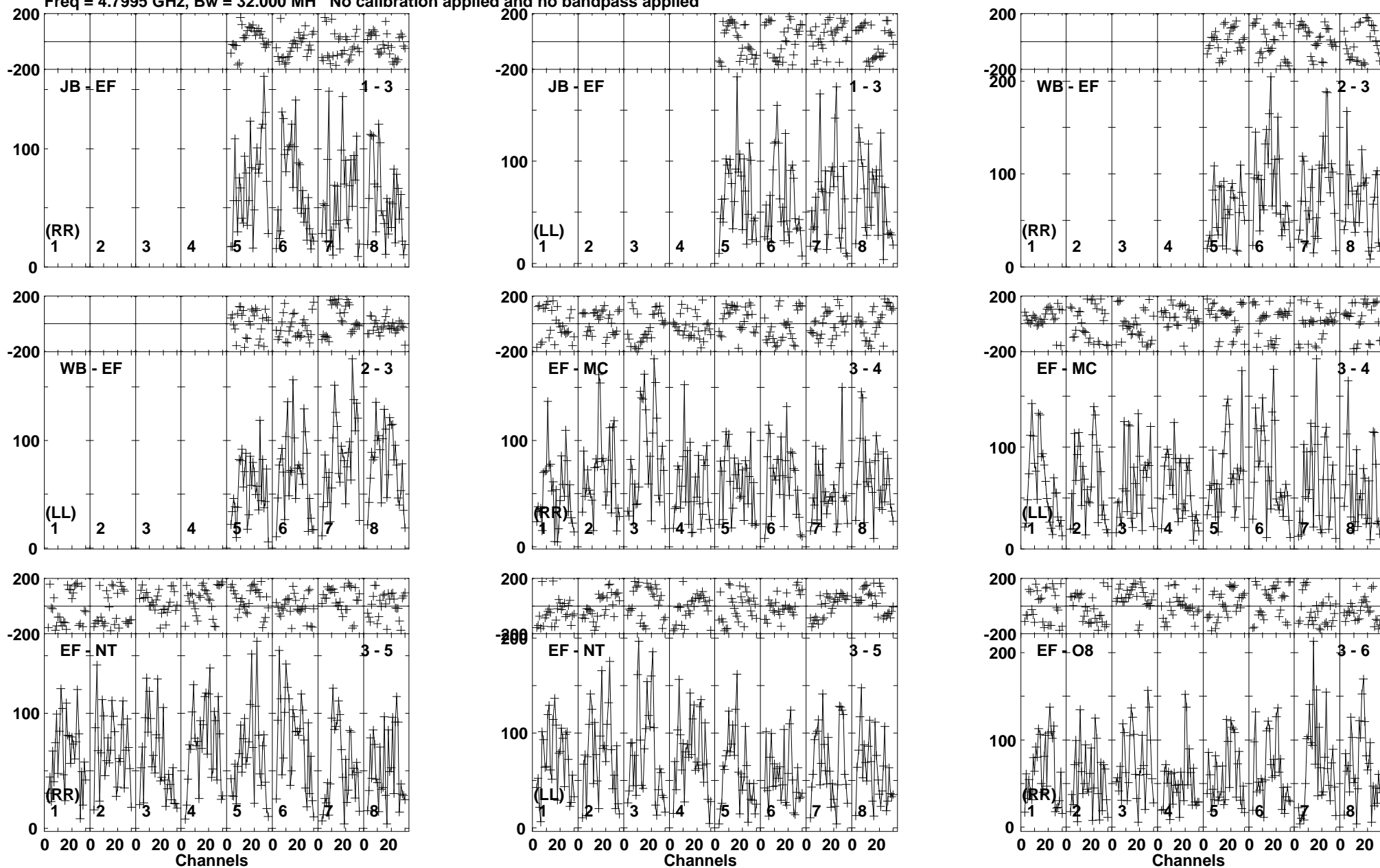
Lower frame: Micro Ampl Jy Top frame: Phas deg Vector averaged cross-power spectrum Baseline: JB (01) - EF (03) Timerange: 00/16:48:34 to 00/16:50:38
