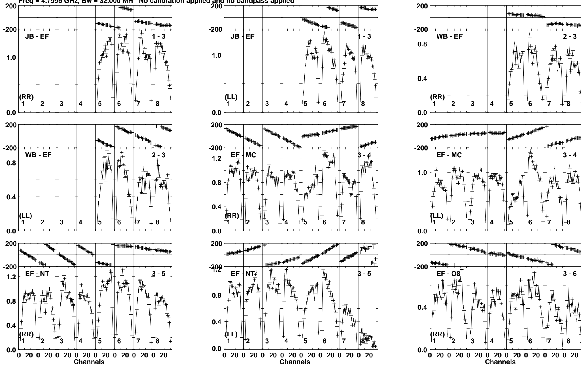
Lower frame: Milli Ampl Jy Top frame: Phas deg Vector averaged cross-power spectrum Baseline: JB (01) - EF (03) Timerange: 00/16:33:14 to 00/16:34:28
