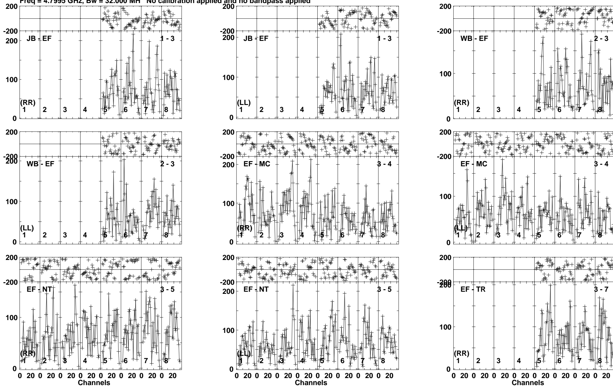
Lower frame: Micro Ampl Jy Top frame: Phas deg Vector averaged cross-power spectrum Baseline: JB (01) - EF (03) Timerange: 00/13:51:34 to 00/13:53:38
