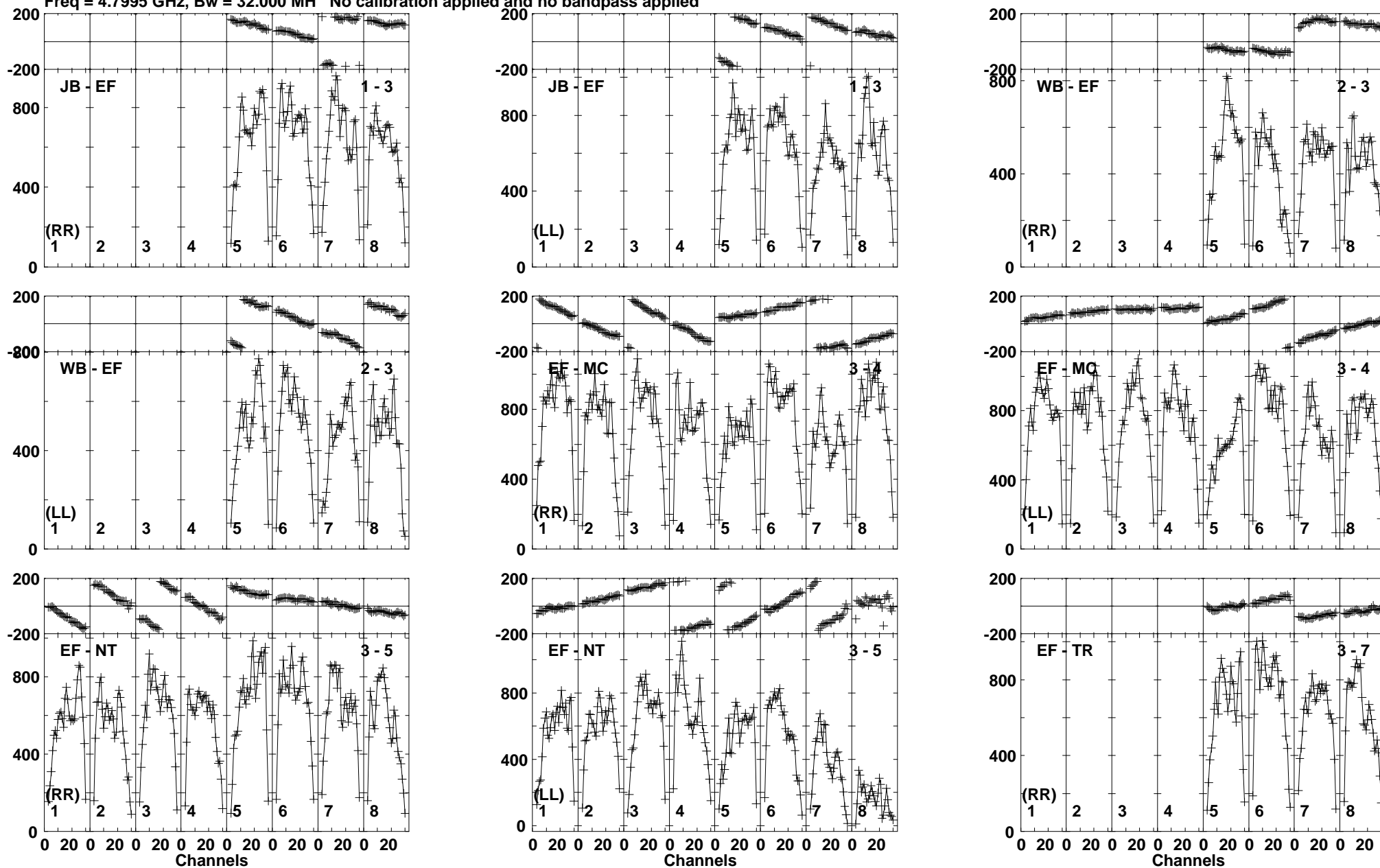
Lower frame: Micro Ampl Jy Top frame: Phas deg Vector averaged cross-power spectrum Baseline: JB (01) - EF (03) Timerange: 00/13:50:41 to 00/13:51:29
