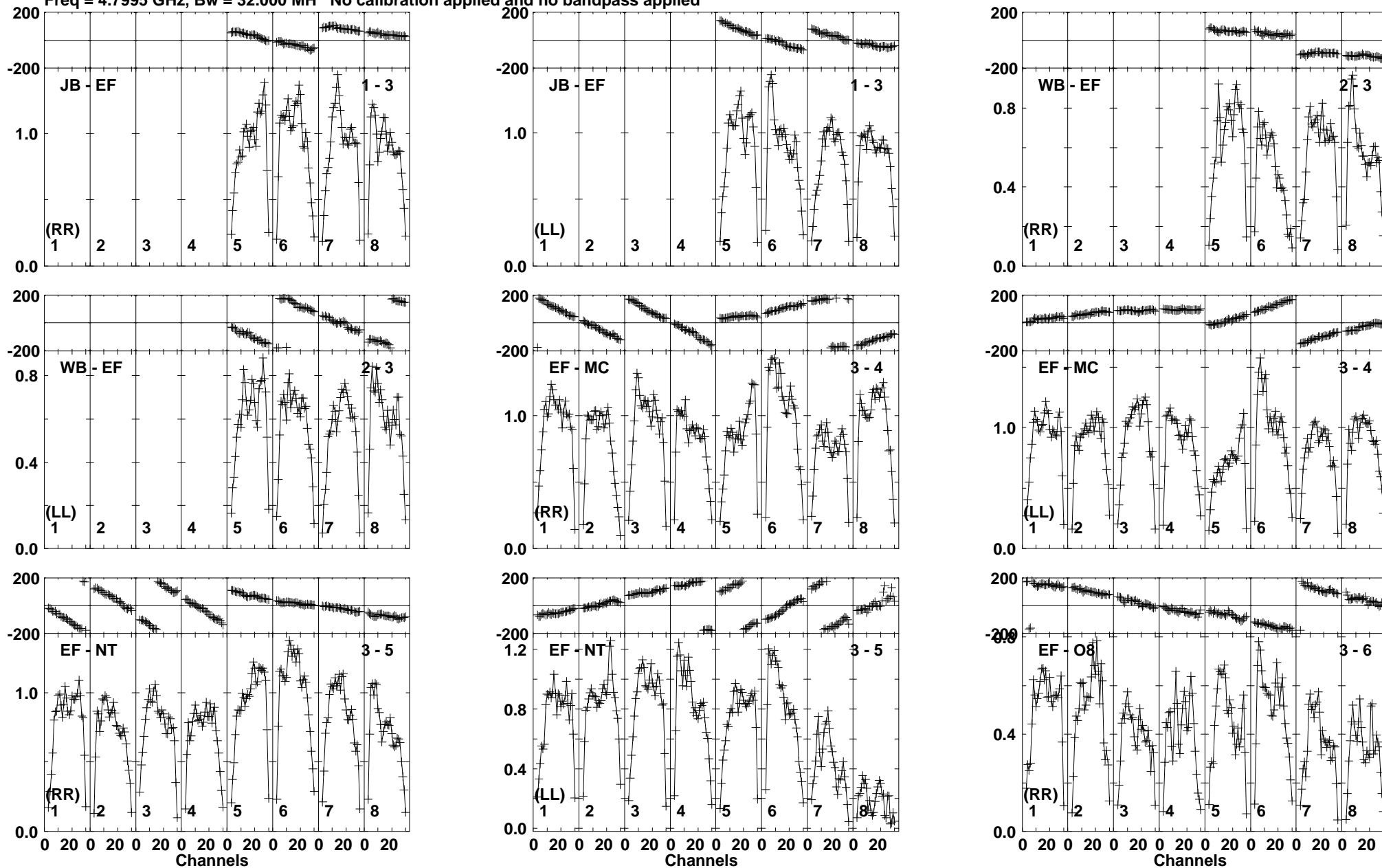
Lower frame: Milli Ampl Jy Top frame: Phas deg Vector averaged cross-power spectrum Baseline: JB (01) - EF (03) Timerange: 00/15:25:11 to 00/15:25:59
