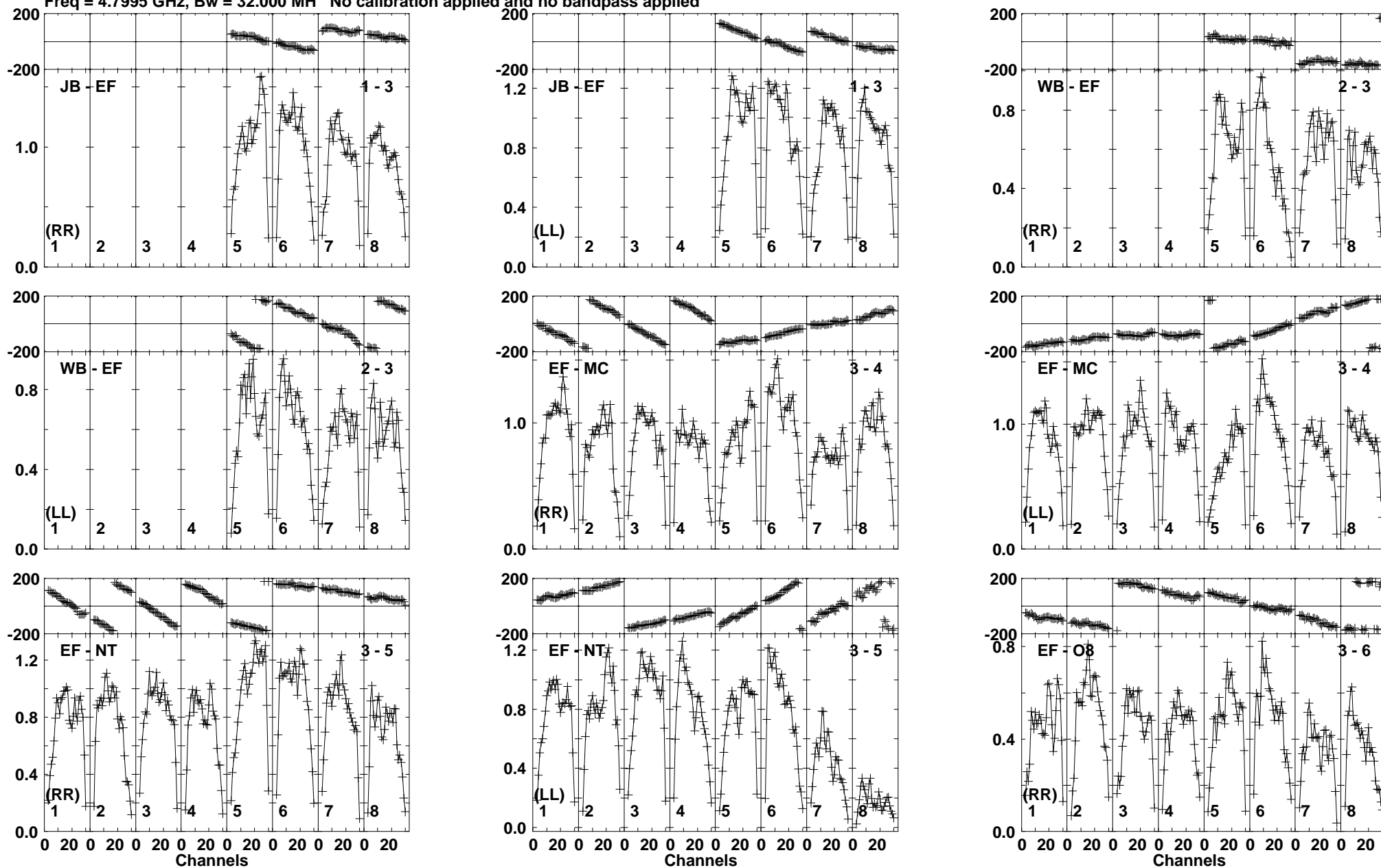
Lower frame: Milli Ampl Jy Top frame: Phas deg Vector averaged cross-power spectrum Baseline: JB (01) - EF (03) Timerange: 00/15:47:31 to 00/15:48:59
