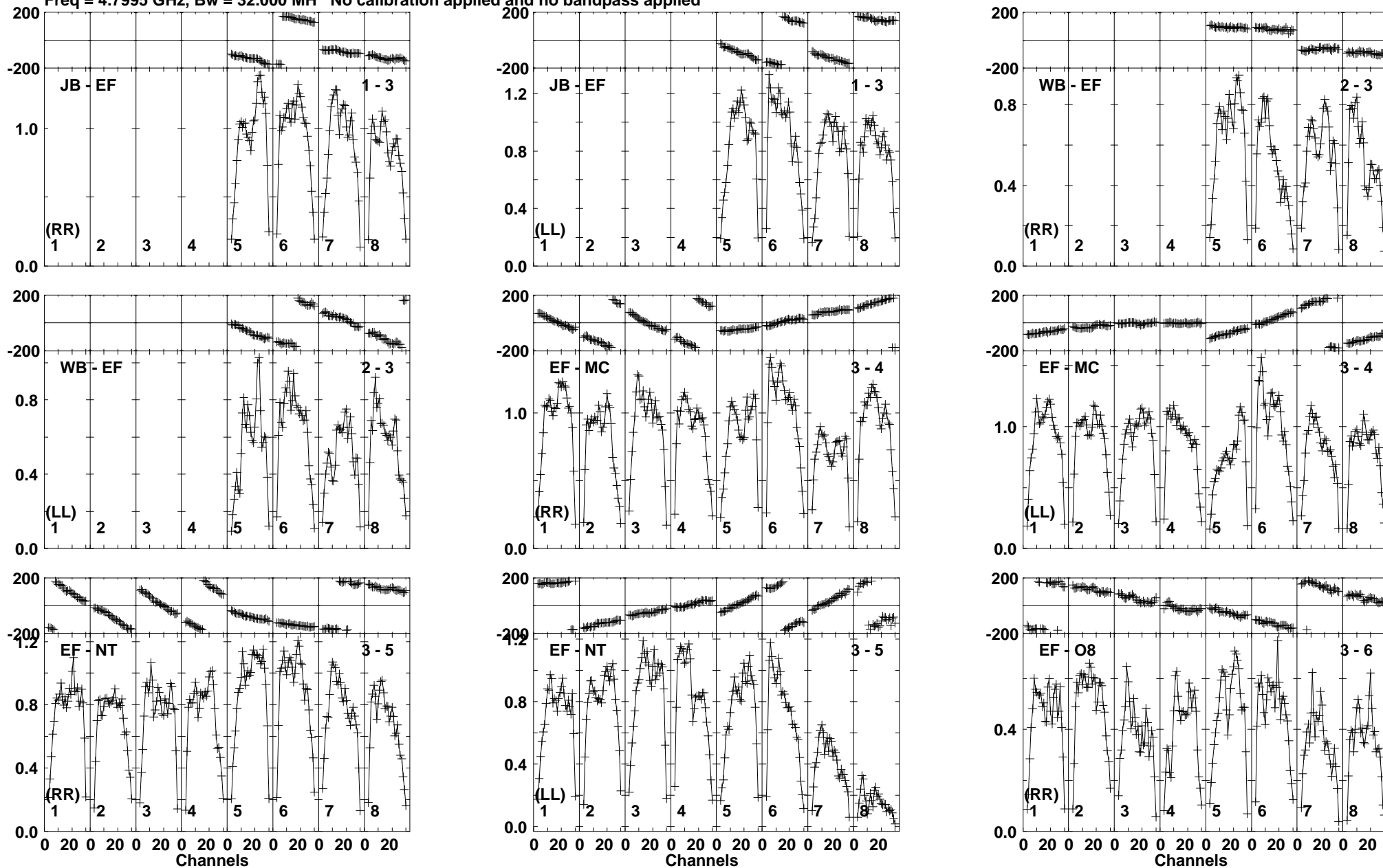
Lower frame: Milli Ampl Jy Top frame: Phas deg Vector averaged cross-power spectrum Baseline: JB (01) - EF (03) Timerange: 00/15:10:44 to 00/15:11:58
