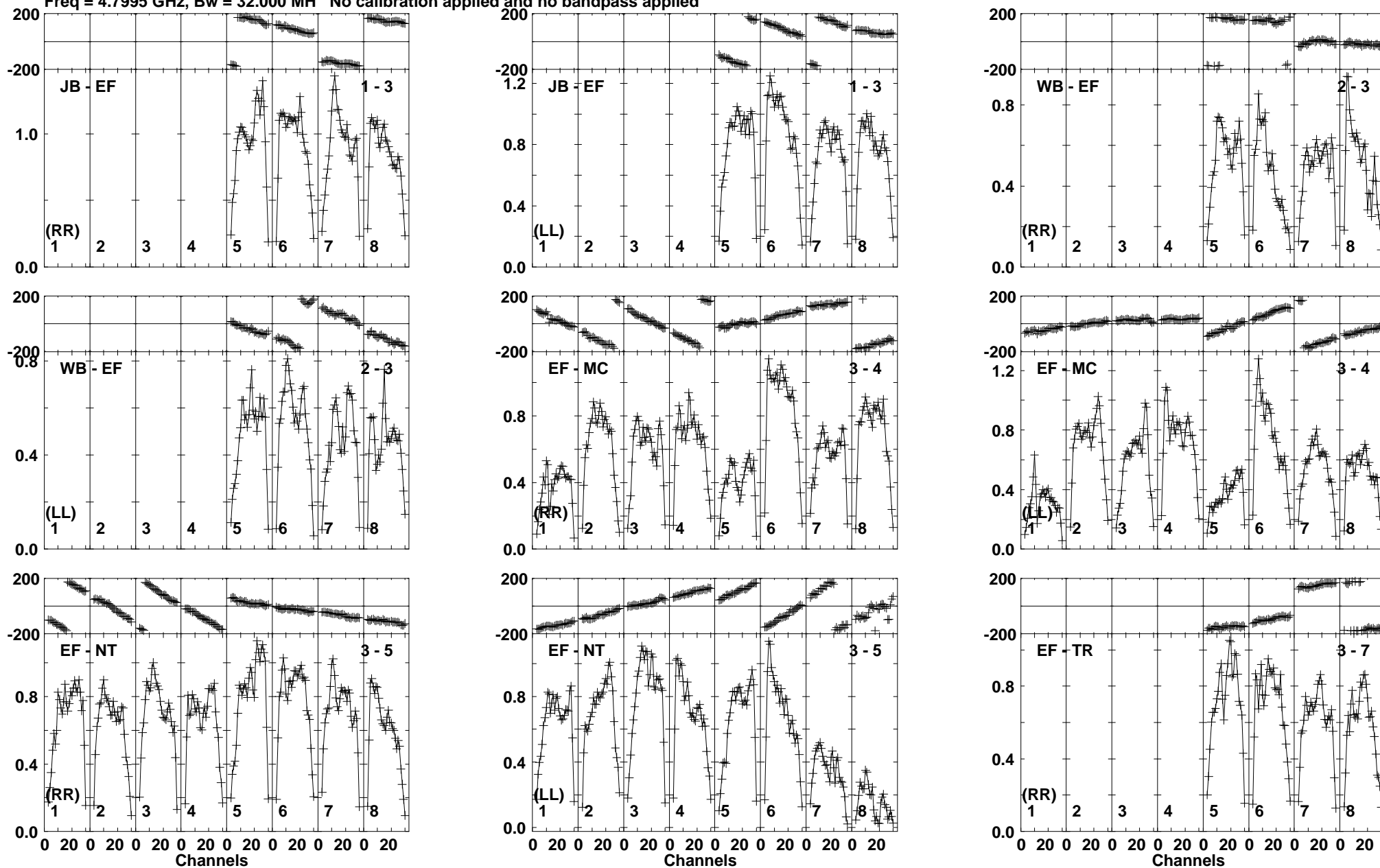
Lower frame: Milli Ampl Jy Top frame: Phas deg Vector averaged cross-power spectrum Baseline: JB (01) - EF (03) Timerange: 00/17:36:14 to 00/17:37:28
