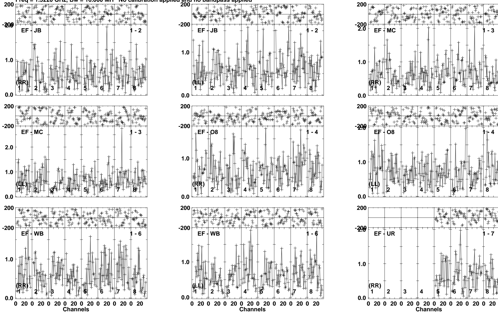
Lower frame: Milli Ampl Jy Top frame: Phas deg Vector averaged cross-power spectrum Baseline: EF (01) - JB (02) Timerange: 00/19:17:20 to 00/19:20:36
