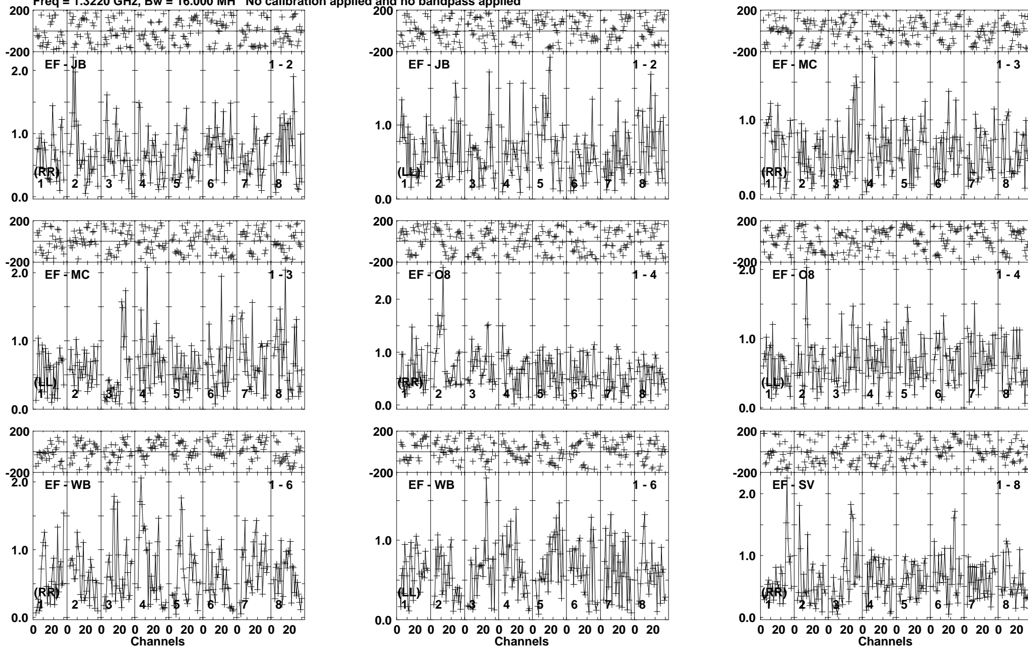
Lower frame: Milli Ampl Jy Top frame: Phas deg Vector averaged cross-power spectrum Baseline: EF (01) - JB (02) Timerange: 00/22:17:16 to 00/22:20:36
