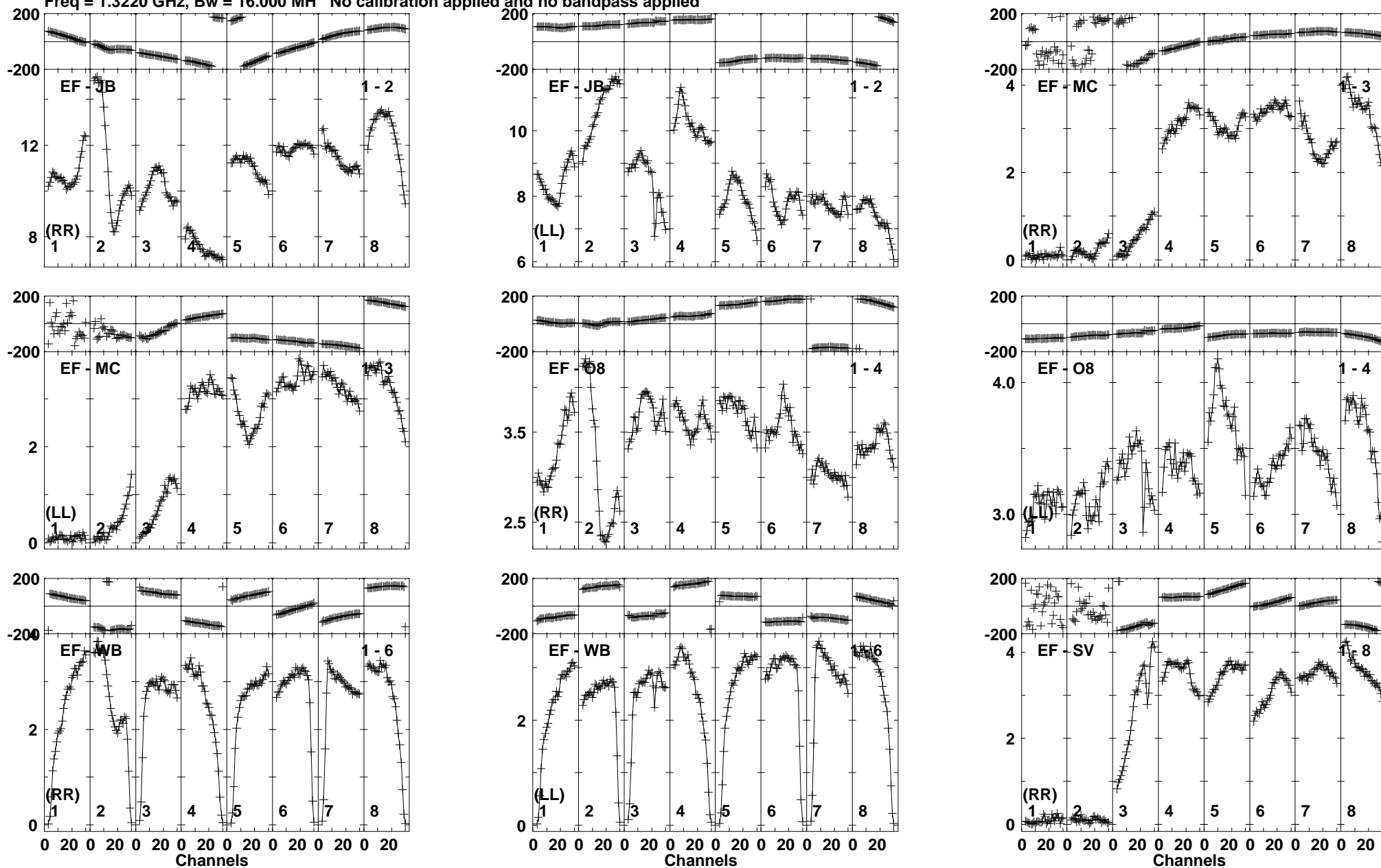
Lower frame: Milli Ampl Jy Top frame: Phas deg Vector averaged cross-power spectrum Baseline: EF (01) - JB (02) Timerange: 00/22:21:12 to 00/22:23:08
