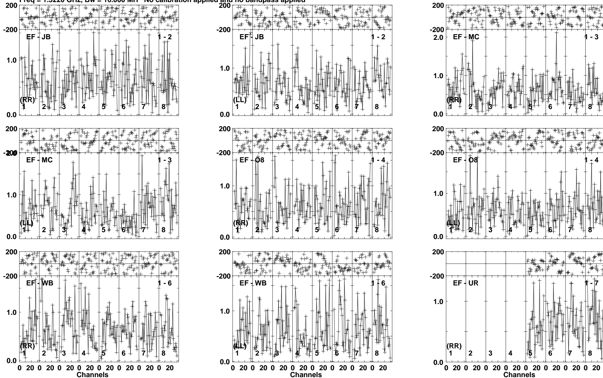
Lower frame: Milli Ampl Jy Top frame: Phas deg Vector averaged cross-power spectrum Baseline: EF (01) - JB (02) Timerange: 00:18:12:10 to 00:18:15:26
