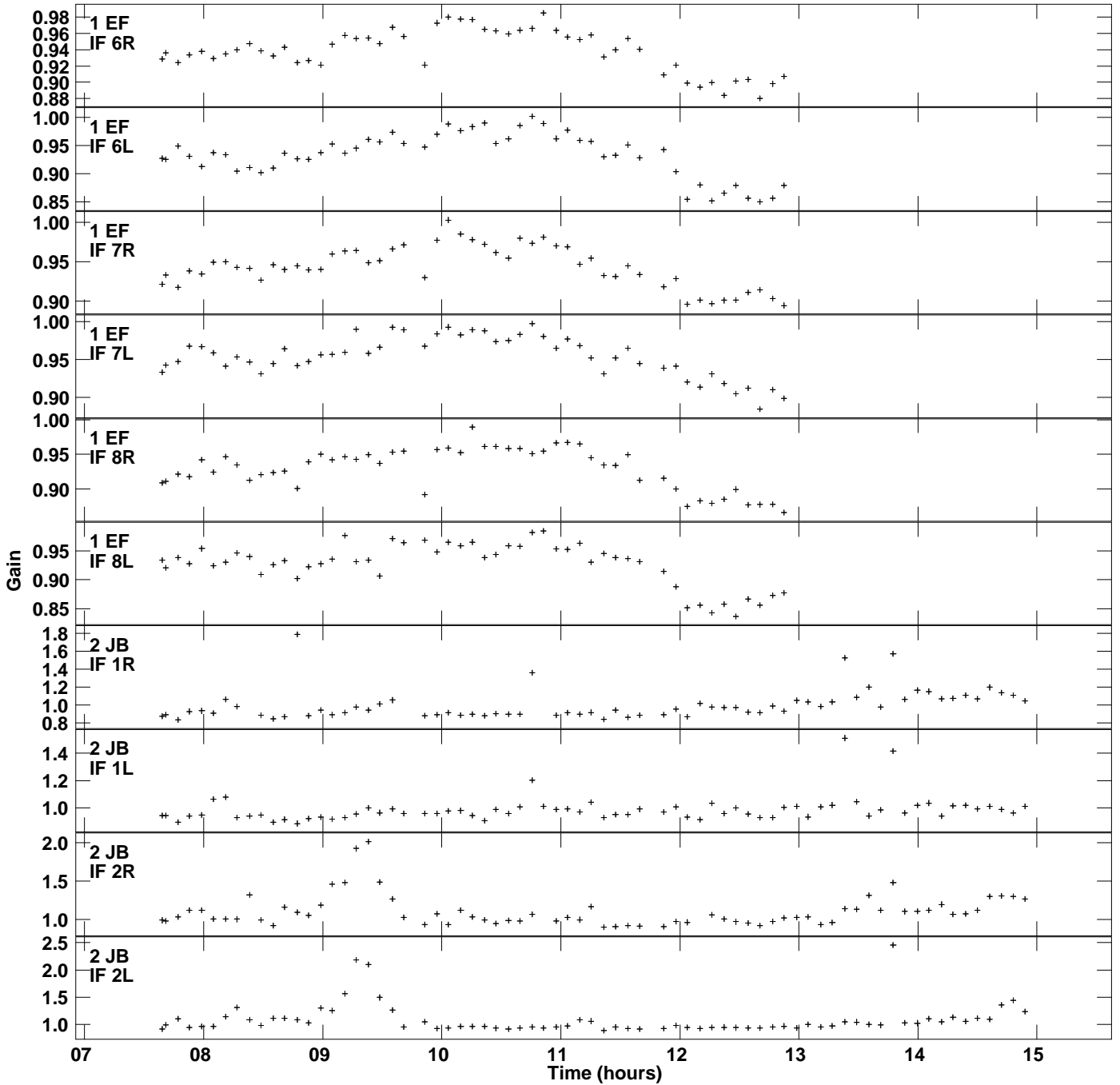
Plot file version 2 created 21-AUG-2018 13:10:55 Gain amp vs UTC time for J0521+2112.MULTI.1 SN 2 Rpol & Lpol IF 1 - 8
