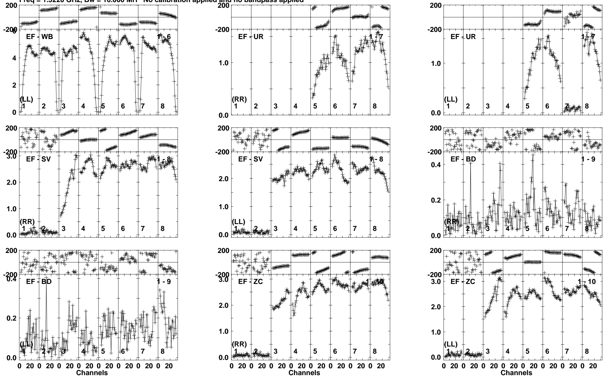
Lower frame: Milli Ampl Jy Top frame: Phas deg Vector averaged cross-power spectrum Baseline: EF (01) - WB (06) Timerange: 00/09:03:40 to 00/09:05:56
