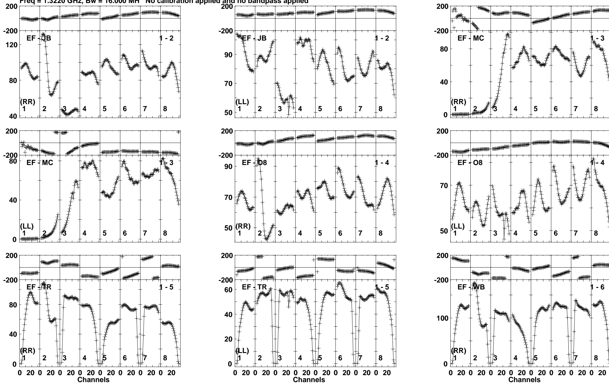
Lower frame: Milli Ampl Jy Top frame: Phas deg Vector averaged cross-power spectrum Baseline: EF (01) - JB (02) Timerange: 00/09:44:32 to 00/09:47:28
