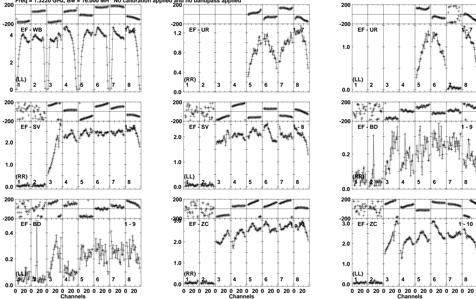
Lower frame: Milli Ampl Jy Top frame: Phas deg Vector averaged cross-power spectrum Baseline: EF (01) - WB (06) Timerange: 00/07:38:02 to 00/07:41:58
