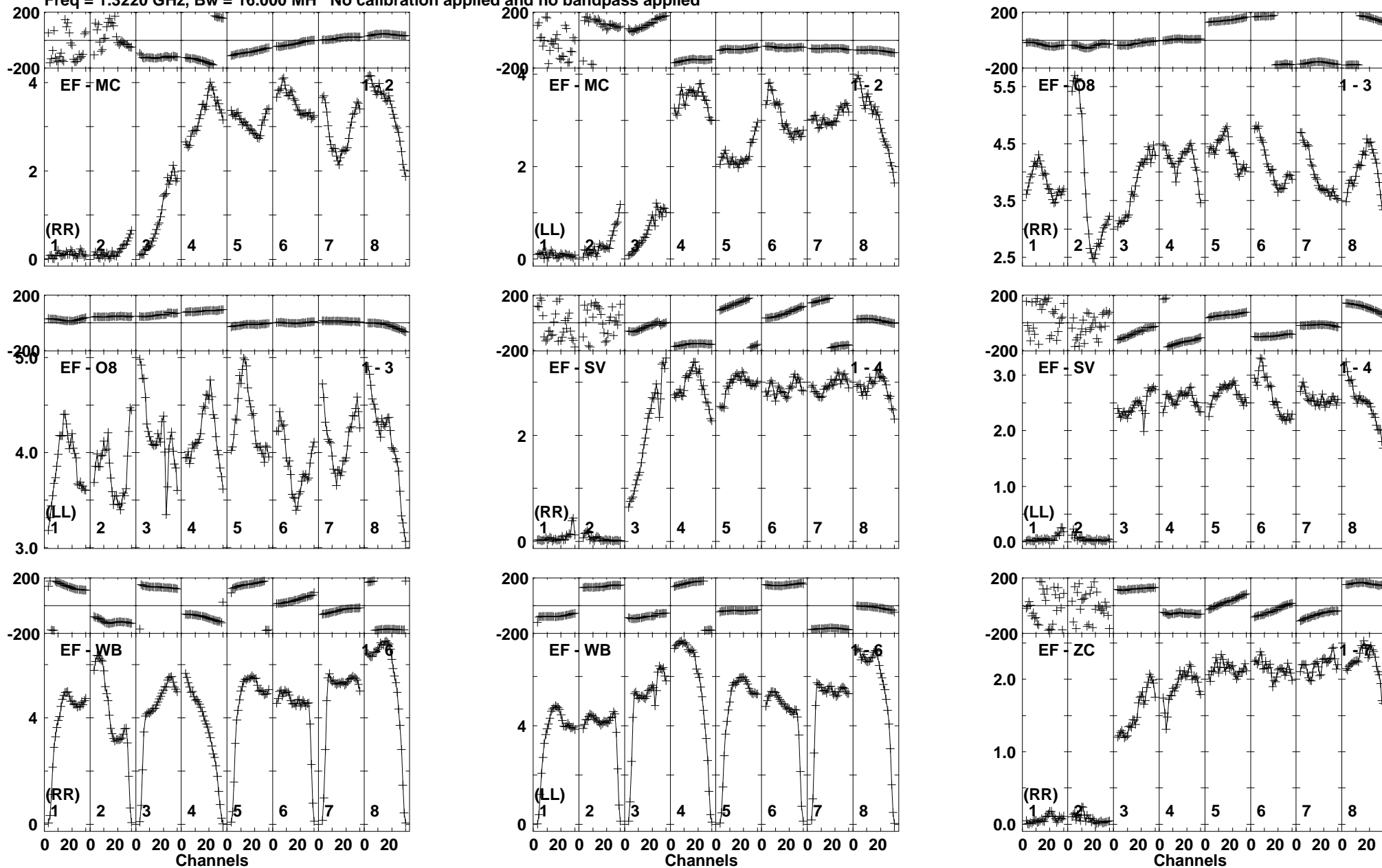
Lower frame: Milli Ampl Jy Top frame: Phas deg Vector averaged cross-power spectrum Baseline: EF (01) - MC (02) Timerange: 00/03:18:01 to 00/03:19:59
