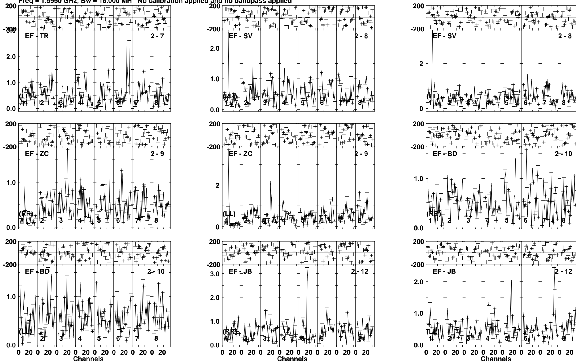
Lower frame: Milli Ampl Jy Top frame: Phas deg Vector averaged cross-power spectrum Baseline: EF (02) - TR (07) Timerange: 00/16:27:03 to 00/16:30:49
