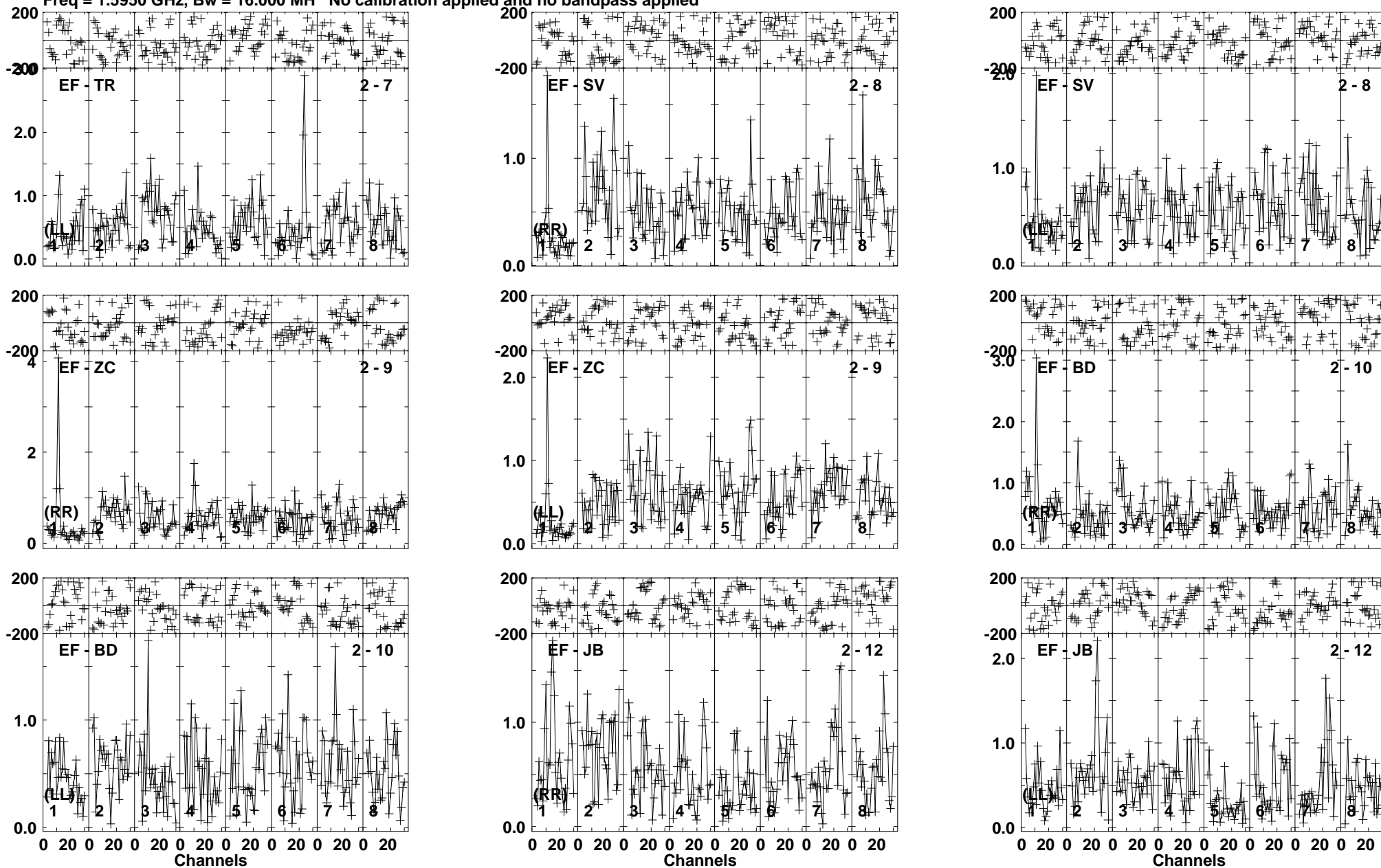
Lower frame: Milli Ampl Jy Top frame: Phas deg Vector averaged cross-power spectrum Baseline: EF (02) - TR (07) Timerange: 00/16:14:35 to 00/16:18:19
