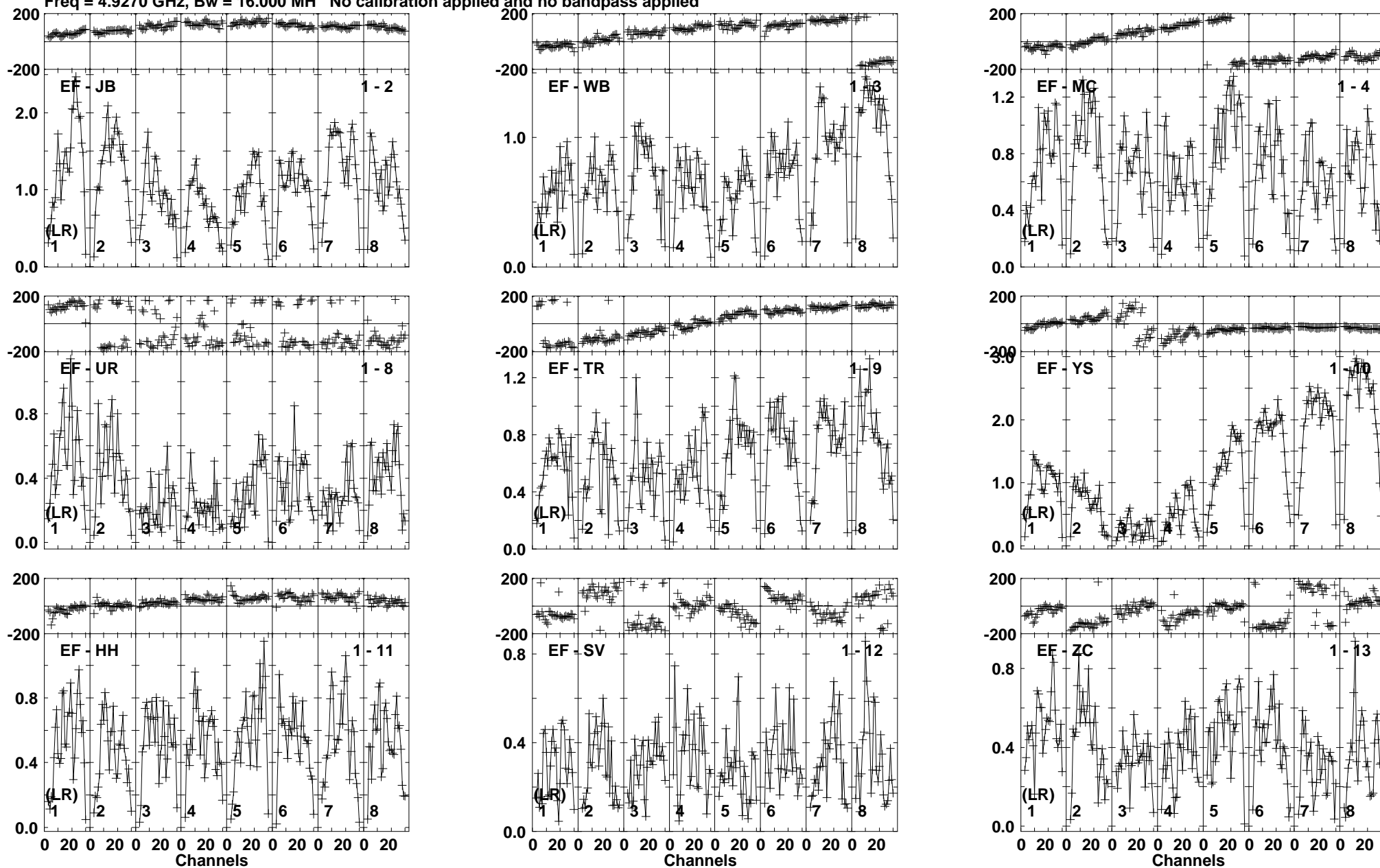
Lower frame: Milli Ampl Jy Top frame: Phas deg Vector averaged cross-power spectrum Baseline: EF (01) - JB (02) Timerange: 00/07:50:31 to 00/07:51:59
