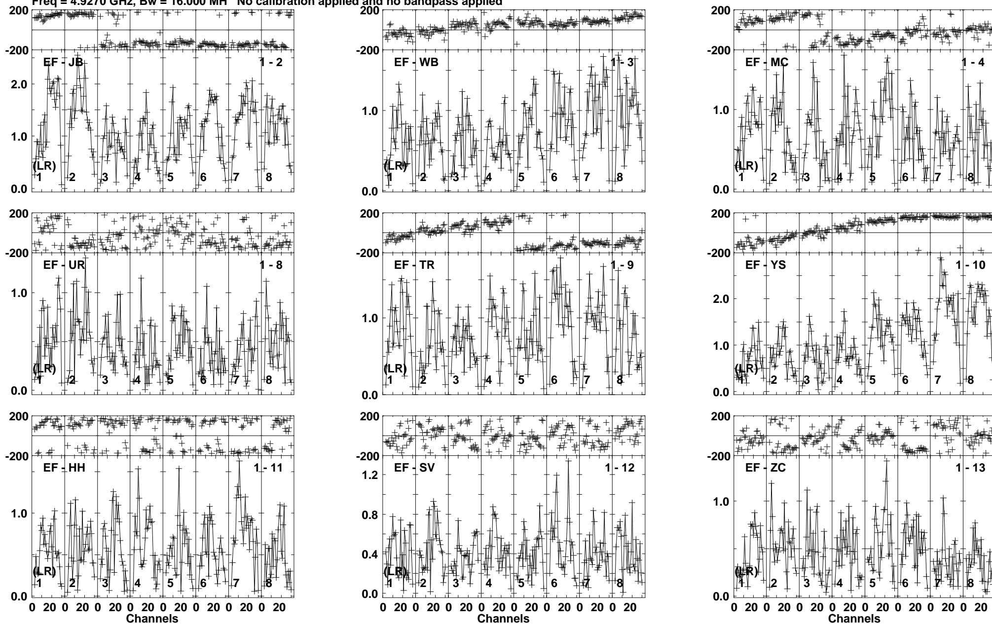
Lower frame: Milli Ampl Jy Top frame: Phas deg Vector averaged cross-power spectrum Baseline: EF (01) - JB (02) Timerange: 00/06:11:51 to 00/06:13:19
