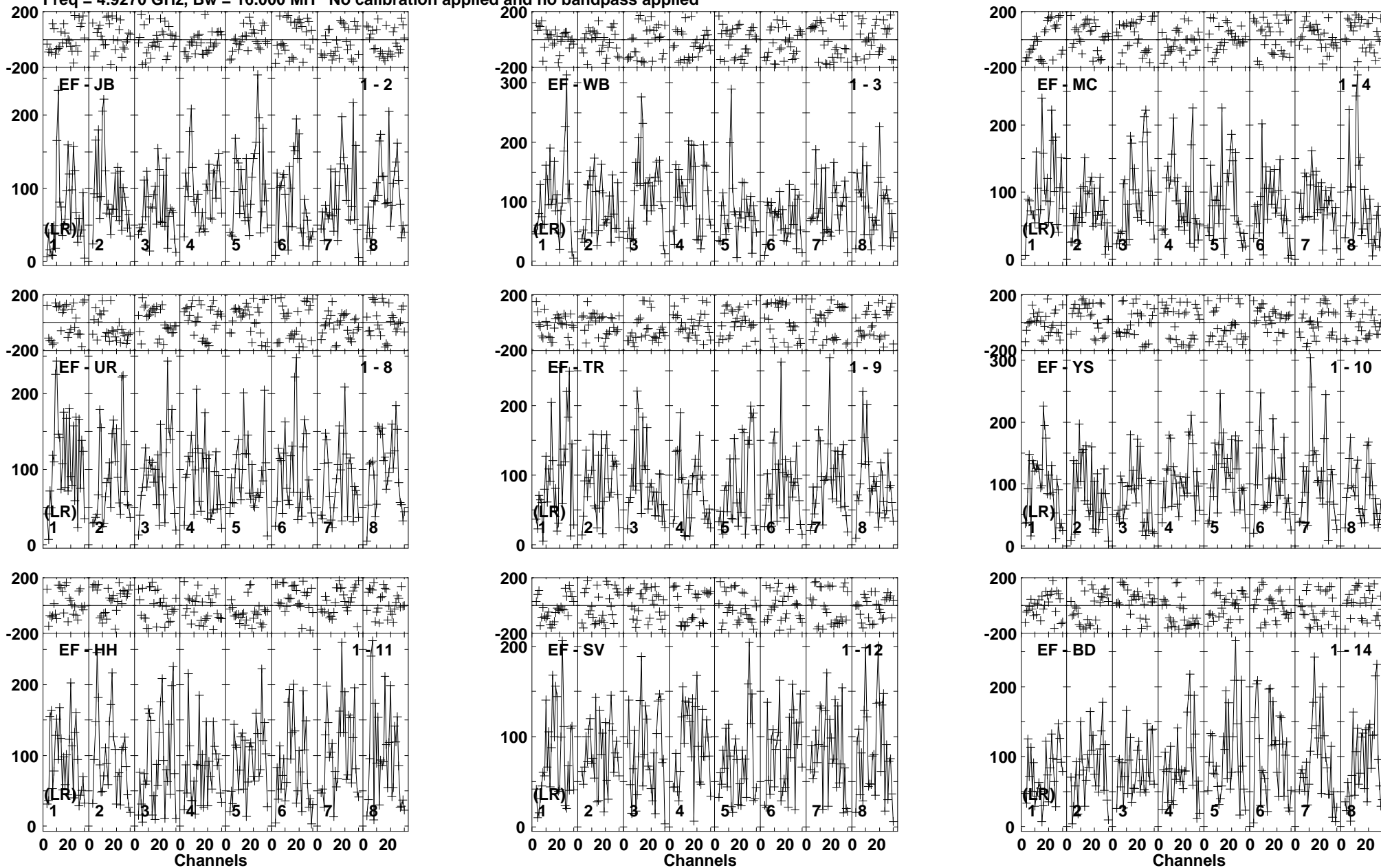
Lower frame: Micro Ampl Jy Top frame: Phas deg Vector averaged cross-power spectrum Baseline: EF (01) - JB (02) Timerange: 00/03:23:23 to 00/03:26:49
