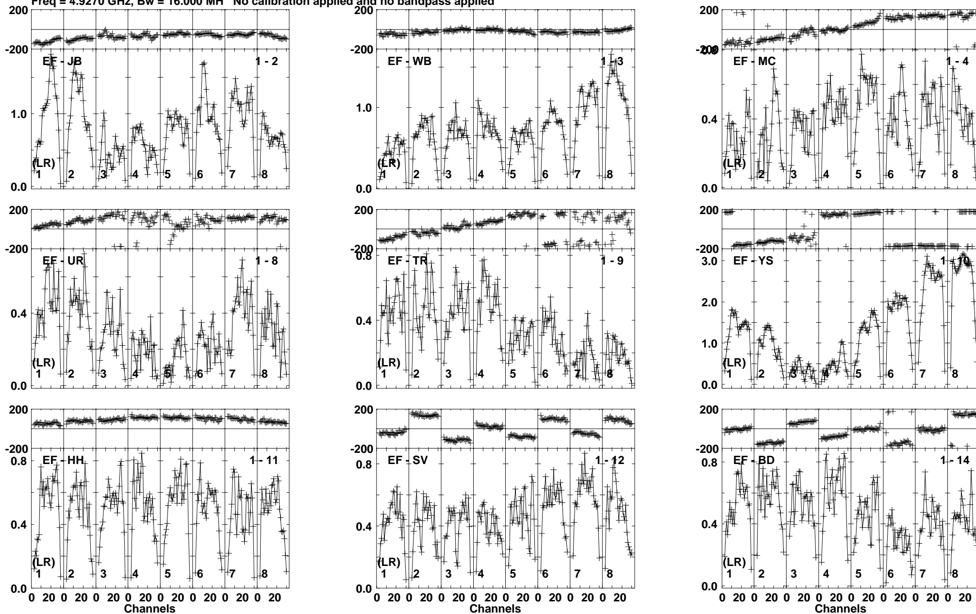
Lower frame: Milli Ampl Jy Top frame: Phas deg Vector averaged cross-power spectrum Baseline: EF (01) - JB (02) Timerange: 00/03:16:51 to 00/03:18:19
