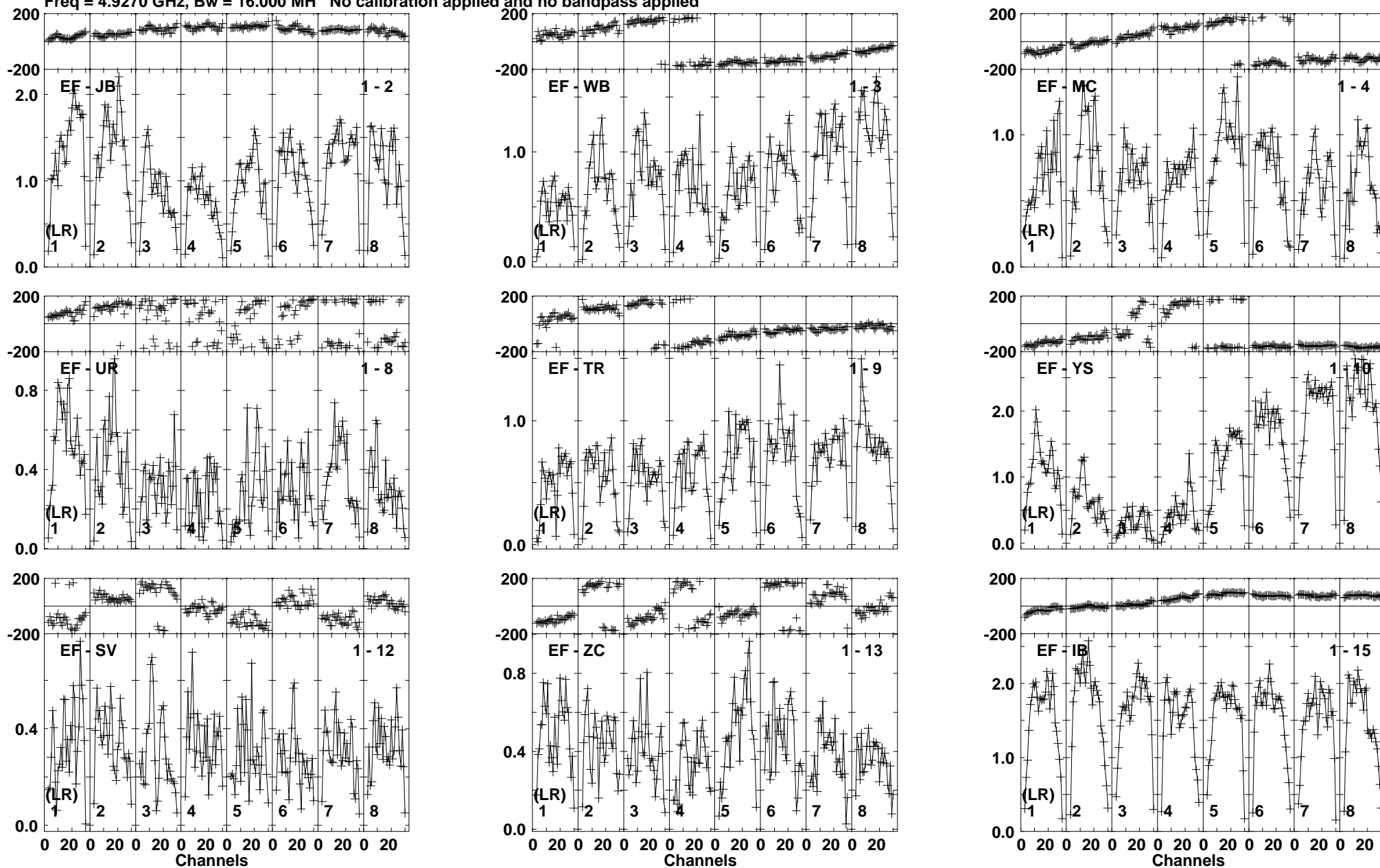
Lower frame: Milli Ampl Jy Top frame: Phas deg Vector averaged cross-power spectrum Baseline: EF (01) - JB (02) Timerange: 00/08:12:11 to 00/08:13:39
