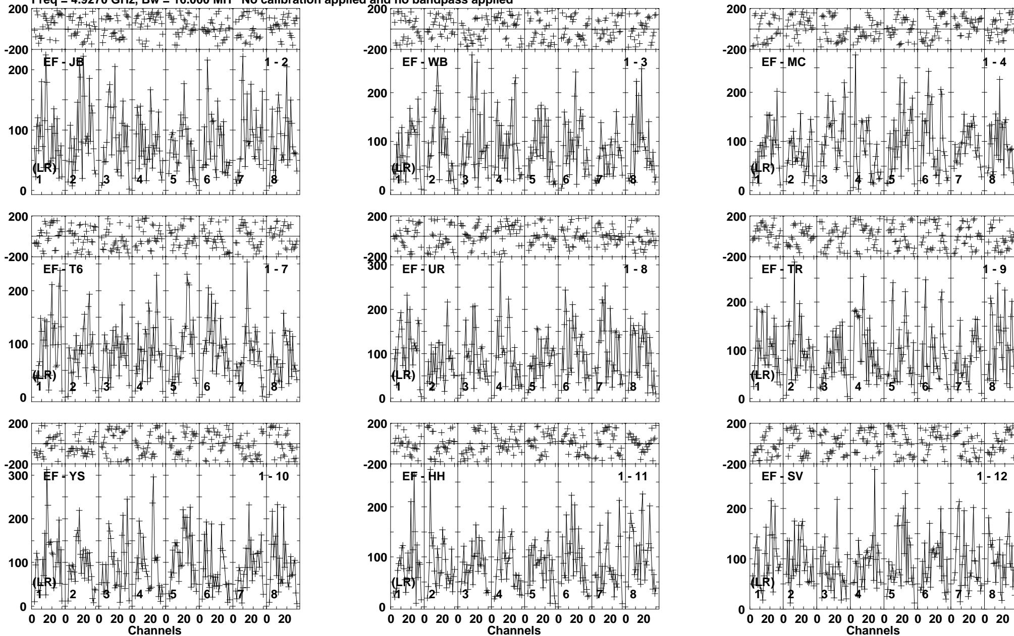
Lower frame: Micro Ampl Jy Top frame: Phas deg Vector averaged cross-power spectrum Baseline: EF (01) - JB (02) Timerange: 00/05:08:23 to 00/05:11:49
