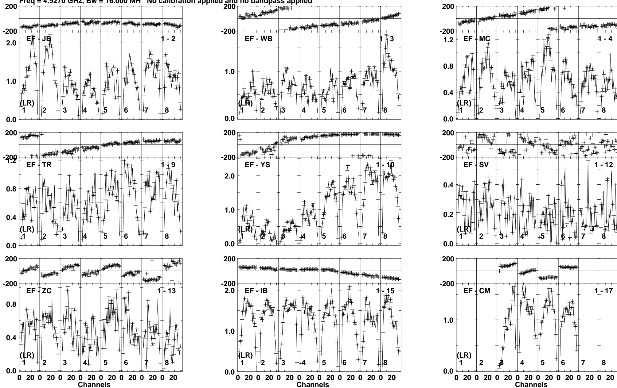
Lower frame: Milli Ampl Jy Top frame: Phas deg Vector averaged cross-power spectrum Baseline: EF (01) - JB (02) Timerange: 00/10:22:11 to 00/10:23:39
