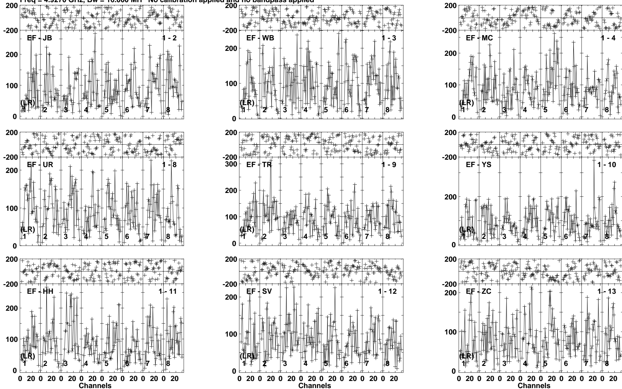
Lower frame: Micro Ampl Jy Top frame: Phas deg Vector averaged cross-power spectrum Baseline: EF (01) - JB (02) Timerange: 00/05:30:03 to 00/05:33:29
