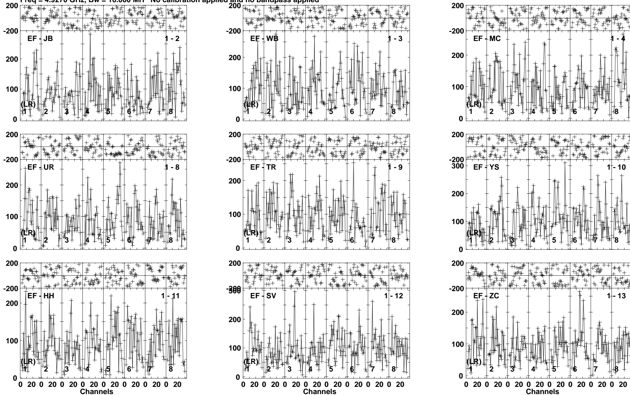
Lower frame: Micro Ampl Jy Top frame: Phas deg Vector averaged cross-power spectrum Baseline: EF (01) - JB (02) Timerange: 00/05:46:41 to 00/05:50:09
