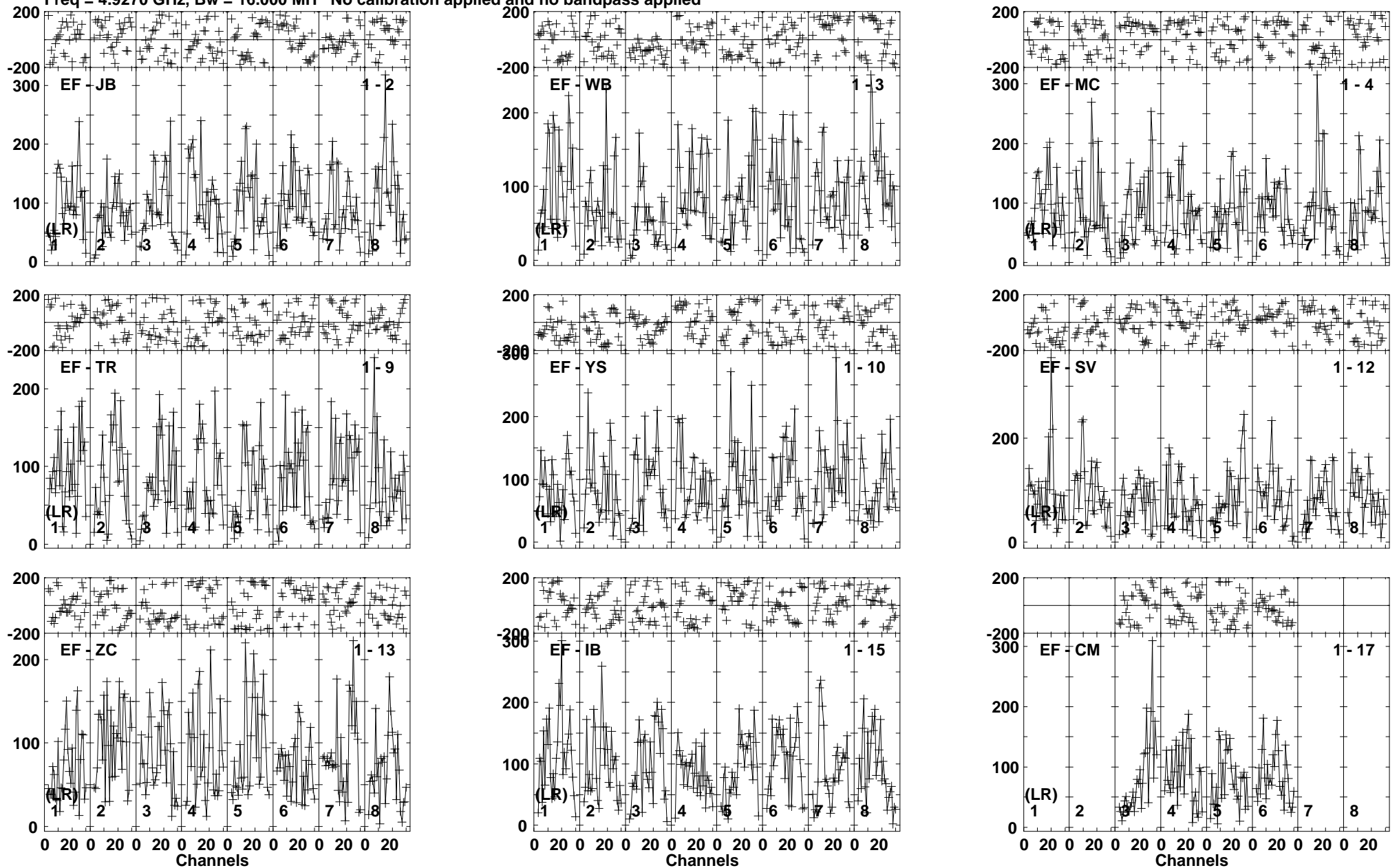
Lower frame: Micro Ampl Jy Top frame: Phas deg Vector averaged cross-power spectrum Baseline: EF (01) - JB (02) Timerange: 00/09:57:01 to 00/10:00:29
