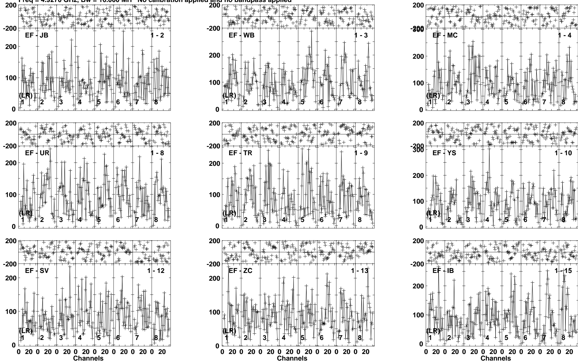
Lower frame: Micro Ampl Jy Top frame: Phas deg Vector averaged cross-power spectrum Baseline: EF (01) - JB (02) Timerange: 00/08:08:41 to 00/08:12:09
