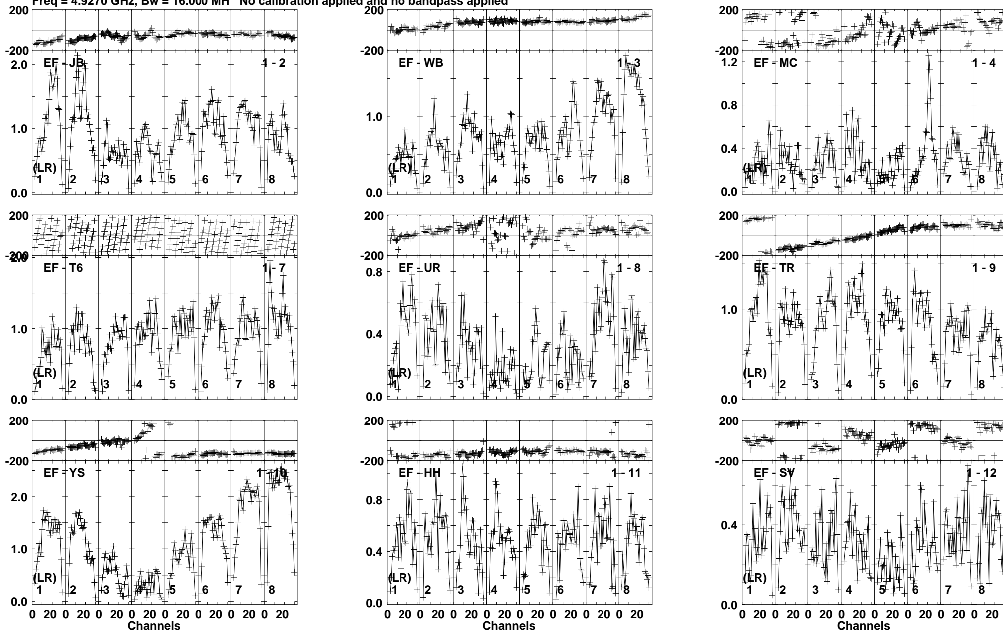
Lower frame: Milli Ampl Jy Top frame: Phas deg Vector averaged cross-power spectrum Baseline: EF (01) - JB (02) Timerange: 00/04:56:01 to 00/04:57:29
