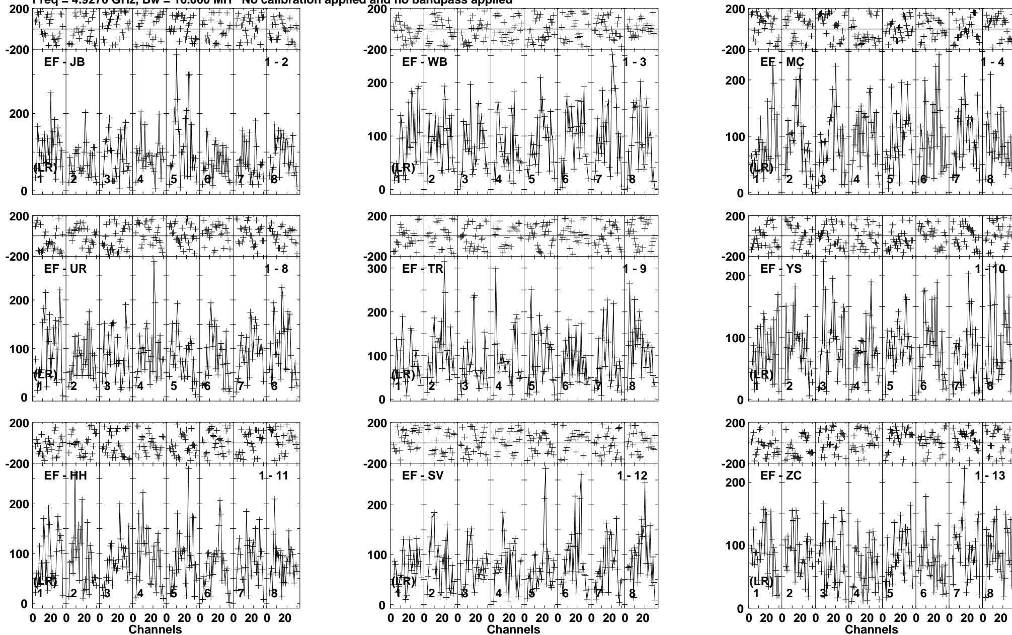
Lower frame: Micro Ampl Jy Top frame: Phas deg Vector averaged cross-power spectrum Baseline: EF (01) - JB (02) Timerange: 00/05:25:01 to 00/05:28:29
