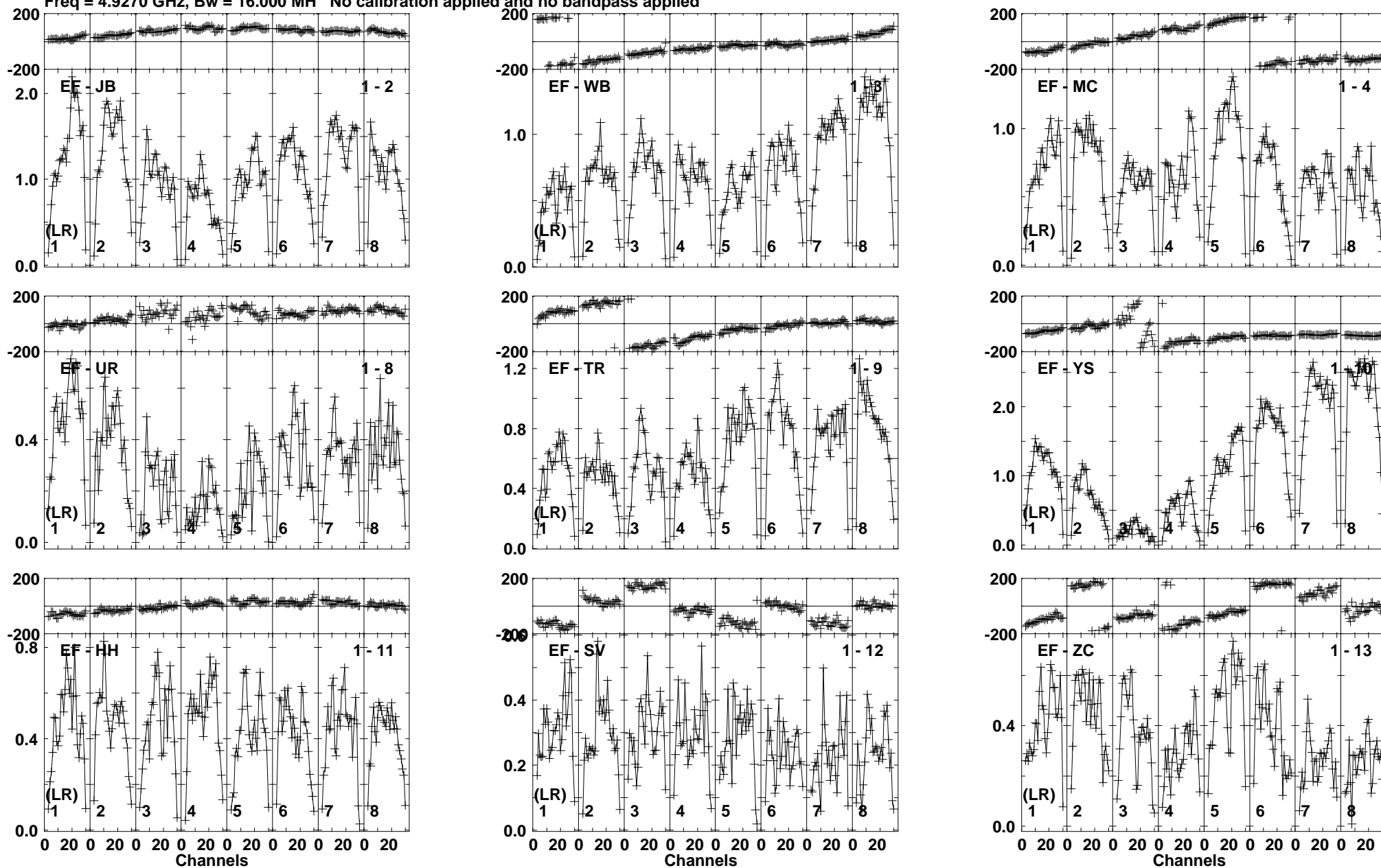
Lower frame: Milli Ampl Jy Top frame: Phas deg Vector averaged cross-power spectrum Baseline: EF (01) - JB (02) Timerange: 00/07:56:21 to 00/07:57:49
