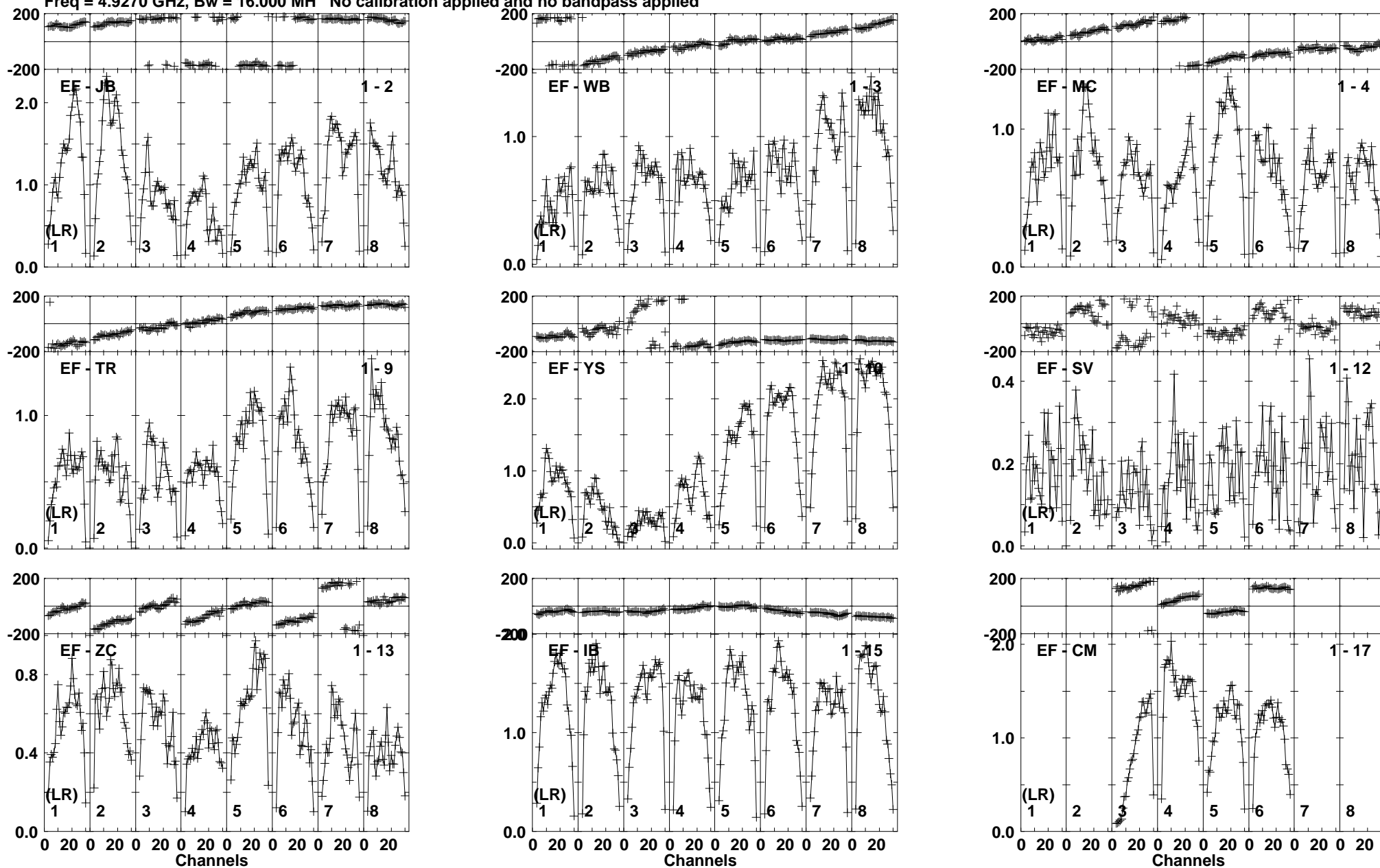
Lower frame: Milli Ampl Jy Top frame: Phas deg Vector averaged cross-power spectrum Baseline: EF (01) - JB (02) Timerange: 00/09:23:01 to 00/09:24:29
