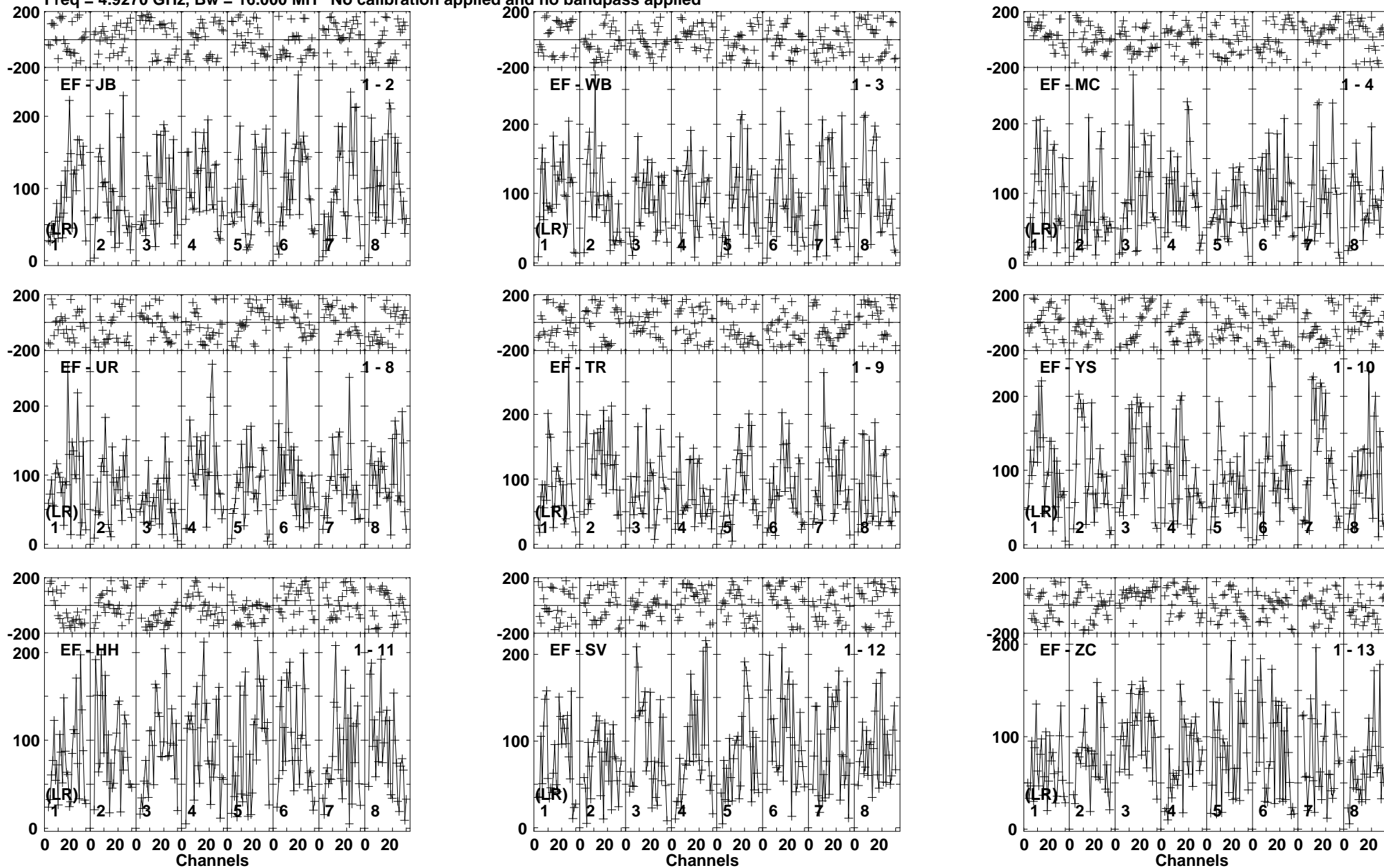
Lower frame: Micro Ampl Jy Top frame: Phas deg Vector averaged cross-power spectrum Baseline: EF (01) - JB (02) Timerange: 00/04:41:41 to 00/04:45:09
