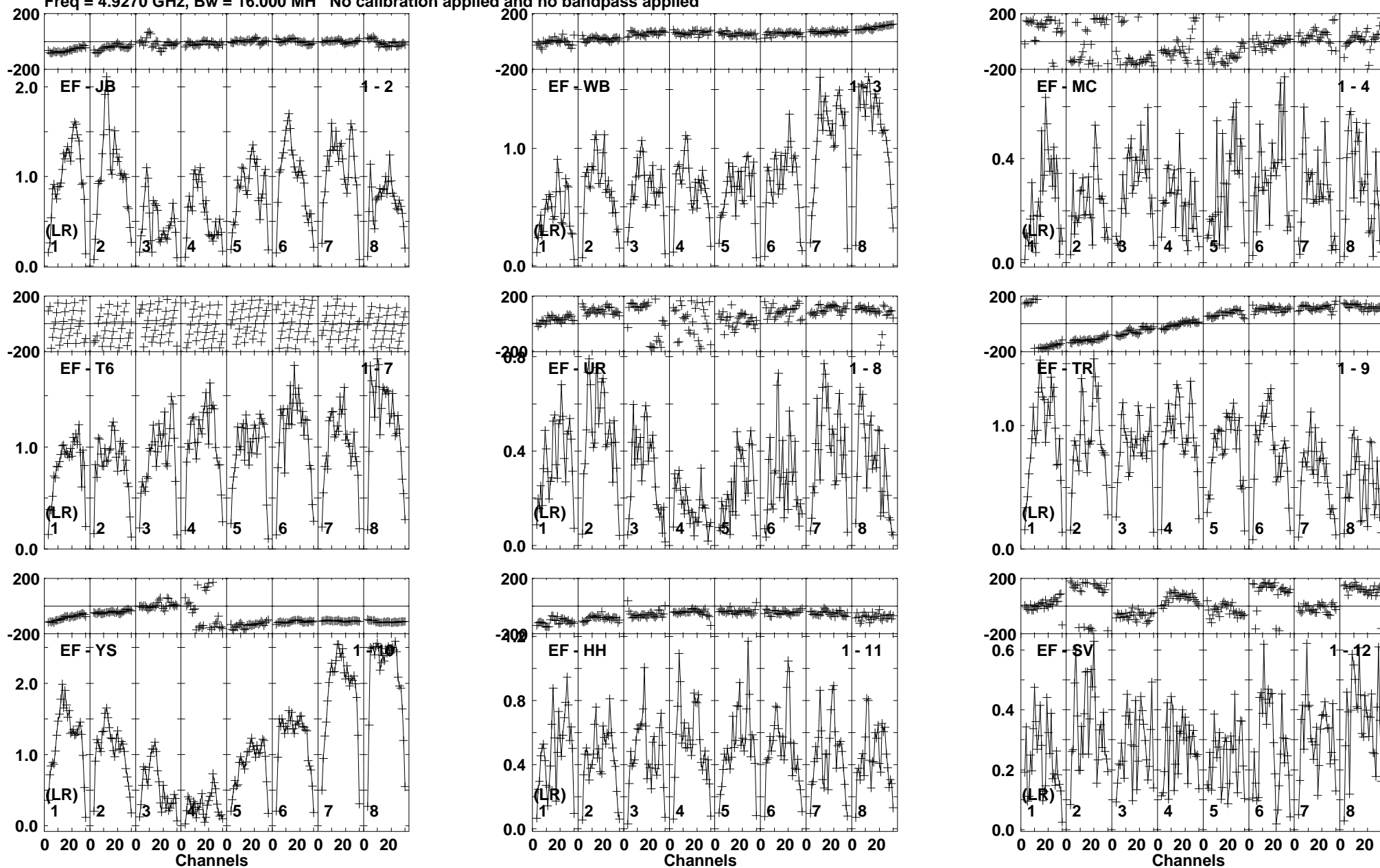
Lower frame: Milli Ampl Jy Top frame: Phas deg Vector averaged cross-power spectrum Baseline: EF (01) - JB (02) Timerange: 00/04:45:11 to 00/04:46:39
