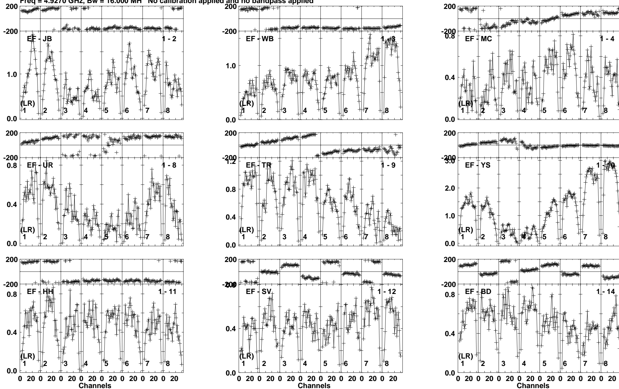
Lower frame: Milli Ampl Jy Top frame: Phas deg Vector averaged cross-power spectrum Baseline: EF (01) - JB (02) Timerange: 00/03:56:51 to 00/03:58:19
