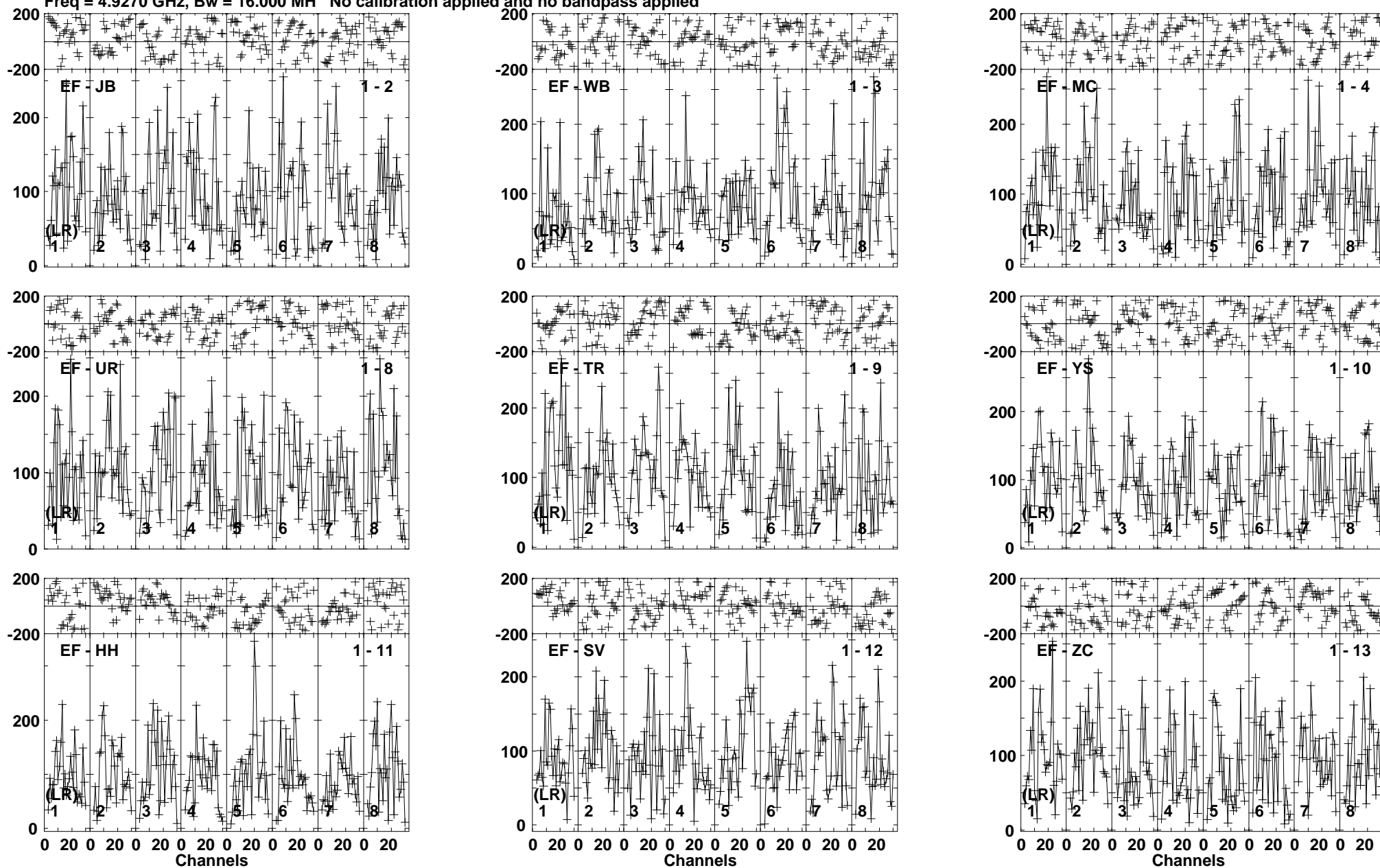
Lower frame: Micro Ampl Jy Top frame: Phas deg Vector averaged cross-power spectrum Baseline: EF (01) - JB (02) Timerange: 00/06:24:11 to 00/06:27:39
