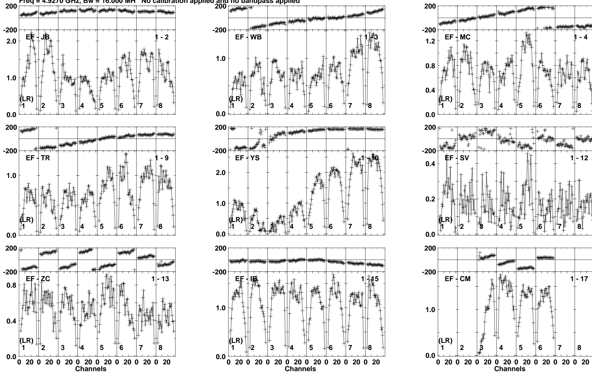
Lower frame: Milli Ampl Jy Top frame: Phas deg Vector averaged cross-power spectrum Baseline: EF (01) - JB (02) Timerange: 00/09:33:51 to 00/09:35:19
