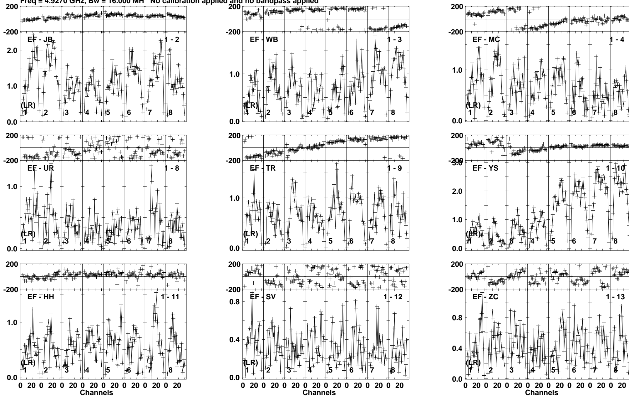
Lower frame: Milli Ampl Jy Top frame: Phas deg Vector averaged cross-power spectrum Baseline: EF (01) - JB (02) Timerange: 00/06:33:31 to 00/06:34:59
