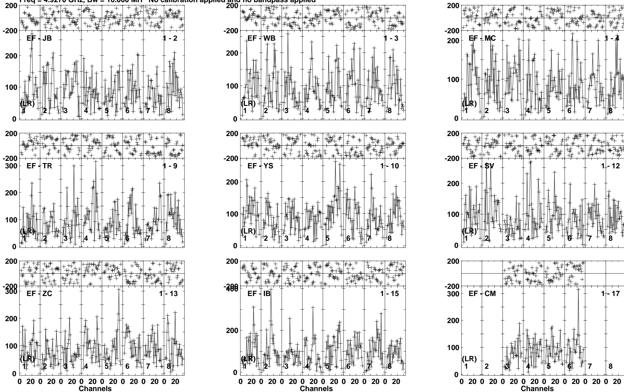
Lower frame: Micro Ampl Jy Top frame: Phas deg Vector averaged cross-power spectrum Baseline: EF (01) - JB (02) Timerange: 00/09:40:21 to 00/09:43:49
