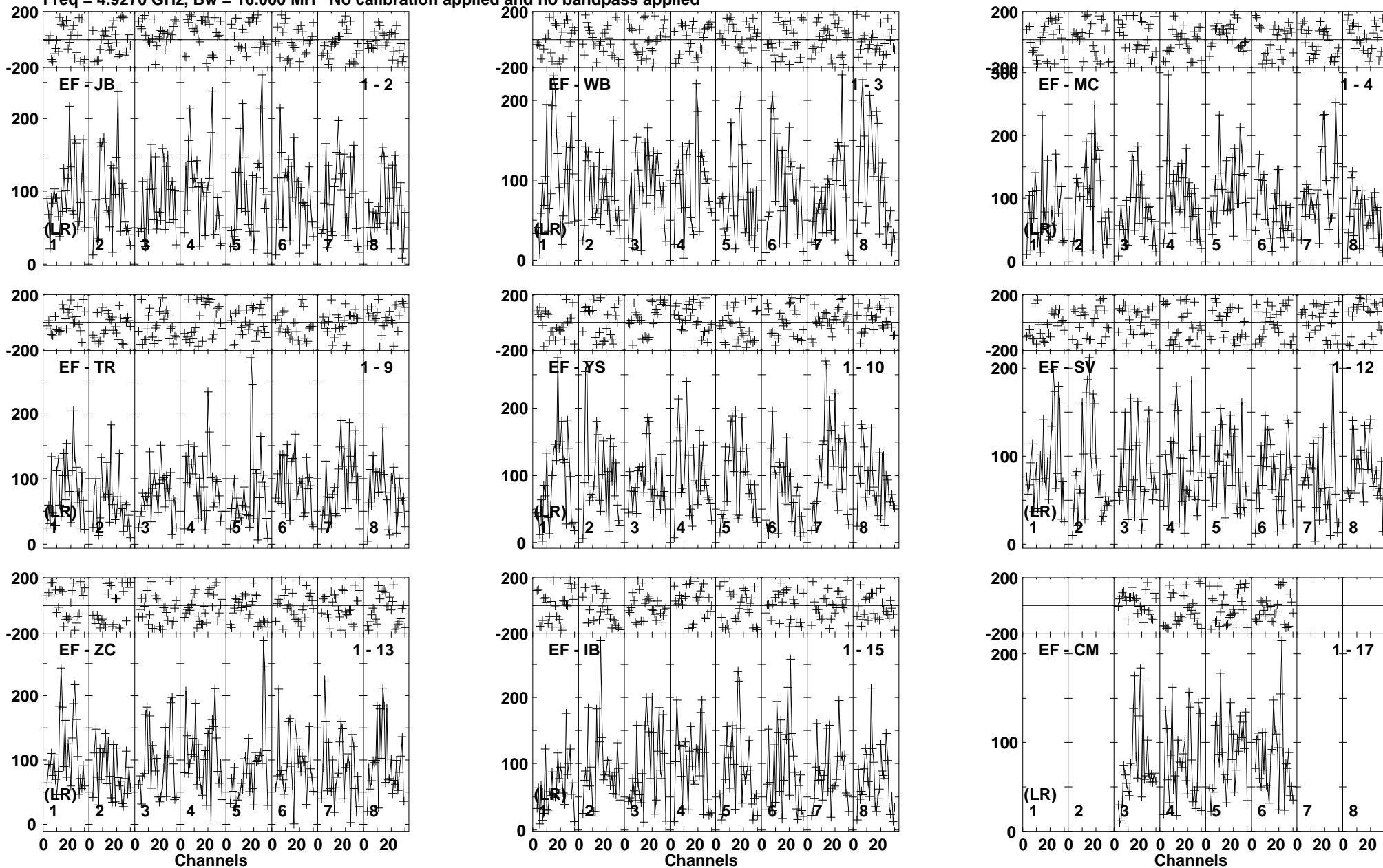
Lower frame: Micro Ampl Jy Top frame: Phas deg Vector averaged cross-power spectrum Baseline: EF (01) - JB (02) Timerange: 00/09:35:21 to 00/09:38:49
