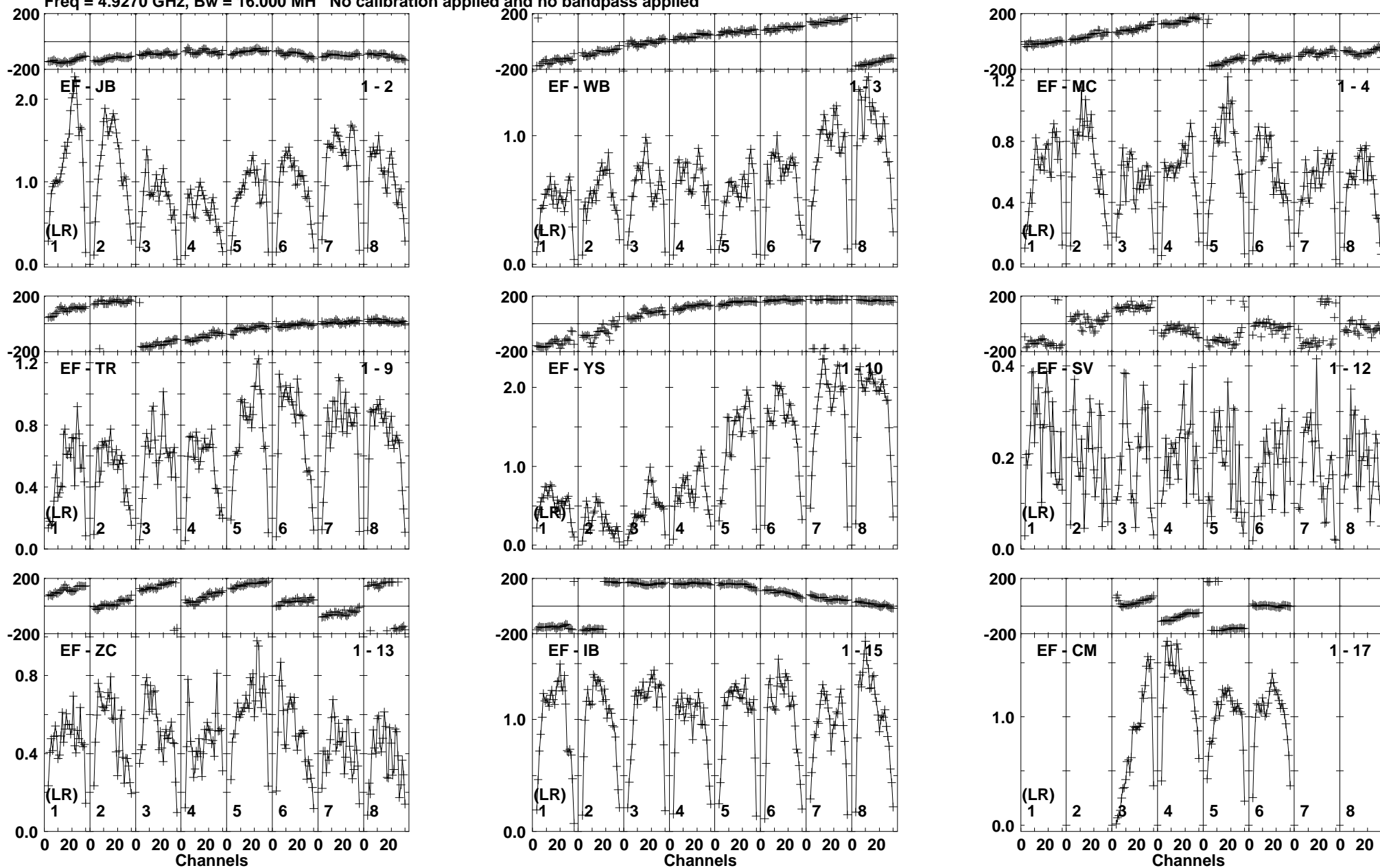
Lower frame: Milli Ampl Jy Top frame: Phas deg Vector averaged cross-power spectrum Baseline: EF (01) - JB (02) Timerange: 00/10:28:01 to 00/10:29:29
