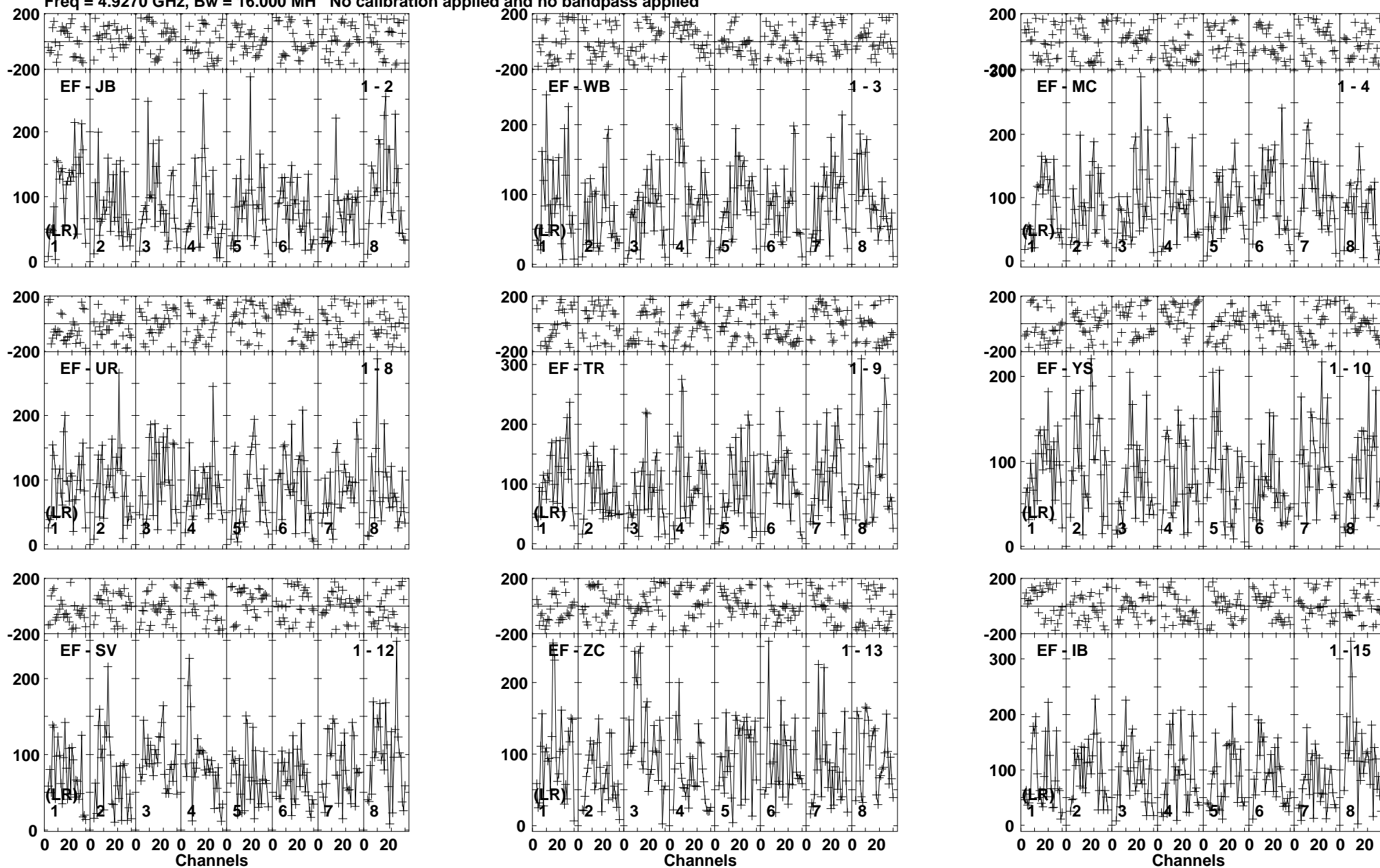
Lower frame: Micro Ampl Jy Top frame: Phas deg Vector averaged cross-power spectrum Baseline: EF (01) - JB (02) Timerange: 00/08:41:11 to 00/08:44:39
