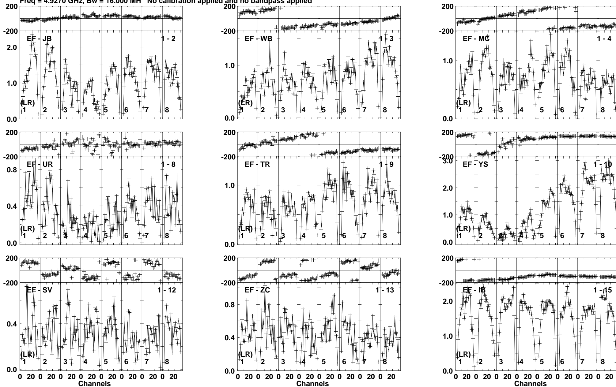
Lower frame: Milli Ampl Jy Top frame: Phas deg Vector averaged cross-power spectrum Baseline: EF (01) - JB (02) Timerange: 00/08:33:51 to 00/08:35:19
