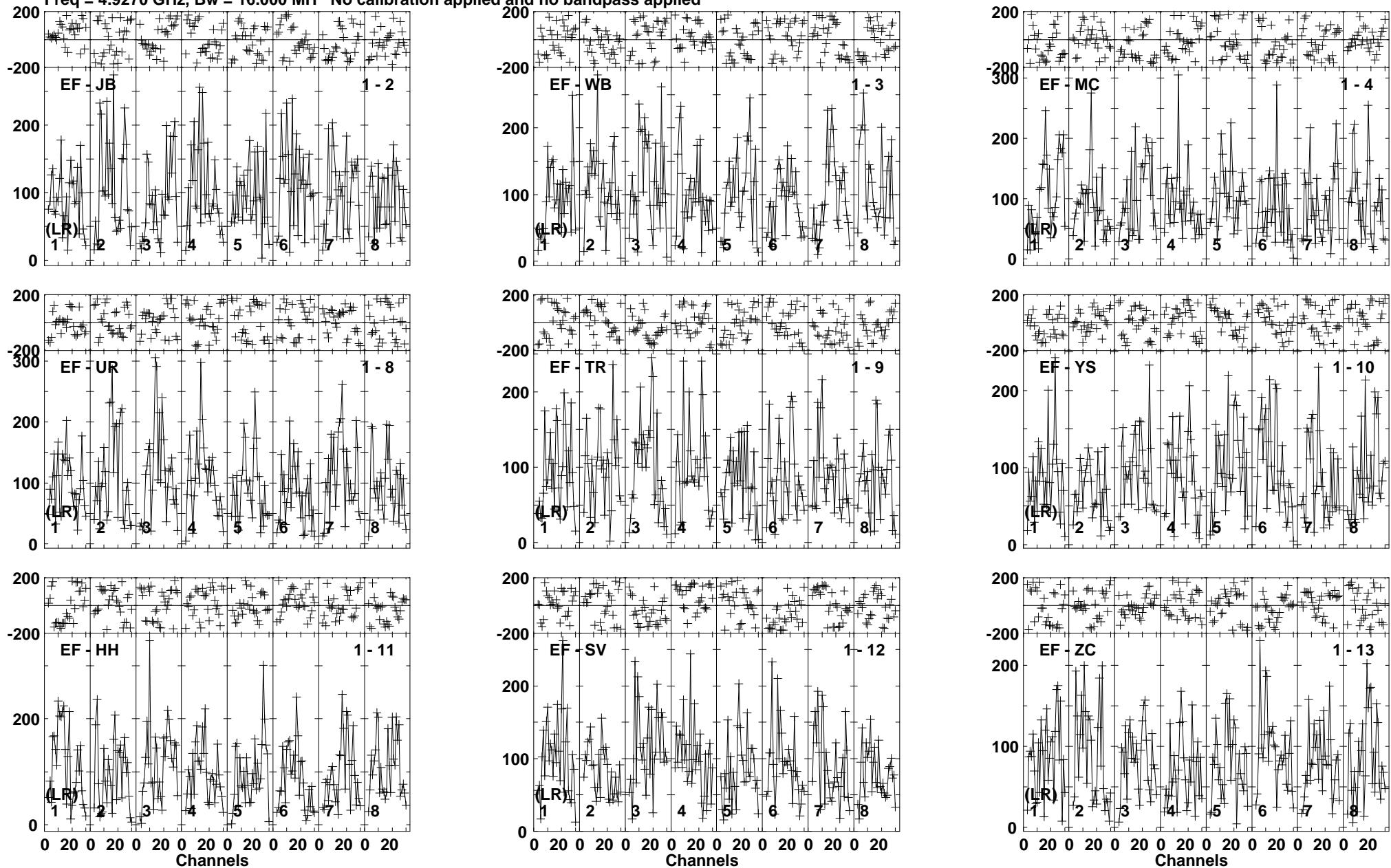
Lower frame: Micro Ampl Jy Top frame: Phas deg Vector averaged cross-power spectrum Baseline: EF (01) - JB (02) Timerange: 00/06:40:51 to 00/06:44:19
