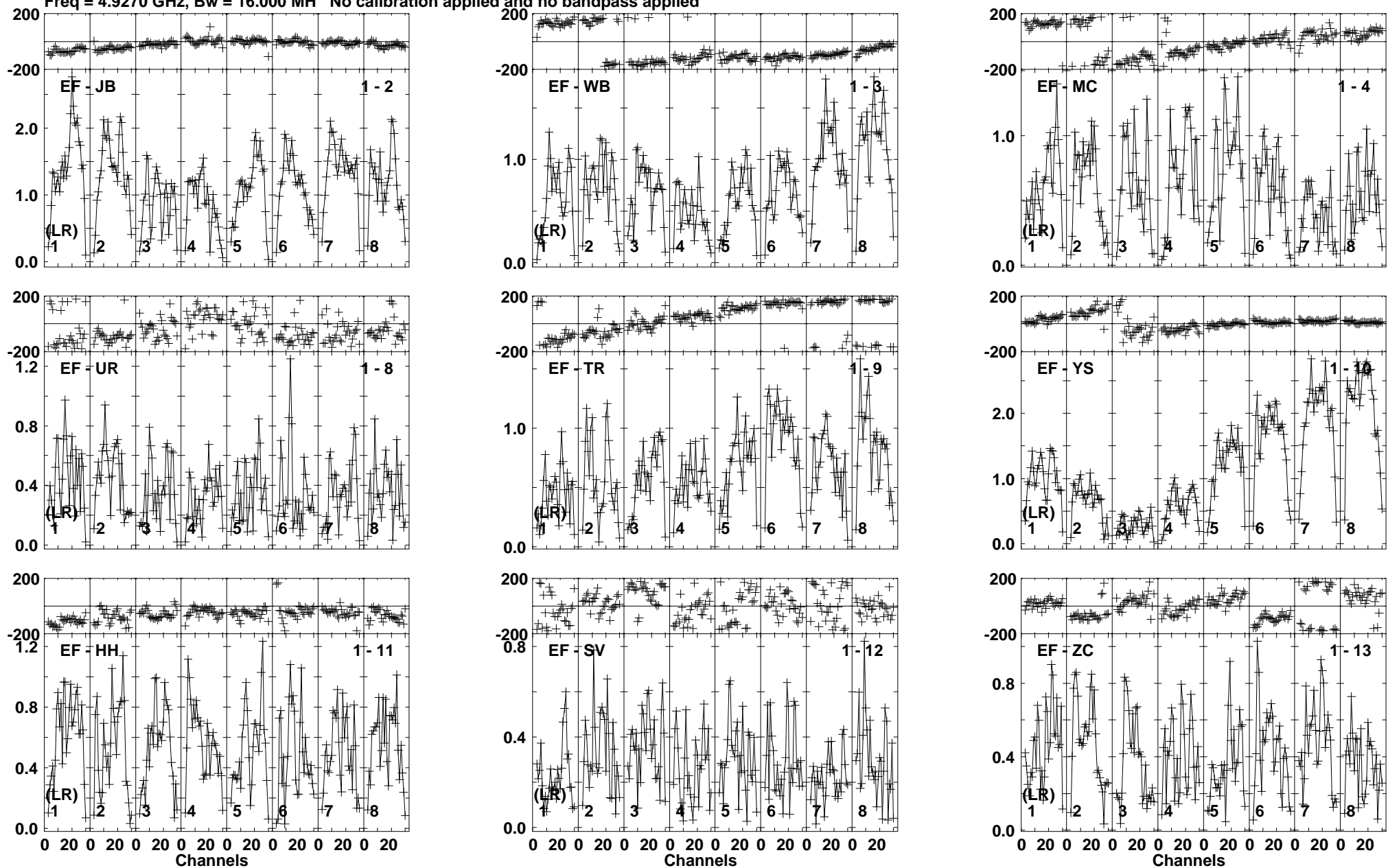
Lower frame: Milli Ampl Jy Top frame: Phas deg Vector averaged cross-power spectrum Baseline: EF (01) - JB (02) Timerange: 00/06:44:21 to 00/06:45:49
