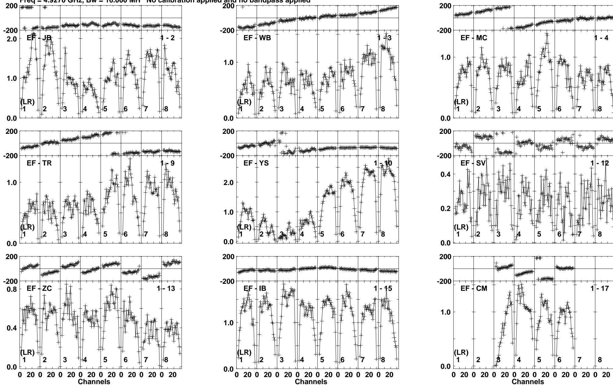
Lower frame: Milli Ampl Jy Top frame: Phas deg Vector averaged cross-power spectrum Baseline: EF (01) - JB (02) Timerange: 00/09:12:11 to 00/09:13:39
