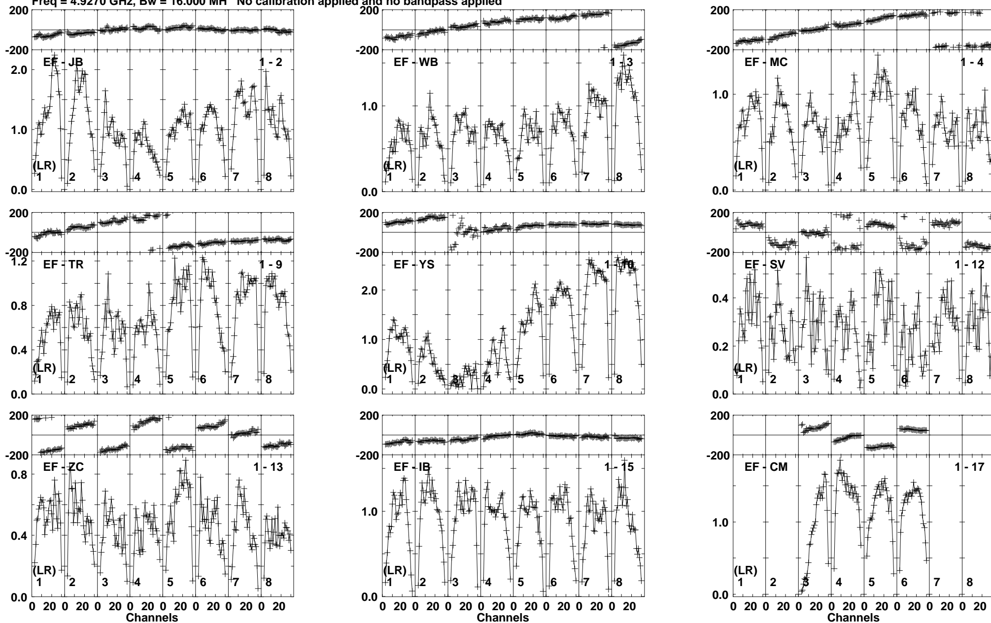
Lower frame: Milli Ampl Jy Top frame: Phas deg Vector averaged cross-power spectrum Baseline: EF (01) - JB (02) Timerange: 00/08:50:31 to 00/08:51:59
