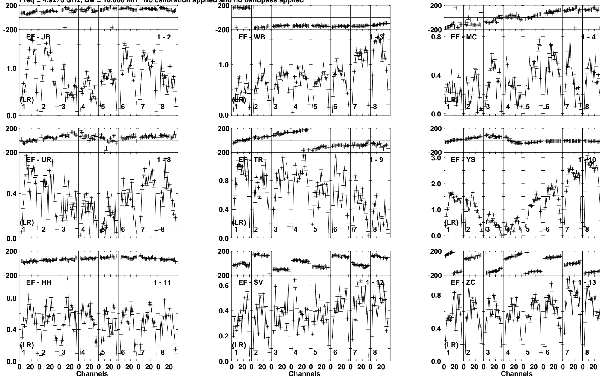
Lower frame: Milli Ampl Jy Top frame: Phas deg Vector averaged cross-power spectrum Baseline: EF (01) - JB (02) Timerange: 00/04:07:41 to 00/04:09:09
