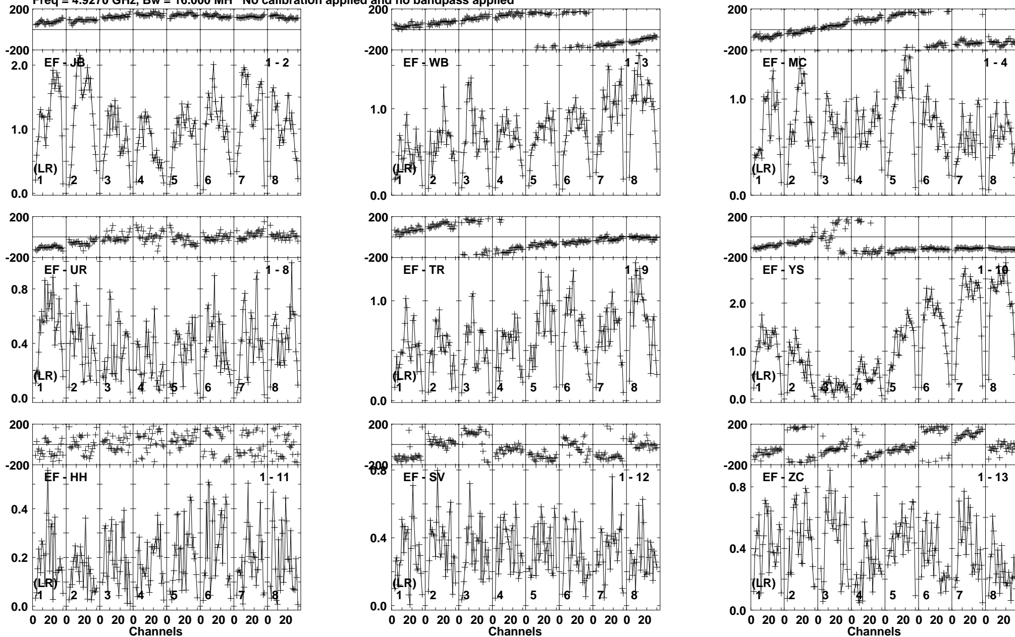
Lower frame: Milli Ampl Jy Top frame: Phas deg Vector averaged cross-power spectrum Baseline: EF (01) - JB (02) Timerange: 00/08:01:21 to 00/08:02:49
