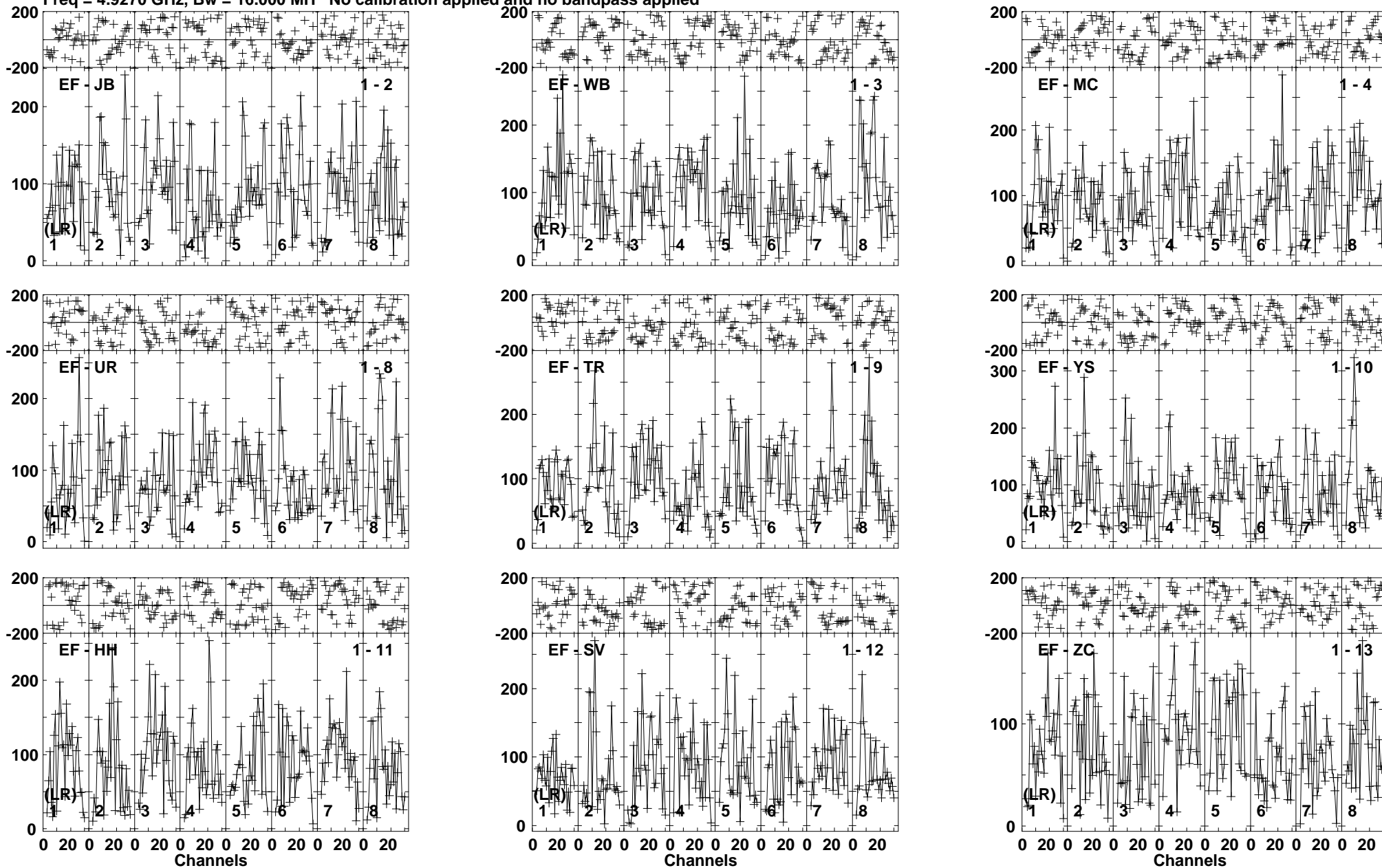
Lower frame: Micro Ampl Jy Top frame: Phas deg Vector averaged cross-power spectrum Baseline: EF (01) - JB (02) Timerange: 00/04:14:11 to 00/04:17:39
