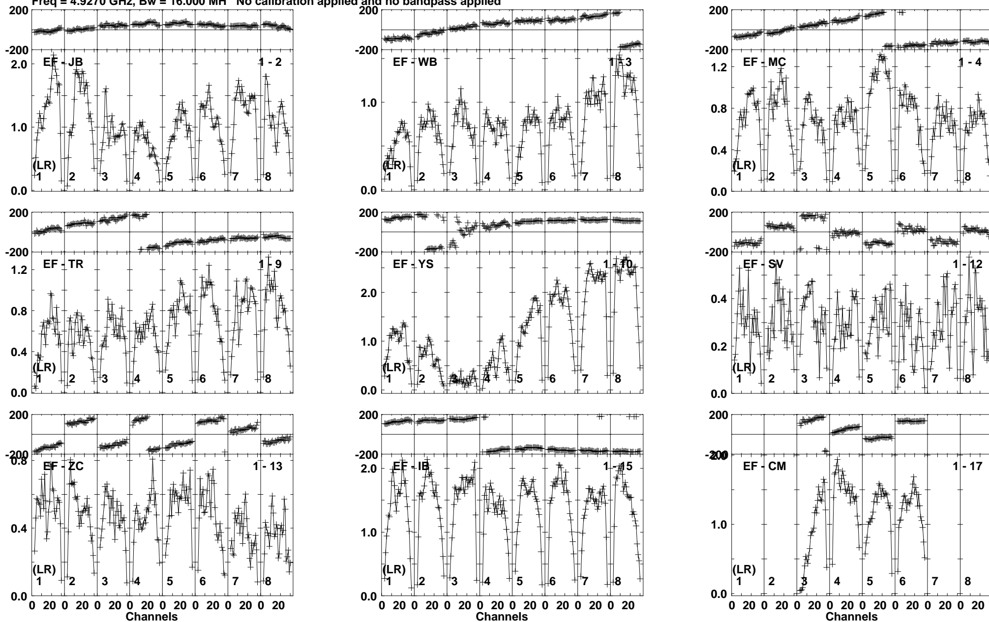
Lower frame: Milli Ampl Jy Top frame: Phas deg Vector averaged cross-power spectrum Baseline: EF (01) - JB (02) Timerange: 00/08:39:41 to 00/08:41:09
