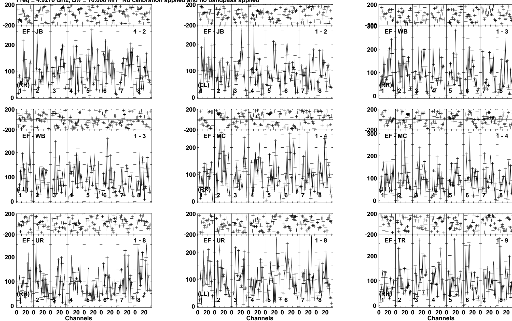
Lower frame: Micro Ampl Jy Top frame: Phas deg Vector averaged cross-power spectrum Baseline: EF (01) - JB (02) Timerange: 00/07:57:51 to 00/08:01:19
