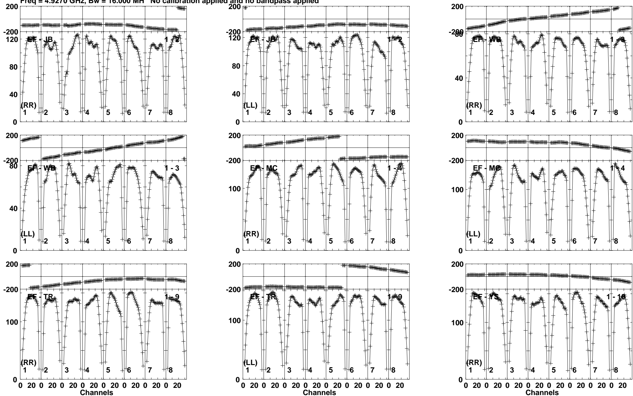
Lower frame: Milli Ampl Jy Top frame: Phas deg Vector averaged cross-power spectrum Baseline: EF (01) - JB (02) Timerange: 00/10:56:13 to 00/10:59:59
