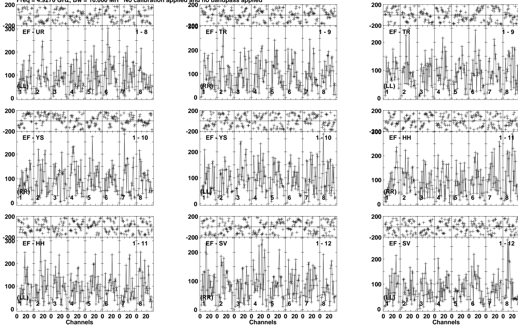
Lower frame: Micro Ampl Jy Top frame: Phas deg Vector averaged cross-power spectrum Baseline: EF (01) - UR (08) Timerange: 00/04:52:31 to 00/04:55:59
