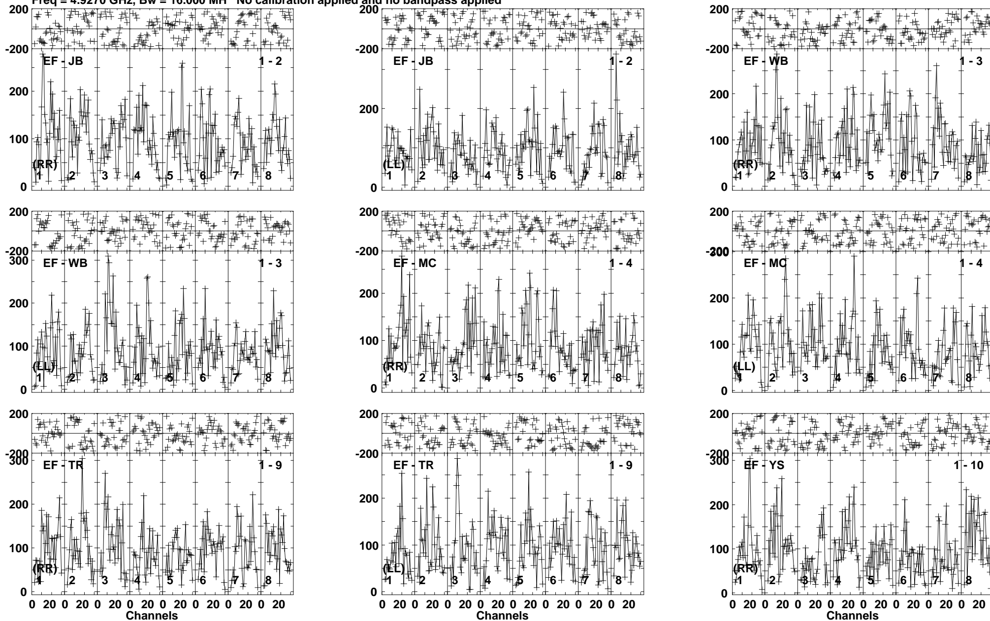
Lower frame: Micro Ampl Jy Top frame: Phas deg Vector averaged cross-power spectrum Baseline: EF (01) - JB (02) Timerange: 00/09:02:51 to 00/09:06:19
