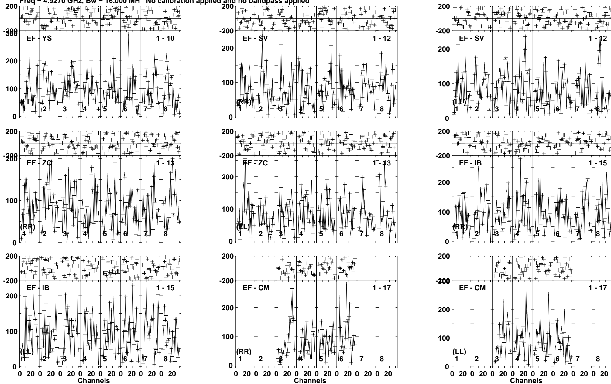
Lower frame: Micro Ampl Jy Top frame: Phas deg Vector averaged cross-power spectrum Baseline: EF (01) - YS (10) Timerange: 00/10:29:31 to 00/10:32:59
