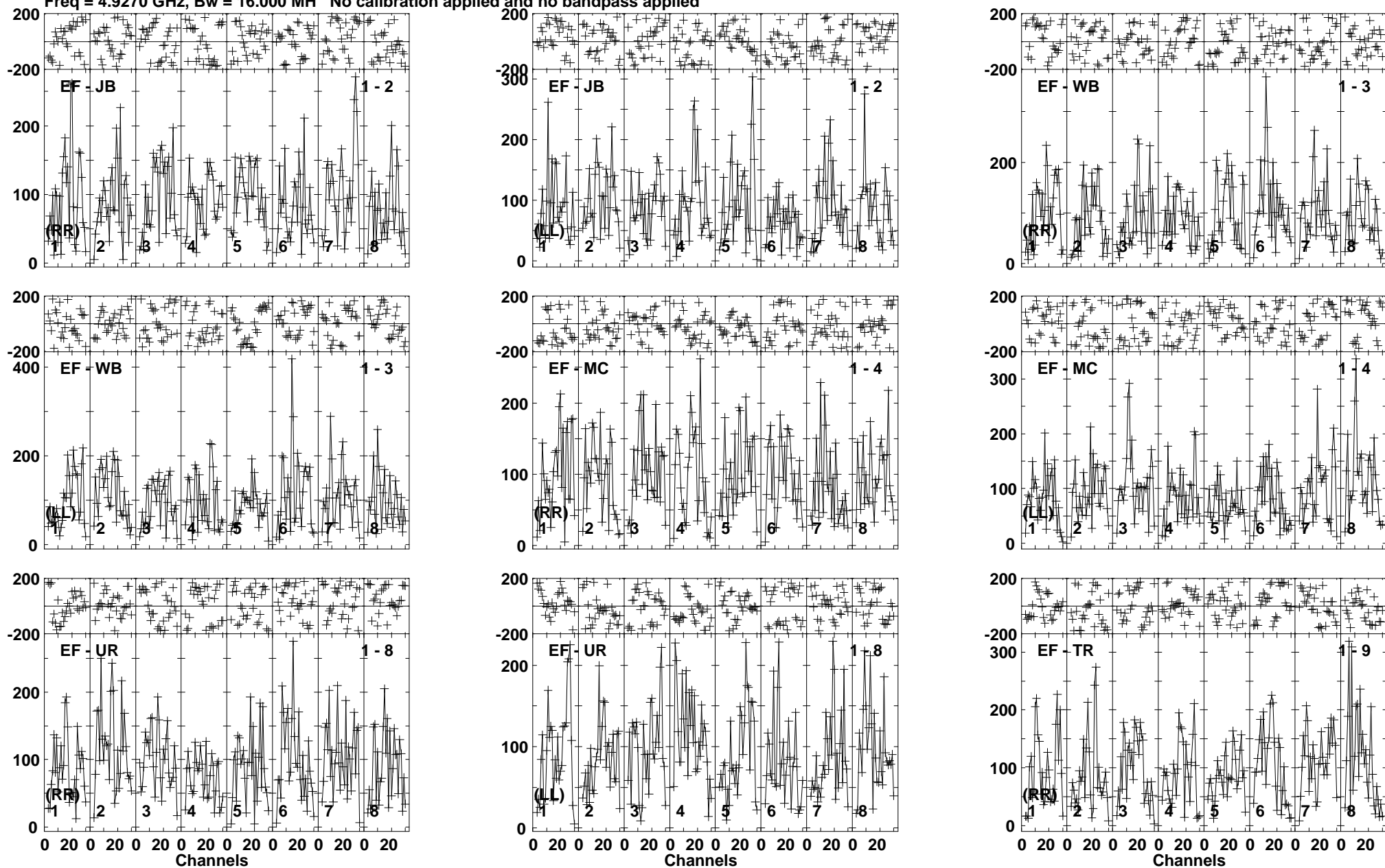
Lower frame: Micro Ampl Jy Top frame: Phas deg Vector averaged cross-power spectrum Baseline: EF (01) - JB (02) Timerange: 00/06:19:11 to 00/06:22:39
