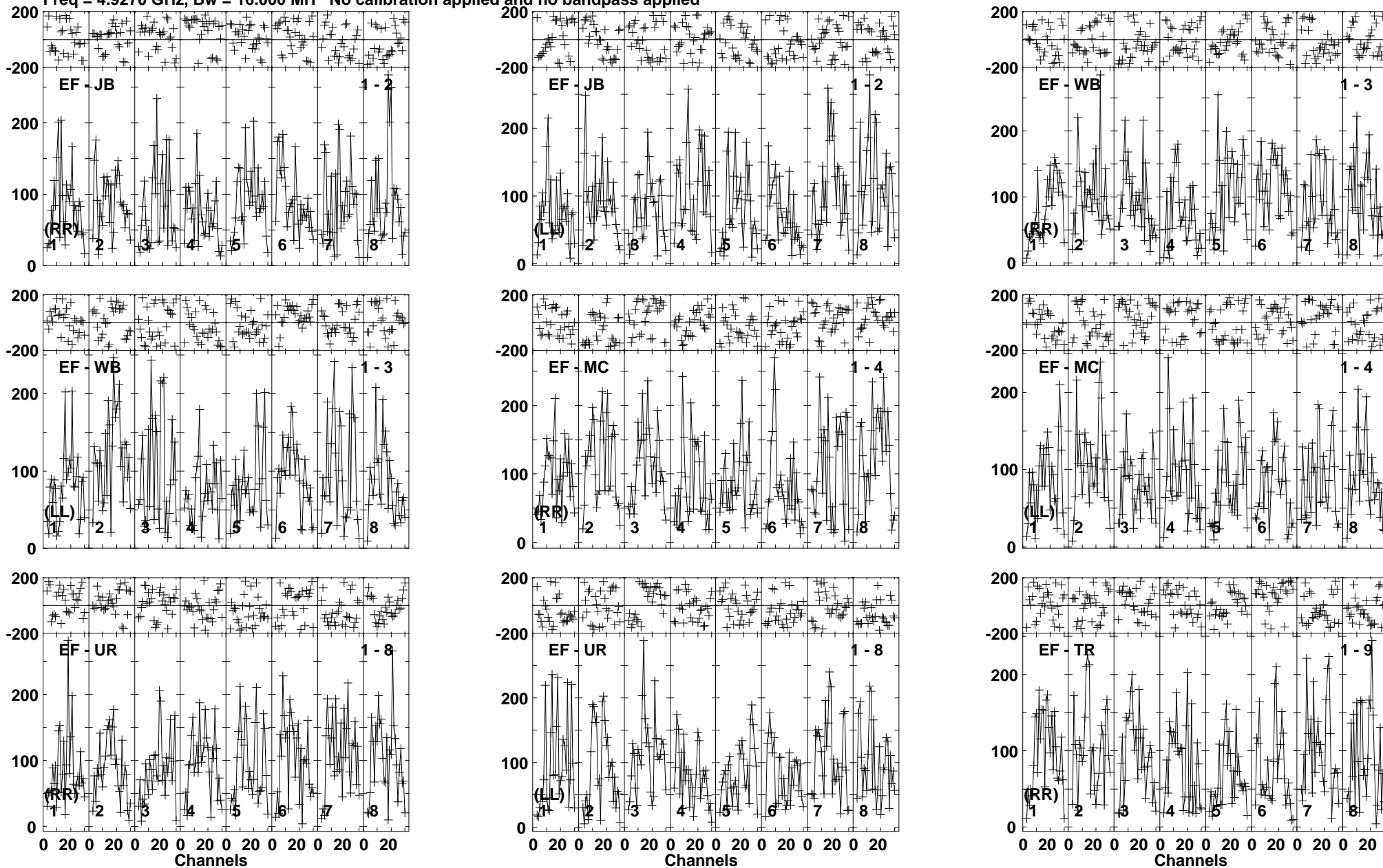
Lower frame: Micro Ampl Jy Top frame: Phas deg Vector averaged cross-power spectrum Baseline: EF (01) - JB (02) Timerange: 00/07:41:13 to 00/07:44:39
