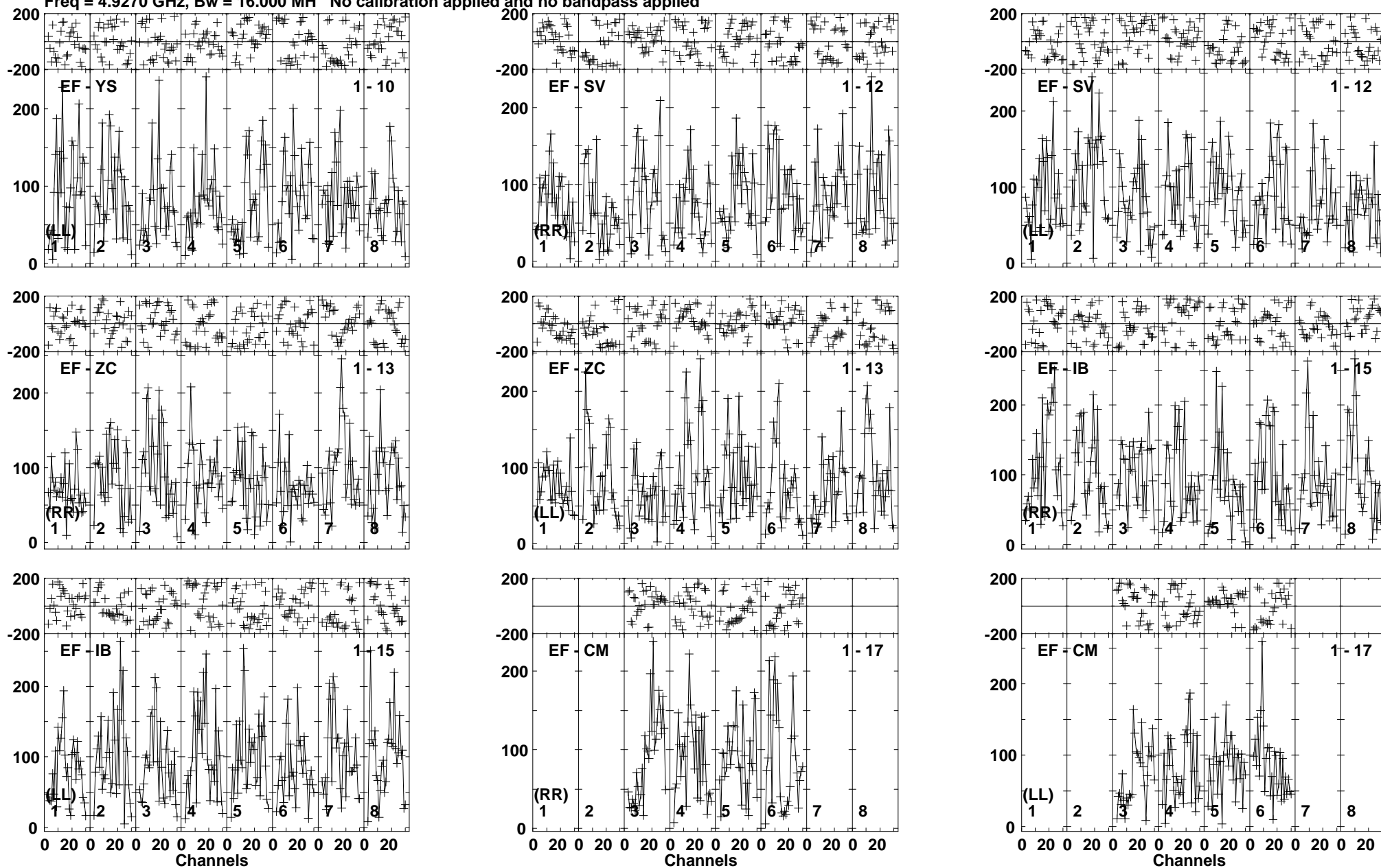
Lower frame: Micro Ampl Jy Top frame: Phas deg Vector averaged cross-power spectrum Baseline: EF (01) - YS (10) Timerange: 00/10:07:51 to 00/10:11:19
