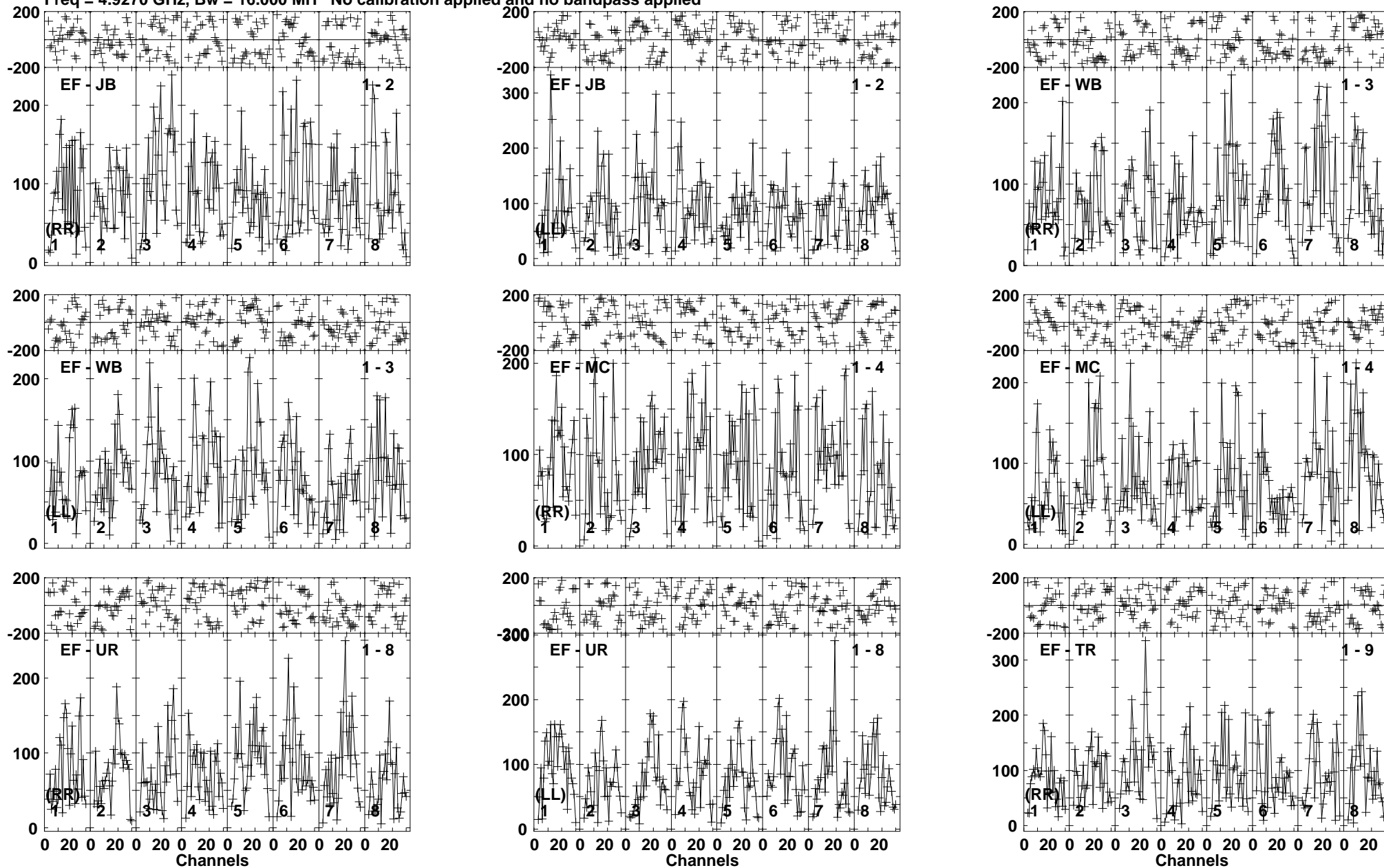
Lower frame: Micro Ampl Jy Top frame: Phas deg Vector averaged cross-power spectrum Baseline: EF (01) - JB (02) Timerange: 00/07:52:03 to 00/07:55:29
