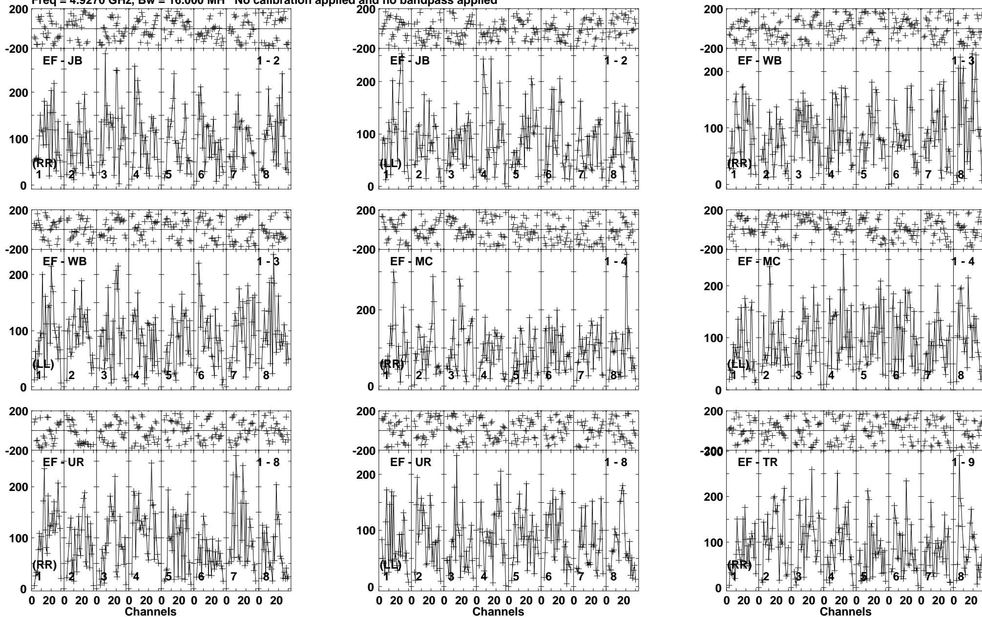
Lower frame: Micro Ampl Jy Top frame: Phas deg Vector averaged cross-power spectrum Baseline: EF (01) - JB (02) Timerange: 00/05:19:13 to 00/05:22:39
