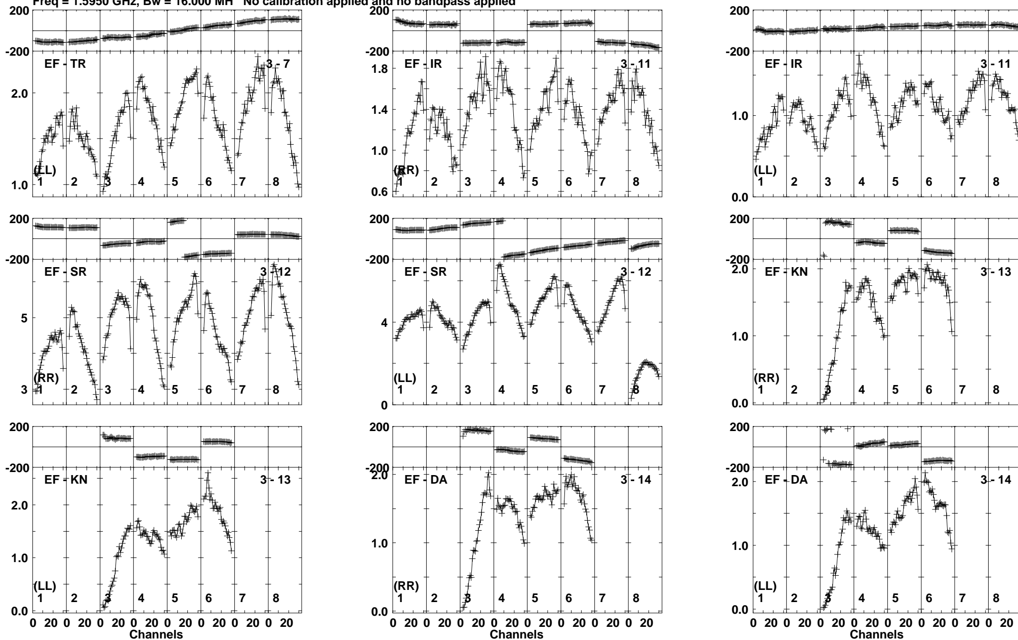
Lower frame: Milli Ampl Jy Top frame: Phas deg Vector averaged cross-power spectrum Baseline: EF (03) - TR (07) Timerange: 00/20:23:10 to 00/20:25:08
