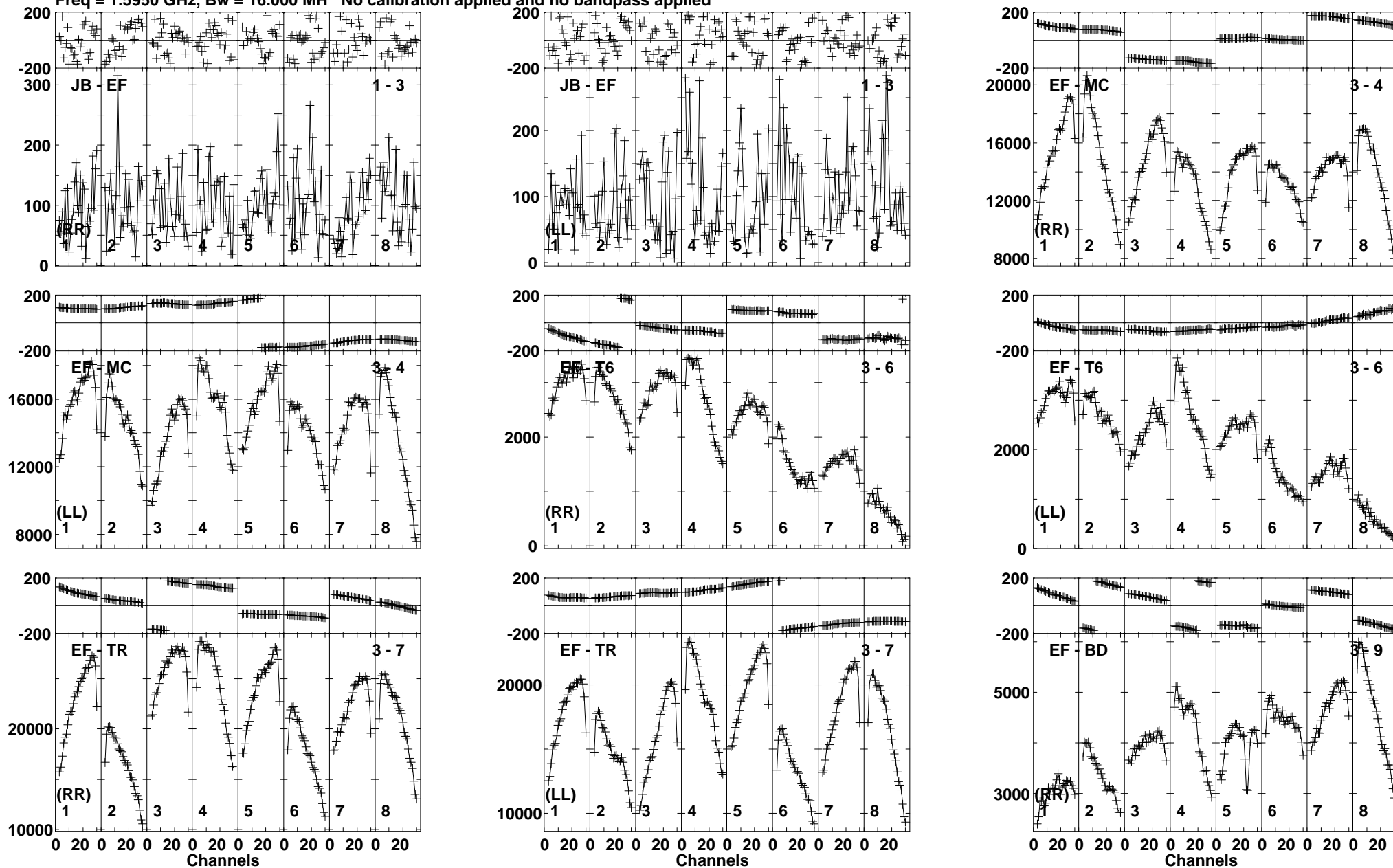
Lower frame: Micro Ampl Jy Top frame: Phas deg Vector averaged cross-power spectrum Baseline: JB (01) - EF (03) Timerange: 00/13:59:32 to 00/14:02:26
