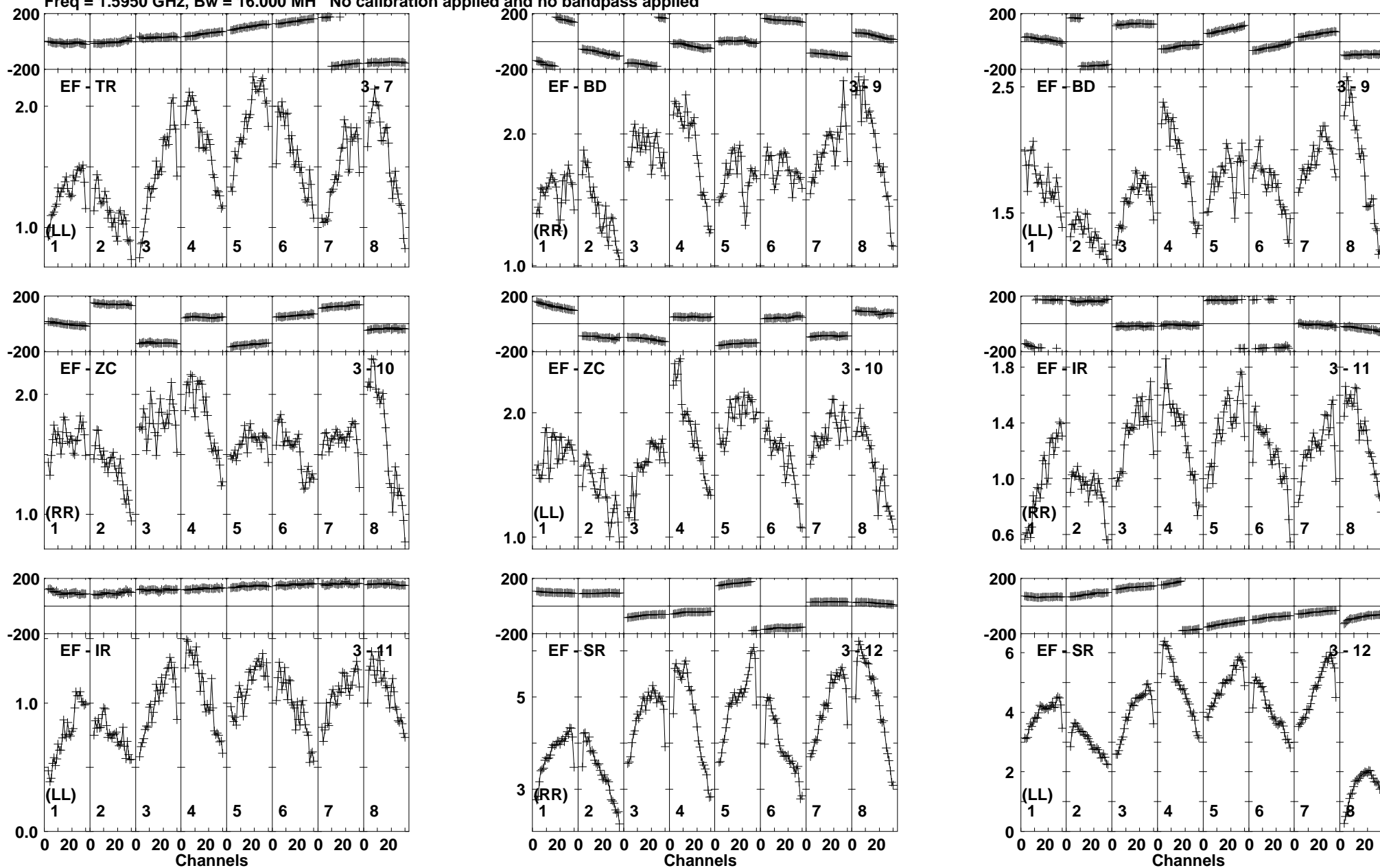
Lower frame: Milli Ampl Jy Top frame: Phas deg Vector averaged cross-power spectrum Baseline: EF (03) - TR (07) Timerange: 00:19:08:27 to 00:19:10:51
