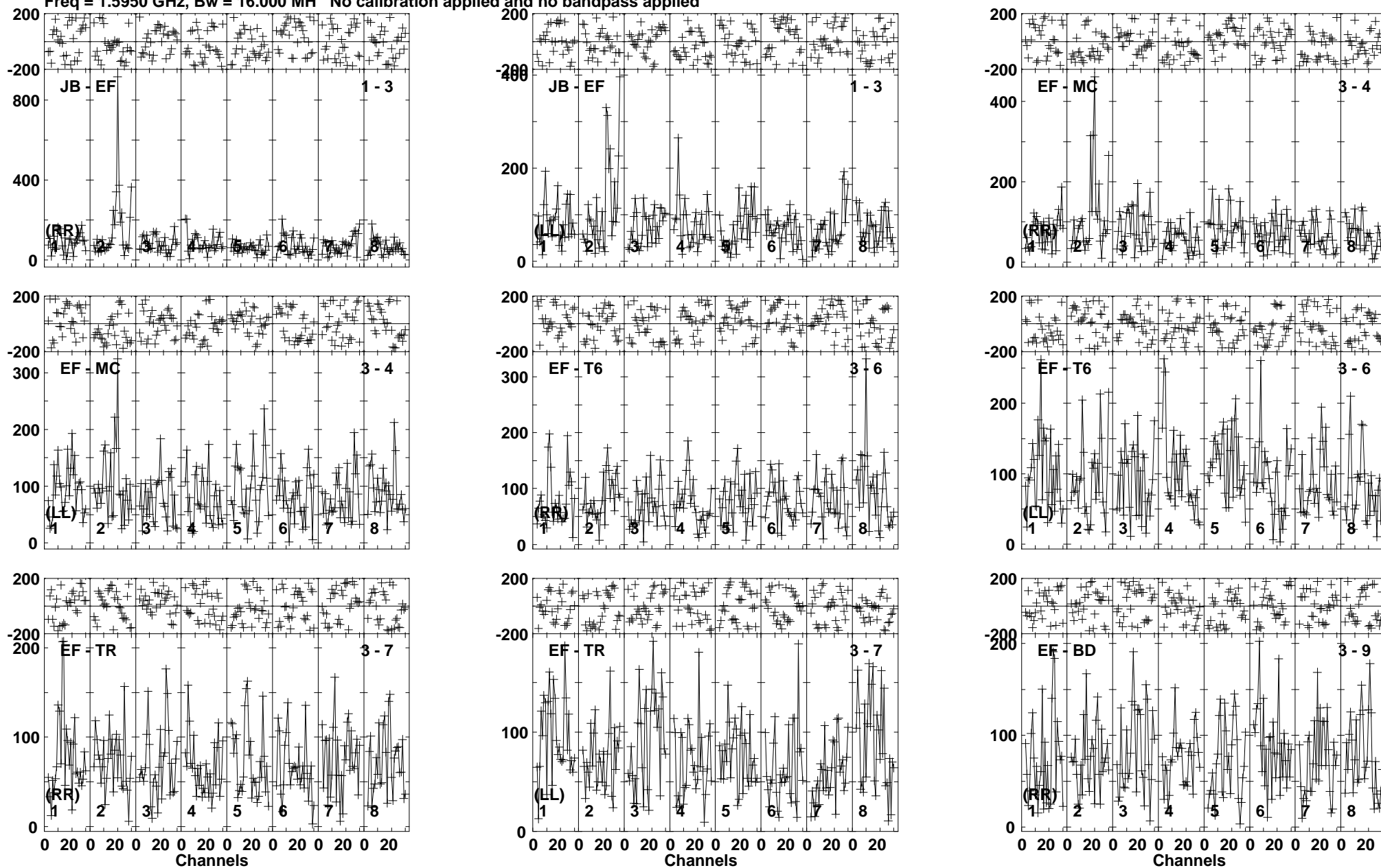
Lower frame: Micro Ampl Jy Top frame: Phas deg Vector averaged cross-power spectrum Baseline: JB (01) - EF (03) Timerange: 00/14:29:19 to 00/14:33:14
