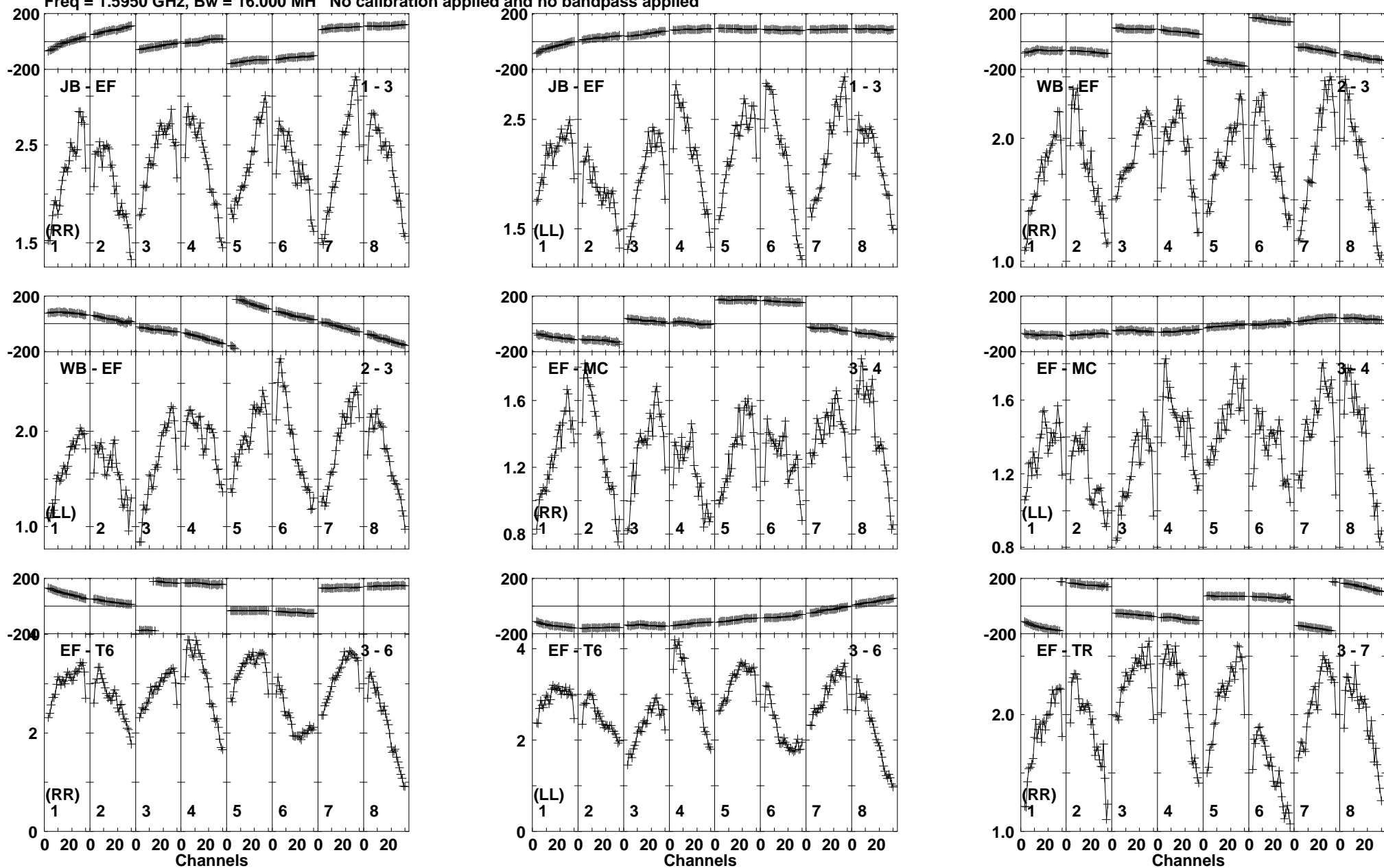
Lower frame: Milli Ampl Jy Top frame: Phas deg Vector averaged cross-power spectrum Baseline: JB (01) - EF (03) Timerange: 00/20:09:46 to 00/20:11:43
