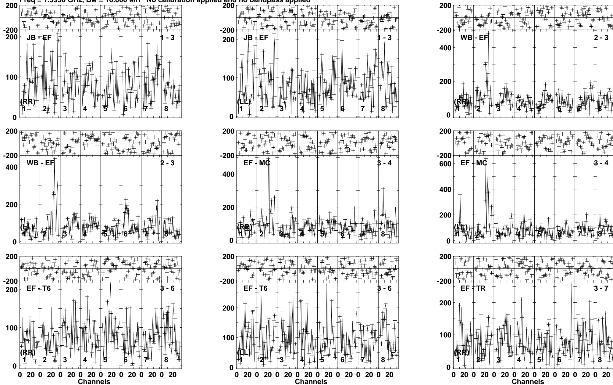
Lower frame: Micro Ampl Jy Top frame: Phas deg Vector averaged cross-power spectrum Baseline: JB (01) - EF (03) Timerange: 00/20:31:48 to 00/20:35:39
