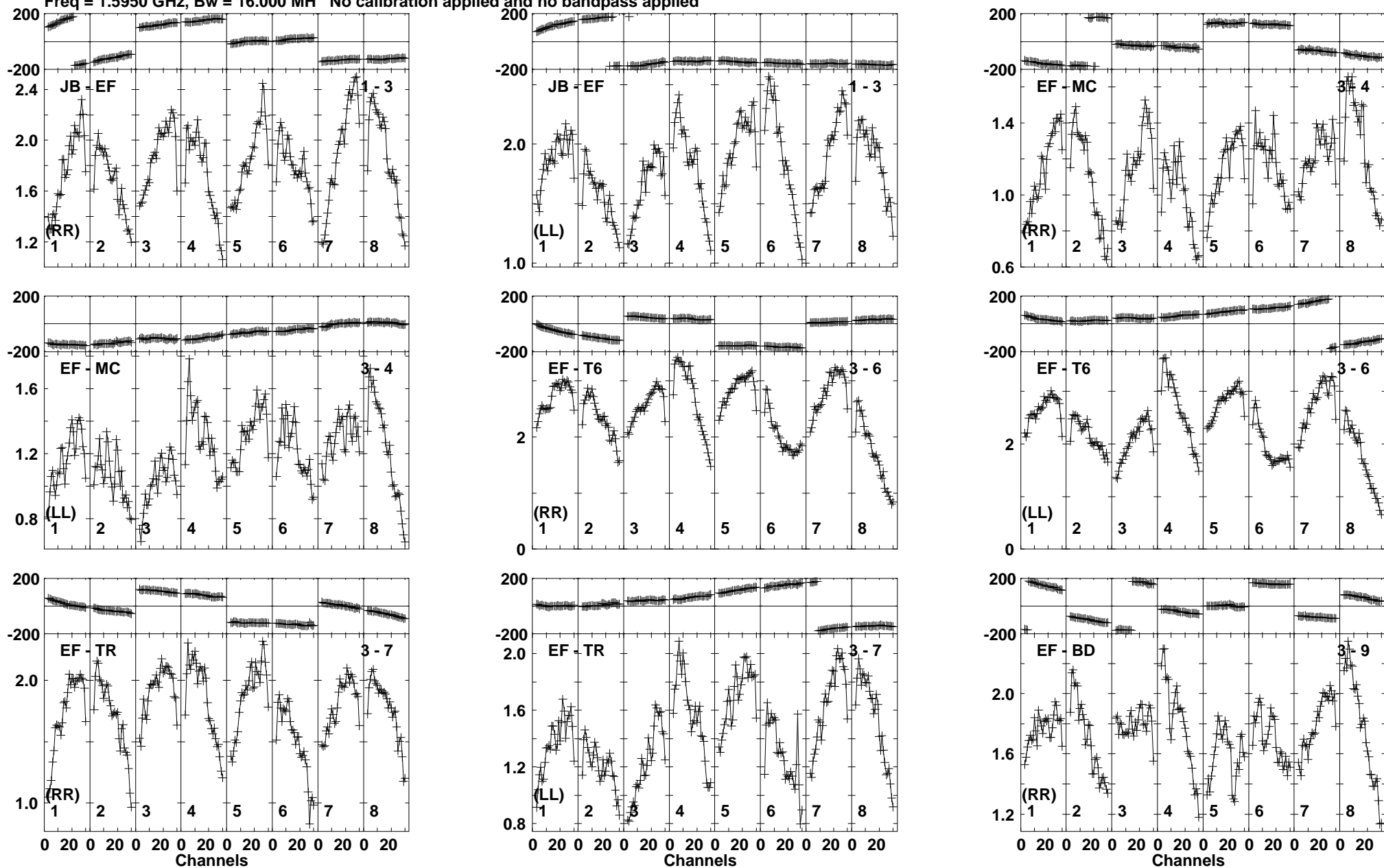
Lower frame: Milli Ampl Jy Top frame: Phas deg Vector averaged cross-power spectrum Baseline: JB (01) - EF (03) Timerange: 00/15:36:38 to 00/15:38:38
