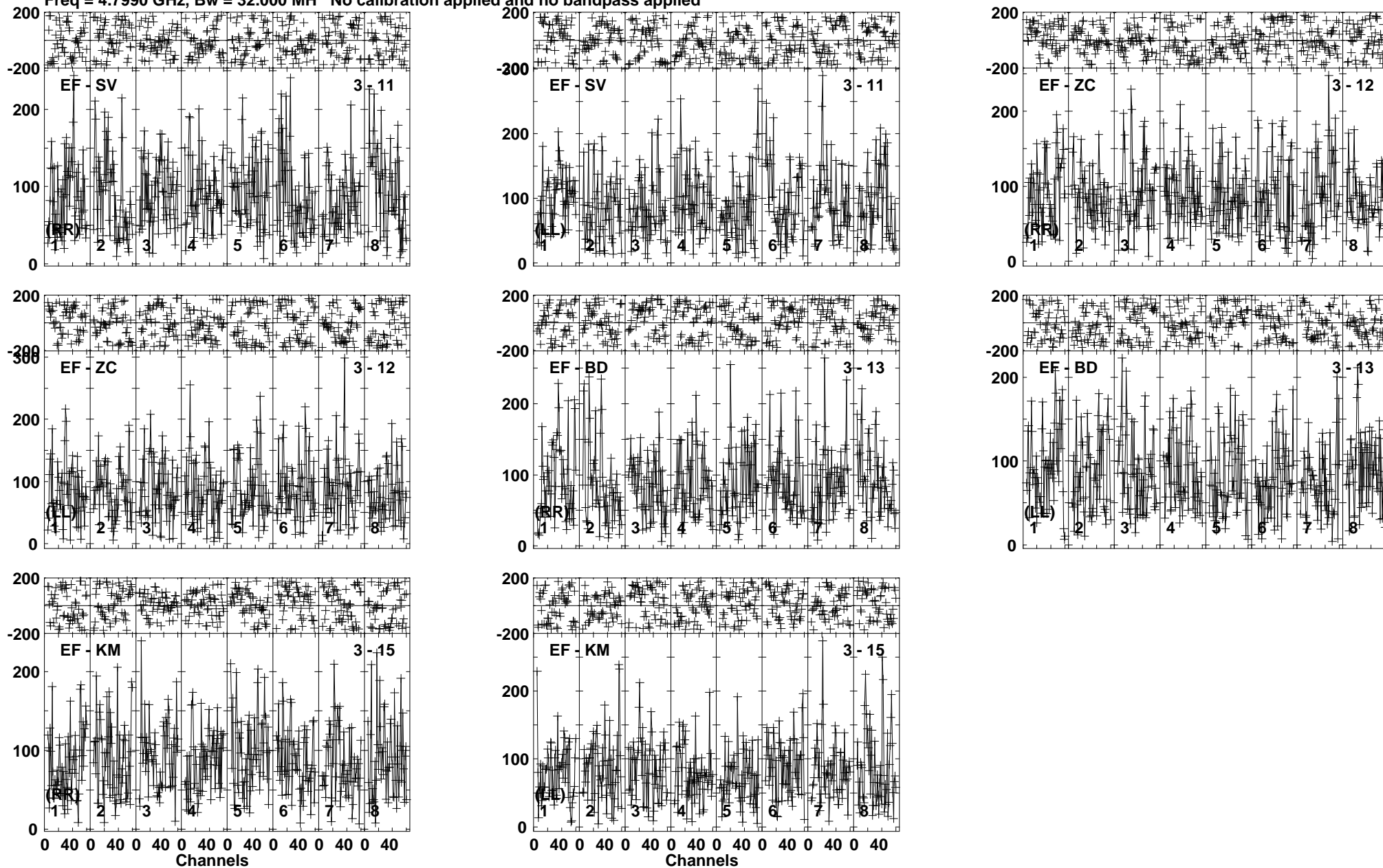
Lower frame: Micro Ampl Jy Top frame: Phas deg Vector averaged cross-power spectrum Baseline: EF (03) - SV (11) Timerange: 00/15:09:31 to 00/15:12:19
