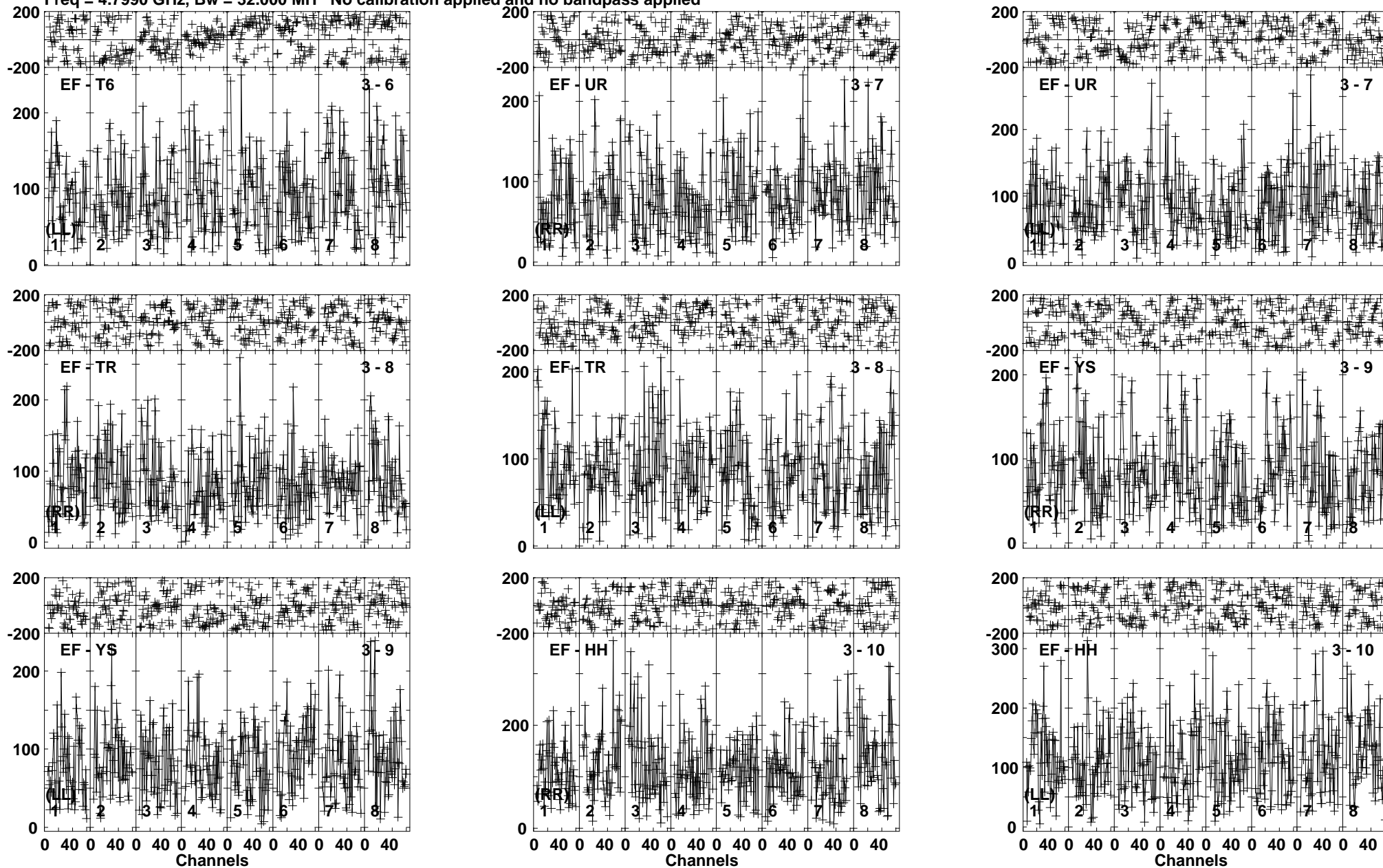
Lower frame: Micro Ampl Jy Top frame: Phas deg Vector averaged cross-power spectrum Baseline: EF (03) - T6 (06) Timerange: 00:13:50:31 to 00:13:53:19
