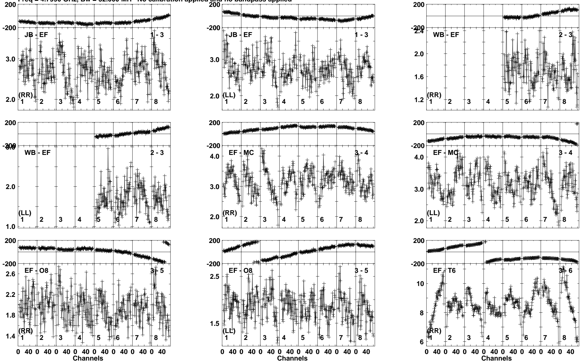
Lower frame: Milli Ampl Jy Top frame: Phas deg Vector averaged cross-power spectrum Baseline: JB (01) - EF (03) Timerange: 00/14:20:11 to 00/14:20:39
