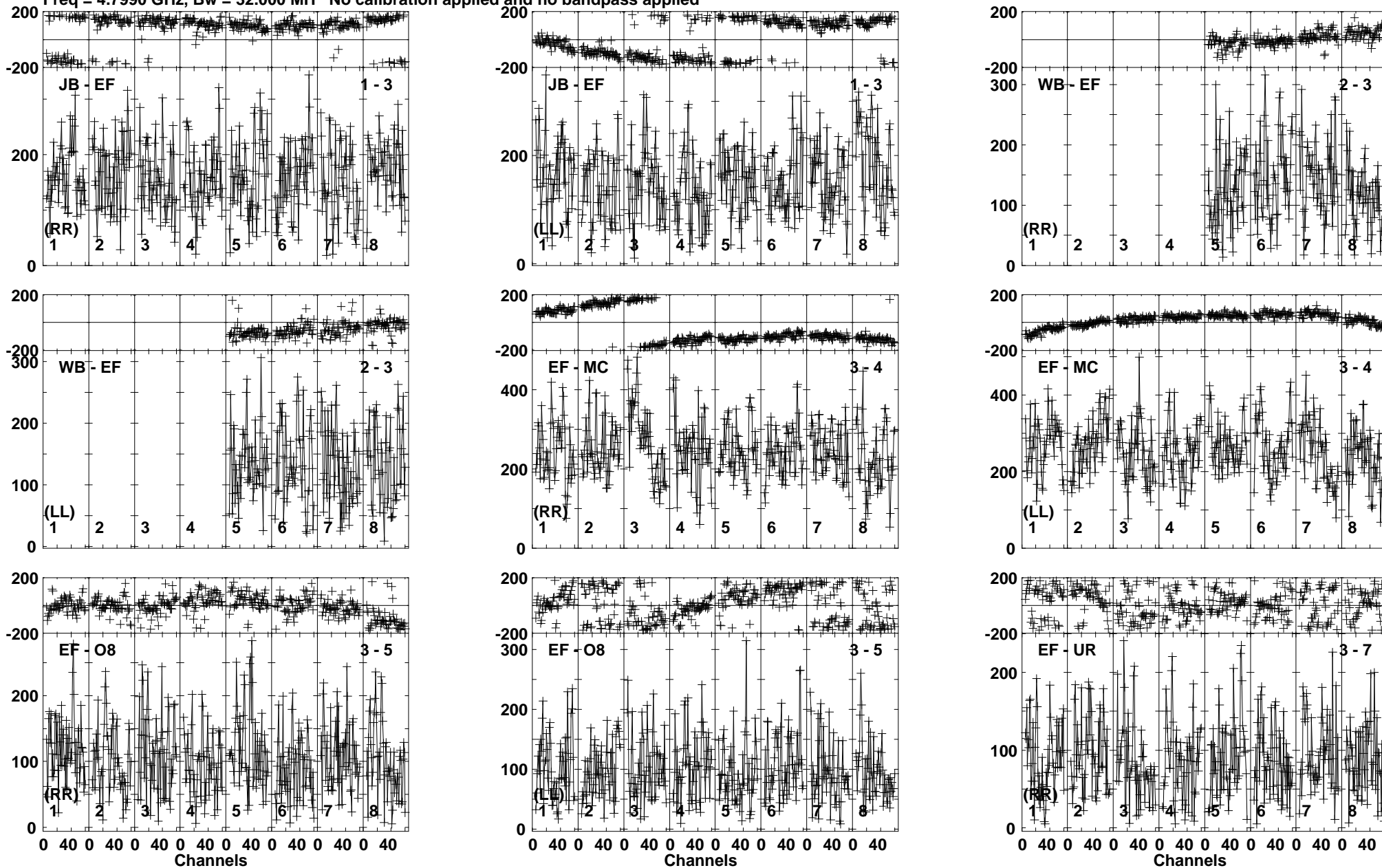
Lower frame: Micro Ampl Jy Top frame: Phas deg Vector averaged cross-power spectrum Baseline: JB (01) - EF (03) Timerange: 00/17:12:31 to 00/17:15:19
