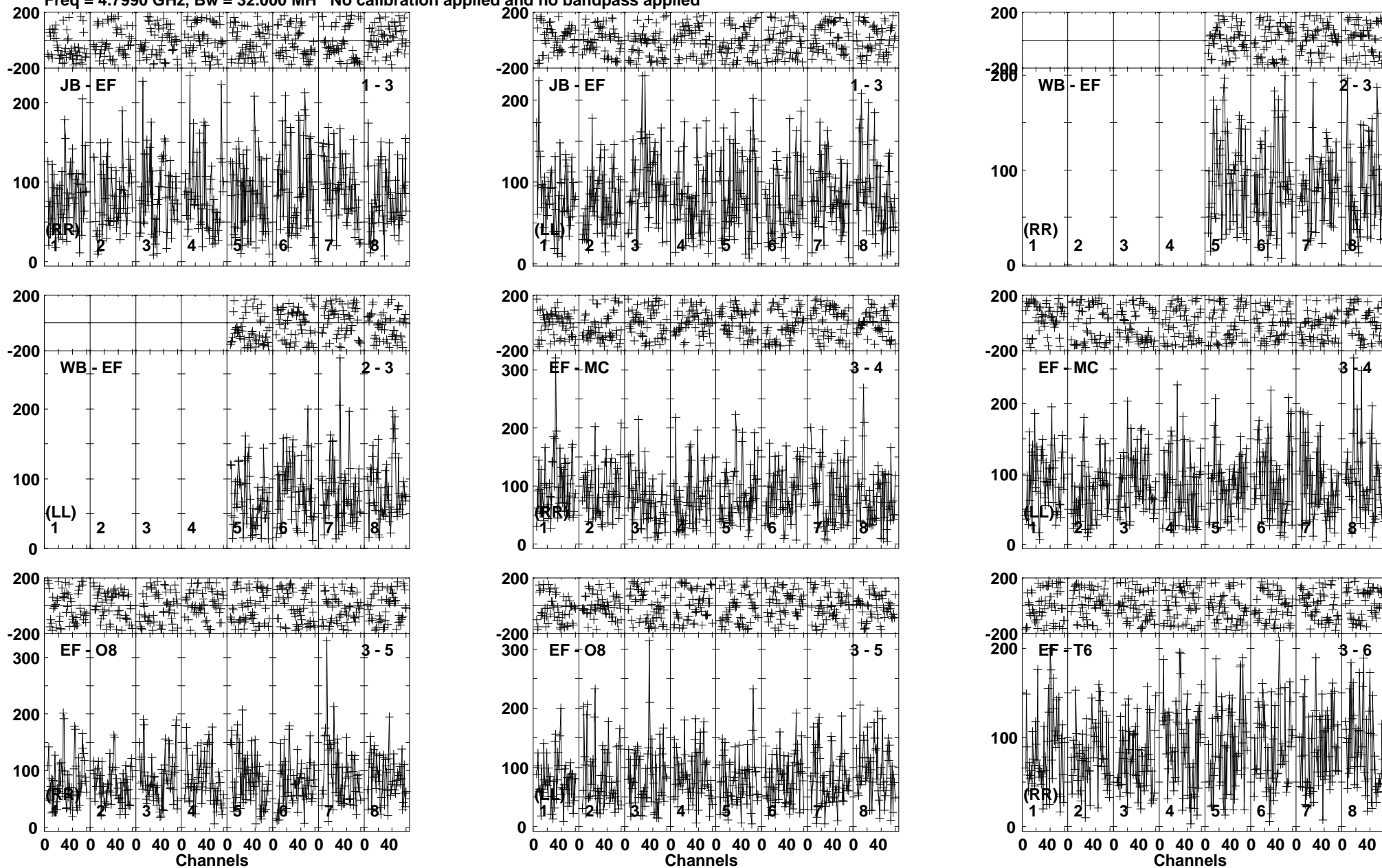
Lower frame: Micro Ampl Jy Top frame: Phas deg Vector averaged cross-power spectrum Baseline: JB (01) - EF (03) Timerange: 00/16:28:31 to 00/16:31:19
