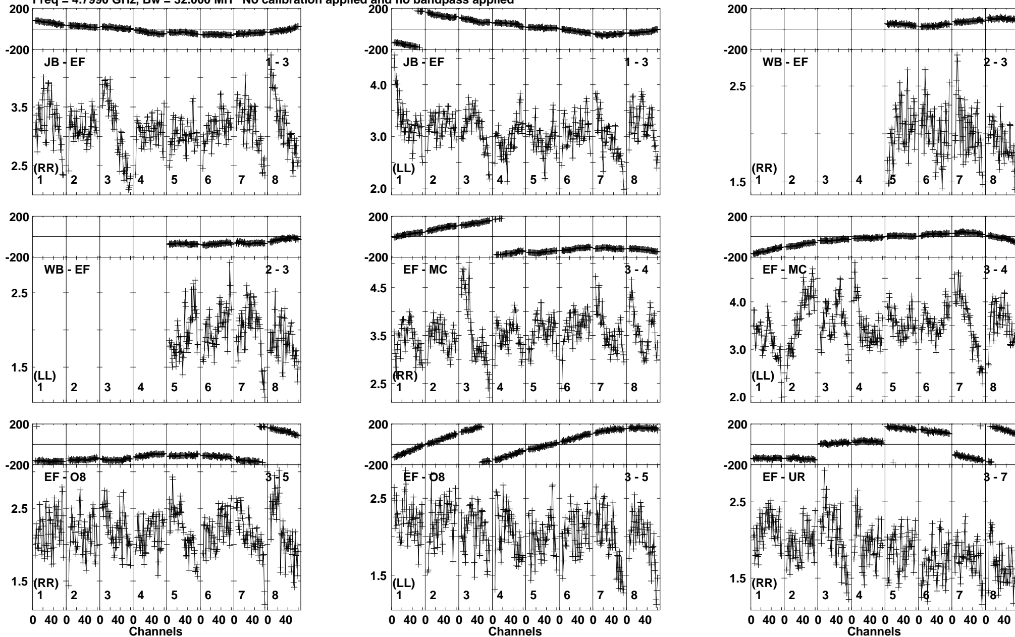
Lower frame: Milli Ampl Jy Top frame: Phas deg Vector averaged cross-power spectrum Baseline: JB (01) - EF (03) Timerange: 00/19:04:51 to 00/19:05:19
