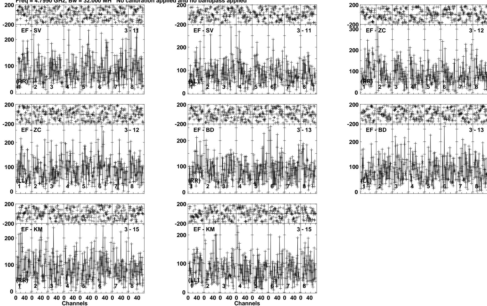
Lower frame: Micro Ampl Jy Top frame: Phas deg Vector averaged cross-power spectrum Baseline: EF (03) - SV (11) Timerange: 00/14:16:51 to 00/14:19:39
