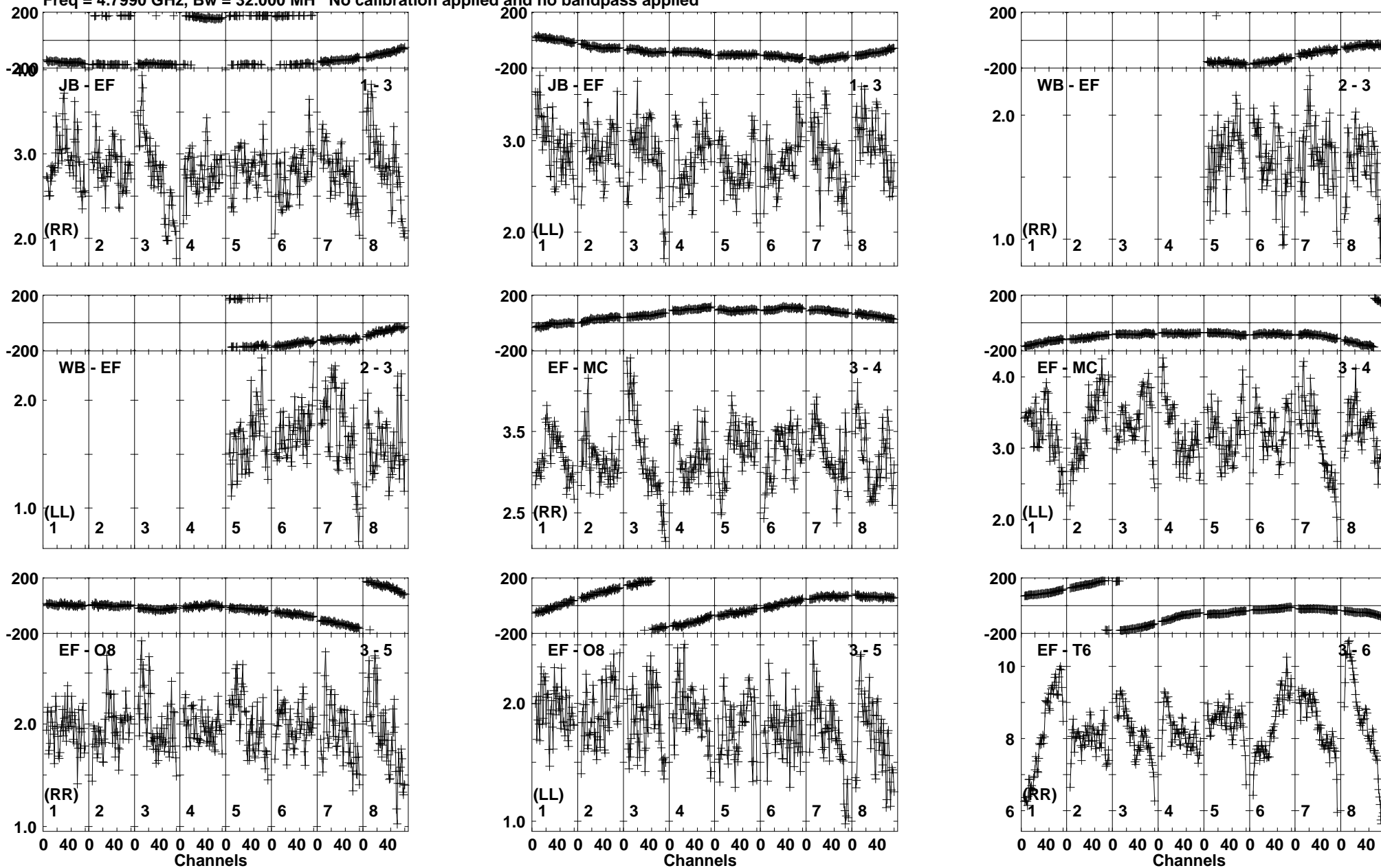
Lower frame: Milli Ampl Jy Top frame: Phas deg Vector averaged cross-power spectrum Baseline: JB (01) - EF (03) Timerange: 00/14:46:31 to 00/14:46:59
