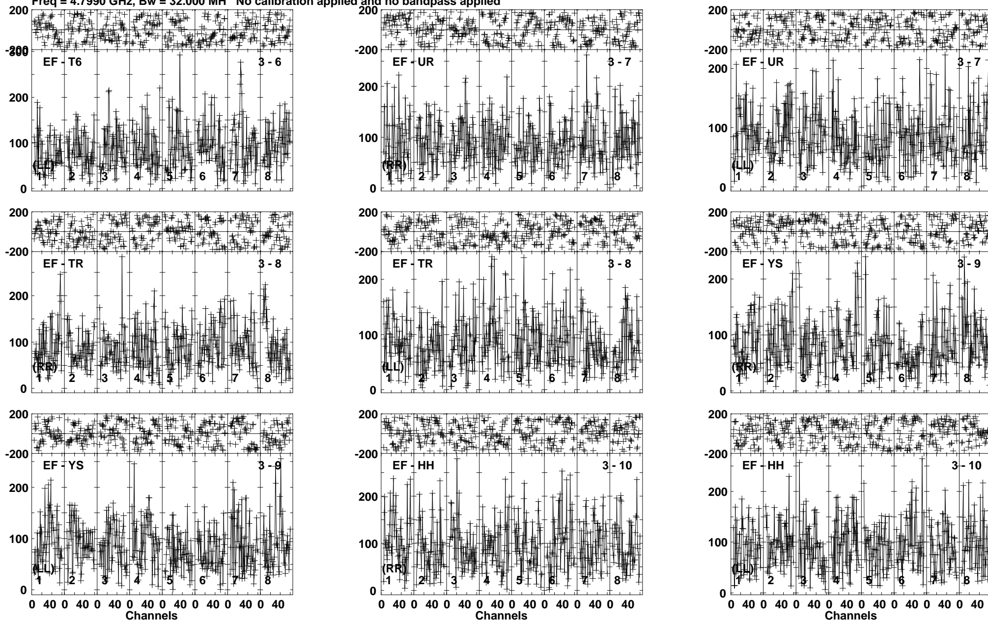
Lower frame: Micro Ampl Jy Top frame: Phas deg Vector averaged cross-power spectrum Baseline: EF (03) - T6 (06) Timerange: 00/16:10:51 to 00/16:13:39
