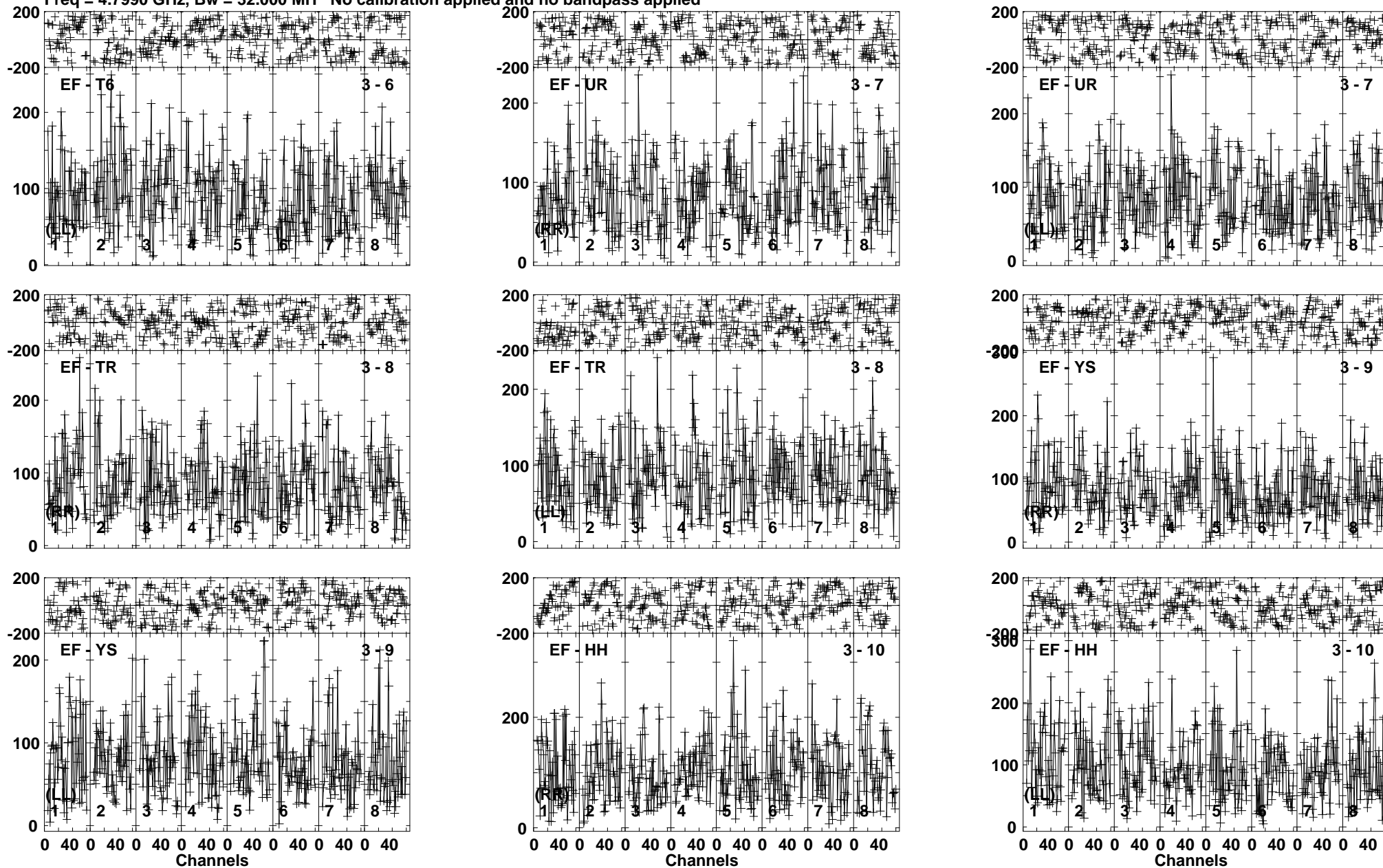
Lower frame: Micro Ampl Jy Top frame: Phas deg Vector averaged cross-power spectrum Baseline: EF (03) - T6 (06) Timerange: 00/14:38:51 to 00/14:41:39
