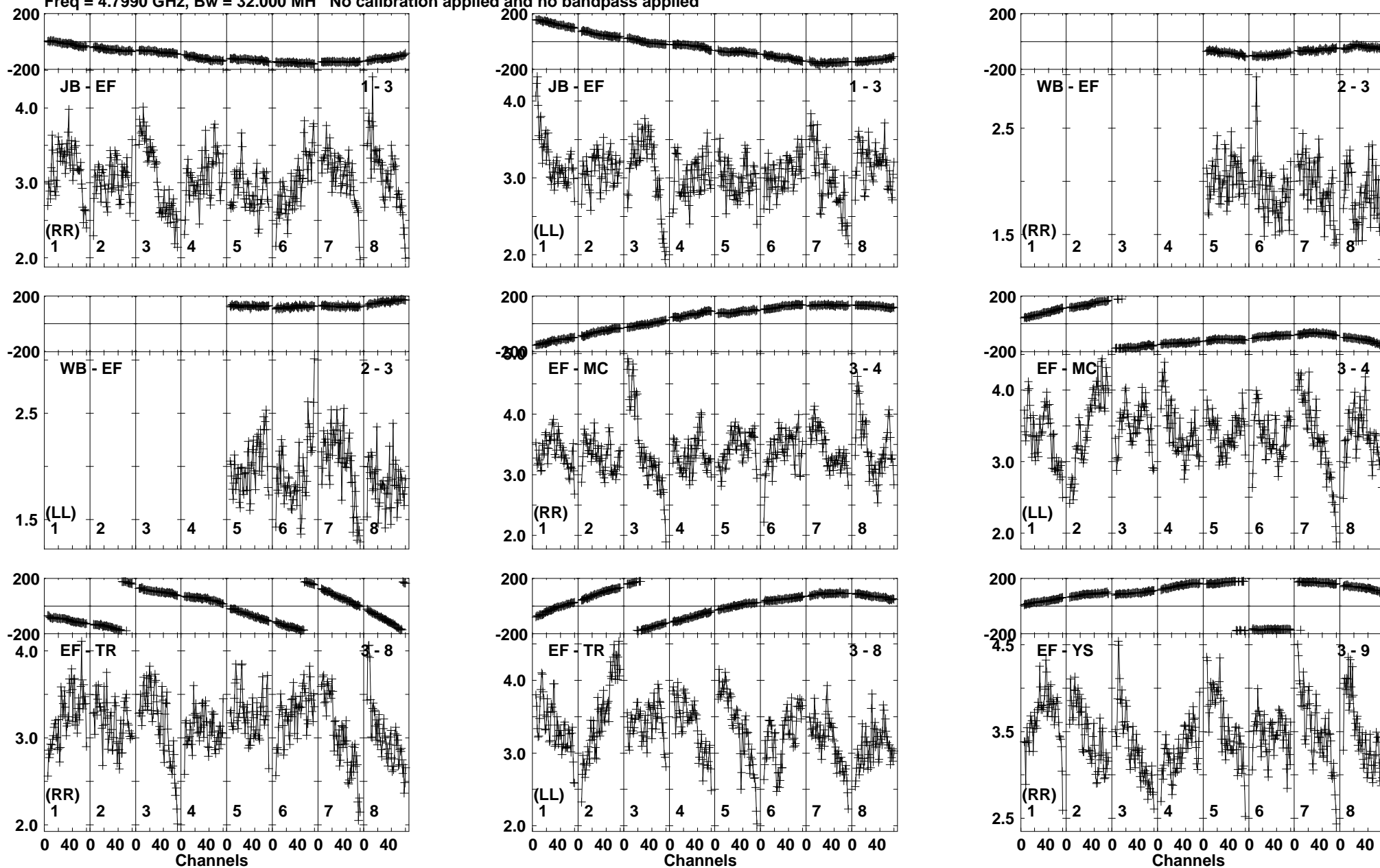
Lower frame: Milli Ampl Jy Top frame: Phas deg Vector averaged cross-power spectrum Baseline: JB (01) - EF (03) Timerange: 00/20:37:11 to 00/20:37:39
