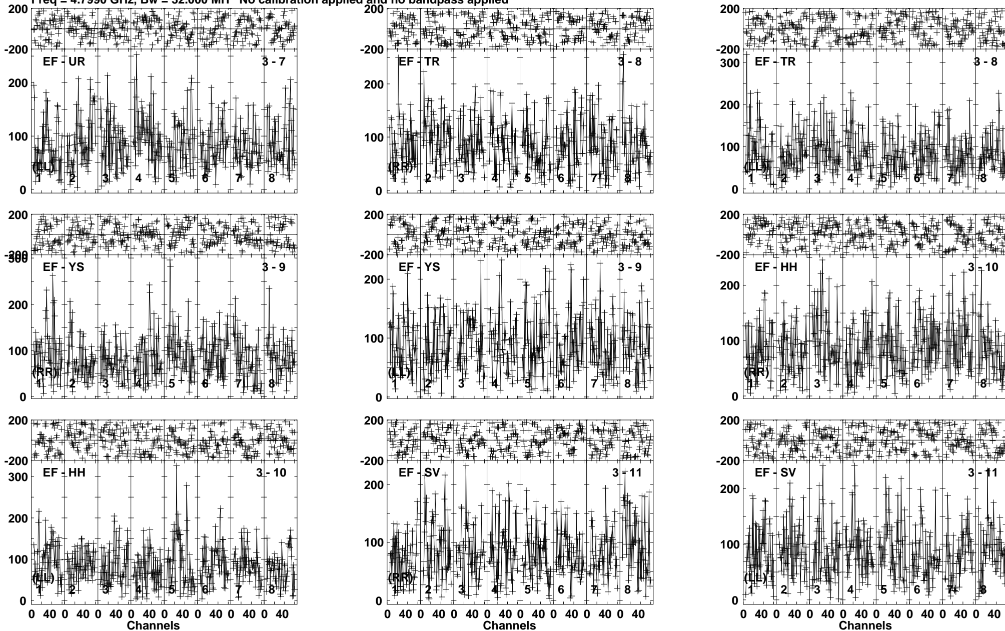
Lower frame: Micro Ampl Jy Top frame: Phas deg Vector averaged cross-power spectrum Baseline: EF (03) - UR (07) Timerange: 00/17:29:51 to 00/17:32:39
