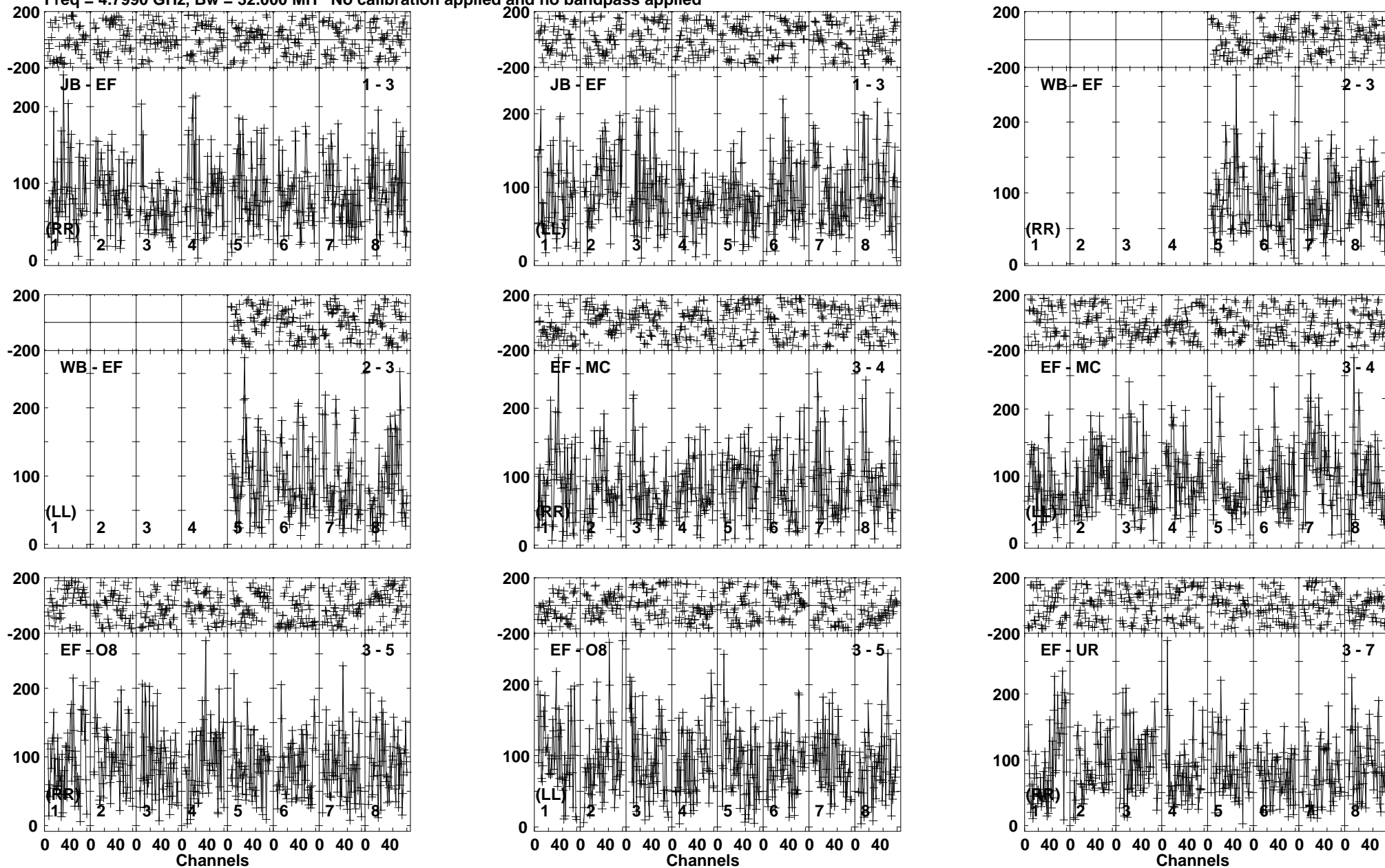
Lower frame: Micro Ampl Jy Top frame: Phas deg Vector averaged cross-power spectrum Baseline: JB (01) - EF (03) Timerange: 00/18:26:31 to 00/18:29:19
