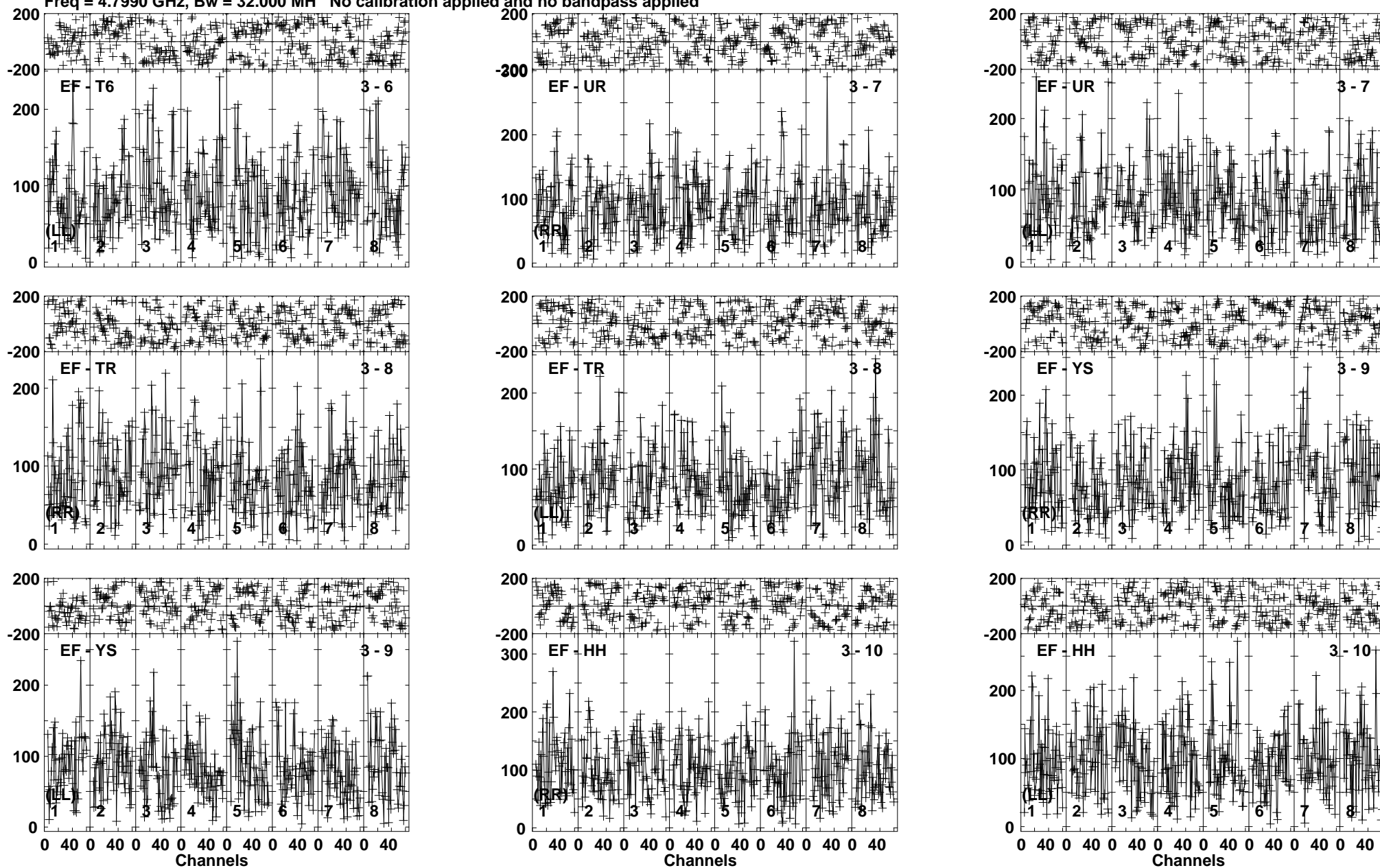
Lower frame: Micro Ampl Jy Top frame: Phas deg Vector averaged cross-power spectrum Baseline: EF (03) - T6 (06) Timerange: 00/15:44:31 to 00/15:47:19
