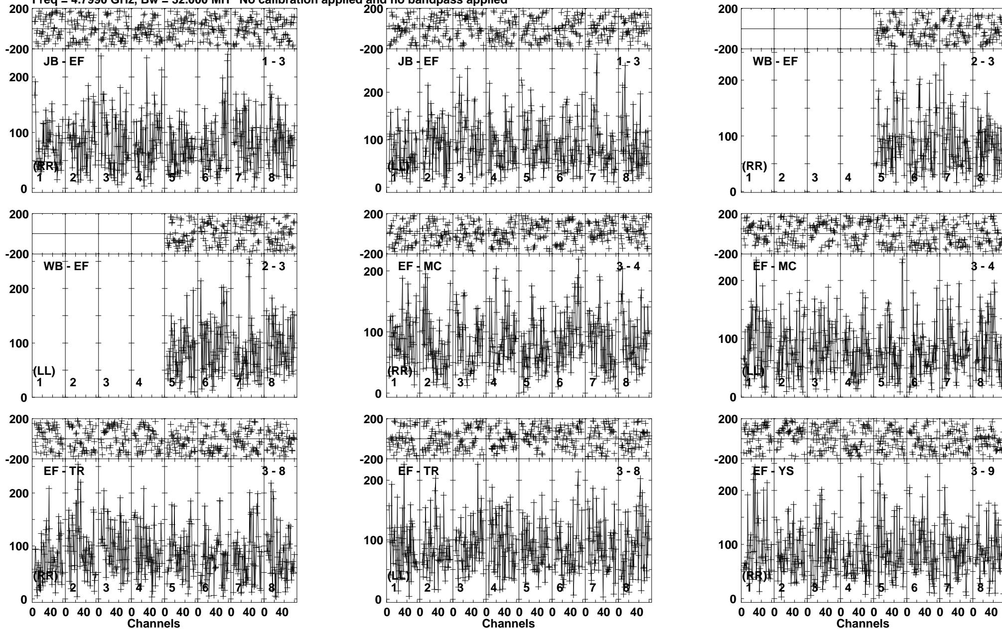
Lower frame: Micro Ampl Jy Top frame: Phas deg Vector averaged cross-power spectrum Baseline: JB (01) - EF (03) Timerange: 00/21:13:11 to 00/21:15:59
