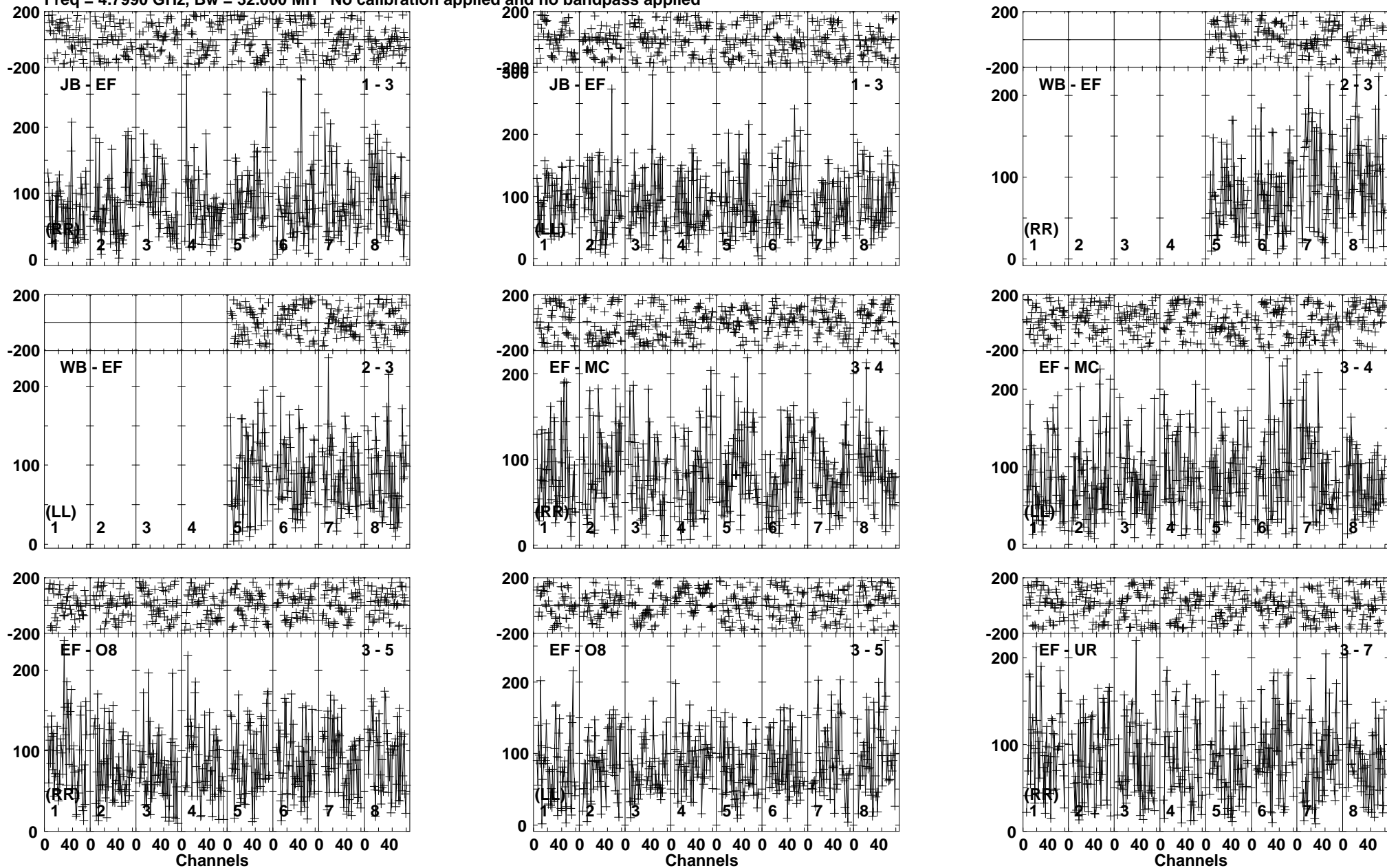
Lower frame: Micro Ampl Jy Top frame: Phas deg Vector averaged cross-power spectrum Baseline: JB (01) - EF (03) Timerange: 00:18:57:11 to 00:18:59:59
