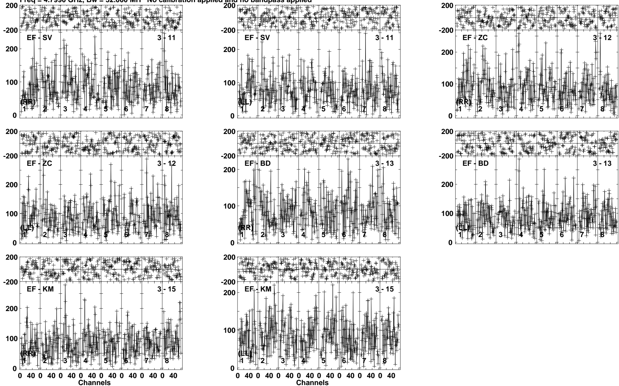
Lower frame: Micro Ampl Jy Top frame: Phas deg Vector averaged cross-power spectrum Baseline: EF (03) - SV (11) Timerange: 00/14:12:31 to 00/14:15:19
