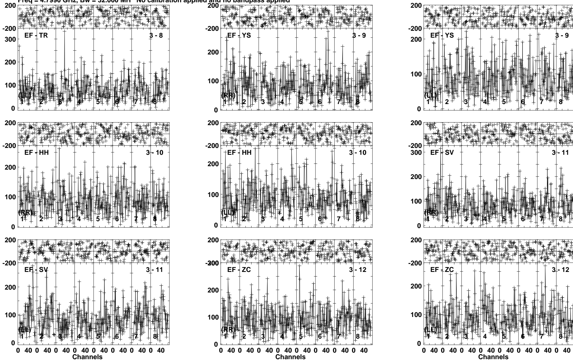
Lower frame: Micro Ampl Jy Top frame: Phas deg Vector averaged cross-power spectrum Baseline: EF (03) - TR (08) Timerange: 00/20:02:51 to 00/20:05:39
