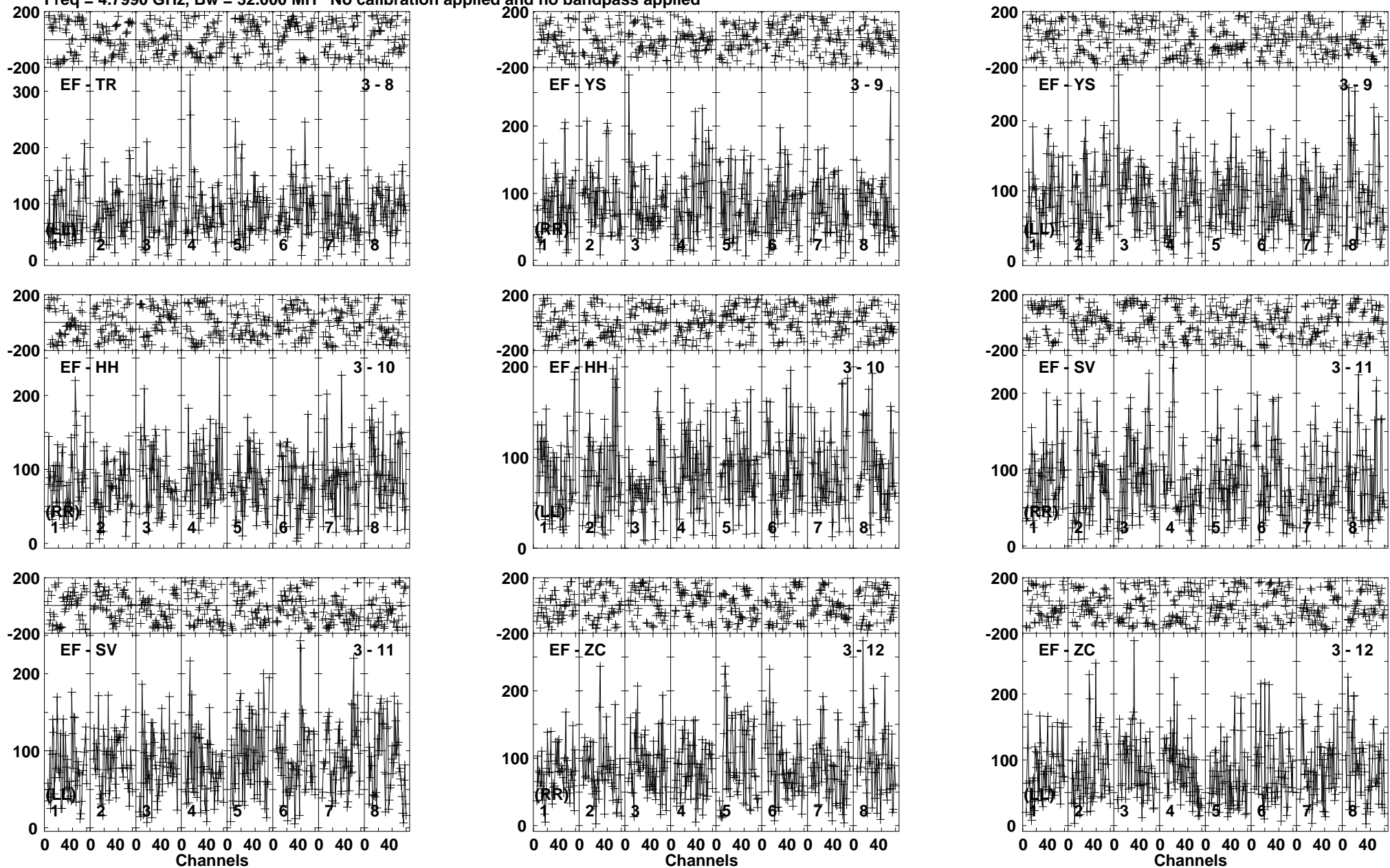
Lower frame: Micro Ampl Jy Top frame: Phas deg Vector averaged cross-power spectrum Baseline: EF (03) - TR (08) Timerange: 00:19:27:51 to 00:19:30:39
