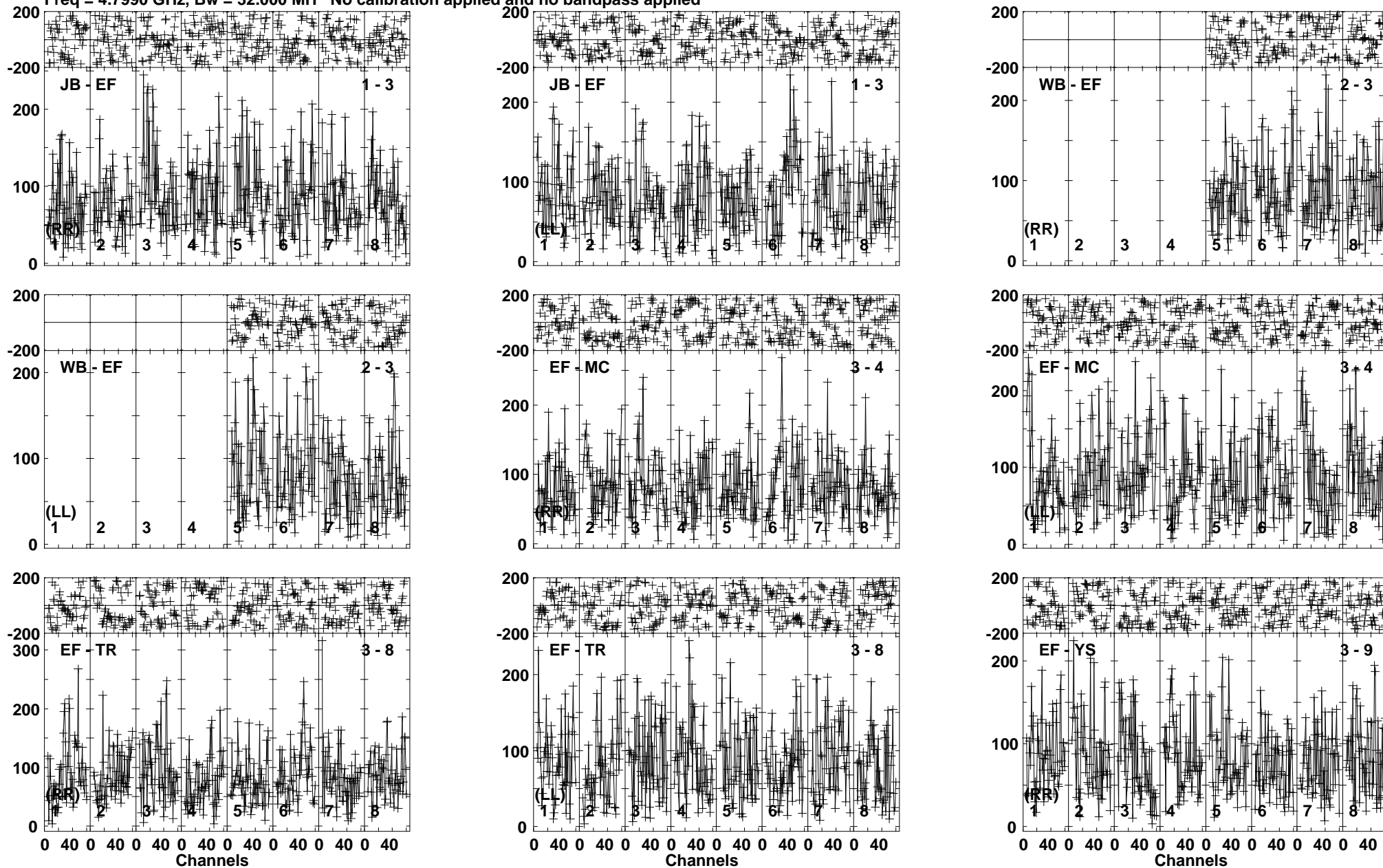
Lower frame: Micro Ampl Jy Top frame: Phas deg Vector averaged cross-power spectrum Baseline: JB (01) - EF (03) Timerange: 00/21:21:51 to 00/21:24:39
