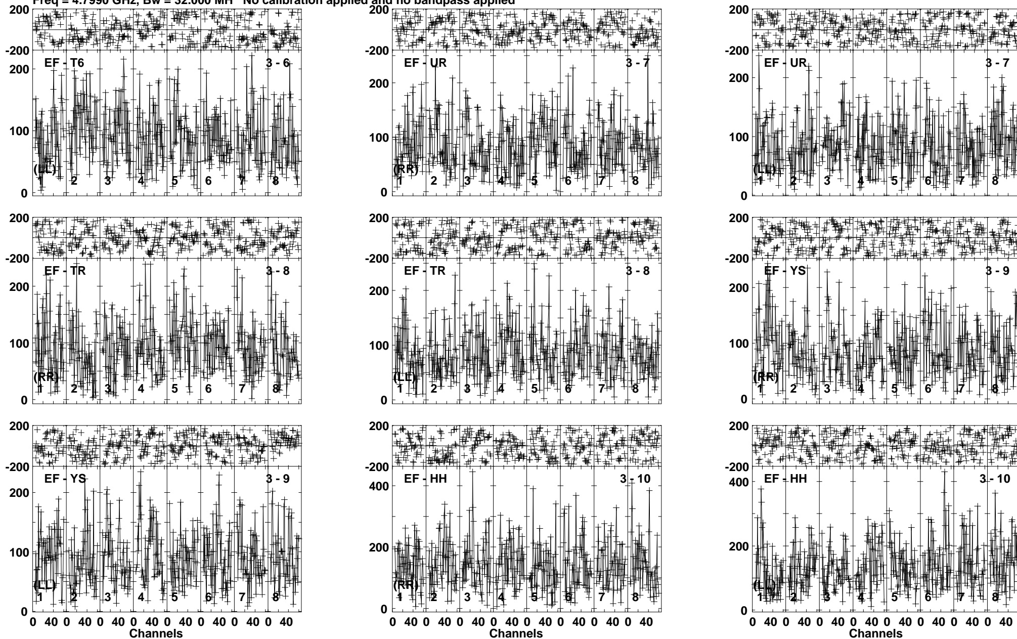
Lower frame: Micro Ampl Jy Top frame: Phas deg Vector averaged cross-power spectrum Baseline: EF (03) - T6 (06) Timerange: 00/14:29:51 to 00/14:32:39
