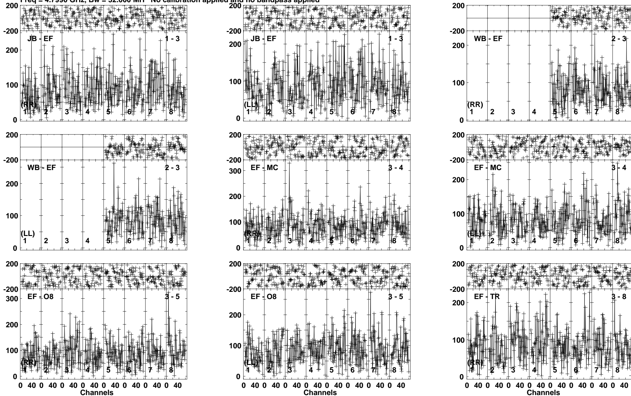
Lower frame: Micro Ampl Jy Top frame: Phas deg Vector averaged cross-power spectrum Baseline: JB (01) - EF (03) Timerange: 00:19:45:31 to 00:19:48:19
