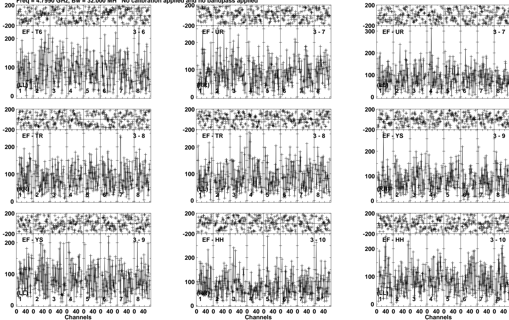
Lower frame: Micro Ampl Jy Top frame: Phas deg Vector averaged cross-power spectrum Baseline: EF (03) - T6 (06) Timerange: 00/16:02:11 to 00/16:04:59
