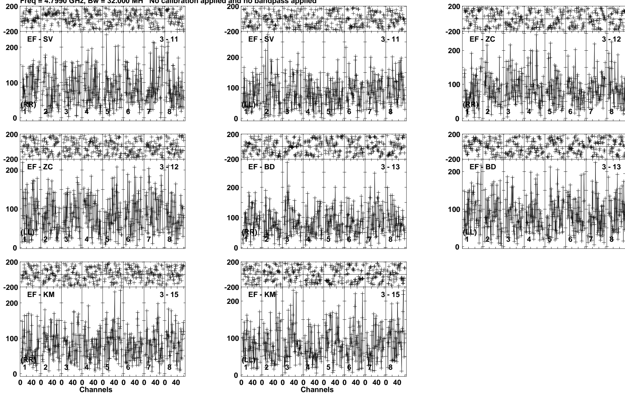
Lower frame: Micro Ampl Jy Top frame: Phas deg Vector averaged cross-power spectrum Baseline: EF (03) - SV (11) Timerange: 00/14:21:11 to 00/14:23:59
