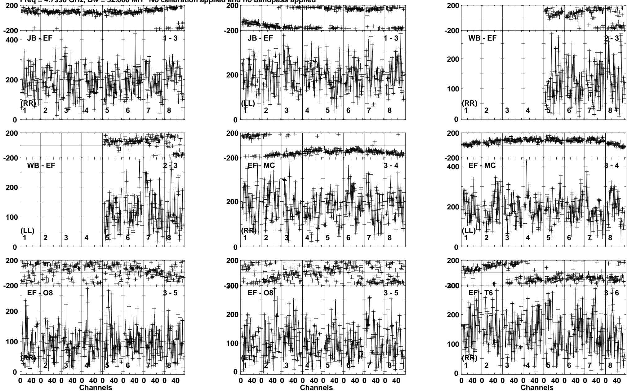
Lower frame: Micro Ampl Jy Top frame: Phas deg Vector averaged cross-power spectrum Baseline: JB (01) - EF (03) Timerange: 00/15:00:51 to 00/15:03:39
