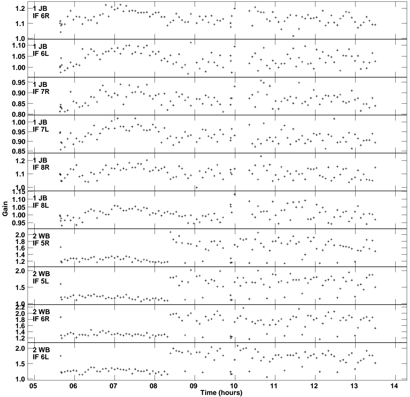
Plot file version 2 created 20-MAY-2020 16:02:38 Gain amp vs UTC time for J2052+1619.MULTI.1 SN 2 Rpol & Lpol IF 1 - 8
