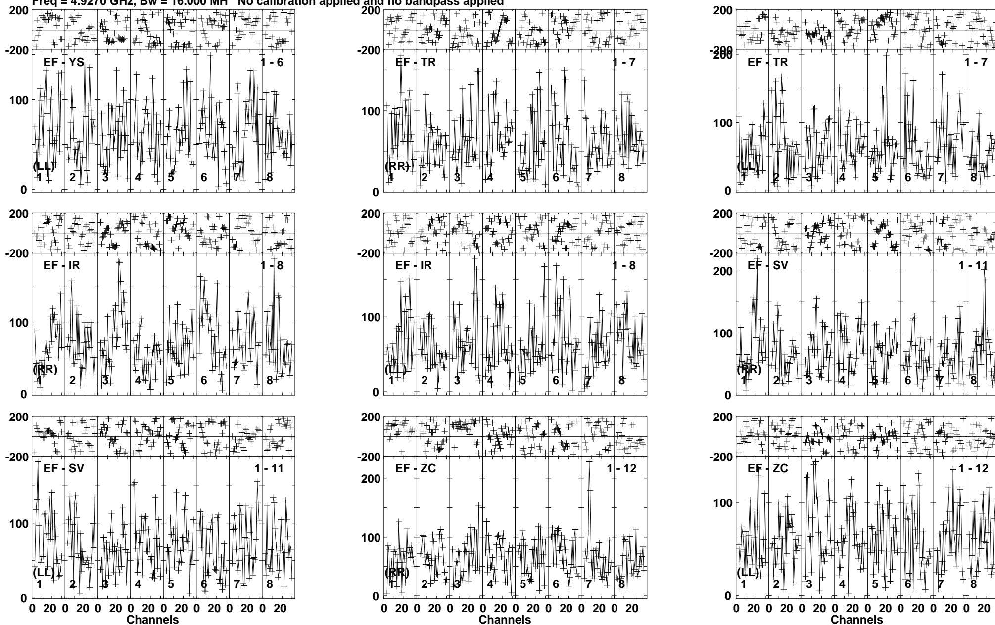
Lower frame: Micro Ampl Jy Top frame: Phas deg Vector averaged cross-power spectrum Baseline: EF (01) - YS (06) Timerange: 00/23:22:11 to 00/23:27:09
