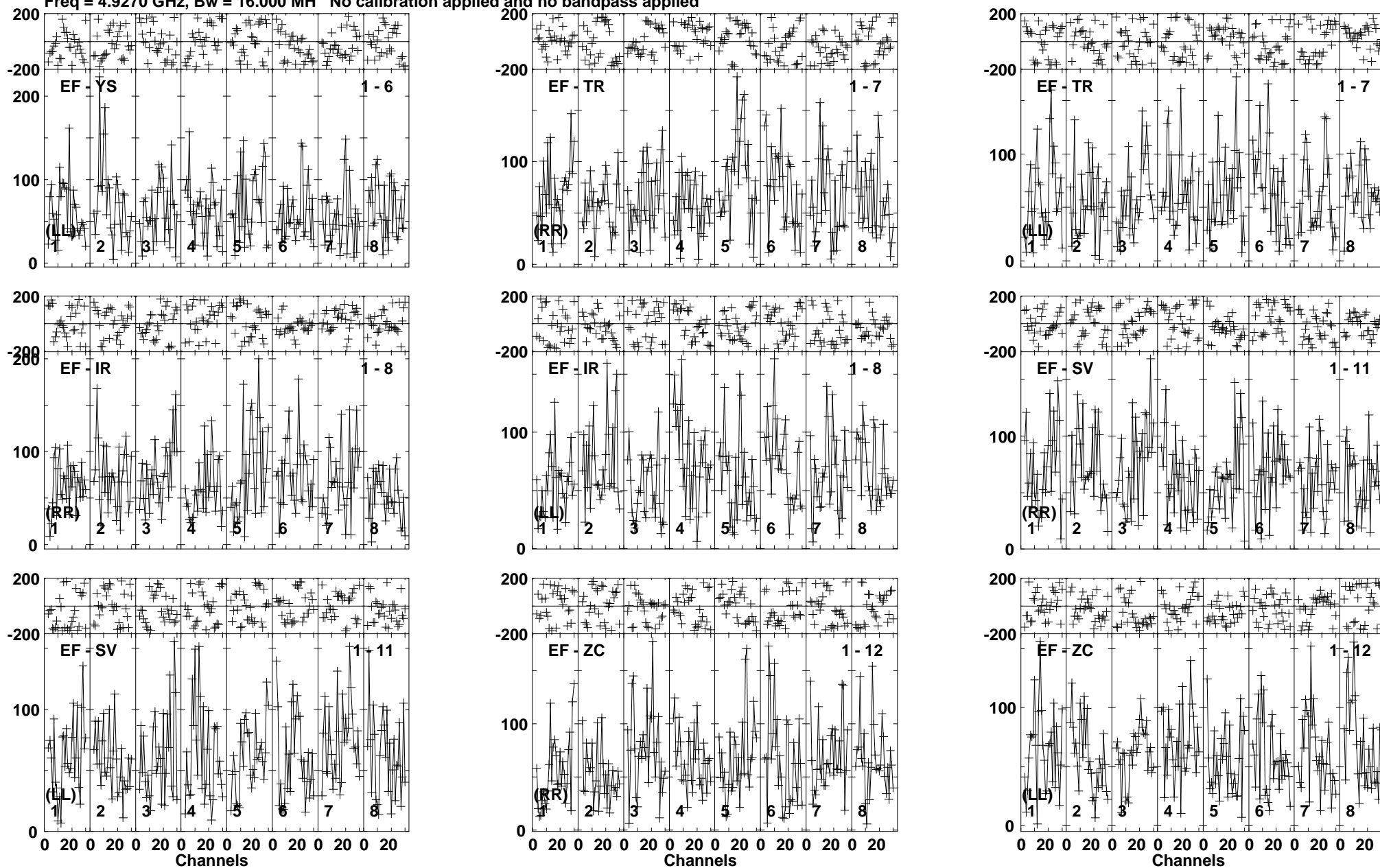
Lower frame: Micro Ampl Jy Top frame: Phas deg Vector averaged cross-power spectrum Baseline: EF (01) - YS (06) Timerange: 01/00:45:41 to 01/00:50:39
