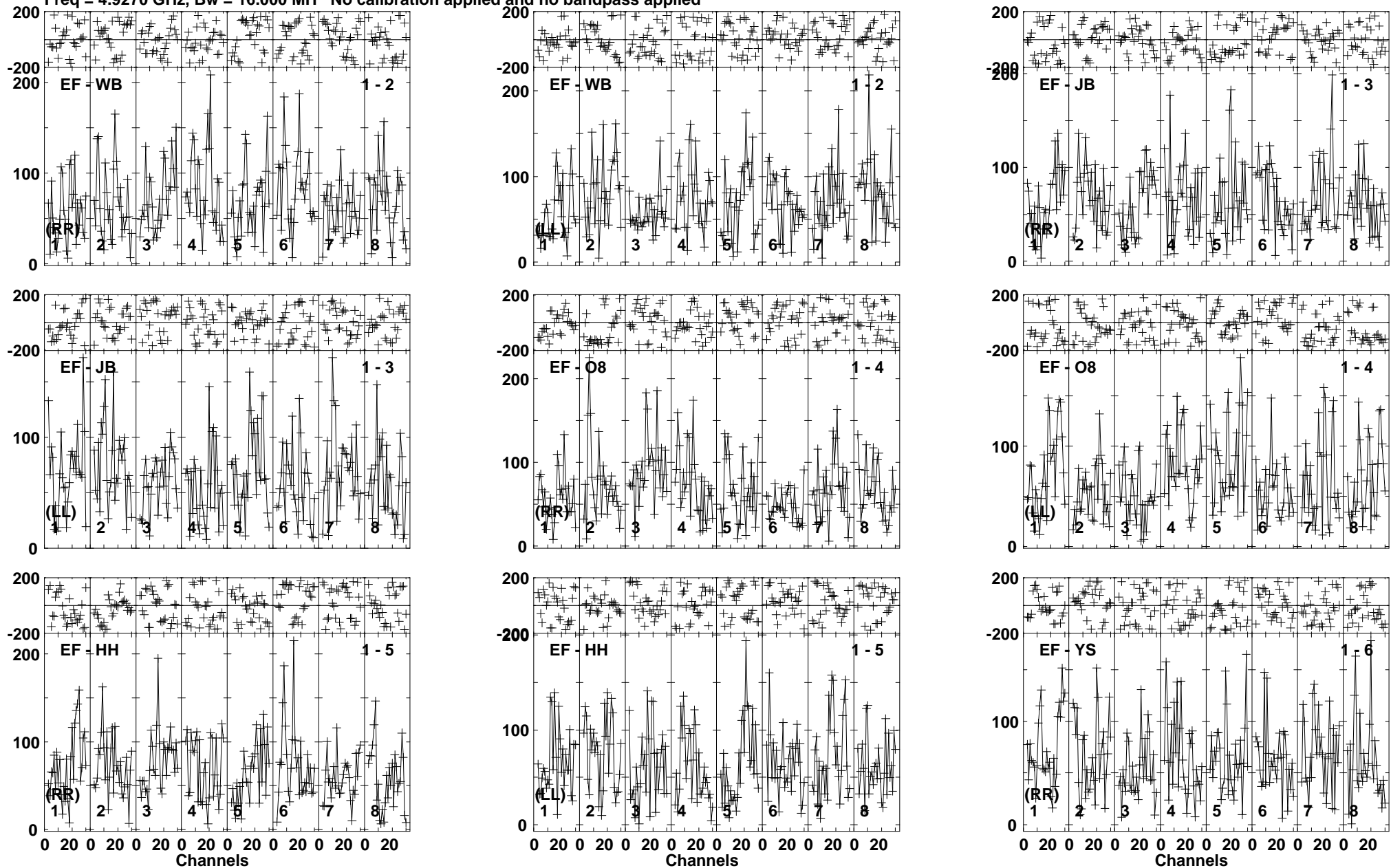
Lower frame: Micro Ampl Jy Top frame: Phas deg Vector averaged cross-power spectrum Baseline: EF (01) - WB (02) Timerange: 00/23:52:31 to 00/23:57:29
