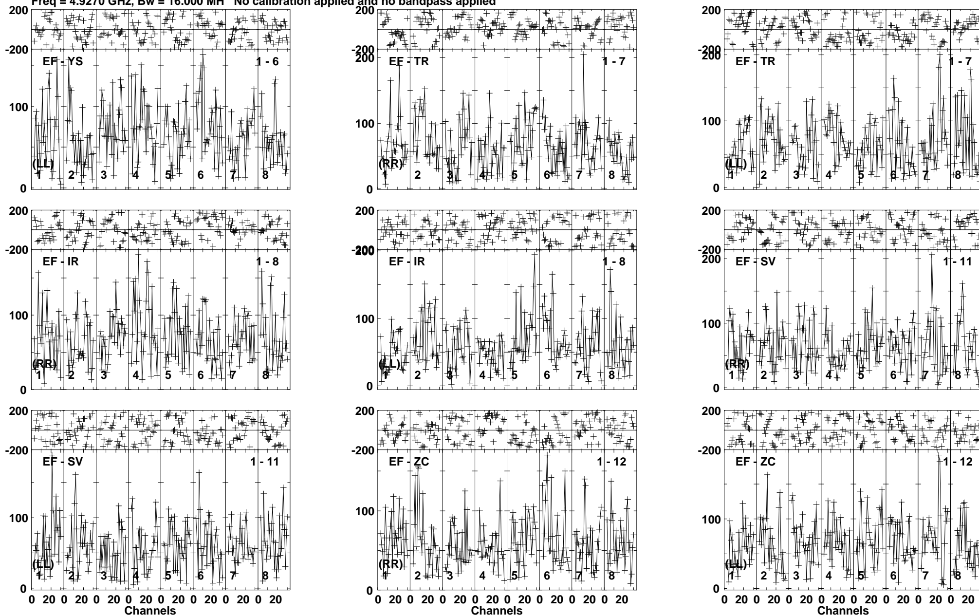
Lower frame: Micro Ampl Jy Top frame: Phas deg Vector averaged cross-power spectrum Baseline: EF (01) - YS (06) Timerange: 01/00:15:21 to 01/00:20:19
