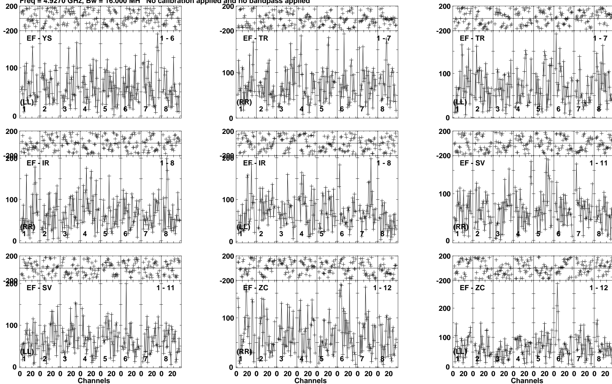
Lower frame: Micro Ampl Jy Top frame: Phas deg Vector averaged cross-power spectrum Baseline: EF (01) - YS (06) Timerange: 00/23:29:51 to 00/23:34:49
