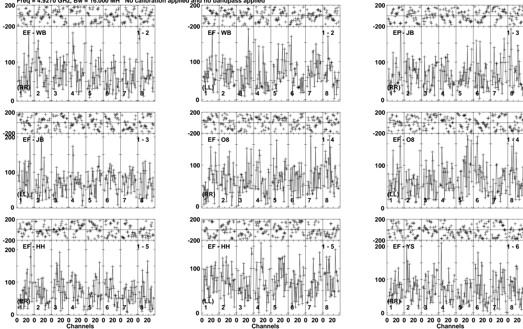
Lower frame: Micro Ampl Jy Top frame: Phas deg Vector averaged cross-power spectrum Baseline: EF (01) - WB (02) Timerange: 00/23:14:41 to 00/23:19:39
