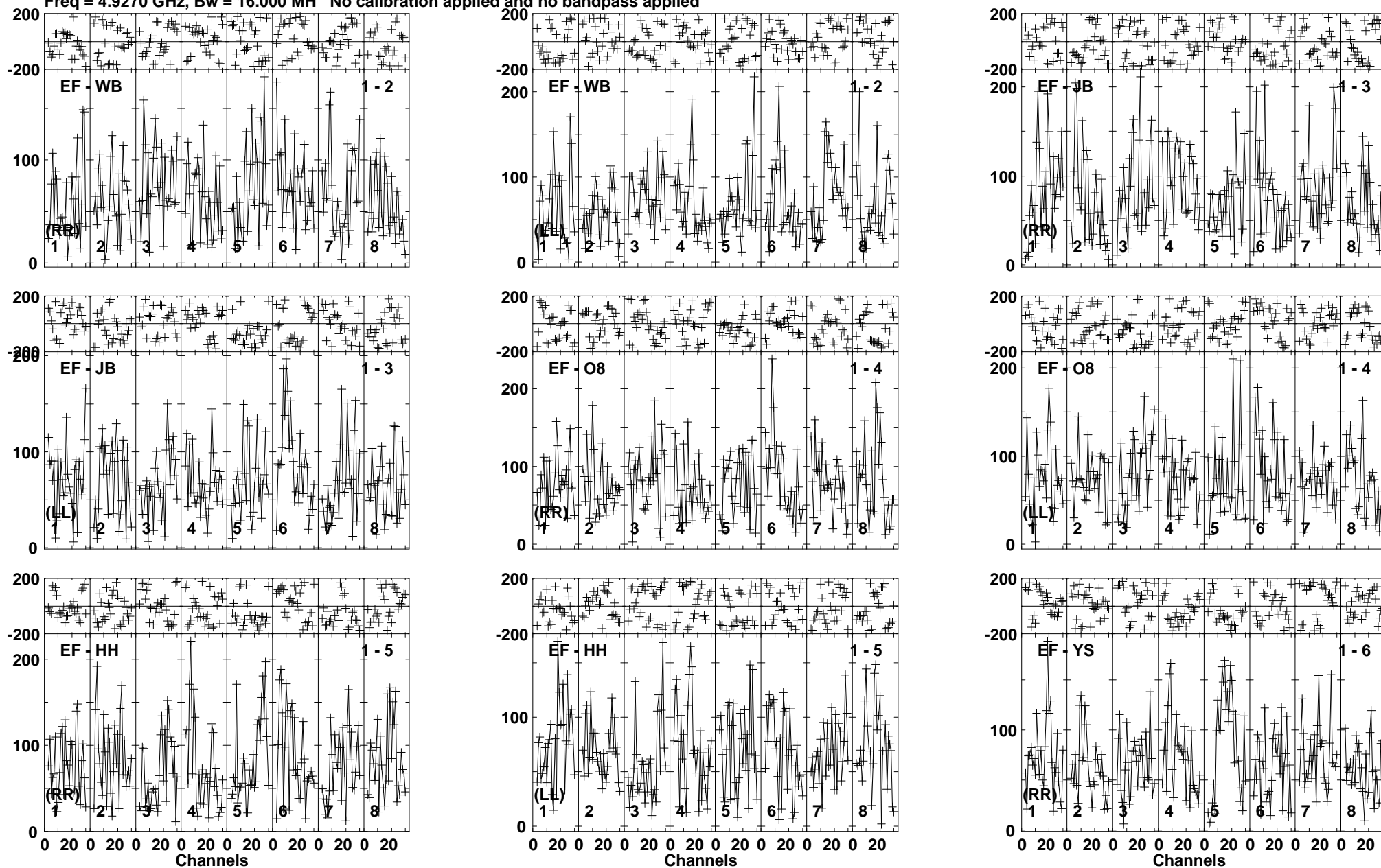
Lower frame: Micro Ampl Jy Top frame: Phas deg Vector averaged cross-power spectrum Baseline: EF (01) - WB (02) Timerange: 01/01:23:31 to 01/01:27:29
