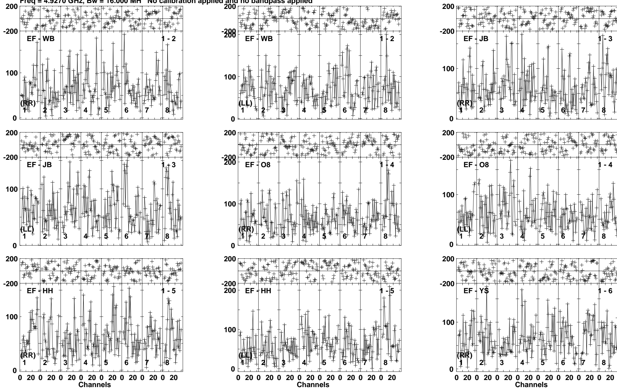
Lower frame: Micro Ampl Jy Top frame: Phas deg Vector averaged cross-power spectrum Baseline: EF (01) - WB (02) Timerange: 00/21:51:11 to 00/21:56:09
