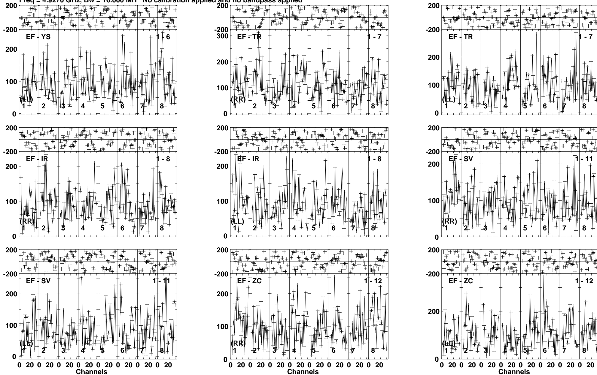
Lower frame: Micro Ampl Jy Top frame: Phas deg Vector averaged cross-power spectrum Baseline: EF (01) - YS (06) Timerange: 01/01:21:01 to 01/01:23:29
