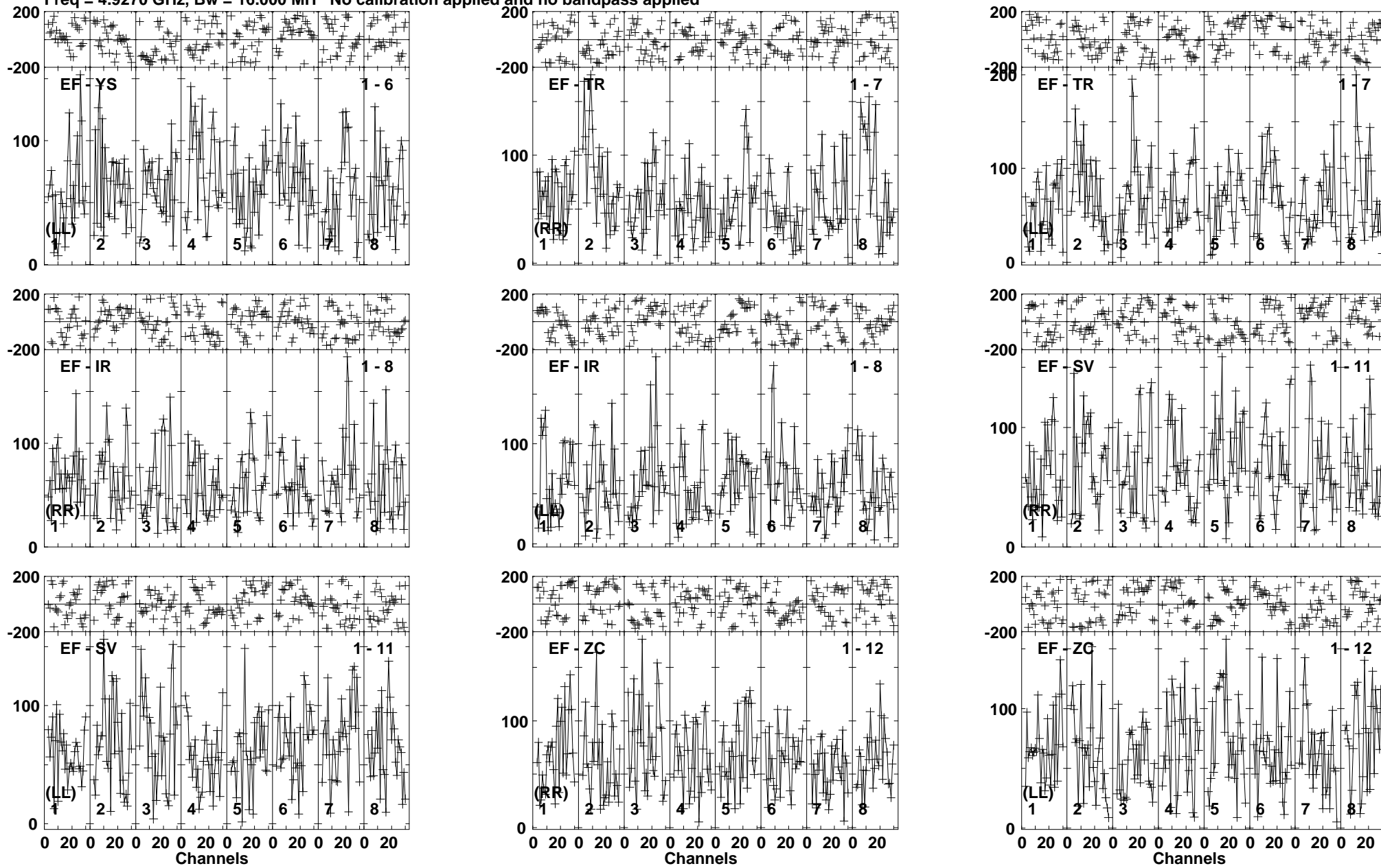
Lower frame: Micro Ampl Jy Top frame: Phas deg Vector averaged cross-power spectrum Baseline: EF (01) - YS (06) Timerange: 01/01:16:01 to 01/01:20:59
