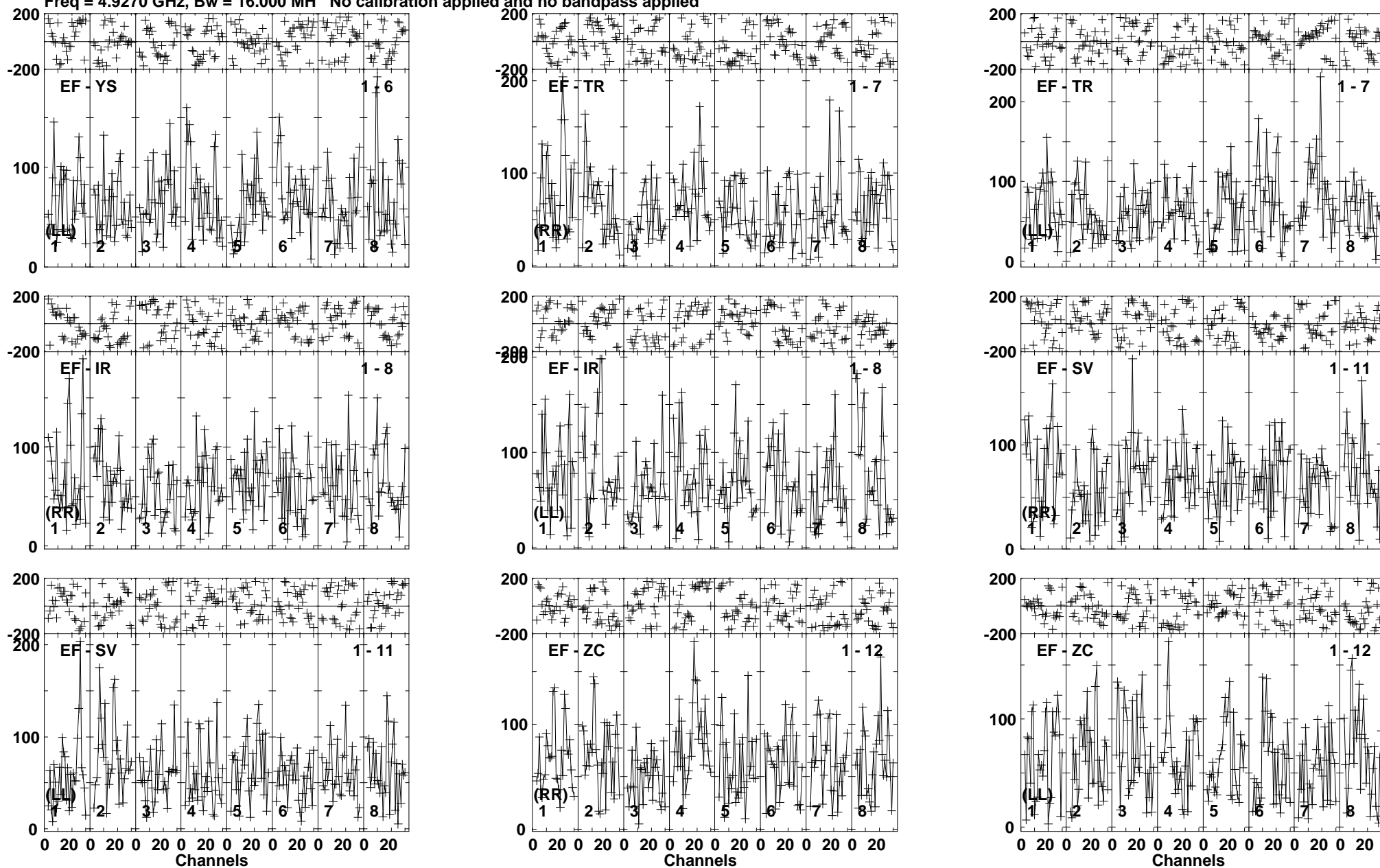
Lower frame: Micro Ampl Jy Top frame: Phas deg Vector averaged cross-power spectrum Baseline: EF (01) - YS (06) Timerange: 00/22:51:51 to 00/22:56:49
