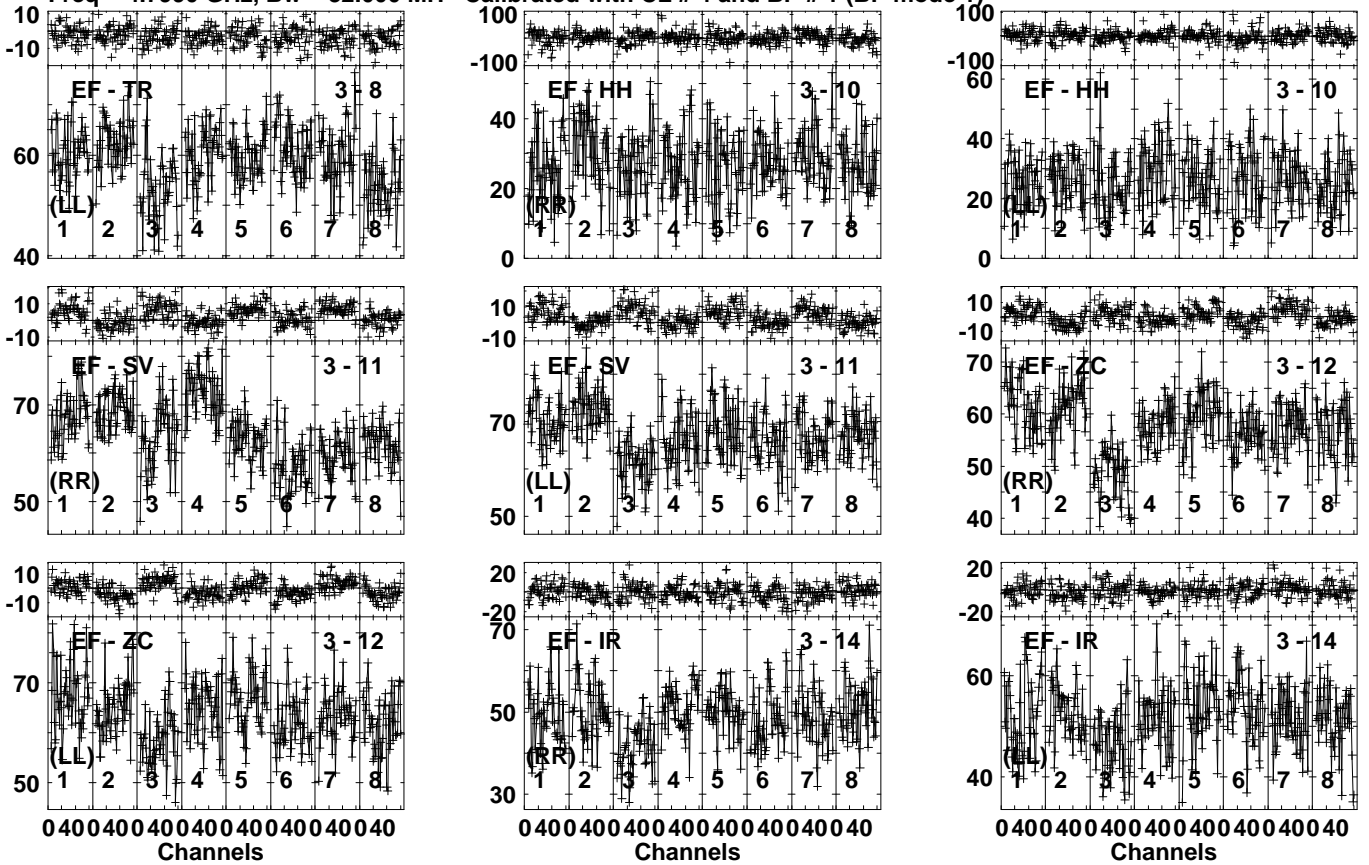
Lower frame: Milli Ampl Jy Top frame: Phas deg Vector averaged cross-power spectrum Several baselines displayed Timerange: 00/08:09:51 to 00/08:11:39
