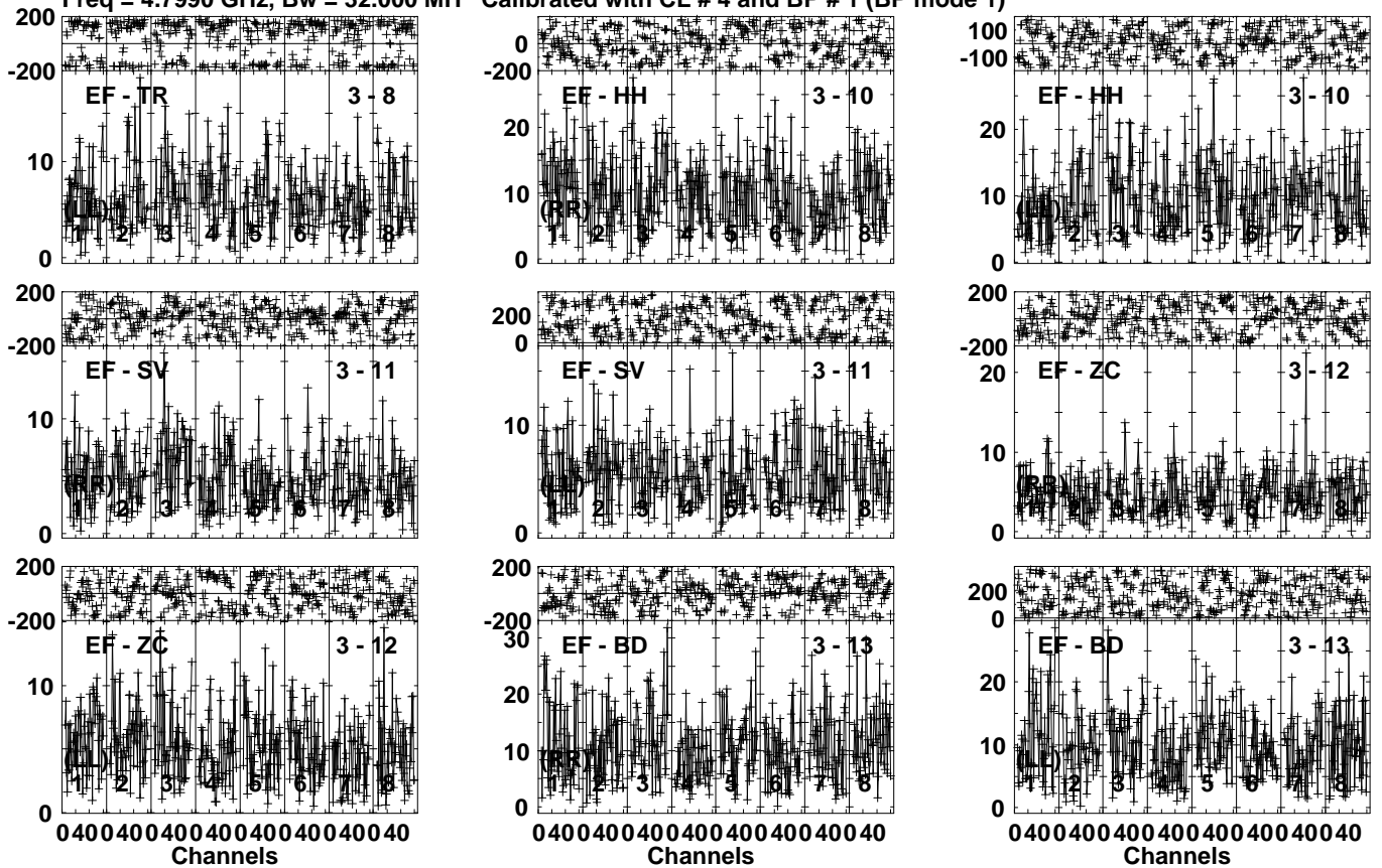
Lower frame: Milli Ampl Jy Top frame: Phas deg Vector averaged cross-power spectrum Several baselines displayed Timerange: 00/07:13:01 to 00/07:16:29
