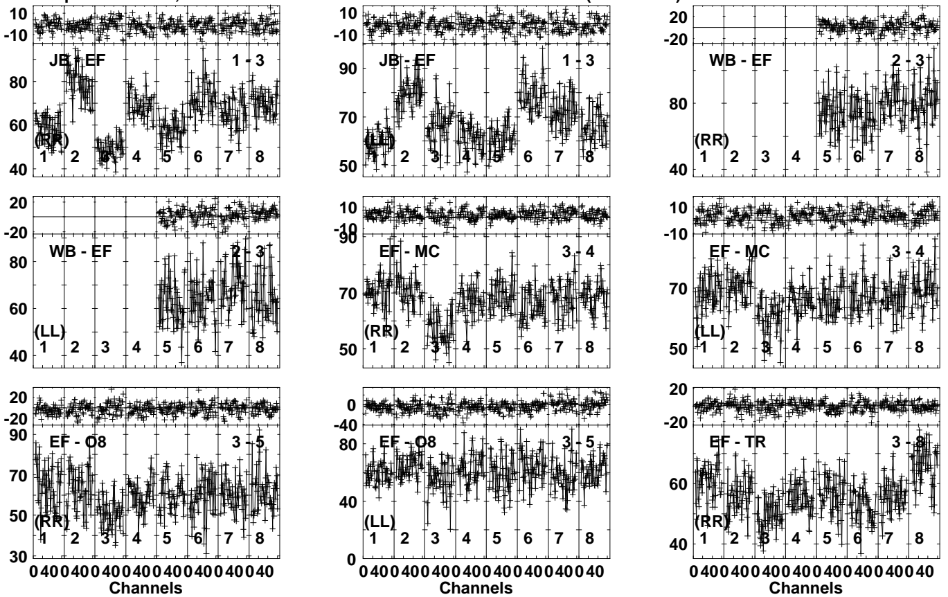
Lower frame: Milli Ampl Jy Top frame: Phas deg Vector averaged cross-power spectrum Several baselines displayed Timerange: 00/05:24:51 to 00/05:26:39
