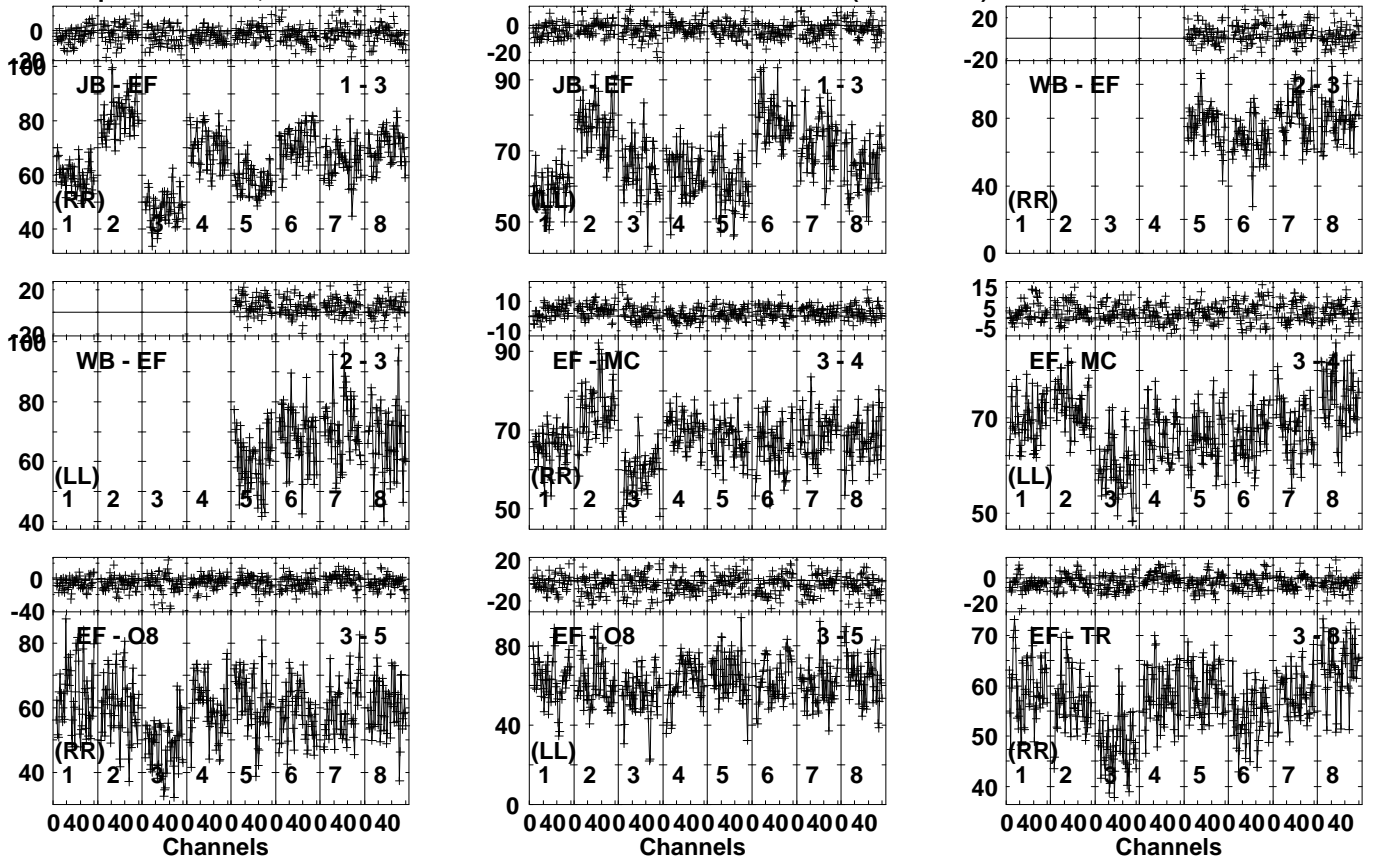
Lower frame: Milli Ampl Jy Top frame: Phas deg Vector averaged cross-power spectrum Several baselines displayed Timerange: 00/05:30:11 to 00/05:32:39
