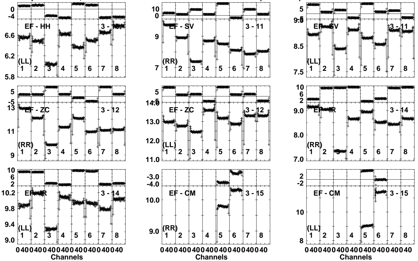
Lower frame: Ampl Jy Top frame: Phas deg Vector averaged cross-power spectrum Several baselines displayed Timerange: 00/11:54:01 to 00/11:59:59
