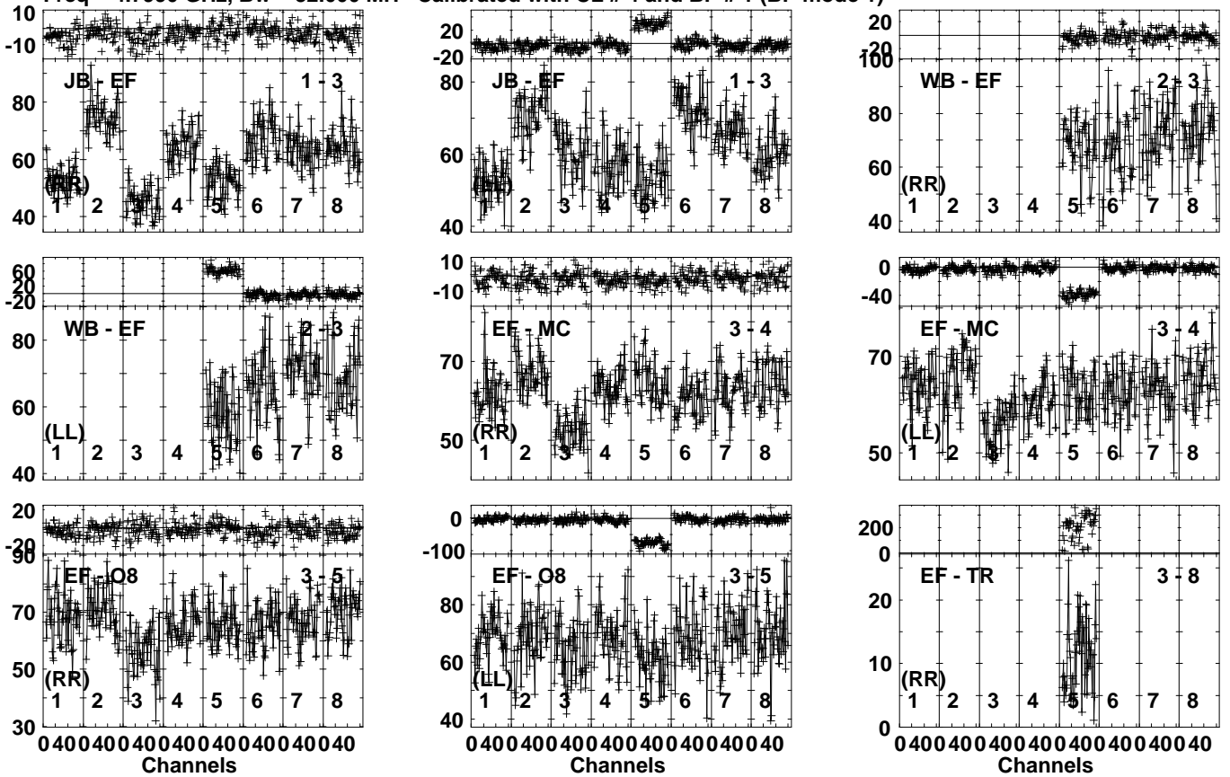
Lower frame: Milli Ampl Jy Top frame: Phas deg Vector averaged cross-power spectrum Several baselines displayed Timerange: 00/09:32:01 to 00/09:33:59
