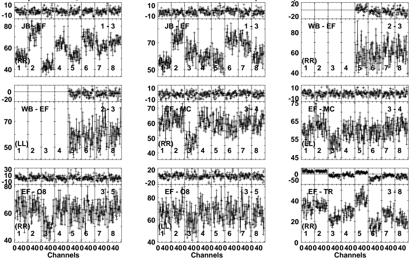
Lower frame: Milli Ampl Jy Top frame: Phas deg Vector averaged cross-power spectrum Several baselines displayed Timerange: 00/11:49:11 to 00/11:52:39
