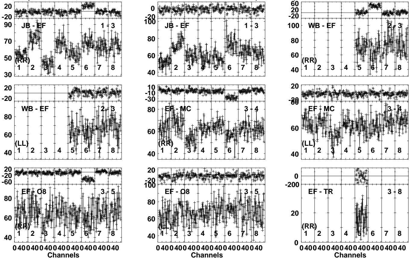
Lower frame: Milli Ampl Jy Top frame: Phas deg Vector averaged cross-power spectrum Several baselines displayed Timerange: 00/09:27:01 to 00/09:28:49
