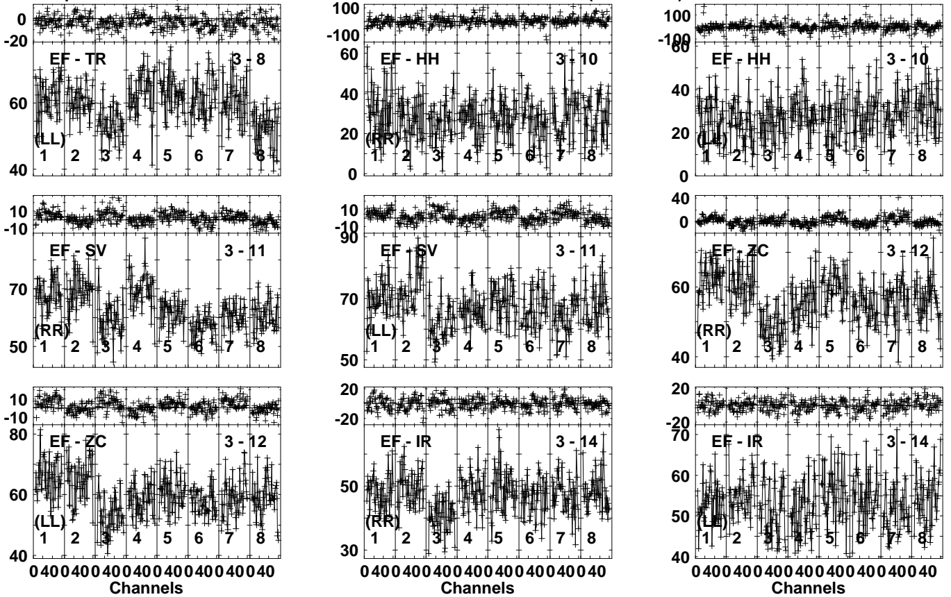
Lower frame: Milli Ampl Jy Top frame: Phas deg Vector averaged cross-power spectrum Several baselines displayed Timerange: 00/08:44:21 to 00/08:46:49
