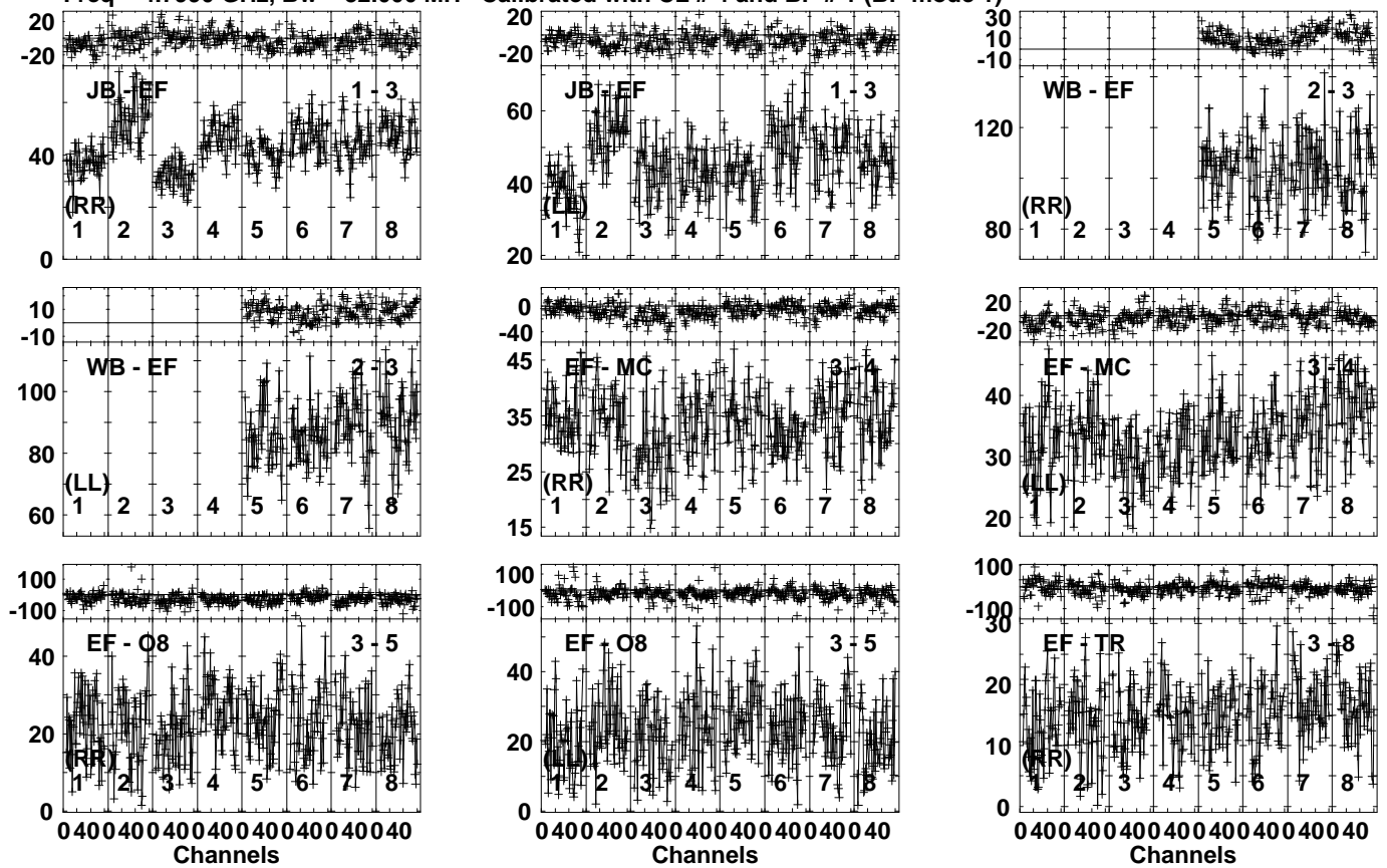
Lower frame: Milli Ampl Jy Top frame: Phas deg Vector averaged cross-power spectrum Several baselines displayed Timerange: 00/05:50:41 to 00/05:53:09
