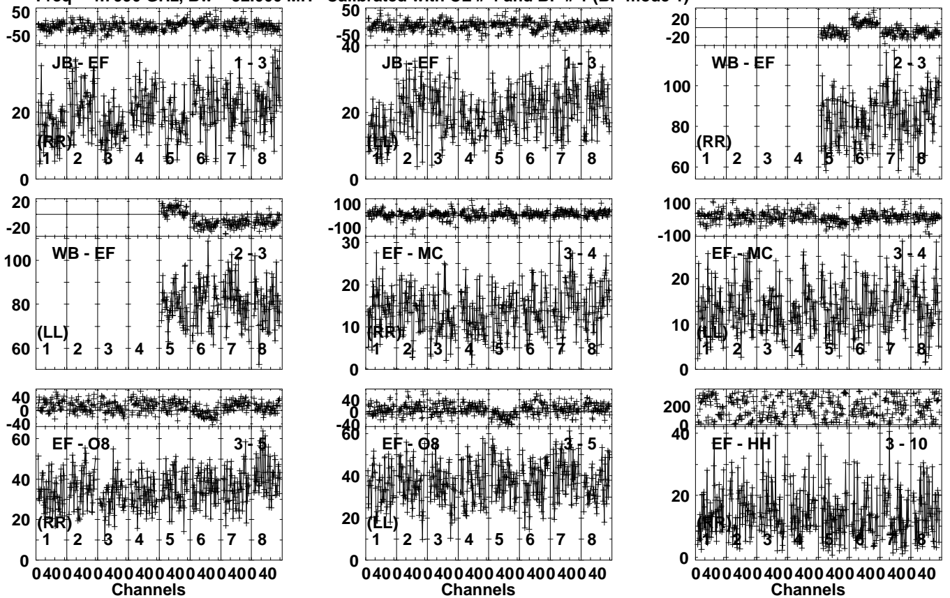
Lower frame: Milli Ampl Jy Top frame: Phas deg Vector averaged cross-power spectrum Several baselines displayed Timerange: 00/09:28:51 to 00/09:31:19
