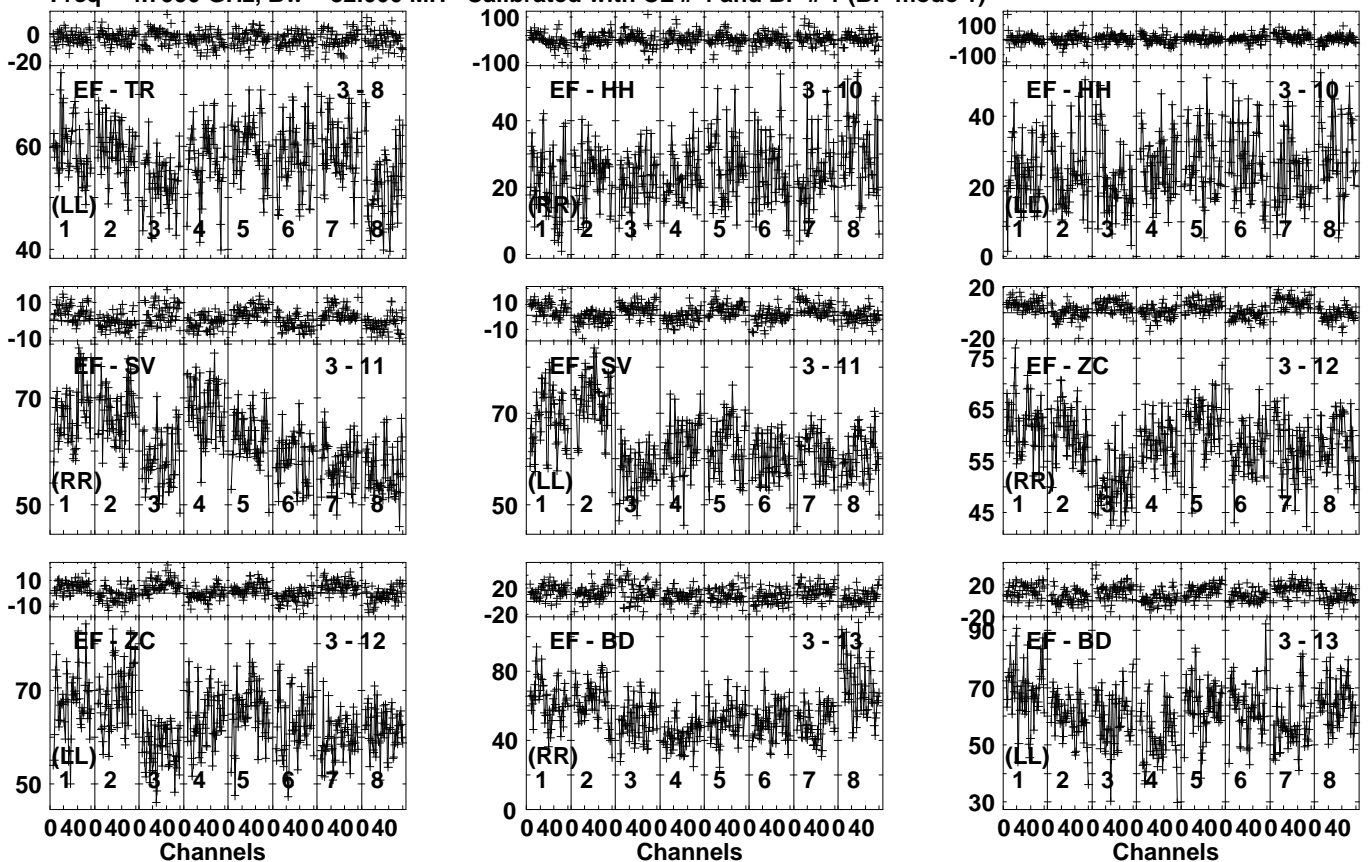
Lower frame: Milli Ampl Jy Top frame: Phas deg Vector averaged cross-power spectrum Several baselines displayed Timerange: 00/06:35:21 to 00/06:37:49
