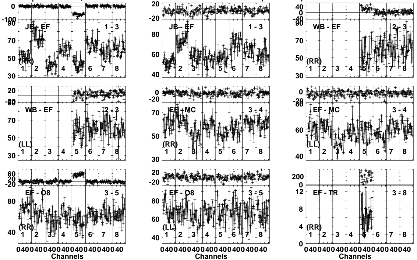
Lower frame: Milli Ampl Jy Top frame: Phas deg Vector averaged cross-power spectrum Several baselines displayed Timerange: 00/10:50:11 to 00/10:52:09
