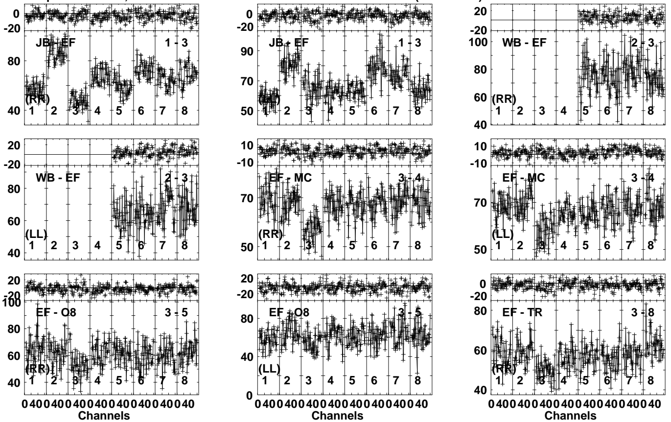
Lower frame: Milli Ampl Jy Top frame: Phas deg Vector averaged cross-power spectrum Several baselines displayed Timerange: 00/05:18:11 to 00/05:20:39
