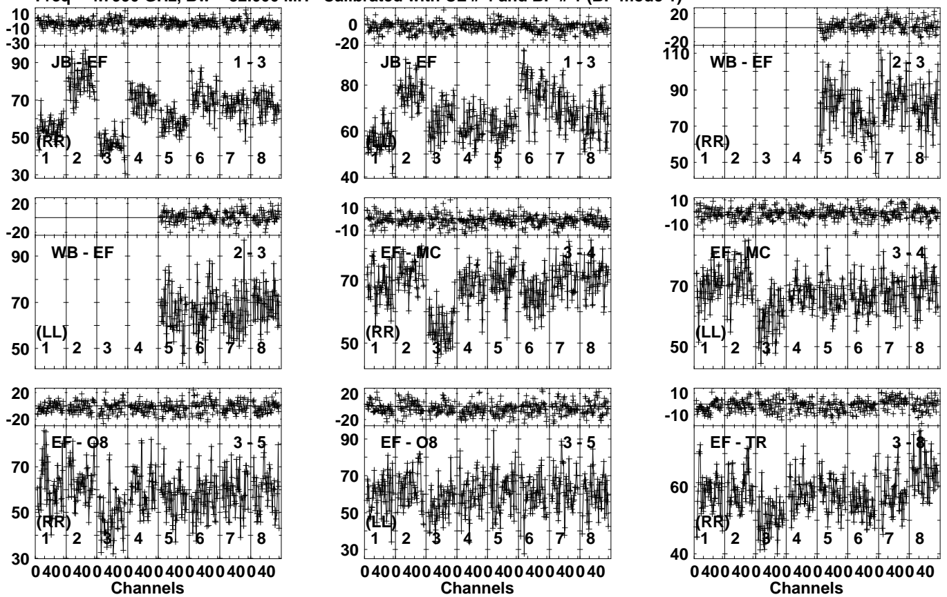
Lower frame: Milli Ampl Jy Top frame: Phas deg Vector averaged cross-power spectrum Several baselines displayed Timerange: 00/06:42:01 to 00/06:43:49
