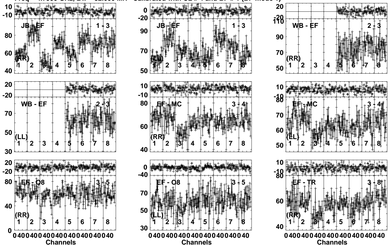
Lower frame: Milli Ampl Jy Top frame: Phas deg Vector averaged cross-power spectrum Several baselines displayed Timerange: 00/04:55:41 to 00/04:57:29
