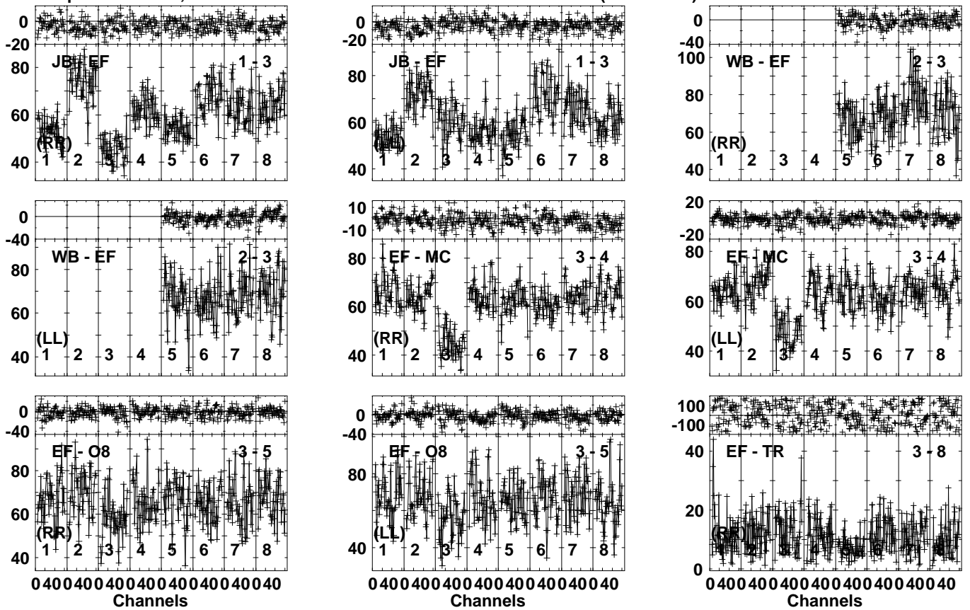
Lower frame: Milli Ampl Jy Top frame: Phas deg Vector averaged cross-power spectrum Several baselines displayed Timerange: 00/09:15:01 to 00/09:16:49
