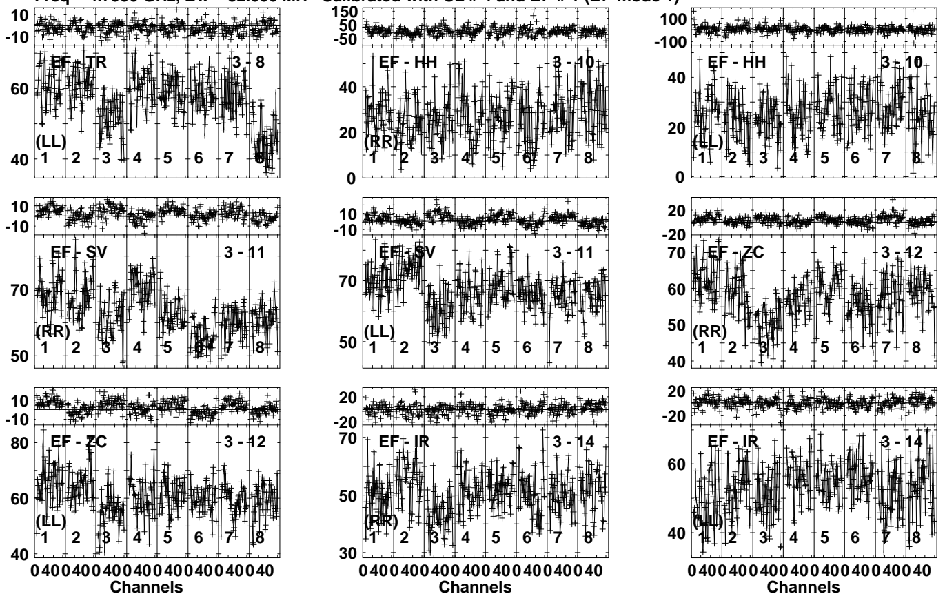
Lower frame: Milli Ampl Jy Top frame: Phas deg Vector averaged cross-power spectrum Several baselines displayed Timerange: 00/07:16:31 to 00/07:18:59
