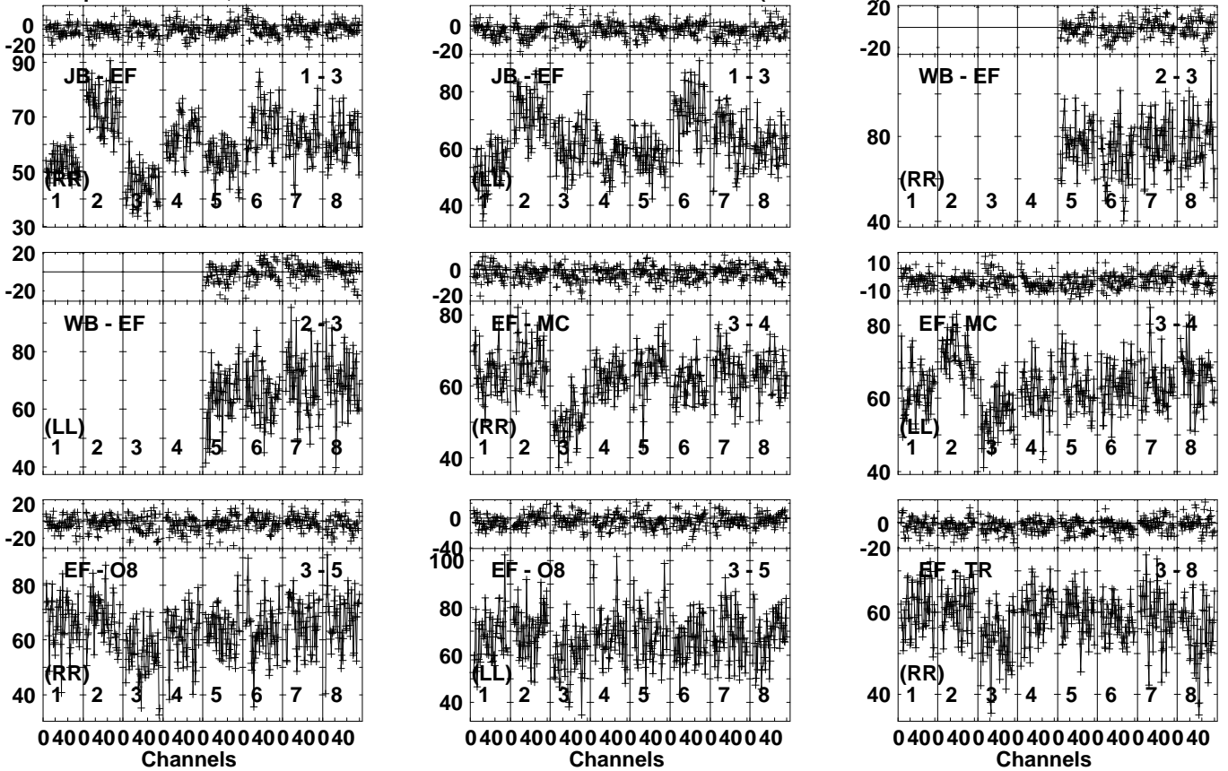
Lower frame: Milli Ampl Jy Top frame: Phas deg Vector averaged cross-power spectrum Several baselines displayed Timerange: 00/08:33:51 to 00/08:35:39
