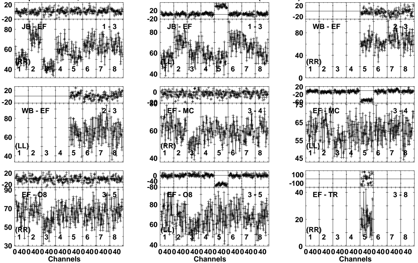
Lower frame: Milli Ampl Jy Top frame: Phas deg Vector averaged cross-power spectrum Several baselines displayed Timerange: 00/11:02:21 to 00/11:04:19
