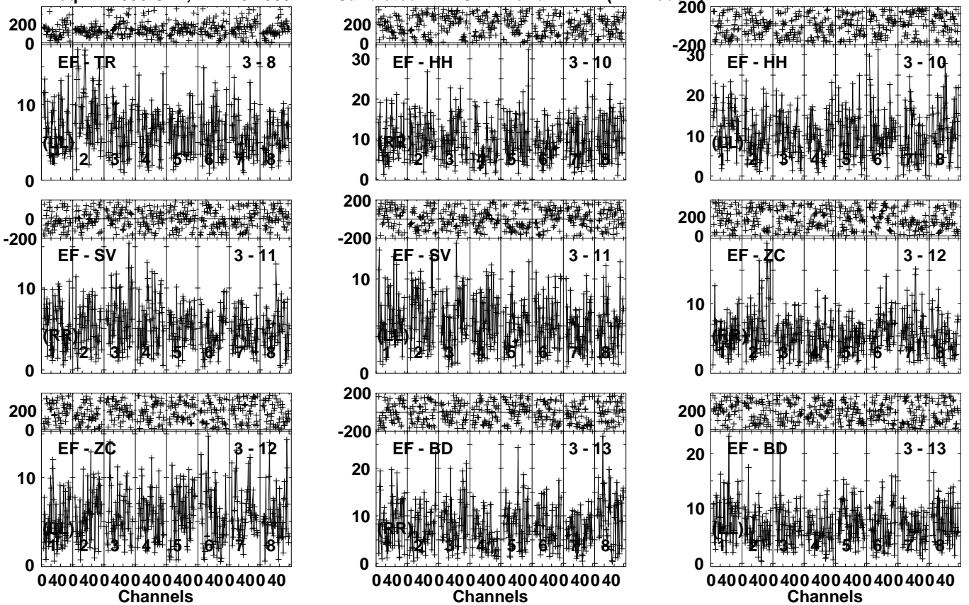
Lower frame: Milli Ampl Jy Top frame: Phas deg Vector averaged cross-power spectrum Several baselines displayed Timerange: 00/04:21:31 to 00/04:24:59
