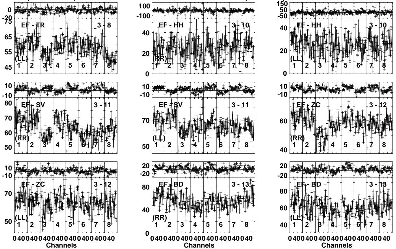
Lower frame: Milli Ampl Jy Top frame: Phas deg Vector averaged cross-power spectrum Several baselines displayed Timerange: 00/06:47:01 to 00/06:48:59
