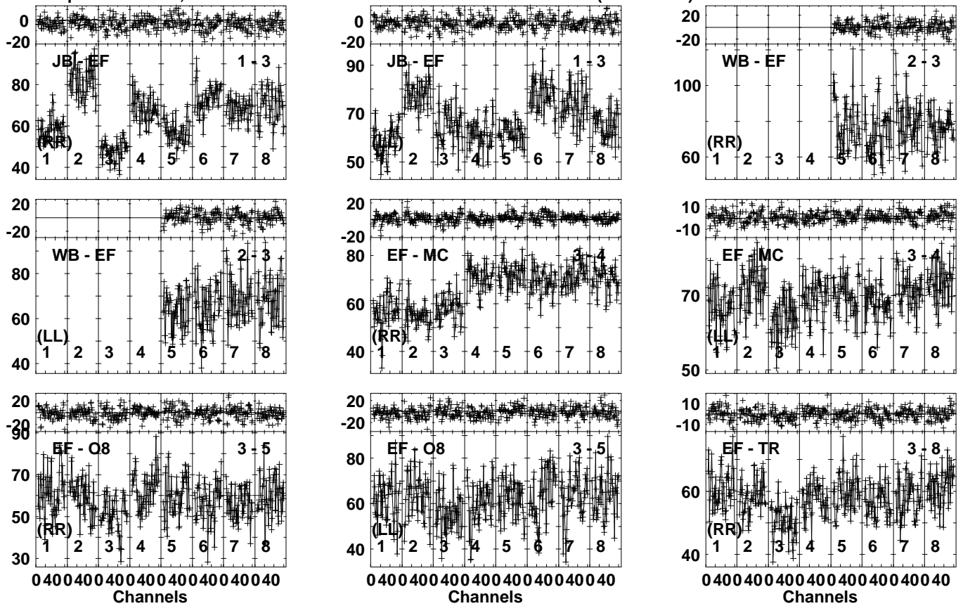
Lower frame: Milli Ampl Jy Top frame: Phas deg Vector averaged cross-power spectrum Several baselines displayed Timerange: 00/06:11:21 to 00/06:13:49
