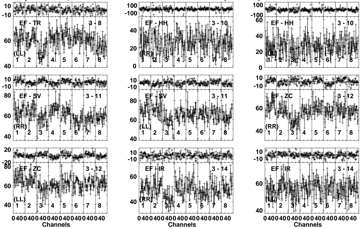
Lower frame: Milli Ampl Jy Top frame: Phas deg Vector averaged cross-power spectrum Several baselines displayed Timerange: 00/09:03:01 to 00/09:04:49
