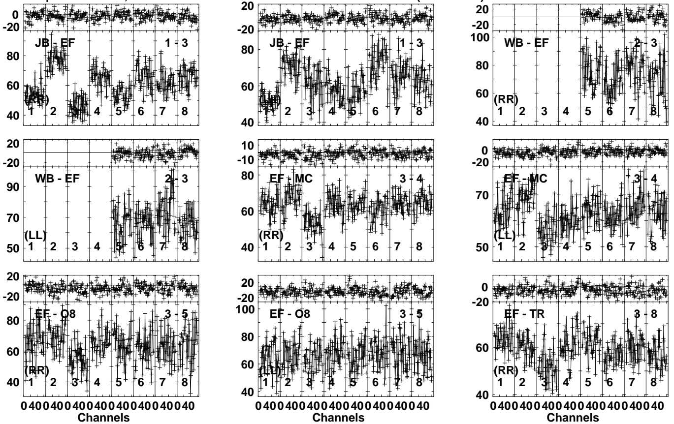
Lower frame: Milli Ampl Jy Top frame: Phas deg Vector averaged cross-power spectrum Several baselines displayed Timerange: 00/08:51:01 to 00/08:52:49
