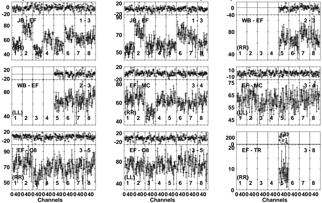
Lower frame: Milli Ampl Jy Top frame: Phas deg Vector averaged cross-power spectrum Several baselines displayed Timerange: 00/10:14:01 to 00/10:16:29
