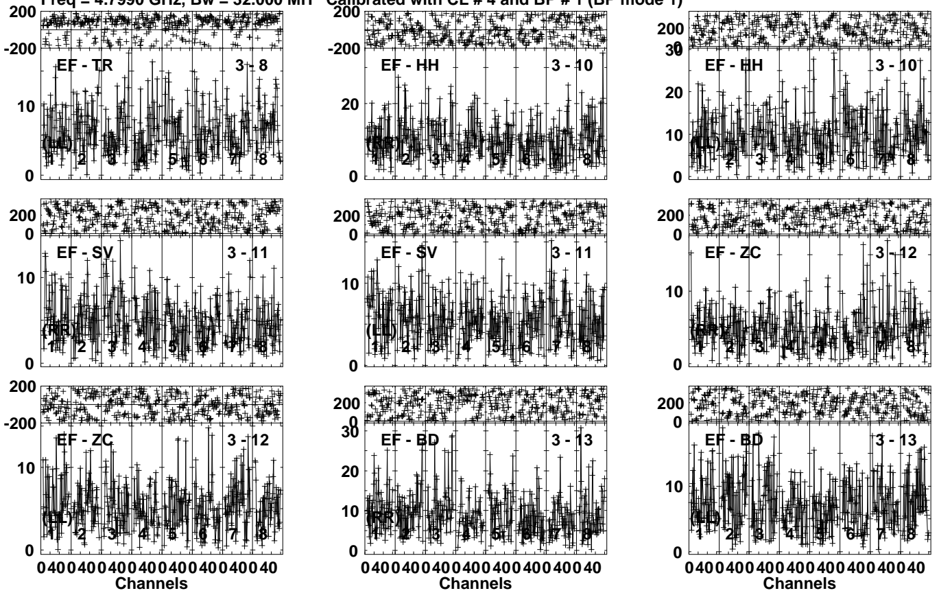
Lower frame: Milli Ampl Jy Top frame: Phas deg Vector averaged cross-power spectrum Several baselines displayed Timerange: 00/05:32:41 to 00/05:36:09
