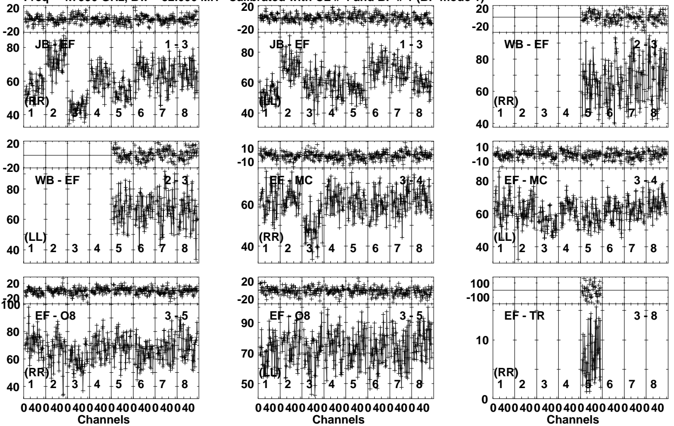
Lower frame: Milli Ampl Jy Top frame: Phas deg Vector averaged cross-power spectrum Several baselines displayed Timerange: 00/10/31:21 to 00/10/33:49
