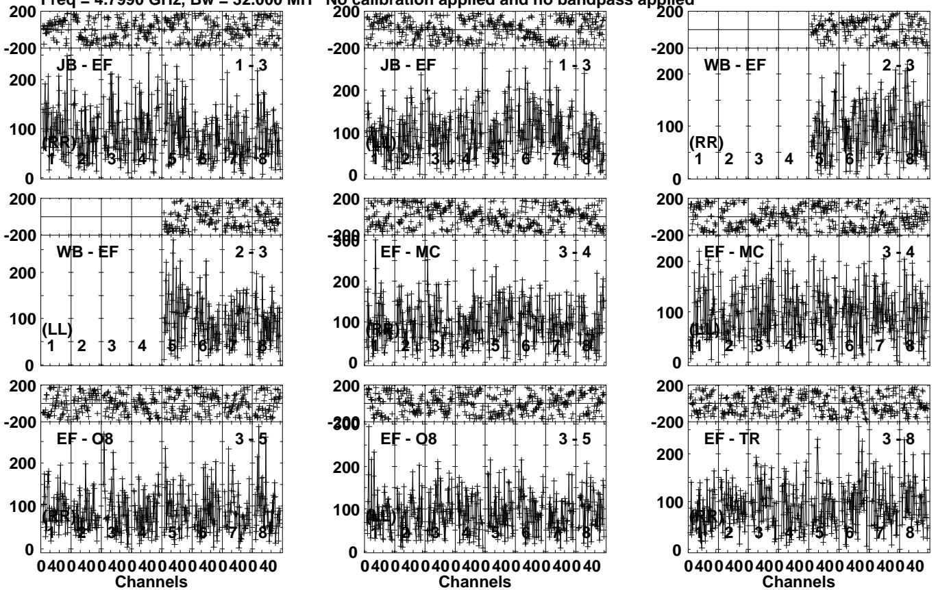
Lower frame: Micro Ampl Jy Top frame: Phas deg Vector averaged cross-power spectrum Several baselines displayed Timerange: 00/10:10:31 to 00/10:13:59
