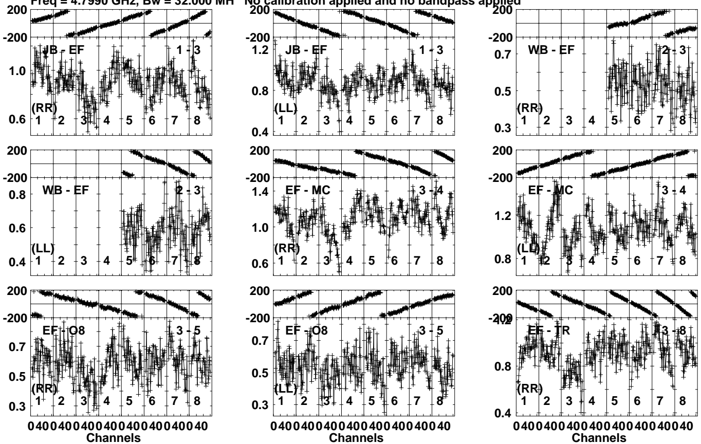
Lower frame: Milli Ampl Jy Top frame: Phas deg Vector averaged cross-power spectrum Several baselines displayed Timerange: 00/06:59:11 to 00/07:00:59
