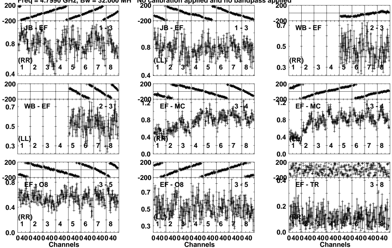
Lower frame: Milli Ampl Jy Top frame: Phas deg Vector averaged cross-power spectrum Several baselines displayed Timerange: 00/11:25:11 to 00/11:27:39
