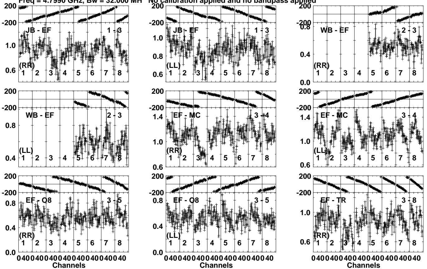
Lower frame: Milli Ampl Jy Top frame: Phas deg Vector averaged cross-power spectrum Several baselines displayed Timerange: 00/05:48:51 to 00/05:50:39
