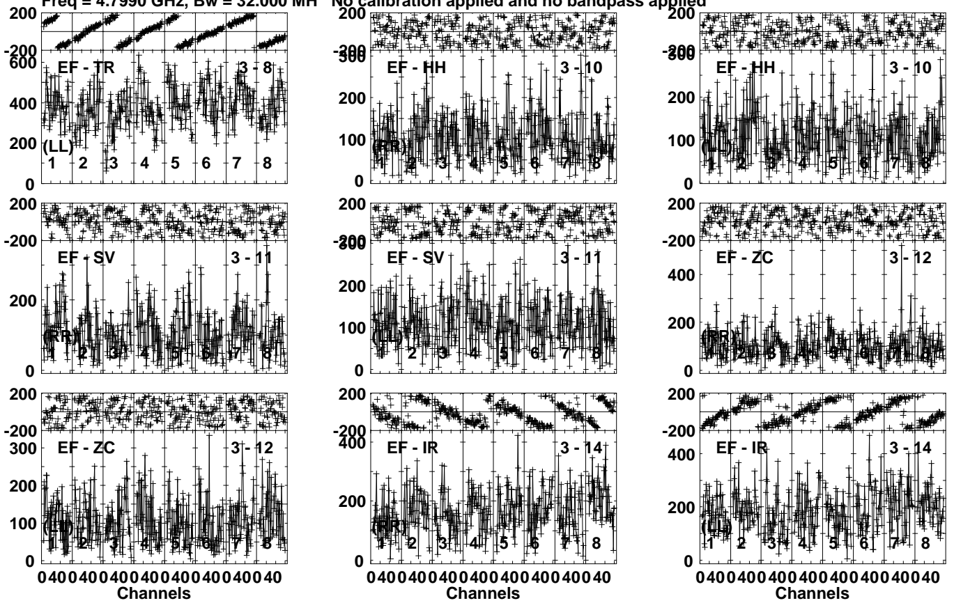
Lower frame: Micro Ampl Jy Top frame: Phas deg Vector averaged cross-power spectrum Several baselines displayed Timerange: 00/08:35:41 to 00/08:38:09
