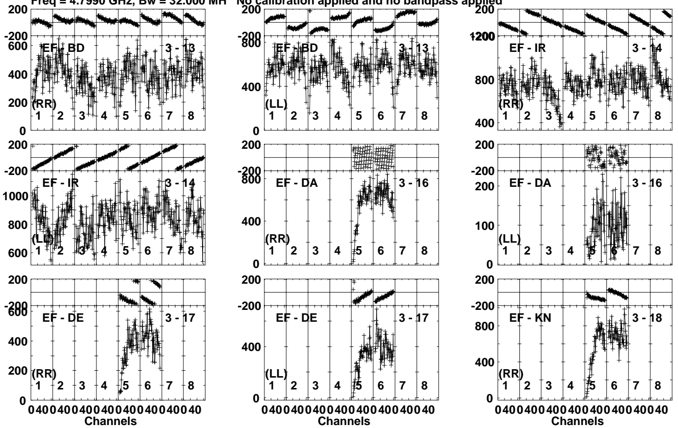
Lower frame: Micro Ampl Jy Top frame: Phas deg Vector averaged cross-power spectrum Several baselines displayed Timerange: 00/04:49:01 to 00/04:51:29
