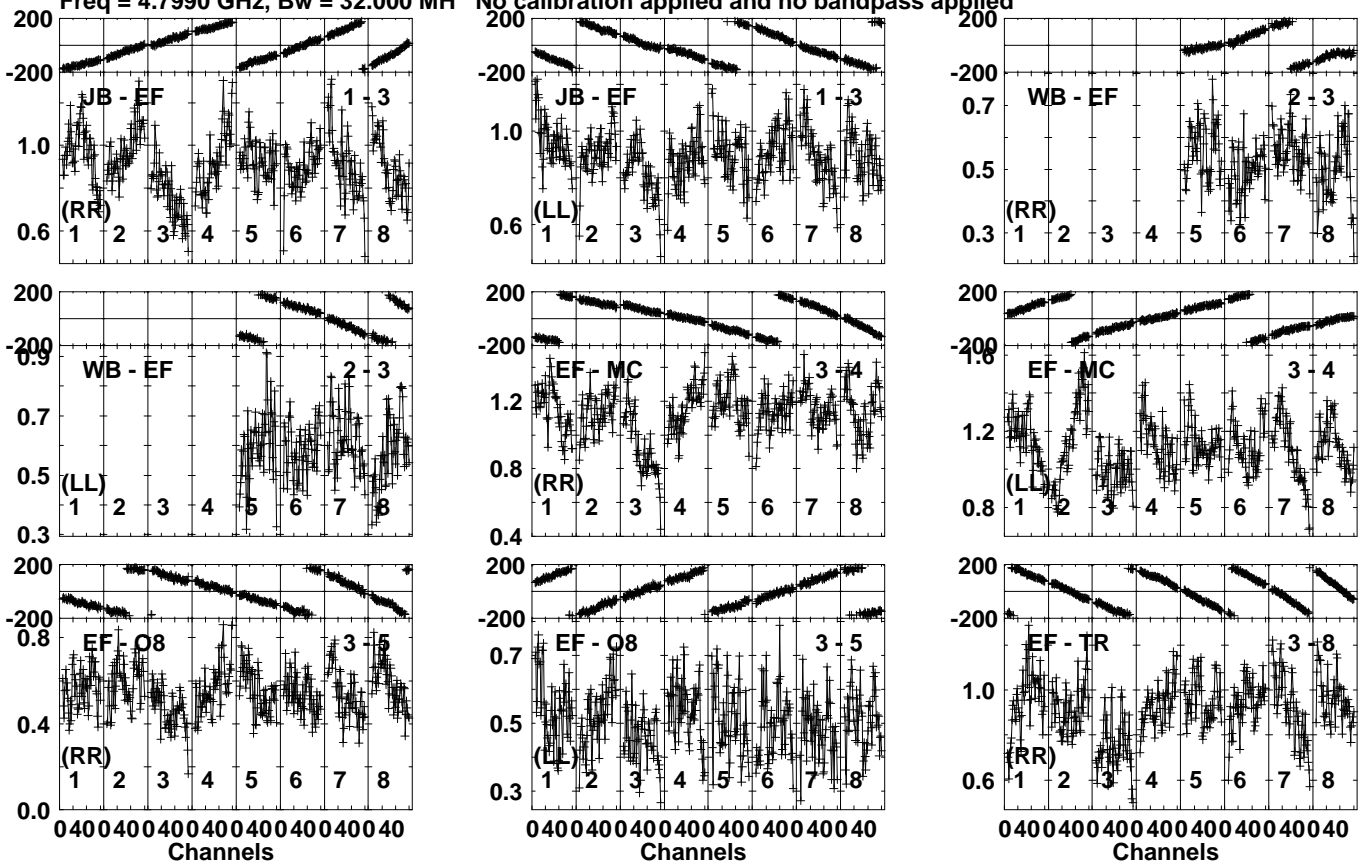
Lower frame: Milli Ampl Jy Top frame: Phas deg Vector averaged cross-power spectrum Several baselines displayed Timerange: 00/06:23:21 to 00/06:25:49
