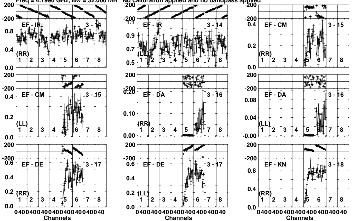
Lower frame: Milli Ampl Jy Top frame: Phas deg Vector averaged cross-power spectrum Several baselines displayed Timerange: 00/07:04:31 to 00/07:06:59
