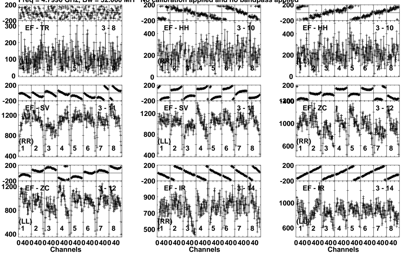
Lower frame: Micro Ampl Jy Top frame: Phas deg Vector averaged cross-power spectrum Several baselines displayed Timerange: 00/09:49:41 to 00/09:52:09
