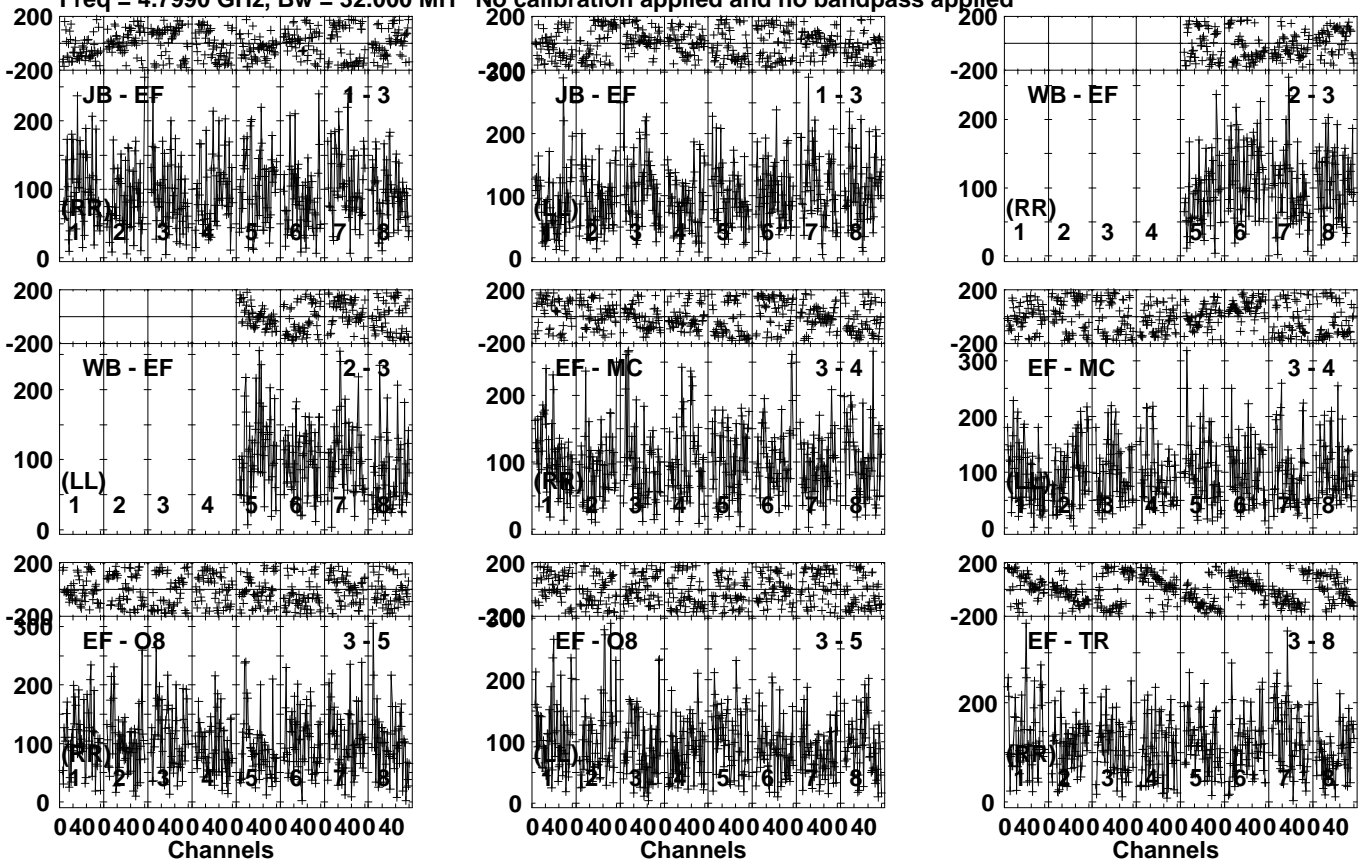
Lower frame: Micro Ampl Jy Top frame: Phas deg Vector averaged cross-power spectrum Several baselines displayed Timerange: 00/07:47:41 to 00/07:51:09
