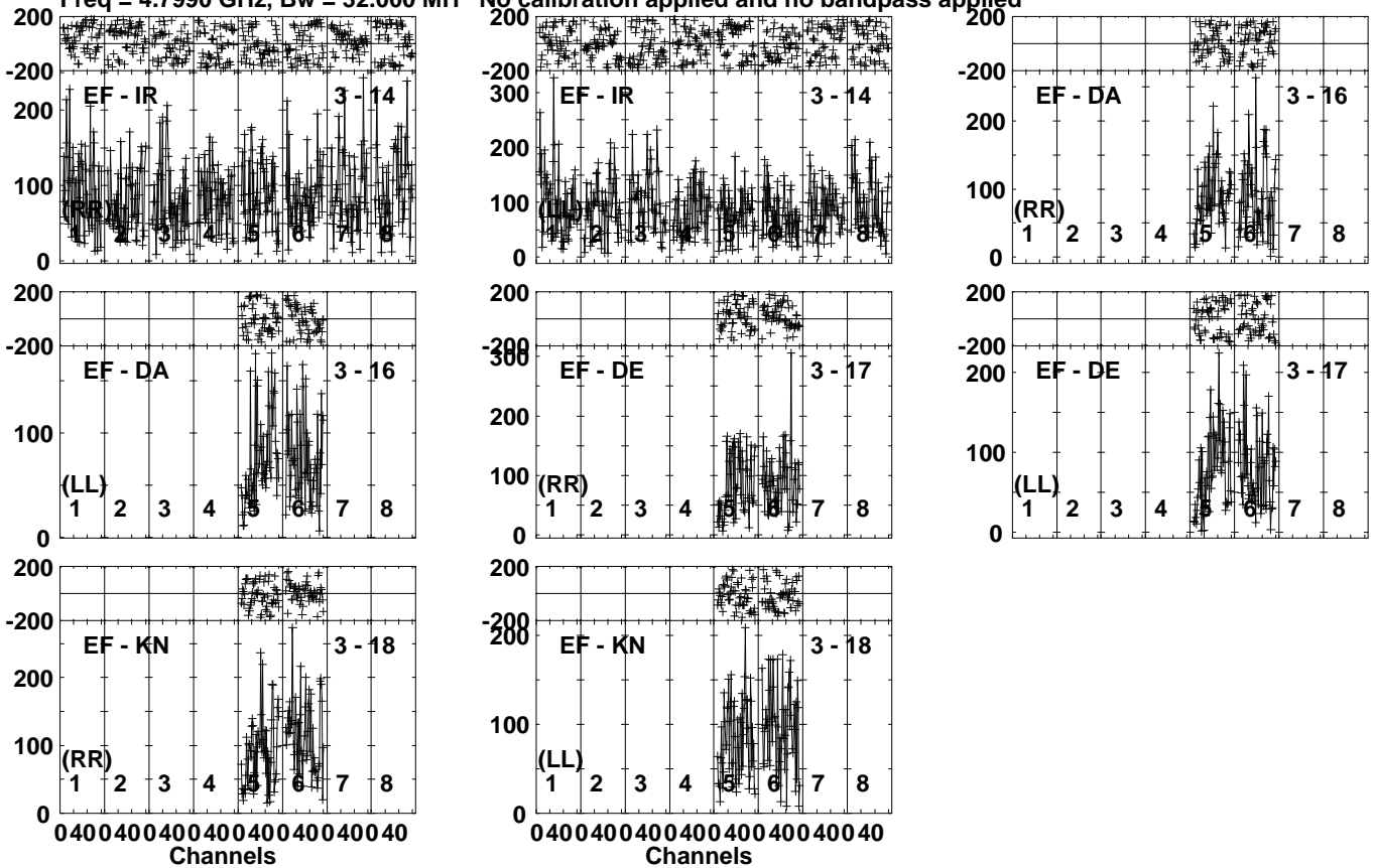
Lower frame: Micro Ampl Jy Top frame: Phas deg Vector averaged cross-power spectrum Several baselines displayed Timerange: 00/05:32:41 to 00/05:36:09
