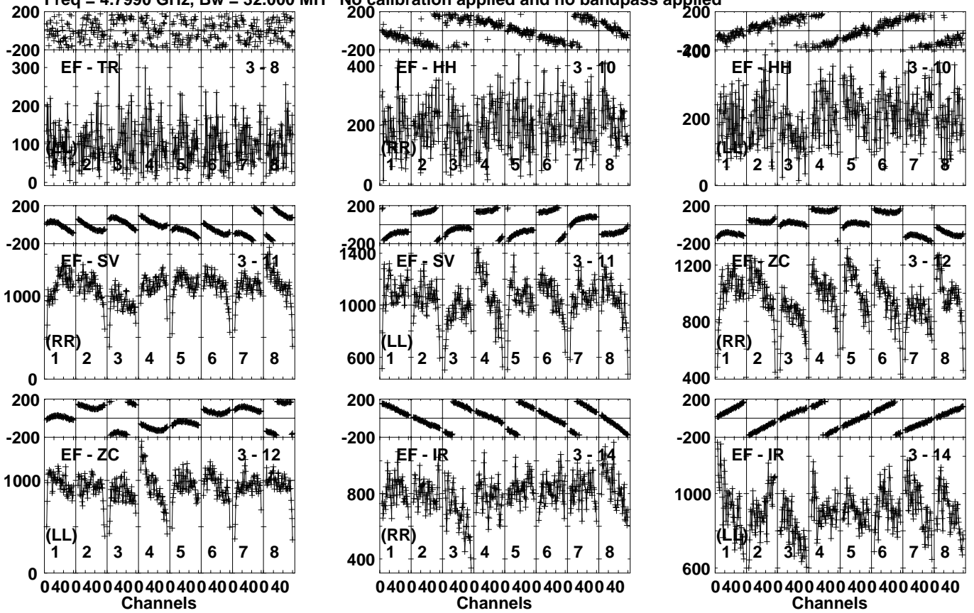
Lower frame: Micro Ampl Jy Top frame: Phas deg Vector averaged cross-power spectrum Several baselines displayed Timerange: 00/10:25:51 to 00/10:27:49
