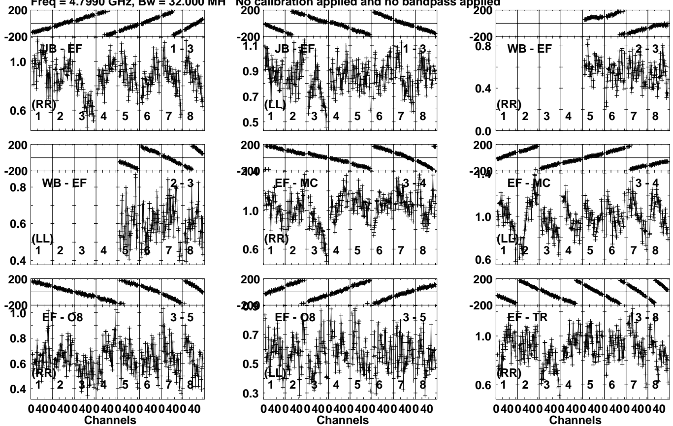
Lower frame: Milli Ampl Jy Top frame: Phas deg Vector averaged cross-power spectrum Several baselines displayed Timerange: 00/08:03:11 to 00/08:05:39
