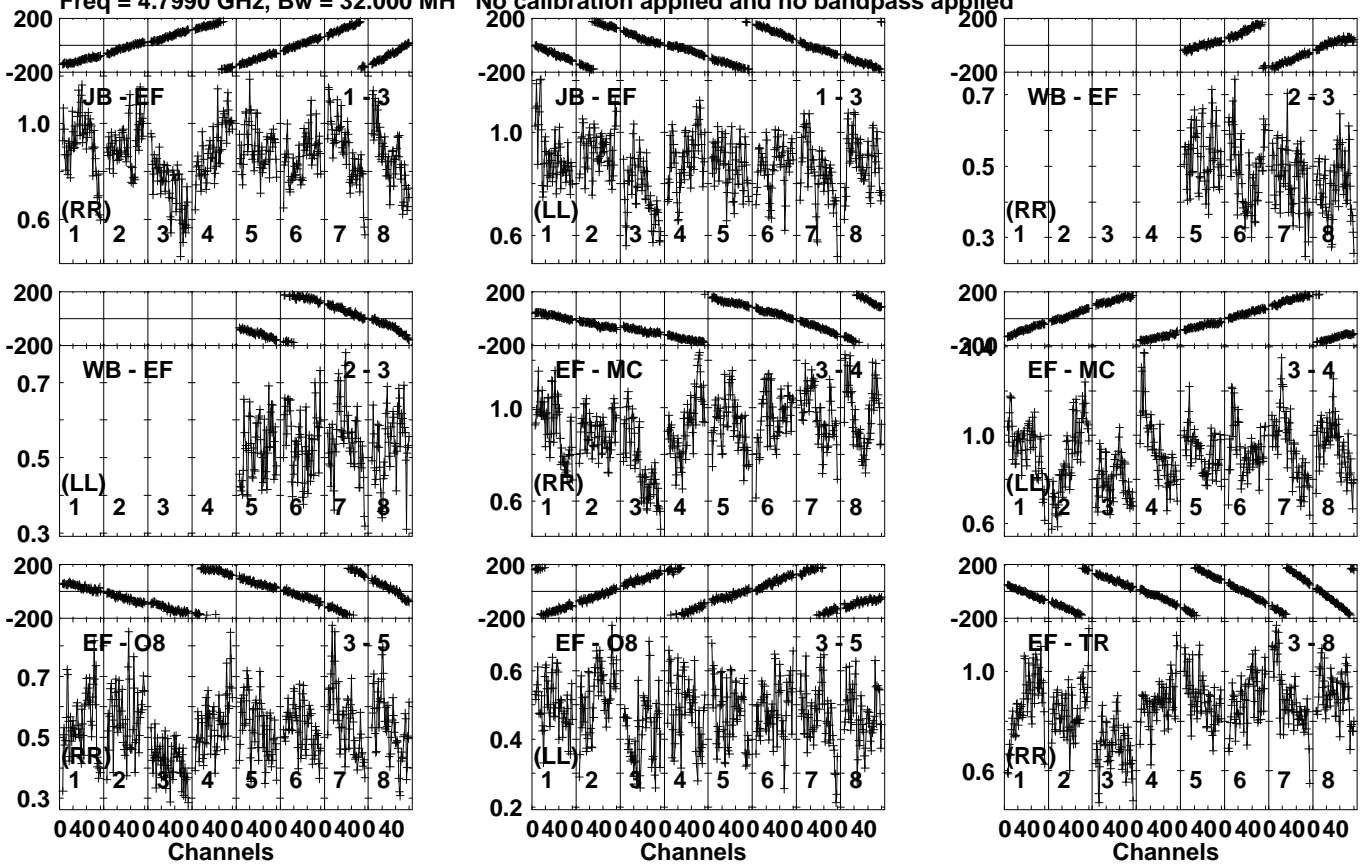
Lower frame: Milli Ampl Jy Top frame: Phas deg Vector averaged cross-power spectrum Several baselines displayed Timerange: 00/04:13:01 to 00/04:15:29
