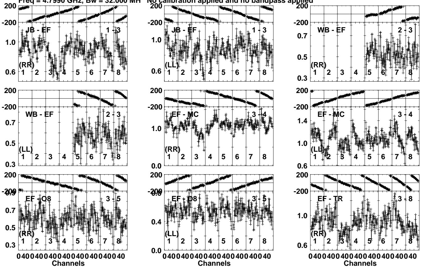
Lower frame: Milli Ampl Jy Top frame: Phas deg Vector averaged cross-power spectrum Several baselines displayed Timerange: 00/07:11:11 to 00/07:12:59
