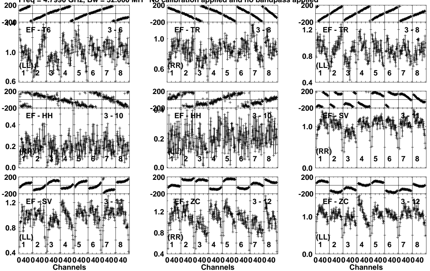
Lower frame: Milli Ampl Jy Top frame: Phas deg Vector averaged cross-power spectrum Several baselines displayed Timerange: 00/04:43:41 to 00/04:45:29
