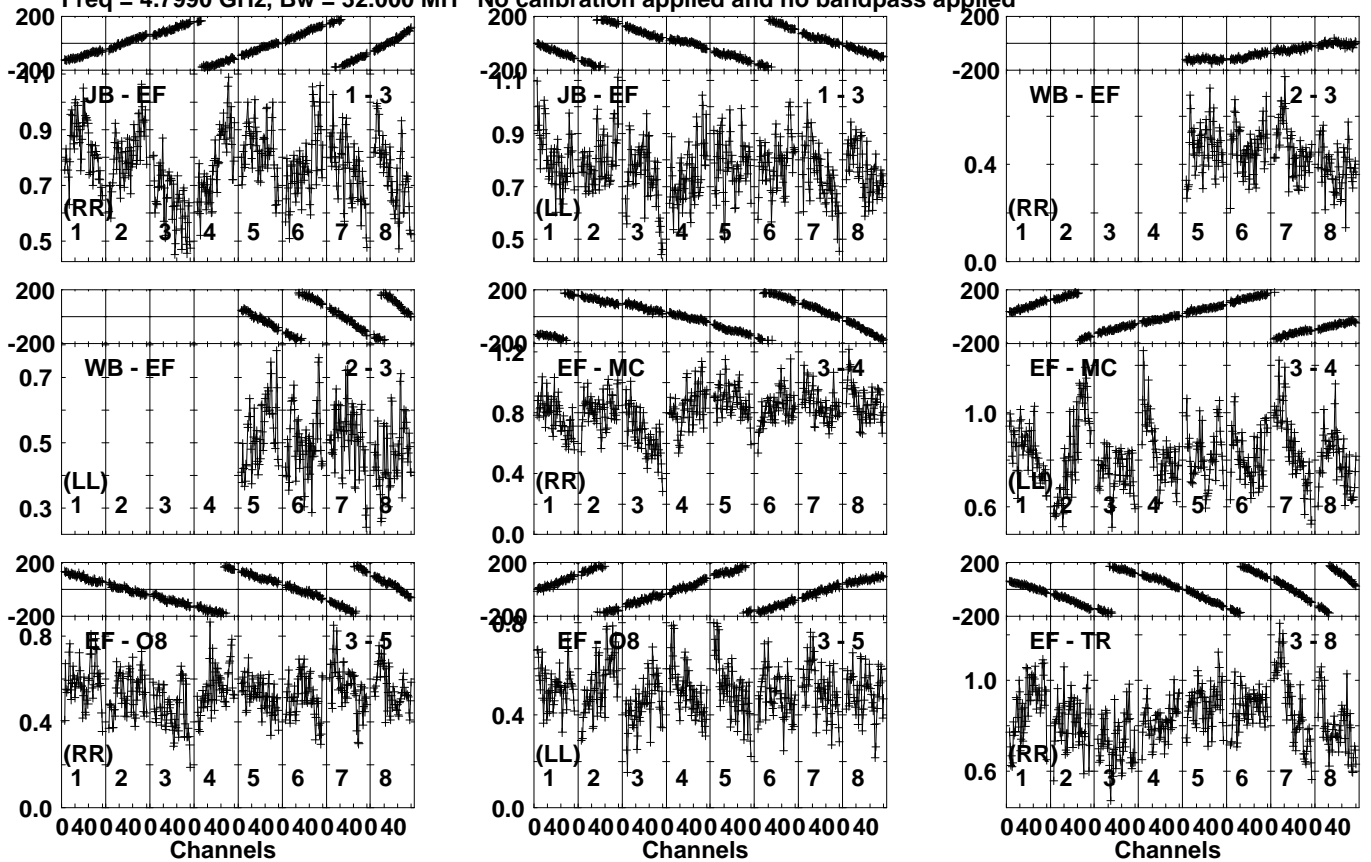
Lower frame: Milli Ampl Jy Top frame: Phas deg Vector averaged cross-power spectrum Several baselines displayed Timerange: 00/11:37:21 to 00/11:39:49
