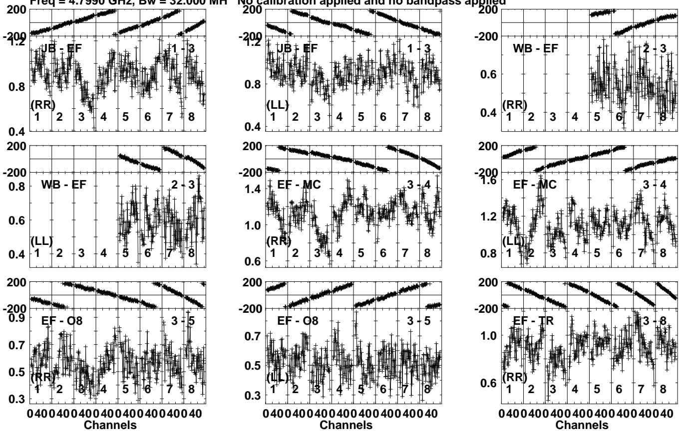
Lower frame: Milli Ampl Jy Top frame: Phas deg Vector averaged cross-power spectrum Several baselines displayed Timerange: 00/06:30:01 to 00/06:31:49
