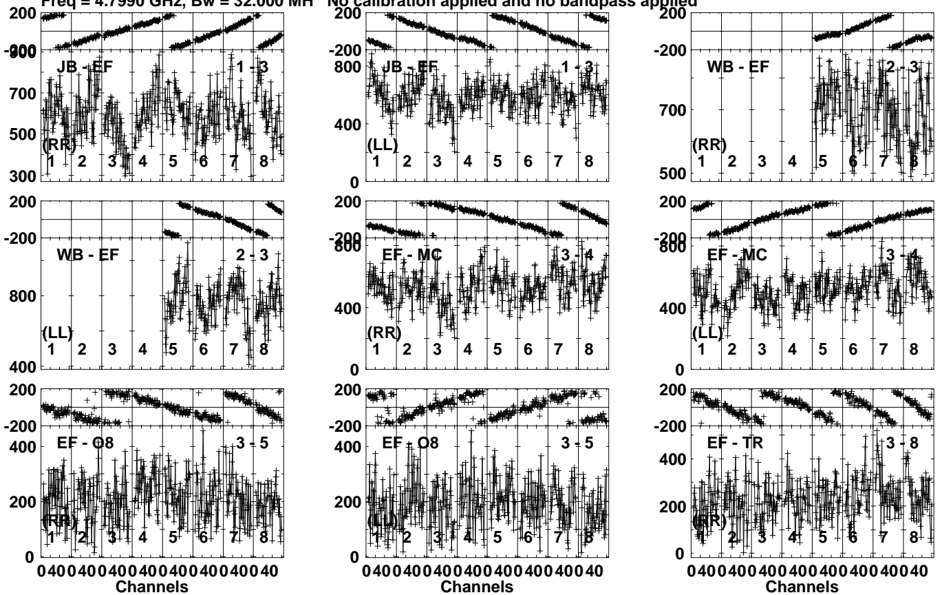
Lower frame: Micro Ampl Jy Top frame: Phas deg Vector averaged cross-power spectrum Several baselines displayed Timerange: 00/05:50:41 to 00/05:53:09
