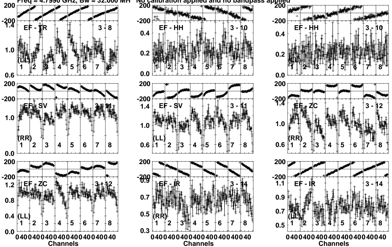
Lower frame: Milli Ampl Jy Top frame: Phas deg Vector averaged cross-power spectrum Several baselines displayed Timerange: 00/08:15:11 to 00/08:17:39
