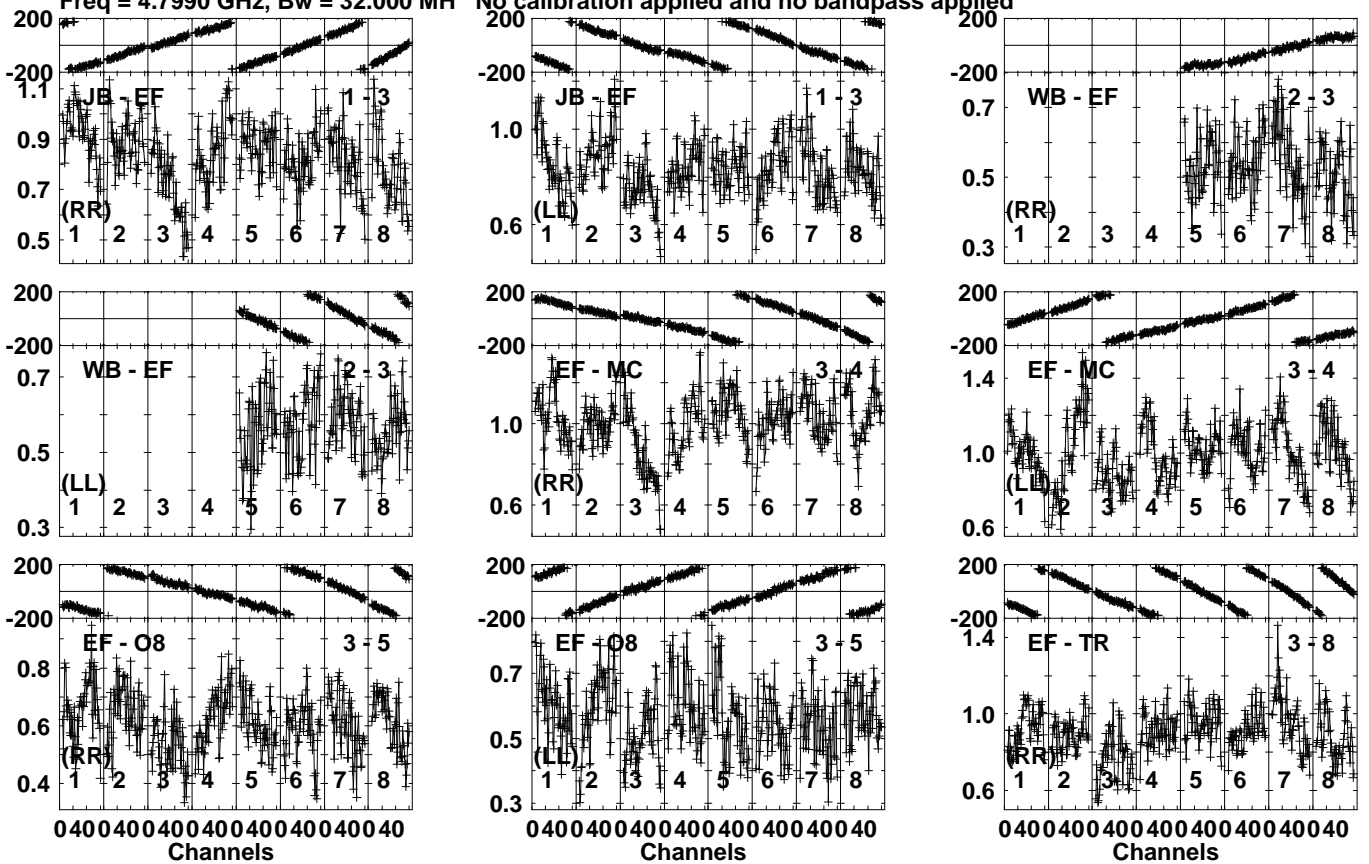
Lower frame: Milli Ampl Jy Top frame: Phas deg Vector averaged cross-power spectrum Several baselines displayed Timerange: 00/09:08:21 to 00/09:10:49
