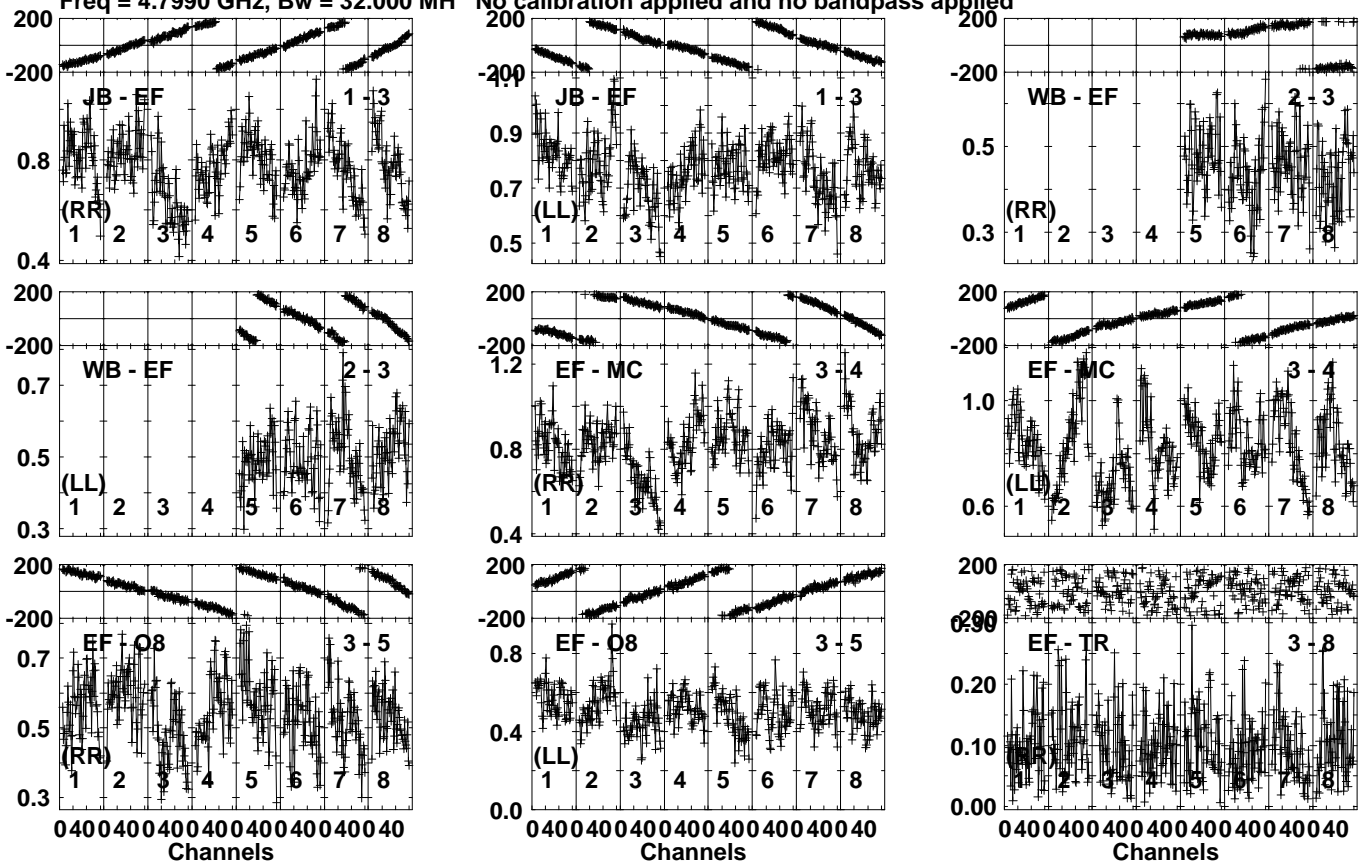
Lower frame: Milli Ampl Jy Top frame: Phas deg Vector averaged cross-power spectrum Several baselines displayed Timerange: 00/11:31:51 to 00/11:33:49
