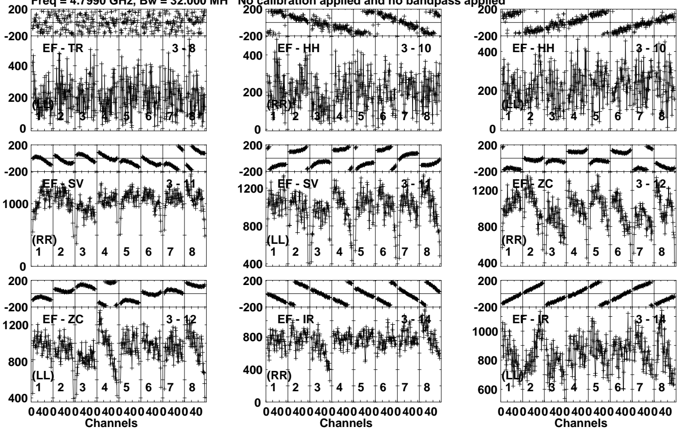
Lower frame: Micro Ampl Jy Top frame: Phas deg Vector averaged cross-power spectrum Several baselines displayed Timerange: 00/09:27:01 to 00/09:28:49
