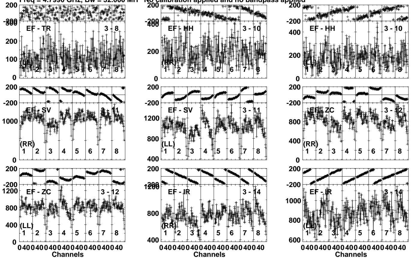
Lower frame: Micro Ampl Jy Top frame: Phas deg Vector averaged cross-power spectrum Several baselines displayed Timerange: 00/11:07:31 to 00/11:09:29
