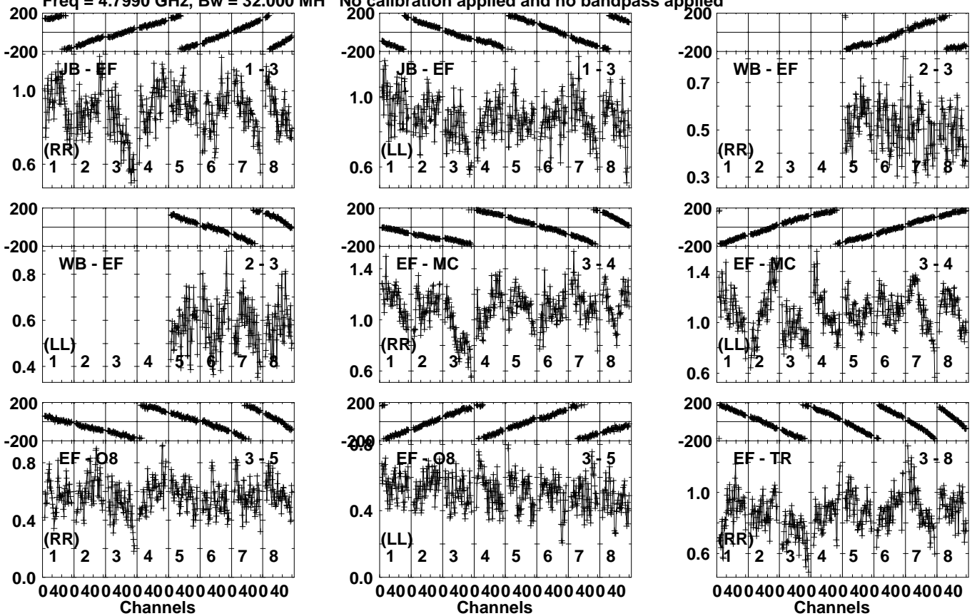
Lower frame: Milli Ampl Jy Top frame: Phas deg Vector averaged cross-power spectrum Several baselines displayed Timerange: 00/05:42:11 to 00/05:44:39
