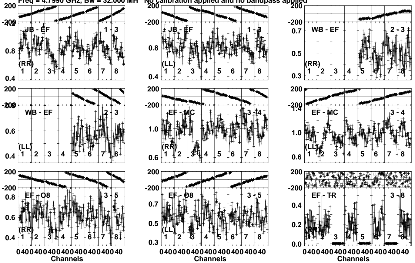
Lower frame: Milli Ampl Jy Top frame: Phas deg Vector averaged cross-power spectrum Several baselines displayed Timerange: 00/09:44:11 to 00/09:46:09
