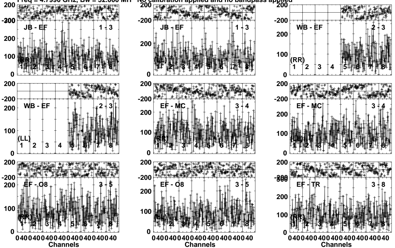
Lower frame: Micro Ampl Jy Top frame: Phas deg Vector averaged cross-power spectrum Several baselines displayed Timerange: 00/05:55:51 to 00/05:59:19
