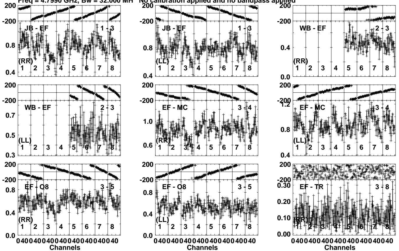
Lower frame: Milli Ampl Jy Top frame: Phas deg Vector averaged cross-power spectrum Several baselines displayed Timerange: 00/10:55:41 to 00/10:58:09
