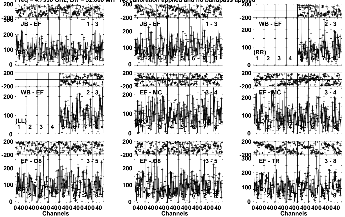
Lower frame: Micro Ampl Jy Top frame: Phas deg Vector averaged cross-power spectrum Several baselines displayed Timerange: 00/11:39:51 to 00/11:43:19
