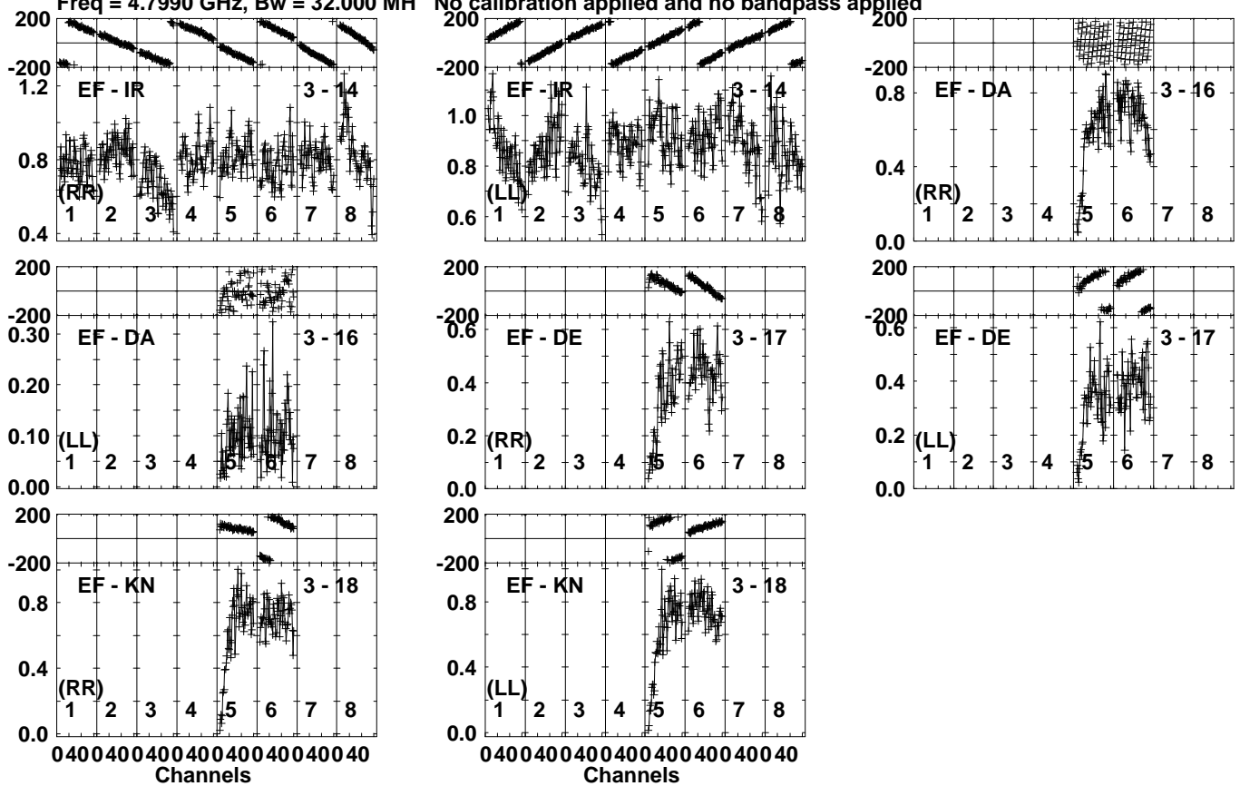
Lower frame: Milli Ampl Jy Top frame: Phas deg Vector averaged cross-power spectrum Several baselines displayed Timerange: 00/06:06:01 to 00/06:07:49
