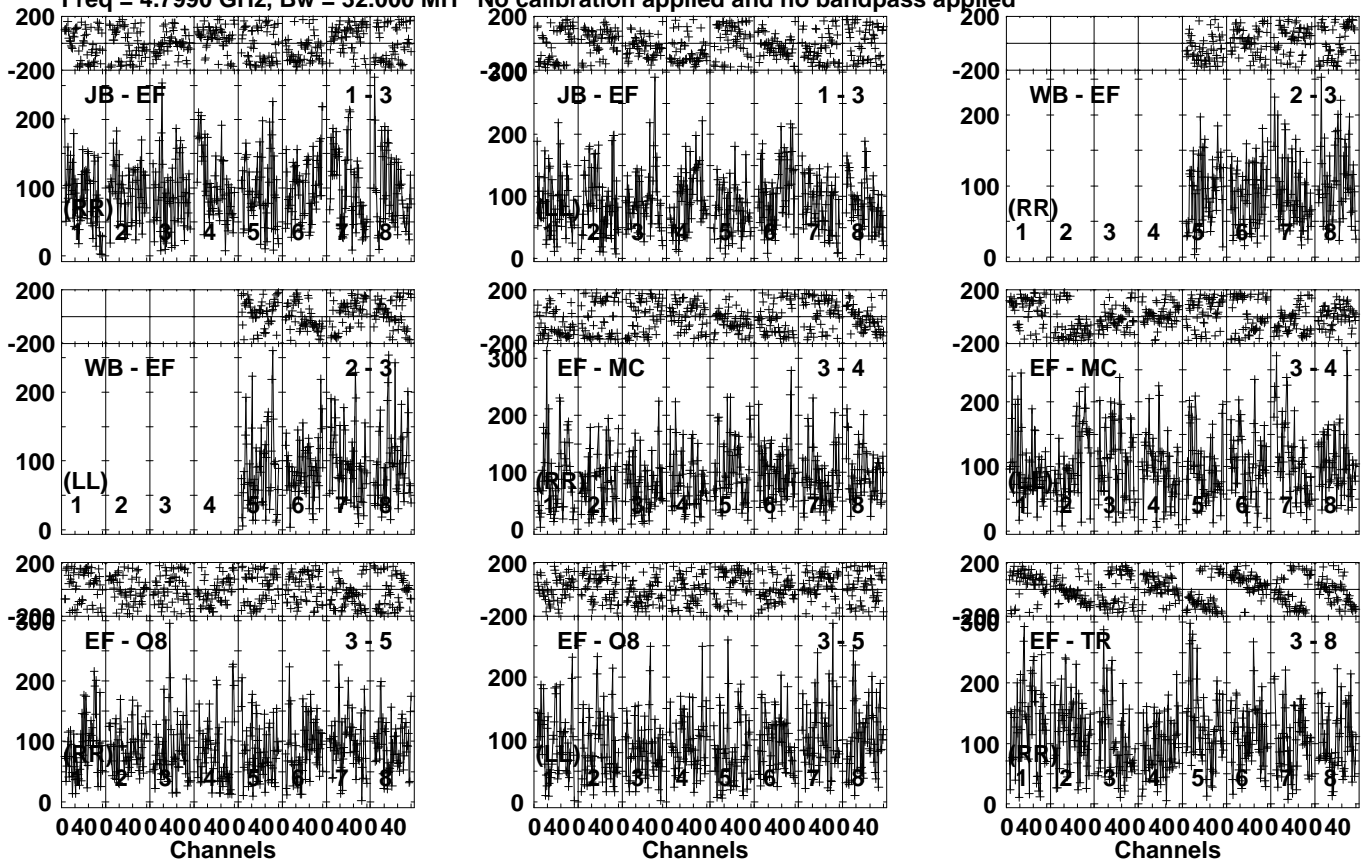
Lower frame: Micro Ampl Jy Top frame: Phas deg Vector averaged cross-power spectrum Several baselines displayed Timerange: 00/08:40:51 to 00/08:44:19
