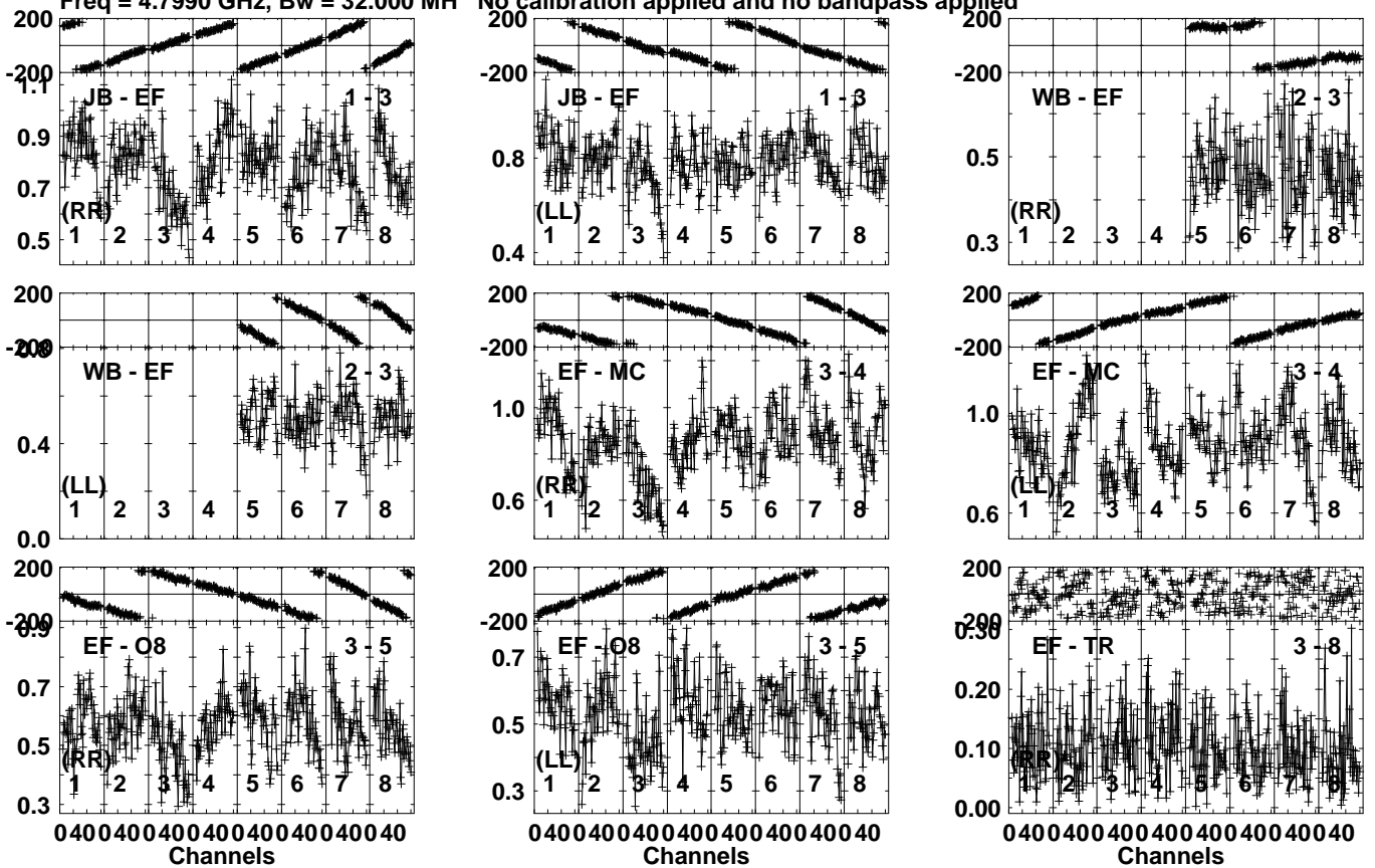
Lower frame: Milli Ampl Jy Top frame: Phas deg Vector averaged cross-power spectrum Several baselines displayed Timerange: 00/11:07:31 to 00/11:09:29
