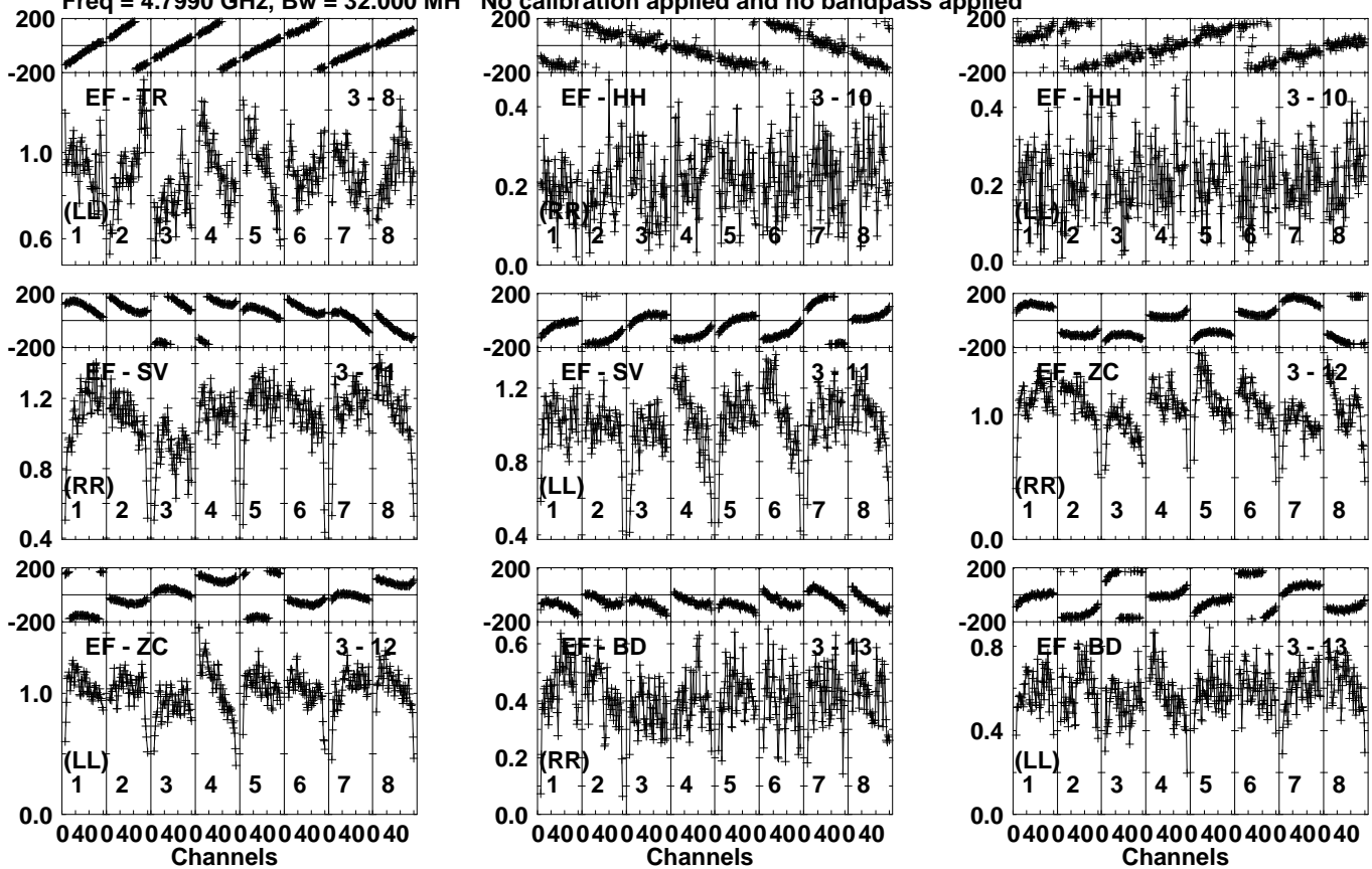
Lower frame: Milli Ampl Jy Top frame: Phas deg Vector averaged cross-power spectrum Several baselines displayed Timerange: 00/05:36:51 to 00/05:38:39
