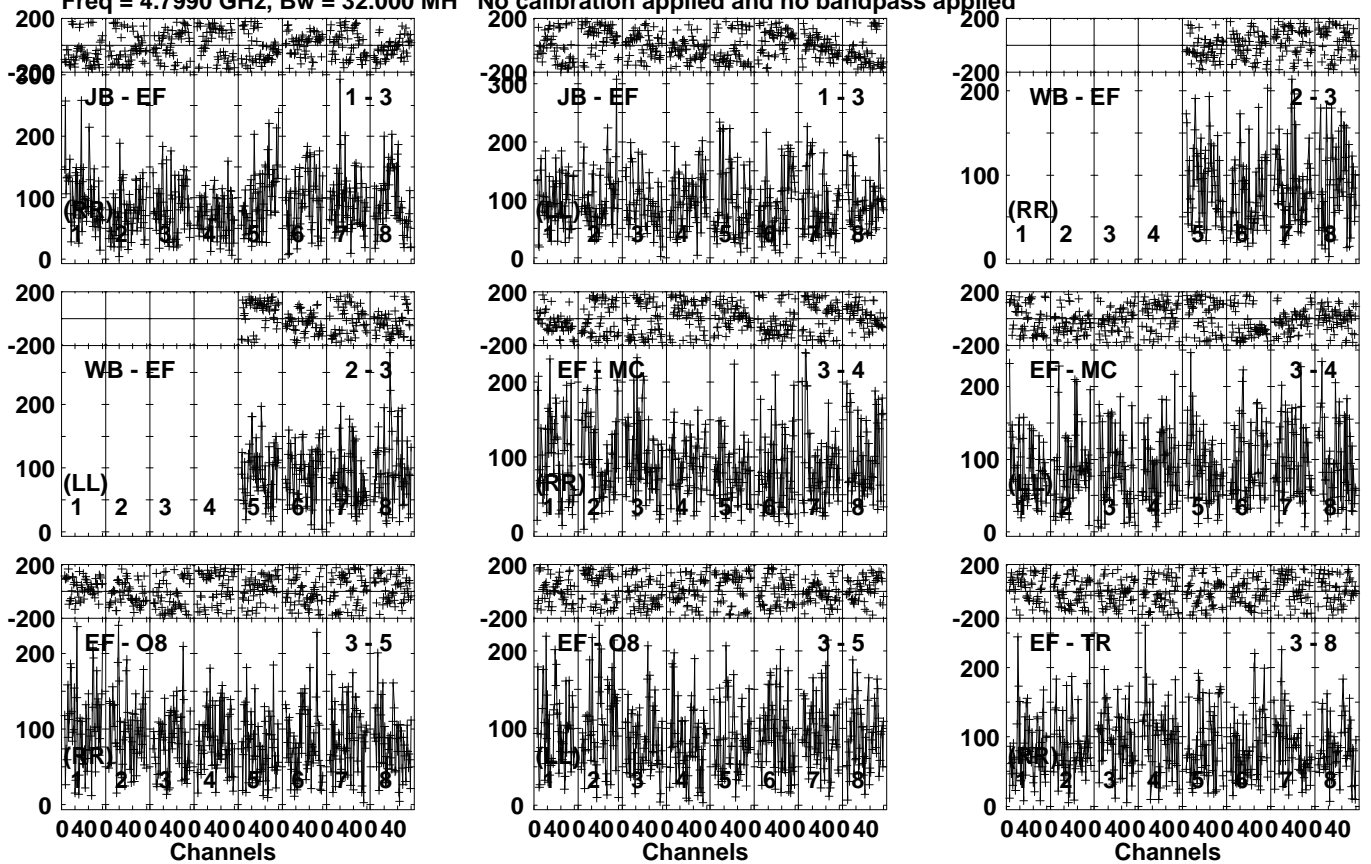
Lower frame: Micro Ampl Jy Top frame: Phas deg Vector averaged cross-power spectrum Several baselines displayed Timerange: 00/10:58:11 to 00/11:01:39
