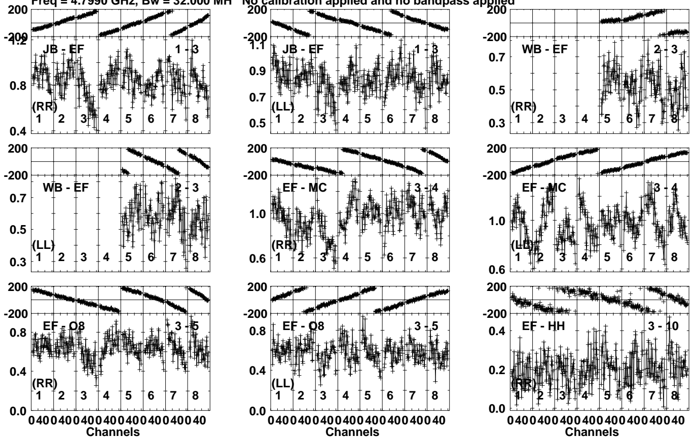
Lower frame: Milli Ampl Jy Top frame: Phas deg Vector averaged cross-power spectrum Several baselines displayed Timerange: 00/09:37:31 to 00/09:39:59
