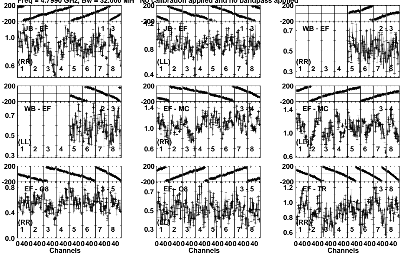
Lower frame: Milli Ampl Jy Top frame: Phas deg Vector averaged cross-power spectrum Several baselines displayed Timerange: 00/05:59:21 to 00/06:01:49
