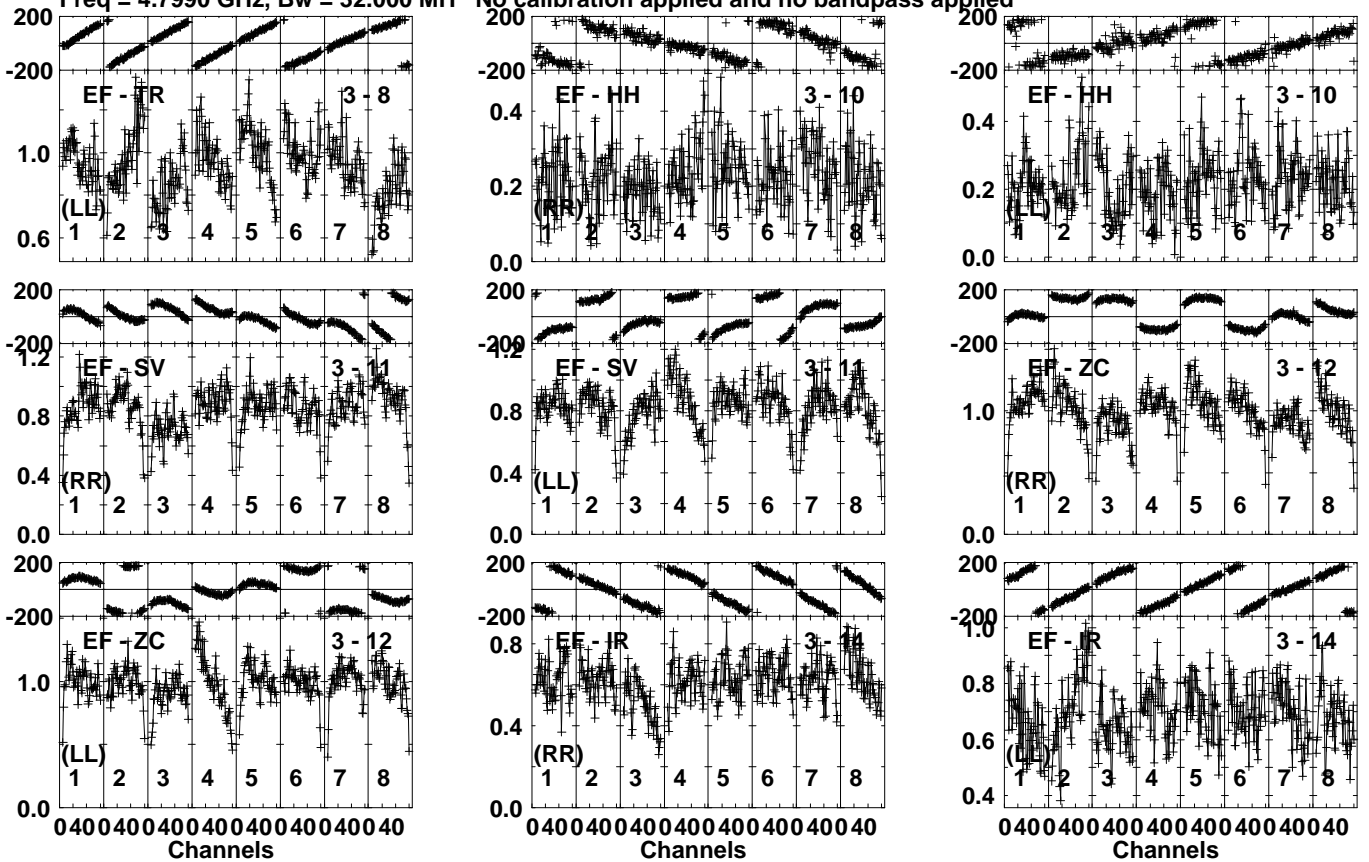
Lower frame: Milli Ampl Jy Top frame: Phas deg Vector averaged cross-power spectrum Several baselines displayed Timerange: 00/07:57:51 to 00/07:59:39
