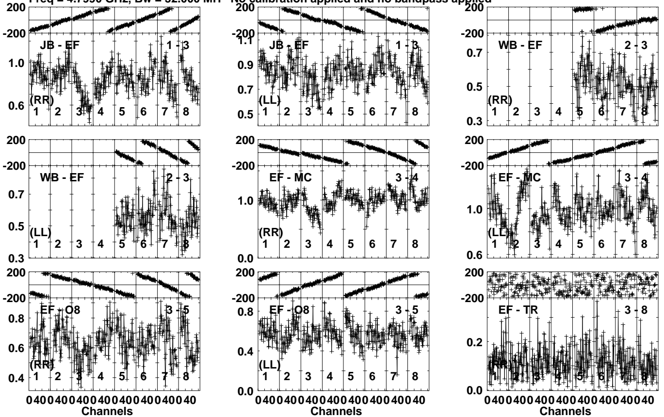
Lower frame: Milli Ampl Jy Top frame: Phas deg Vector averaged cross-power spectrum Several baselines displayed Timerange: 00/09:20:21 to 00/09:22:49
