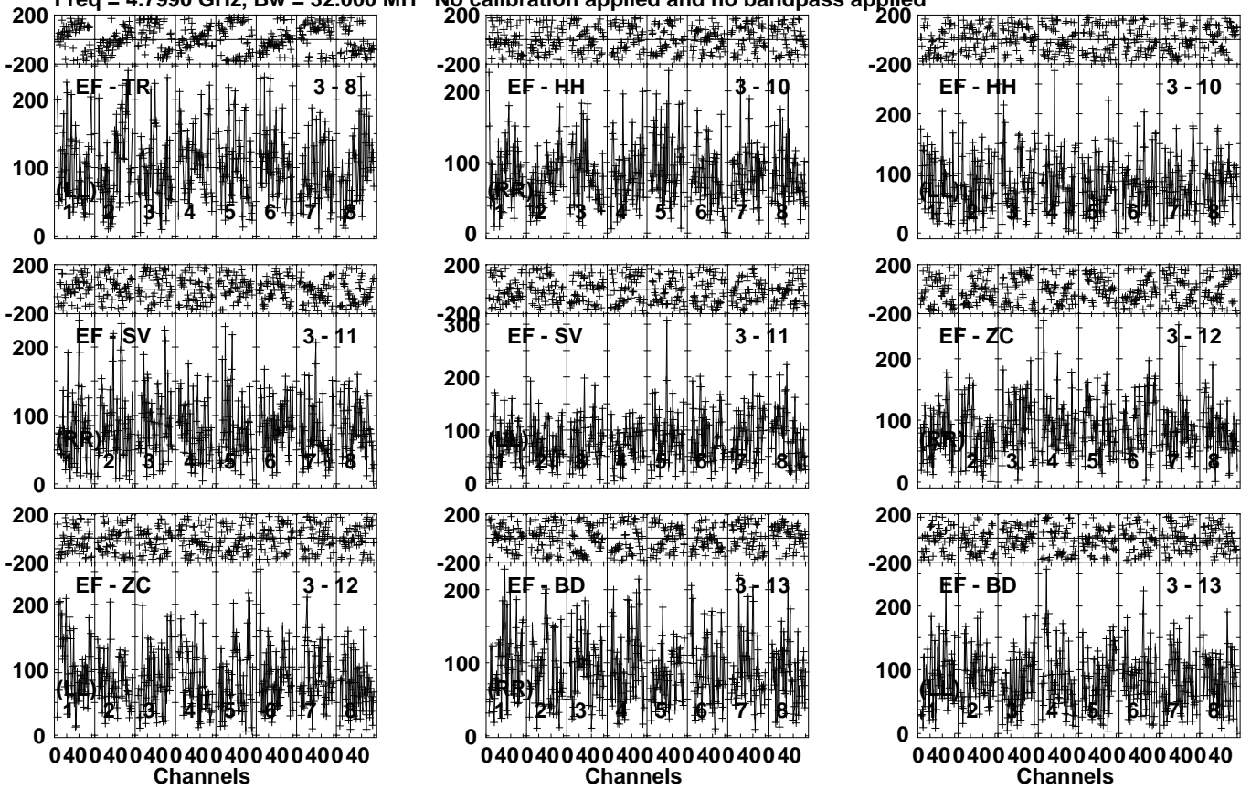
Lower frame: Micro Ampl Jy Top frame: Phas deg Vector averaged cross-power spectrum Several baselines displayed Timerange: 00/05:20:41 to 00/05:24:09
