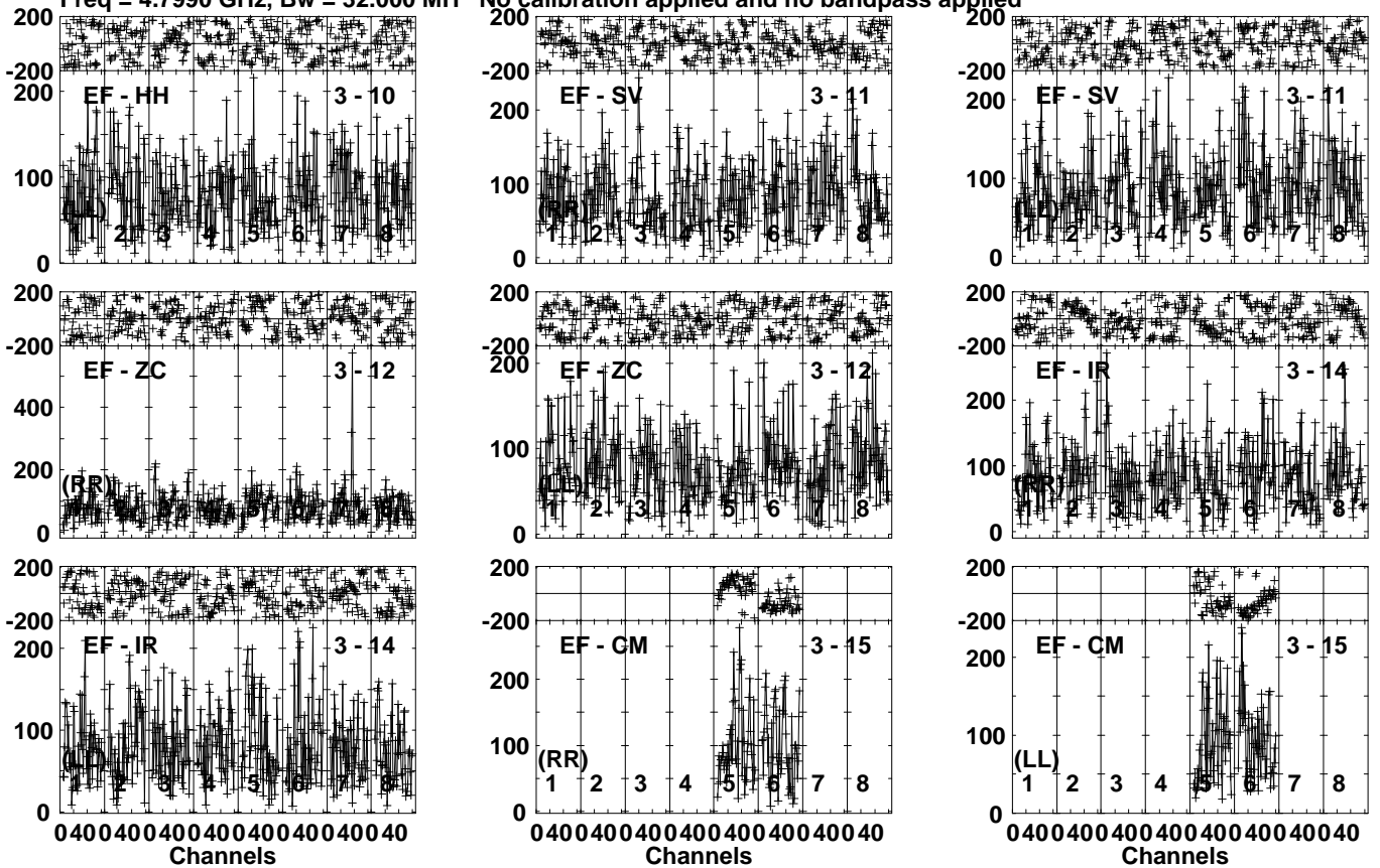
Lower frame: Micro Ampl Jy Top frame: Phas deg Vector averaged cross-power spectrum Several baselines displayed Timerange: 00/09:40:01 to 00/09:43:29
