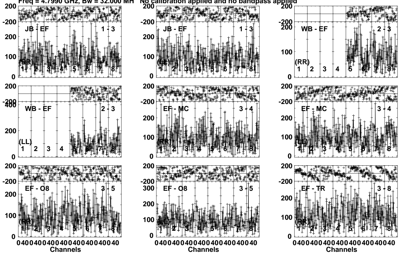
Lower frame: Micro Ampl Jy Top frame: Phas deg Vector averaged cross-power spectrum Several baselines displayed Timerange: 00/08:05:41 to 00/08:09:09
