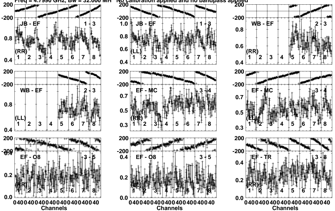
Lower frame: Milli Ampl Jy Top frame: Phas deg Vector averaged cross-power spectrum Several baselines displayed Timerange: 00/04:57:31 to 00/04:59:59
