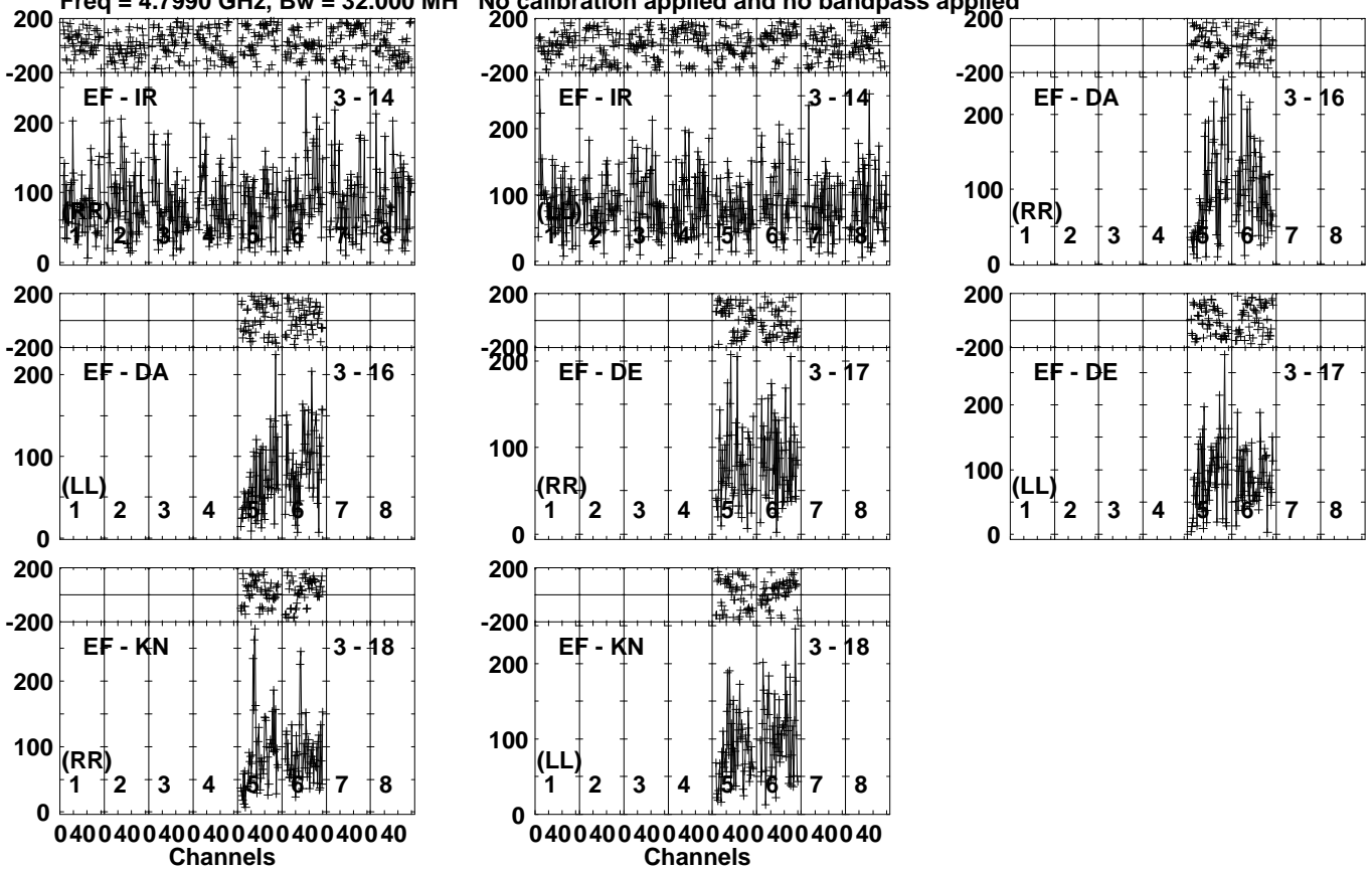
Lower frame: Micro Ampl Jy Top frame: Phas deg Vector averaged cross-power spectrum Several baselines displayed Timerange: 00/06:07:51 to 00/06:11:19
