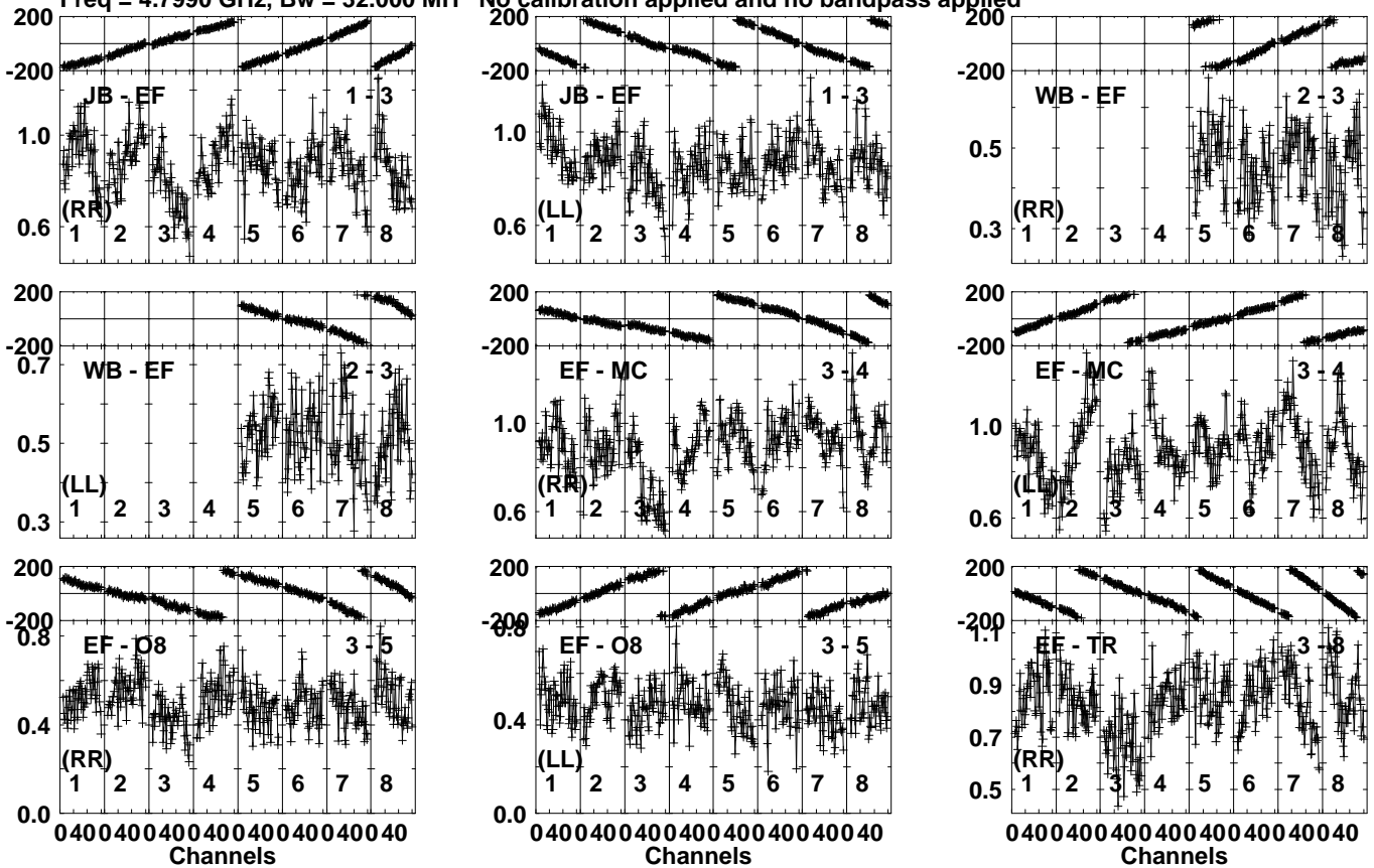
Lower frame: Milli Ampl Jy Top frame: Phas deg Vector averaged cross-power spectrum Several baselines displayed Timerange: 00/04:07:01 to 00/04:09:29
