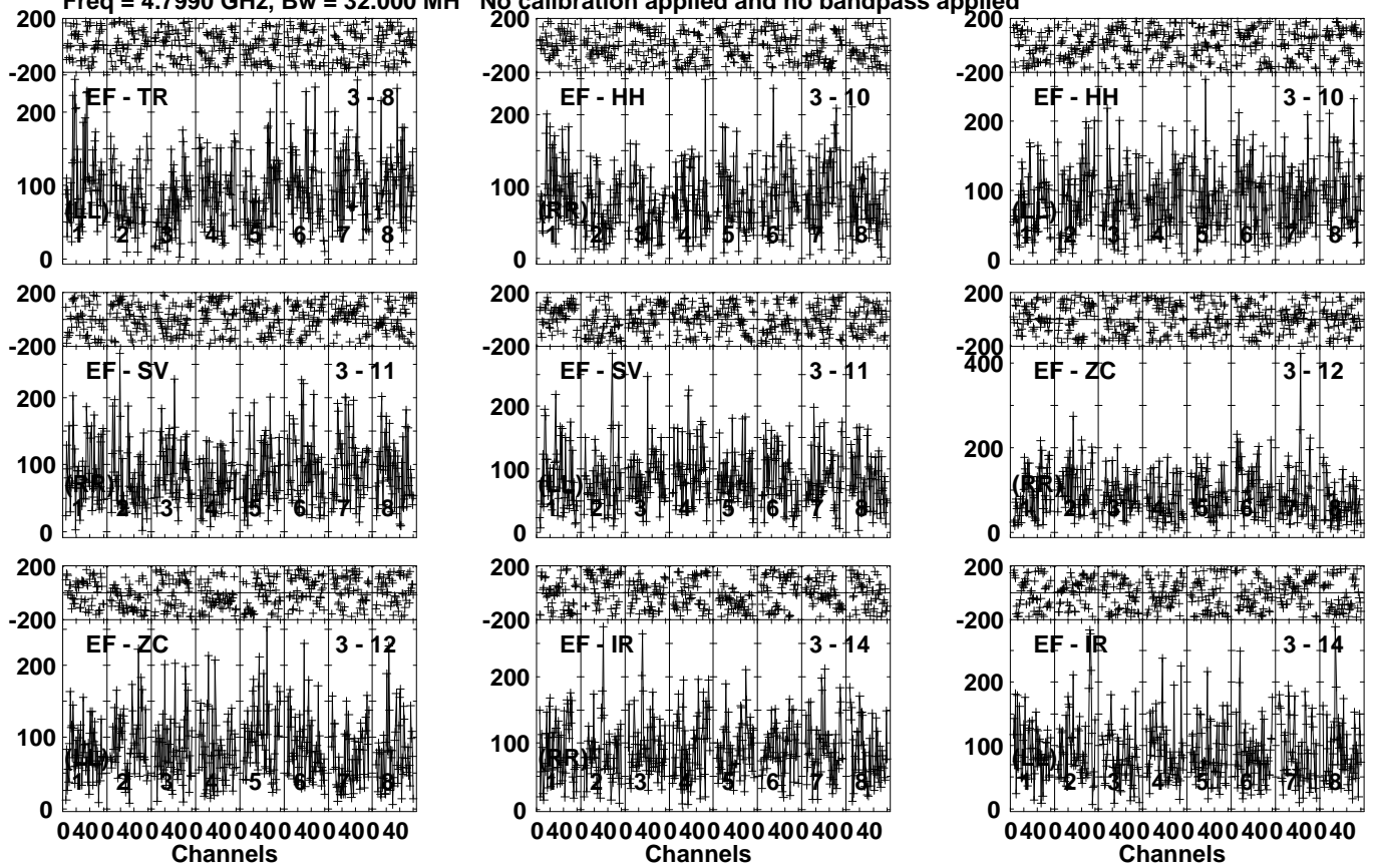
Lower frame: Micro Ampl Jy Top frame: Phas deg Vector averaged cross-power spectrum Several baselines displayed Timerange: 00/09:16:53 to 00/09:20:19
