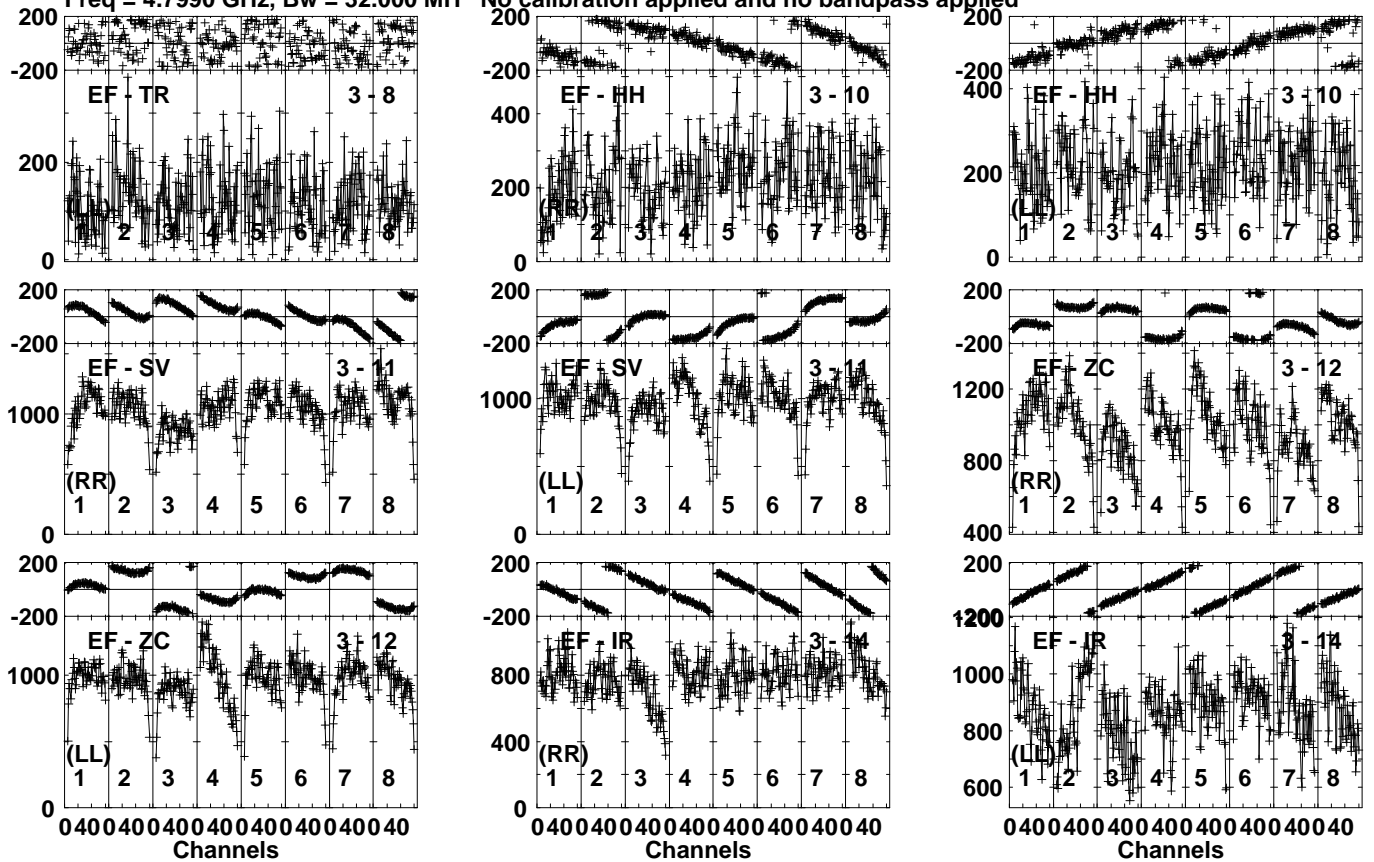
Lower frame: Micro Ampl Jy Top frame: Phas deg Vector averaged cross-power spectrum Several baselines displayed Timerange: 00/09:20:21 to 00/09:22:49
