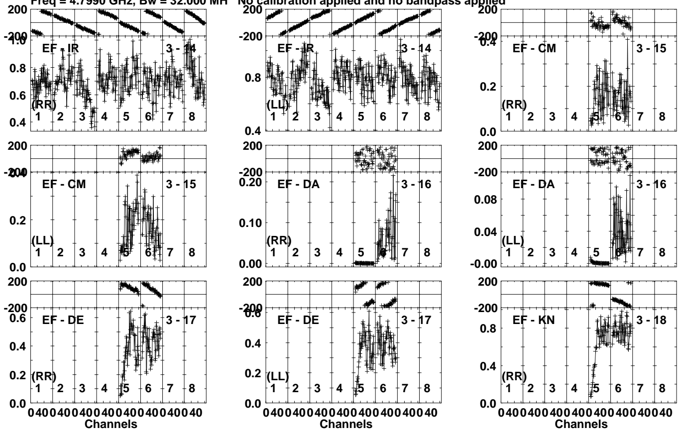
Lower frame: Milli Ampl Jy Top frame: Phas deg Vector averaged cross-power spectrum Several baselines displayed Timerange: 00/06:52:31 to 00/06:54:59
