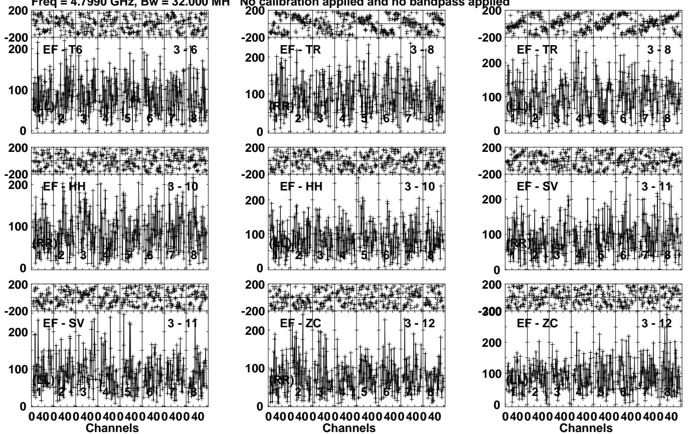
Lower frame: Micro Ampl Jy Top frame: Phas deg Vector averaged cross-power spectrum Several baselines displayed Timerange: 00/04:45:31 to 00/04:48:59
