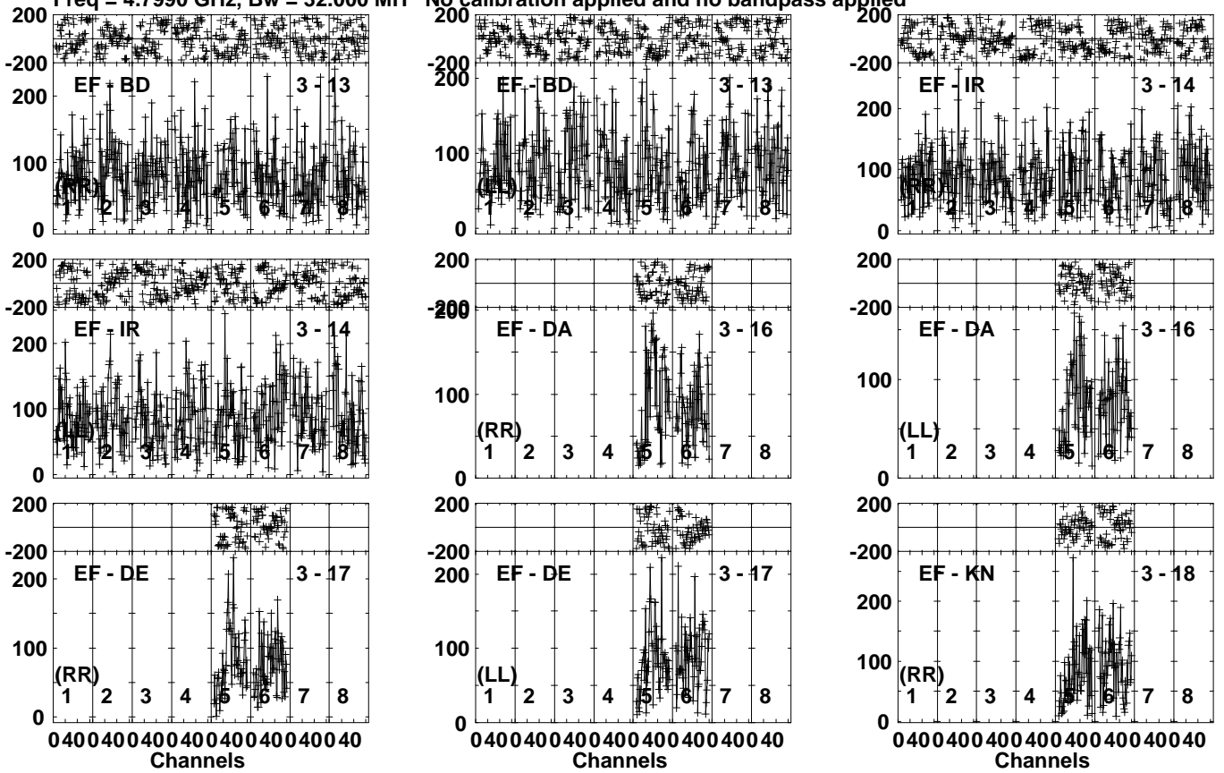
Lower frame: Micro Ampl Jy Top frame: Phas deg Vector averaged cross-power spectrum Several baselines displayed Timerange: 00/04:51:31 to 00/04:54:59
