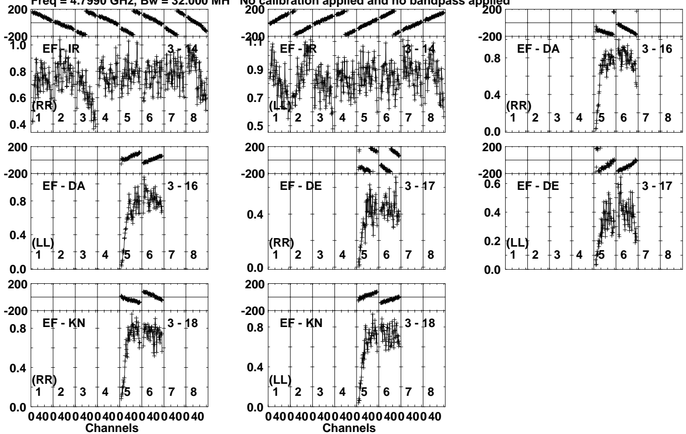
Lower frame: Milli Ampl Jy Top frame: Phas deg Vector averaged cross-power spectrum Several baselines displayed Timerange: 00/04:19:41 to 00/04:21:29
