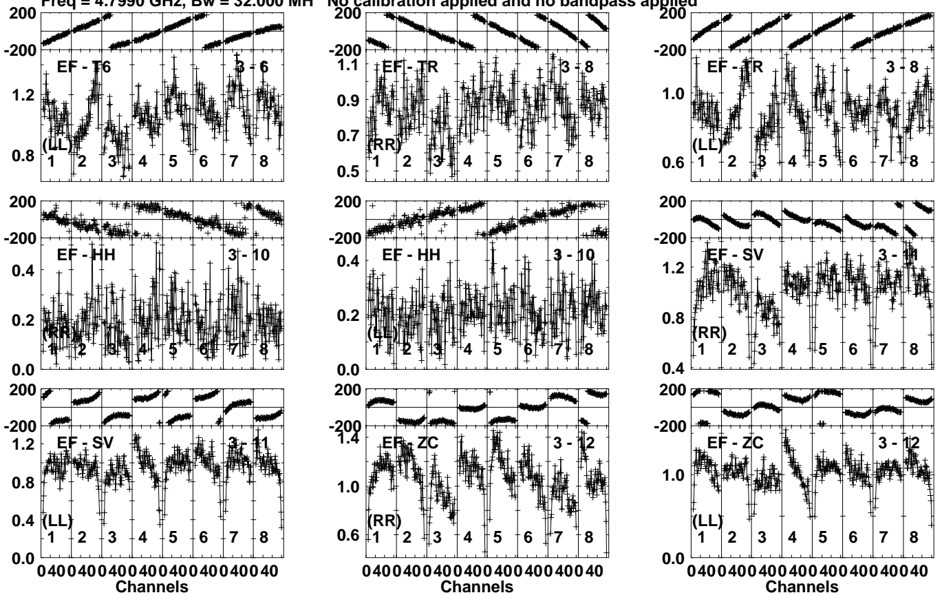
Lower frame: Milli Ampl Jy Top frame: Phas deg Vector averaged cross-power spectrum Several baselines displayed Timerange: 00/04:31:41 to 00/04:33:29
