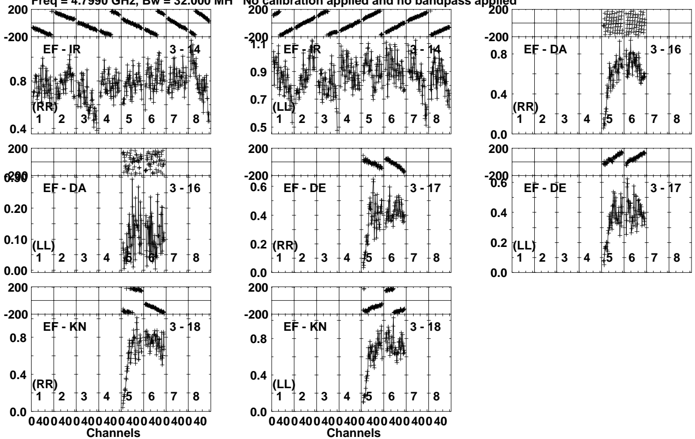
Lower frame: Milli Ampl Jy Top frame: Phas deg Vector averaged cross-power spectrum Several baselines displayed Timerange: 00/05:12:51 to 00/05:14:39
