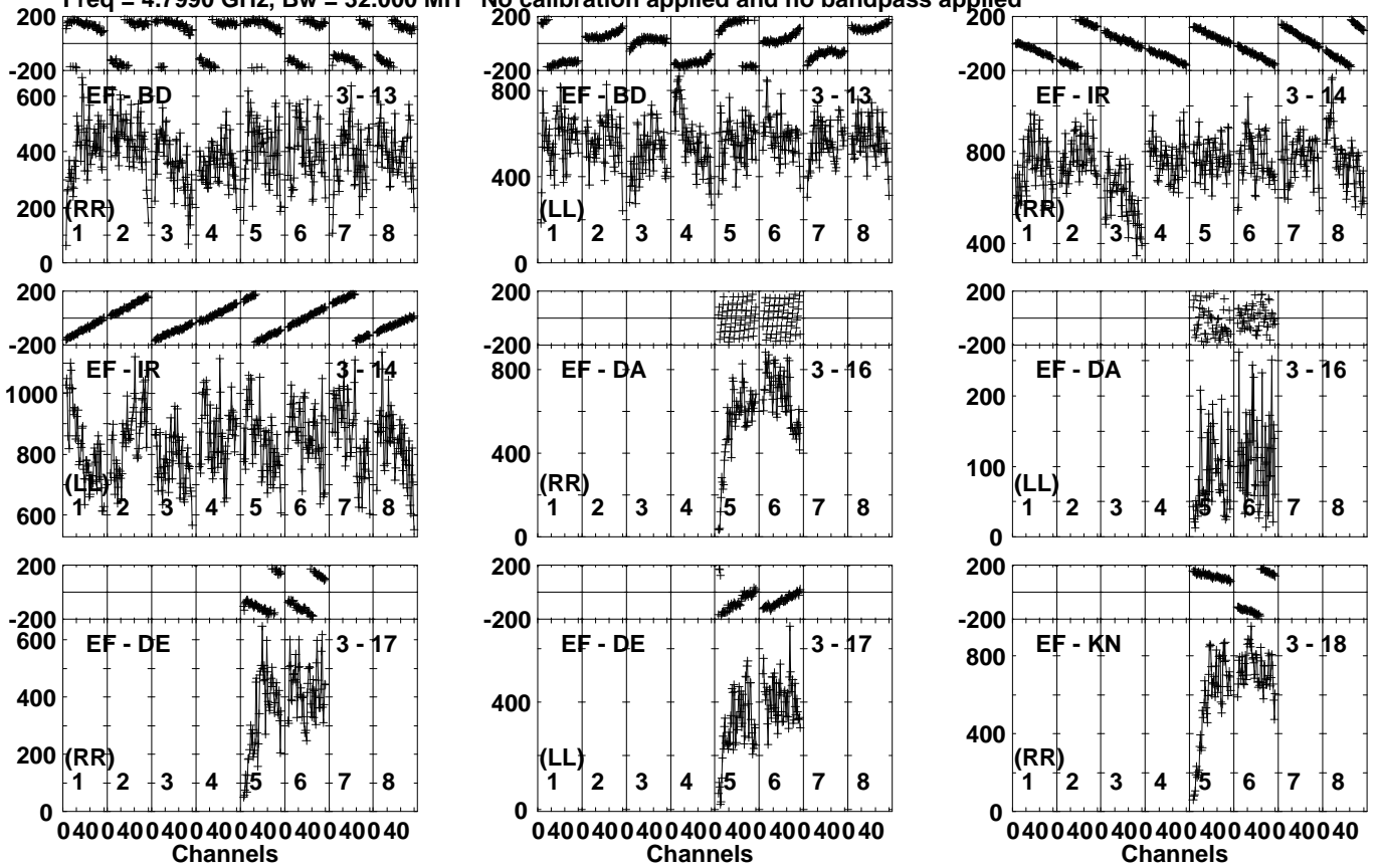
Lower frame: Micro Ampl Jy Top frame: Phas deg Vector averaged cross-power spectrum Several baselines displayed Timerange: 00/04:43:41 to 00/04:45:29
