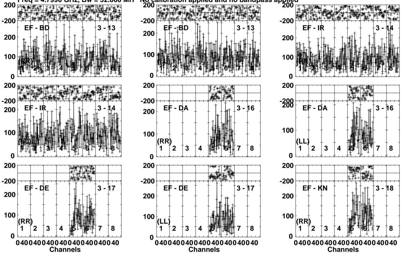
Lower frame: Micro Ampl Jy Top frame: Phas deg Vector averaged cross-power spectrum Several baselines displayed Timerange: 00/04:39:31 to 00/04:42:59
