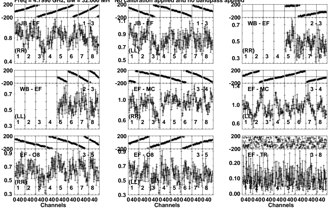
Lower frame: Milli Ampl Jy Top frame: Phas deg Vector averaged cross-power spectrum Several baselines displayed Timerange: 00/10:20:41 to 00/10:22:39
