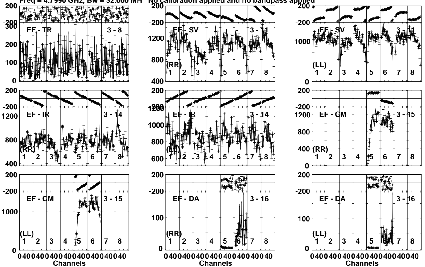
Lower frame: Micro Ampl Jy Top frame: Phas deg Vector averaged cross-power spectrum Several baselines displayed Timerange: 00/11:31:51 to 00/11:33:49
