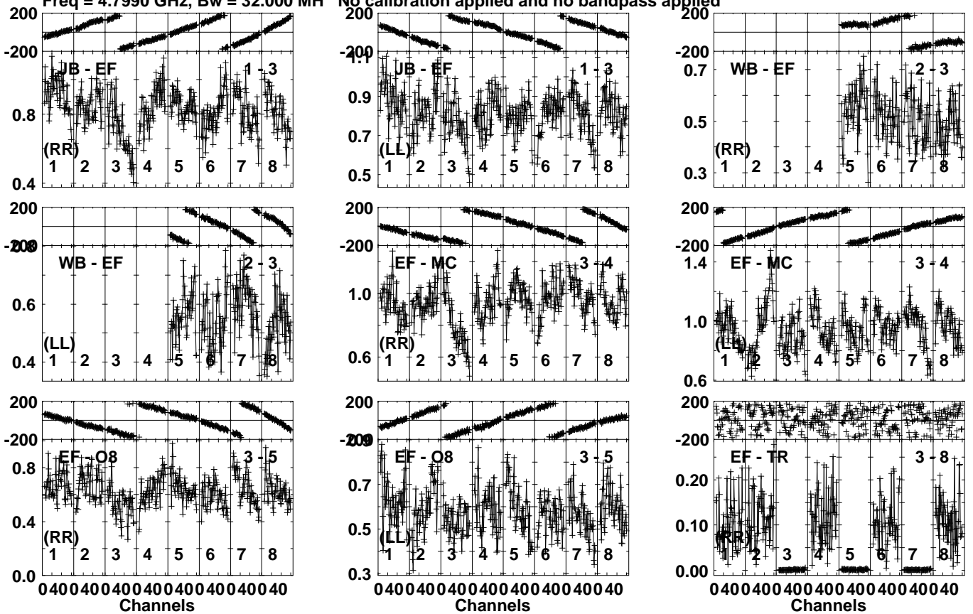
Lower frame: Milli Ampl Jy Top frame: Phas deg Vector averaged cross-power spectrum Several baselines displayed Timerange: 00/09:49:41 to 00/09:52:09
