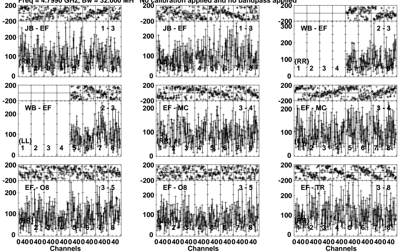
Lower frame: Micro Ampl Jy Top frame: Phas deg Vector averaged cross-power spectrum Several baselines displayed Timerange: 00/07:07:01 to 00/07:10:29
