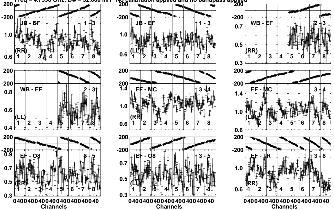
Lower frame: Milli Ampl Jy Top frame: Phas deg Vector averaged cross-power spectrum Several baselines displayed Timerange: 00/07:23:11 to 00/07:24:59
