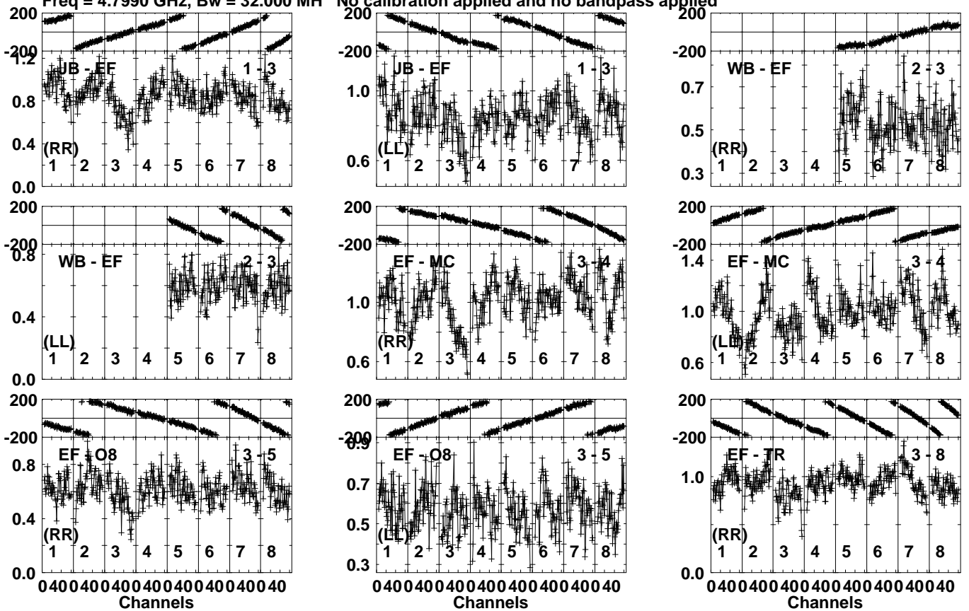
Lower frame: Milli Ampl Jy Top frame: Phas deg Vector averaged cross-power spectrum Several baselines displayed Timerange: 00/08:56:21 to 00/08:58:49
