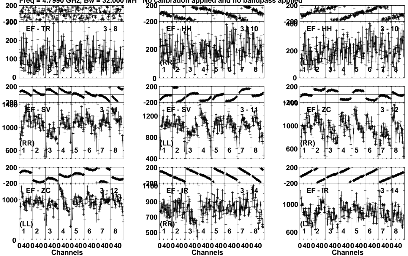
Lower frame: Micro Ampl Jy Top frame: Phas deg Vector averaged cross-power spectrum Several baselines displayed Timerange: 00/10:20:41 to 00/10:22:39
