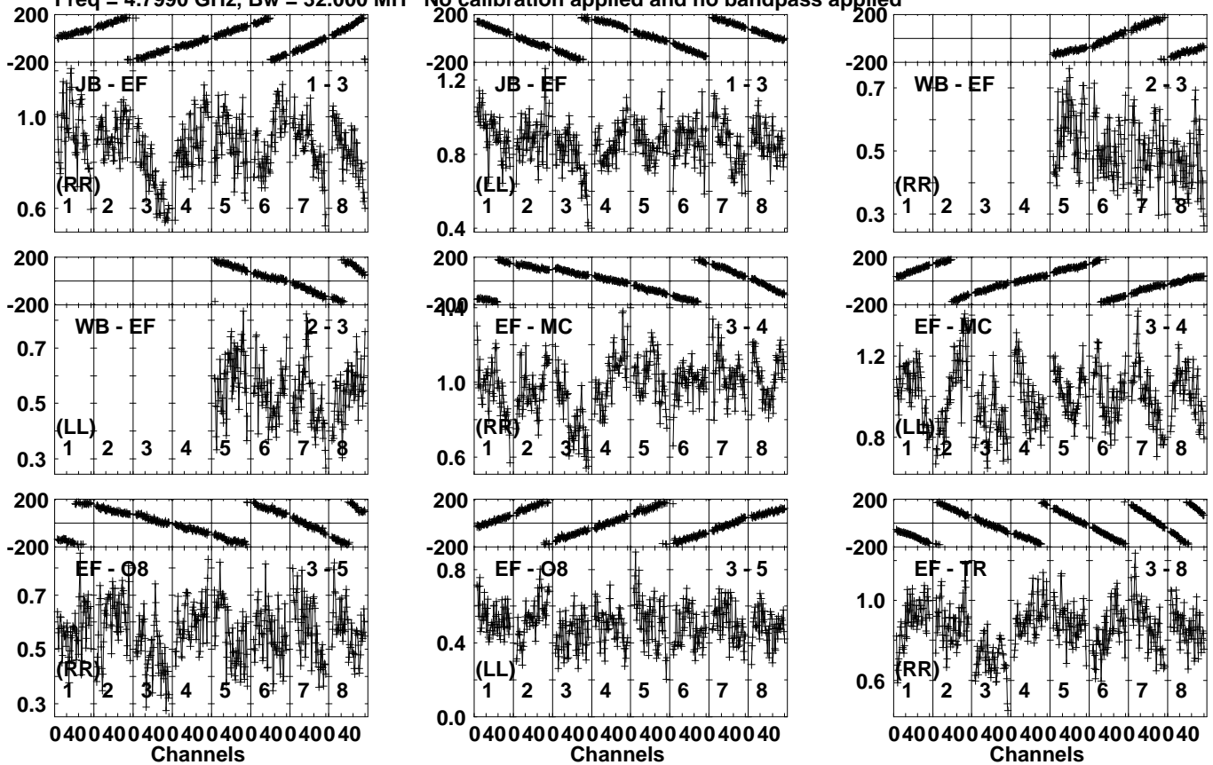
Lower frame: Milli Ampl Jy Top frame: Phas deg Vector averaged cross-power spectrum Several baselines displayed Timerange: 00/05:06:11 to 00/05:08:39
