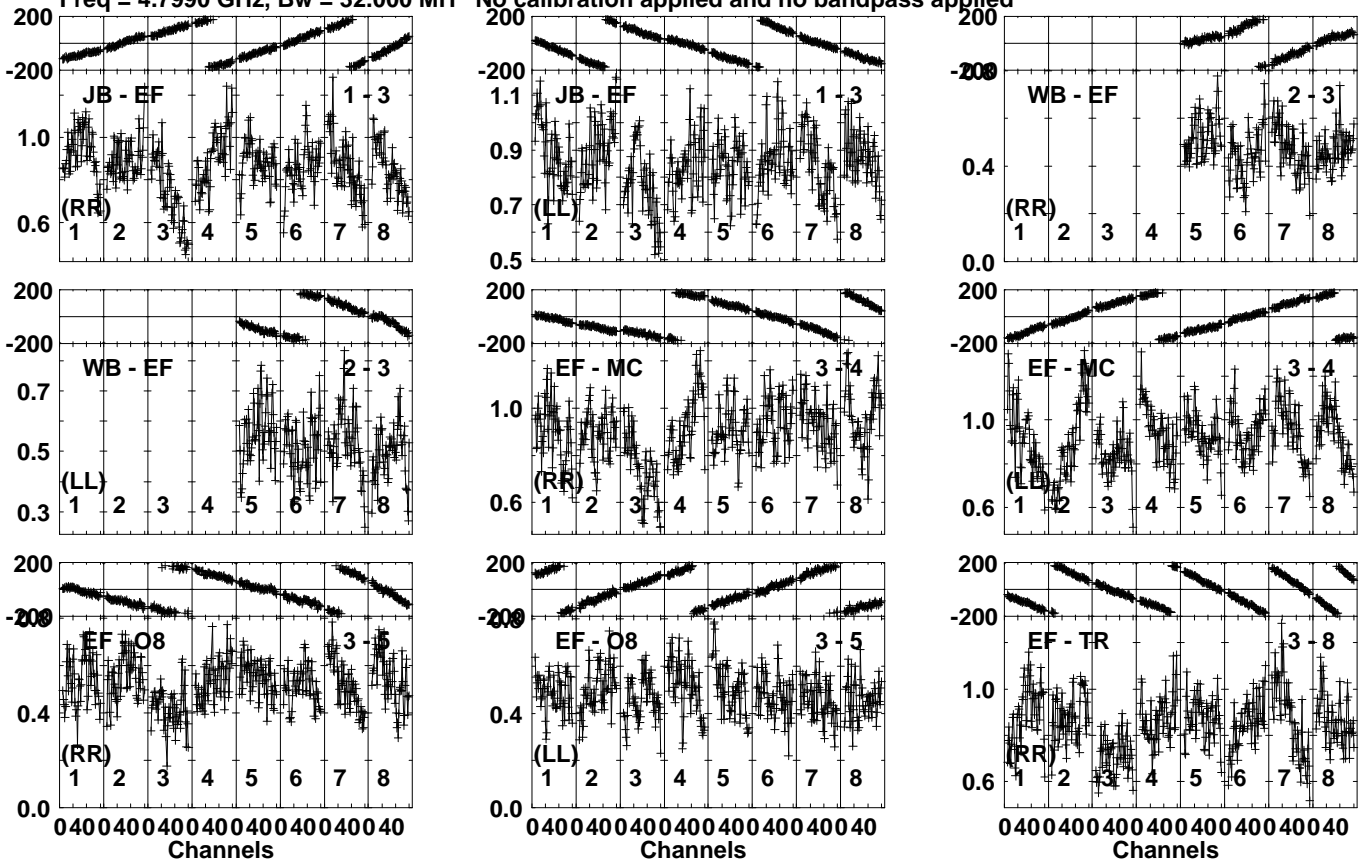
Lower frame: Milli Ampl Jy Top frame: Phas deg Vector averaged cross-power spectrum Several baselines displayed Timerange: 00/04:25:01 to 00/04:27:29
