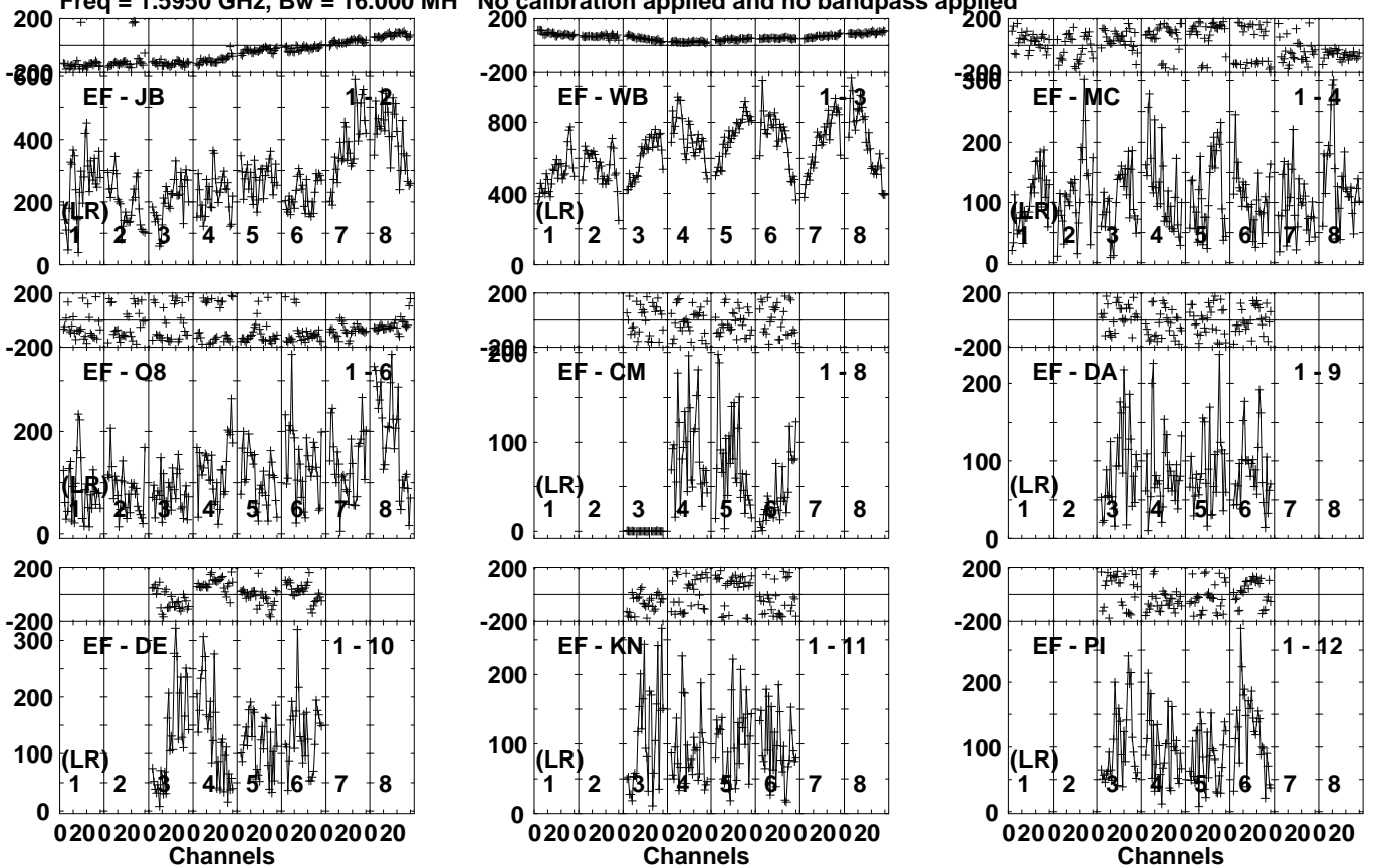
Lower frame: Micro Ampl Jy Top frame: Phas deg Vector averaged cross-power spectrum Several baselines displayed Timerange: 00/12:49:31 to 00/12:52:29
