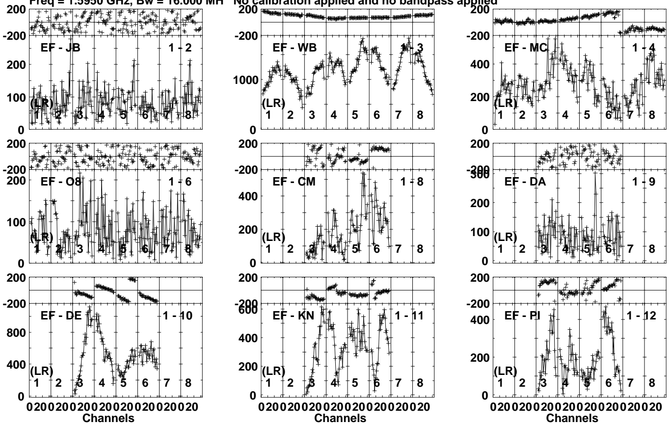
Lower frame: Micro Ampl Jy Top frame: Phas deg Vector averaged cross-power spectrum Several baselines displayed Timerange: 00/21:31:21 to 00/21:34:49
