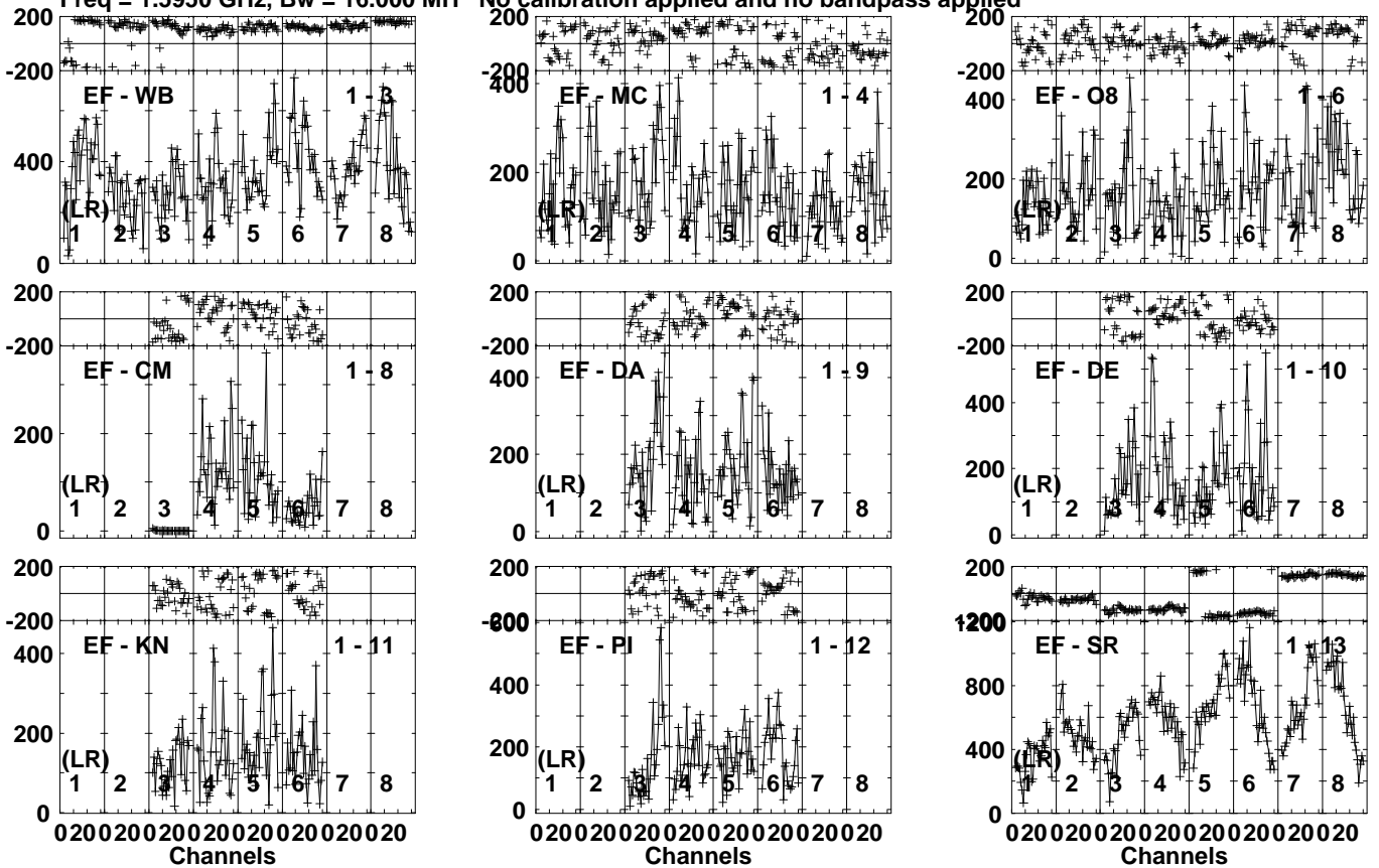
Lower frame: Micro Ampl Jy Top frame: Phas deg Vector averaged cross-power spectrum Several baselines displayed Timerange: 00/13:28:01 to 00/13:29:29
