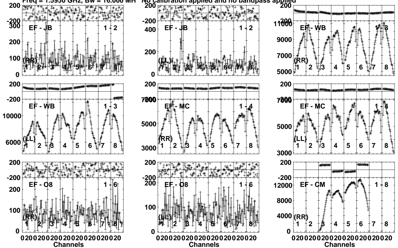
Lower frame: Micro Ampl Jy Top frame: Phas deg Vector averaged cross-power spectrum Several baselines displayed Timerange: 00/21:36:21 to 00/21:39:49
