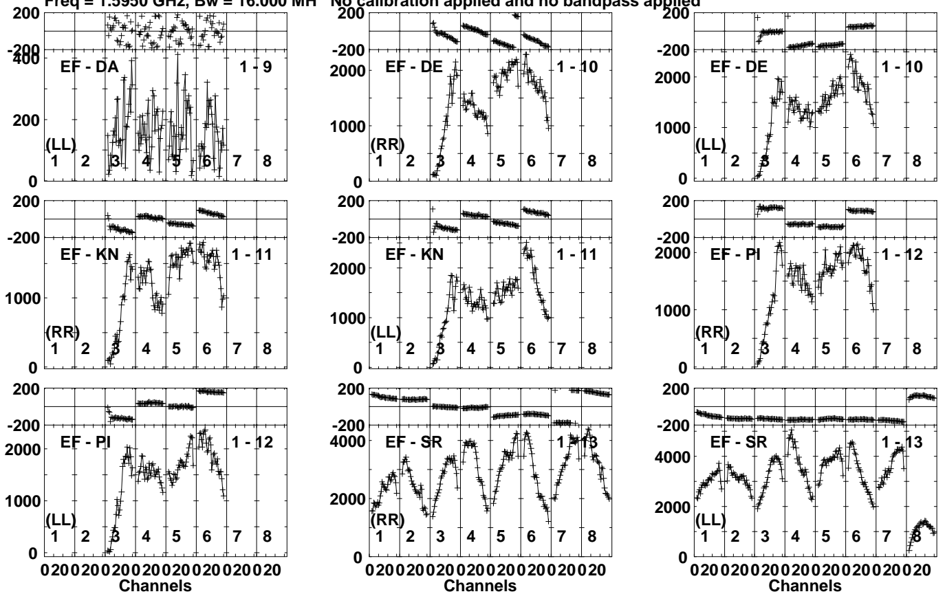
Lower frame: Micro Ampl Jy Top frame: Phas deg Vector averaged cross-power spectrum Several baselines displayed Timerange: 00/21:45:21 to 00/21:46:49
