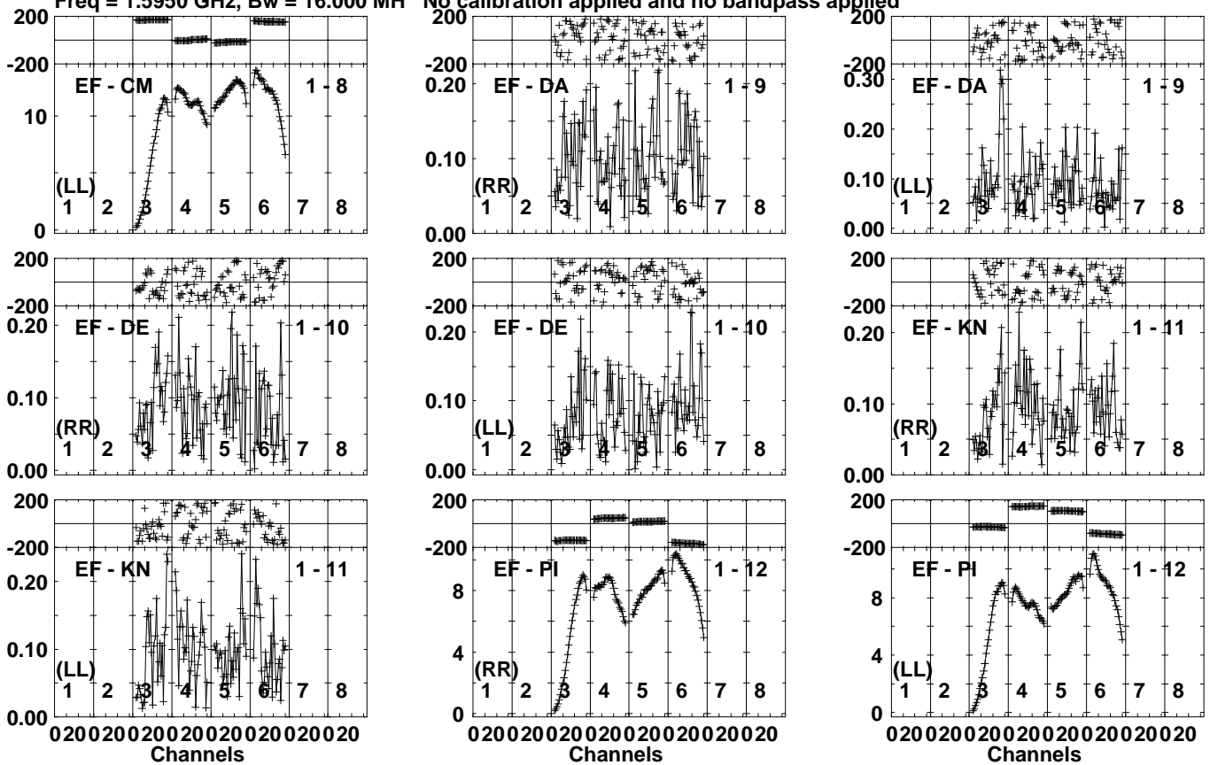
Lower frame: Milli Ampl Jy Top frame: Phas deg Vector averaged cross-power spectrum Several baselines displayed Timerange: 00/20:54:21 to 00/20:57:49
