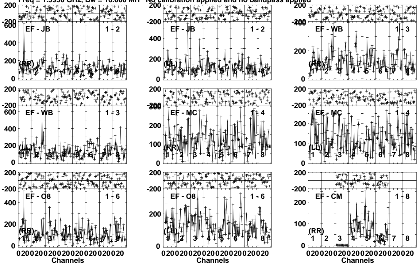
Lower frame: Micro Ampl Jy Top frame: Phas deg Vector averaged cross-power spectrum Several baselines displayed Timerange: 00/14:27:01 to 00/14:28:29
