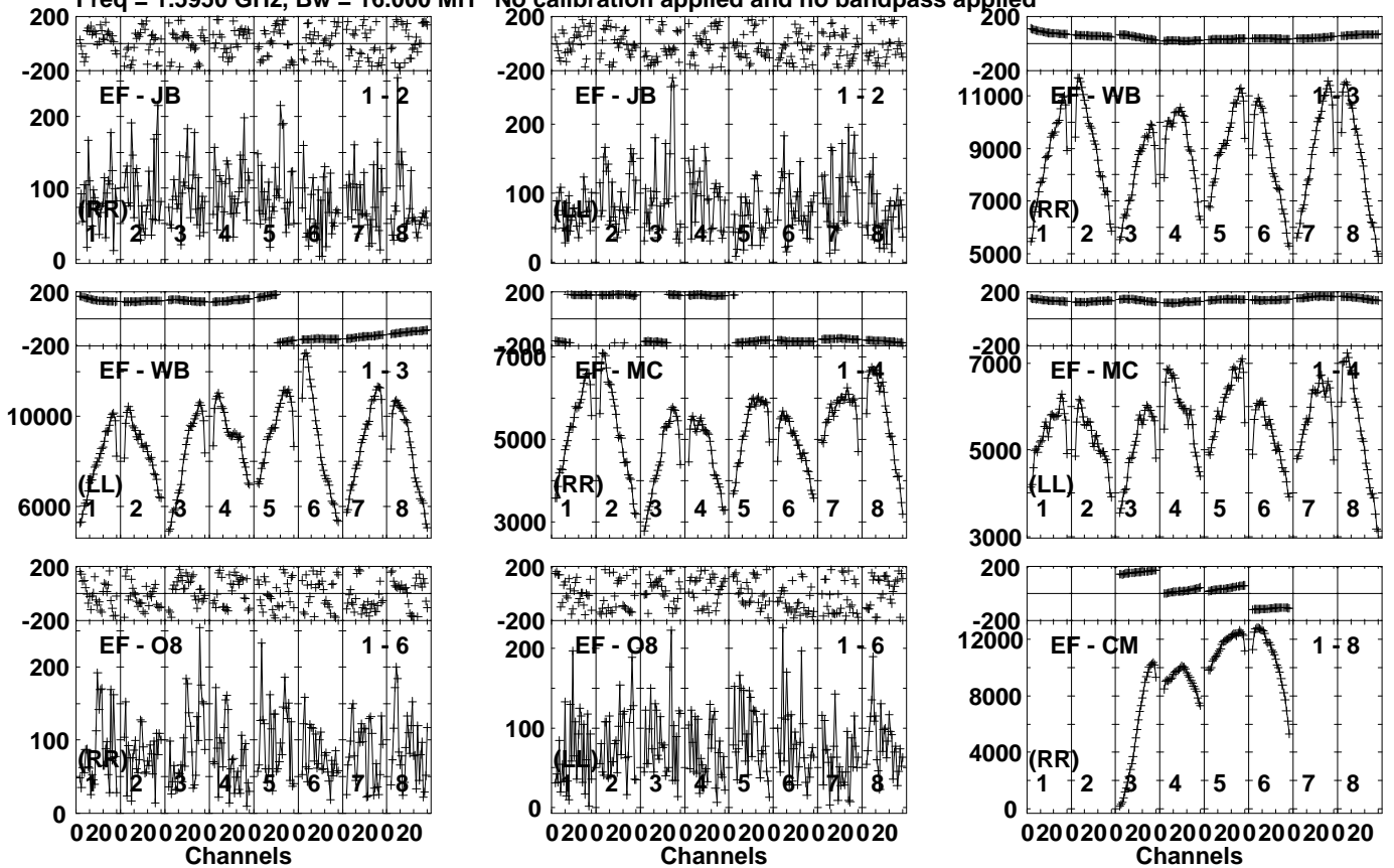
Lower frame: Micro Ampl Jy Top frame: Phas deg Vector averaged cross-power spectrum Several baselines displayed Timerange: 00/20:01:51 to 00/20:05:19
