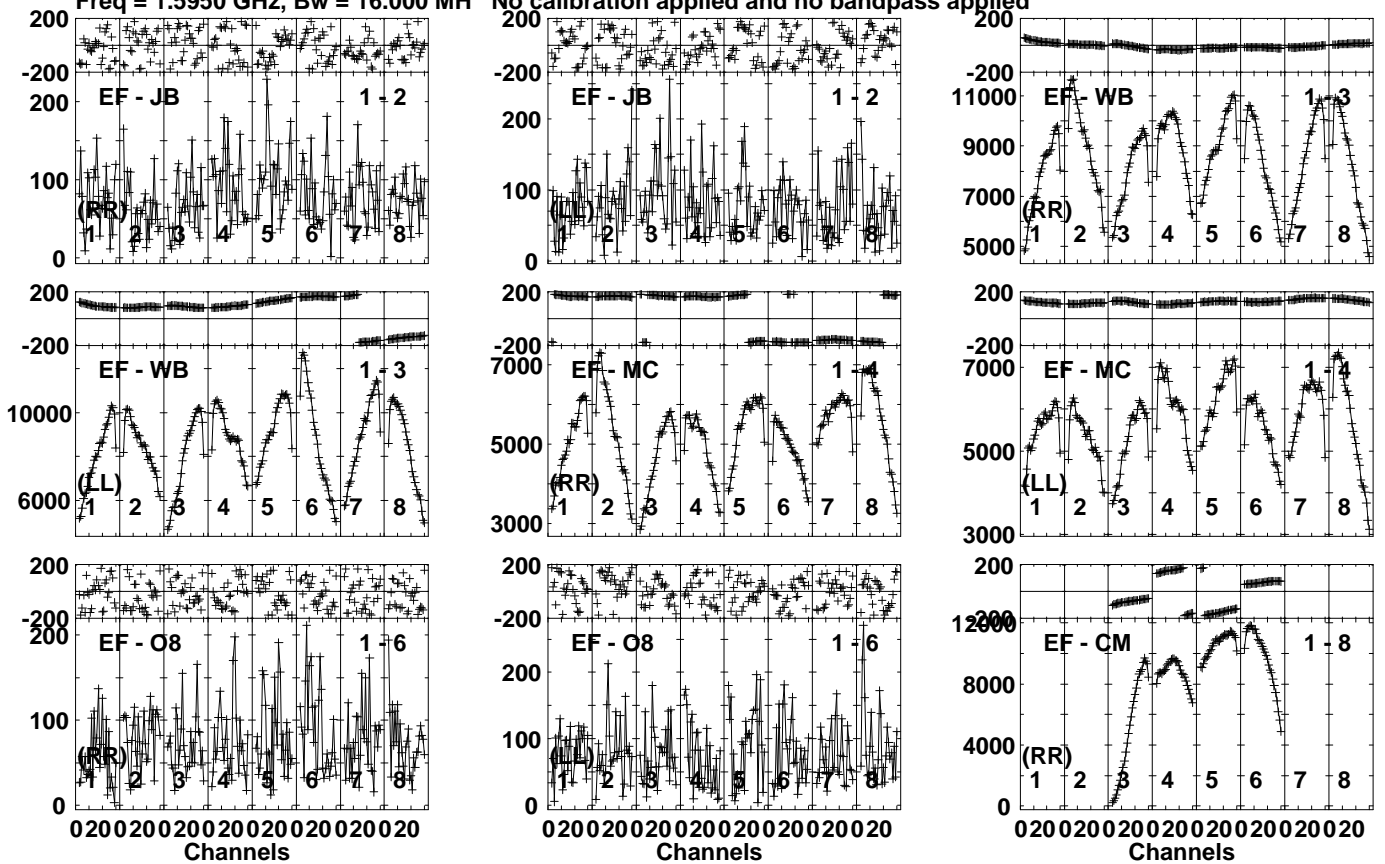
Lower frame: Micro Ampl Jy Top frame: Phas deg Vector averaged cross-power spectrum Several baselines displayed Timerange: 00/19:24:51 to 00/19:28:29
