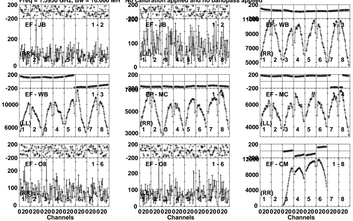
Lower frame: Micro Ampl Jy Top frame: Phas deg Vector averaged cross-power spectrum Several baselines displayed Timerange: 00/19:40:51 to 00/19:44:19
