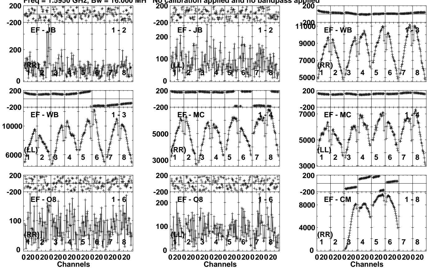
Lower frame: Micro Ampl Jy Top frame: Phas deg Vector averaged cross-power spectrum Several baselines displayed Timerange: 00/19:19:01 to 00/19:22:39
