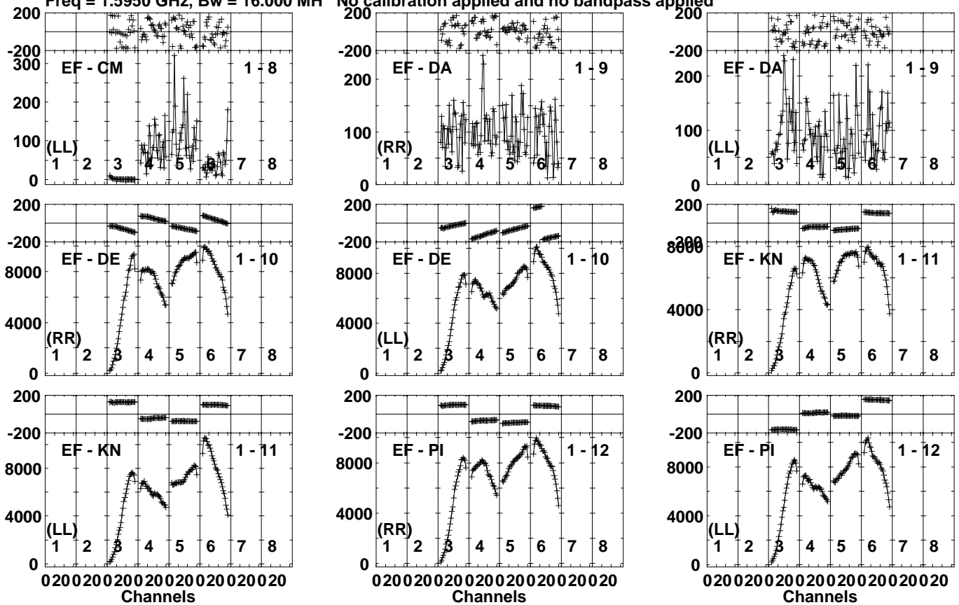
Lower frame: Micro Ampl Jy Top frame: Phas deg Vector averaged cross-power spectrum Several baselines displayed Timerange: 00/13:13:51 to 00/13:17:19
