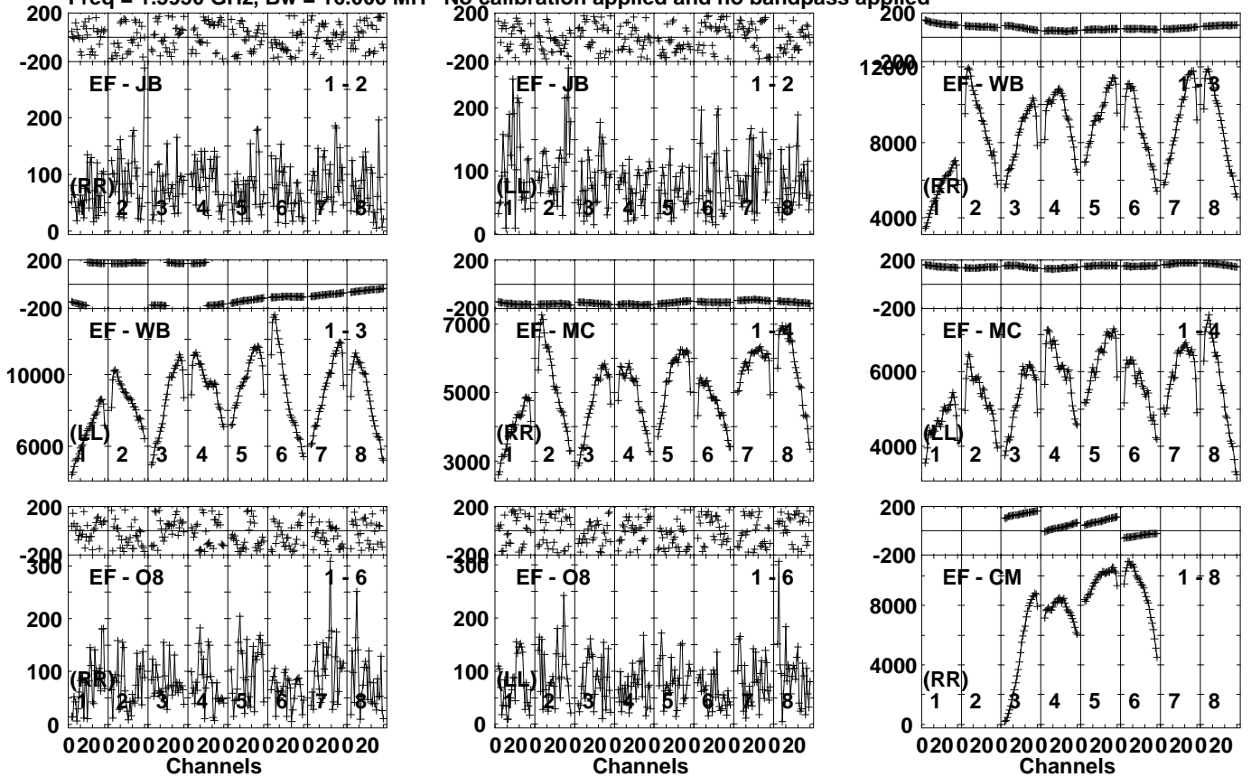
Lower frame: Micro Ampl Jy Top frame: Phas deg Vector averaged cross-power spectrum Several baselines displayed Timerange: 00/18:57:01 to 00/19:00:39
