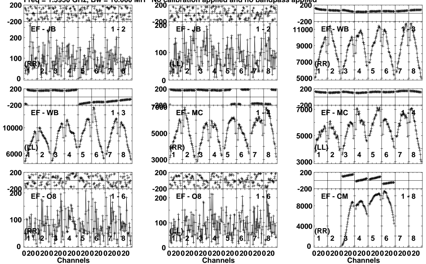
Lower frame: Micro Ampl Jy Top frame: Phas deg Vector averaged cross-power spectrum Several baselines displayed Timerange: 00/19:02:51 to 00/19:06:29
