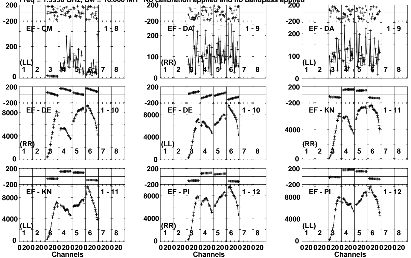
Lower frame: Micro Ampl Jy Top frame: Phas deg Vector averaged cross-power spectrum Several baselines displayed Timerange: 00/14:01:31 to 00/14:04:59
