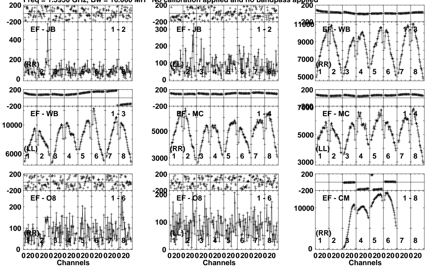
Lower frame: Micro Ampl Jy Top frame: Phas deg Vector averaged cross-power spectrum Several baselines displayed Timerange: 00/21:25:51 to 00/21:29:19
