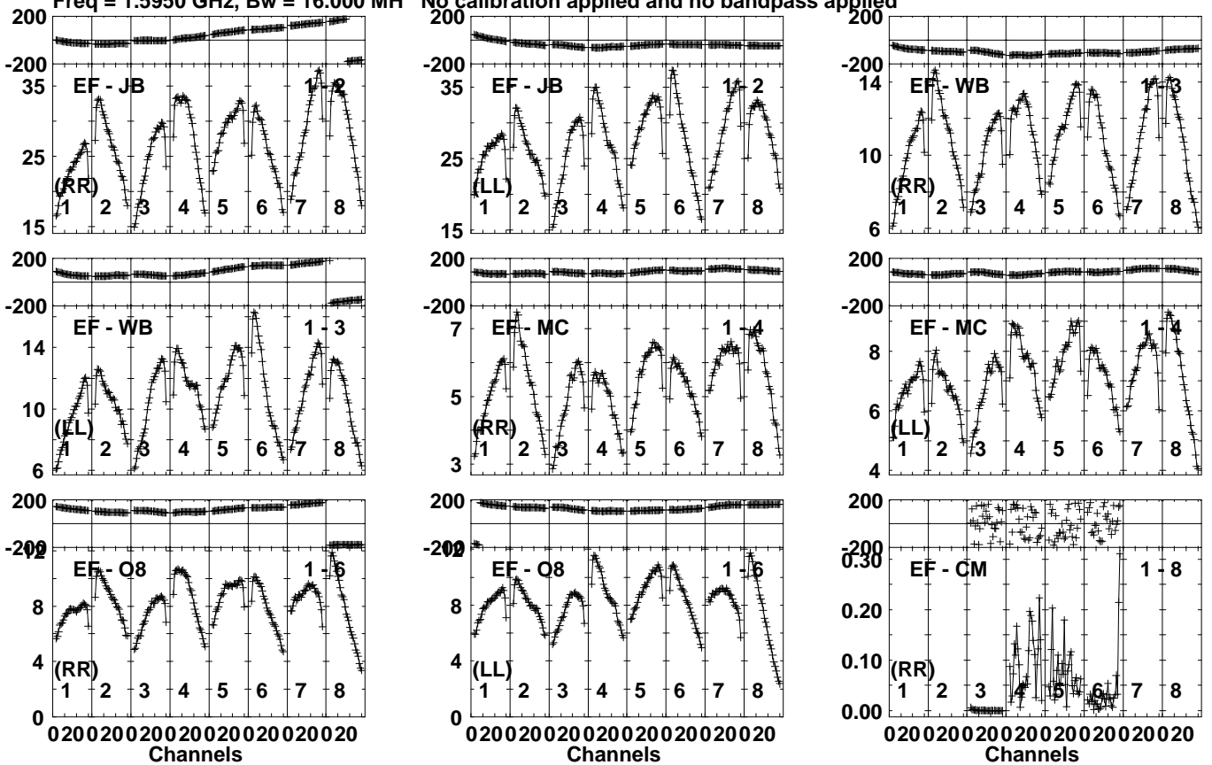
Lower frame: Milli Ampl Jy Top frame: Phas deg Vector averaged cross-power spectrum Several baselines displayed Timerange: 00/13:13:51 to 00/13:17:19
