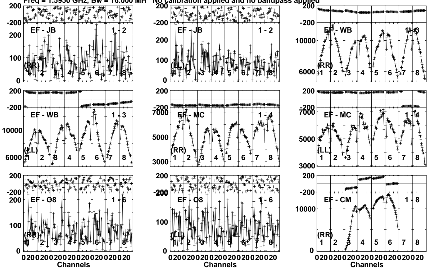
Lower frame: Micro Ampl Jy Top frame: Phas deg Vector averaged cross-power spectrum Several baselines displayed Timerange: 00/19:51:21 to 00/19:54:49
