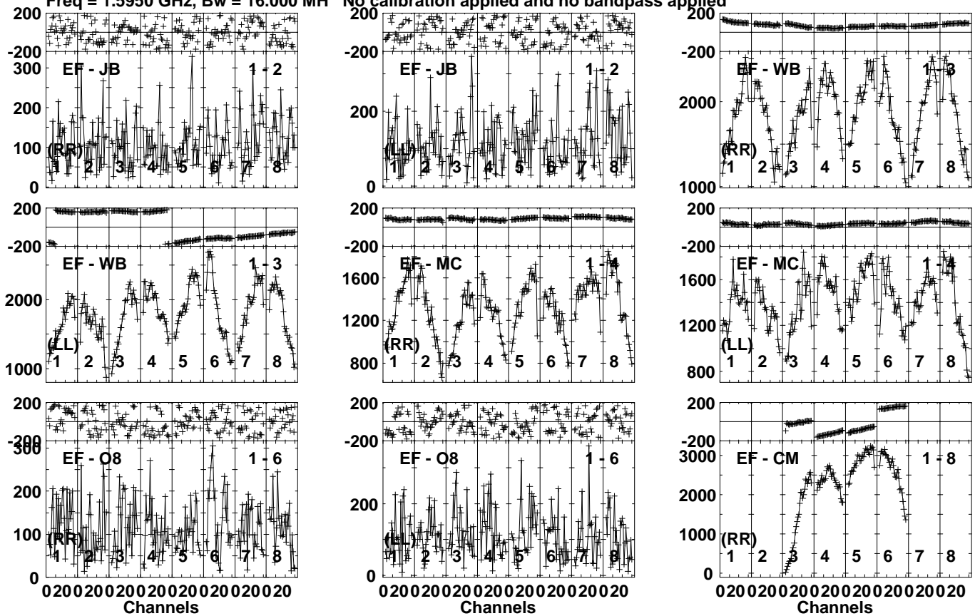
Lower frame: Micro Ampl Jy Top frame: Phas deg Vector averaged cross-power spectrum Several baselines displayed Timerange: 00/19:12:21 to 00/19:13:49
