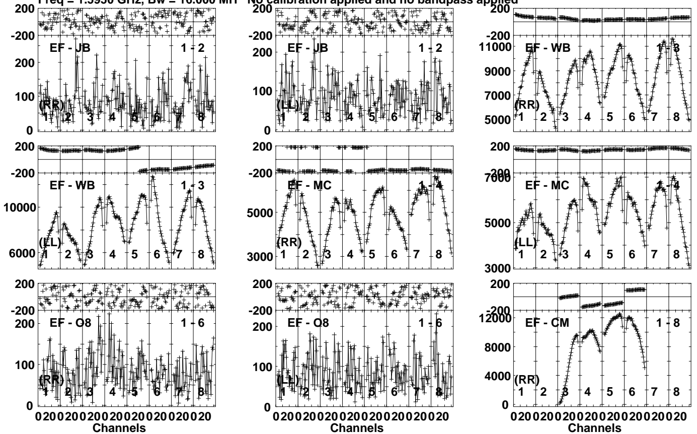
Lower frame: Micro Ampl Jy Top frame: Phas deg Vector averaged cross-power spectrum Several baselines displayed Timerange: 00/19:56:51 to 00/20:00:19
