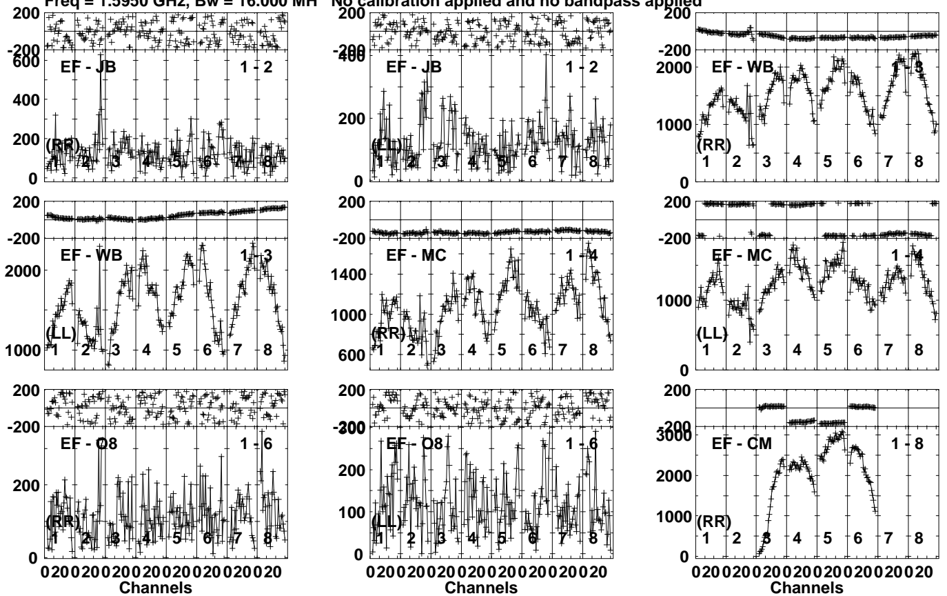
Lower frame: Micro Ampl Jy Top frame: Phas deg Vector averaged cross-power spectrum Several baselines displayed Timerange: 00/22:01:21 to 00/22:02:49
