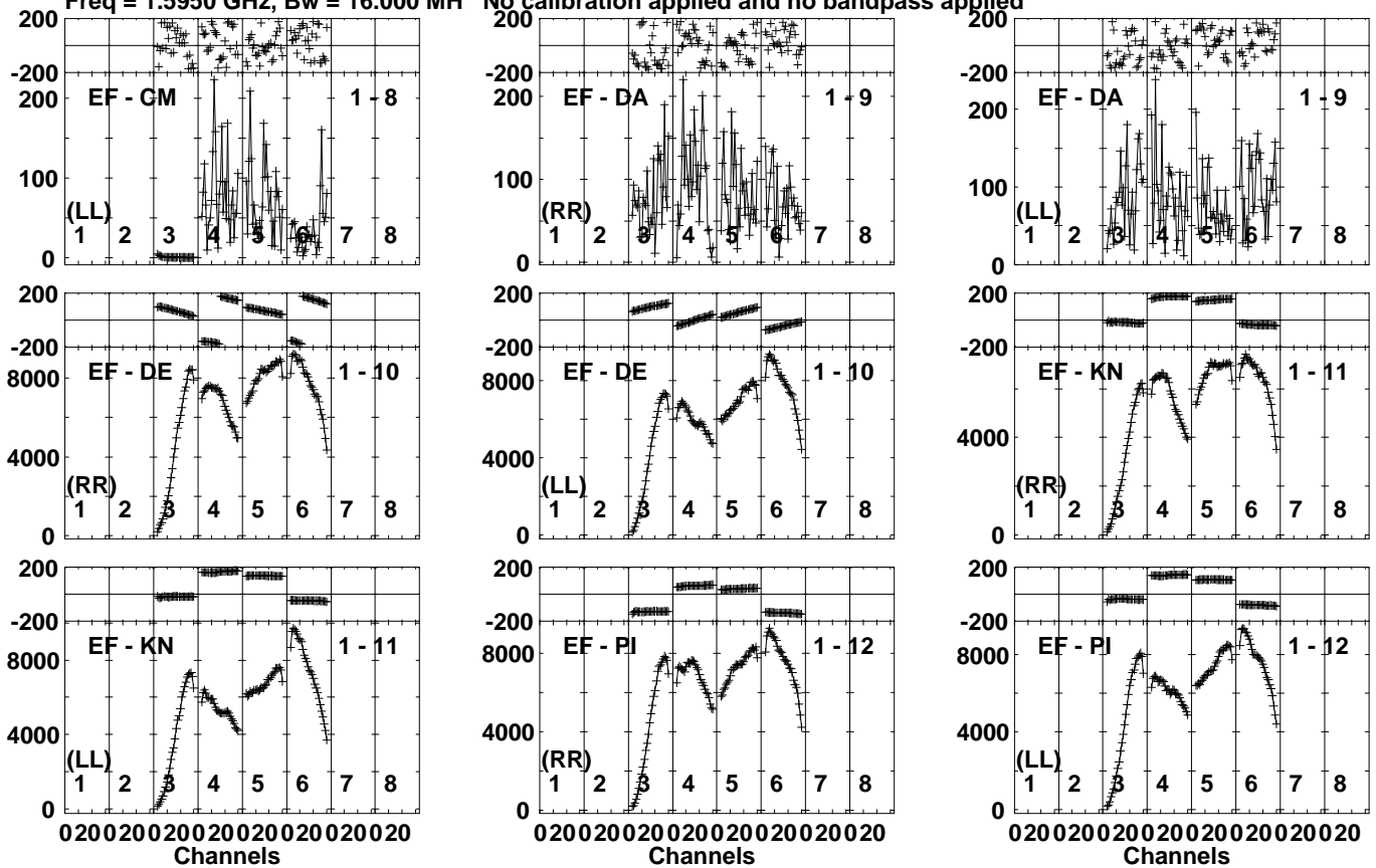
Lower frame: Micro Ampl Jy Top frame: Phas deg Vector averaged cross-power spectrum Several baselines displayed Timerange: 00/14:17:51 to 00/14:21:19
