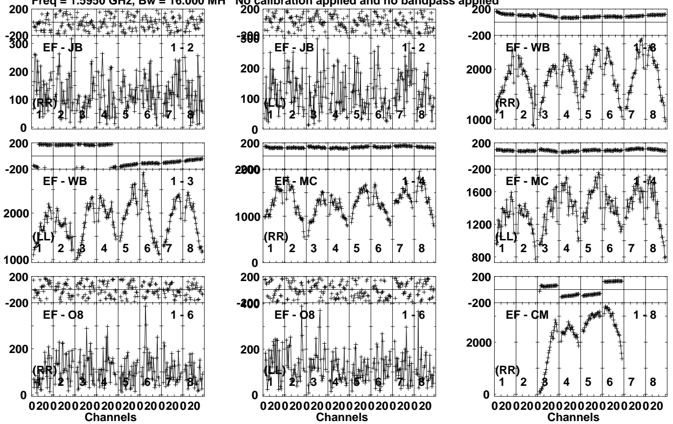
Lower frame: Micro Ampl Jy Top frame: Phas deg Vector averaged cross-power spectrum Several baselines displayed Timerange: 00/20:16:21 to 00/20:17:49
