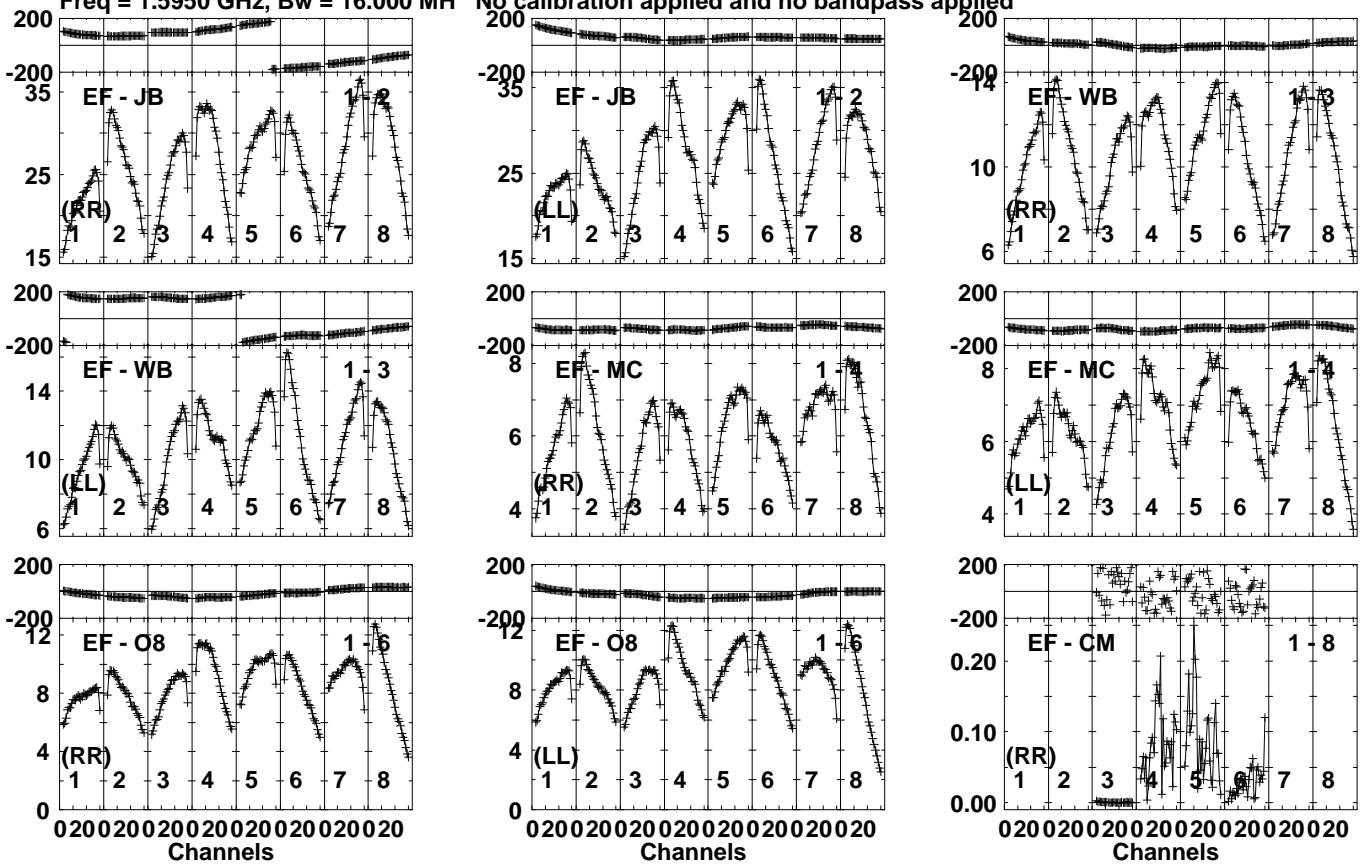
Lower frame: Milli Ampl Jy Top frame: Phas deg Vector averaged cross-power spectrum Several baselines displayed Timerange: 00/13:56:31 to 00/13:59:59
