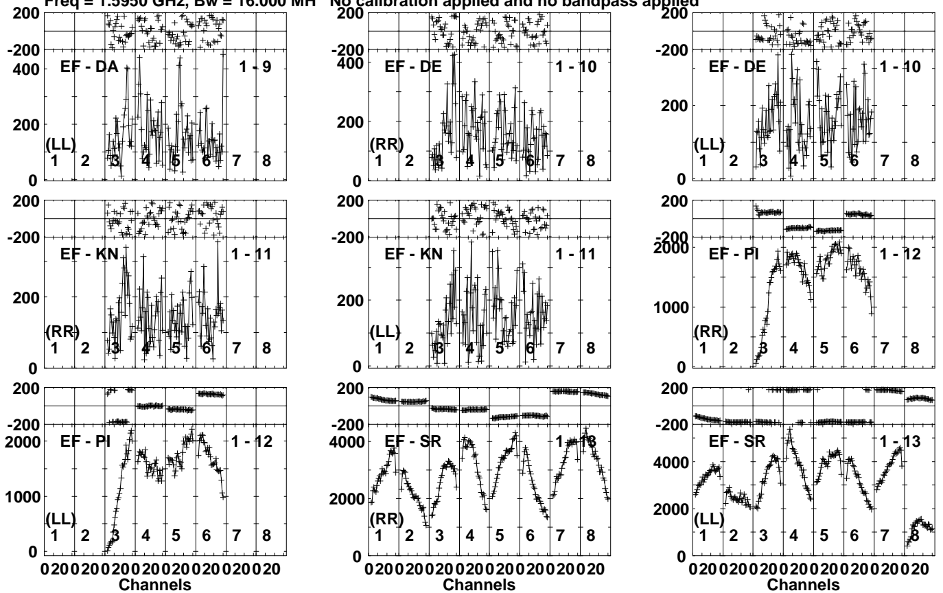
Lower frame: Micro Ampl Jy Top frame: Phas deg Vector averaged cross-power spectrum Several baselines displayed Timerange: 00/19:39:21 to 00/19:40:49
