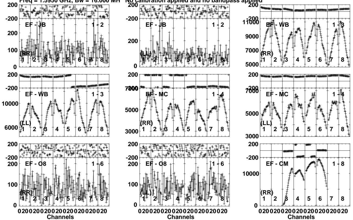
Lower frame: Micro Ampl Jy Top frame: Phas deg Vector averaged cross-power spectrum Several baselines displayed Timerange: 00/21:10:21 to 00/21:13:49
