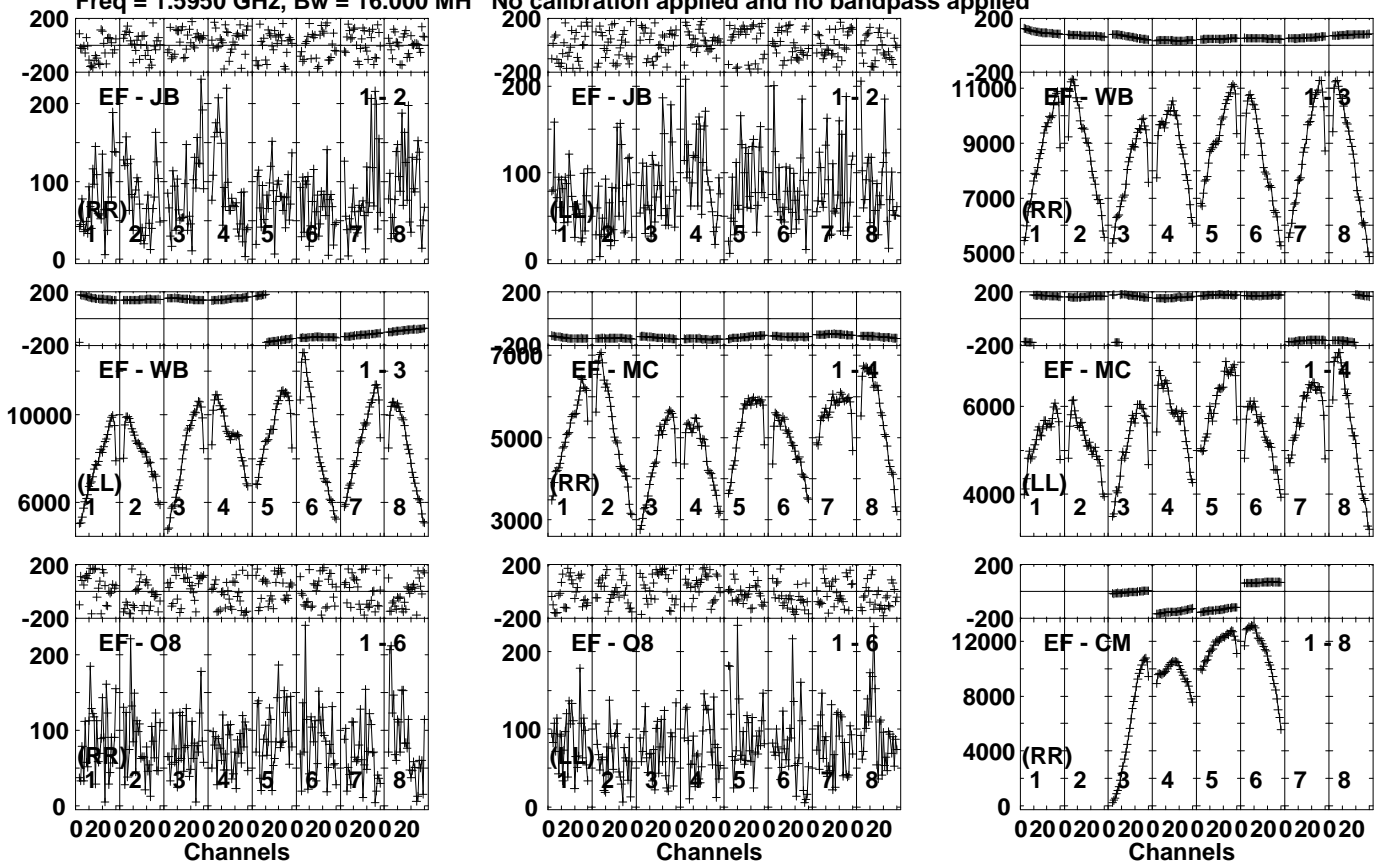
Lower frame: Micro Ampl Jy Top frame: Phas deg Vector averaged cross-power spectrum Several baselines displayed Timerange: 00/20:17:51 to 00/20:21:19
