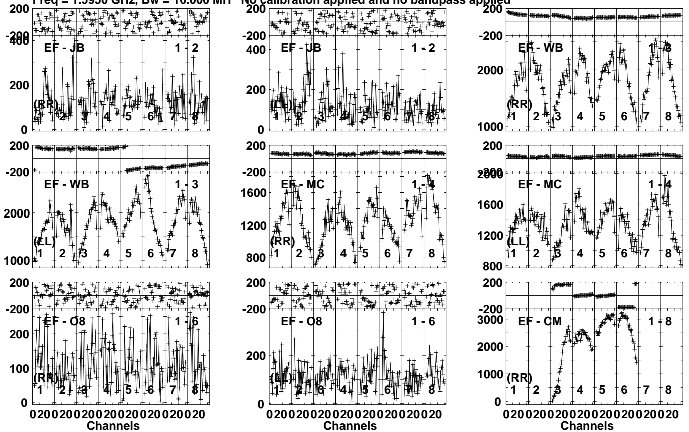
Lower frame: Micro Ampl Jy Top frame: Phas deg Vector averaged cross-power spectrum Several baselines displayed Timerange: 00/21:19:21 to 00/21:20:49
