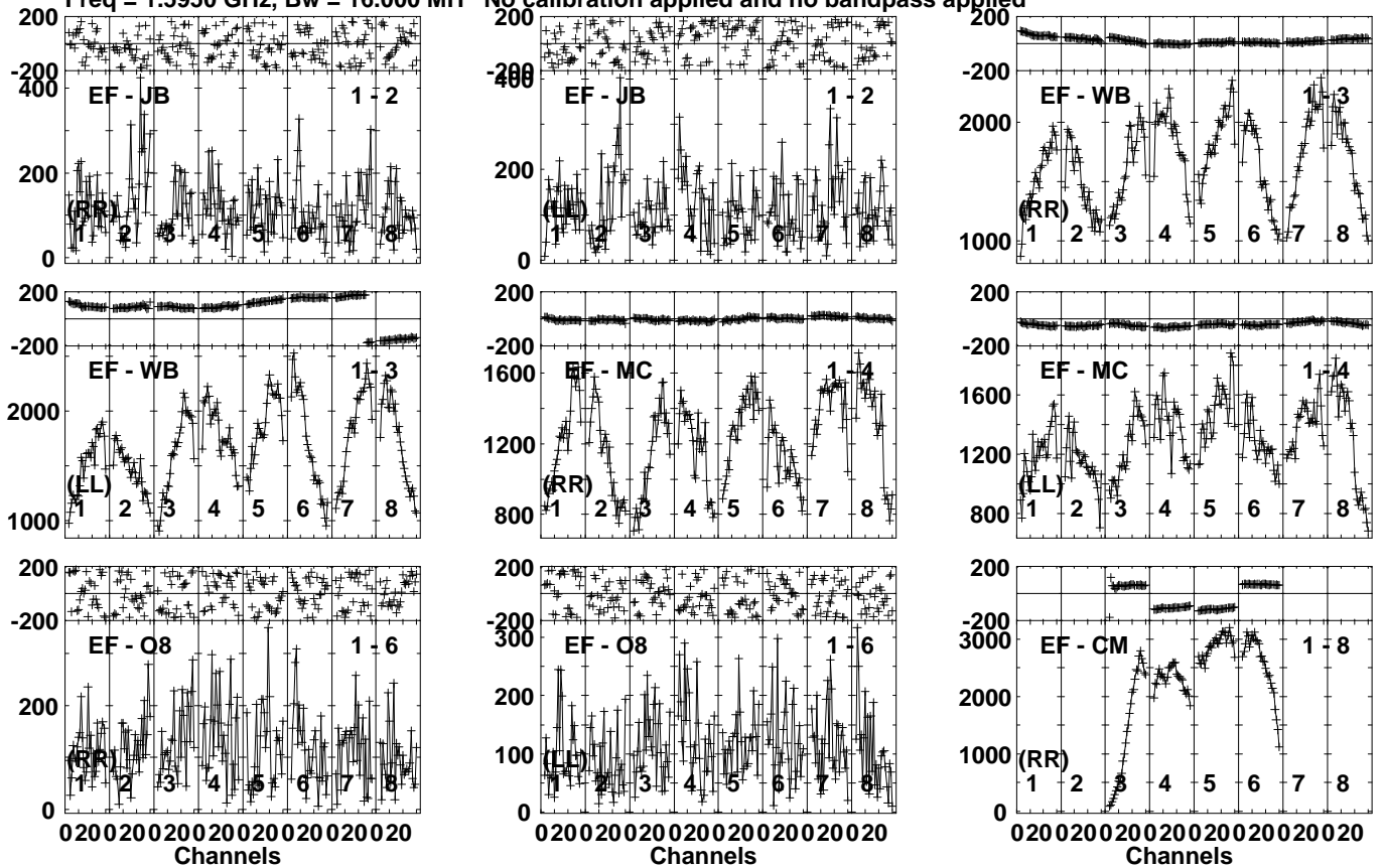
Lower frame: Micro Ampl Jy Top frame: Phas deg Vector averaged cross-power spectrum Several baselines displayed Timerange: 00/21:40:21 to 00/21:41:49
