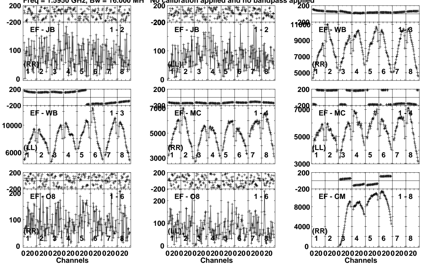
Lower frame: Micro Ampl Jy Top frame: Phas deg Vector averaged cross-power spectrum Several baselines displayed Timerange: 00/20:28:21 to 00/20:31:49
