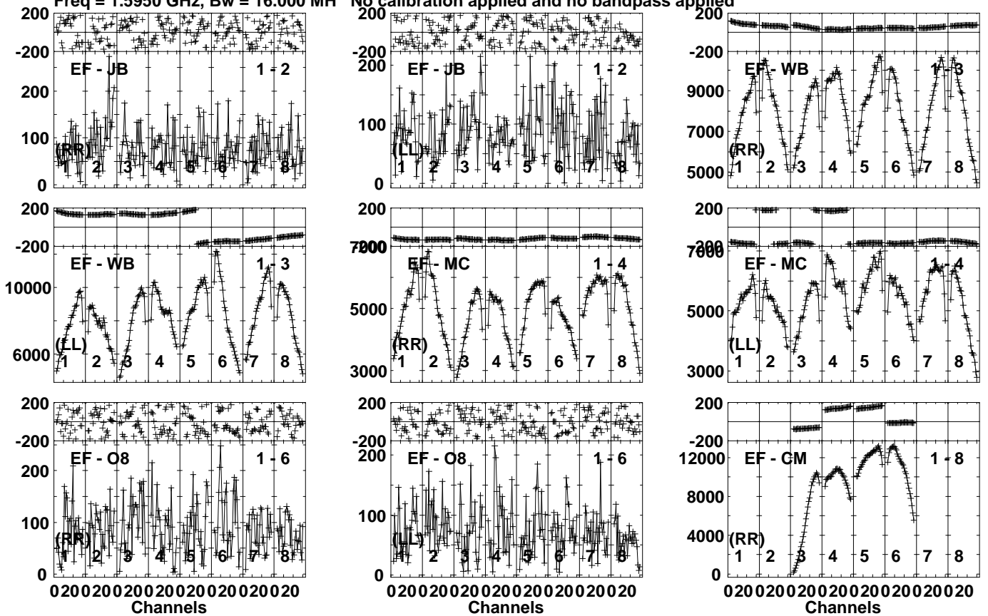
Lower frame: Micro Ampl Jy Top frame: Phas deg Vector averaged cross-power spectrum Several baselines displayed Timerange: 00/20:33:21 to 00/20:36:49
