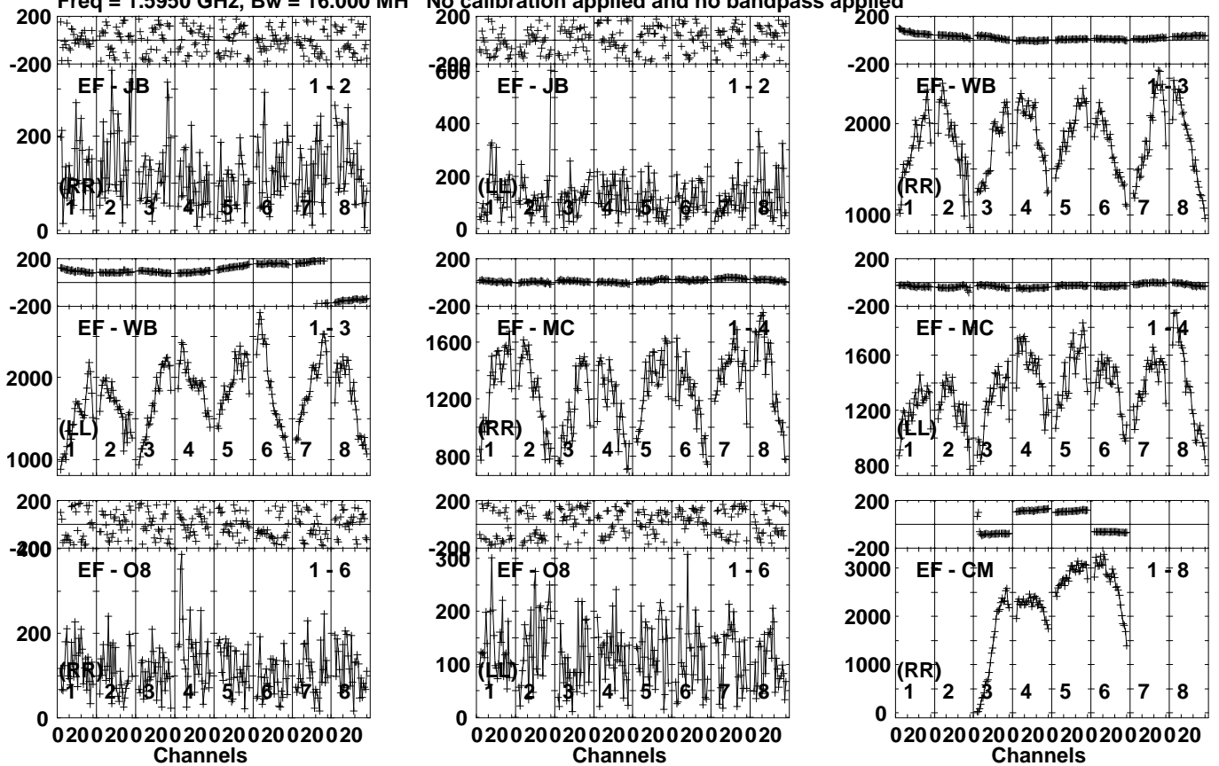
Lower frame: Micro Ampl Jy Top frame: Phas deg Vector averaged cross-power spectrum Several baselines displayed Timerange: 00/21:29:51 to 00/21:31:19
