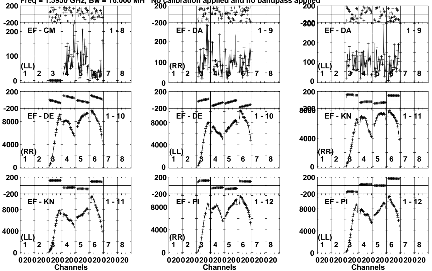
Lower frame: Micro Ampl Jy Top frame: Phas deg Vector averaged cross-power spectrum Several baselines displayed Timerange: 00/13:18:51 to 00/13:22:19
