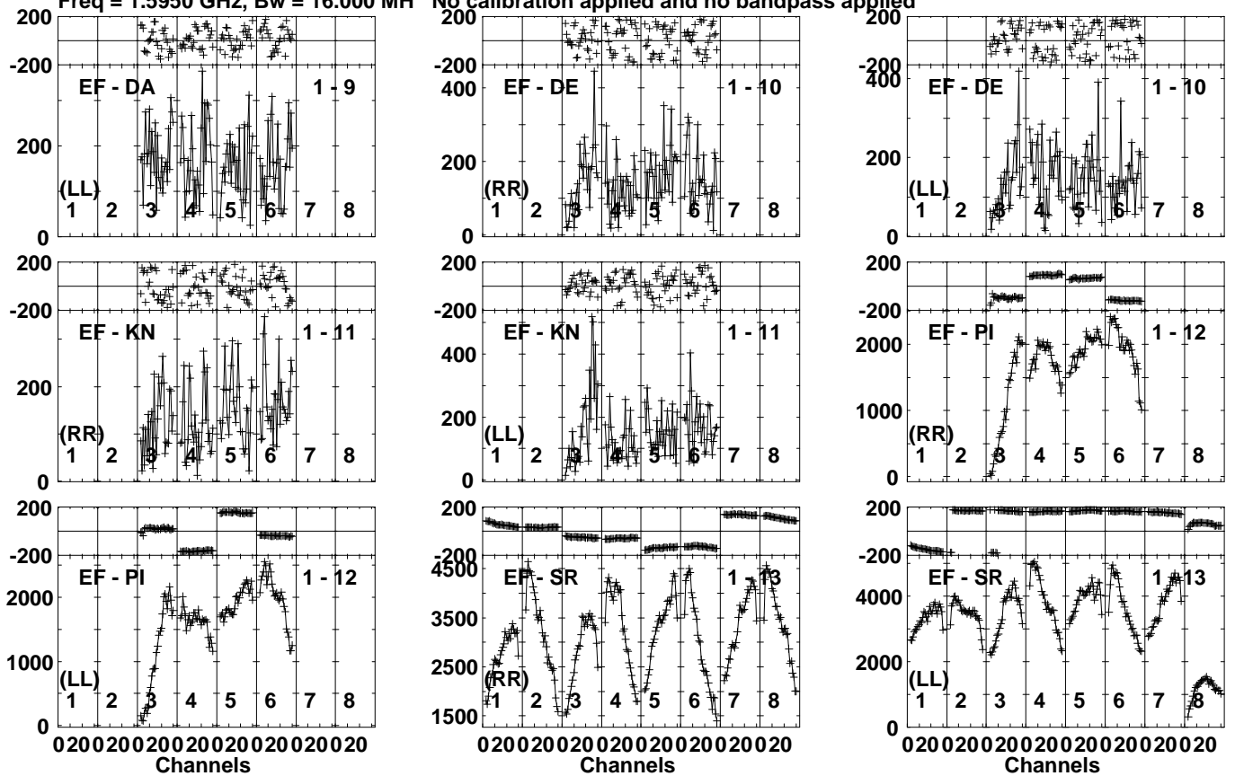
Lower frame: Micro Ampl Jy Top frame: Phas deg Vector averaged cross-power spectrum Several baselines displayed Timerange: 00/20:10:51 to 00/20:12:19
