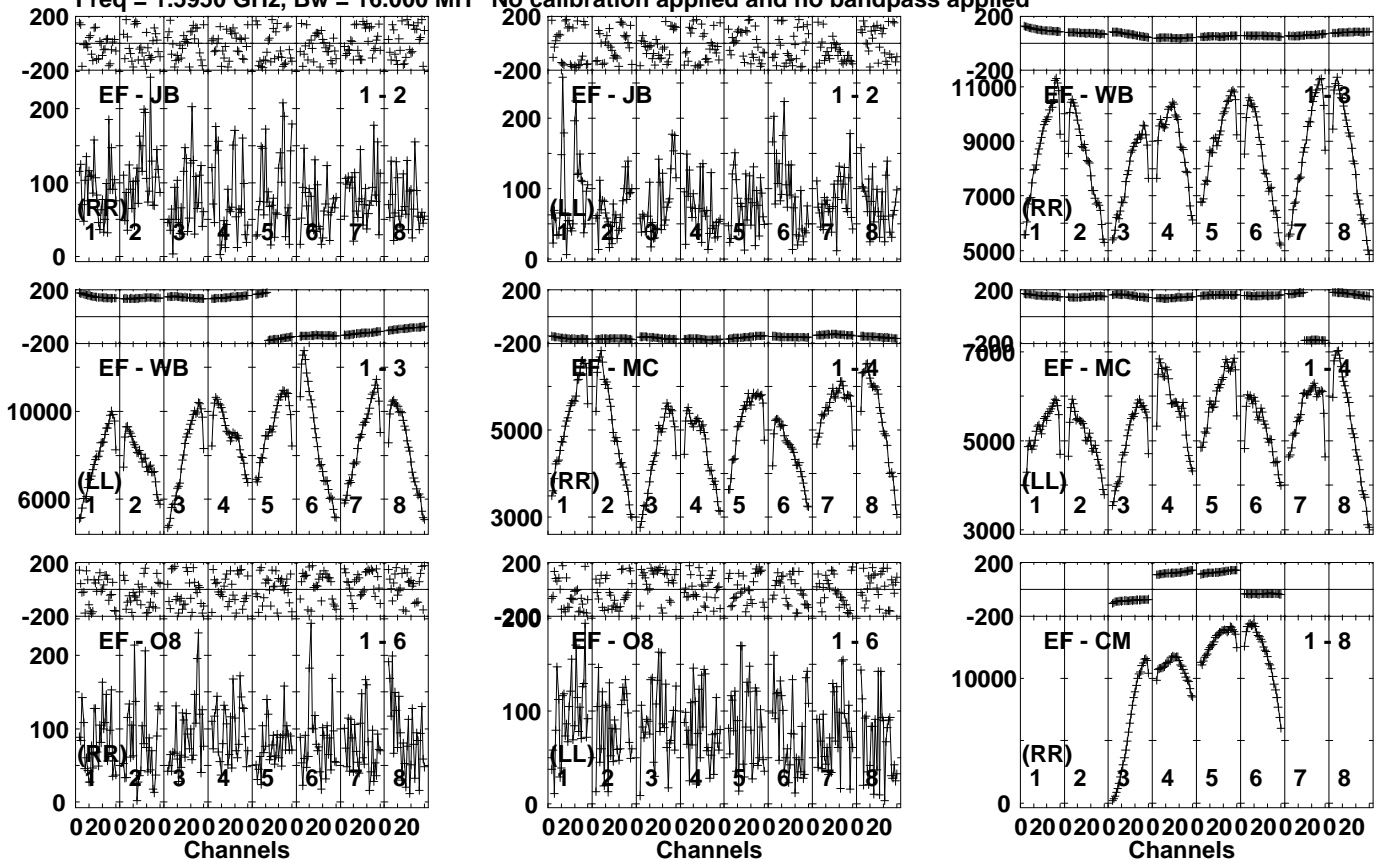
Lower frame: Micro Ampl Jy Top frame: Phas deg Vector averaged cross-power spectrum Several baselines displayed Timerange: 00/20:43:51 to 00/20:47:19
