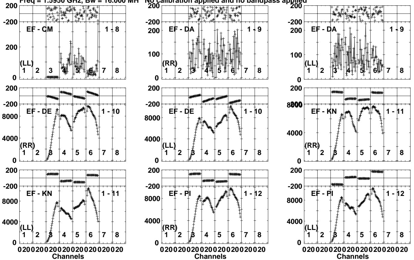
Lower frame: Micro Ampl Jy Top frame: Phas deg Vector averaged cross-power spectrum Several baselines displayed Timerange: 00/13:08:11 to 00/13:11:39
