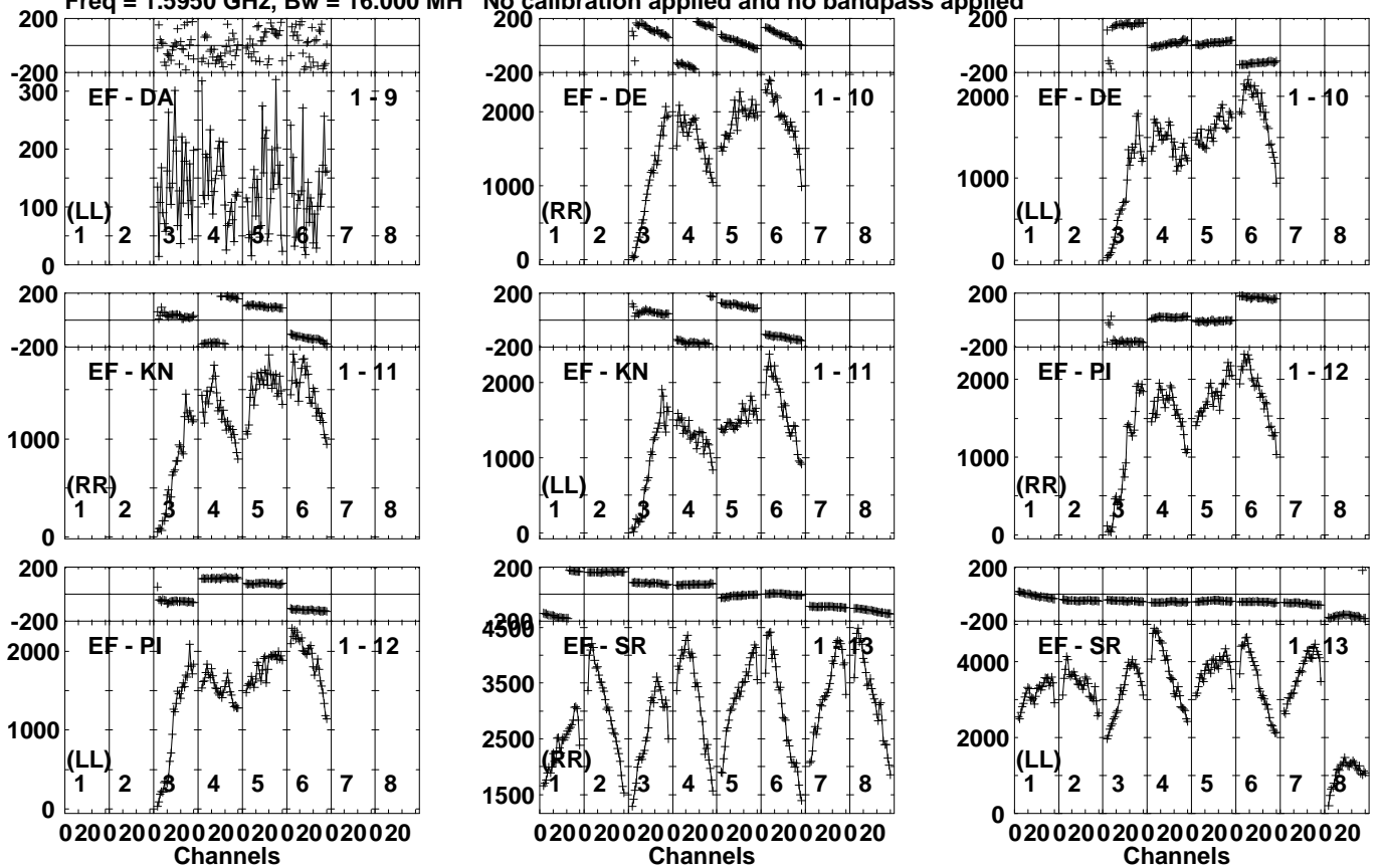
Lower frame: Micro Ampl Jy Top frame: Phas deg Vector averaged cross-power spectrum Several baselines displayed Timerange: 00/21:34:51 to 00/21:36:19
