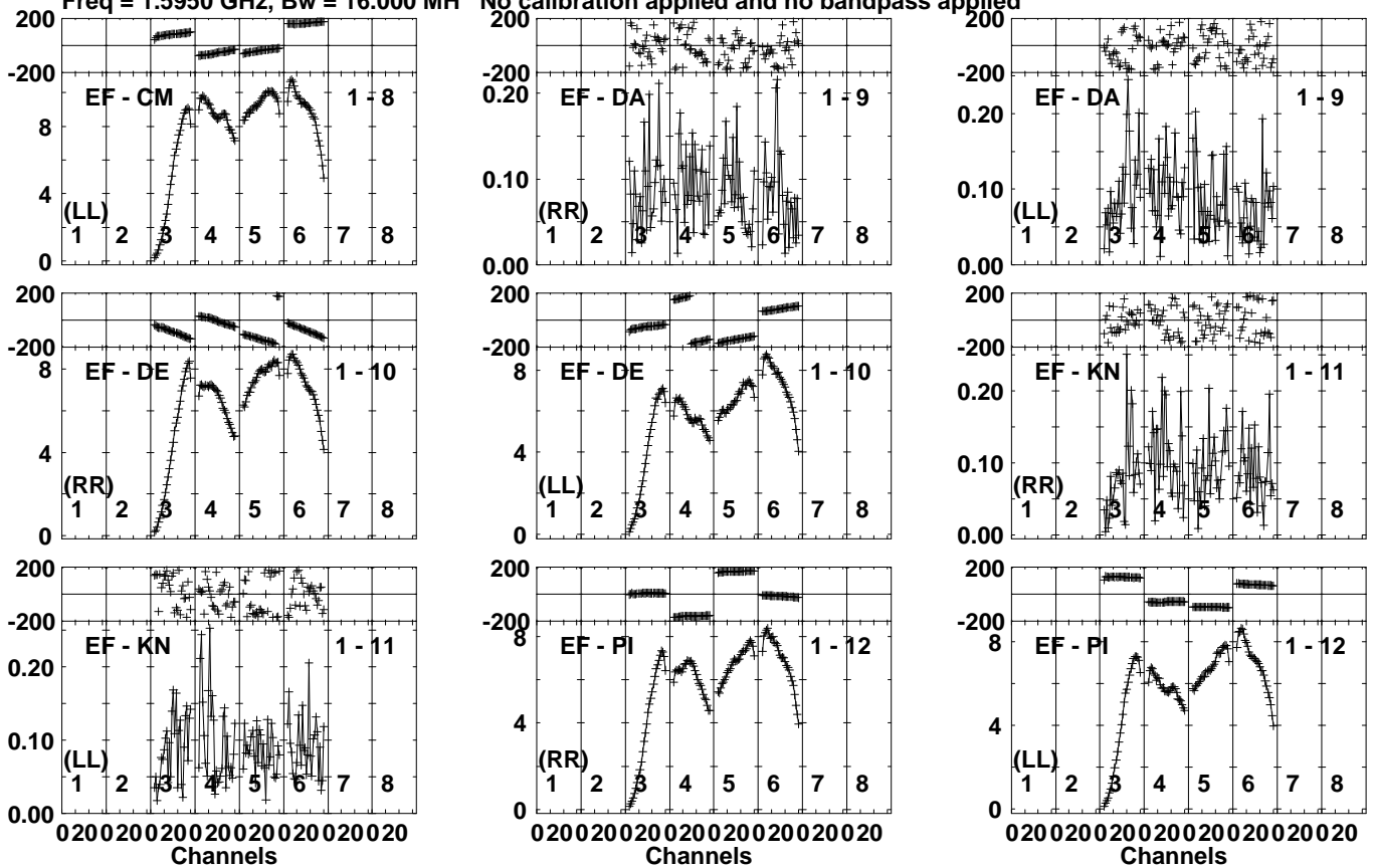
Lower frame: Milli Ampl Jy Top frame: Phas deg Vector averaged cross-power spectrum Several baselines displayed Timerange: 00/19:24:51 to 00/19:28:29
