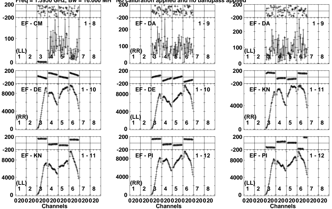
Lower frame: Micro Ampl Jy Top frame: Phas deg Vector averaged cross-power spectrum Several baselines displayed Timerange: 00/13:29:31 to 00/13:32:59
