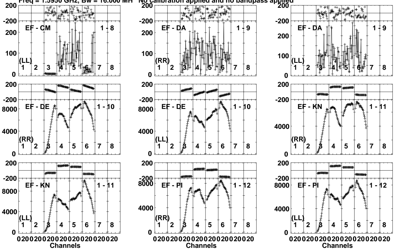
Lower frame: Micro Ampl Jy Top frame: Phas deg Vector averaged cross-power spectrum Several baselines displayed Timerange: 00/14:22:51 to 00/14:26:19
