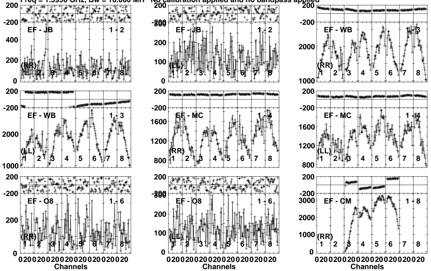
Lower frame: Micro Ampl Jy Top frame: Phas deg Vector averaged cross-power spectrum Several baselines displayed Timerange: 00/20:05:51 to 00/20:07:19
