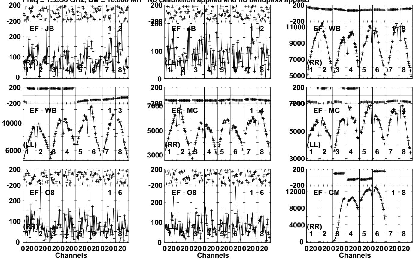
Lower frame: Micro Ampl Jy Top frame: Phas deg Vector averaged cross-power spectrum Several baselines displayed Timerange: 00/20:38:51 to 00/20:42:19
