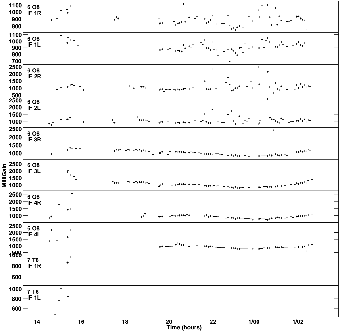
Plot file version 5 created 29-SEP-2021 15:11:11 Gain amp vs UTC time for J1415+1320.MULTI.1 SN 2 Rpol & Lpol IF 1 - 4
