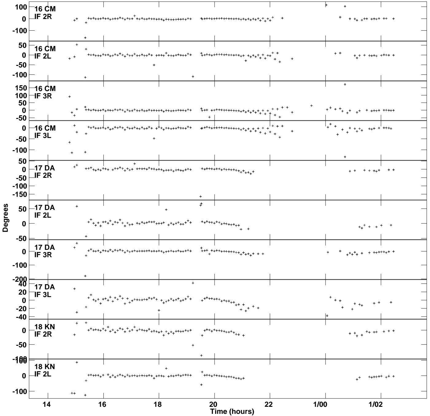
Plot file version 13 created 29-SEP-2021 15:10:55 Gain phs vs UTC time for J1415+1320.MULTI.1 SN 1 Rpol & Lpol IF 1 - 4
