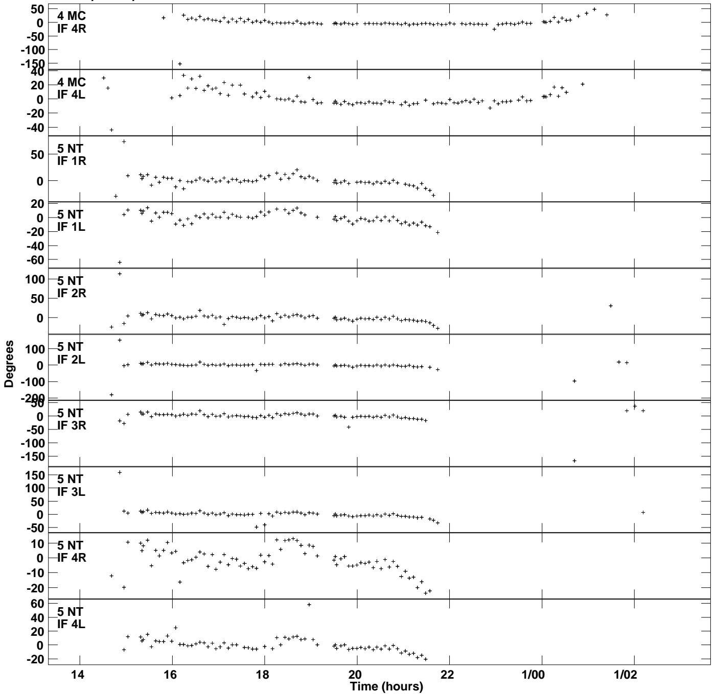
Plot file version 4 created 29-SEP-2021 15:10:54 Gain phs vs UTC time for J1415+1320.MULTI.1 SN 1 Rpol & Lpol IF 1 - 4
