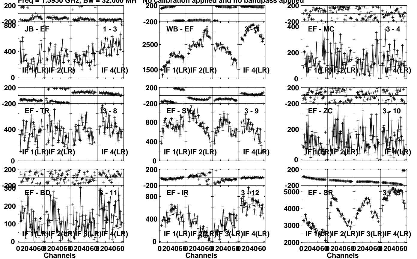
Lower frame: Micro Ampl Jy Top frame: Phas deg Vector averaged cross-power spectrum Several baselines displayed Timerange: 01/03:26:11 to 01/03:27:33
