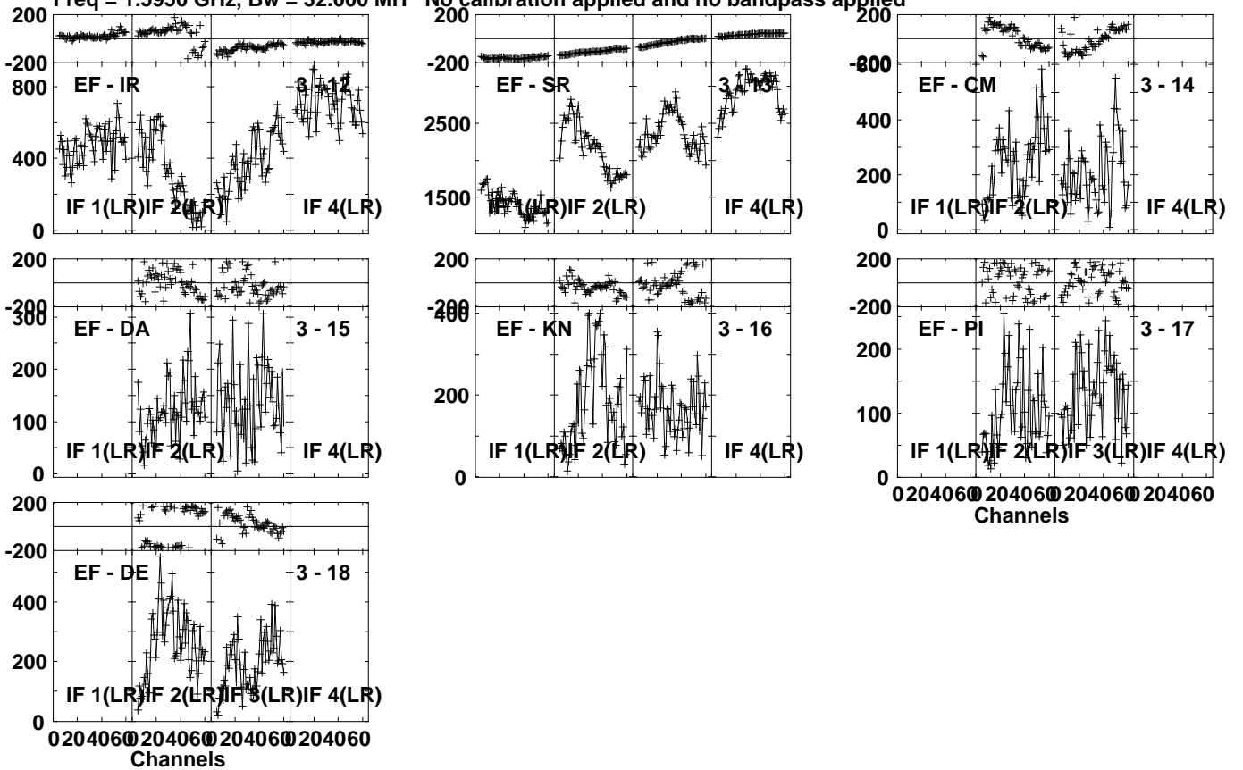
Lower frame: Micro Ampl Jy Top frame: Phas deg Vector averaged cross-power spectrum Several baselines displayed Timerange: 00/21:30:11 to 00/21:31:33
