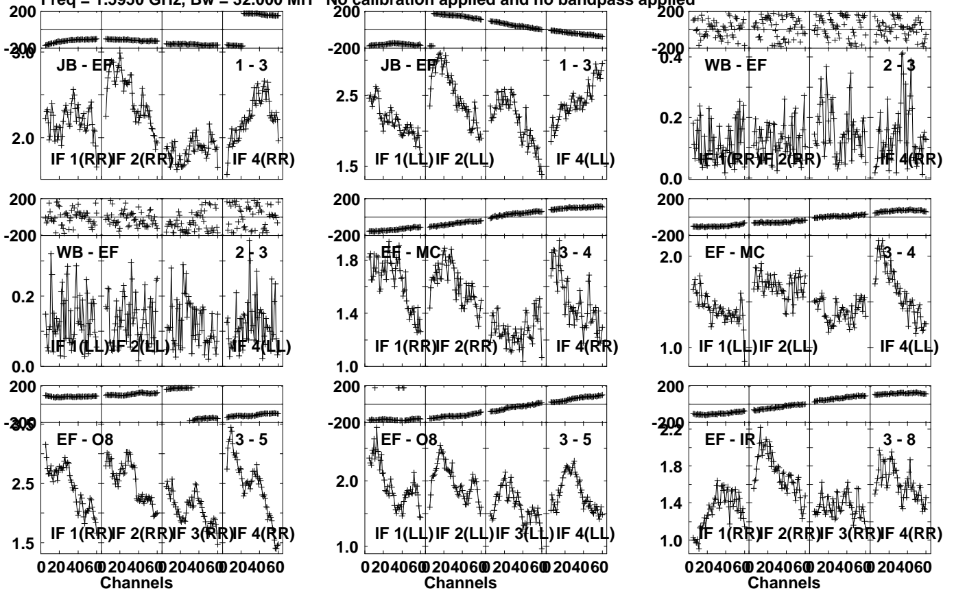
Lower frame: Milli Ampl Jy Top frame: Phas deg Vector averaged cross-power spectrum Several baselines displayed Timerange: 00/10:45:31 to 00/10:46:59
