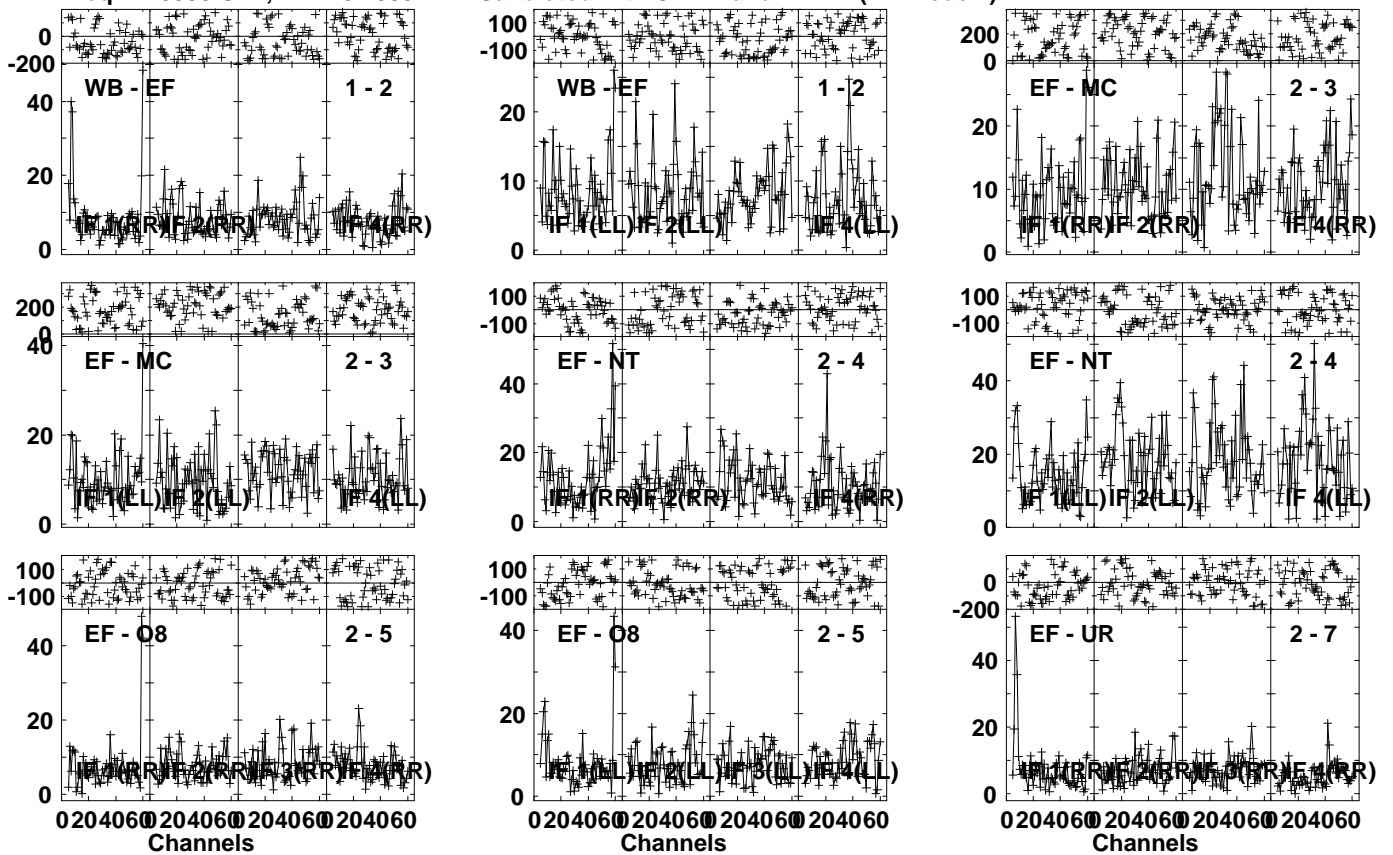
Lower frame: Milli Ampl Jy Top frame: Phas deg Vector averaged cross-power spectrum Several baselines displayed Timerange: 00/02:40:21 to 00/02:44:49
