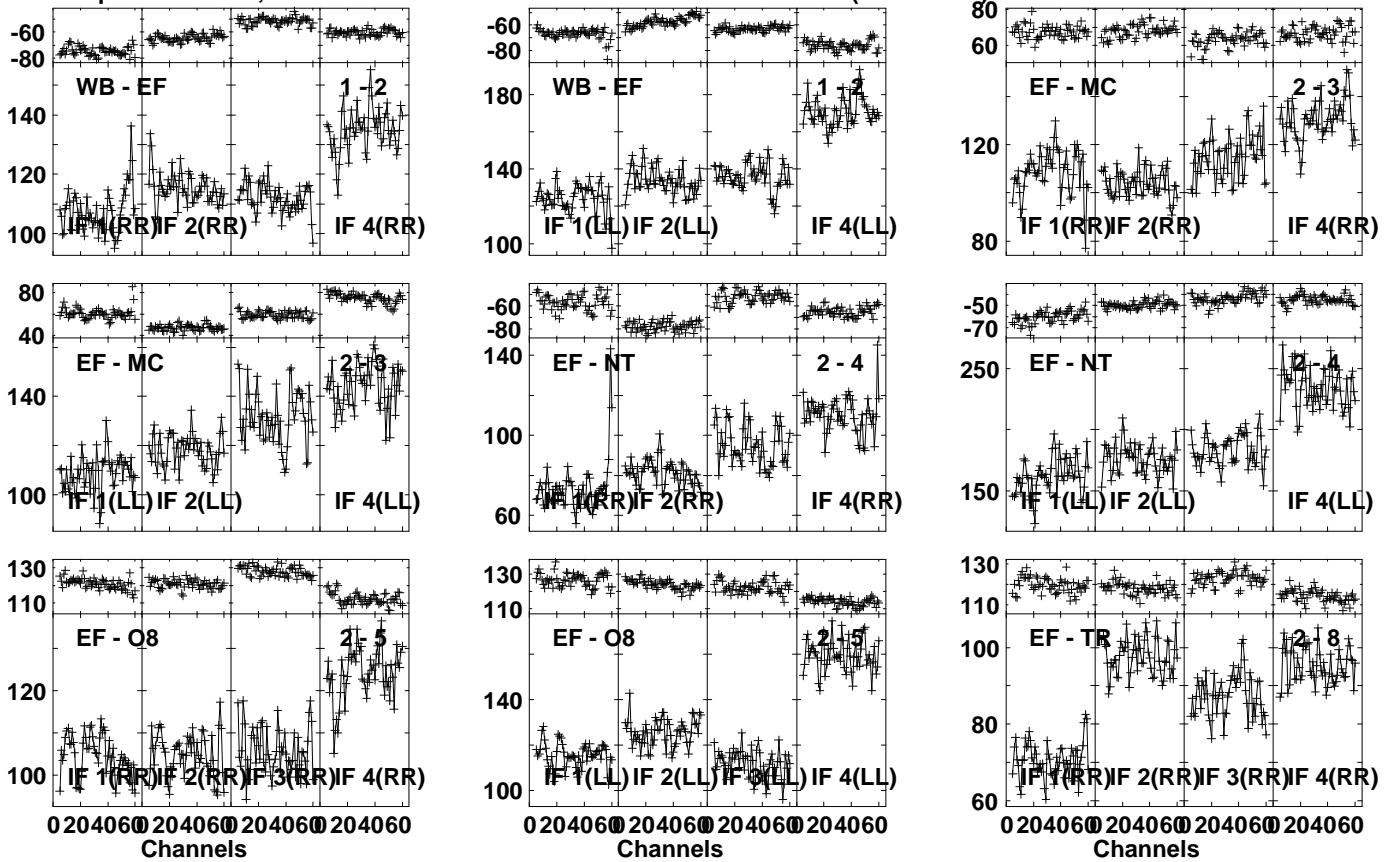
Lower frame: Milli Ampl Jy Top frame: Phas deg Vector averaged cross-power spectrum Several baselines displayed Timerange: 00/07:41:21 to 00/07:45:49
