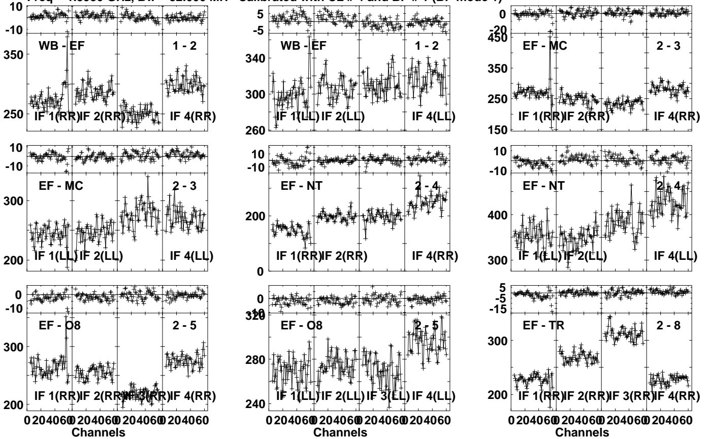
Lower frame: Milli Ampl Jy Top frame: Phas deg Vector averaged cross-power spectrum Several baselines displayed Timerange: 00/05:55:51 to 00/05:57:39
