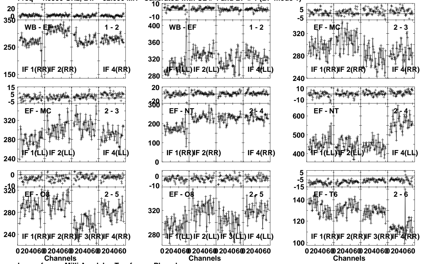
Lower frame: Milli Ampl Jy Top frame: Phas deg Vector averaged cross-power spectrum Several baselines displayed Timerange: 00/02:20:21 to 00/02:21:29
