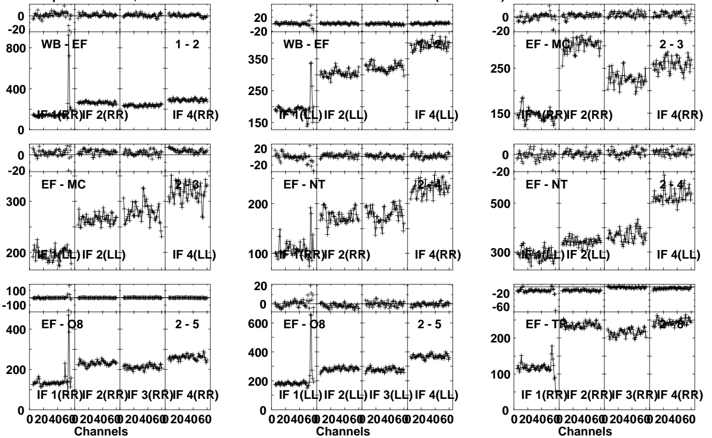
Lower frame: Milli Ampl Jy Top frame: Phas deg Vector averaged cross-power spectrum Several baselines displayed Timerange: 00/07:02:11 to 00/07:03:59
