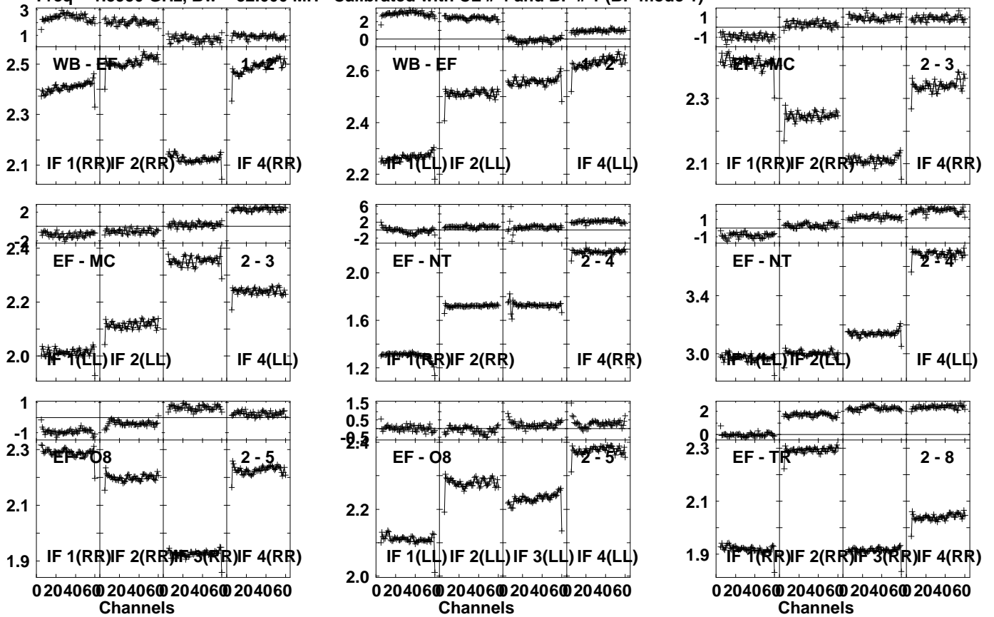
Lower frame: Ampl Jy Top frame: Phas deg Vector averaged cross-power spectrum Several baselines displayed Timerange: 00/06:12:31 to 00/06:16:29
