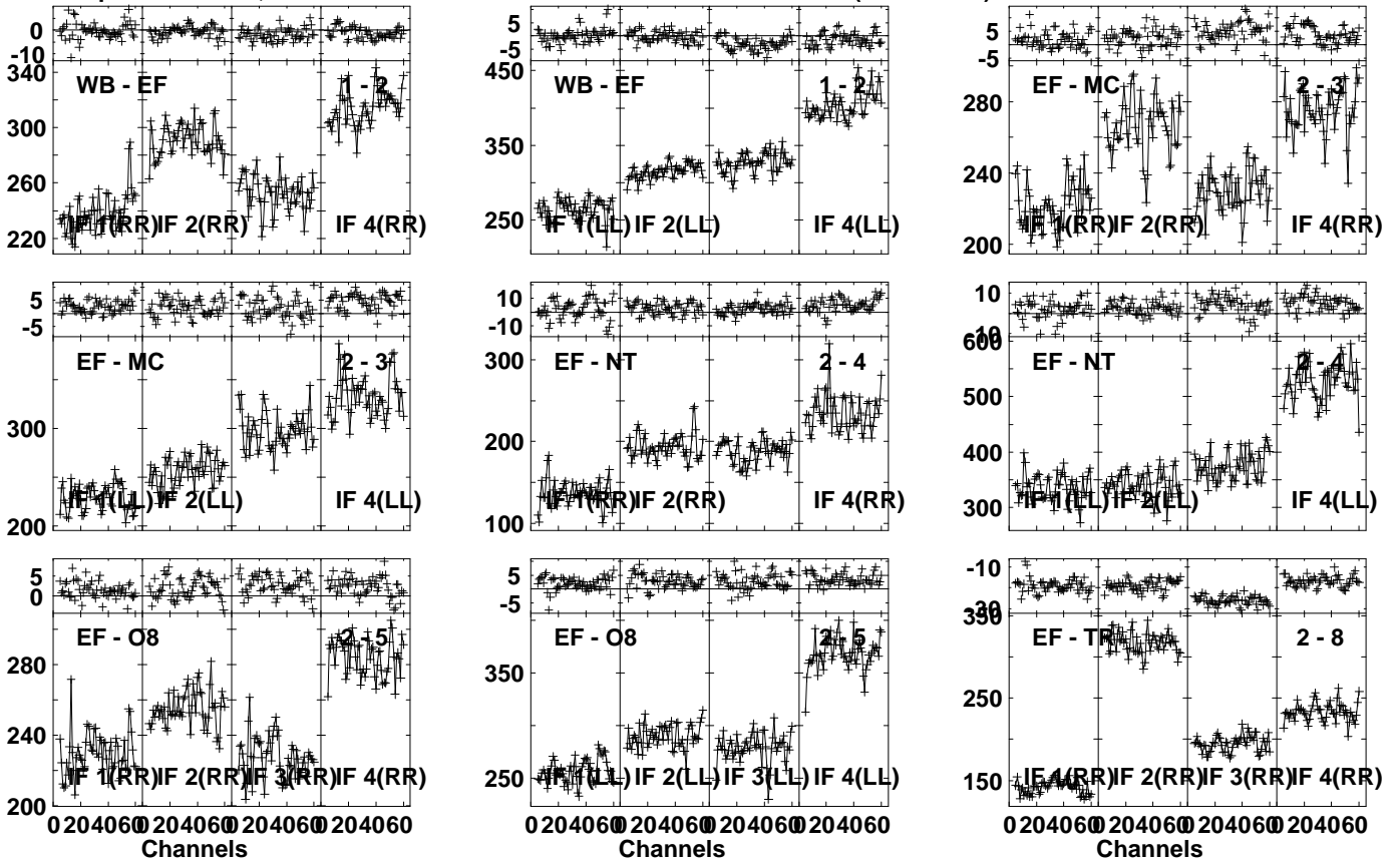
Lower frame: Milli Ampl Jy Top frame: Phas deg Vector averaged cross-power spectrum Several baselines displayed Timerange: 00/06:56:31 to 00/06:57:39
