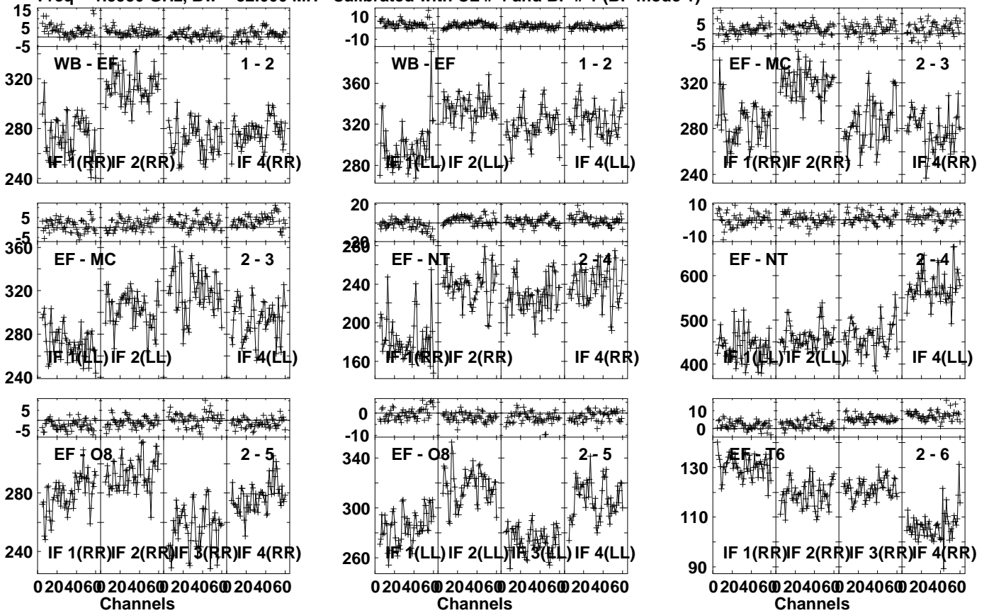
Lower frame: Milli Ampl Jy Top frame: Phas deg Vector averaged cross-power spectrum Several baselines displayed Timerange: 00/02:26:01 to 00/02:27:49
