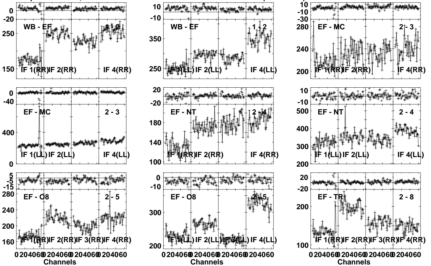
Lower frame: Milli Ampl Jy Top frame: Phas deg Vector averaged cross-power spectrum Several baselines displayed Timerange: 00/07:58:51 to 00/07:59:59
