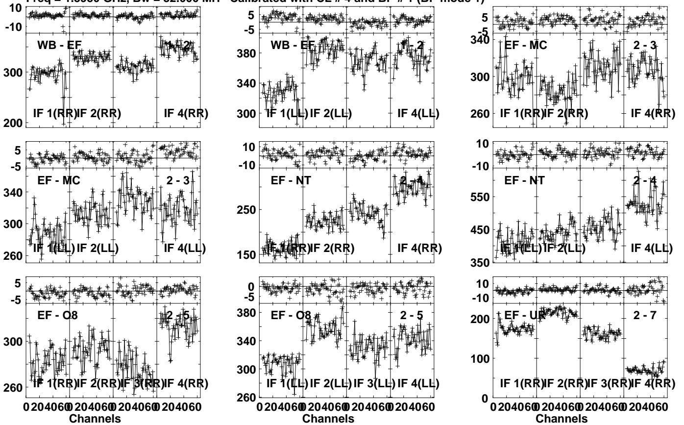
Lower frame: Milli Ampl Jy Top frame: Phas deg Vector averaged cross-power spectrum Several baselines displayed Timerange: 00/03:03:31 to 00/03:05:19
