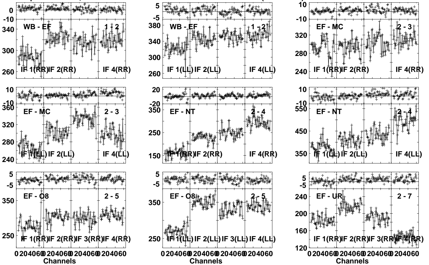
Lower frame: Milli Ampl Jy Top frame: Phas deg Vector averaged cross-power spectrum Several baselines displayed Timerange: 00/03:35:21 to 00/03:36:29
