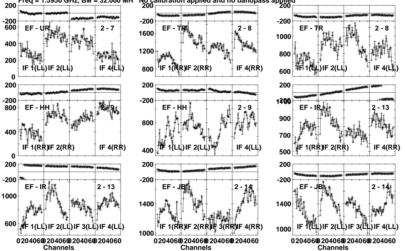
Lower frame: Micro Ampl Jy Top frame: Phas deg Vector averaged cross-power spectrum Several baselines displayed Timerange: 00/02:34:01 to 00/02:38:29
