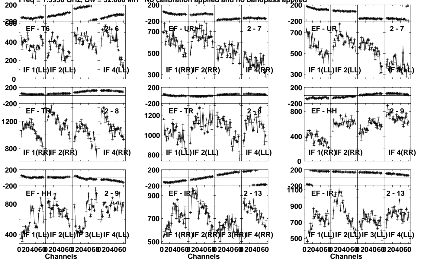
Lower frame: Micro Ampl Jy Top frame: Phas deg Vector averaged cross-power spectrum Several baselines displayed Timerange: 00/01:56:31 to 00/02:00:59
