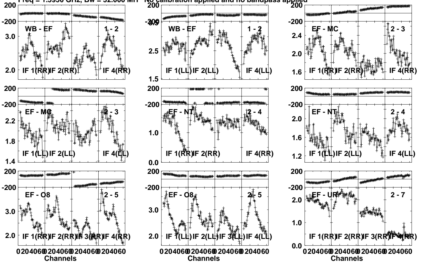
Lower frame: Milli Ampl Jy Top frame: Phas deg Vector averaged cross-power spectrum Several baselines displayed Timerange: 00/03:10:21 to 00/03:11:29
