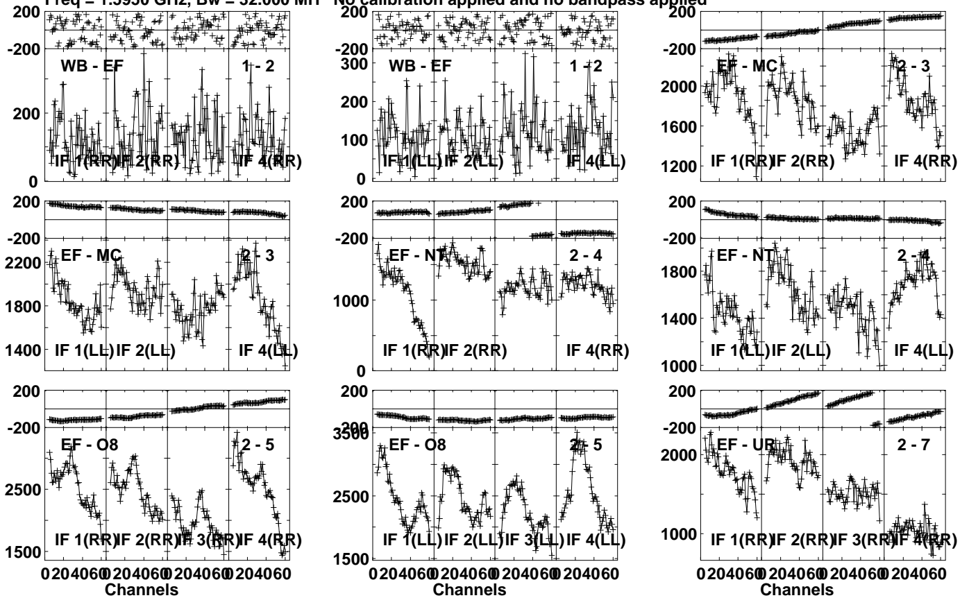
Lower frame: Micro Ampl Jy Top frame: Phas deg Vector averaged cross-power spectrum Several baselines displayed Timerange: 00/03:53:31 to 00/03:55:19
